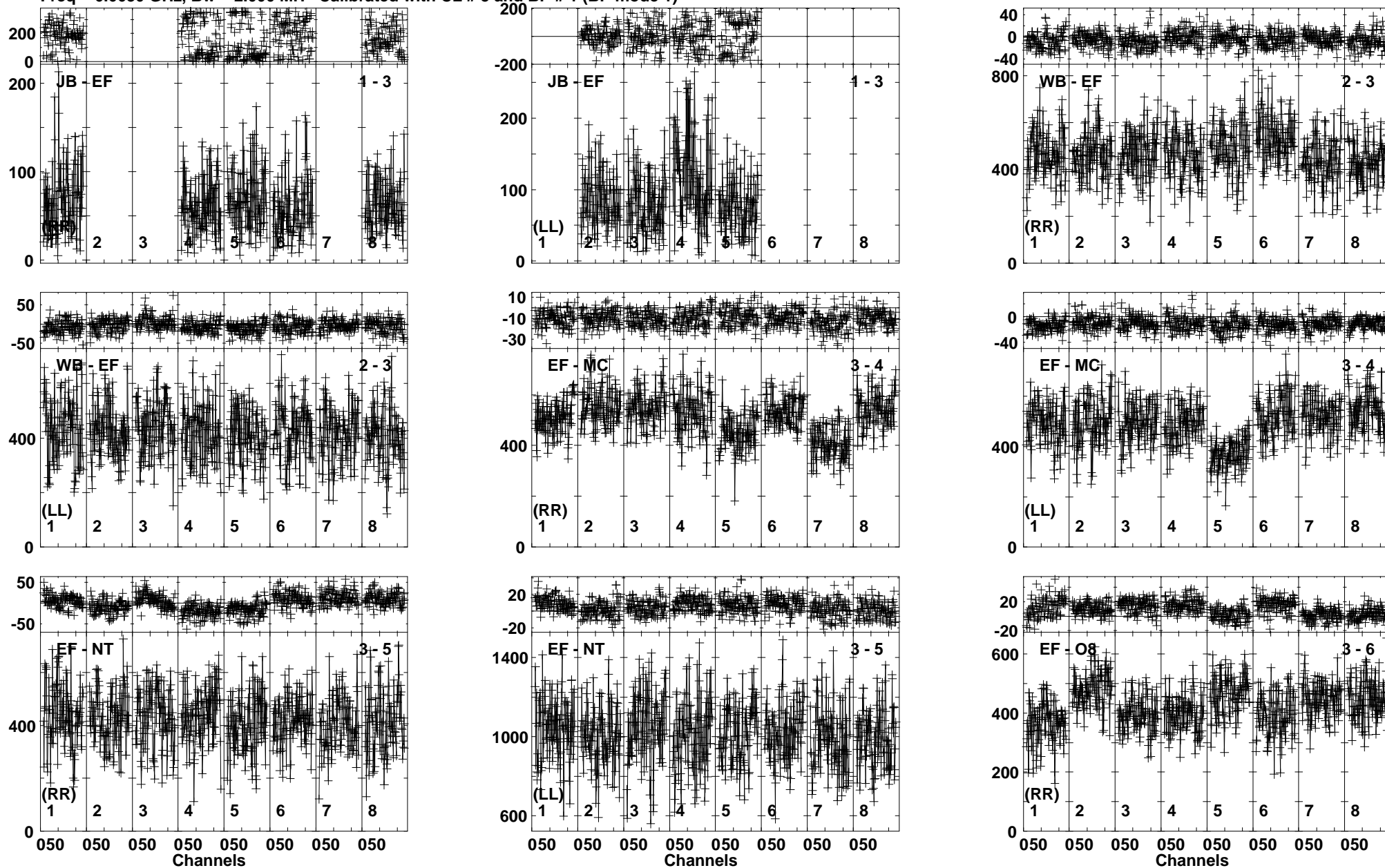
Lower frame: Milli Ampl Jy Top frame: Phas deg Vector averaged cross-power spectrum Baseline: JB (01) - EF (03) Timerange: 01/04:52:49 to 01/04:54:47
