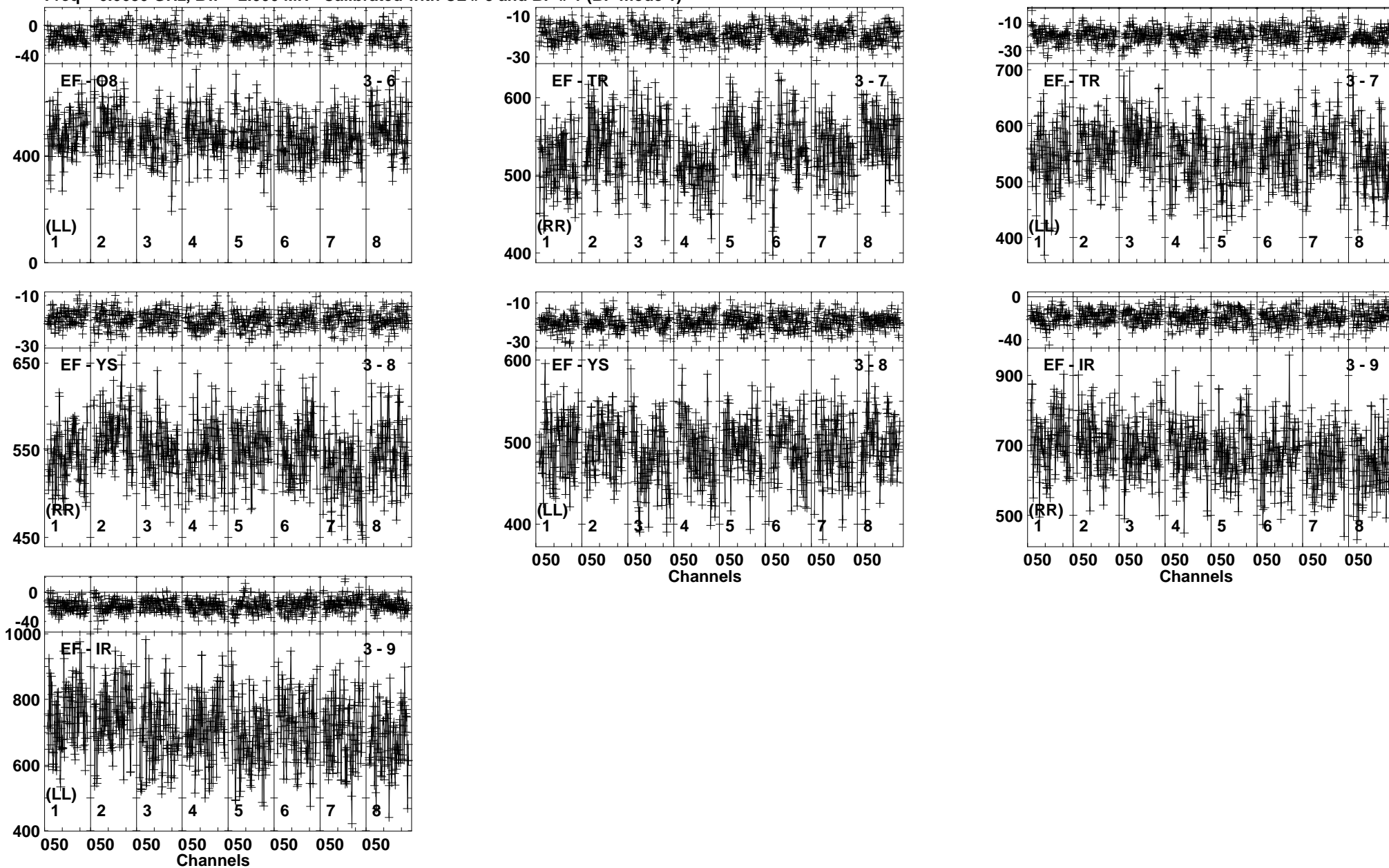
Lower frame: Milli Ampl Jy Top frame: Phas deg Vector averaged cross-power spectrum Baseline: EF (03) - O8 (06) Timerange: 00/23:23:41 to 00/23:25:39
