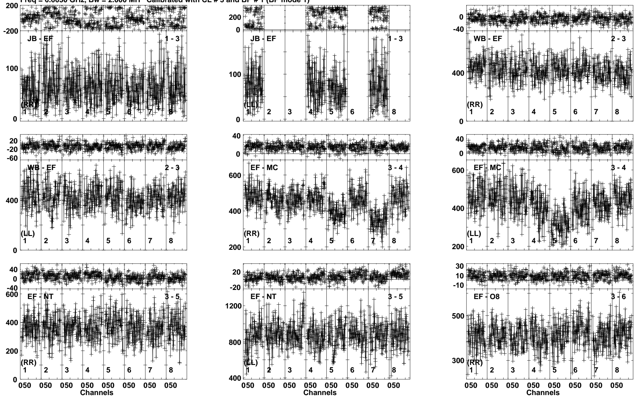
Lower frame: Milli Ampl Jy Top frame: Phas deg Vector averaged cross-power spectrum Baseline: JB (01) - EF (03) Timerange: 01/05:11:29 to 01/05:13:27
