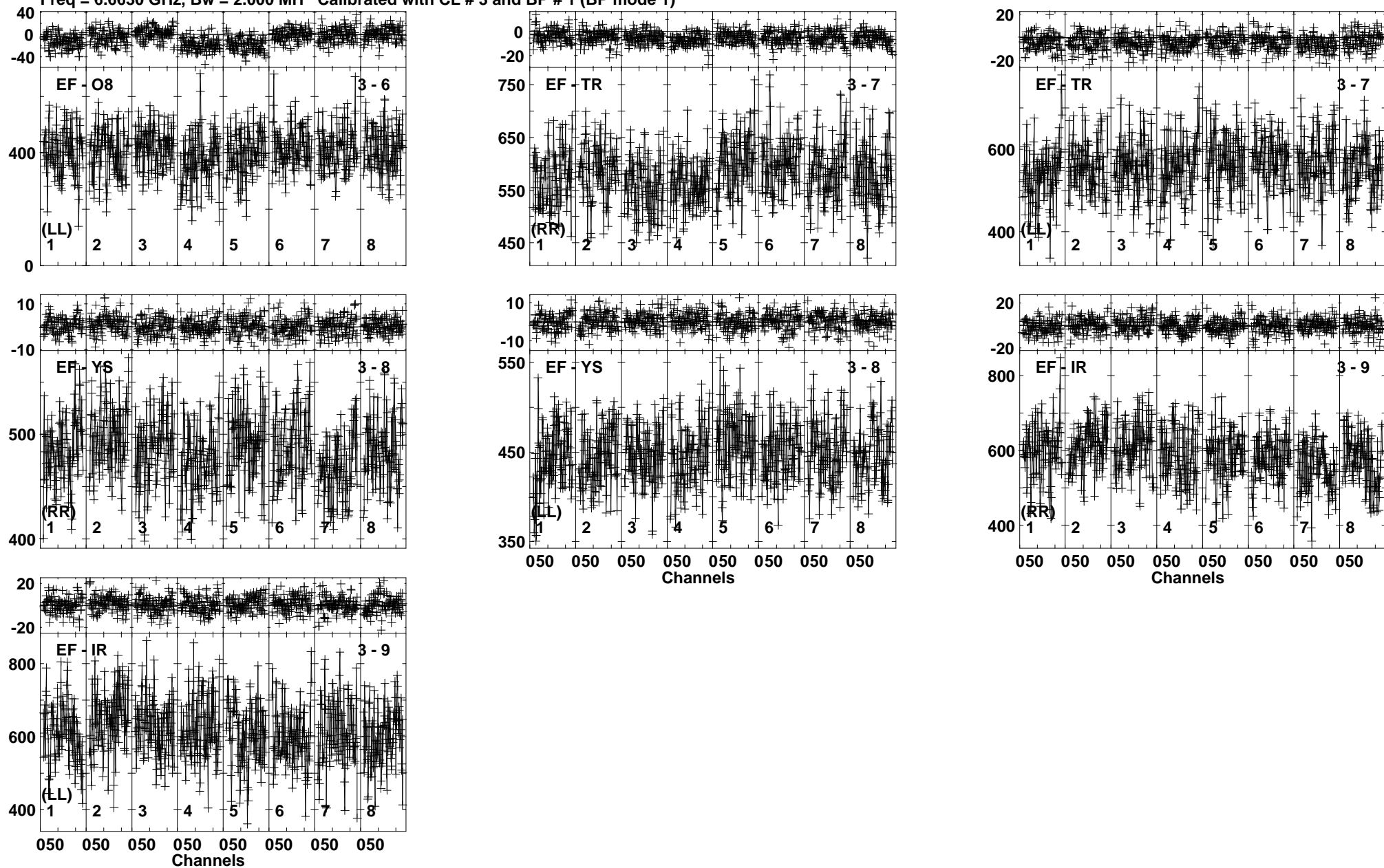
Lower frame: Milli Ampl Jy Top frame: Phas deg Vector averaged cross-power spectrum Baseline: EF (03) - O8 (06) Timerange: 01/05:41:01 to 01/05:42:59
