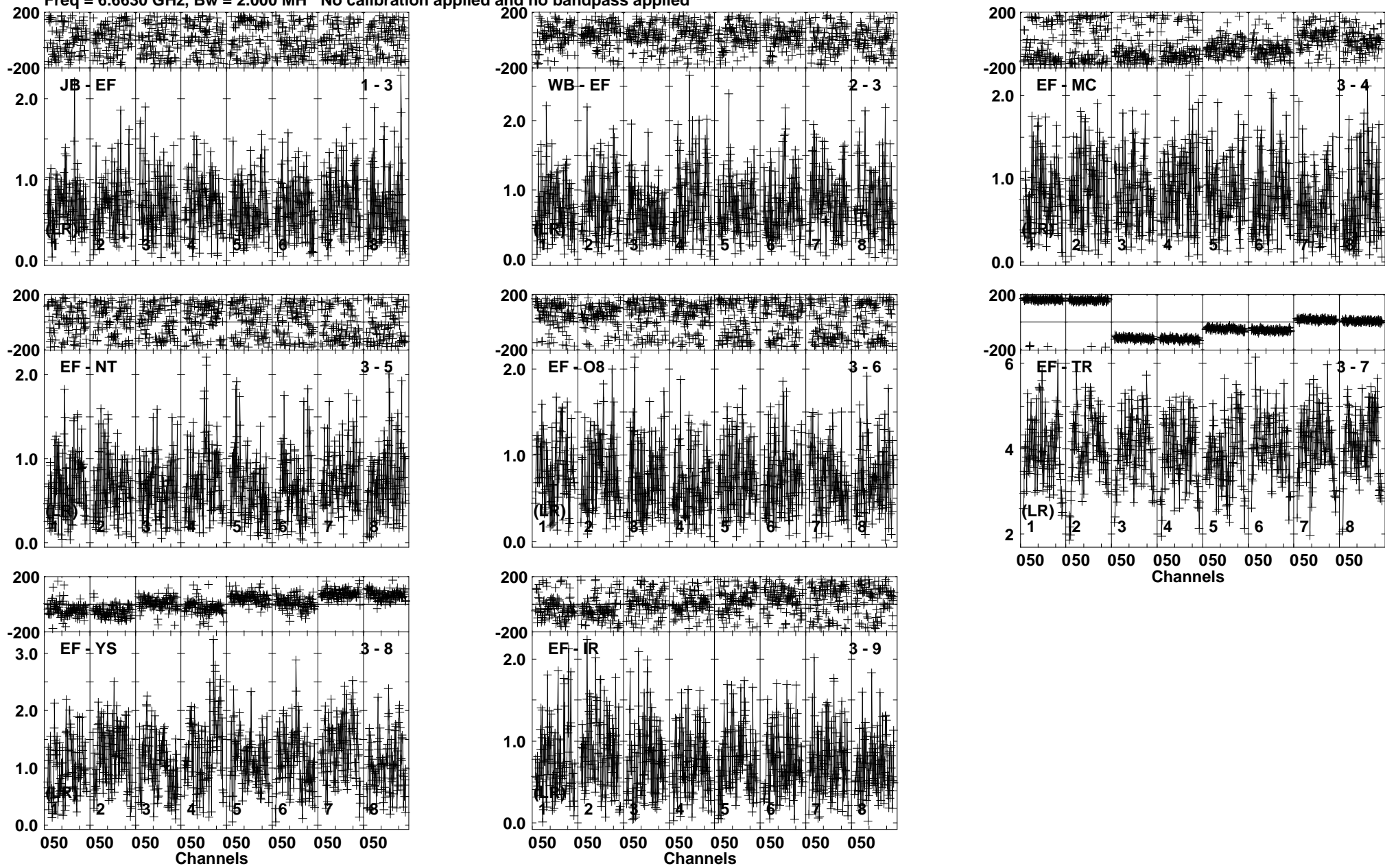
Lower frame: Milli Ampl Jy Top frame: Phas deg Vector averaged cross-power spectrum Baseline: JB (01) - EF (03) Timerange: 01/03:49:40 to 01/03:51:38
