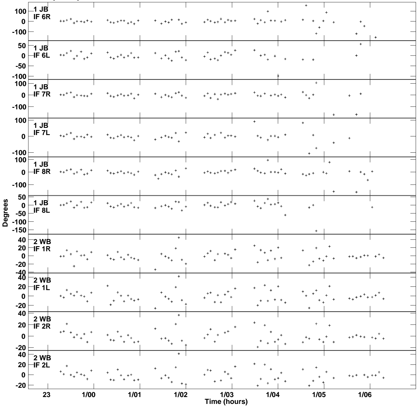
Plot file version 2 created 17-JAN-2018 18:38:40 Gain phs vs UTC time for J1930+1532.MULTI.1 SN 1 Rpol & Lpol IF 1 - 8
