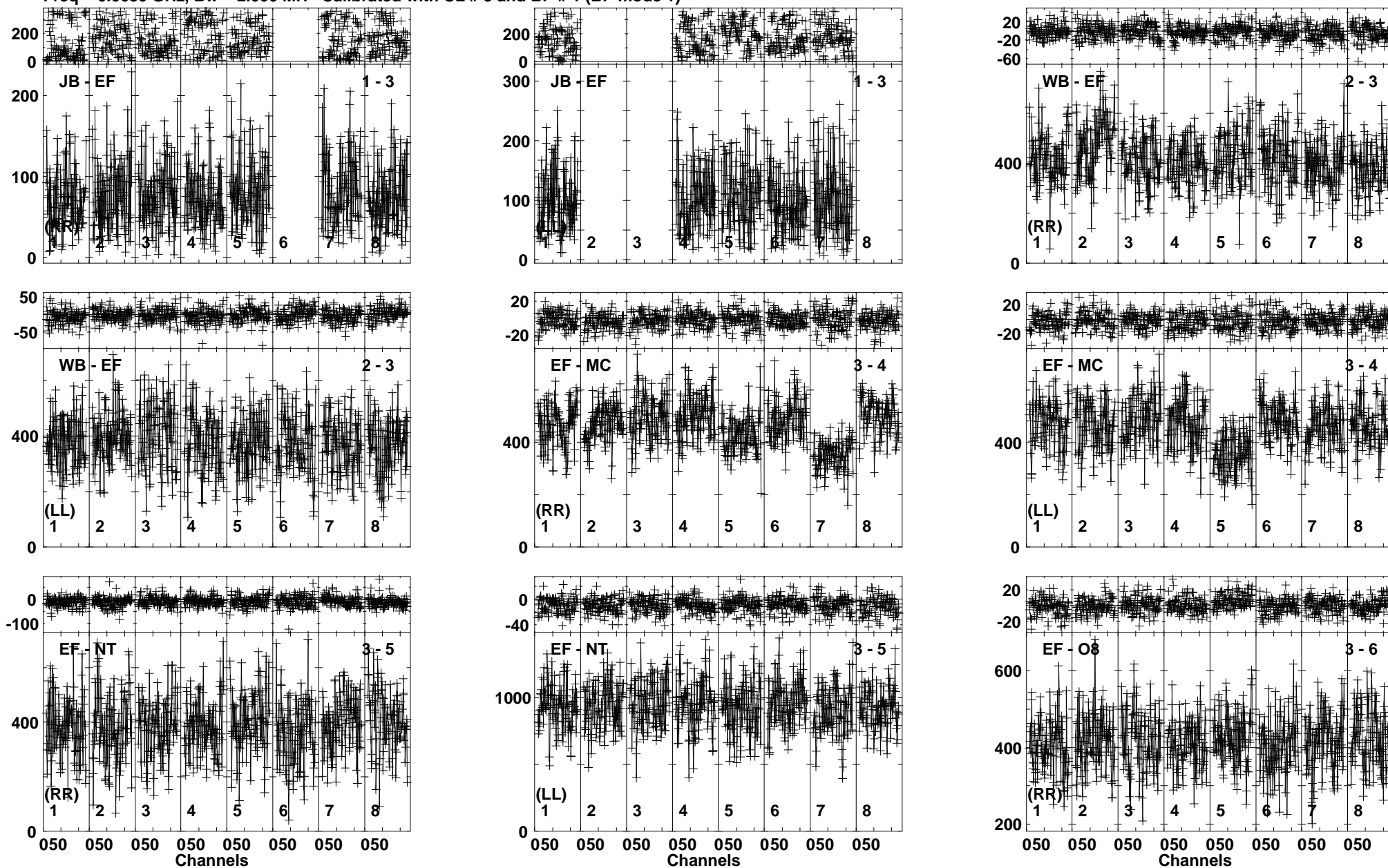
Lower frame: Milli Ampl Jy Top frame: Phas deg Vector averaged cross-power spectrum Baseline: JB (01) - EF (03) Timerange: 01/05:36:33 to 01/05:38:29
