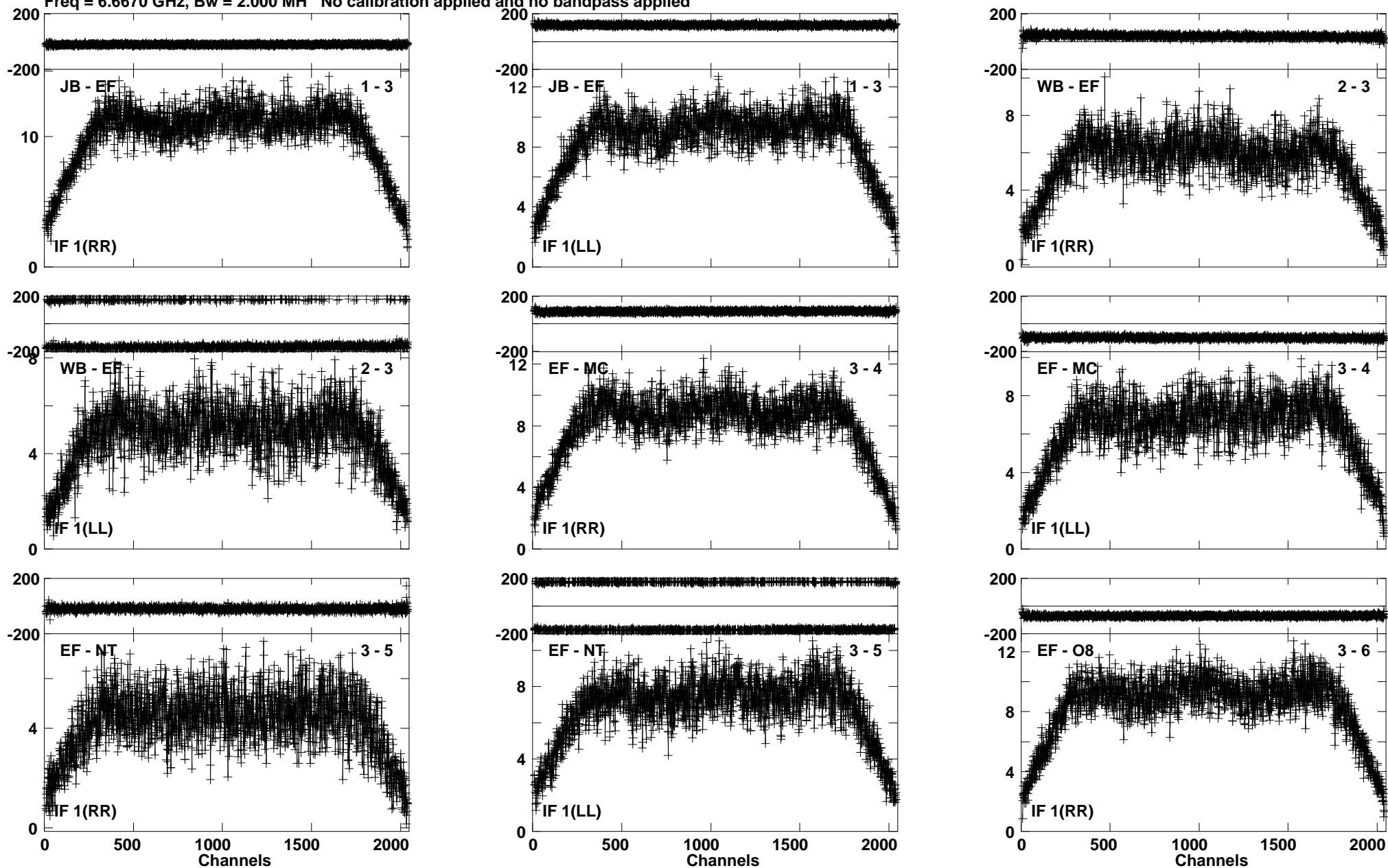
Lower frame: Milli Ampl Jy Top frame: Phas deg Vector averaged cross-power spectrum Baseline: JB (01) - EF (03) Timerange: 01/03:09:45 to 01/03:17:43
