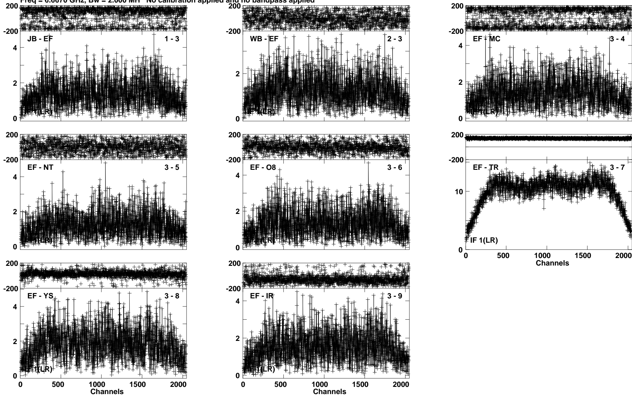
Lower frame: Milli Ampl Jy Top frame: Phas deg Vector averaged cross-power spectrum Baseline: JB (01) - EF (03) Timerange: 01/06:21:38 to 01/06:29:36
