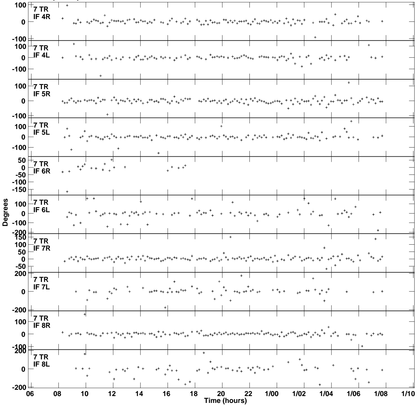
Plot file version 8 created 18-MAY-2015 15:48:21 Gain phs vs UTC time for J1234+619.MULTI.1 SN 1 Rpol & Lpol IF 1 - 8
