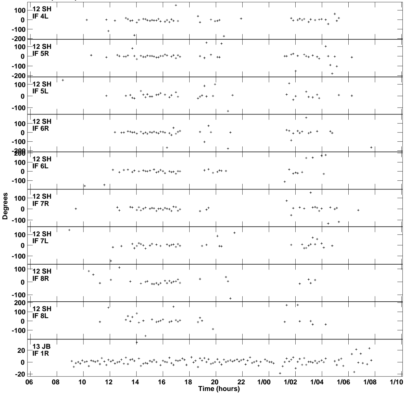
Plot file version 14 created 18-MAY-2015 15:48:21 Gain phs vs UTC time for J1234+619.MULTI.1 SN 1 Rpol & Lpol IF 1 - 8
