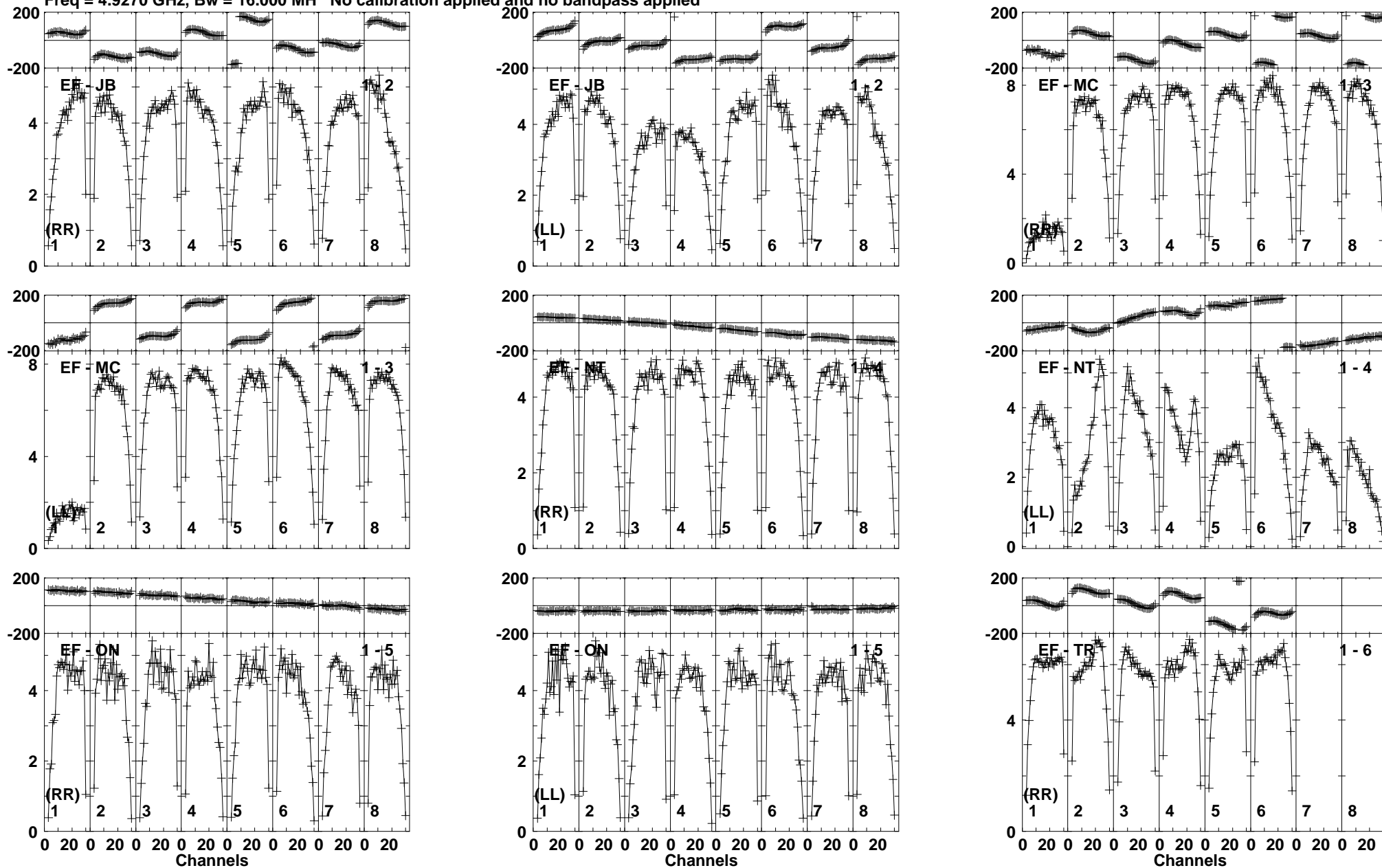
Lower frame: Milli Ampl Jy Top frame: Phas deg Vector averaged cross-power spectrum Baseline: EF (01) - JB (02) Timerange: 00/22:15:11 to 00/22:16:39
