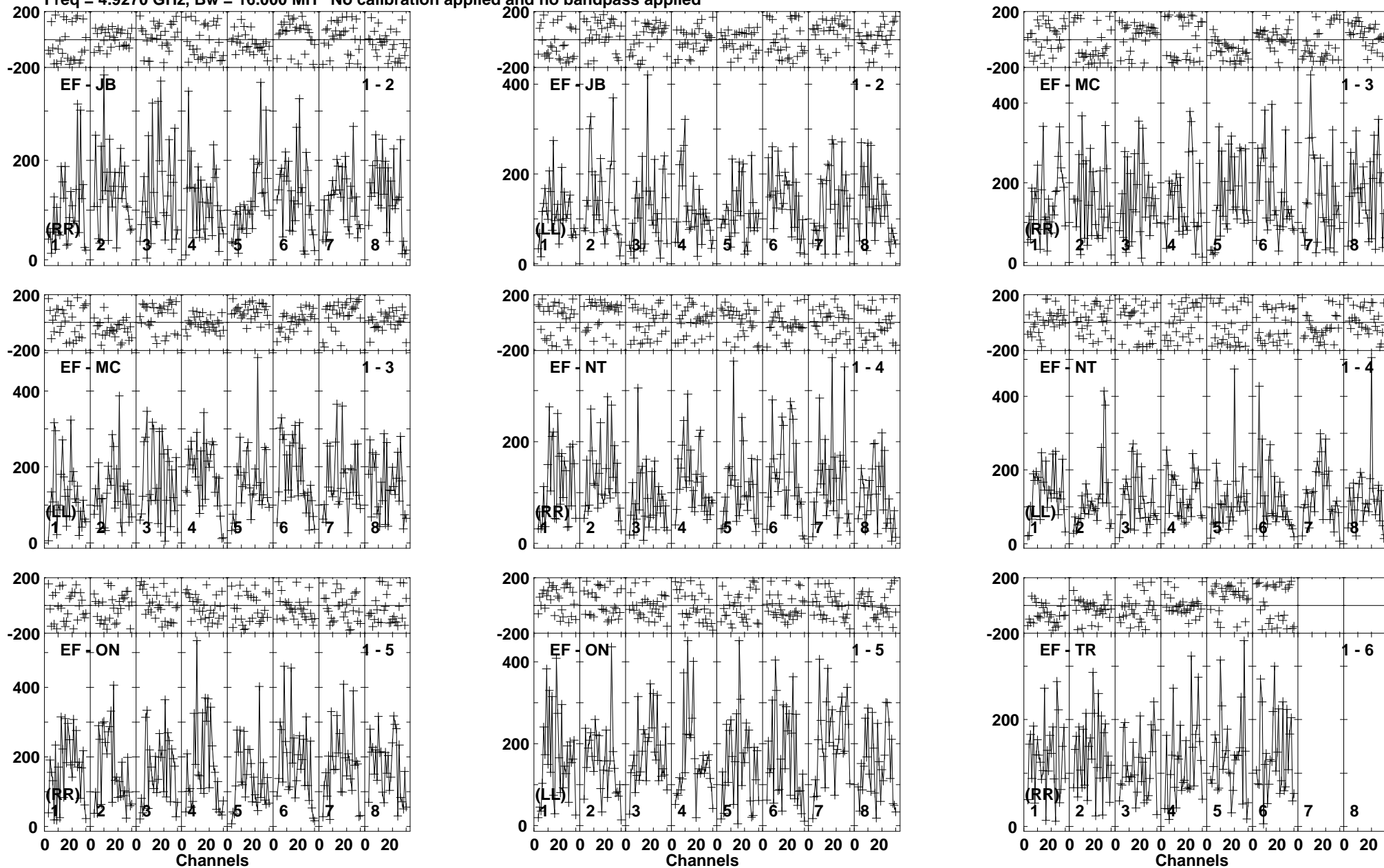
Lower frame: Micro Ampl Jy Top frame: Phas deg Vector averaged cross-power spectrum Baseline: EF (01) - JB (02) Timerange: 00/20:41:41 to 00/20:45:09
