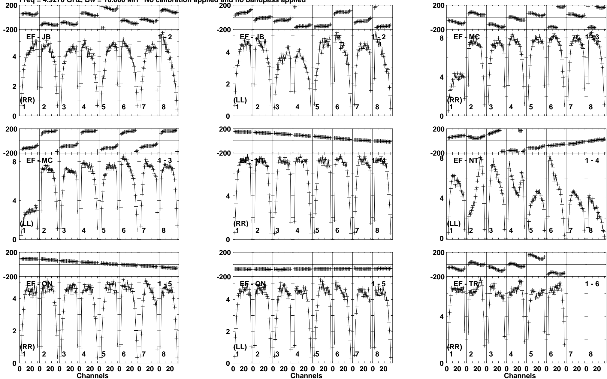
Lower frame: Milli Ampl Jy Top frame: Phas deg Vector averaged cross-power spectrum Baseline: EF (01) - JB (02) Timerange: 00/23:16:41 to 00/23:17:39
