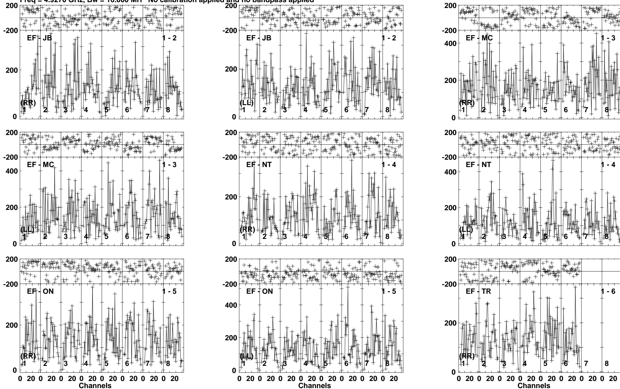
Lower frame: Micro Ampl Jy Top frame: Phas deg Vector averaged cross-power spectrum Baseline: EF (01) - JB (02) Timerange: 01/01:36:41 to 01/01:40:09
