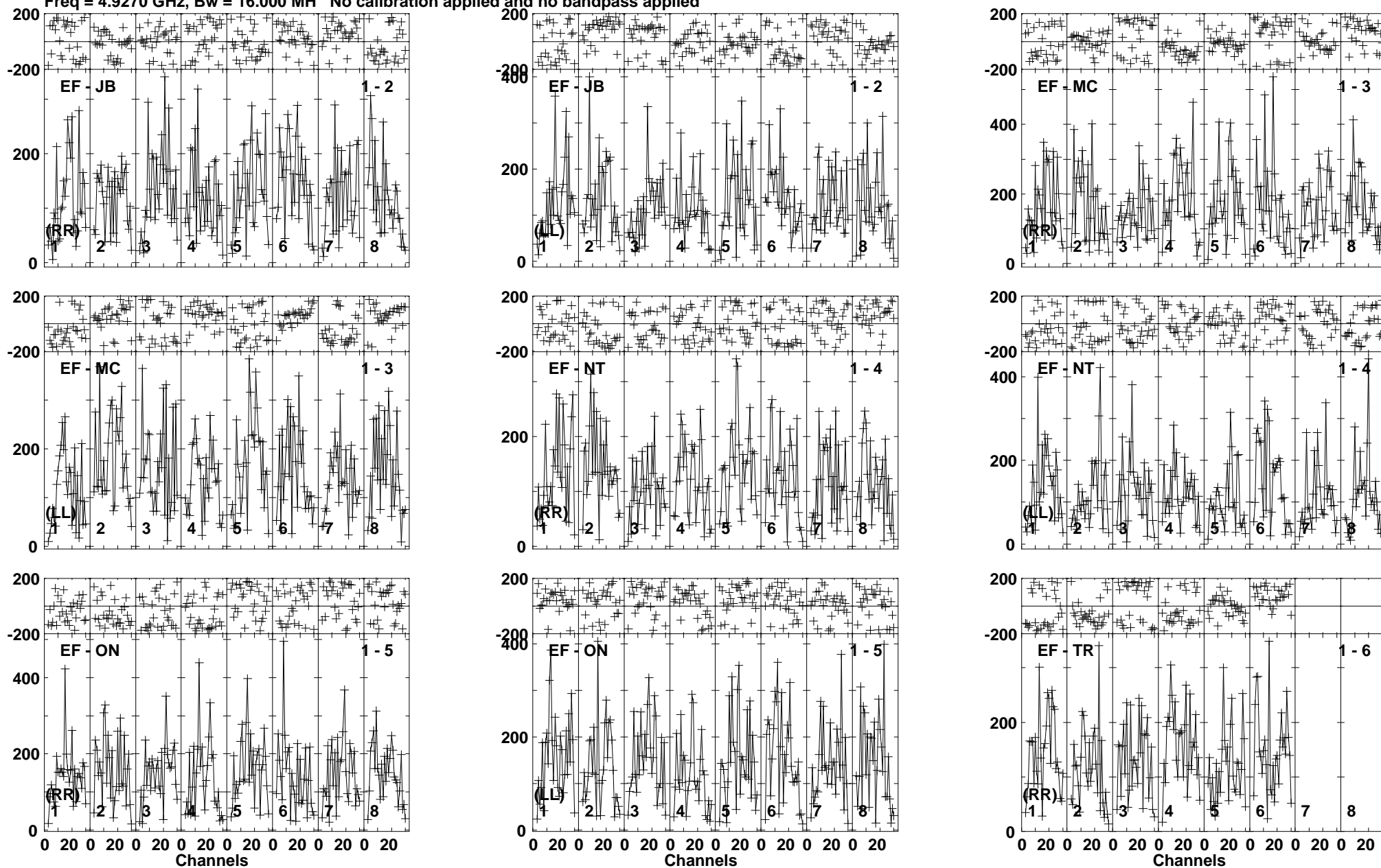
Lower frame: Micro Ampl Jy Top frame: Phas deg Vector averaged cross-power spectrum Baseline: EF (01) - JB (02) Timerange: 00/23:02:41 to 00/23:06:09
