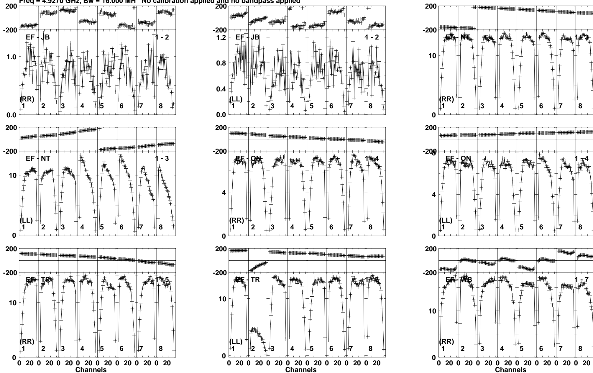
Lower frame: Milli Ampl Jy Top frame: Phas deg Vector averaged cross-power spectrum Baseline: EF (01) - JB (02) Timerange: 00/19:16:01 to 00/19:16:59
