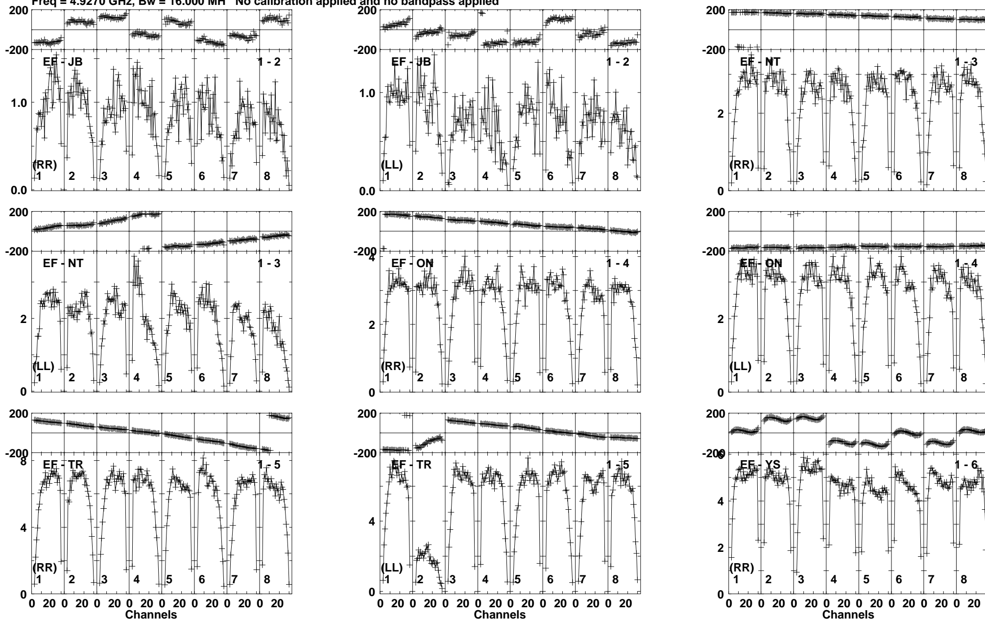
Lower frame: Milli Ampl Jy Top frame: Phas deg Vector averaged cross-power spectrum Baseline: EF (01) - JB (02) Timerange: 01/06:04:21 to 01/06:05:19
