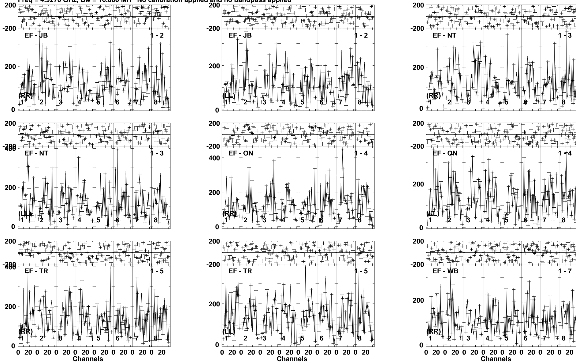
Lower frame: Micro Ampl Jy Top frame: Phas deg Vector averaged cross-power spectrum Baseline: EF (01) - JB (02) Timerange: 00/22:38:31 to 00/22:41:59
