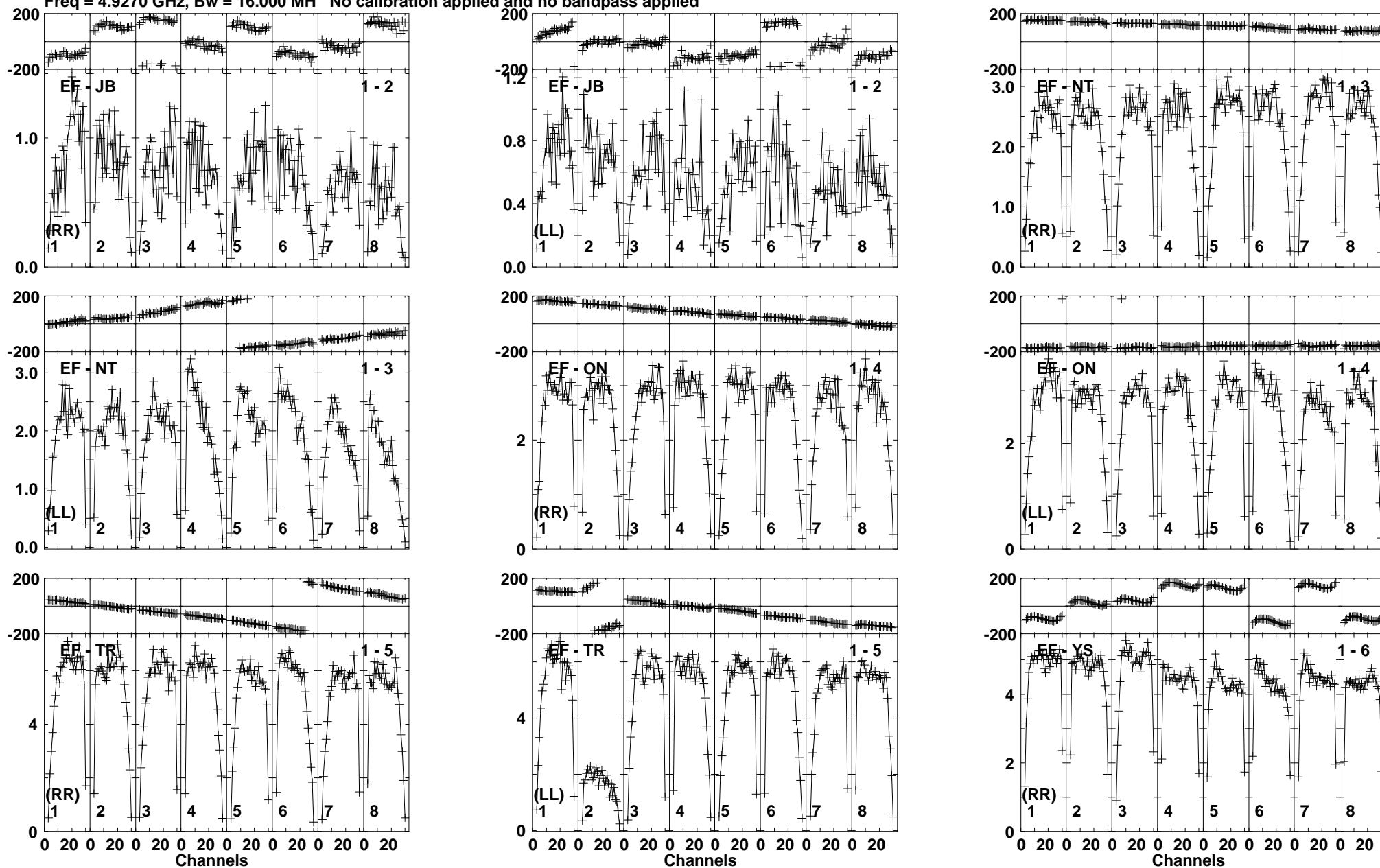
Lower frame: Milli Ampl Jy Top frame: Phas deg Vector averaged cross-power spectrum Baseline: EF (01) - JB (02) Timerange: 01/06:34:21 to 01/06:35:19
