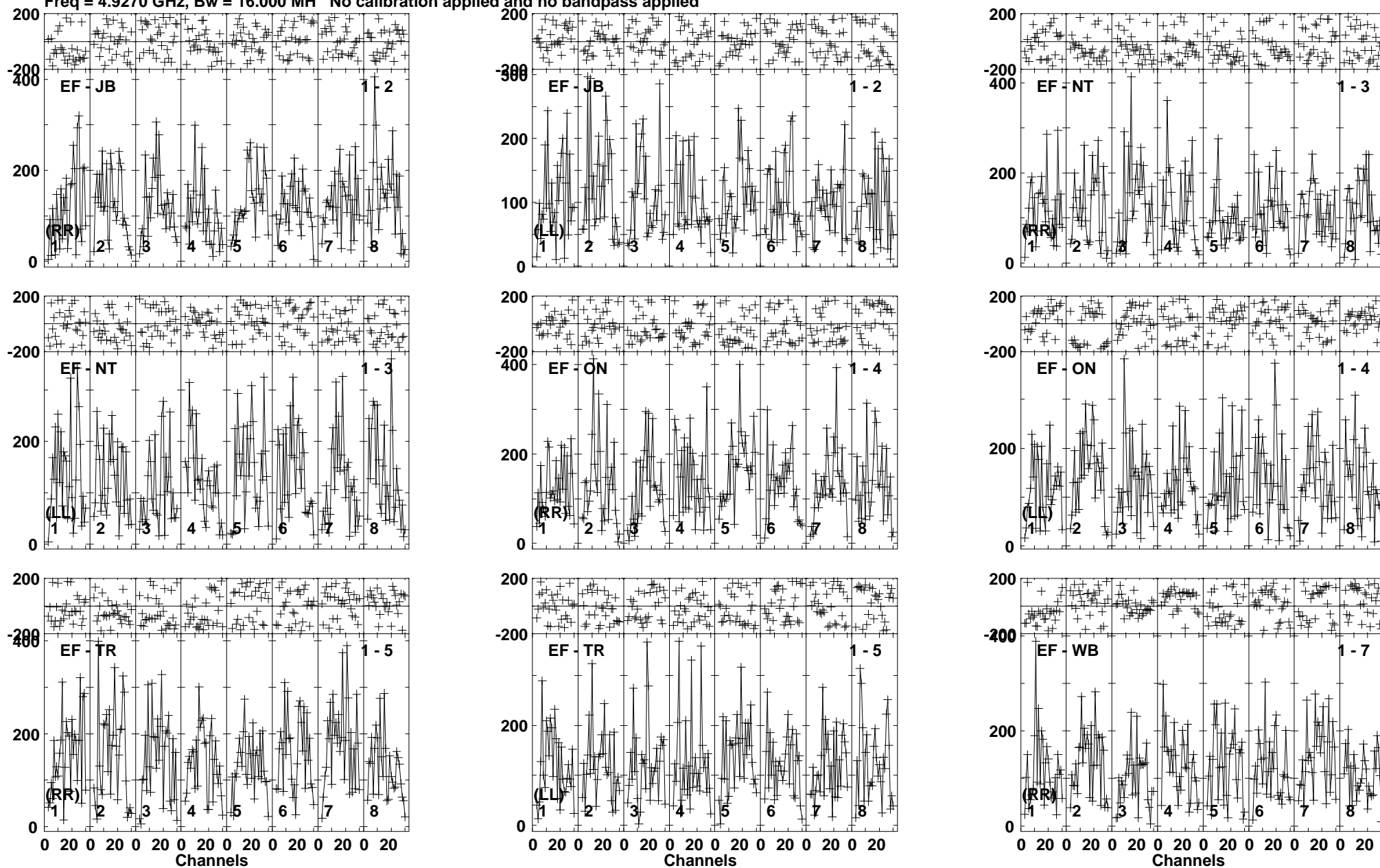
Lower frame: Micro Ampl Jy Top frame: Phas deg Vector averaged cross-power spectrum Baseline: EF (01) - JB (02) Timerange: 01/05:11:01 to 01/05:14:29
