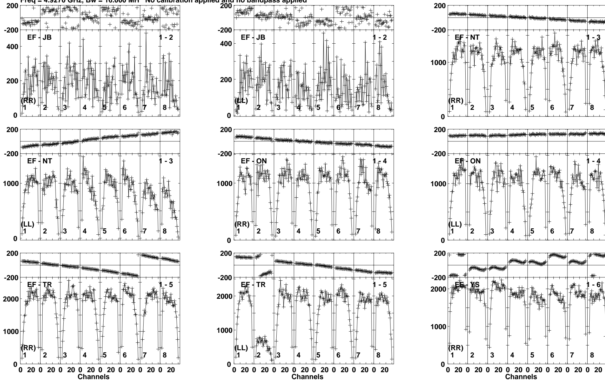
Lower frame: Micro Ampl Jy Top frame: Phas deg Vector averaged cross-power spectrum Baseline: EF (01) - JB (02) Timerange: 01/06:50:21 to 01/06:53:49
