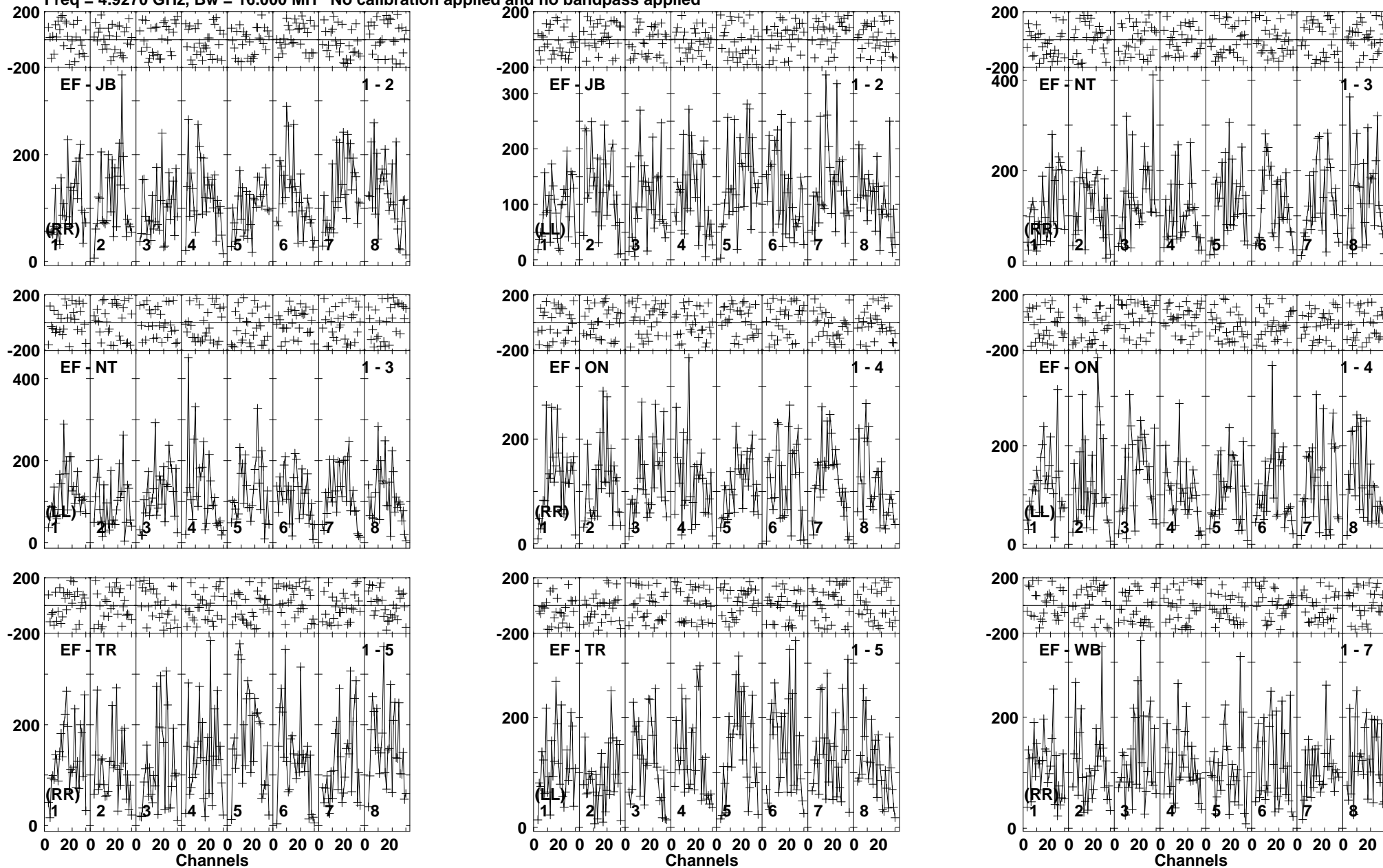
Lower frame: Micro Ampl Jy Top frame: Phas deg Vector averaged cross-power spectrum Baseline: EF (01) - JB (02) Timerange: 01/00:06:41 to 01/00:10:09
