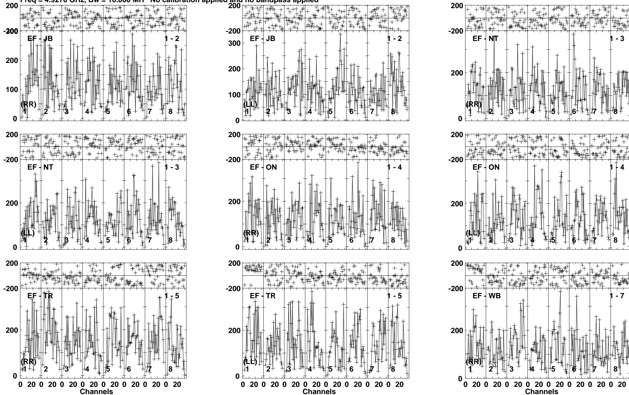
Lower frame: Micro Ampl Jy Top frame: Phas deg Vector averaged cross-power spectrum Baseline: EF (01) - JB (02) Timerange: 01/03:56:01 to 01/03:59:29
