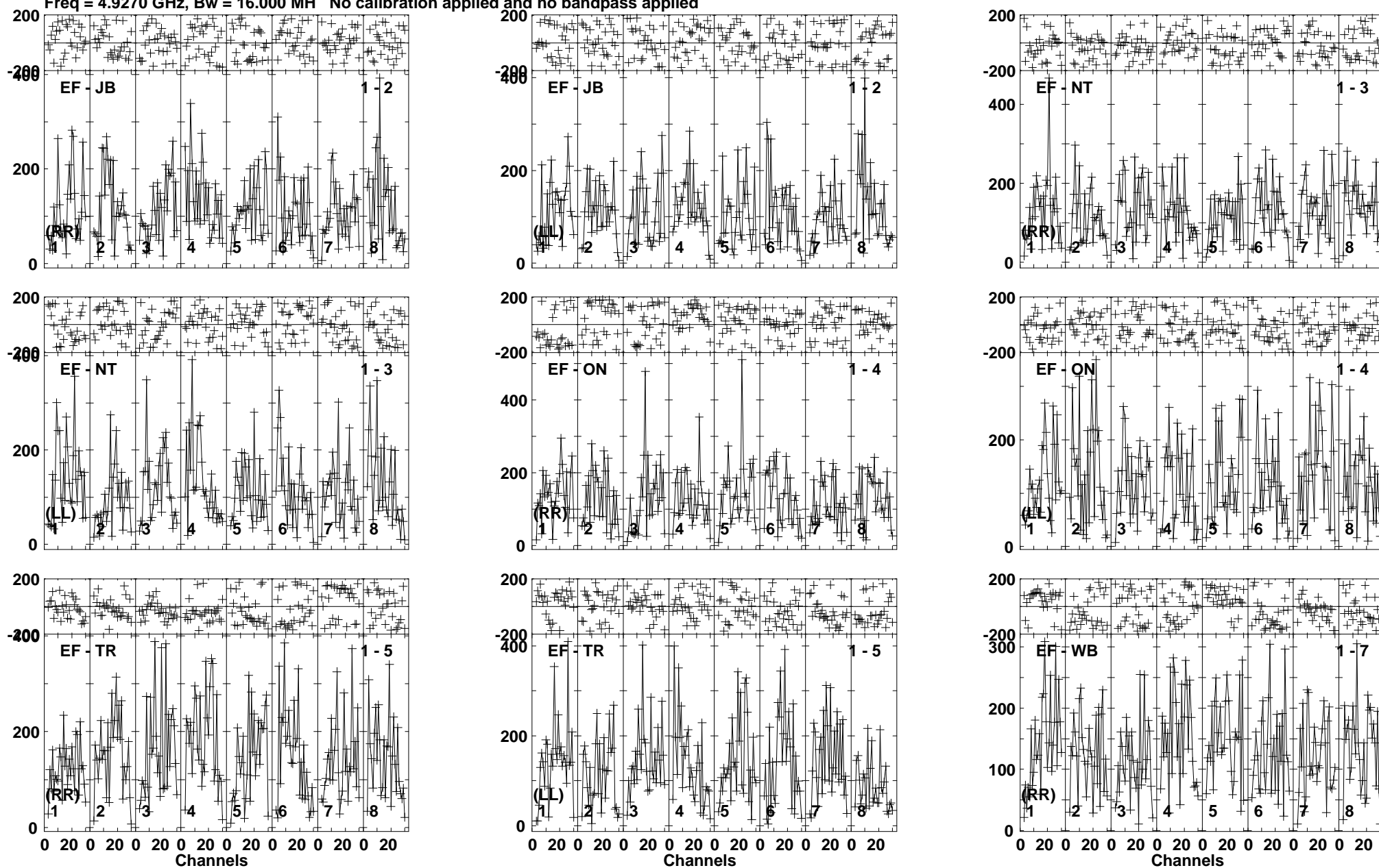
Lower frame: Micro Ampl Jy Top frame: Phas deg Vector averaged cross-power spectrum Baseline: EF (01) - JB (02) Timerange: 01/03:26:01 to 01/03:29:29
