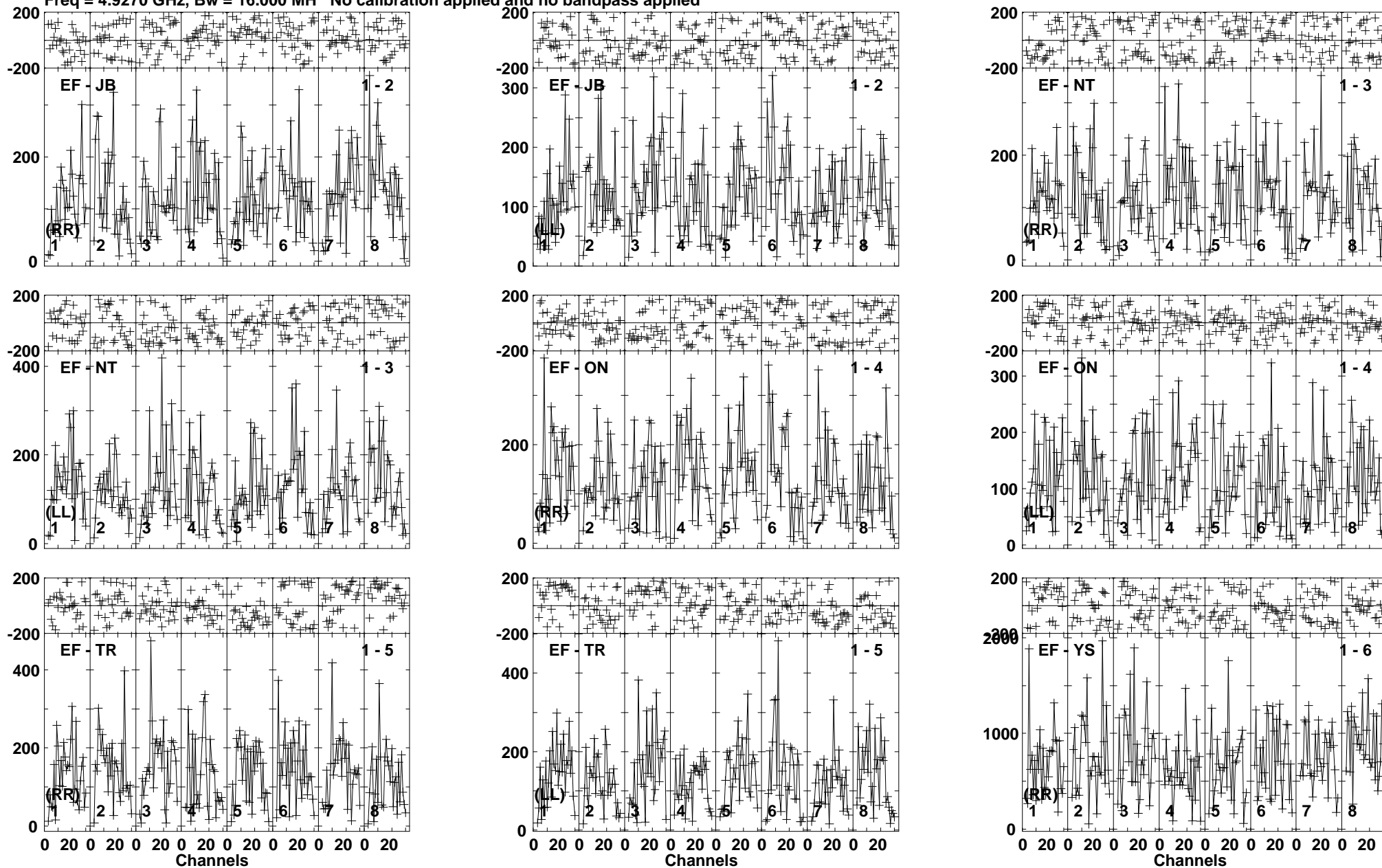
Lower frame: Micro Ampl Jy Top frame: Phas deg Vector averaged cross-power spectrum Baseline: EF (01) - JB (02) Timerange: 01/05:21:01 to 01/05:24:29
