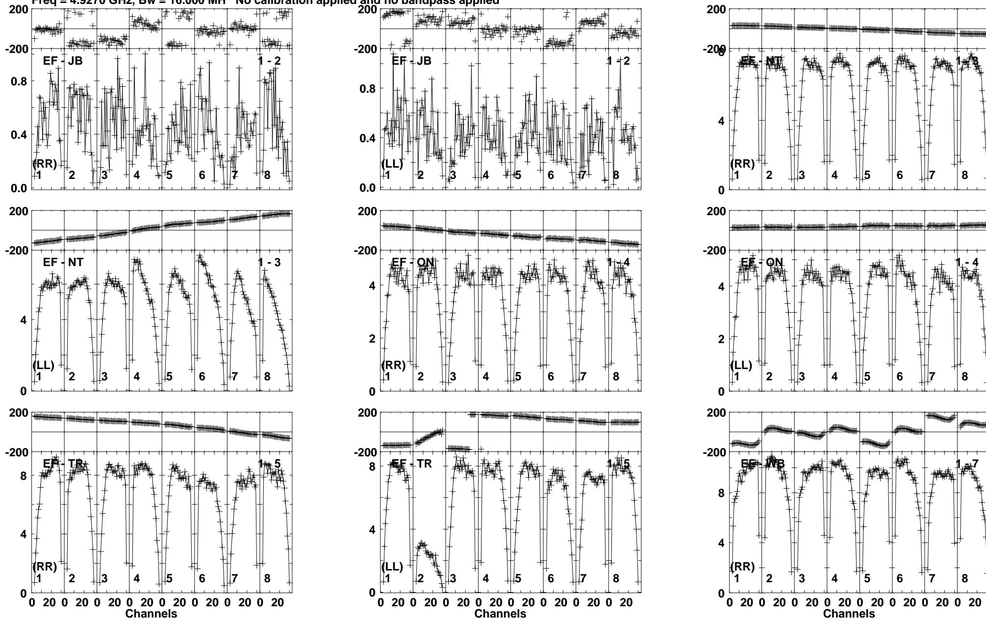
Lower frame: Milli Ampl Jy Top frame: Phas deg Vector averaged cross-power spectrum Baseline: EF (01) - JB (02) Timerange: 00/21:00:31 to 00/21:01:59
