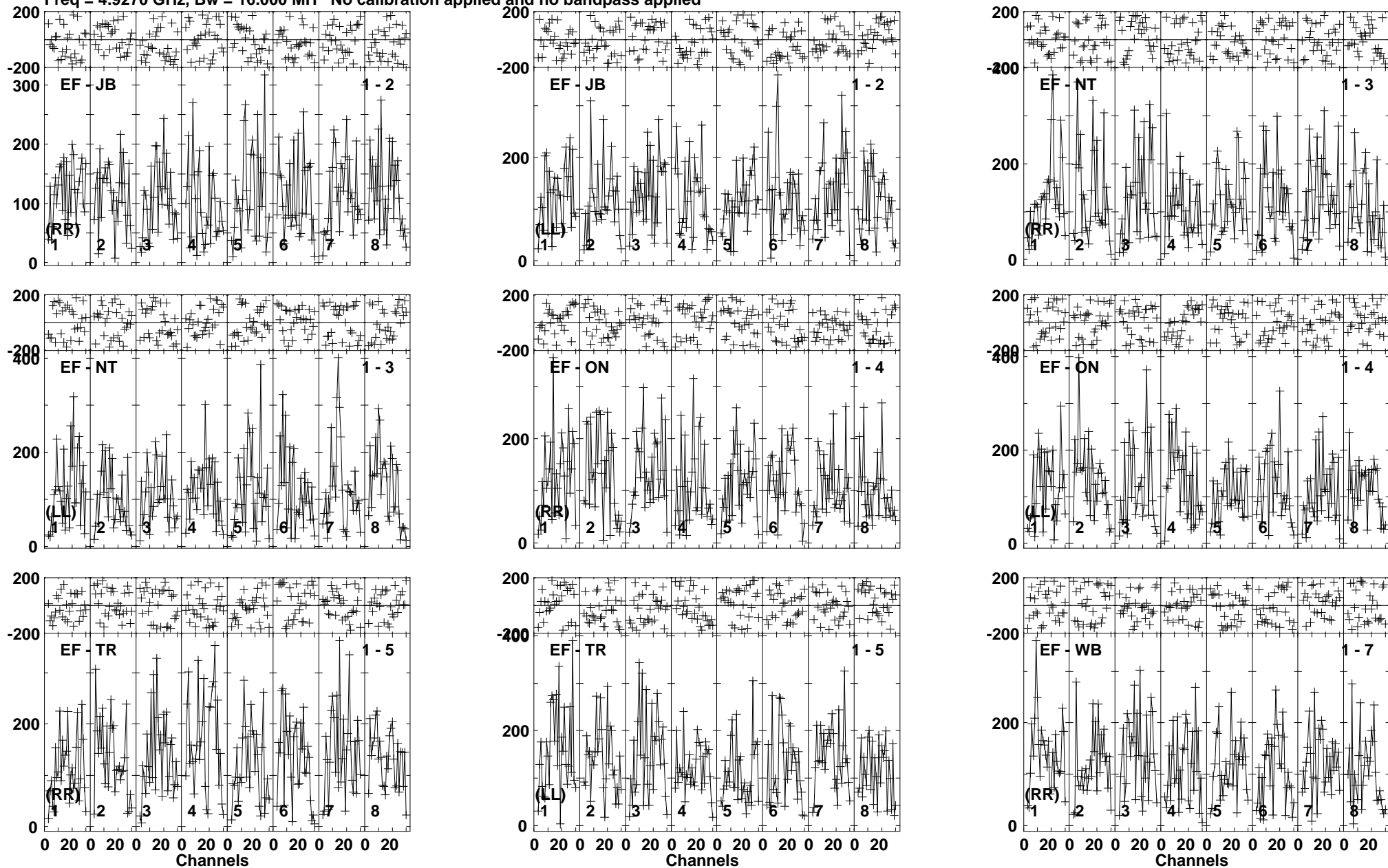
Lower frame: Micro Ampl Jy Top frame: Phas deg Vector averaged cross-power spectrum Baseline: EF (01) - JB (02) Timerange: 00/21:58:31 to 00/22:01:59
