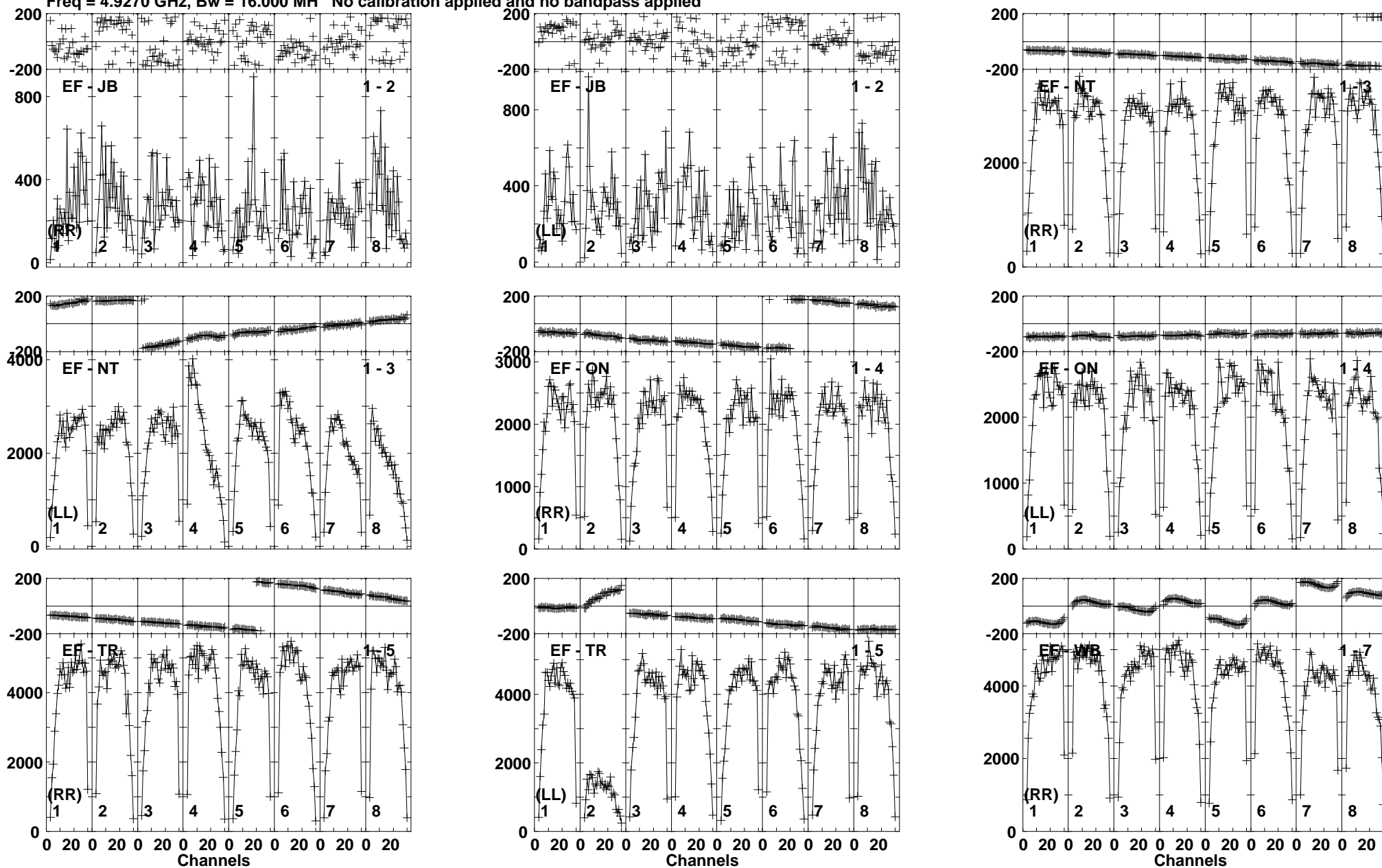
Lower frame: Micro Ampl Jy Top frame: Phas deg Vector averaged cross-power spectrum Baseline: EF (01) - JB (02) Timerange: 01/02:40:11 to 01/02:41:39
