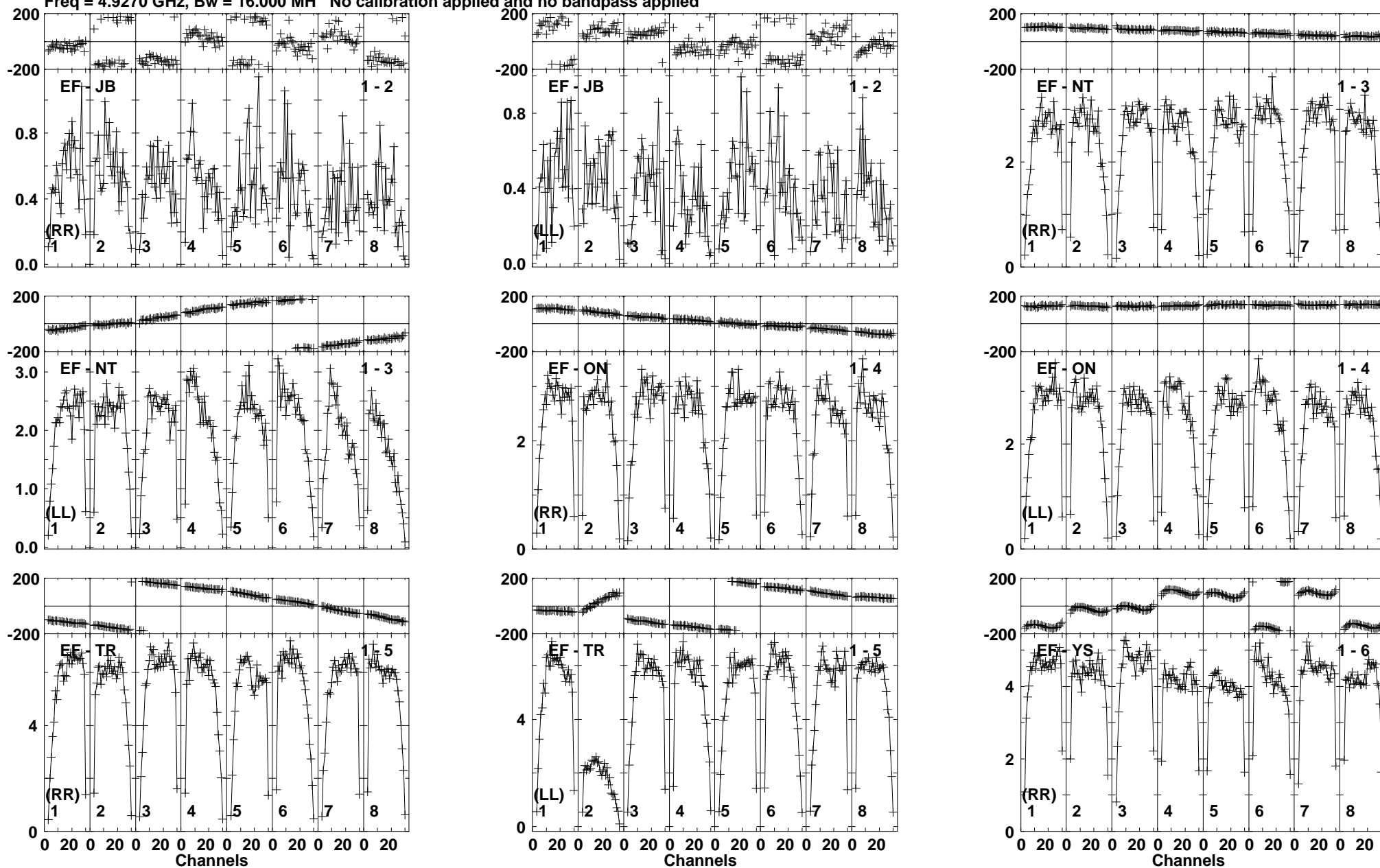
Lower frame: Milli Ampl Jy Top frame: Phas deg Vector averaged cross-power spectrum Baseline: EF (01) - JB (02) Timerange: 01/07:04:21 to 01/07:05:19
