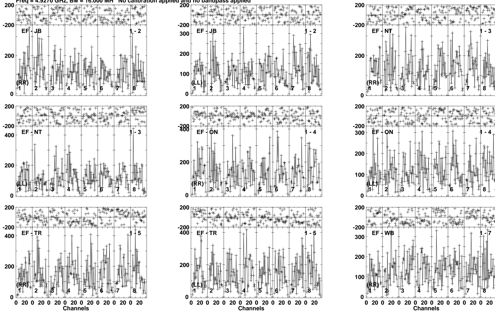
Lower frame: Micro Ampl Jy Top frame: Phas deg Vector averaged cross-power spectrum Baseline: EF (01) - JB (02) Timerange: 01/04:16:01 to 01/04:19:29
