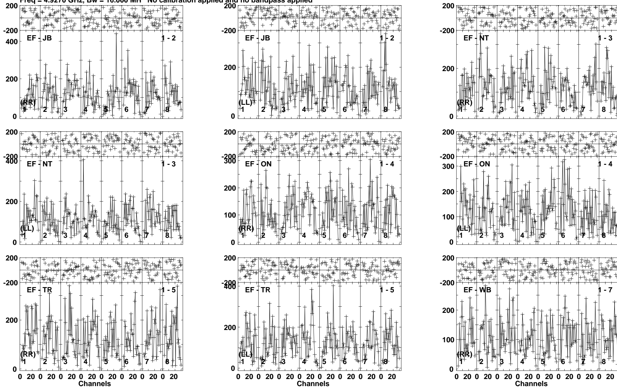
Lower frame: Micro Ampl Jy Top frame: Phas deg Vector averaged cross-power spectrum Baseline: EF (01) - JB (02) Timerange: 00/19:12:01 to 00/19:15:29
