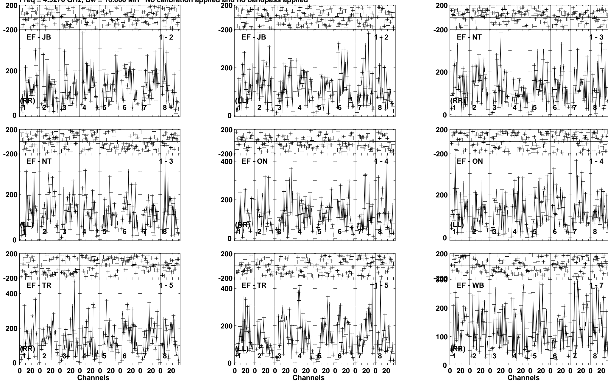
Lower frame: Micro Ampl Jy Top frame: Phas deg Vector averaged cross-power spectrum Baseline: EF (01) - JB (02) Timerange: 01/04:41:01 to 01/04:44:29
