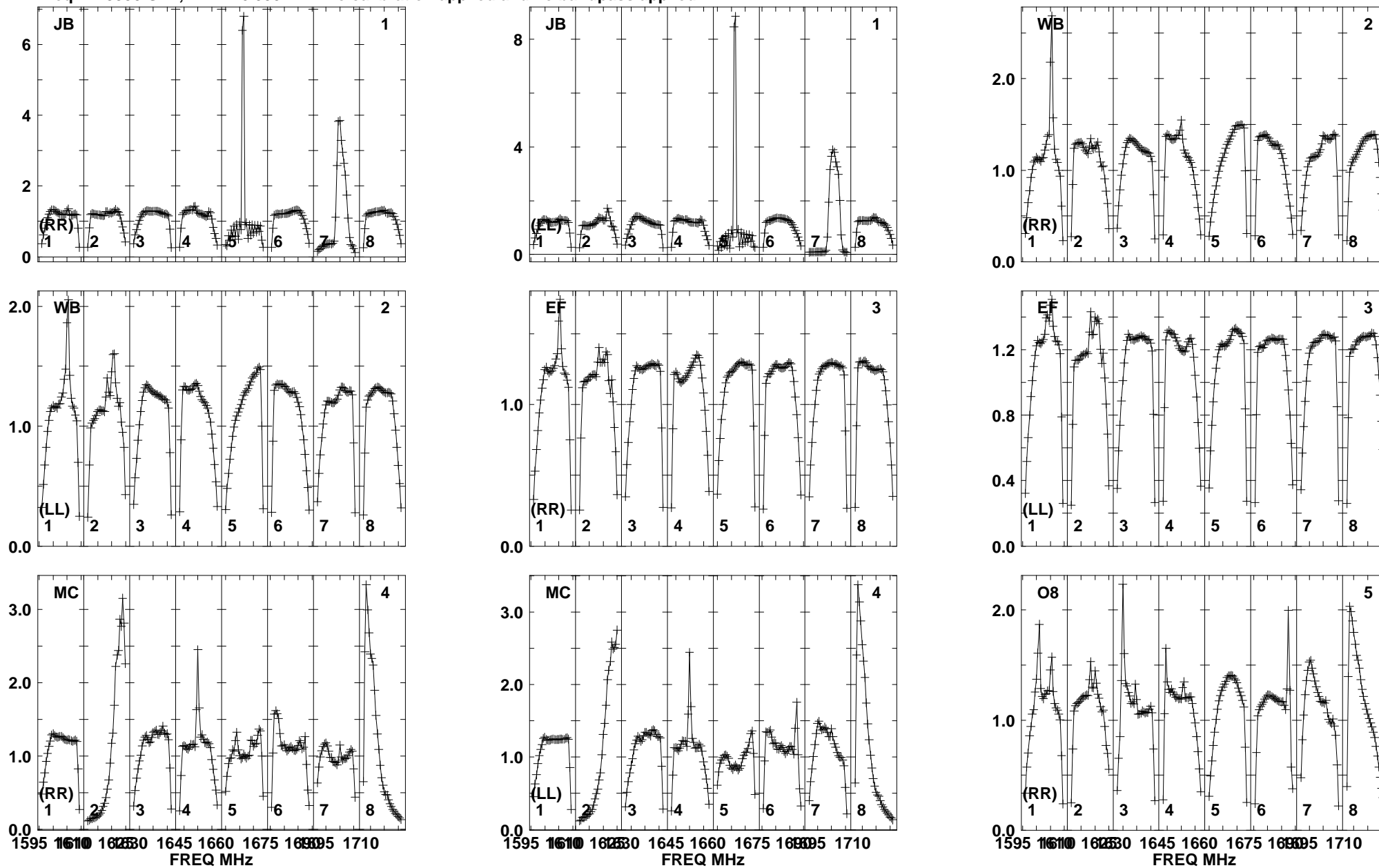
Lower frame: Real Jy Total-power spectrum Antenna: JB (01) Timerange: 00/20:28:48 to 00/20:32:16
