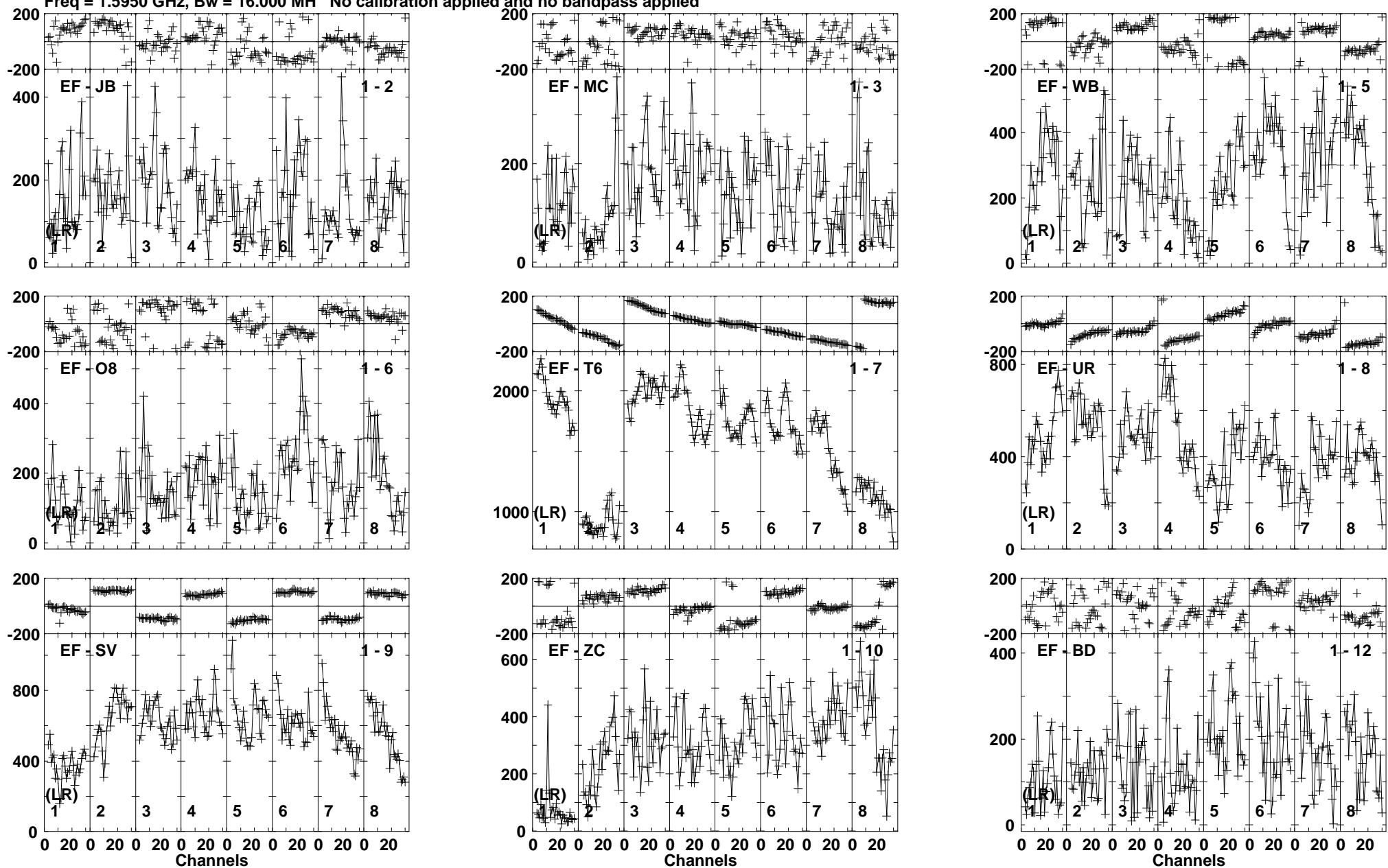
Lower frame: Micro Ampl Jy Top frame: Phas deg Vector averaged cross-power spectrum Baseline: EF (01) - JB (02) Timerange: 00/20:51:59 to 00/20:53:49
