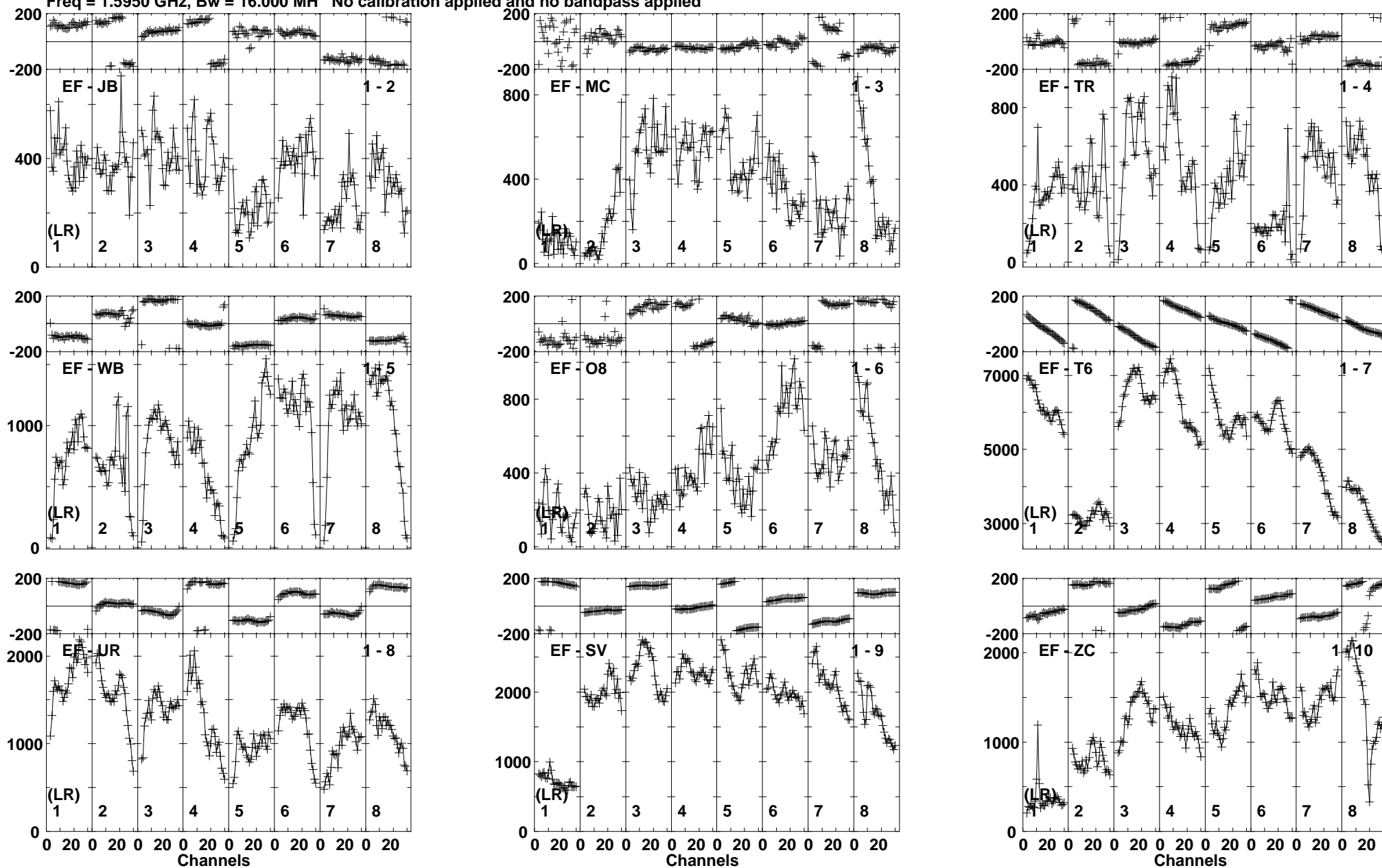
Lower frame: Micro Ampl Jy Top frame: Phas deg Vector averaged cross-power spectrum Baseline: EF (01) - JB (02) Timerange: 00/13:44:09 to 00/13:45:59
