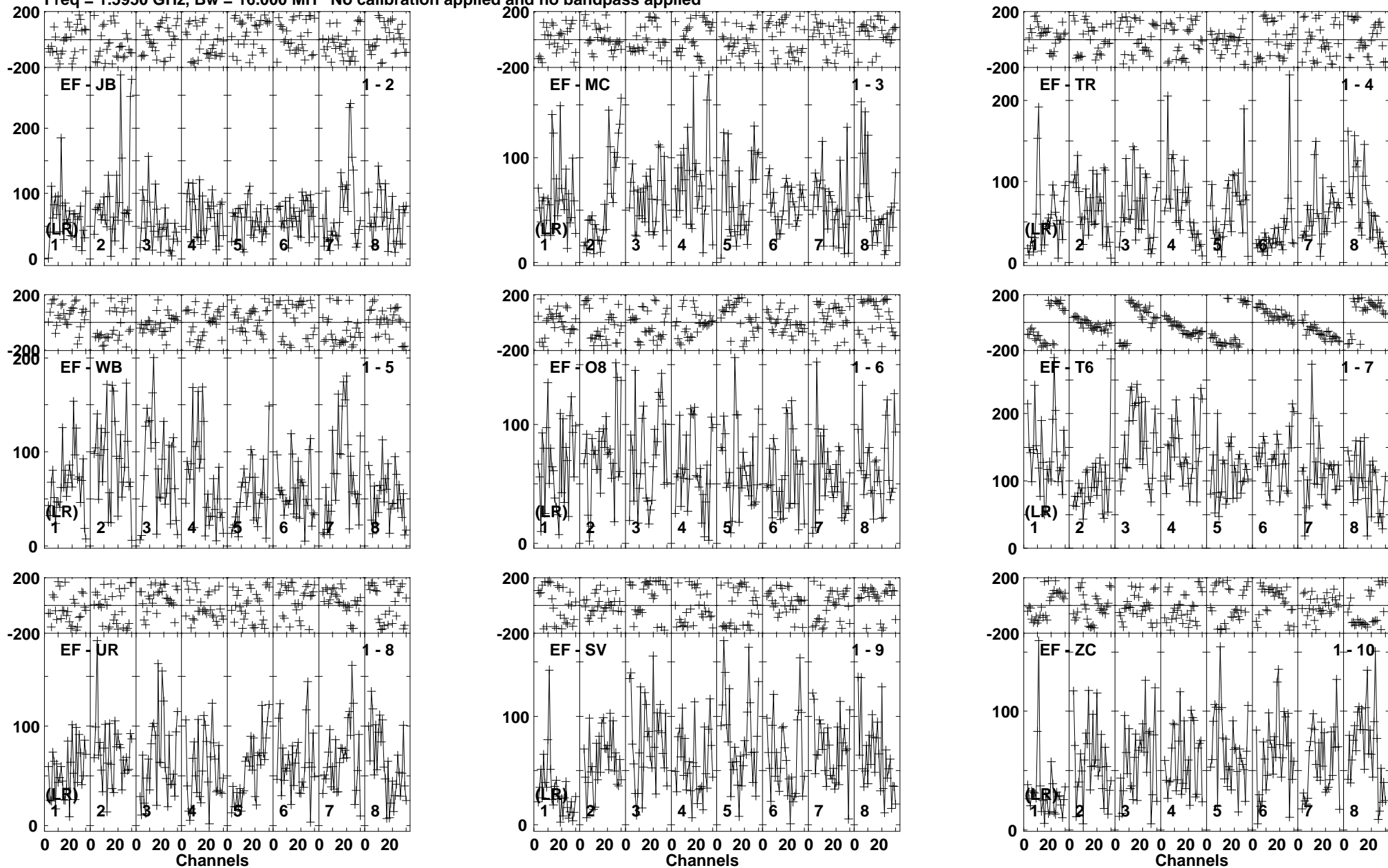
Lower frame: Micro Ampl Jy Top frame: Phas deg Vector averaged cross-power spectrum Baseline: EF (01) - JB (02) Timerange: 00/13:32:09 to 00/13:36:59
