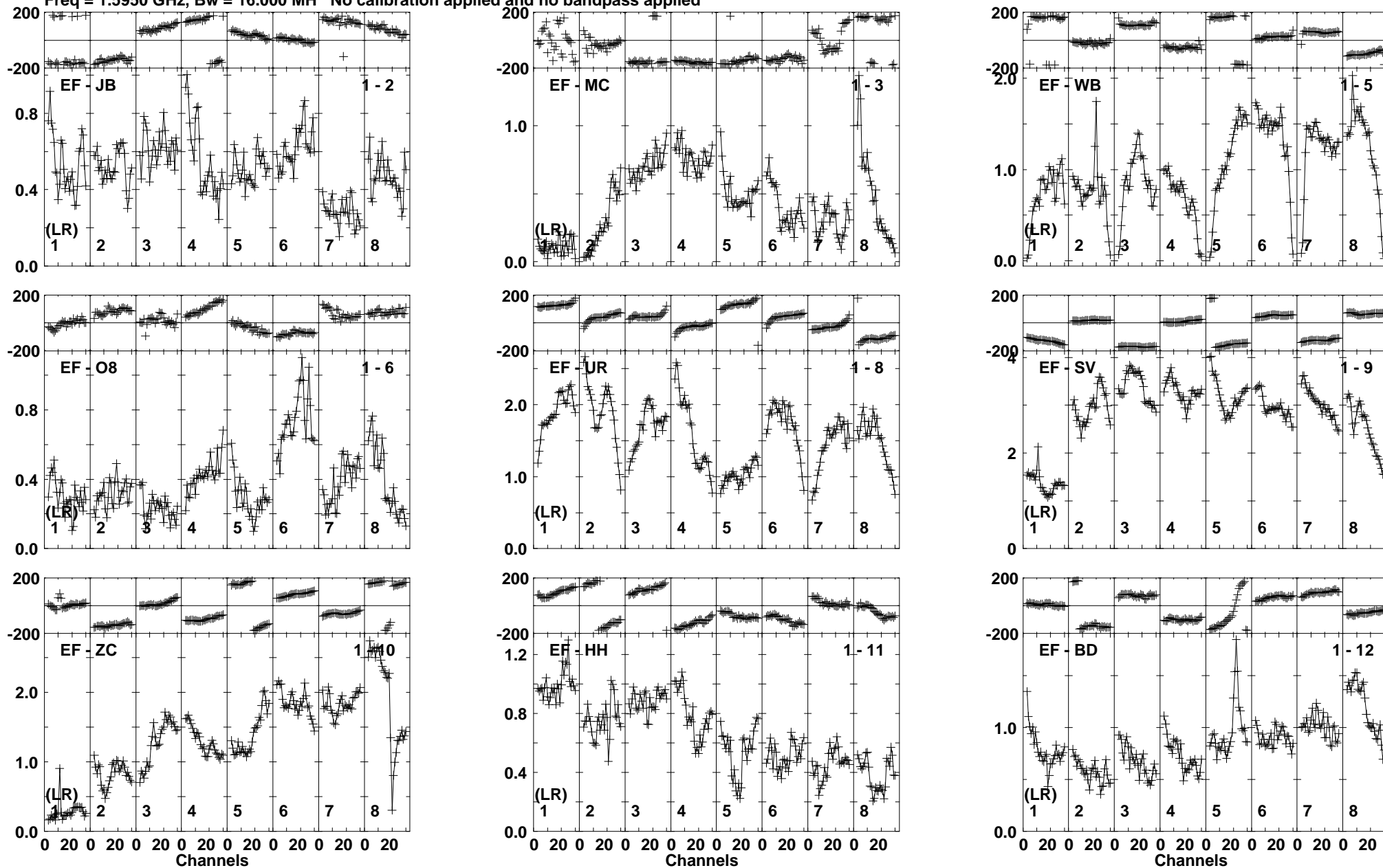
Lower frame: Milli Ampl Jy Top frame: Phas deg Vector averaged cross-power spectrum Baseline: EF (01) - JB (02) Timerange: 00/18:16:01 to 00/18:17:19
