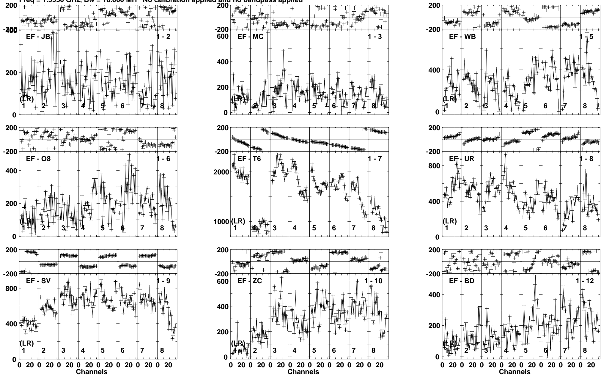
Lower frame: Micro Ampl Jy Top frame: Phas deg Vector averaged cross-power spectrum Baseline: EF (01) - JB (02) Timerange: 00/21:19:59 to 00/21:21:49
