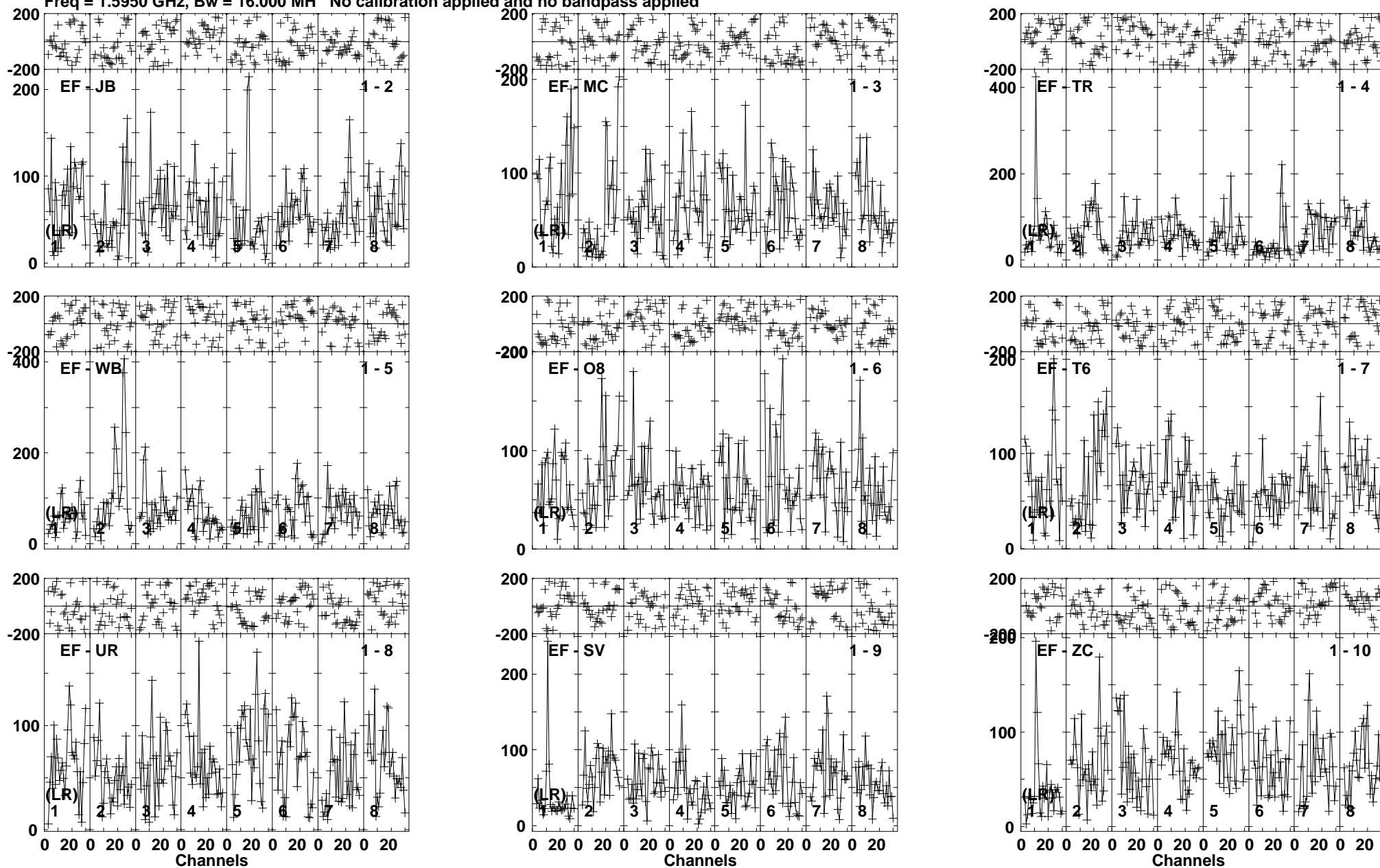
Lower frame: Micro Ampl Jy Top frame: Phas deg Vector averaged cross-power spectrum Baseline: EF (01) - JB (02) Timerange: 00/14:28:19 to 00/14:33:09
