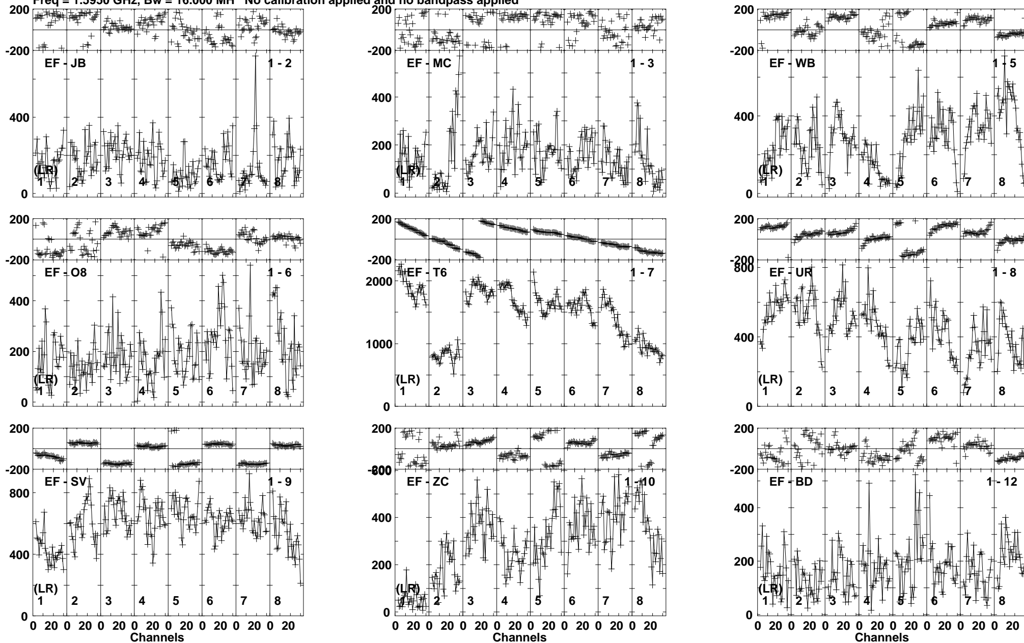
Lower frame: Micro Ampl Jy Top frame: Phas deg Vector averaged cross-power spectrum Baseline: EF (01) - JB (02) Timerange: 00/20:59:31 to 00/21:00:49
