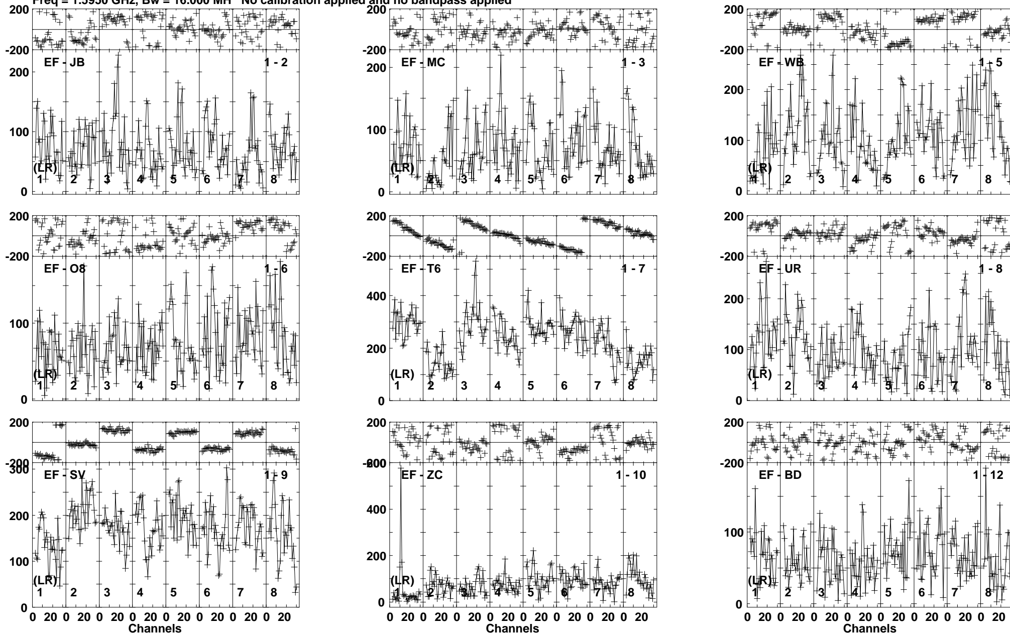
Lower frame: Micro Ampl Jy Top frame: Phas deg Vector averaged cross-power spectrum Baseline: EF (01) - JB (02) Timerange: 00/21:35:57 to 00/21:40:49
