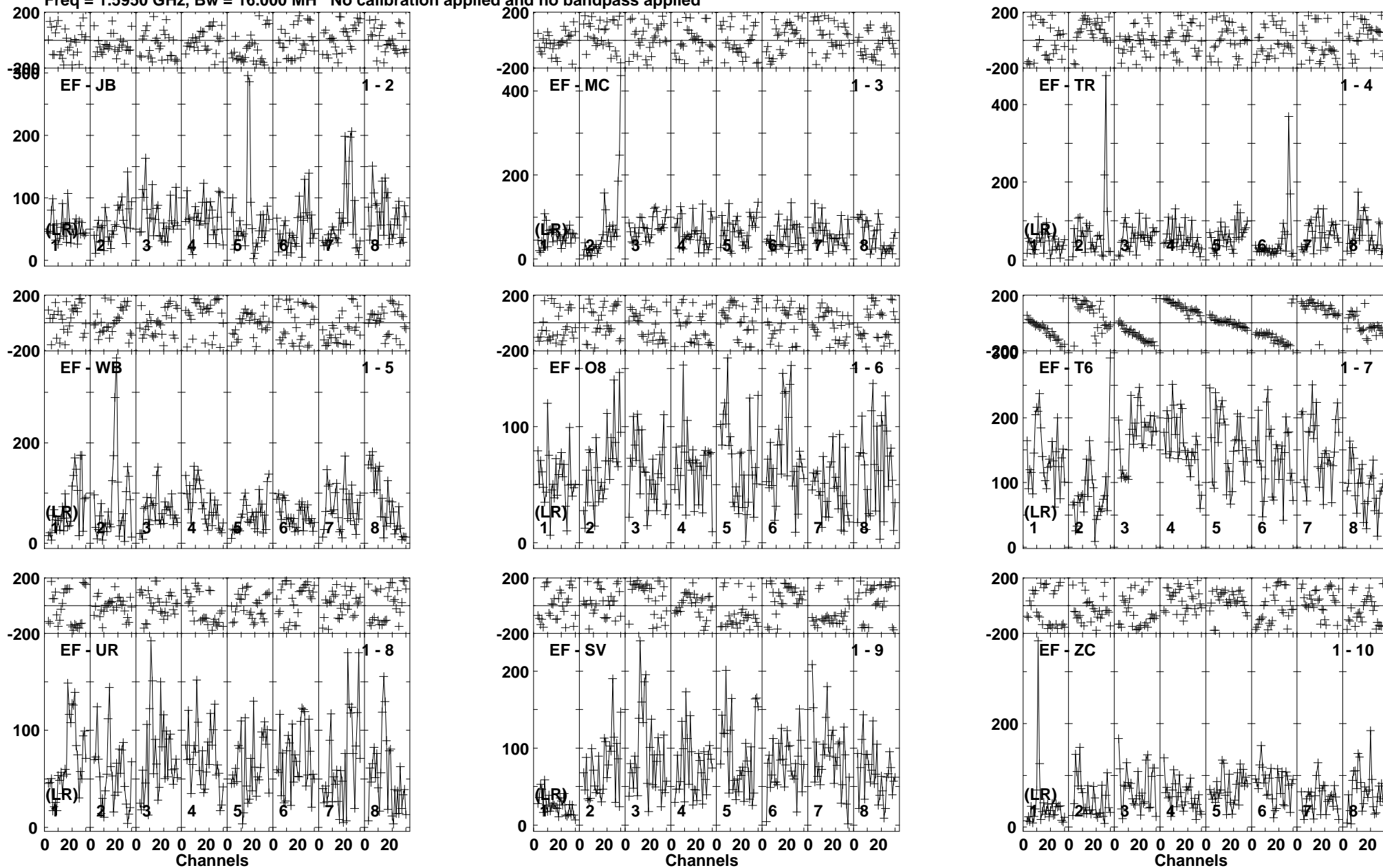
Lower frame: Micro Ampl Jy Top frame: Phas deg Vector averaged cross-power spectrum Baseline: EF (01) - JB (02) Timerange: 00/14:14:07 to 00/14:18:59
