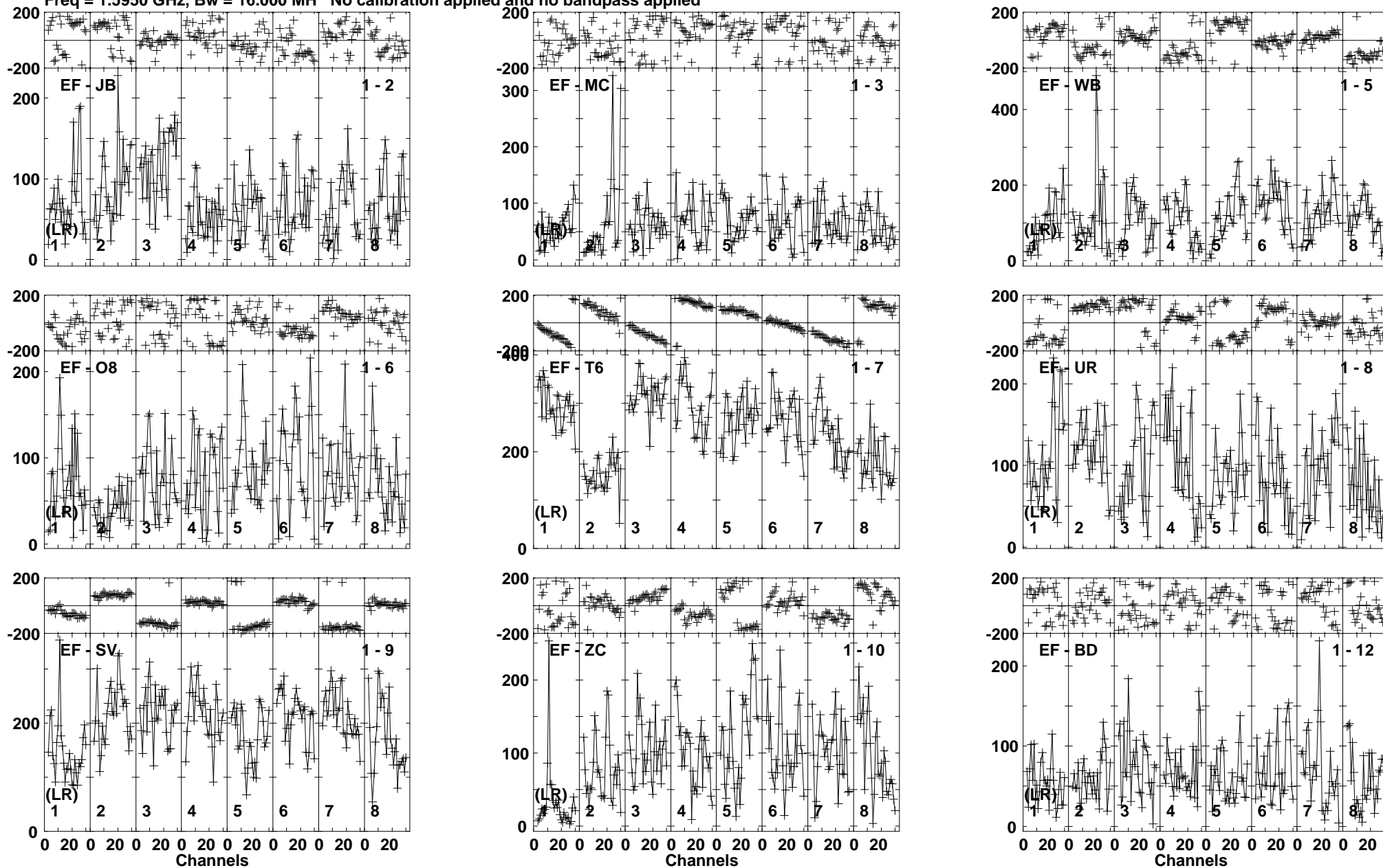
Lower frame: Micro Ampl Jy Top frame: Phas deg Vector averaged cross-power spectrum Baseline: EF (01) - JB (02) Timerange: 00/20:53:59 to 00/20:58:49
