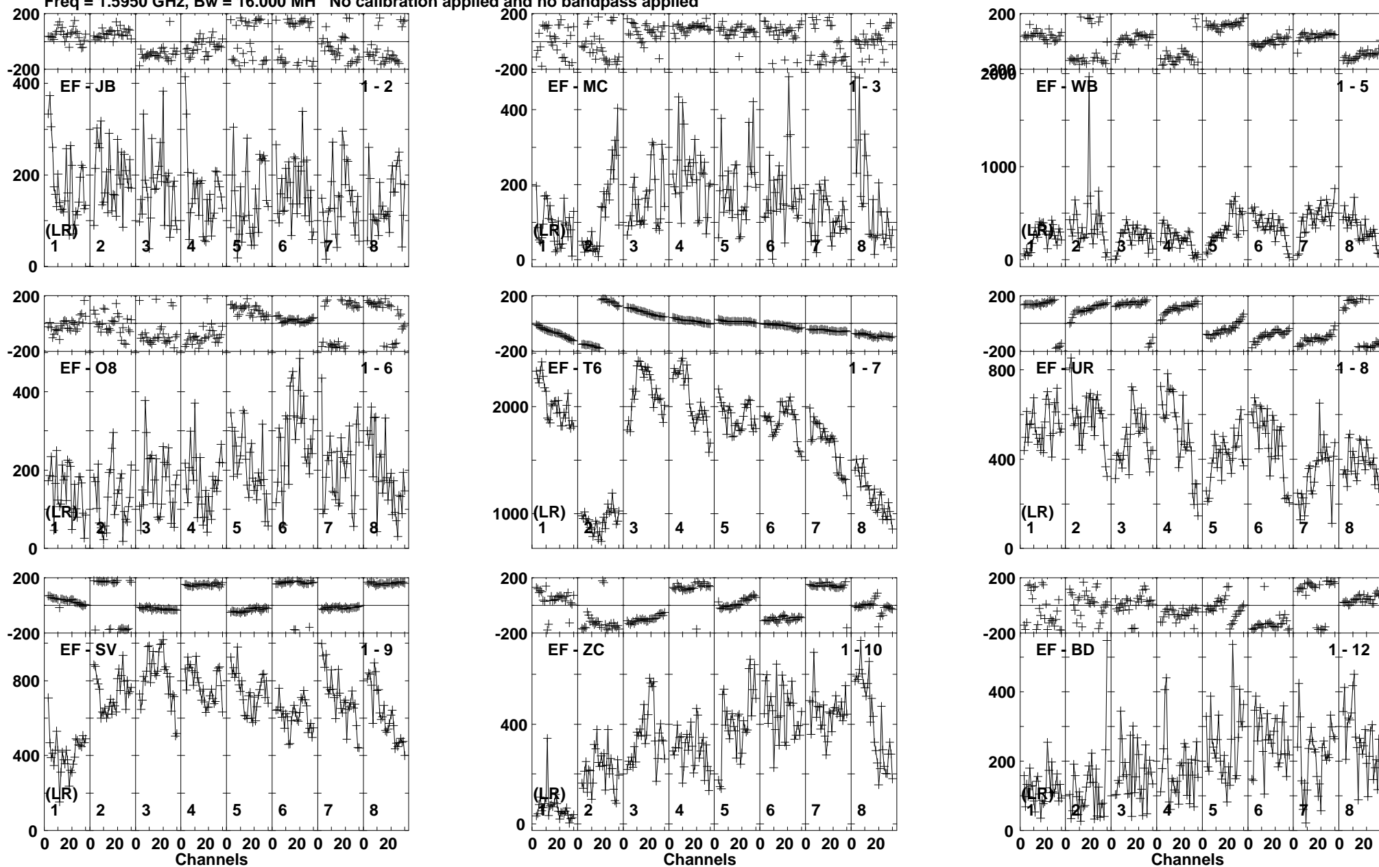
Lower frame: Micro Ampl Jy Top frame: Phas deg Vector averaged cross-power spectrum Baseline: EF (01) - JB (02) Timerange: 00/22:23:31 to 00/22:24:49
