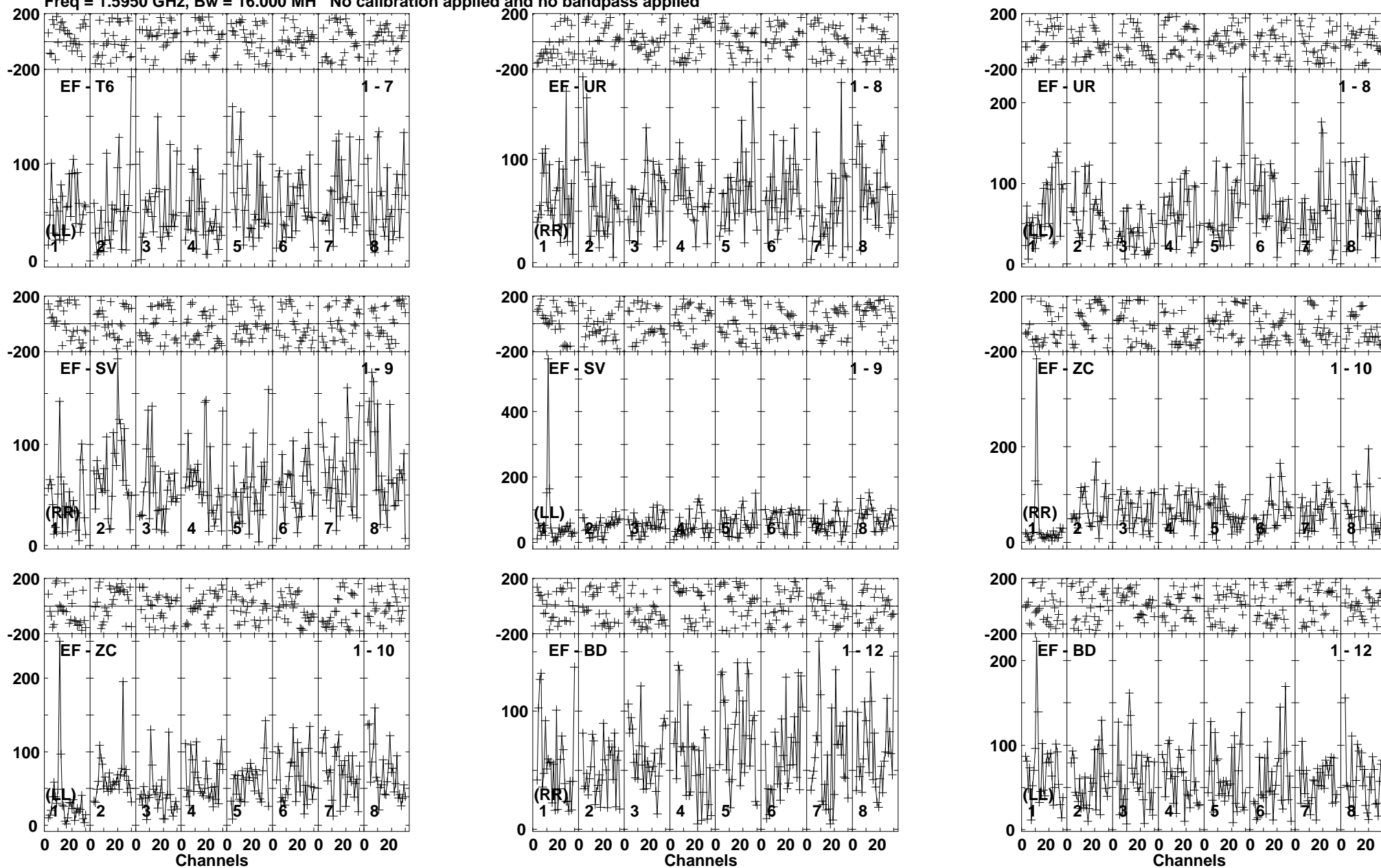
Lower frame: Micro Ampl Jy Top frame: Phas deg Vector averaged cross-power spectrum Baseline: EF (01) - T6 (07) Timerange: 00/21:14:59 to 00/21:19:49
