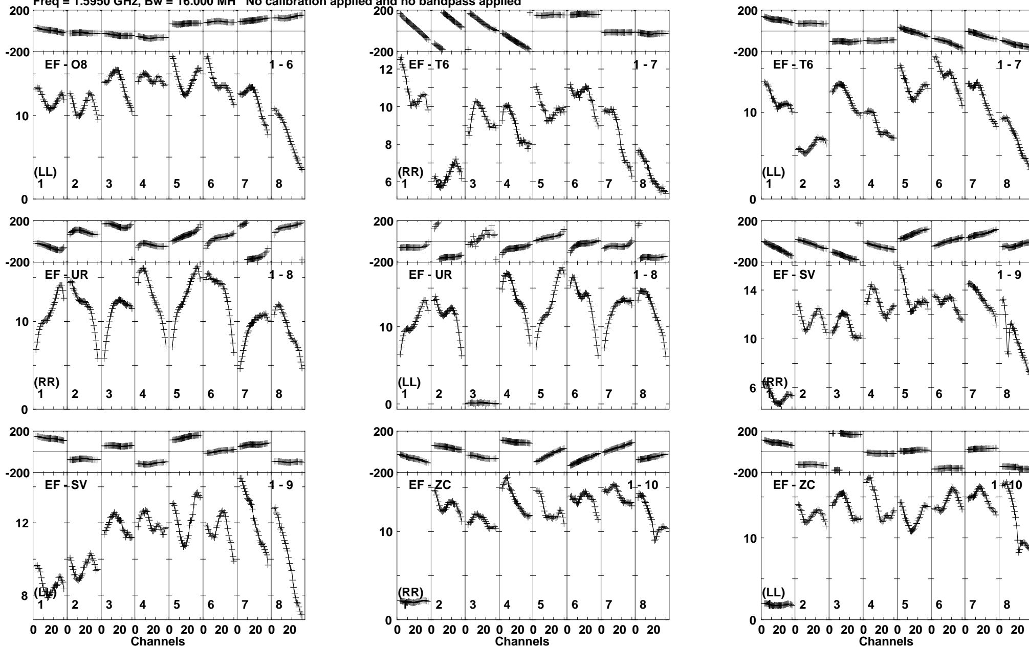
Lower frame: Milli Ampl Jy Top frame: Phas deg Vector averaged cross-power spectrum Baseline: EF (01) - O8 (06) Timerange: 00/17:06:01 to 00/17:07:19
