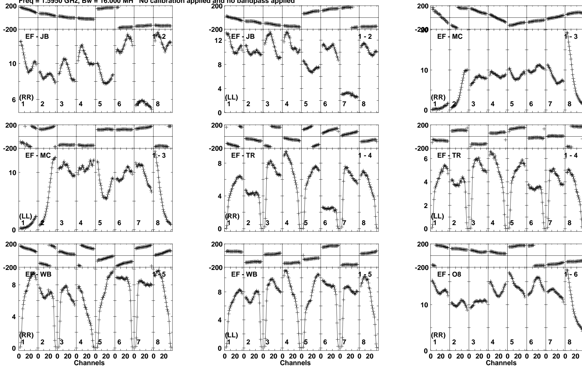
Lower frame: Milli Ampl Jy Top frame: Phas deg Vector averaged cross-power spectrum Baseline: EF (01) - JB (02) Timerange: 00:17:34:01 to 00:17:35:19
