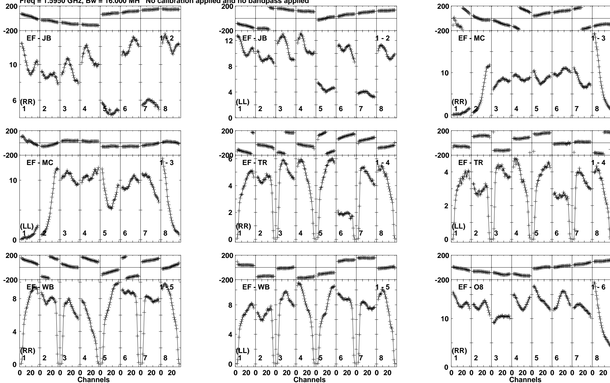
Lower frame: Milli Ampl Jy Top frame: Phas deg Vector averaged cross-power spectrum Baseline: EF (01) - JB (02) Timerange: 00/16:52:01 to 00/16:53:19
