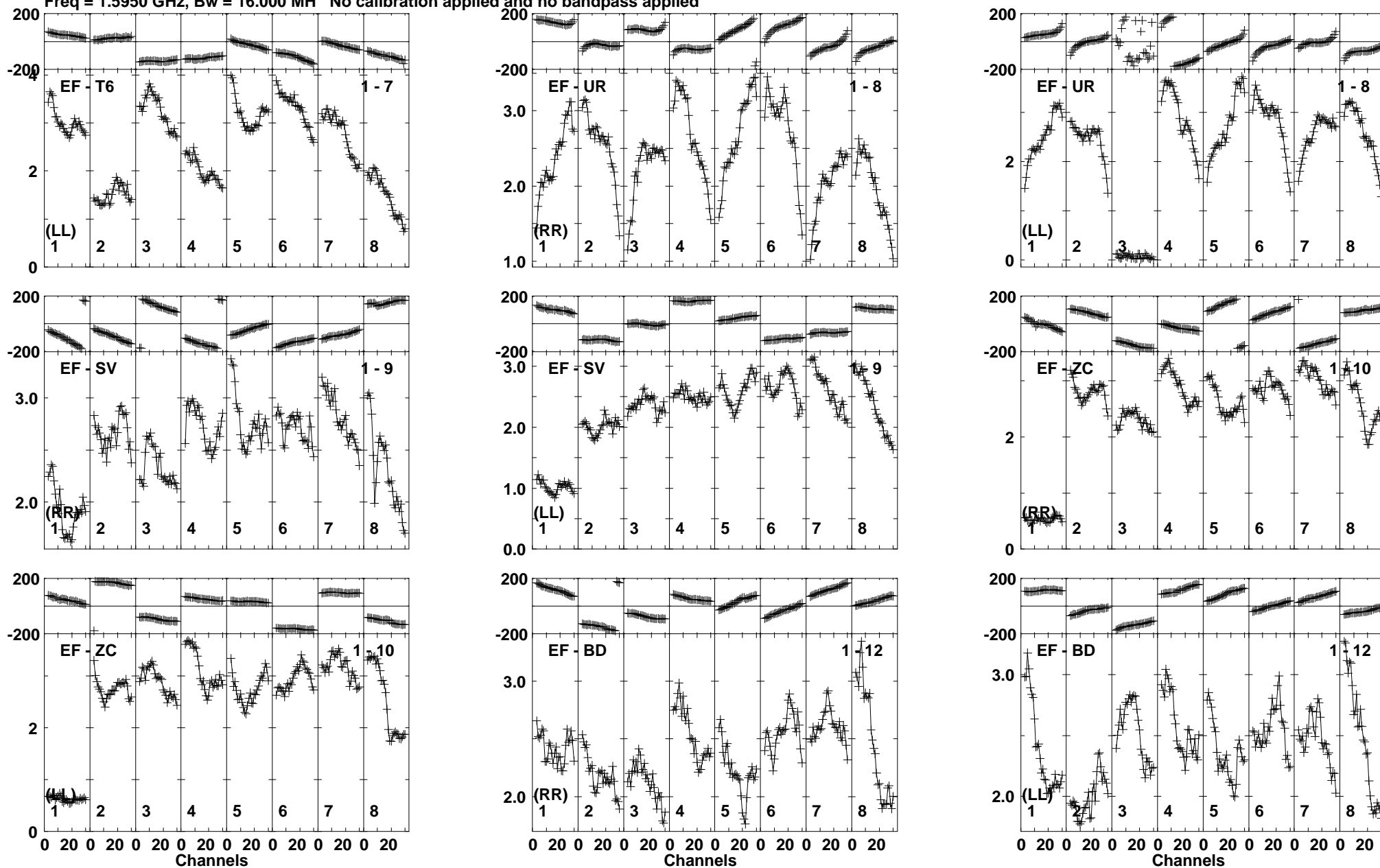
Lower frame: Milli Ampl Jy Top frame: Phas deg Vector averaged cross-power spectrum Baseline: EF (01) - T6 (07) Timerange: 00/21:33:59 to 00/21:35:49
