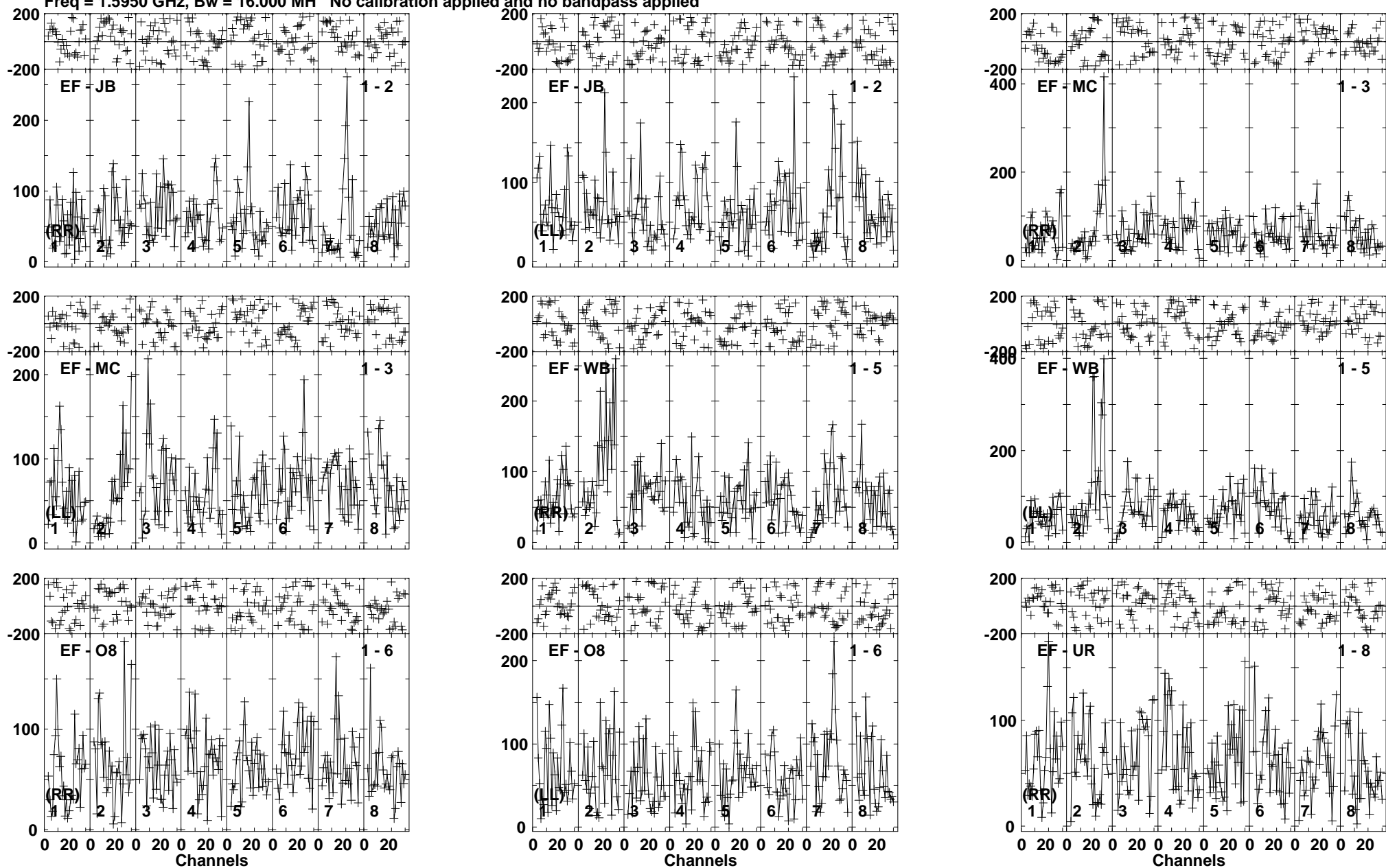
Lower frame: Micro Ampl Jy Top frame: Phas deg Vector averaged cross-power spectrum Baseline: EF (01) - JB (02) Timerange: 00/18:24:31 to 00/18:29:19
