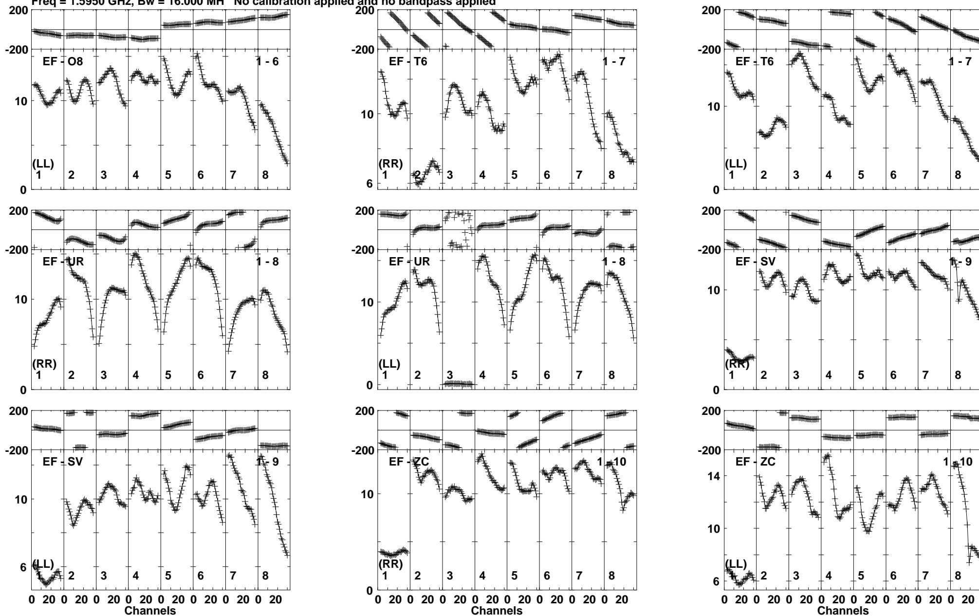
Lower frame: Milli Ampl Jy Top frame: Phas deg Vector averaged cross-power spectrum Baseline: EF (01) - O8 (06) Timerange: 00/14:40:19 to 00/14:42:09
