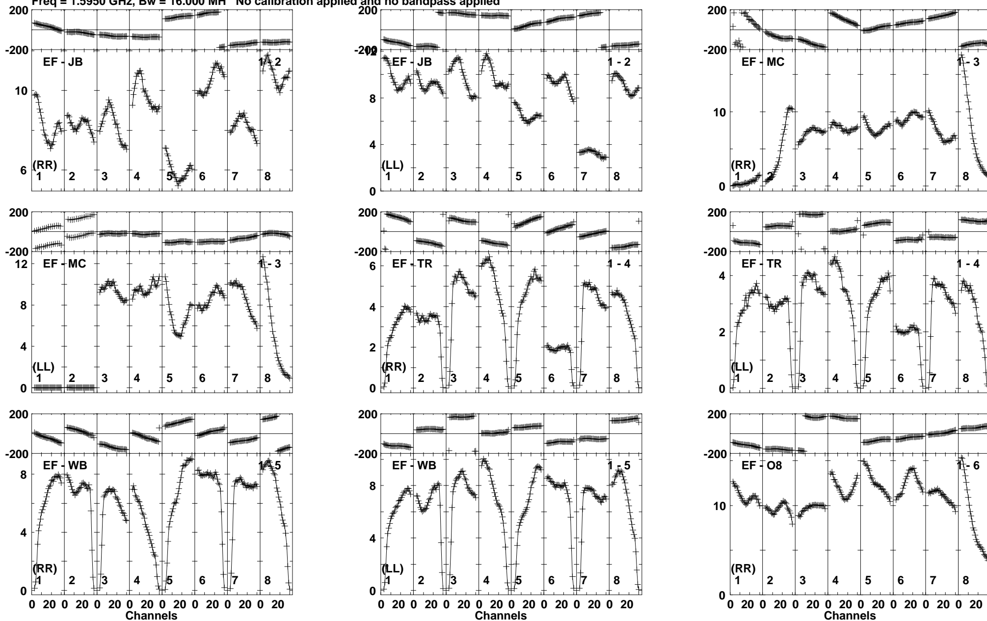
Lower frame: Milli Ampl Jy Top frame: Phas deg Vector averaged cross-power spectrum Baseline: EF (01) - JB (02) Timerange: 00/15:08:31 to 00/15:10:19
