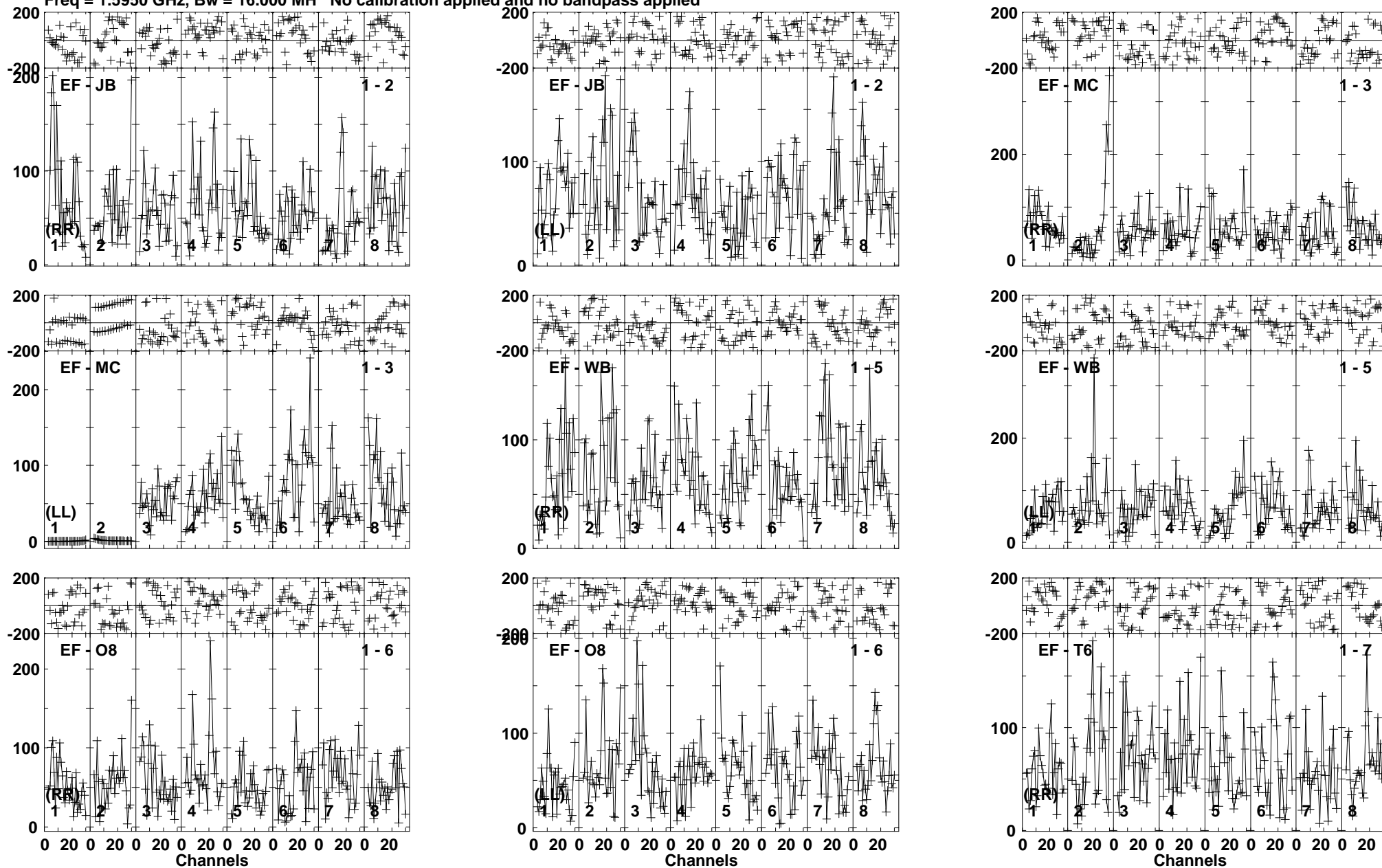
Lower frame: Micro Ampl Jy Top frame: Phas deg Vector averaged cross-power spectrum Baseline: EF (01) - JB (02) Timerange: 00/20:25:59 to 00/20:30:49
