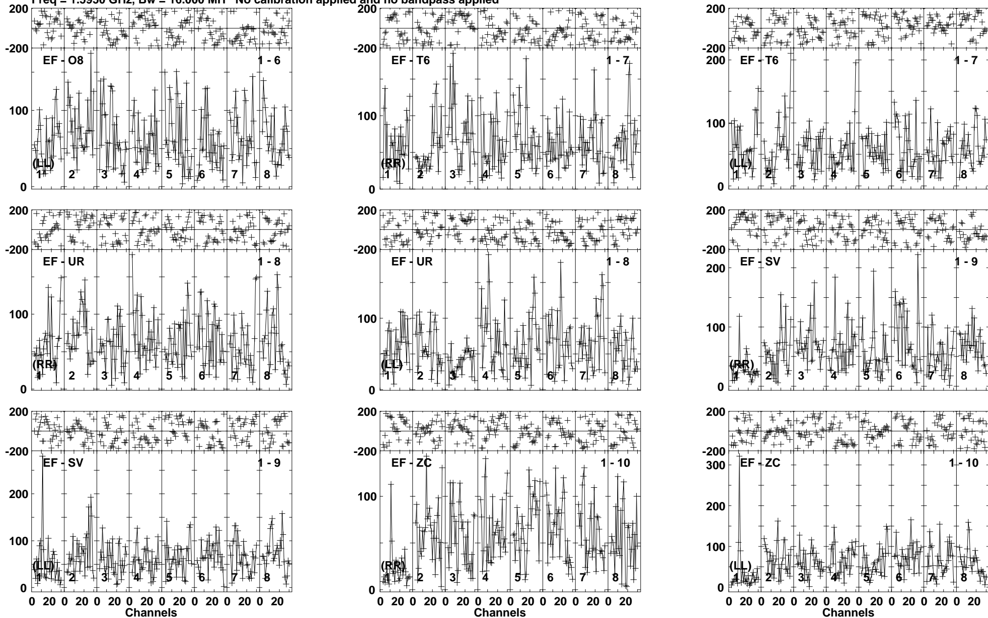
Lower frame: Micro Ampl Jy Top frame: Phas deg Vector averaged cross-power spectrum Baseline: EF (01) - O8 (06) Timerange: 00/16:11:31 to 00/16:16:19
