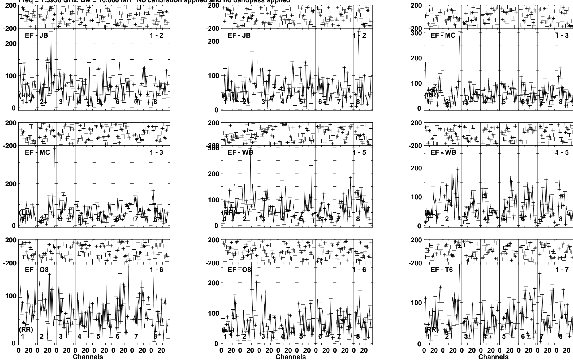
Lower frame: Micro Ampl Jy Top frame: Phas deg Vector averaged cross-power spectrum Baseline: EF (01) - JB (02) Timerange: 00/23:07:59 to 00/23:12:49
