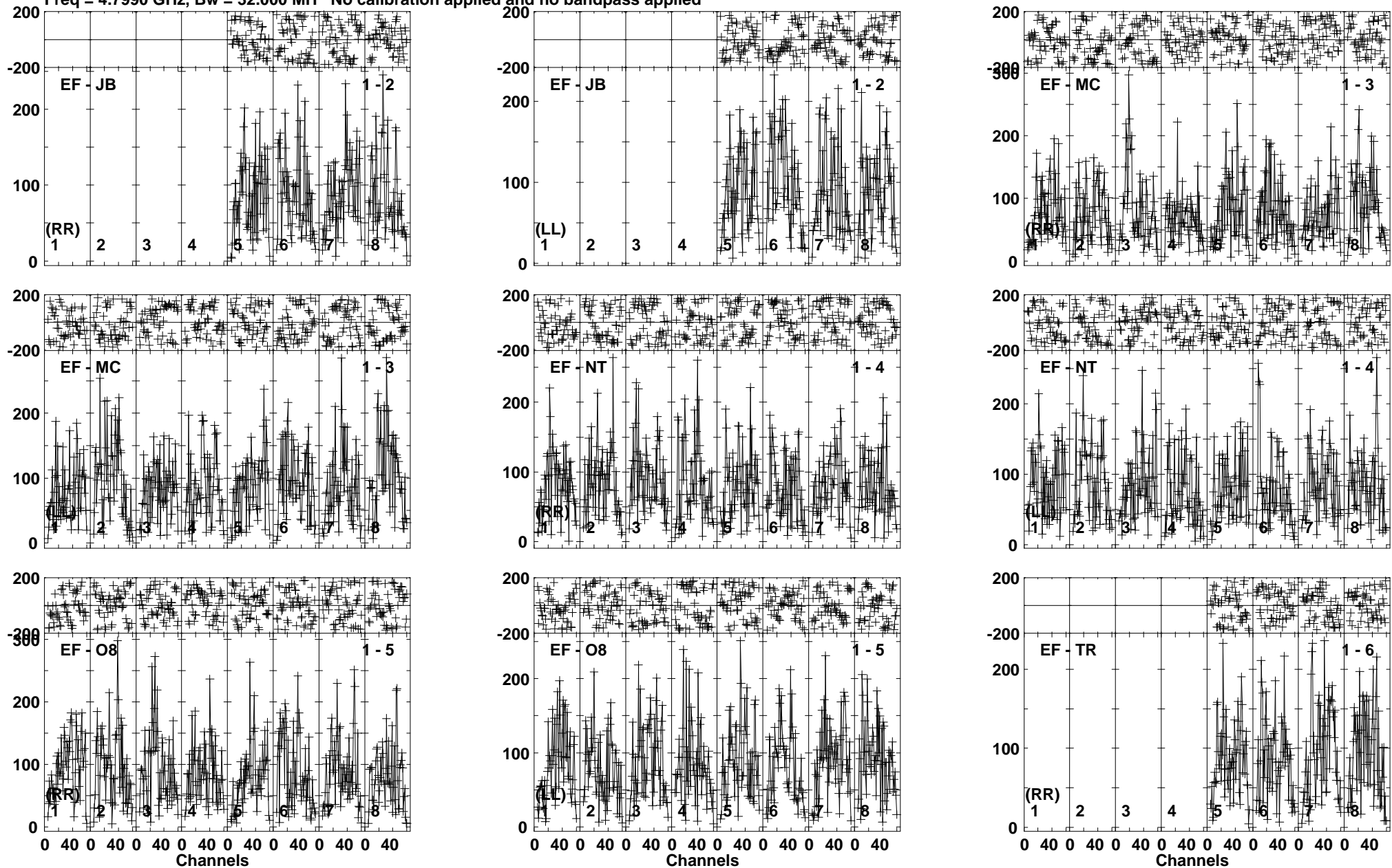
Lower frame: Micro Ampl Jy Top frame: Phas deg Vector averaged cross-power spectrum Baseline: EF (01) - JB (02) Timerange: 00/23:14:50 to 00/23:18:19
