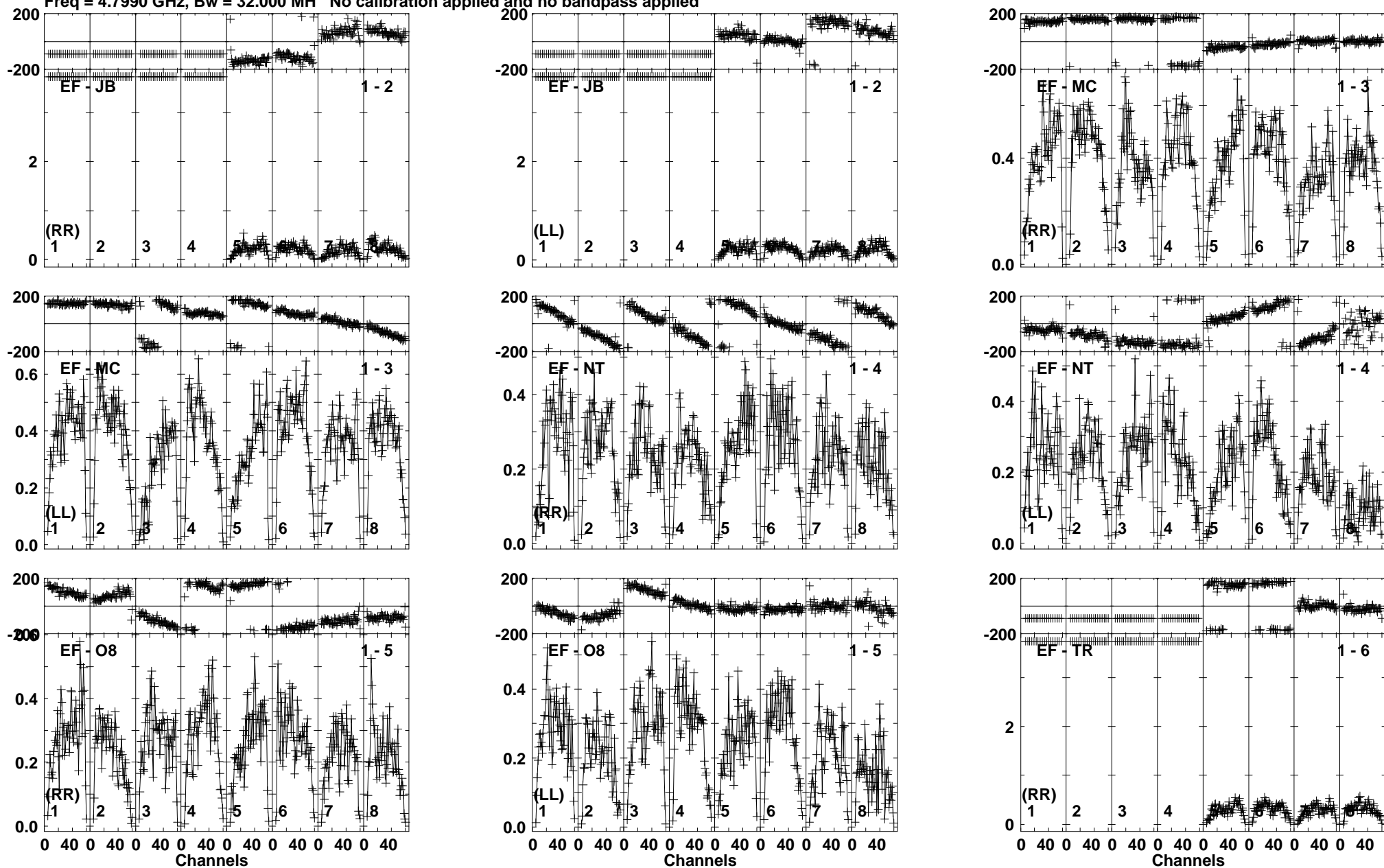
Lower frame: Milli Ampl Jy Top frame: Phas deg Vector averaged cross-power spectrum Baseline: EF (01) - JB (02) Timerange: 01/00:00:40 to 01/00:04:09
