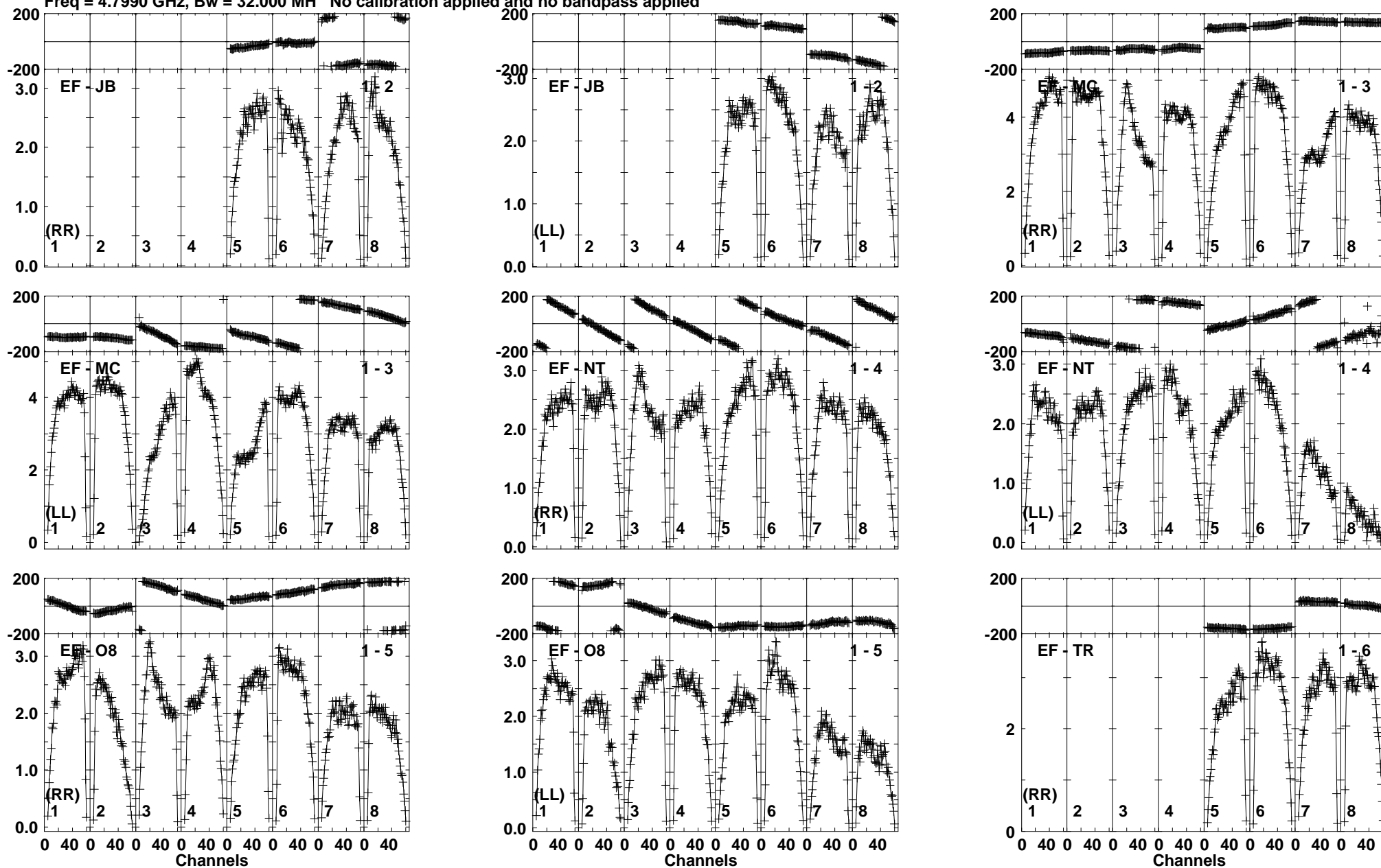
Lower frame: Milli Ampl Jy Top frame: Phas deg Vector averaged cross-power spectrum Baseline: EF (01) - JB (02) Timerange: 00:22:32:40 to 00:22:34:09
