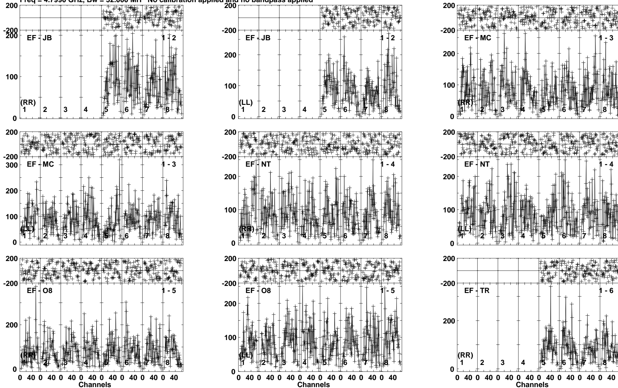
Lower frame: Micro Ampl Jy Top frame: Phas deg Vector averaged cross-power spectrum Baseline: EF (01) - JB (02) Timerange: 00/21:18:00 to 00/21:21:29
