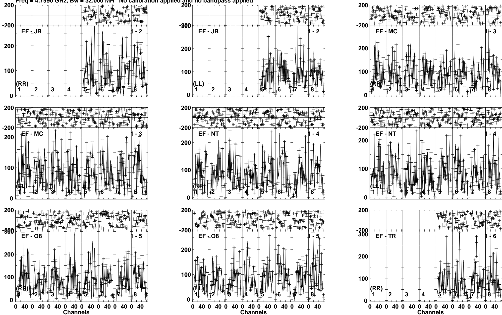
Lower frame: Micro Ampl Jy Top frame: Phas deg Vector averaged cross-power spectrum Baseline: EF (01) - JB (02) Timerange: 01/00:10:50 to 01/00:14:19
