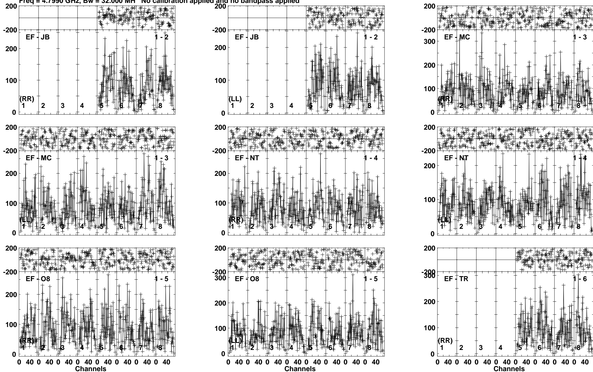
Lower frame: Micro Ampl Jy Top frame: Phas deg Vector averaged cross-power spectrum Baseline: EF (01) - JB (02) Timerange: 00/23:50:30 to 00/23:53:59
