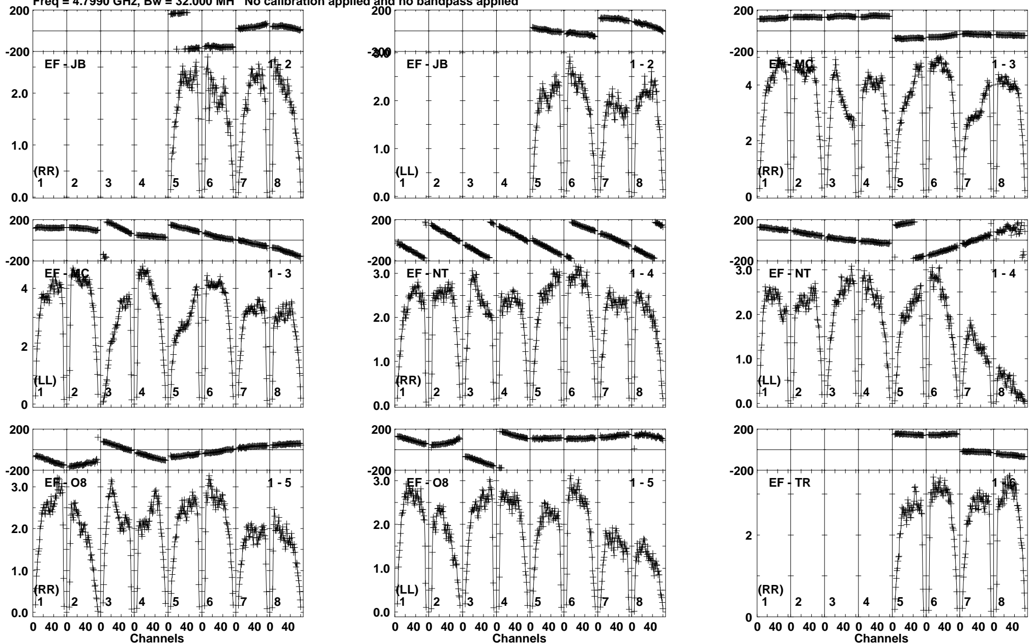
Lower frame: Milli Ampl Jy Top frame: Phas deg Vector averaged cross-power spectrum Baseline: EF (01) - JB (02) Timerange: 00/23:49:31 to 00/23:50:30
