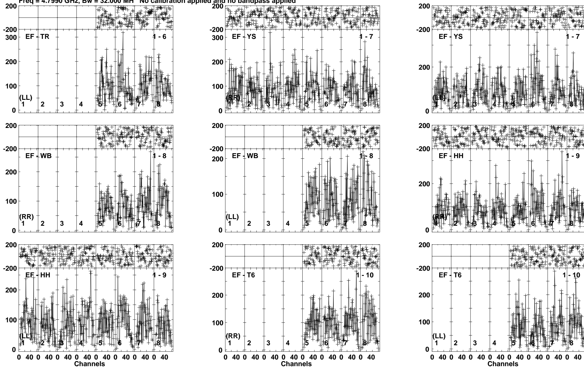
Lower frame: Micro Ampl Jy Top frame: Phas deg Vector averaged cross-power spectrum Baseline: EF (01) - TR (06) Timerange: 00/22:13:50 to 00/22:17:19
