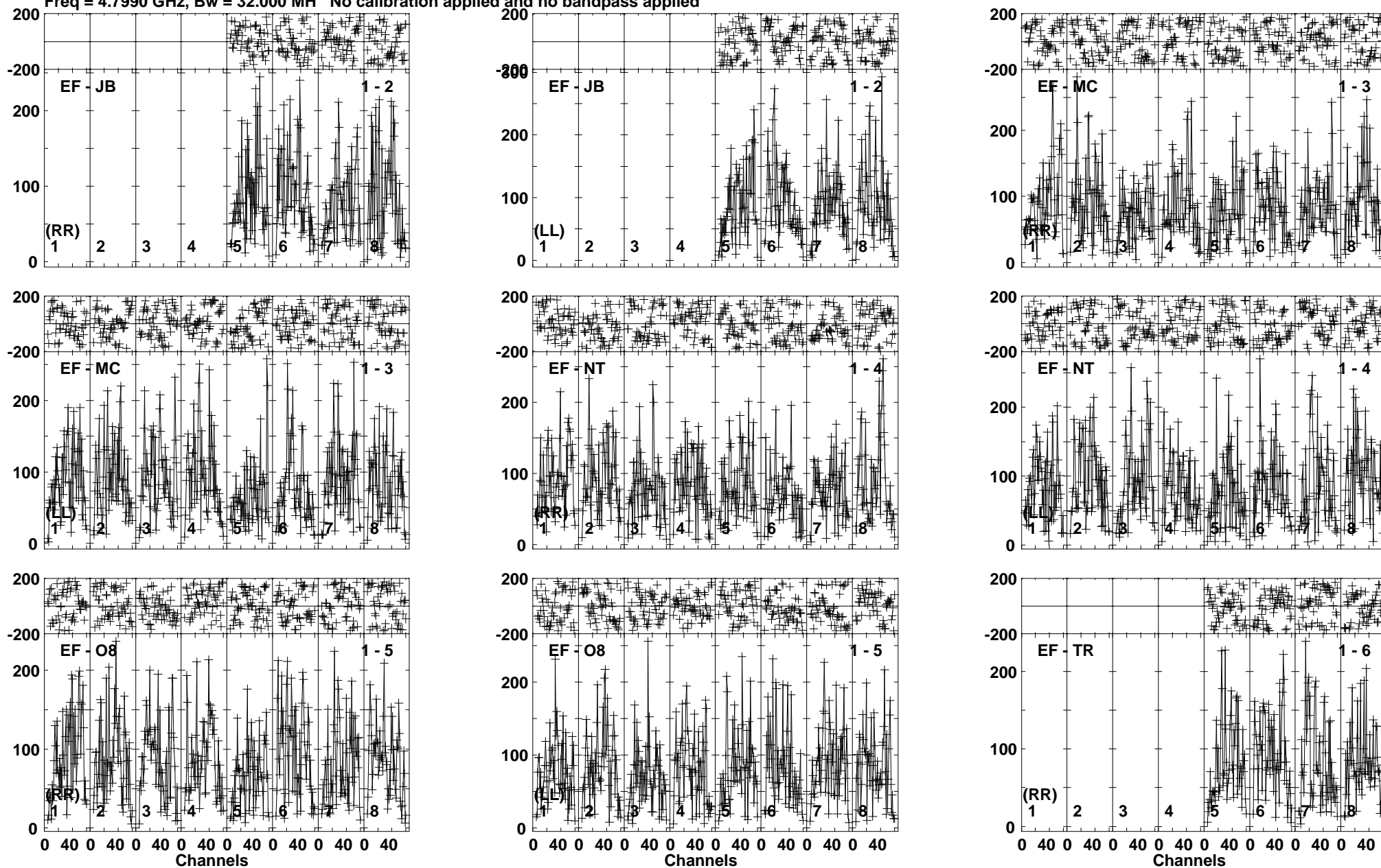
Lower frame: Micro Ampl Jy Top frame: Phas deg Vector averaged cross-power spectrum Baseline: EF (01) - JB (02) Timerange: 00/21:48:30 to 00/21:51:59
