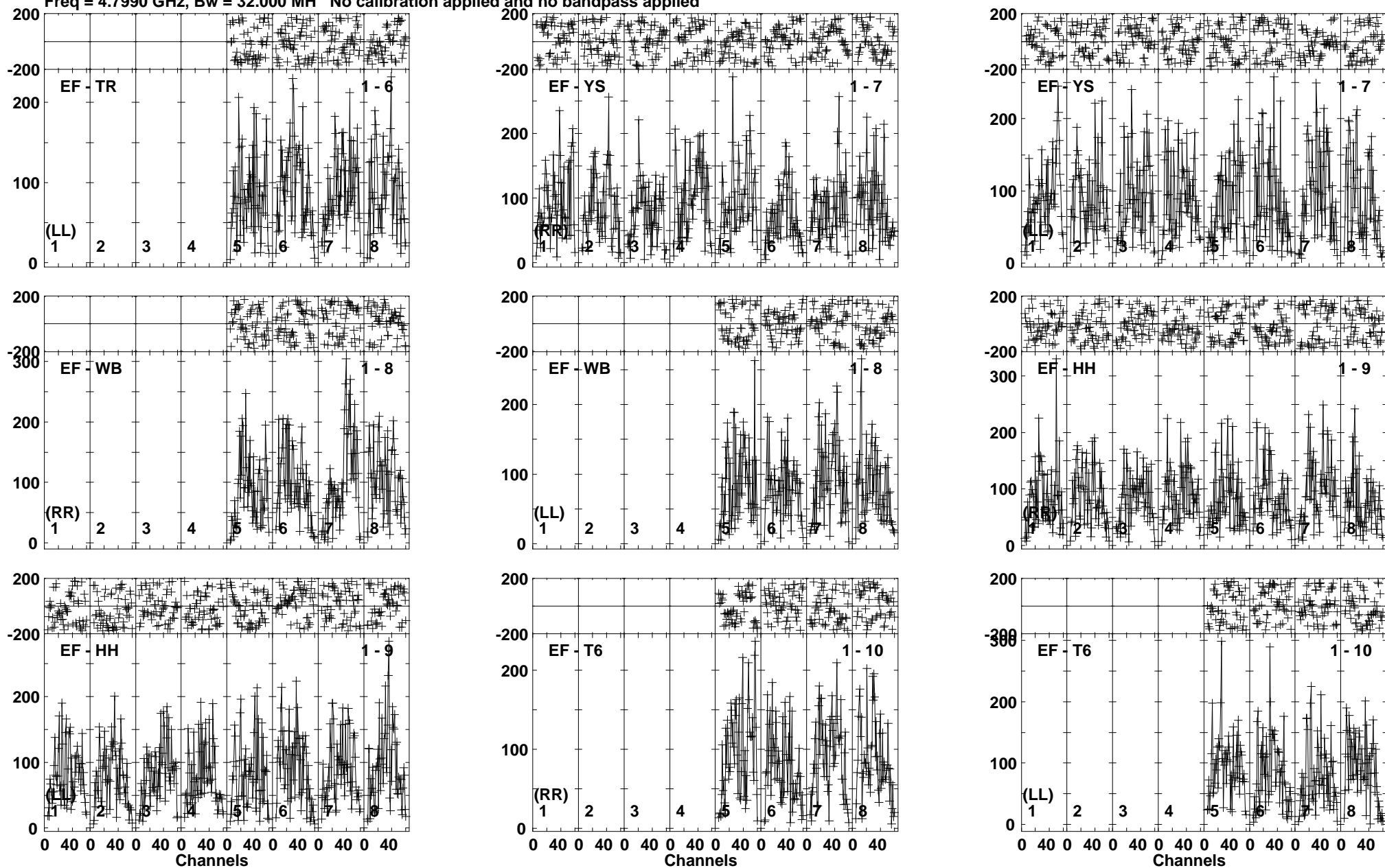
Lower frame: Micro Ampl Jy Top frame: Phas deg Vector averaged cross-power spectrum Baseline: EF (01) - TR (06) Timerange: 00/21:48:30 to 00/21:51:59
