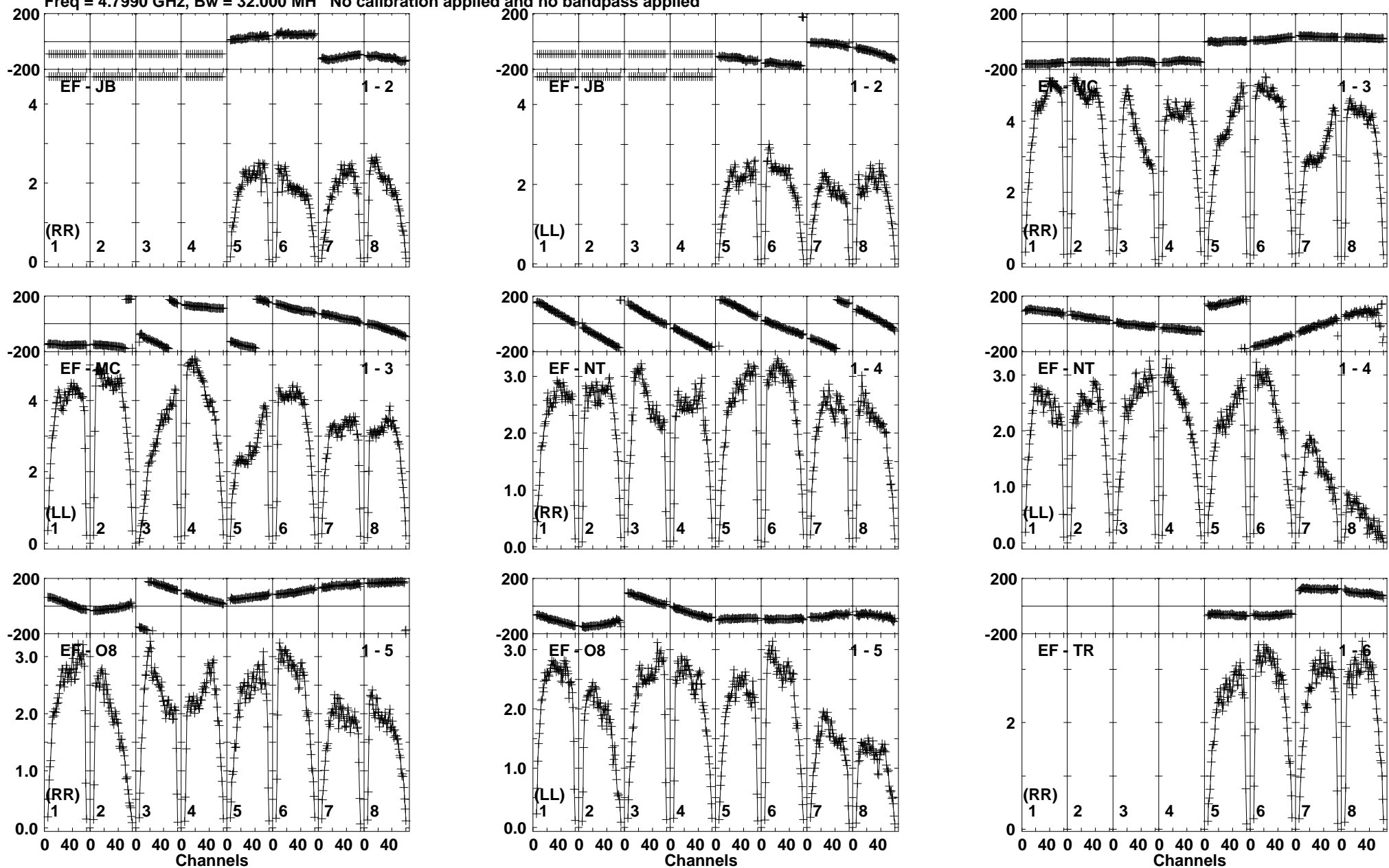
Lower frame: Milli Ampl Jy Top frame: Phas deg Vector averaged cross-power spectrum Baseline: EF (01) - JB (02) Timerange: 01/00:30:10 to 01/00:31:09
