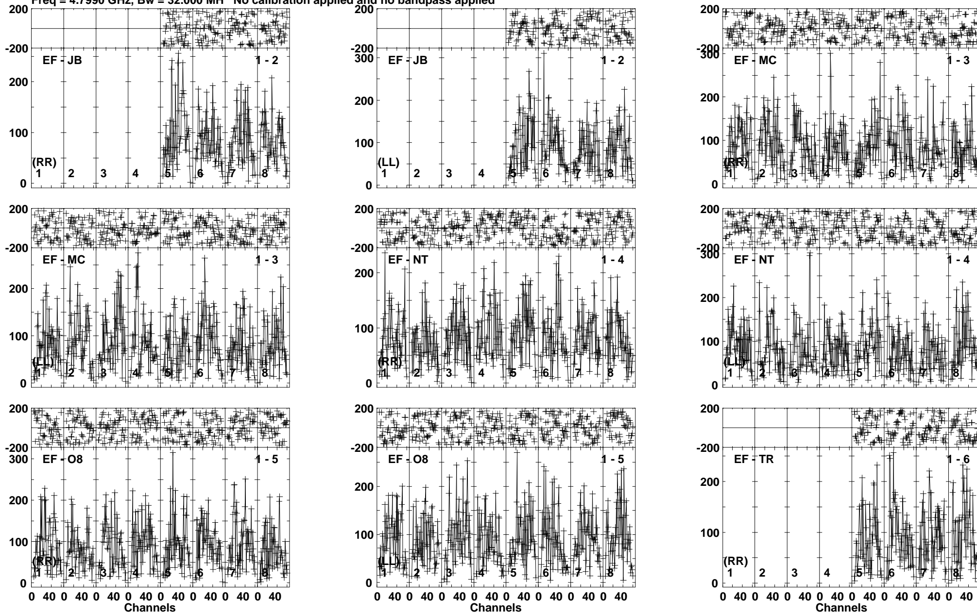
Lower frame: Micro Ampl Jy Top frame: Phas deg Vector averaged cross-power spectrum Baseline: EF (01) - JB (02) Timerange: 00/21:38:21 to 00/21:41:50
