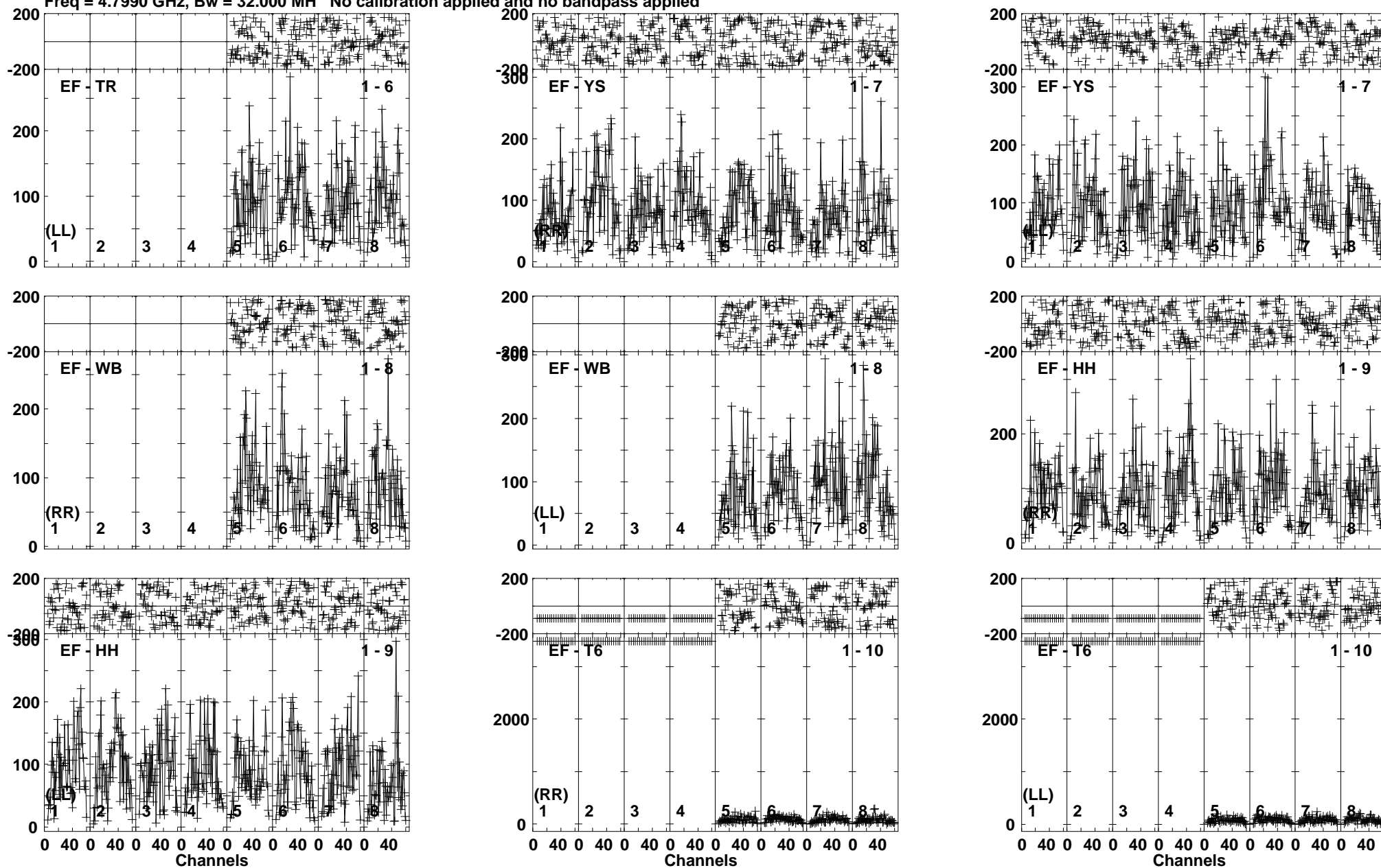
Lower frame: Micro Ampl Jy Top frame: Phas deg Vector averaged cross-power spectrum Baseline: EF (01) - TR (06) Timerange: 00/21:07:51 to 00/21:11:20
