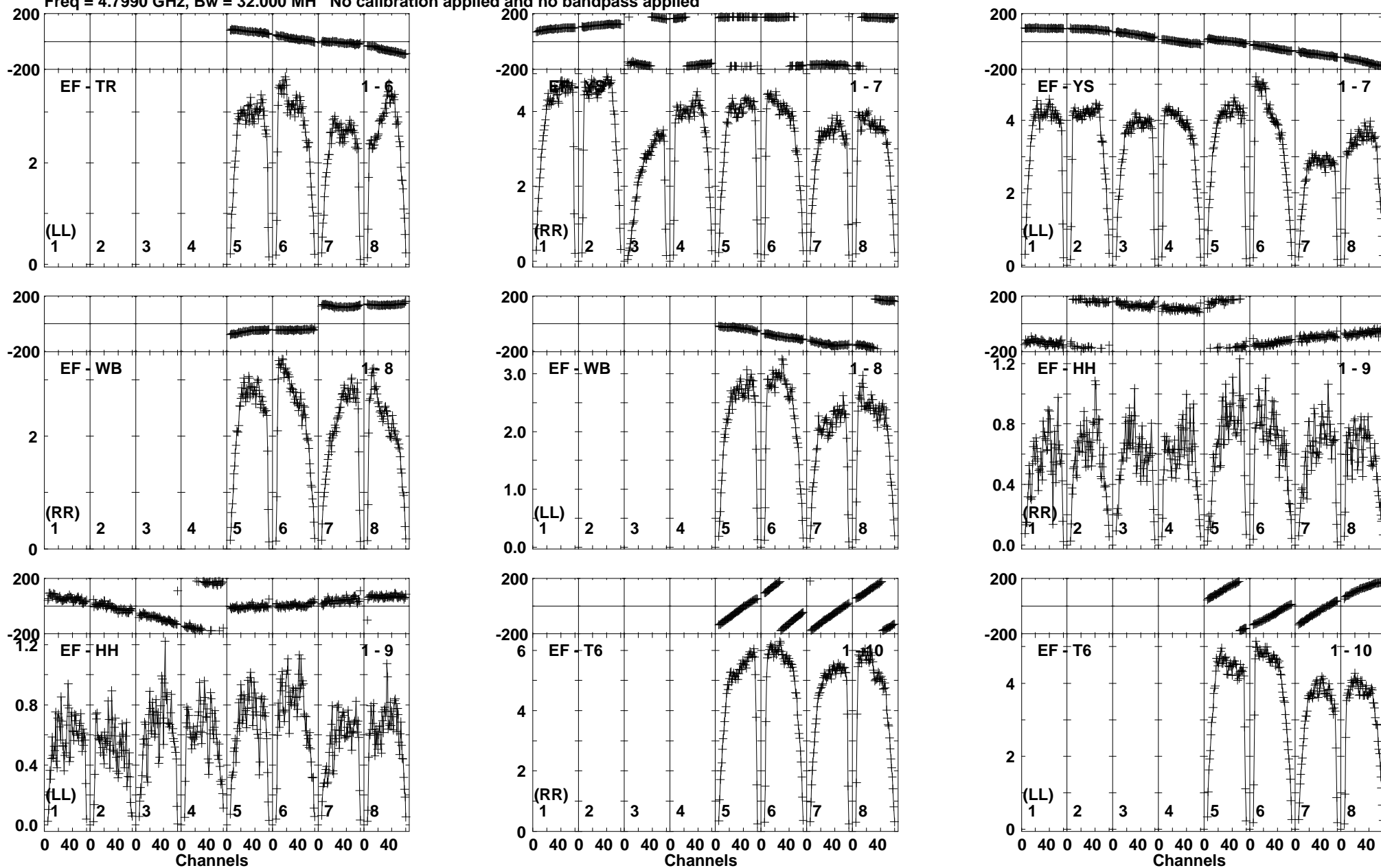
Lower frame: Milli Ampl Jy Top frame: Phas deg Vector averaged cross-power spectrum Baseline: EF (01) - TR (06) Timerange: 00/23:39:21 to 00/23:40:20
