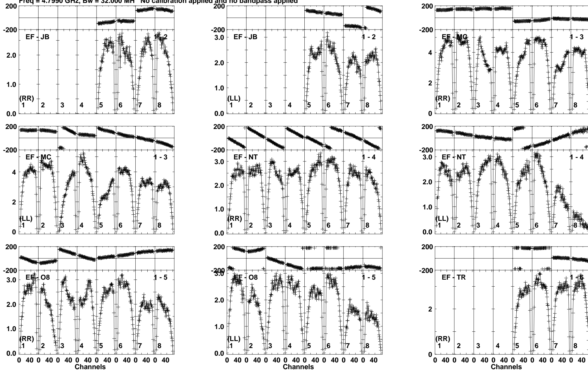
Lower frame: Milli Ampl Jy Top frame: Phas deg Vector averaged cross-power spectrum Baseline: EF (01) - JB (02) Timerange: 00/23:39:21 to 00/23:40:20
