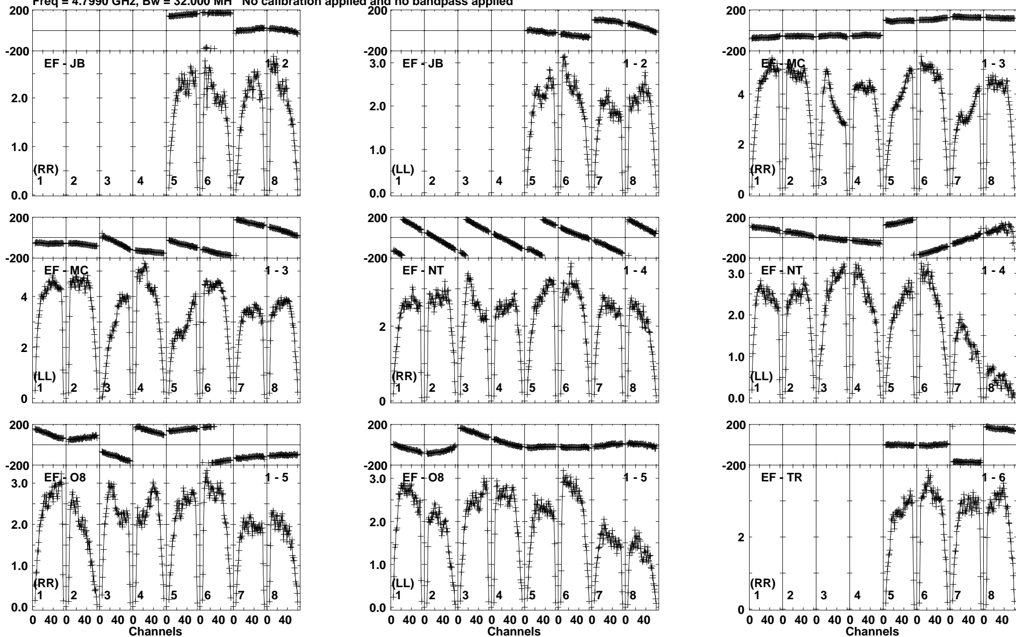
Lower frame: Milli Ampl Jy Top frame: Phas deg Vector averaged cross-power spectrum Baseline: EF (01) - JB (02) Timerange: 01/00:14:20 to 01/00:15:49
