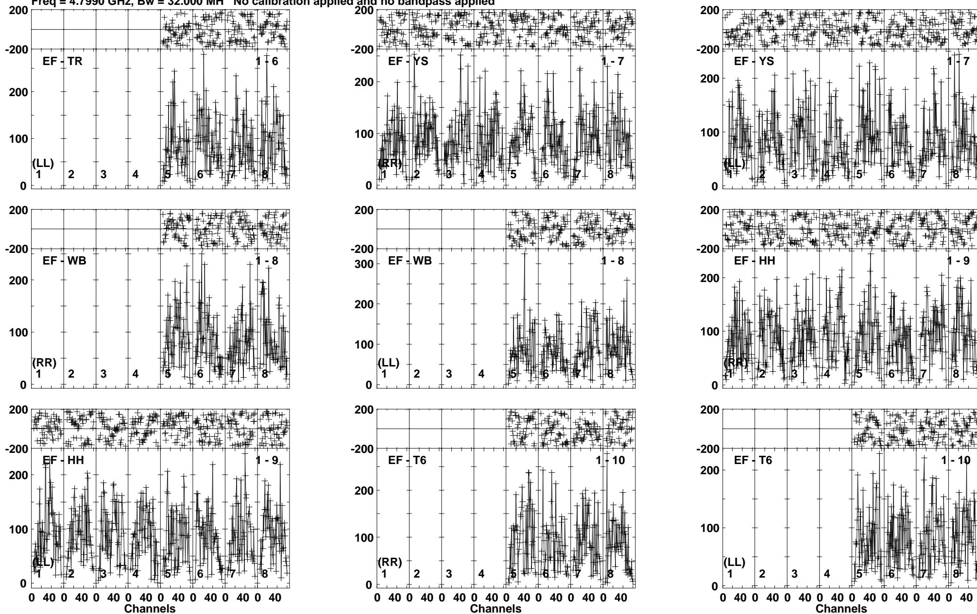
Lower frame: Micro Ampl Jy Top frame: Phas deg Vector averaged cross-power spectrum Baseline: EF (01) - TR (06) Timerange: 00/21:33:11 to 00/21:36:40
