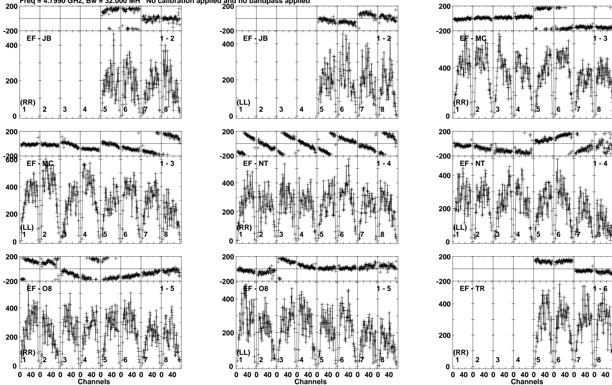
Lower frame: Micro Ampl Jy Top frame: Phas deg Vector averaged cross-power spectrum Baseline: EF (01) - JB (02) Timerange: 00/23:30:11 to 00/23:33:40
