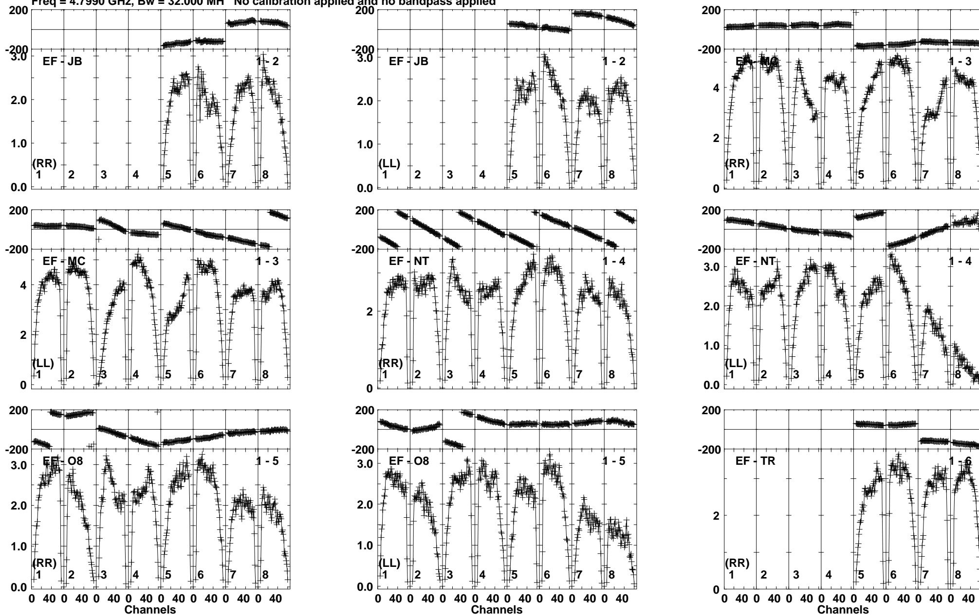
Lower frame: Milli Ampl Jy Top frame: Phas deg Vector averaged cross-power spectrum Baseline: EF (01) - JB (02) Timerange: 00/23:59:40 to 01/00:00:39
