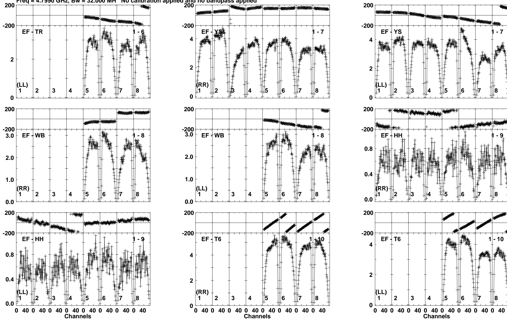
Lower frame: Milli Ampl Jy Top frame: Phas deg Vector averaged cross-power spectrum Baseline: EF (01) - TR (06) Timerange: 00/23:54:00 to 00/23:55:30
