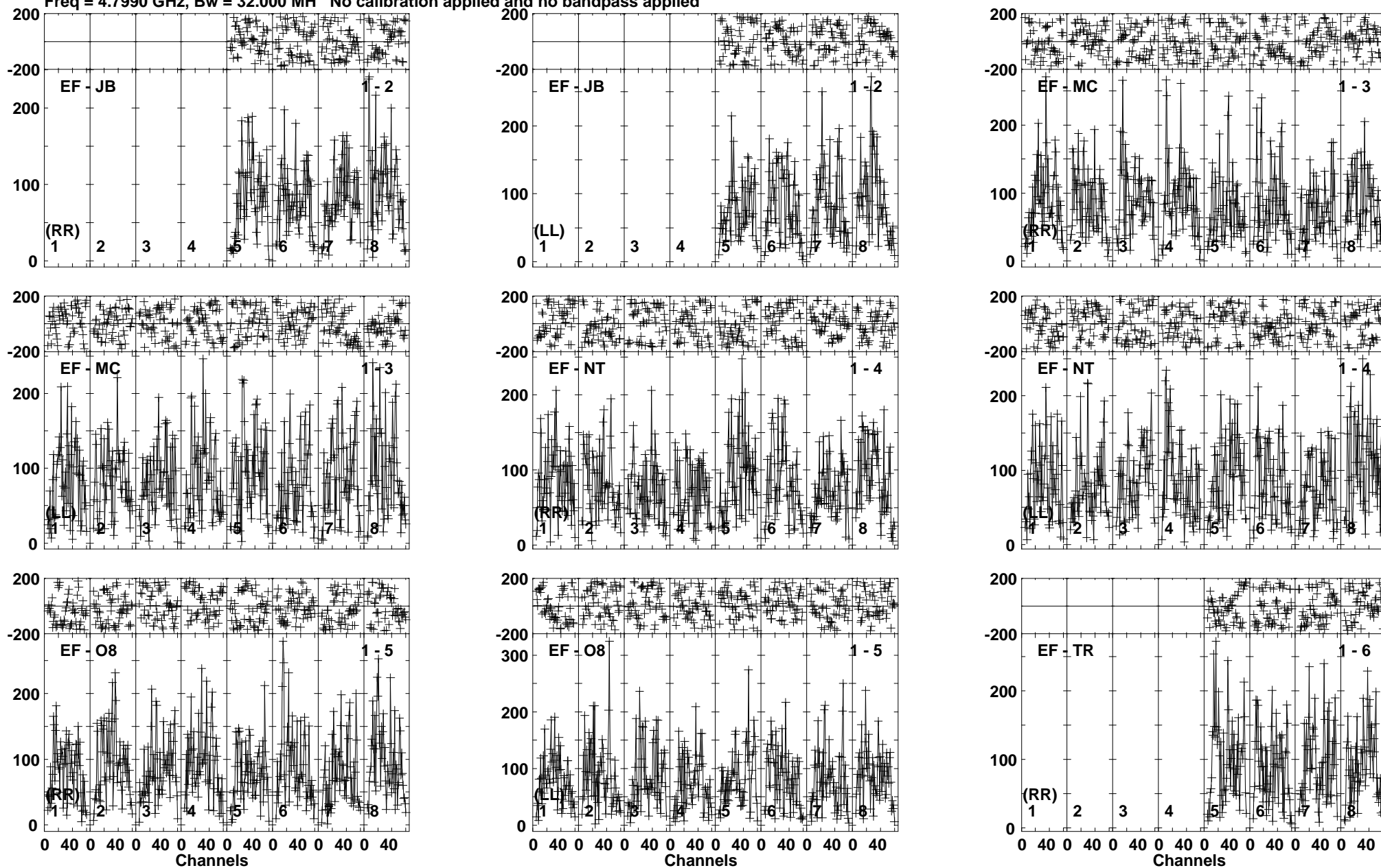
Lower frame: Micro Ampl Jy Top frame: Phas deg Vector averaged cross-power spectrum Baseline: EF (01) - JB (02) Timerange: 00/23:35:11 to 00/23:38:40
