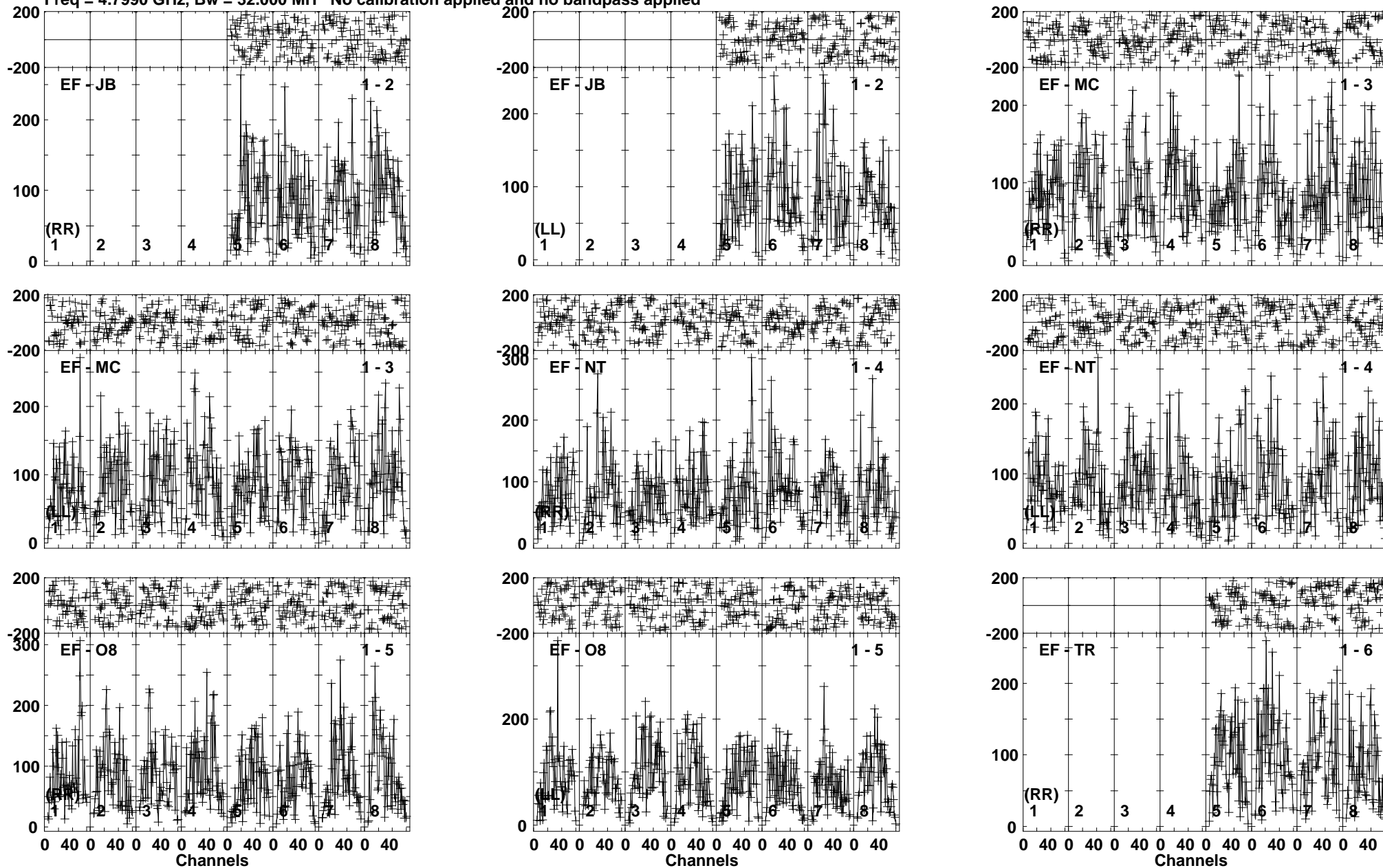
Lower frame: Micro Ampl Jy Top frame: Phas deg Vector averaged cross-power spectrum Baseline: EF (01) - JB (02) Timerange: 00/22:08:51 to 00/22:12:20
