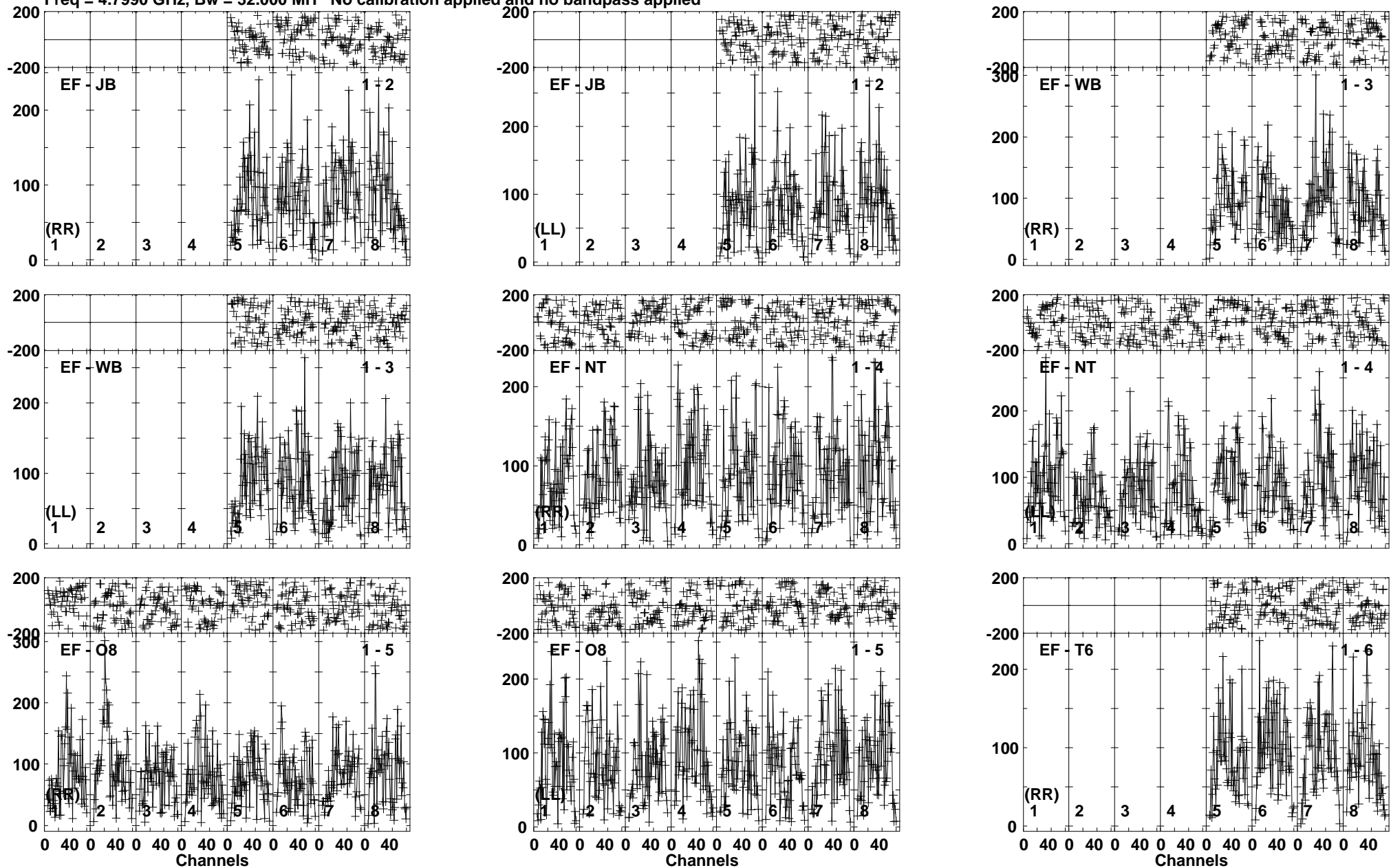
Lower frame: Micro Ampl Jy Top frame: Phas deg Vector averaged cross-power spectrum Baseline: EF (01) - JB (02) Timerange: 00/07:46:59 to 00/07:50:28
