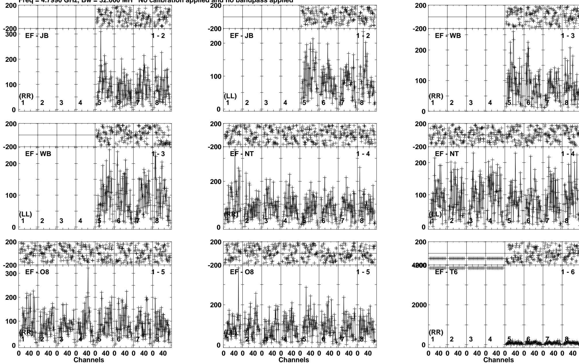
Lower frame: Micro Ampl Jy Top frame: Phas deg Vector averaged cross-power spectrum Baseline: EF (01) - JB (02) Timerange: 00/08:32:49 to 00/08:36:18
