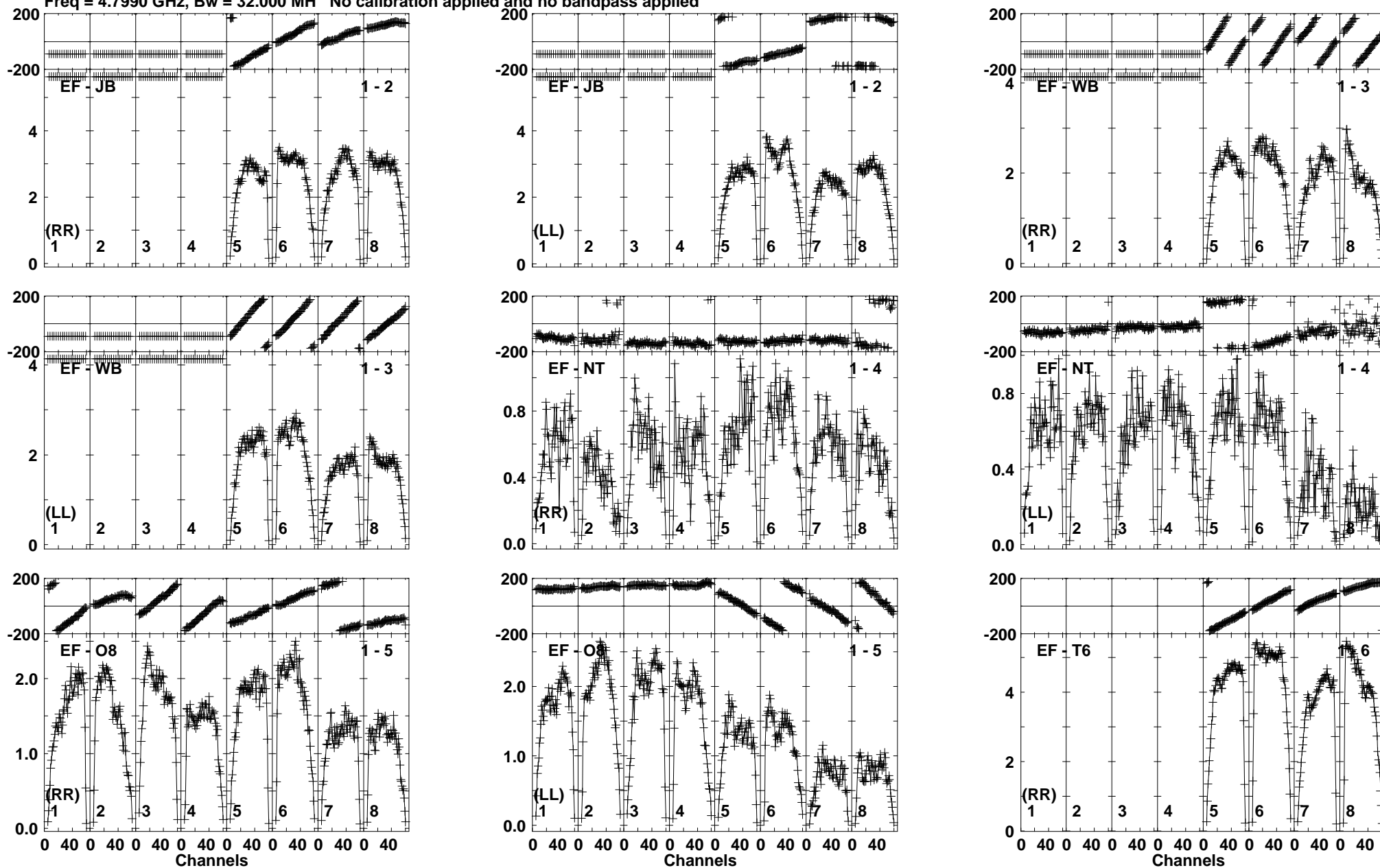
Lower frame: Milli Ampl Jy Top frame: Phas deg Vector averaged cross-power spectrum Baseline: EF (01) - JB (02) Timerange: 00/08:46:30 to 00/08:47:59
