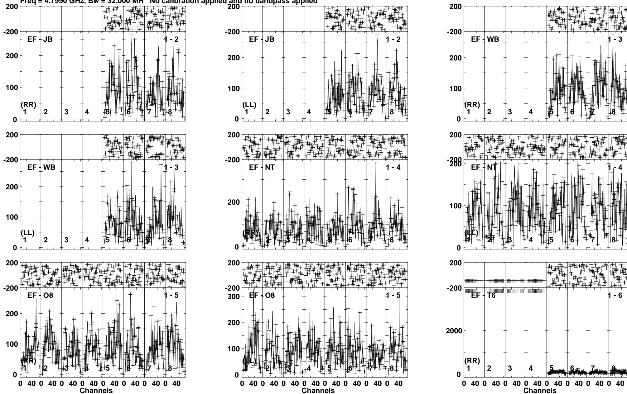
Lower frame: Micro Ampl Jy Top frame: Phas deg Vector averaged cross-power spectrum Baseline: EF (01) - JB (02) Timerange: 00/07:52:09 to 00/07:55:38
