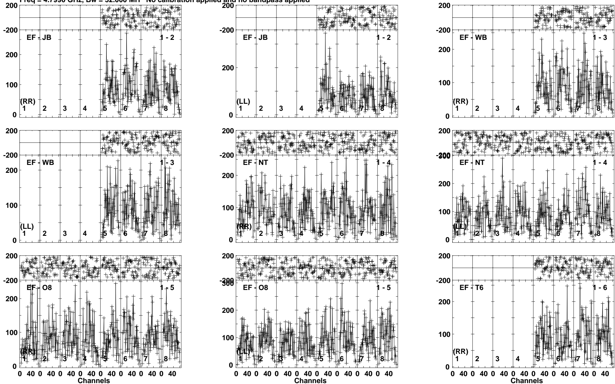
Lower frame: Micro Ampl Jy Top frame: Phas deg Vector averaged cross-power spectrum Baseline: EF (01) - JB (02) Timerange: 00/08:48:00 to 00/08:51:29
