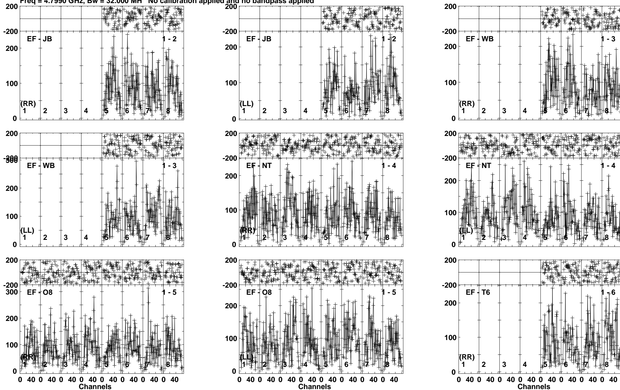
Lower frame: Micro Ampl Jy Top frame: Phas deg Vector averaged cross-power spectrum Baseline: EF (01) - JB (02) Timerange: 00/09:18:29 to 00/09:21:59
