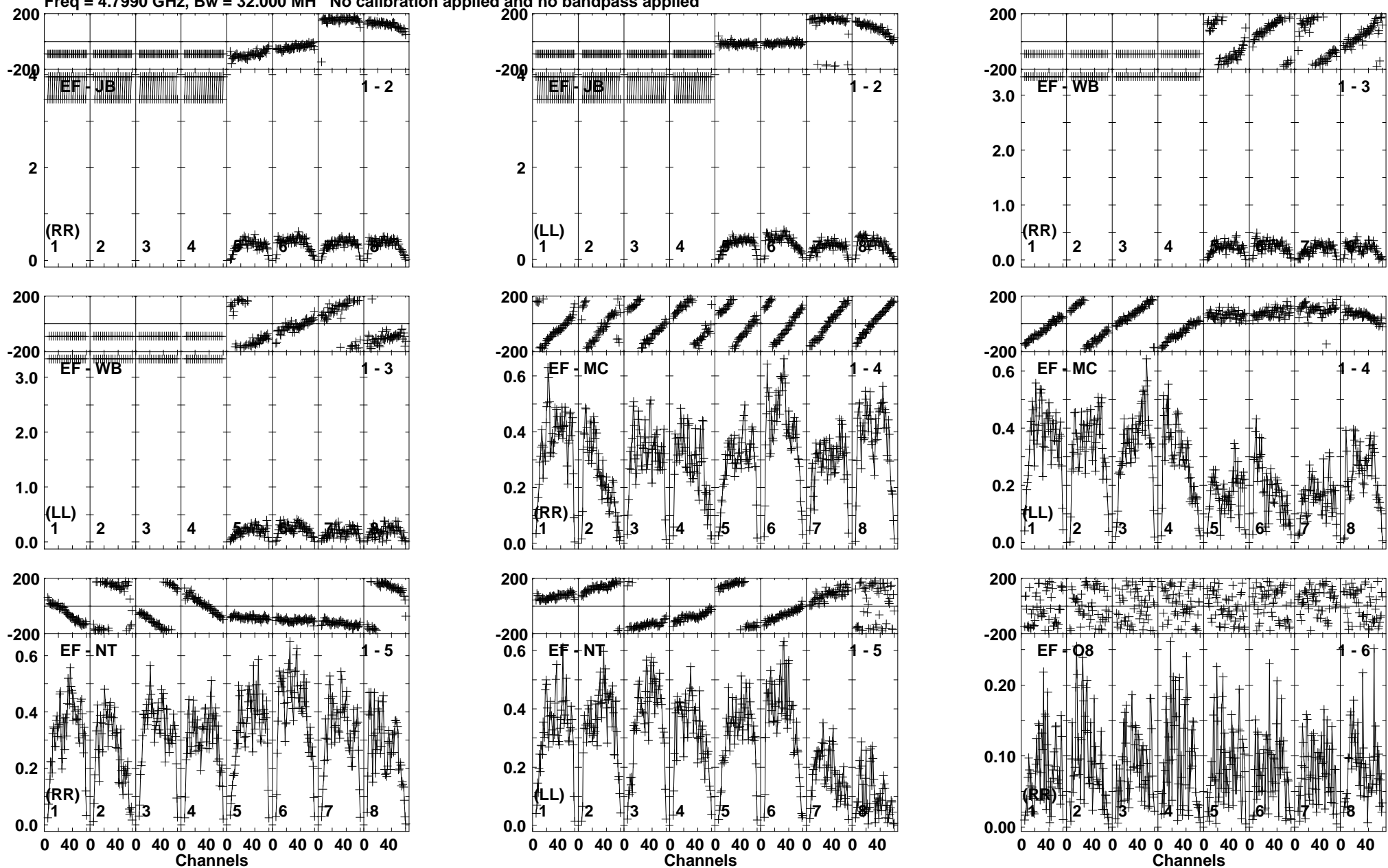
Lower frame: Milli Ampl Jy Top frame: Phas deg Vector averaged cross-power spectrum Baseline: EF (01) - JB (02) Timerange: 00/02:08:31 to 00/02:11:59
