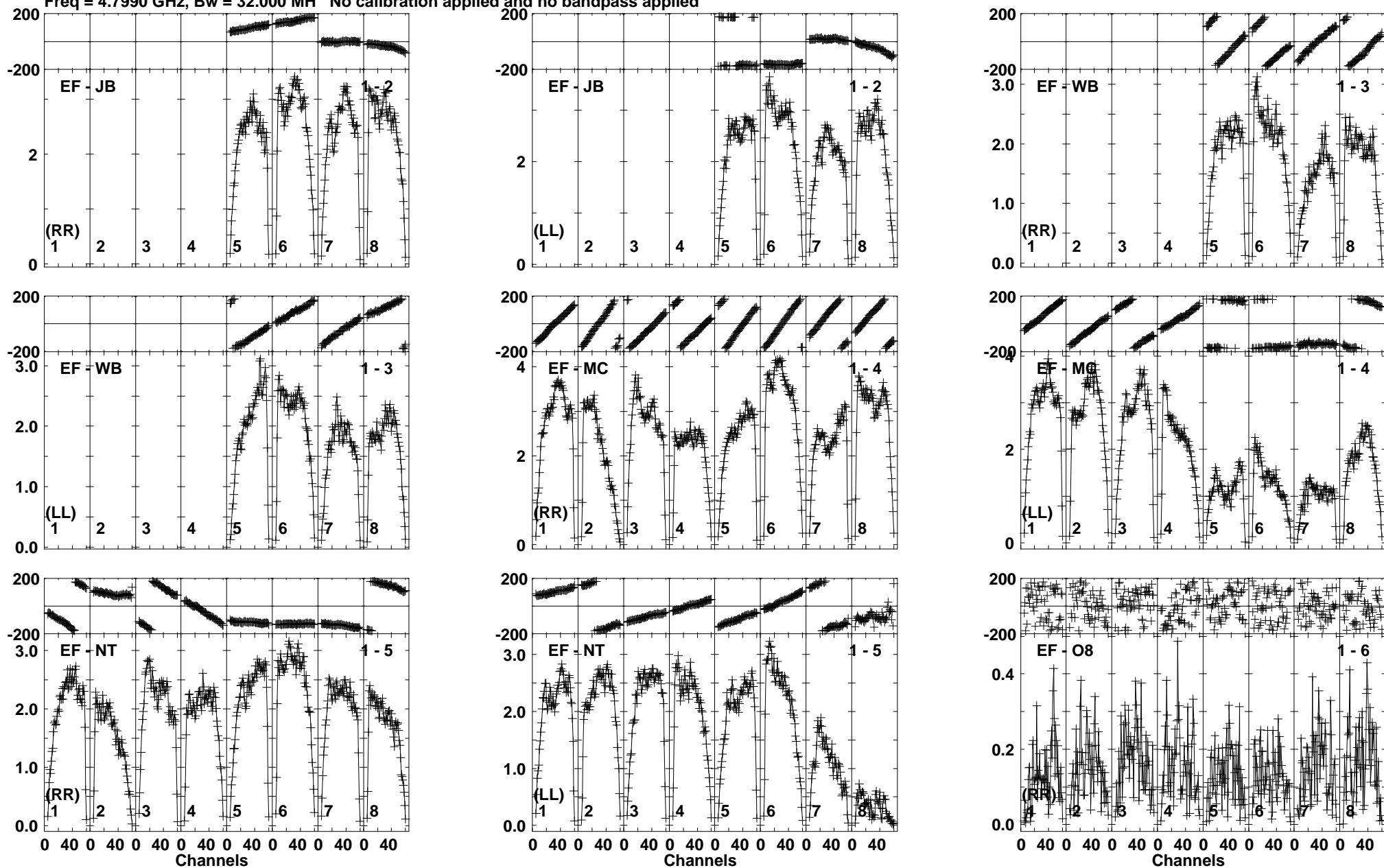
Lower frame: Milli Ampl Jy Top frame: Phas deg Vector averaged cross-power spectrum Baseline: EF (01) - JB (02) Timerange: 00/05:58:00 to 00/05:59:29
