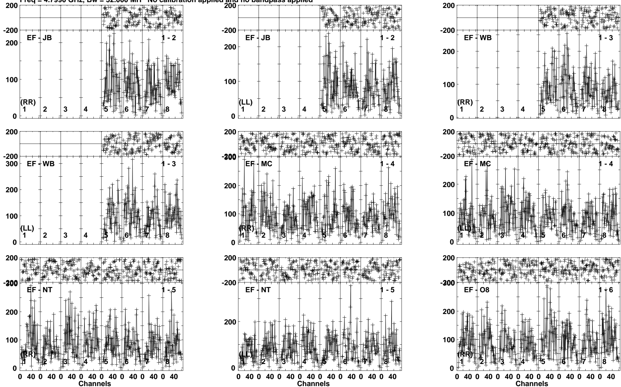
Lower frame: Micro Ampl Jy Top frame: Phas deg Vector averaged cross-power spectrum Baseline: EF (01) - JB (02) Timerange: 00/04:28:00 to 00/04:31:30
