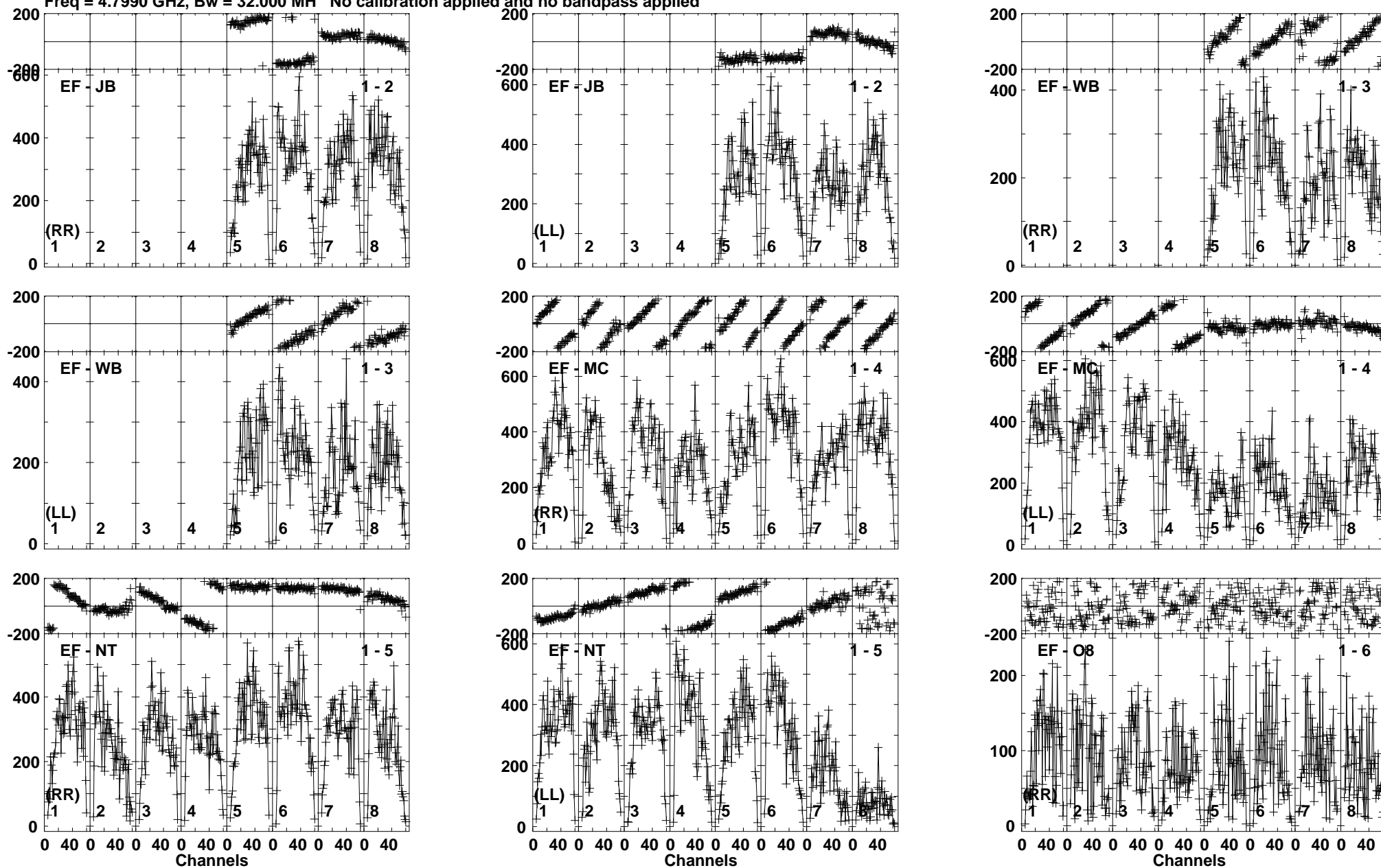
Lower frame: Micro Ampl Jy Top frame: Phas deg Vector averaged cross-power spectrum Baseline: EF (01) - JB (02) Timerange: 00/05:24:00 to 00/05:27:30
