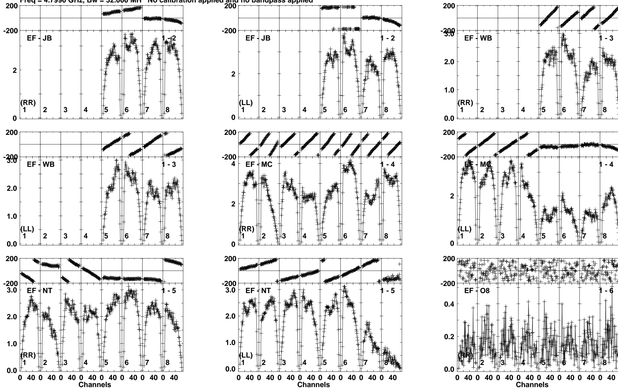
Lower frame: Milli Ampl Jy Top frame: Phas deg Vector averaged cross-power spectrum Baseline: EF (01) - JB (02) Timerange: 00/05:33:10 to 00/05:34:10
