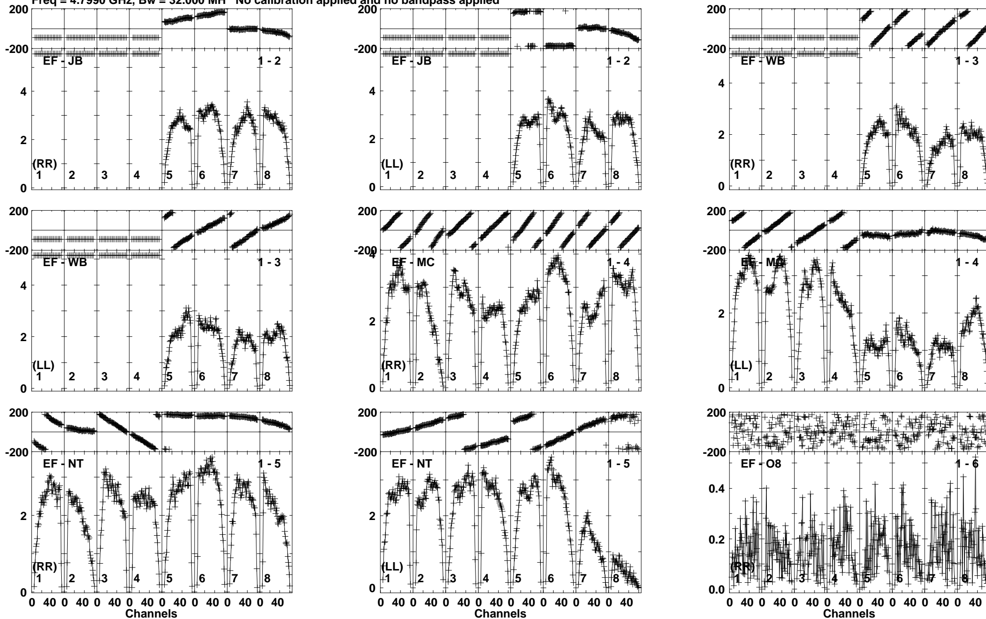
Lower frame: Milli Ampl Jy Top frame: Phas deg Vector averaged cross-power spectrum Baseline: EF (01) - JB (02) Timerange: 00/05:37:41 to 00/05:39:09
