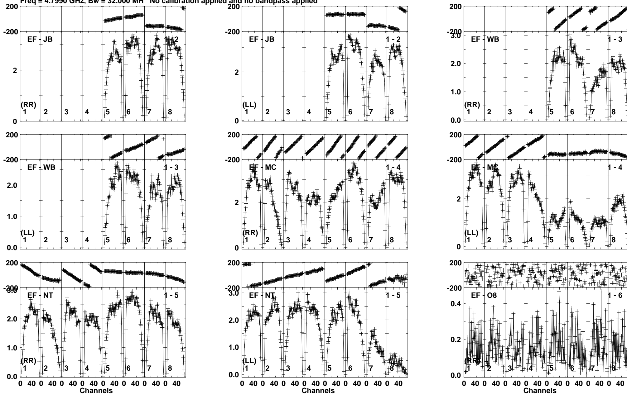
Lower frame: Milli Ampl Jy Top frame: Phas deg Vector averaged cross-power spectrum Baseline: EF (01) - JB (02) Timerange: 00/02:22:10 to 00/02:23:39
