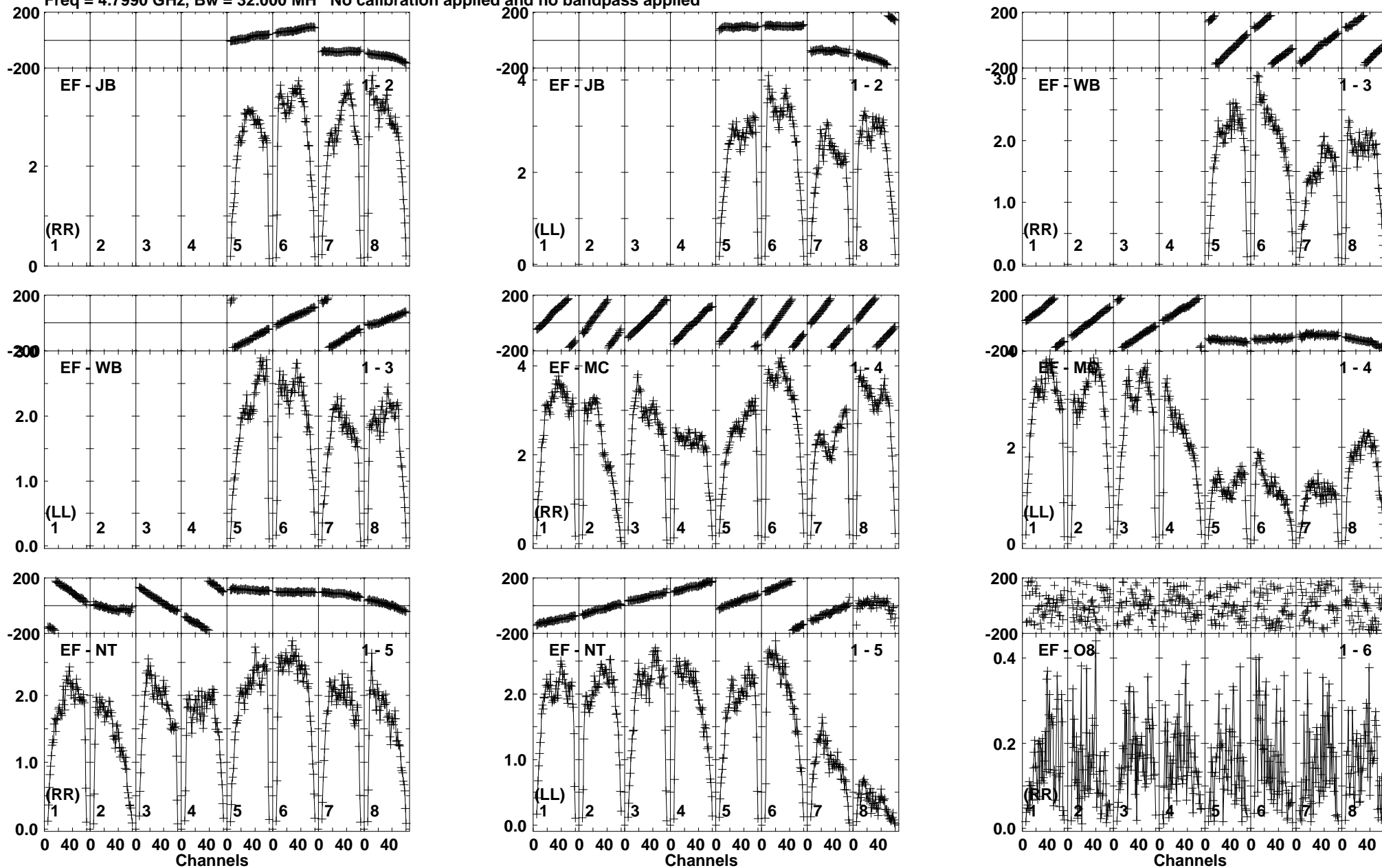
Lower frame: Milli Ampl Jy Top frame: Phas deg Vector averaged cross-power spectrum Baseline: EF (01) - JB (02) Timerange: 00/04:01:40 to 00/04:02:40
