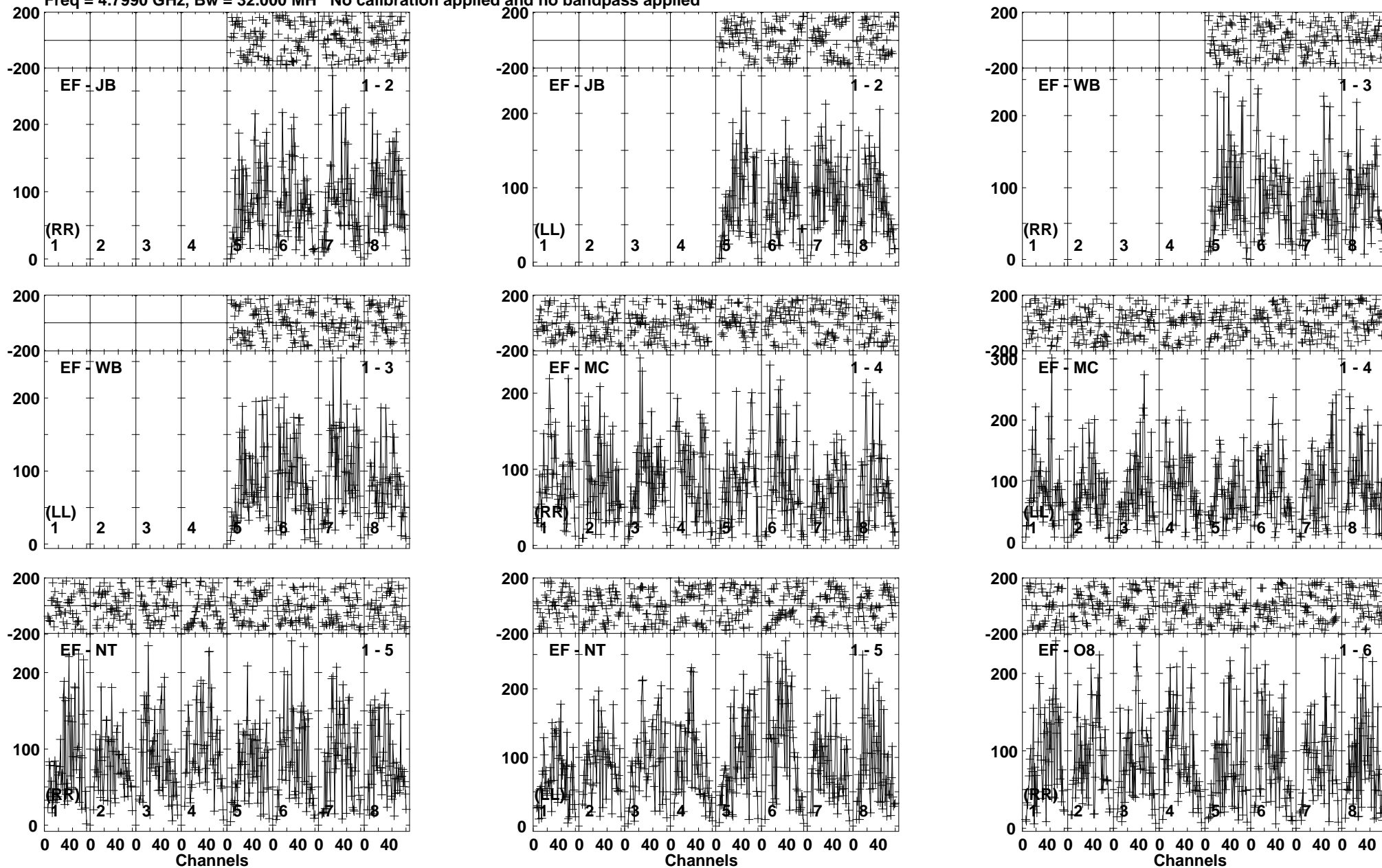
Lower frame: Micro Ampl Jy Top frame: Phas deg Vector averaged cross-power spectrum Baseline: EF (01) - JB (02) Timerange: 00/01:27:51 to 00/01:31:19
