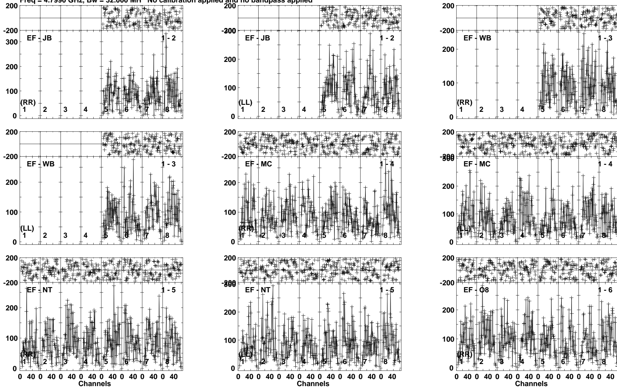
Lower frame: Micro Ampl Jy Top frame: Phas deg Vector averaged cross-power spectrum Baseline: EF (01) - JB (02) Timerange: 00/01:32:51 to 00/01:36:20
