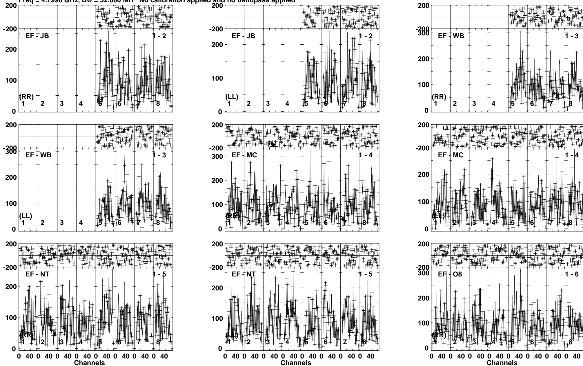
Lower frame: Micro Ampl Jy Top frame: Phas deg Vector averaged cross-power spectrum Baseline: EF (01) - JB (02) Timerange: 00/06:04:40 to 00/06:08:09
