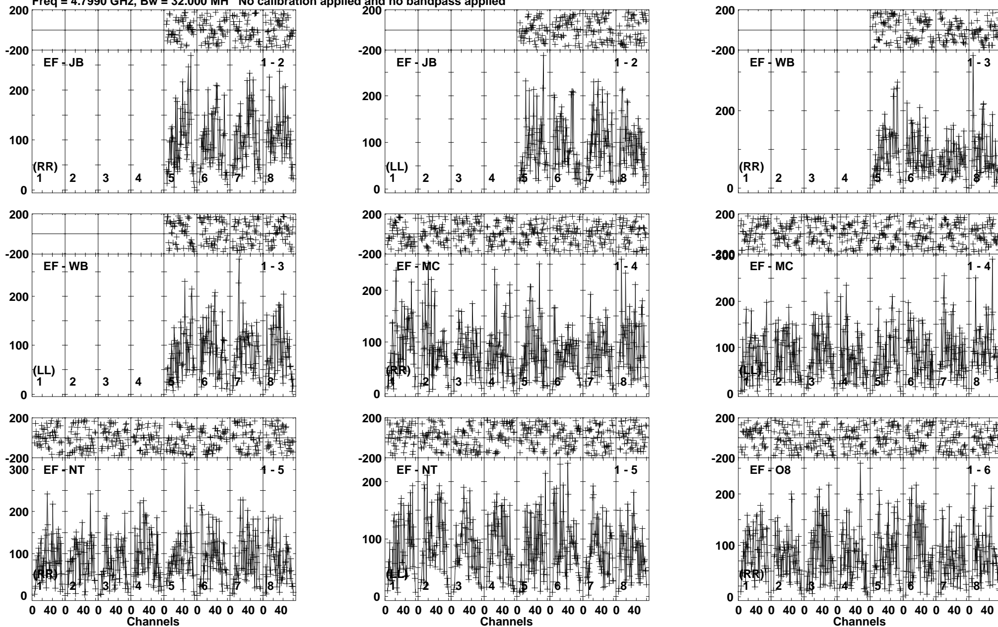
Lower frame: Micro Ampl Jy Top frame: Phas deg Vector averaged cross-power spectrum Baseline: EF (01) - JB (02) Timerange: 00/02:28:51 to 00/02:32:19
