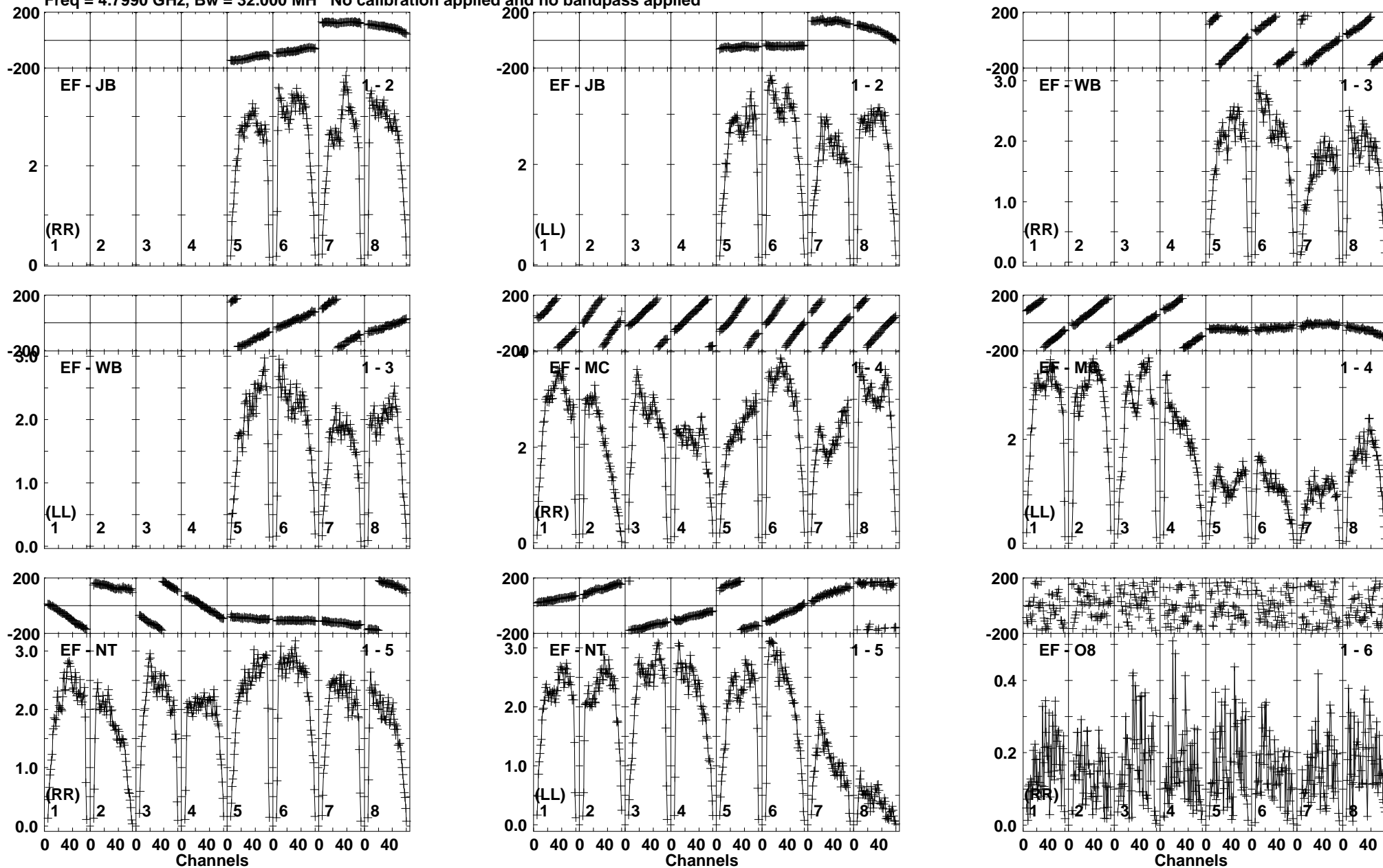
Lower frame: Milli Ampl Jy Top frame: Phas deg Vector averaged cross-power spectrum Baseline: EF (01) - JB (02) Timerange: 00/03:15:21 to 00/03:16:50
