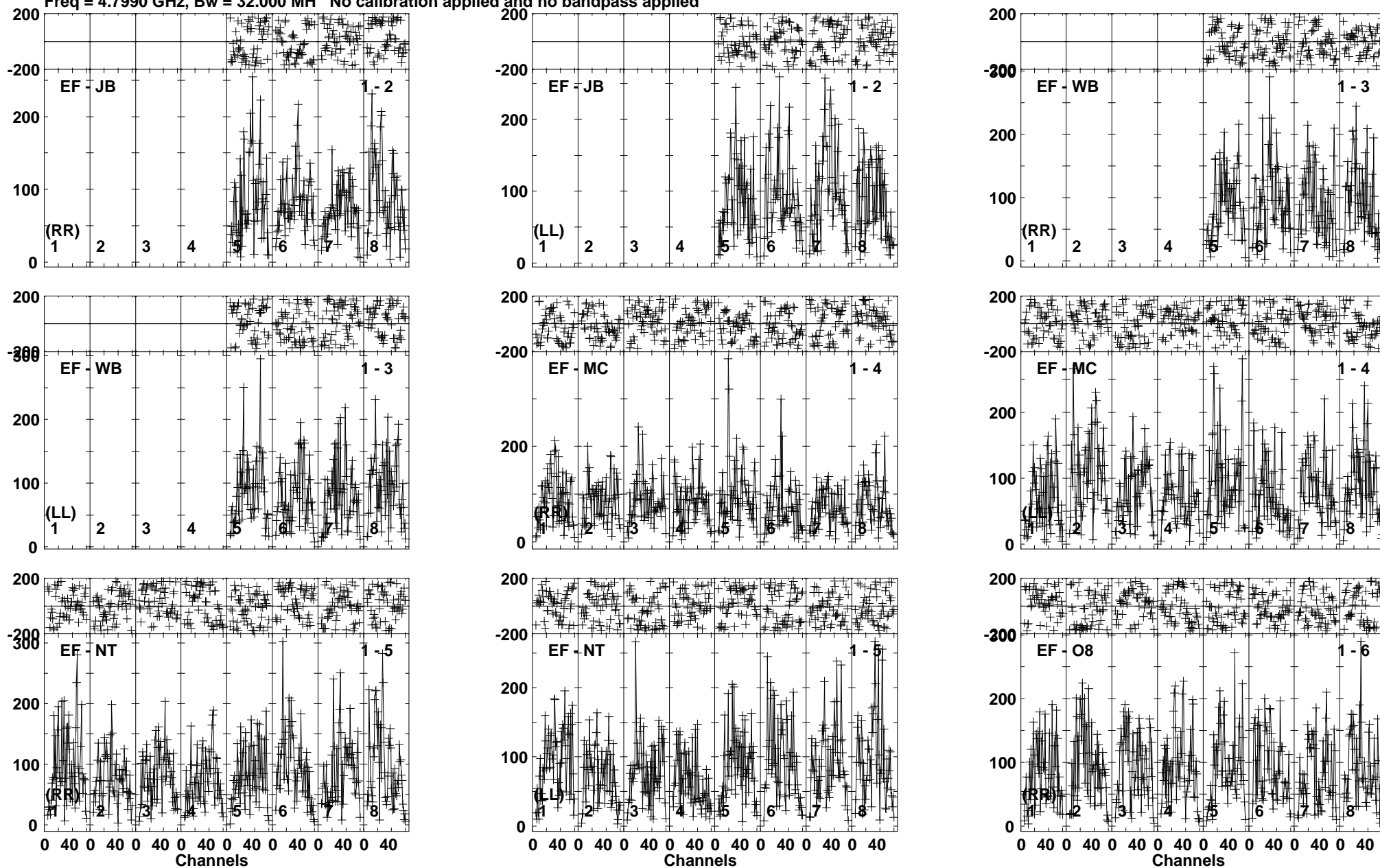
Lower frame: Micro Ampl Jy Top frame: Phas deg Vector averaged cross-power spectrum Baseline: EF (01) - JB (02) Timerange: 00/05:18:51 to 00/05:22:20
