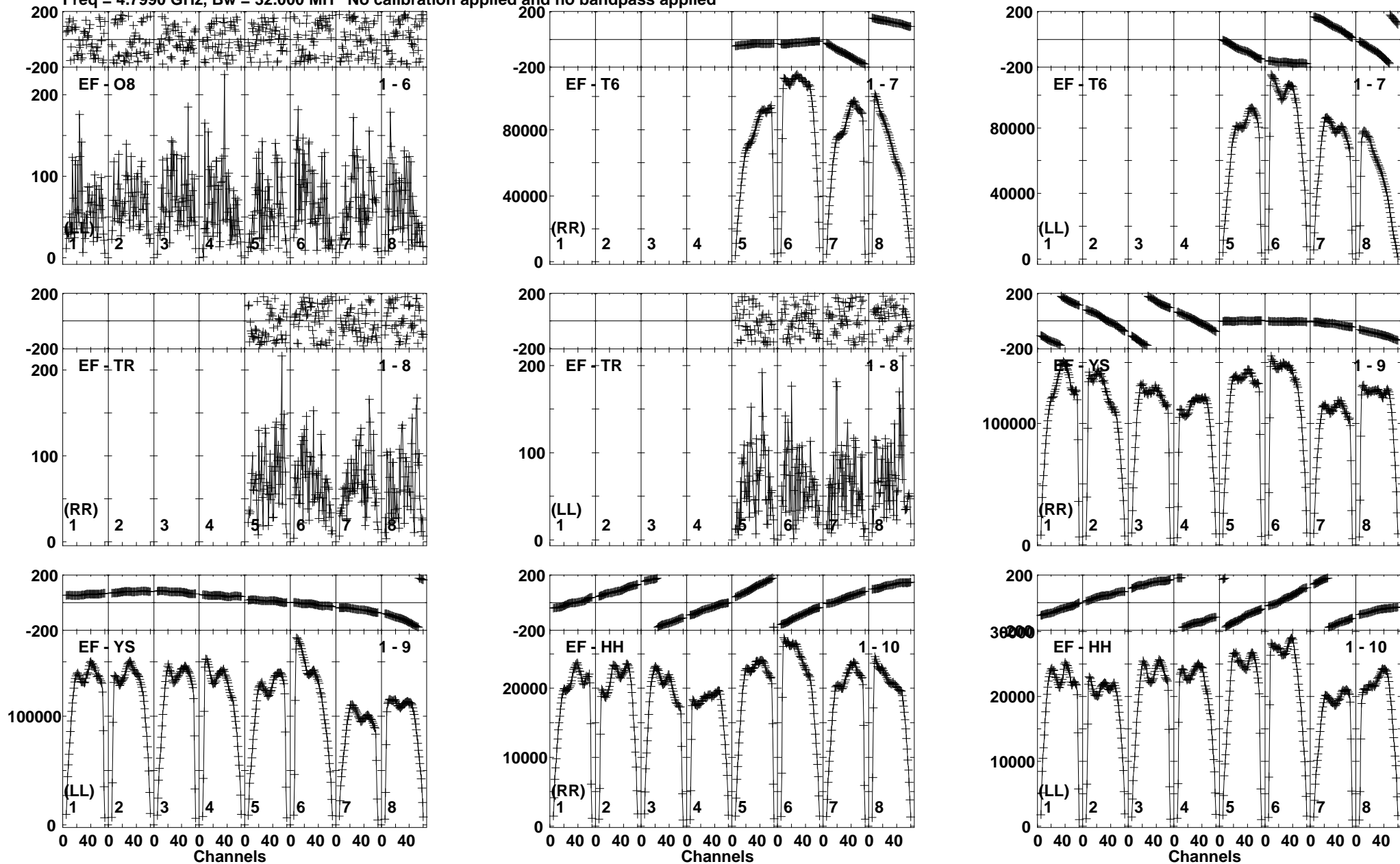
Lower frame: Micro Ampl Jy Top frame: Phas deg Vector averaged cross-power spectrum Baseline: EF (01) - O8 (06) Timerange: 00/02:40:51 to 00/02:45:50
