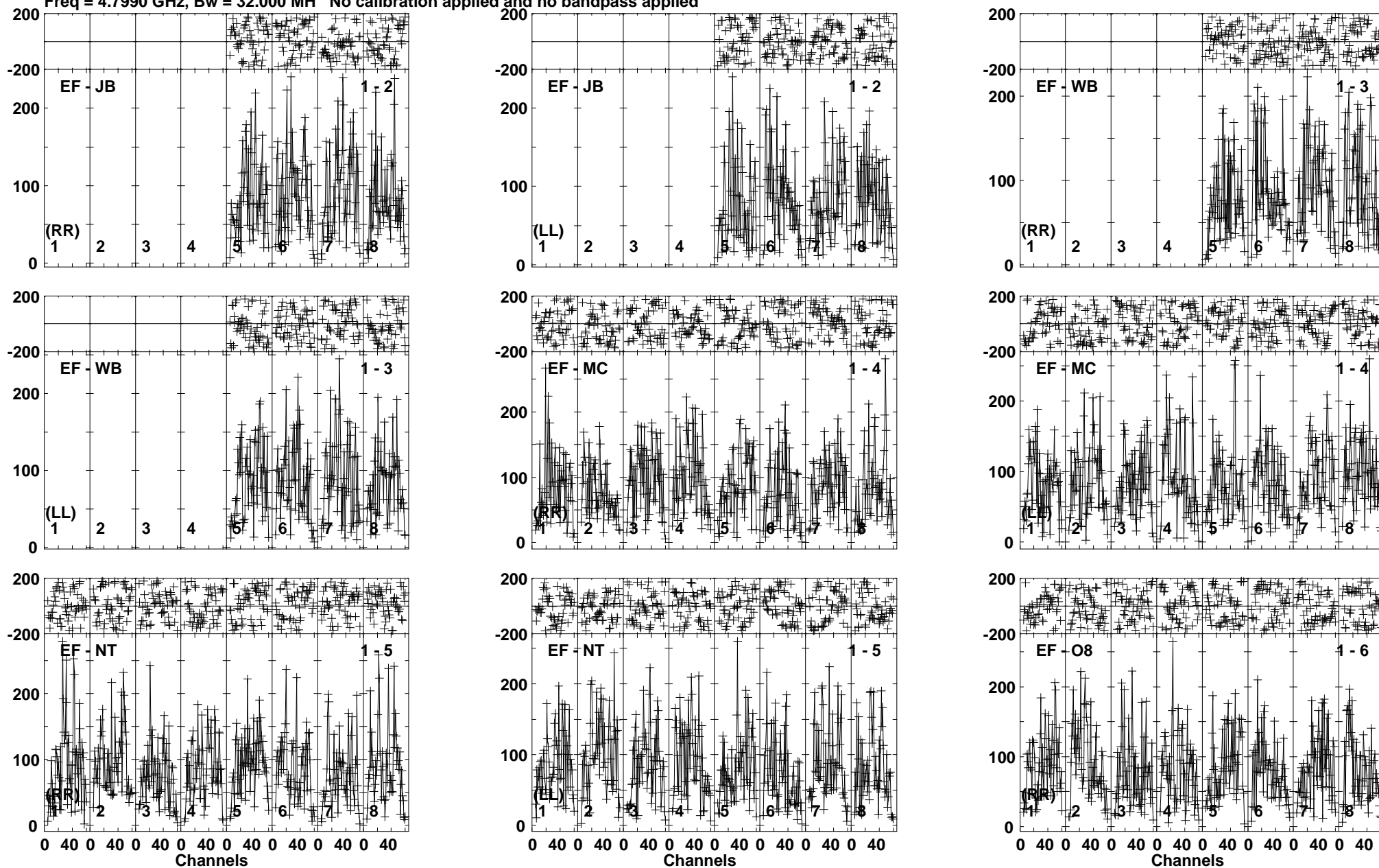
Lower frame: Micro Ampl Jy Top frame: Phas deg Vector averaged cross-power spectrum Baseline: EF (01) - JB (02) Timerange: 00/05:39:10 to 00/05:42:40
