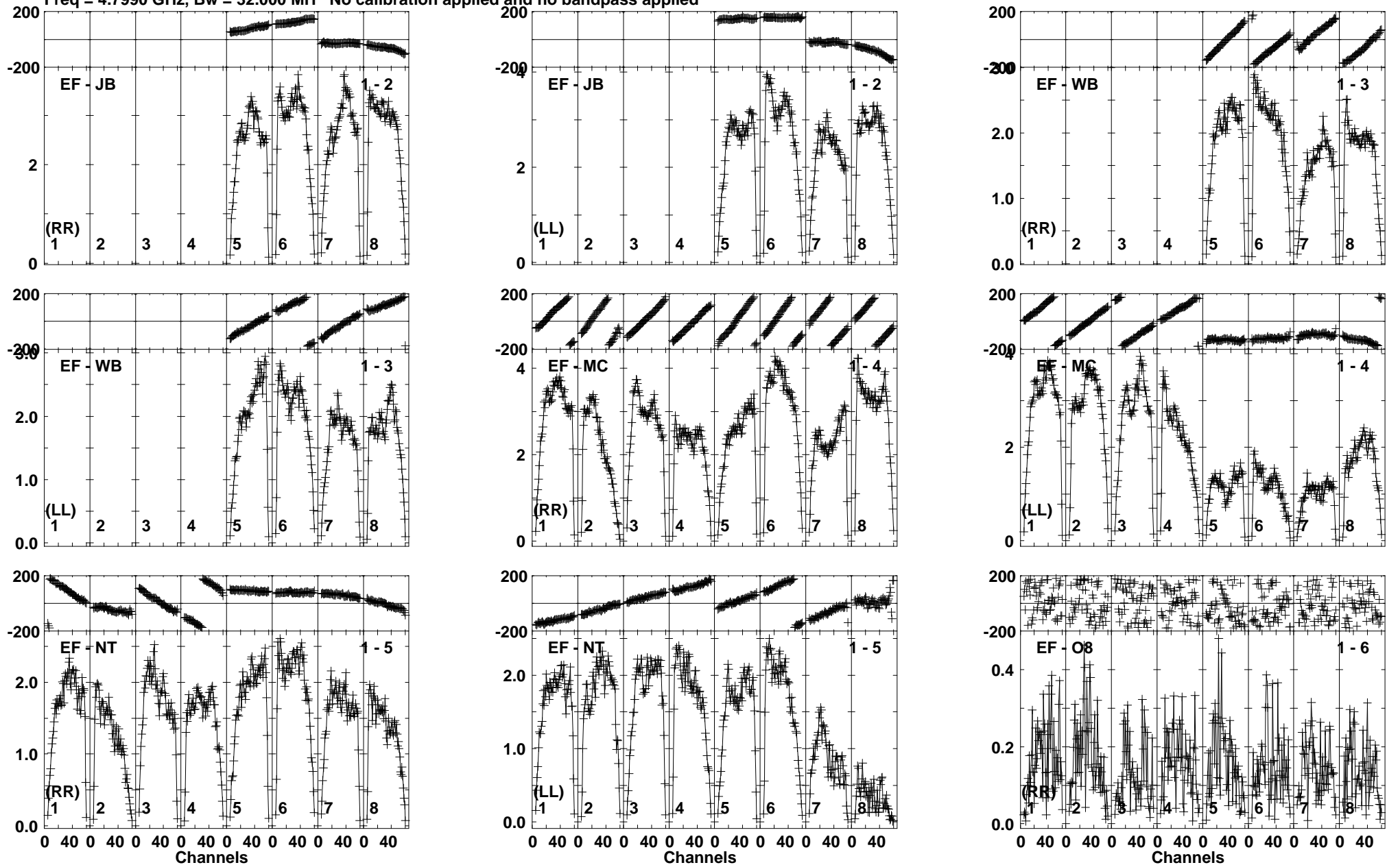
Lower frame: Milli Ampl Jy Top frame: Phas deg Vector averaged cross-power spectrum Baseline: EF (01) - JB (02) Timerange: 00/04:22:00 to 00/04:23:00
