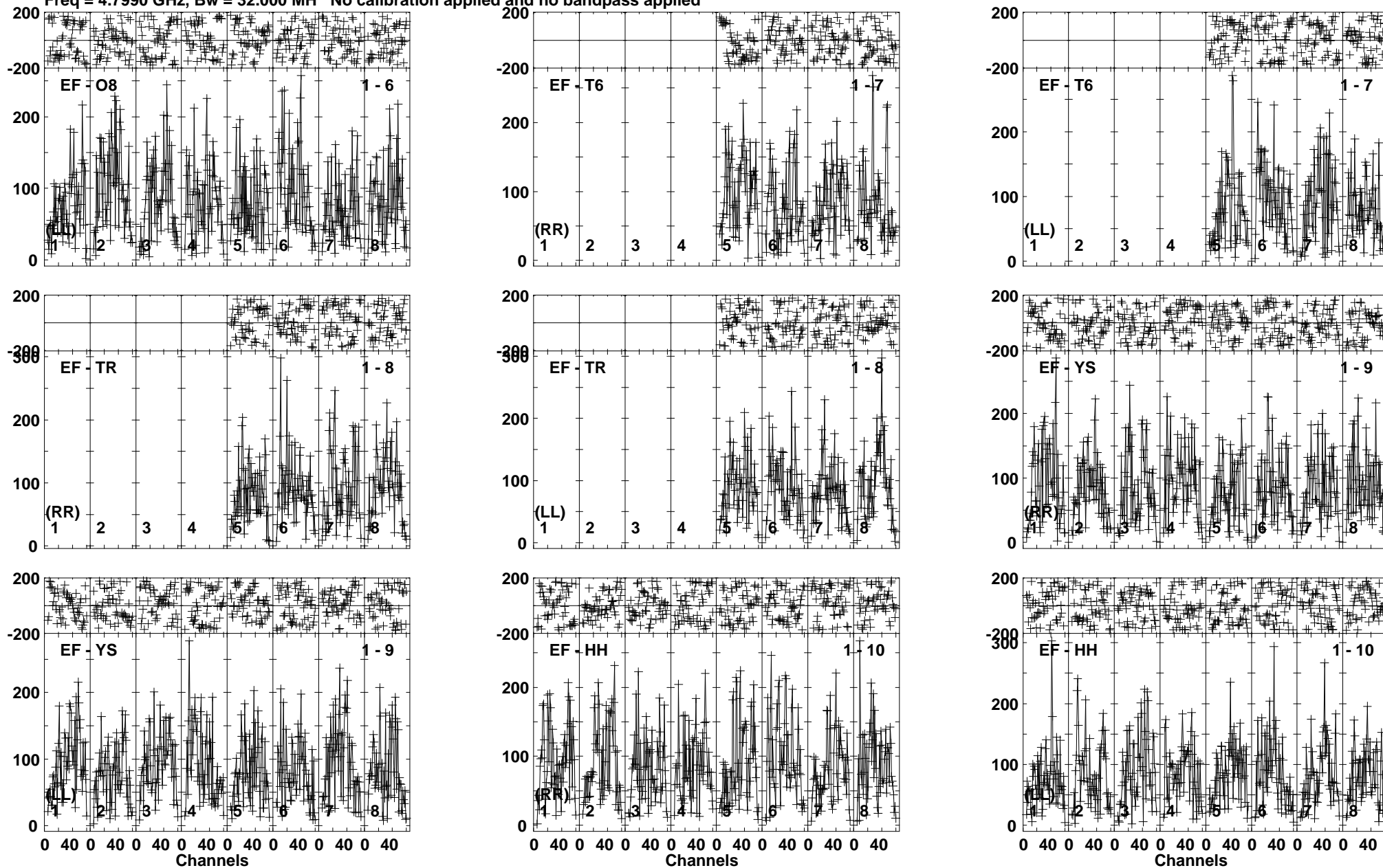
Lower frame: Micro Ampl Jy Top frame: Phas deg Vector averaged cross-power spectrum Baseline: EF (01) - O8 (06) Timerange: 00/03:37:10 to 00/03:40:40
