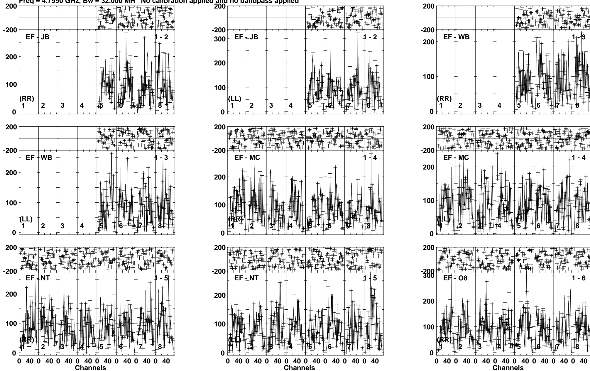
Lower frame: Micro Ampl Jy Top frame: Phas deg Vector averaged cross-power spectrum Baseline: EF (01) - JB (02) Timerange: 00/04:33:10 to 00/04:36:40
