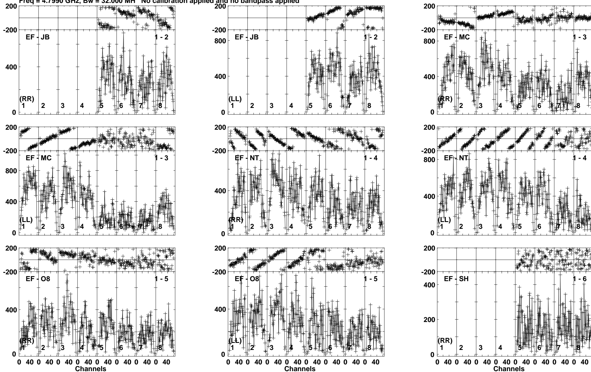
Lower frame: Micro Ampl Jy Top frame: Phas deg Vector averaged cross-power spectrum Baseline: EF (01) - JB (02) Timerange: 00/23:51:01 to 00/23:51:59
