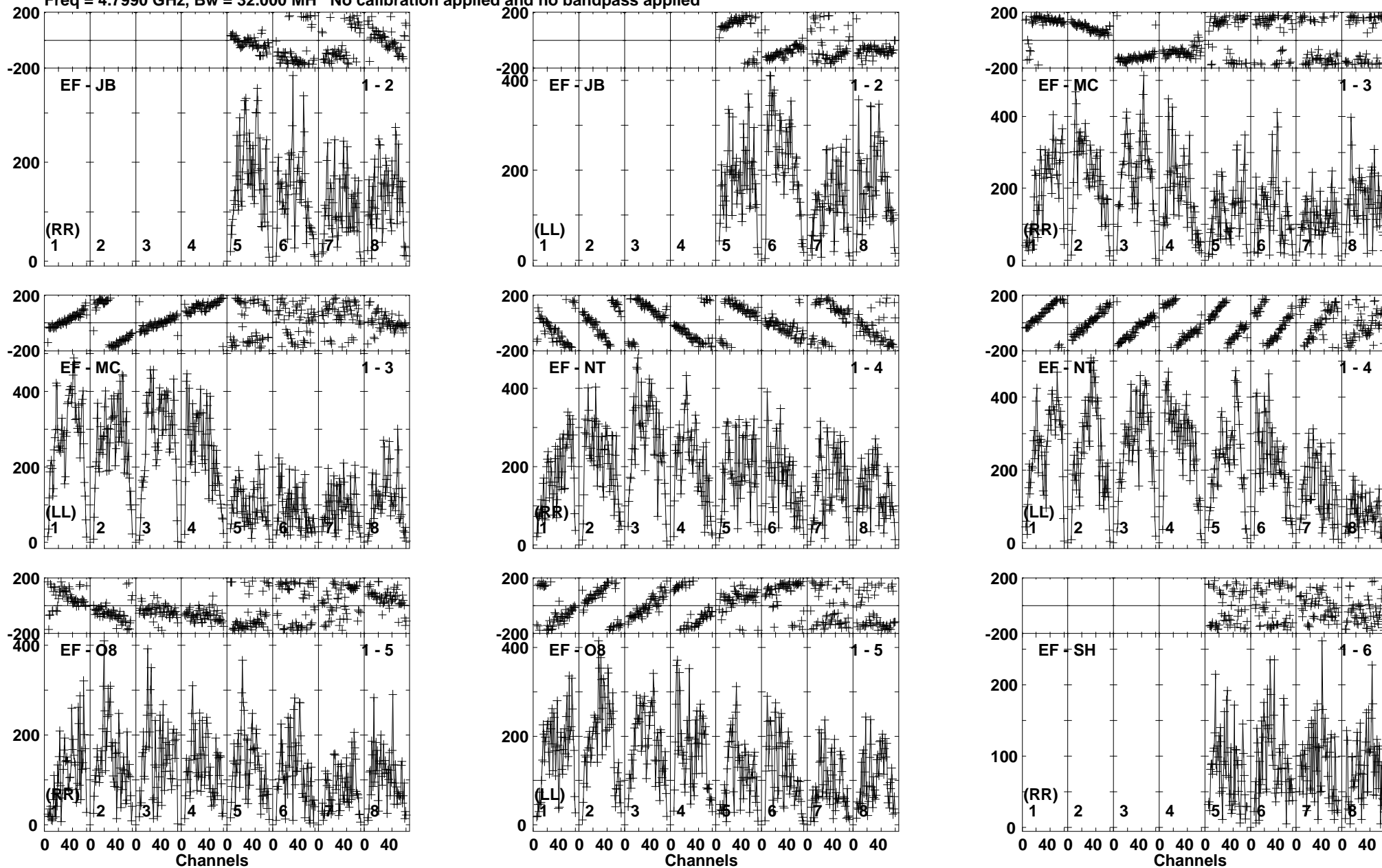
Lower frame: Micro Ampl Jy Top frame: Phas deg Vector averaged cross-power spectrum Baseline: EF (01) - JB (02) Timerange: 00/20:26:21 to 00/20:29:50
