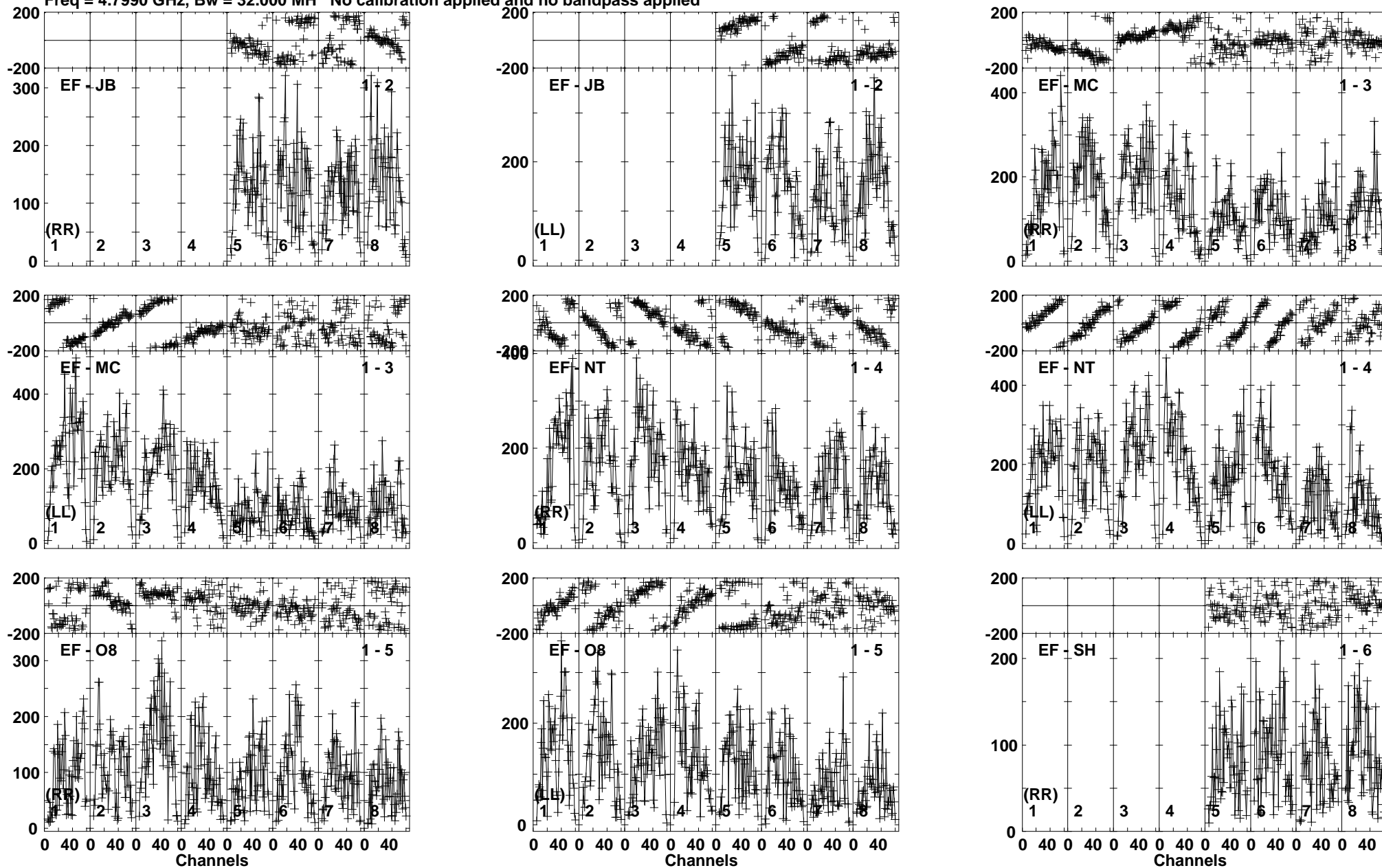
Lower frame: Micro Ampl Jy Top frame: Phas deg Vector averaged cross-power spectrum Baseline: EF (01) - JB (02) Timerange: 00/20:56:50 to 00/21:00:20
