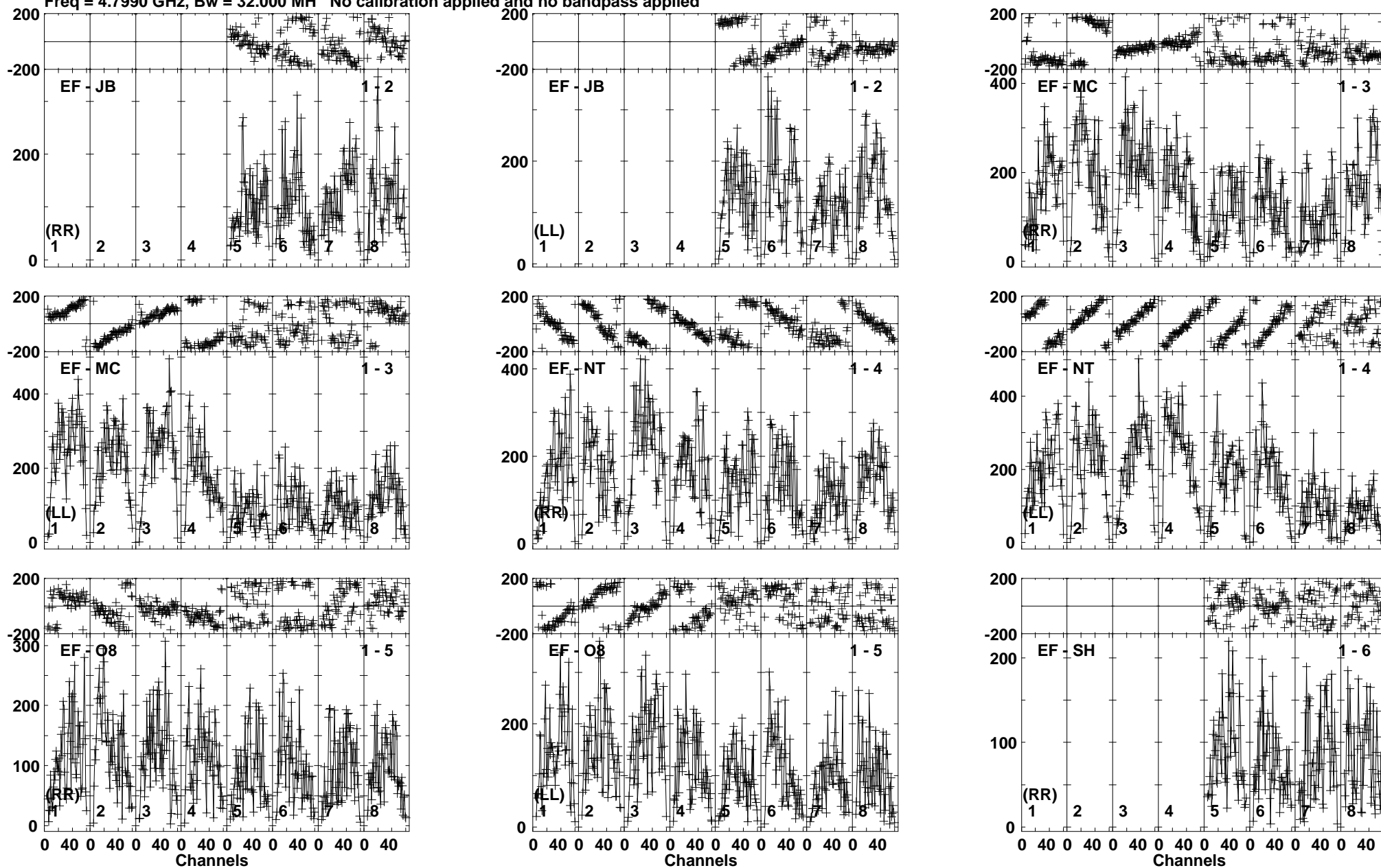
Lower frame: Micro Ampl Jy Top frame: Phas deg Vector averaged cross-power spectrum Baseline: EF (01) - JB (02) Timerange: 00/21:27:21 to 00/21:30:50
