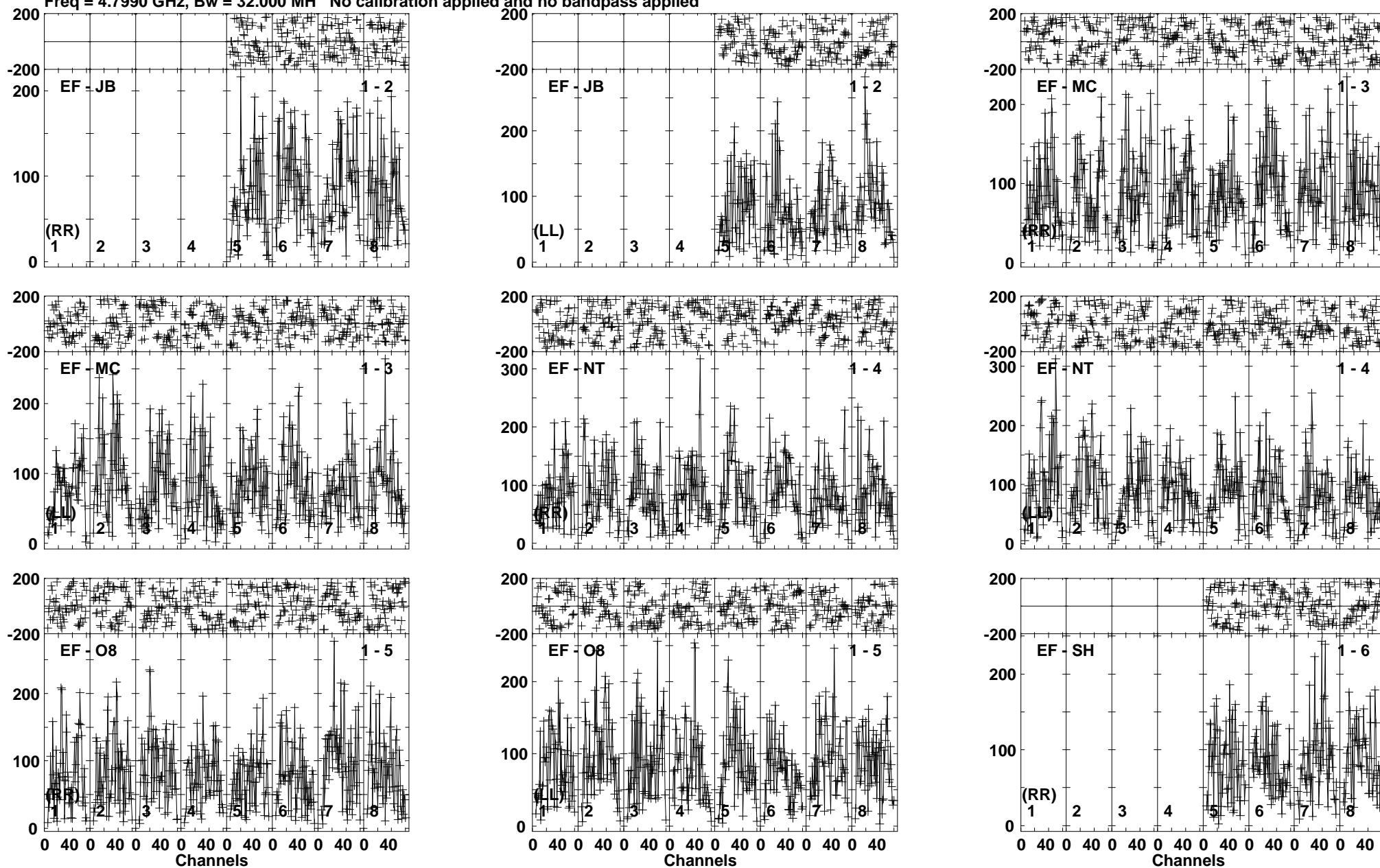
Lower frame: Micro Ampl Jy Top frame: Phas deg Vector averaged cross-power spectrum Baseline: EF (01) - JB (02) Timerange: 00/21:22:10 to 00/21:25:40
