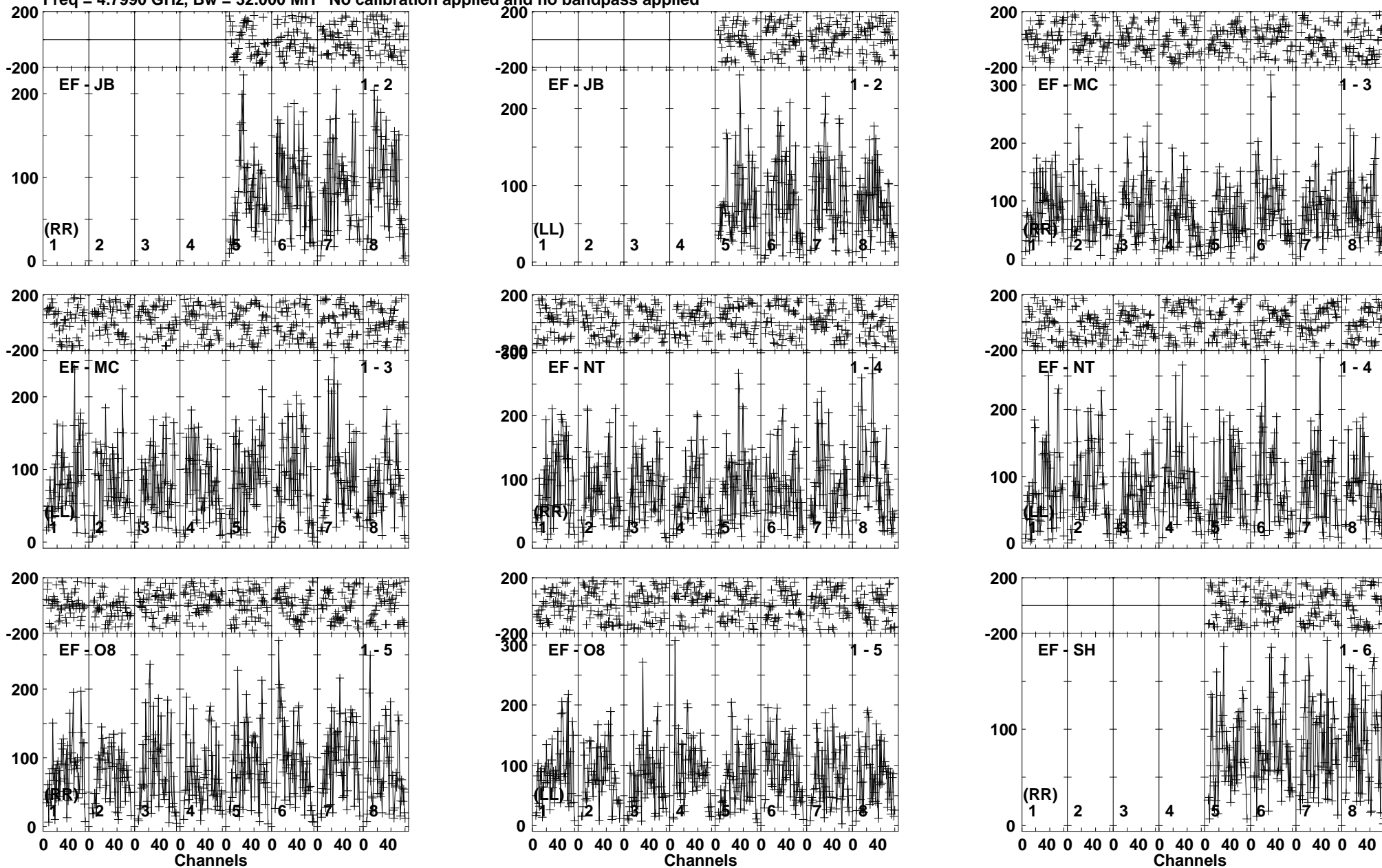
Lower frame: Micro Ampl Jy Top frame: Phas deg Vector averaged cross-power spectrum Baseline: EF (01) - JB (02) Timerange: 00/22:15:21 to 00/22:18:50
