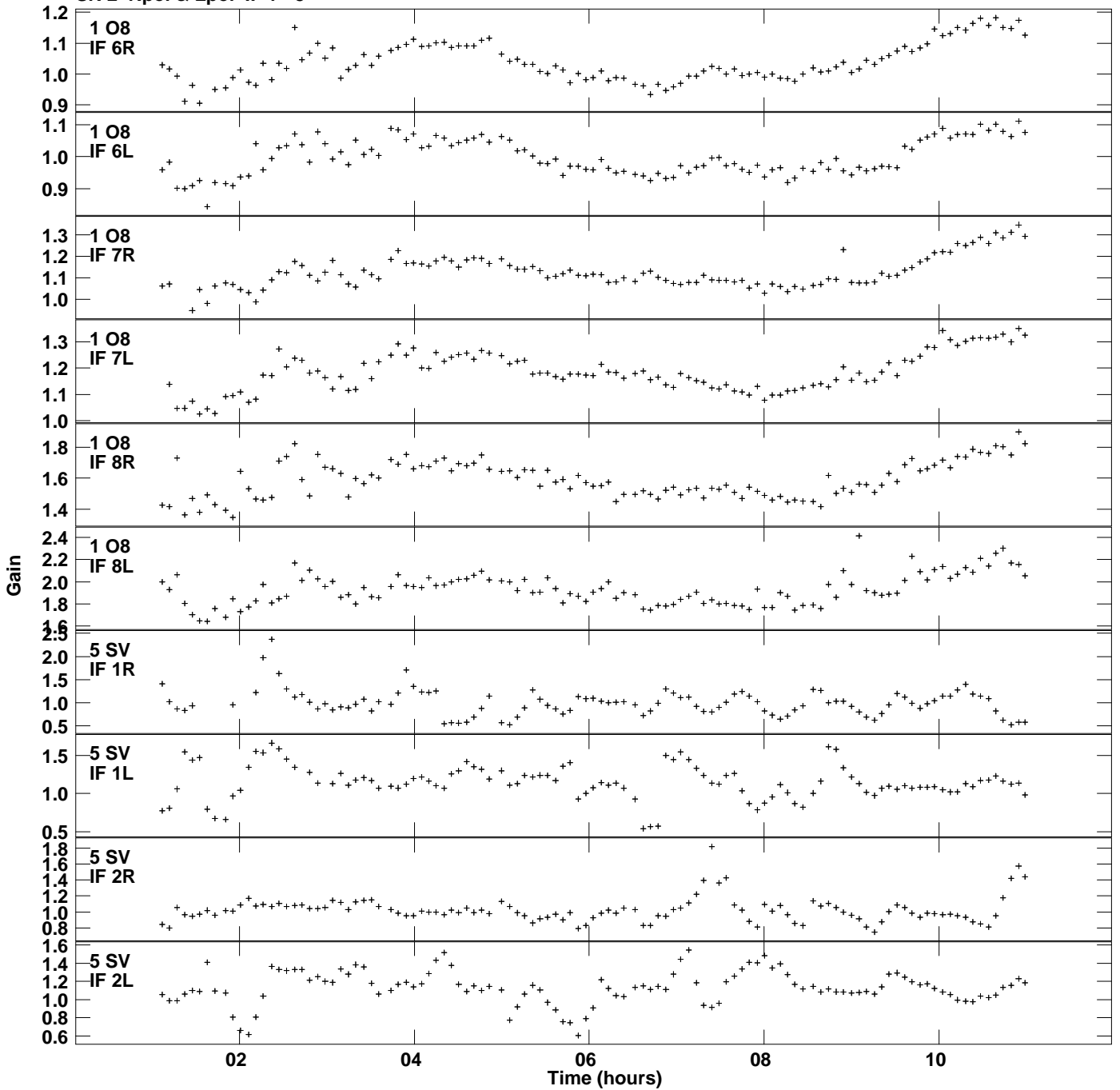
Plot file version 2 created 12-DEC-2017 12:05:52 Gain amp vs UTC time for J0304+3348.MULTI.1 SN 2 Rpol & Lpol IF 1 - 8
