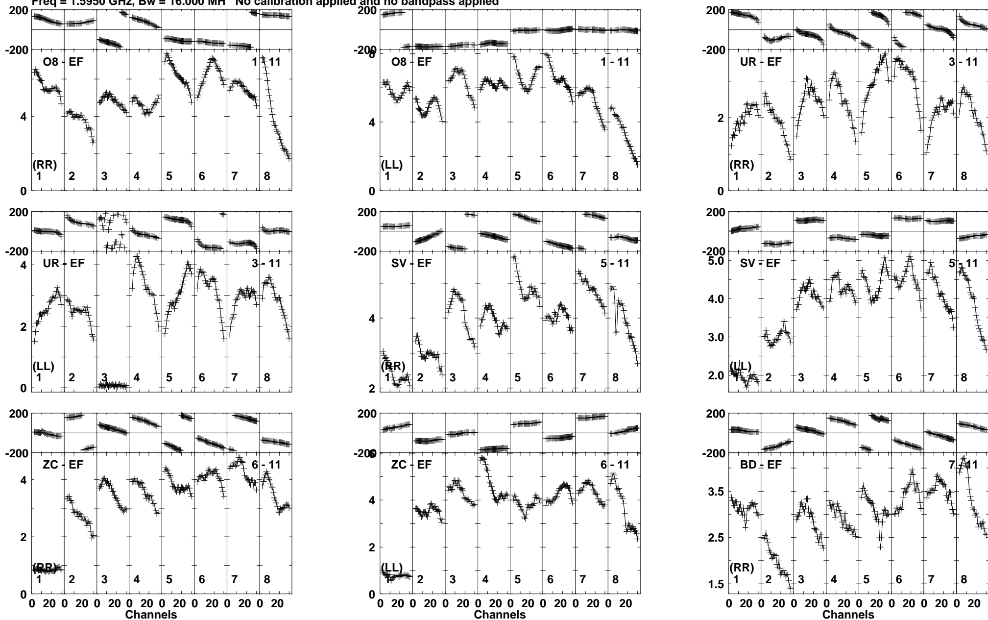
Lower frame: Milli Ampl Jy Top frame: Phas deg Vector averaged cross-power spectrum Baseline: O8 (01) - EF (11) Timerange: 00/09:09:21 to 00/09:10:49
