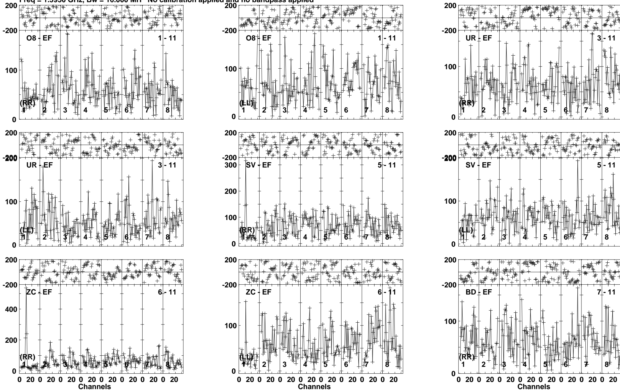
Lower frame: Micro Ampl Jy Top frame: Phas deg Vector averaged cross-power spectrum Baseline: O8 (01) - EF (11) Timerange: 00/03:49:41 to 00/03:53:09
