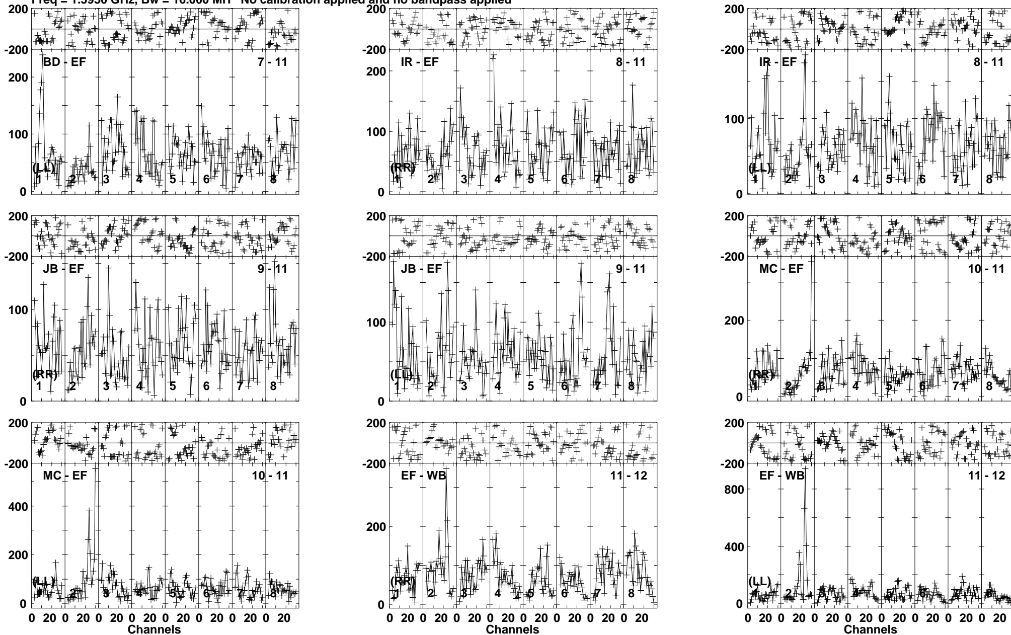
Lower frame: Micro Ampl Jy Top frame: Phas deg Vector averaged cross-power spectrum Baseline: BD (07) - EF (11) Timerange: 00/05:16:21 to 00/05:19:49
