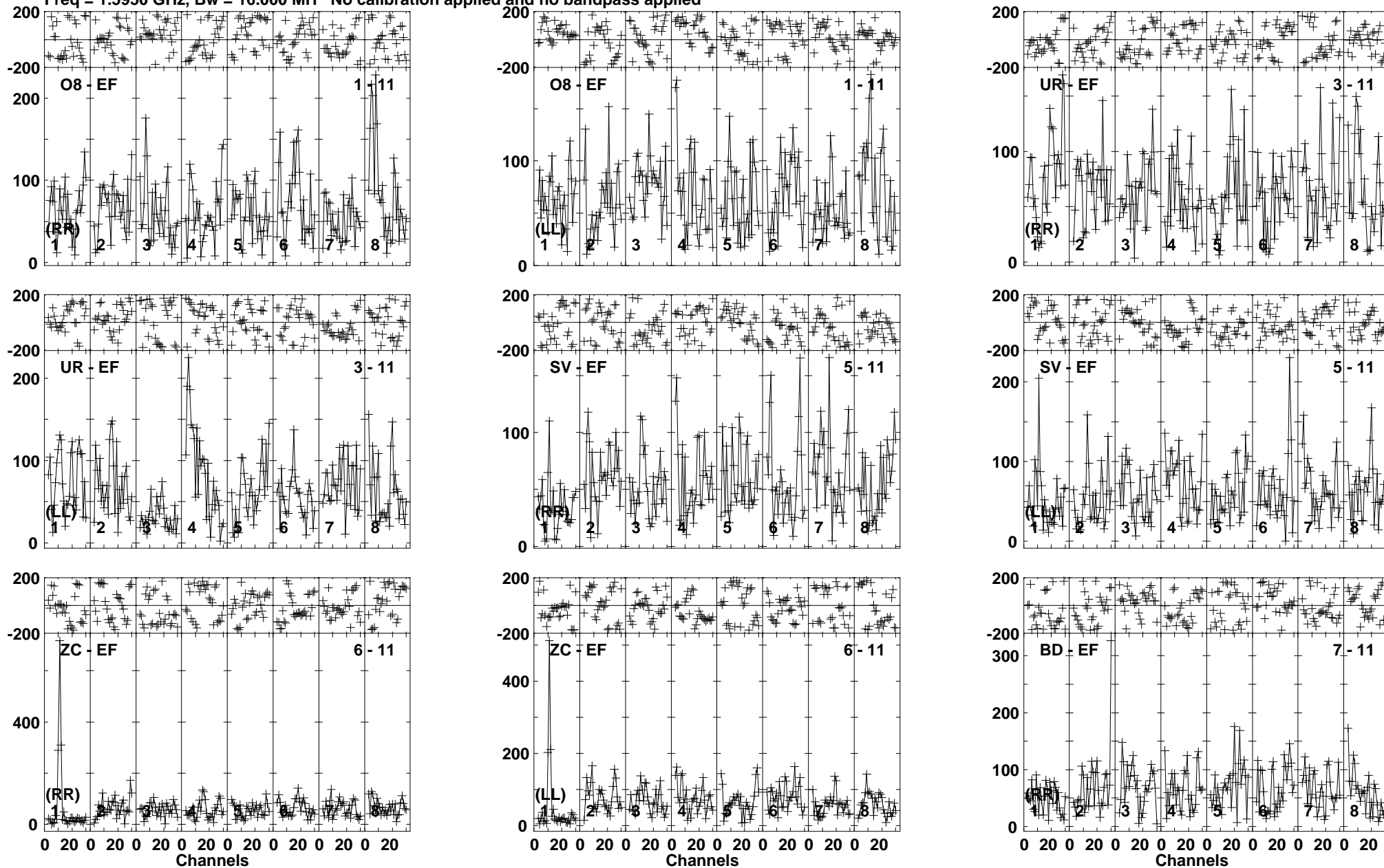
Lower frame: Micro Ampl Jy Top frame: Phas deg Vector averaged cross-power spectrum Baseline: O8 (01) - EF (11) Timerange: 00/05:22:01 to 00/05:25:29
