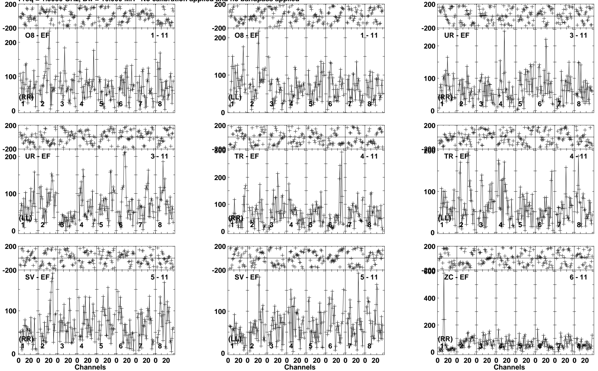
Lower frame: Micro Ampl Jy Top frame: Phas deg Vector averaged cross-power spectrum Baseline: O8 (01) - EF (11) Timerange: 00/10:34:51 to 00/10:38:19
