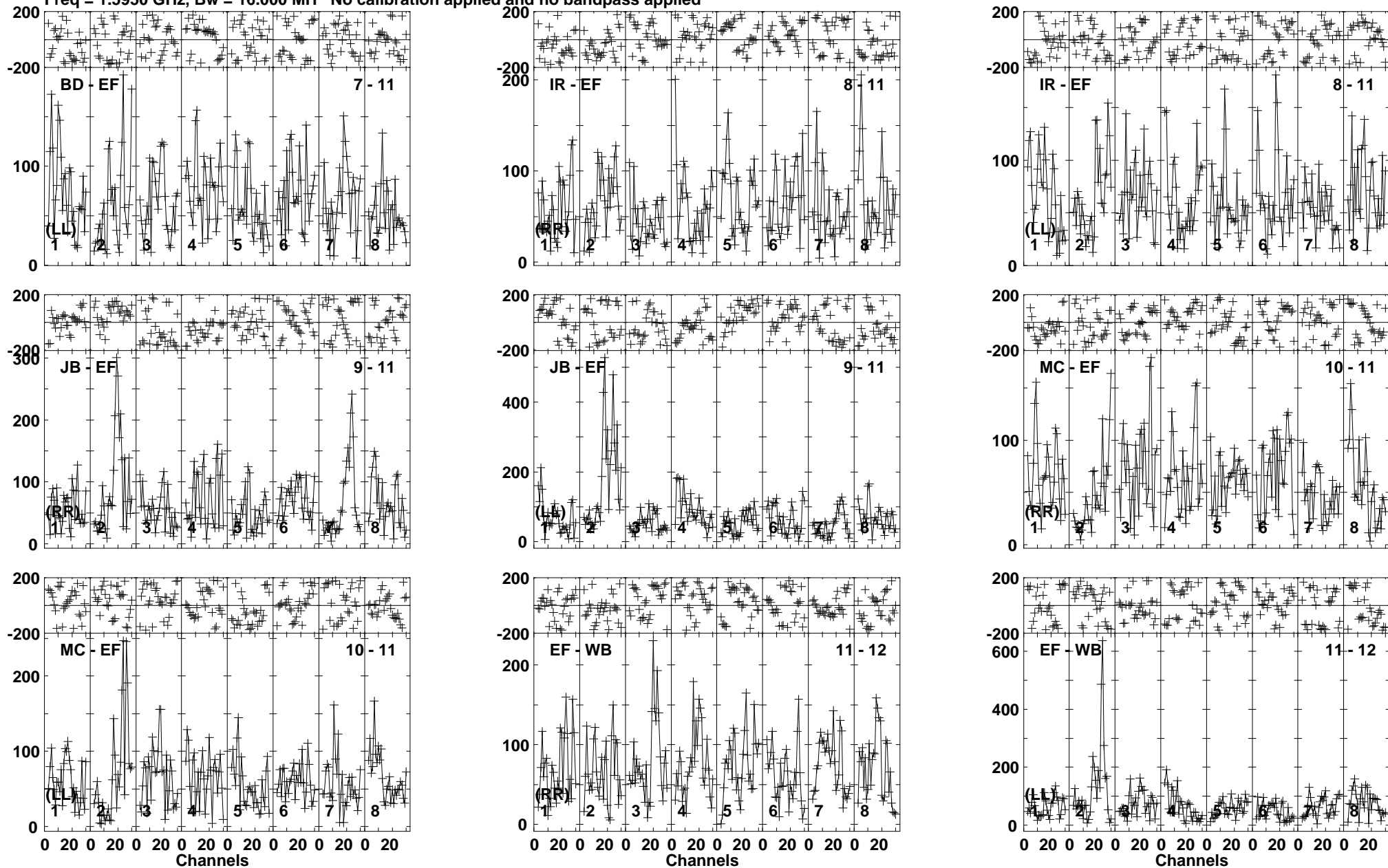
Lower frame: Micro Ampl Jy Top frame: Phas deg Vector averaged cross-power spectrum Baseline: BD (07) - EF (11) Timerange: 00/06:19:01 to 00/06:22:29
