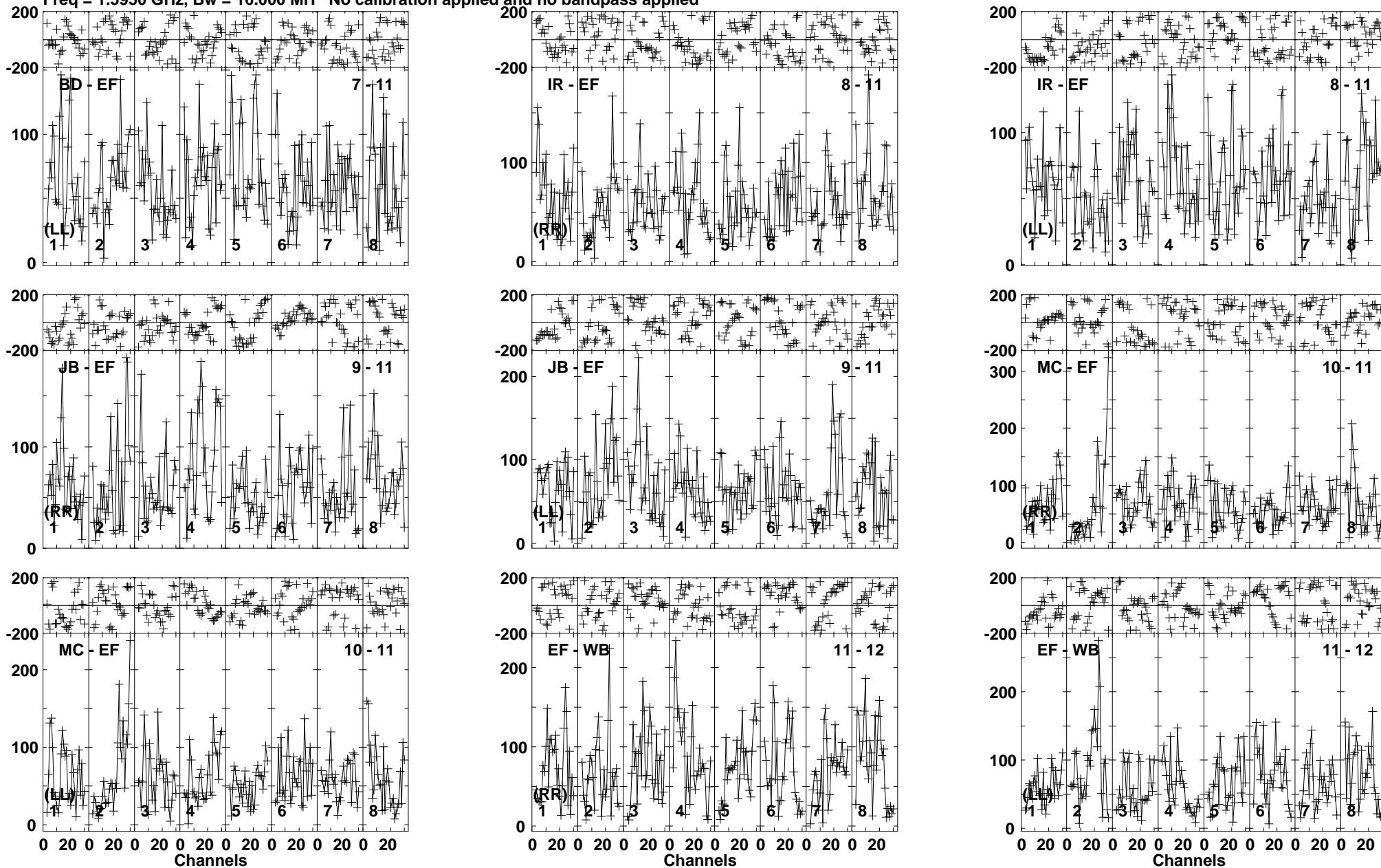
Lower frame: Micro Ampl Jy Top frame: Phas deg Vector averaged cross-power spectrum Baseline: BD (07) - EF (11) Timerange: 00/04:31:11 to 00/04:34:39
