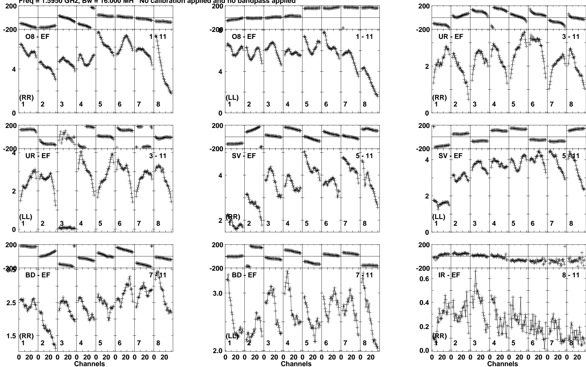
Lower frame: Milli Ampl Jy Top frame: Phas deg Vector averaged cross-power spectrum Baseline: O8 (01) - EF (11) Timerange: 00/07:54:41 to 00/07:56:09
