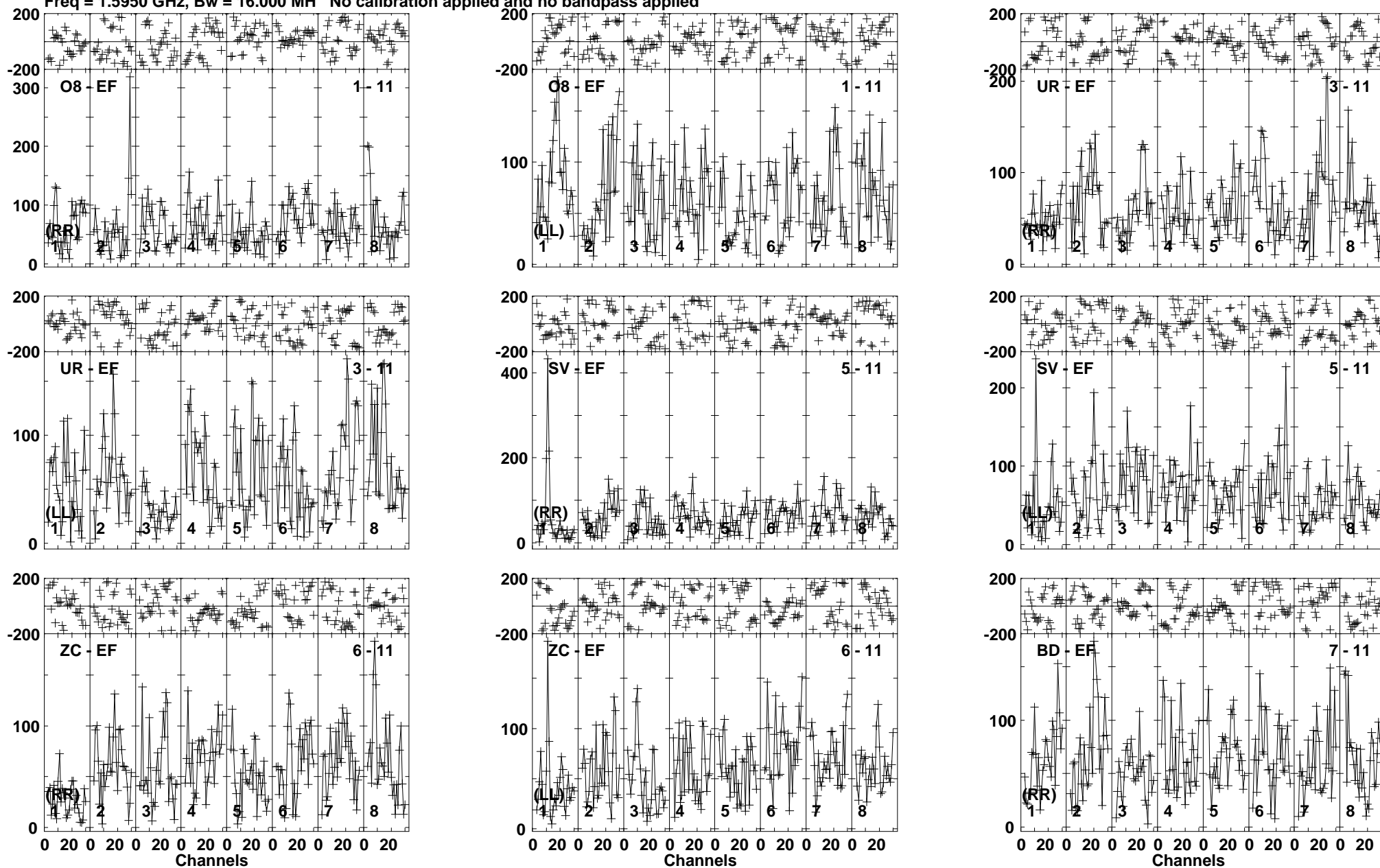
Lower frame: Micro Ampl Jy Top frame: Phas deg Vector averaged cross-power spectrum Baseline: O8 (01) - EF (11) Timerange: 00/04:05:41 to 00/04:09:09
