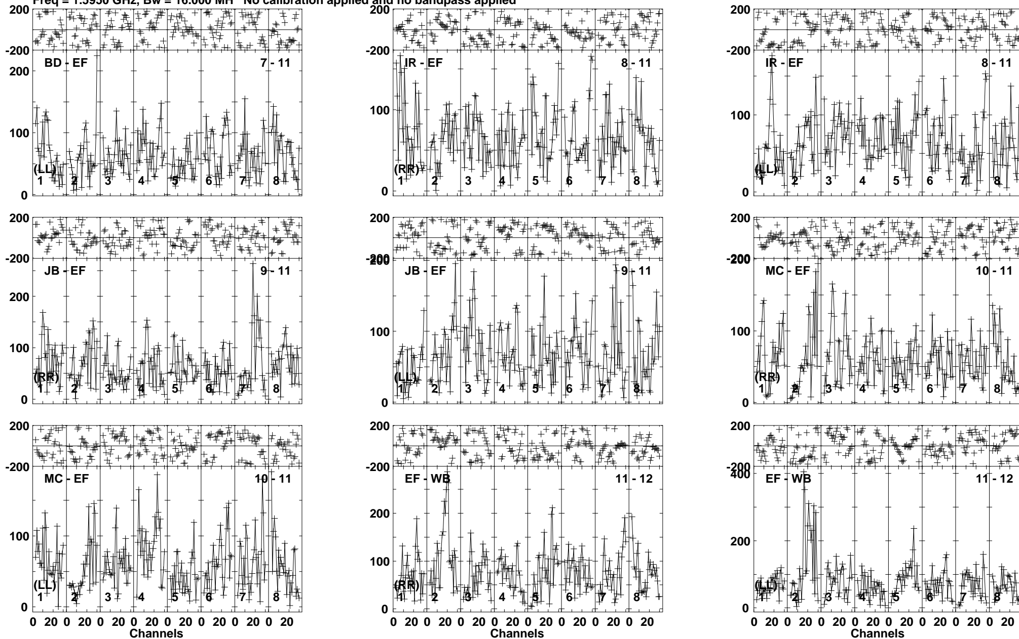
Lower frame: Micro Ampl Jy Top frame: Phas deg Vector averaged cross-power spectrum Baseline: BD (07) - EF (11) Timerange: 00/06:42:51 to 00/06:46:19
