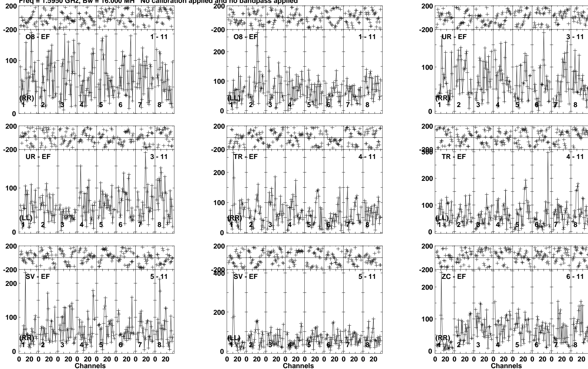
Lower frame: Micro Ampl Jy Top frame: Phas deg Vector averaged cross-power spectrum Baseline: O8 (01) - EF (11) Timerange: 00/10:39:51 to 00/10:43:19
