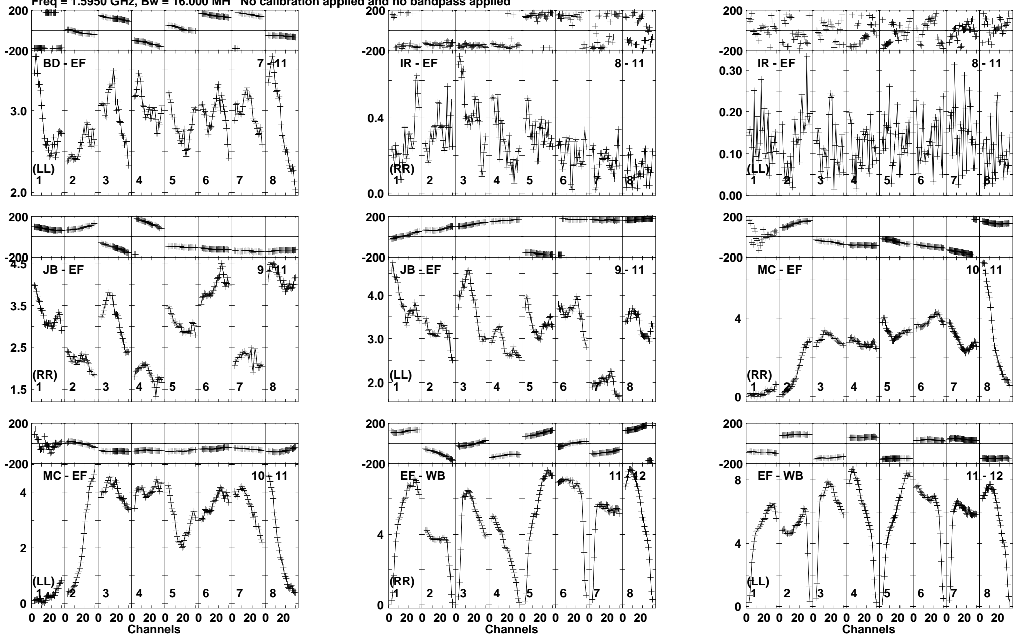
Lower frame: Milli Ampl Jy Top frame: Phas deg Vector averaged cross-power spectrum Baseline: BD (07) - EF (11) Timerange: 00/08:53:41 to 00/08:55:09
