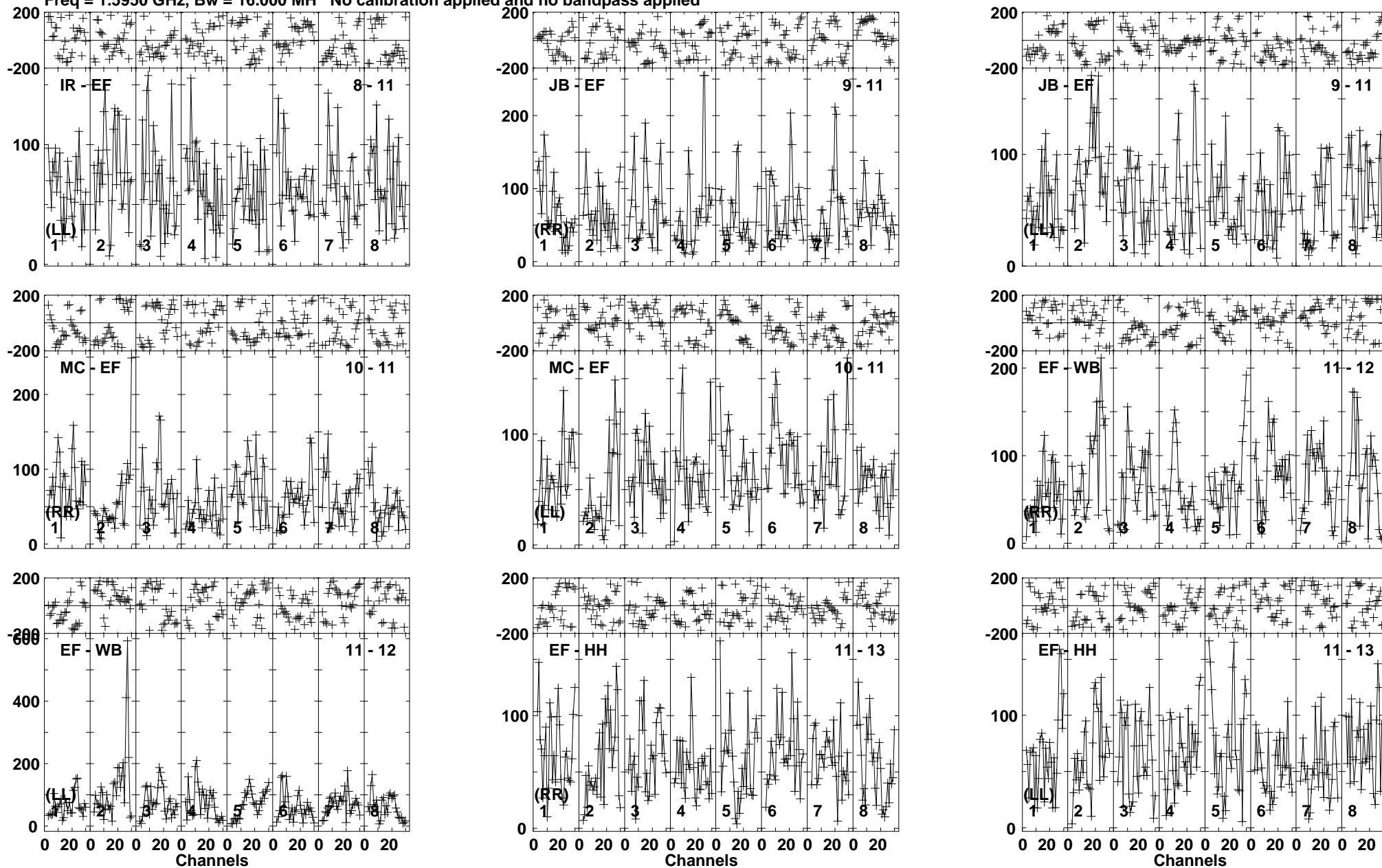
Lower frame: Micro Ampl Jy Top frame: Phas deg Vector averaged cross-power spectrum Baseline: IR (08) - EF (11) Timerange: 00/07:40:31 to 00/07:43:59
