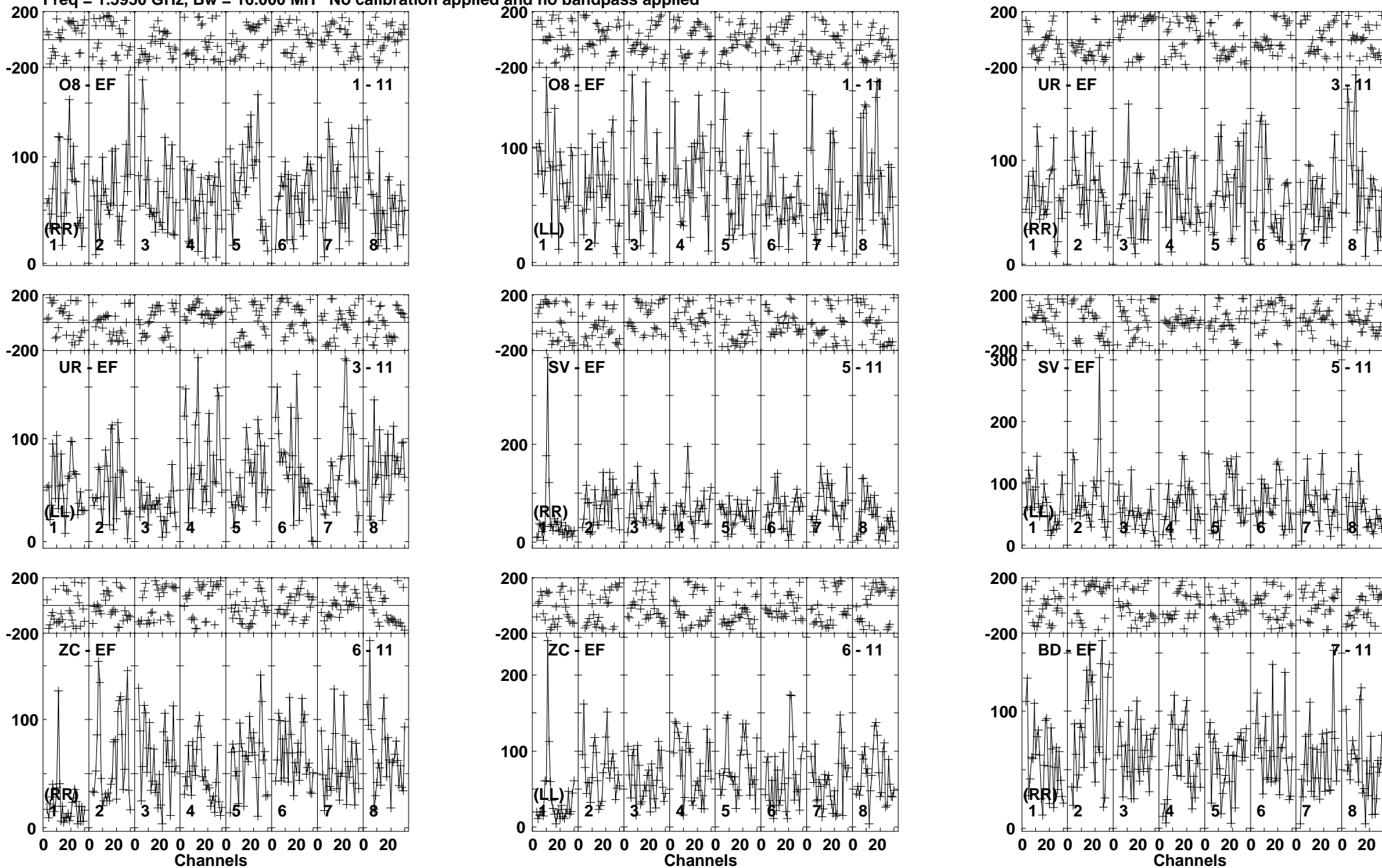
Lower frame: Micro Ampl Jy Top frame: Phas deg Vector averaged cross-power spectrum Baseline: O8 (01) - EF (11) Timerange: 00/04:31:11 to 00/04:34:39
