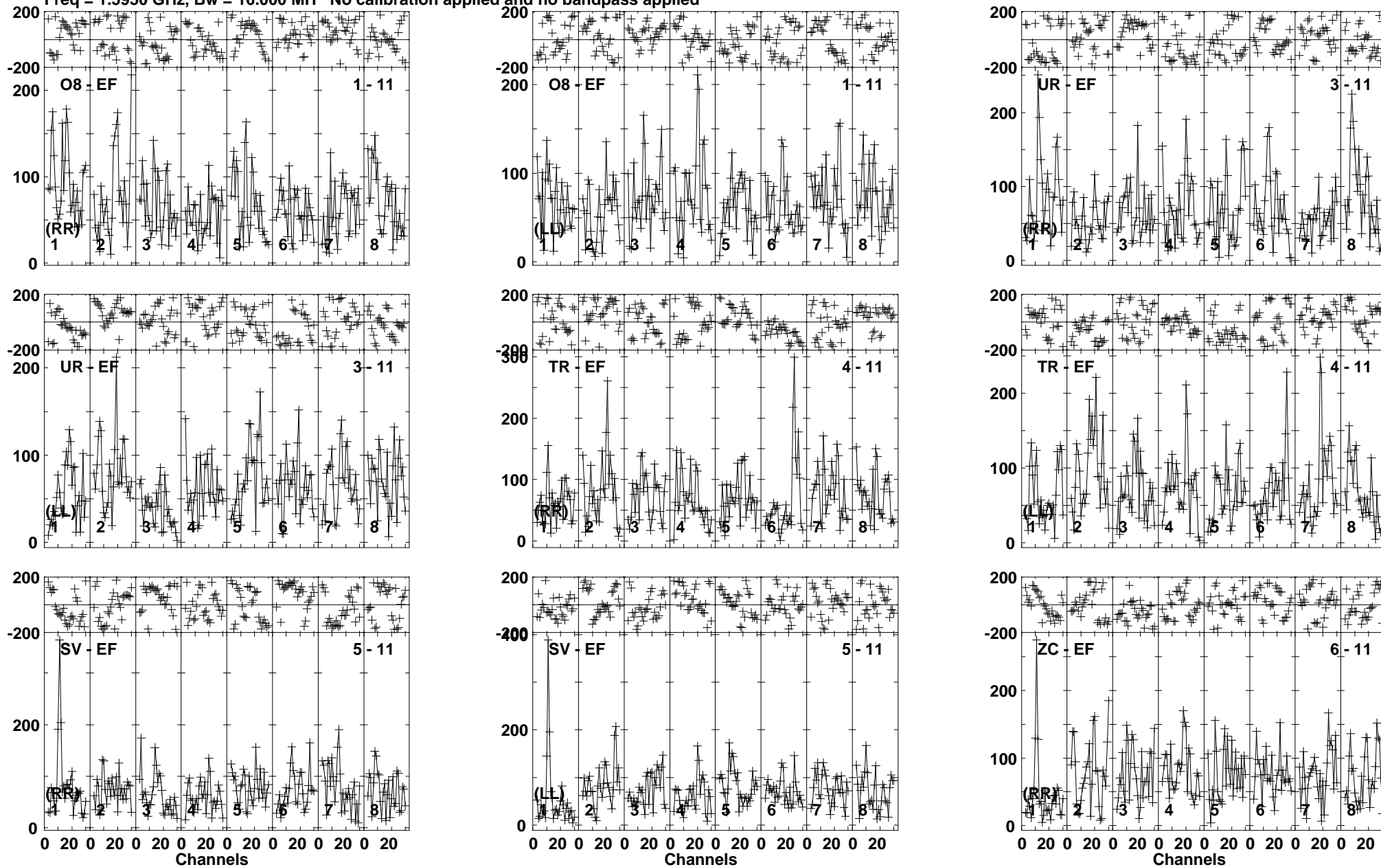
Lower frame: Micro Ampl Jy Top frame: Phas deg Vector averaged cross-power spectrum Baseline: O8 (01) - EF (11) Timerange: 00/10:55:31 to 00/10:58:29
