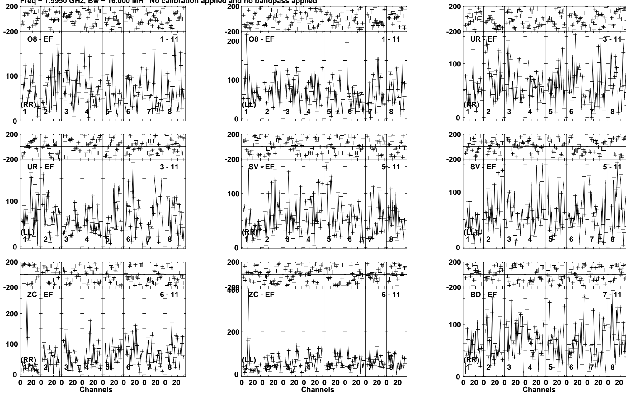
Lower frame: Micro Ampl Jy Top frame: Phas deg Vector averaged cross-power spectrum Baseline: O8 (01) - EF (11) Timerange: 00/08:55:11 to 00/08:58:39
