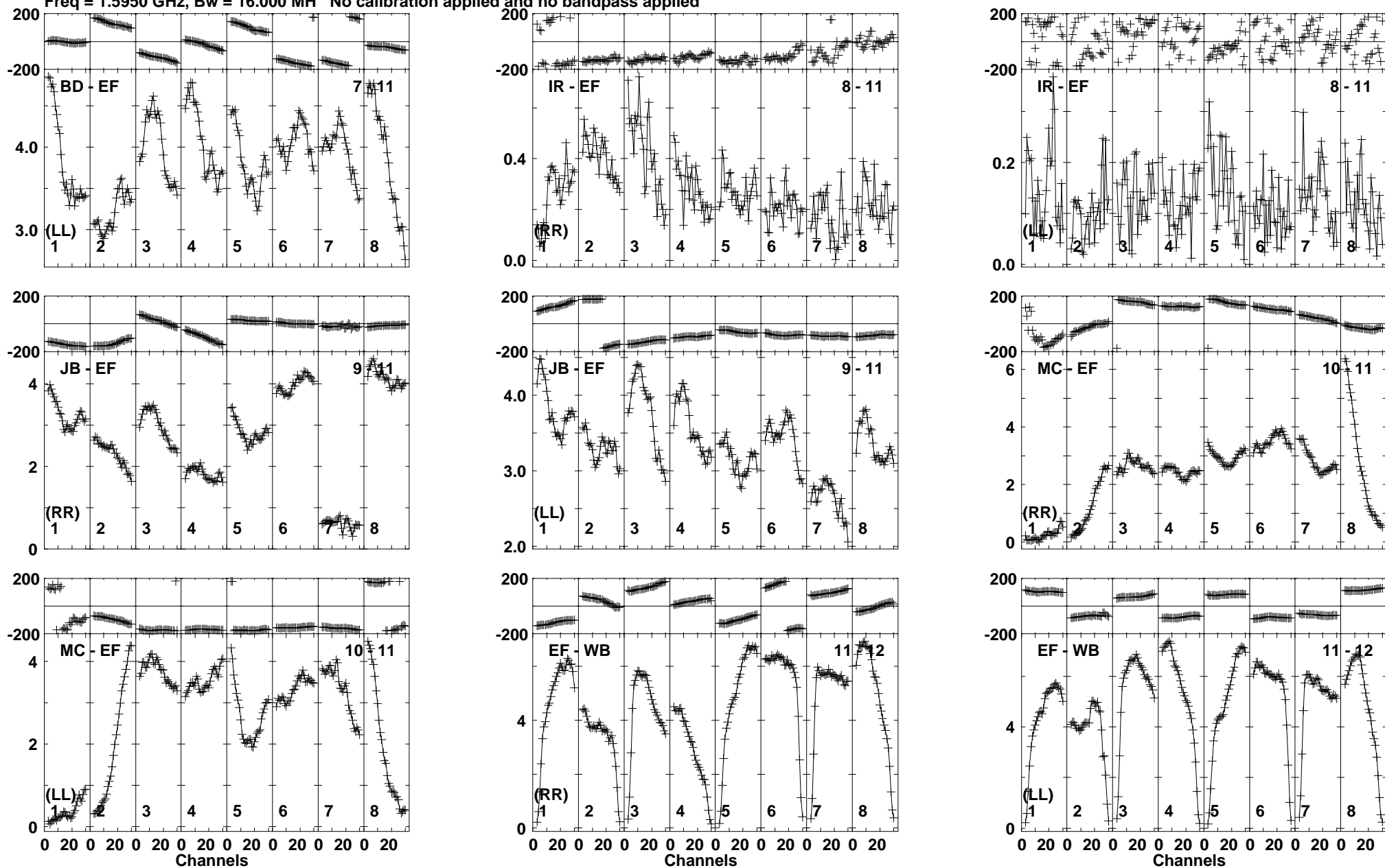
Lower frame: Milli Ampl Jy Top frame: Phas deg Vector averaged cross-power spectrum Baseline: BD (07) - EF (11) Timerange: 00/10:12:01 to 00/10:13:29
