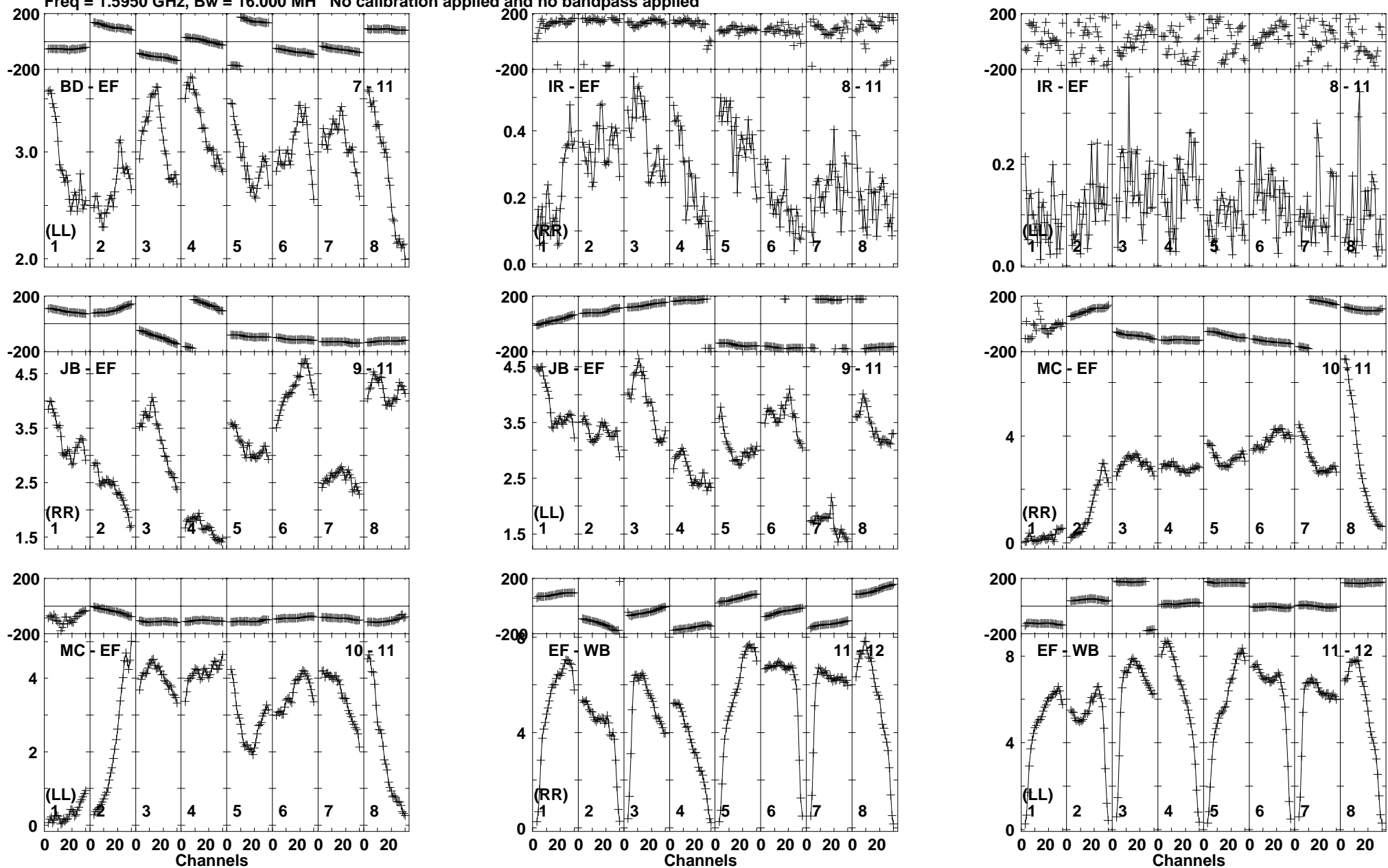
Lower frame: Milli Ampl Jy Top frame: Phas deg Vector averaged cross-power spectrum Baseline: BD (07) - EF (11) Timerange: 00/08:48:41 to 00/08:50:09
