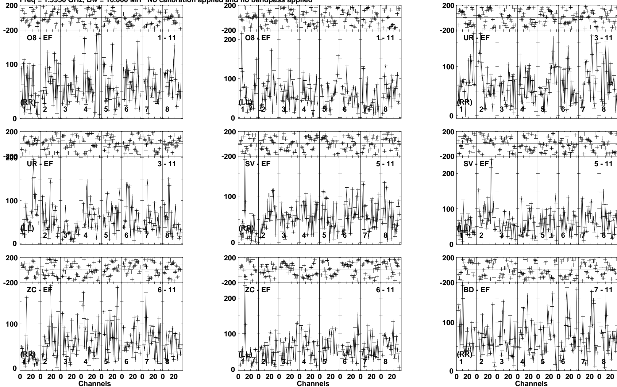
Lower frame: Micro Ampl Jy Top frame: Phas deg Vector averaged cross-power spectrum Baseline: O8 (01) - EF (11) Timerange: 00/04:26:11 to 00/04:29:39
