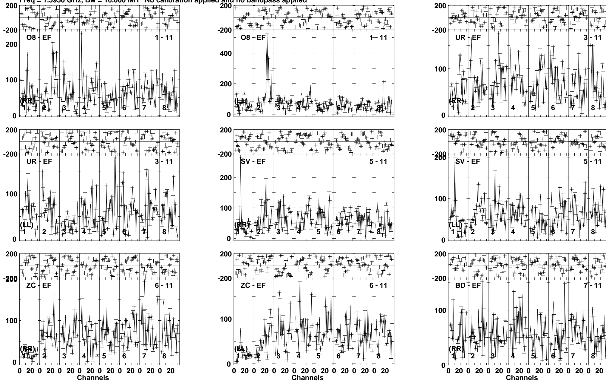
Lower frame: Micro Ampl Jy Top frame: Phas deg Vector averaged cross-power spectrum Baseline: O8 (01) - EF (11) Timerange: 00/08:39:31 to 00/08:42:59
