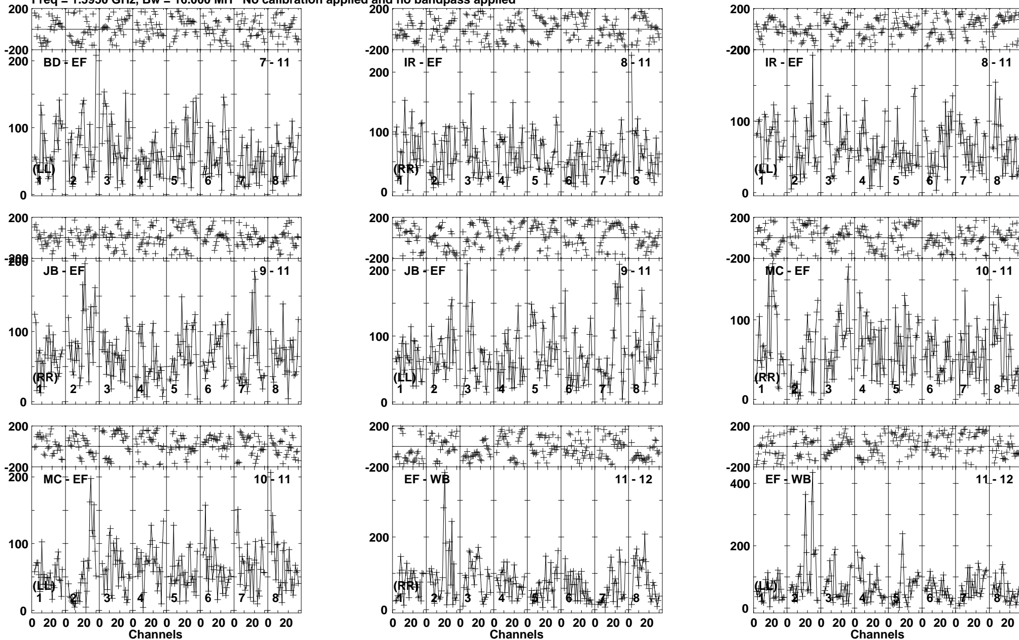
Lower frame: Micro Ampl Jy Top frame: Phas deg Vector averaged cross-power spectrum Baseline: BD (07) - EF (11) Timerange: 00/05:06:21 to 00/05:09:49
