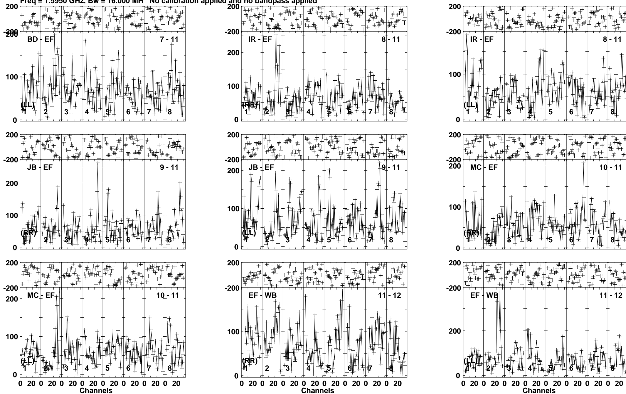
Lower frame: Micro Ampl Jy Top frame: Phas deg Vector averaged cross-power spectrum Baseline: BD (07) - EF (11) Timerange: 00/08:34:31 to 00/08:37:59
