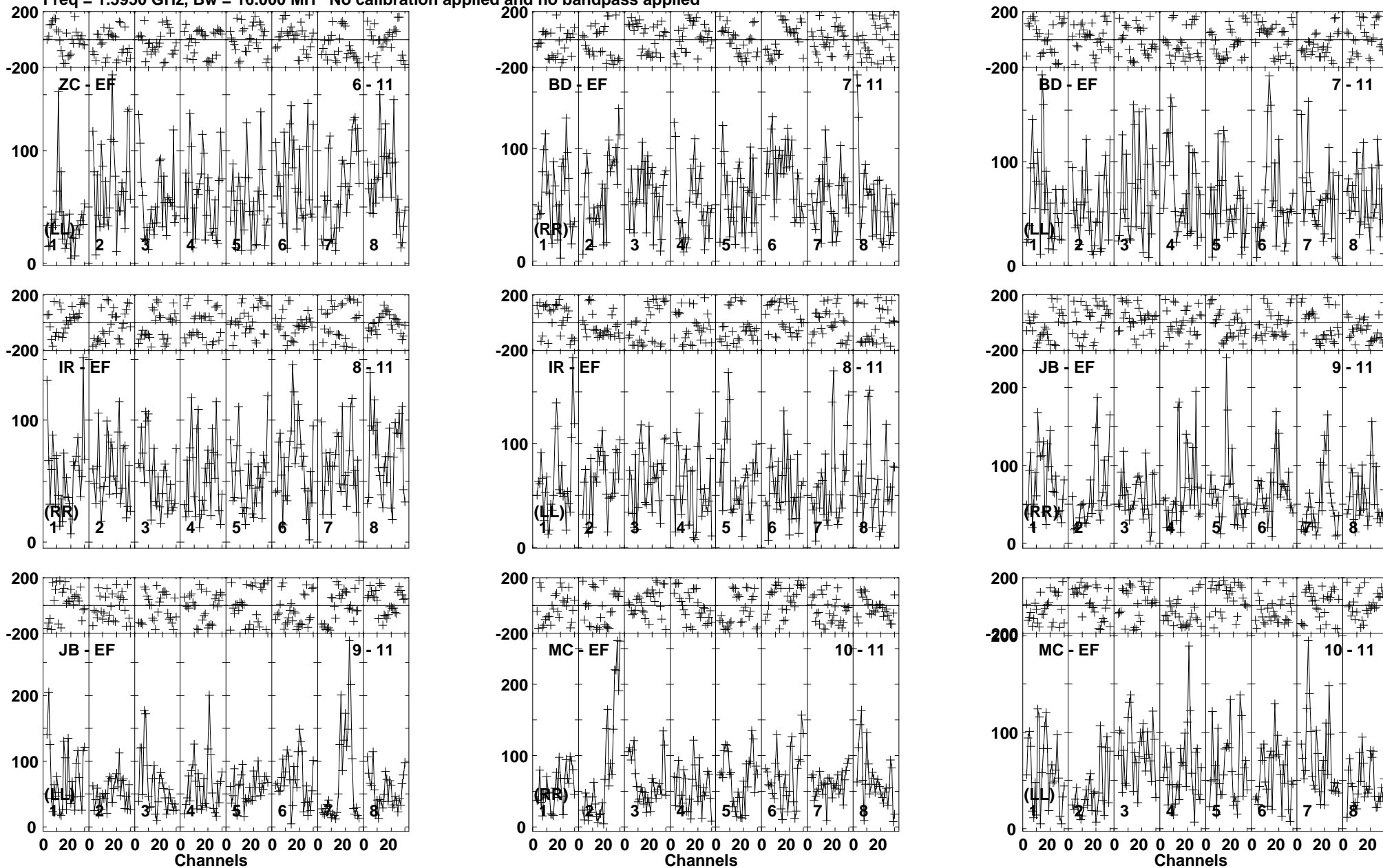
Lower frame: Micro Ampl Jy Top frame: Phas deg Vector averaged cross-power spectrum Baseline: ZC (06) - EF (11) Timerange: 00/10:44:51 to 00/10:48:19
