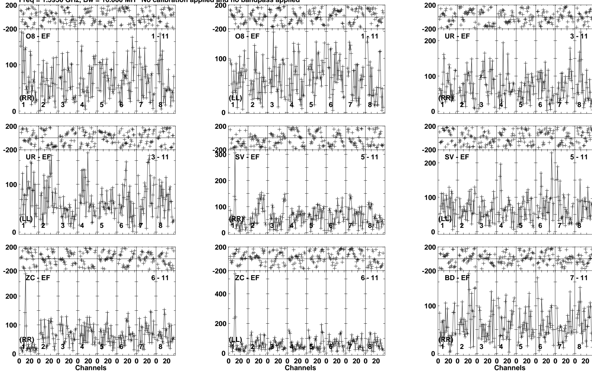
Lower frame: Micro Ampl Jy Top frame: Phas deg Vector averaged cross-power spectrum Baseline: O8 (01) - EF (11) Timerange: 00/04:46:41 to 00/04:50:09
