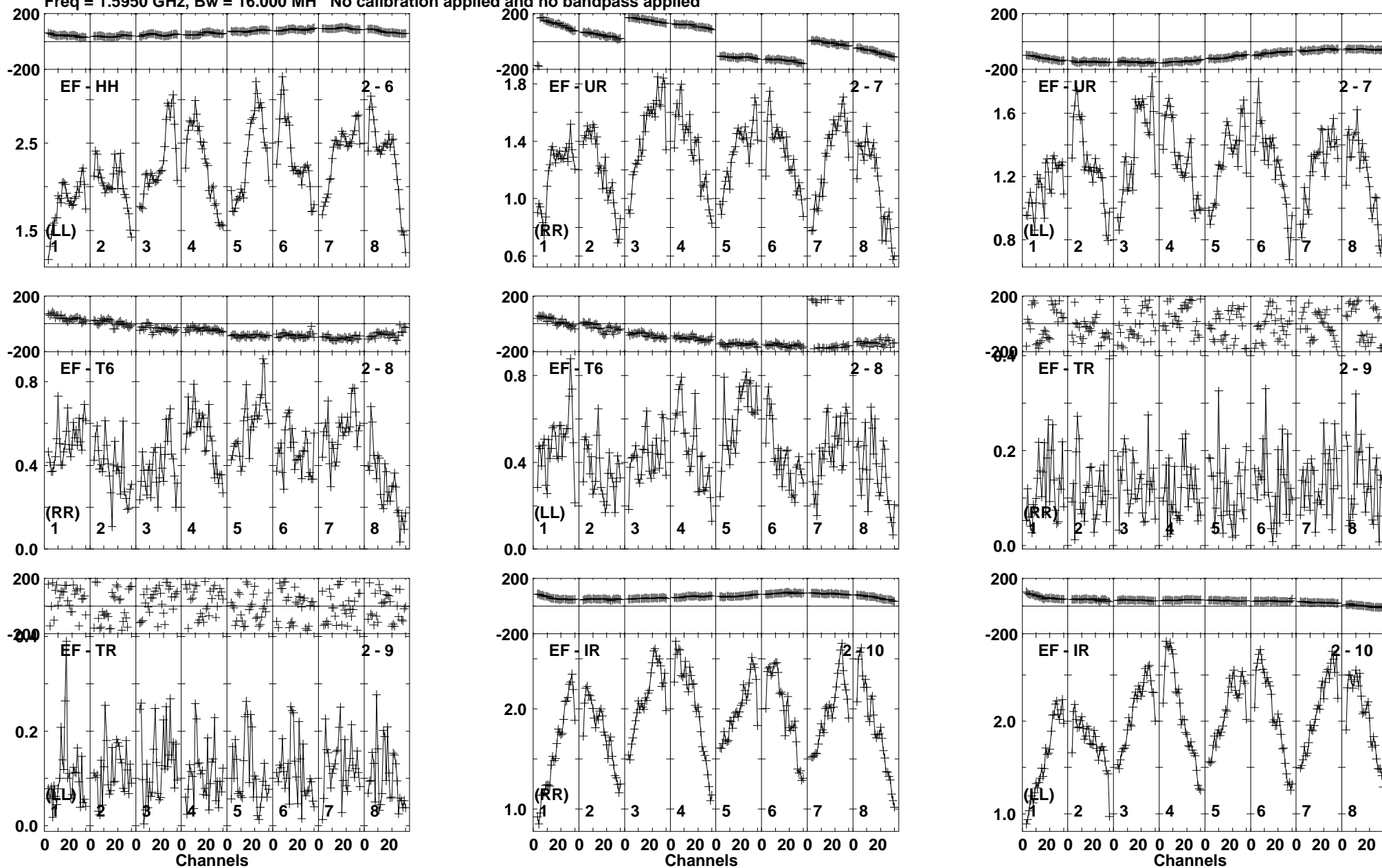
Lower frame: Milli Ampl Jy Top frame: Phas deg Vector averaged cross-power spectrum Baseline: EF (02) - HH (06) Timerange: 00/21:58:36 to 00/21:59:54
