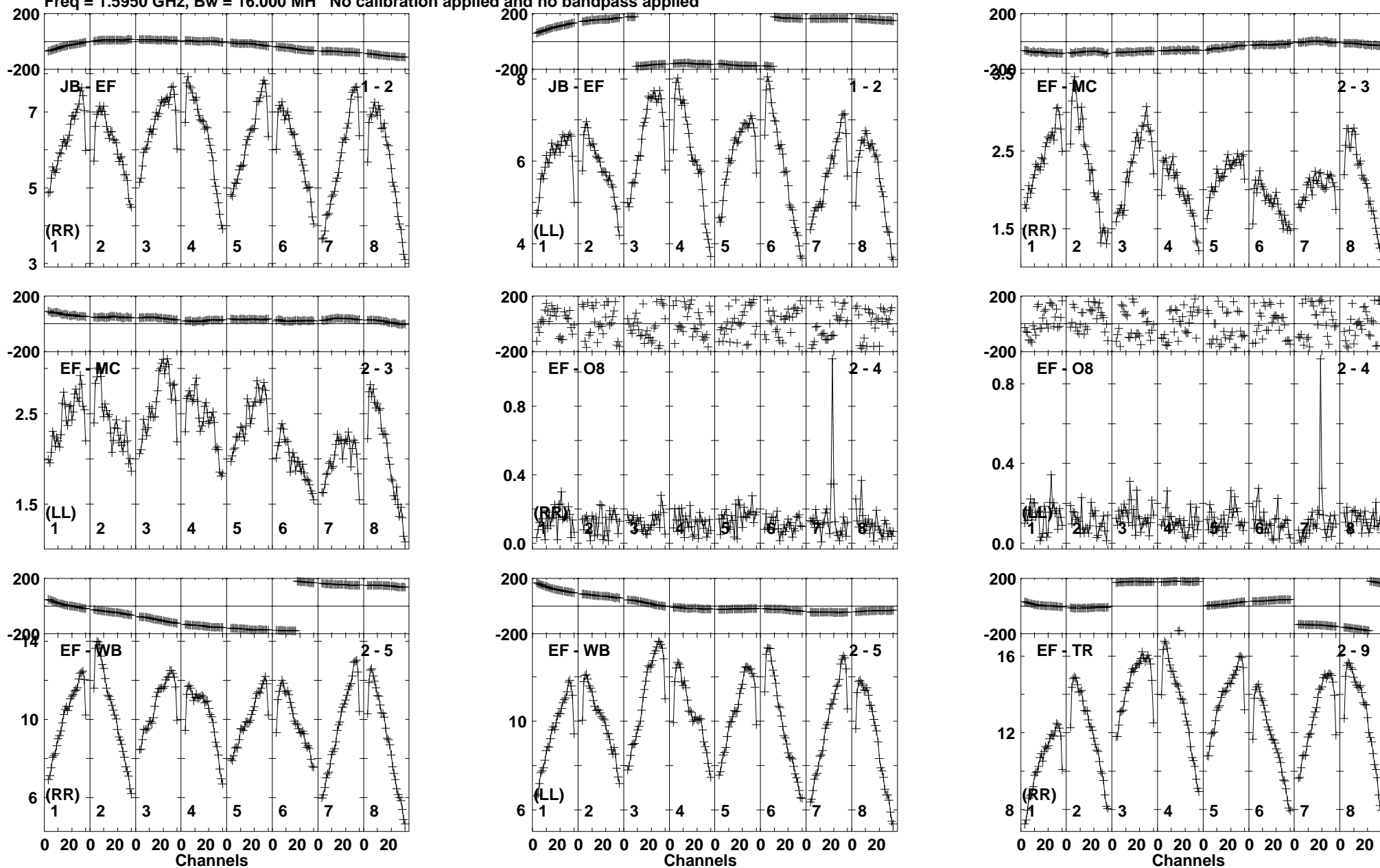
Lower frame: Milli Ampl Jy Top frame: Phas deg Vector averaged cross-power spectrum Baseline: JB (01) - EF (02) Timerange: 00/21:30:11 to 00/21:31:29
