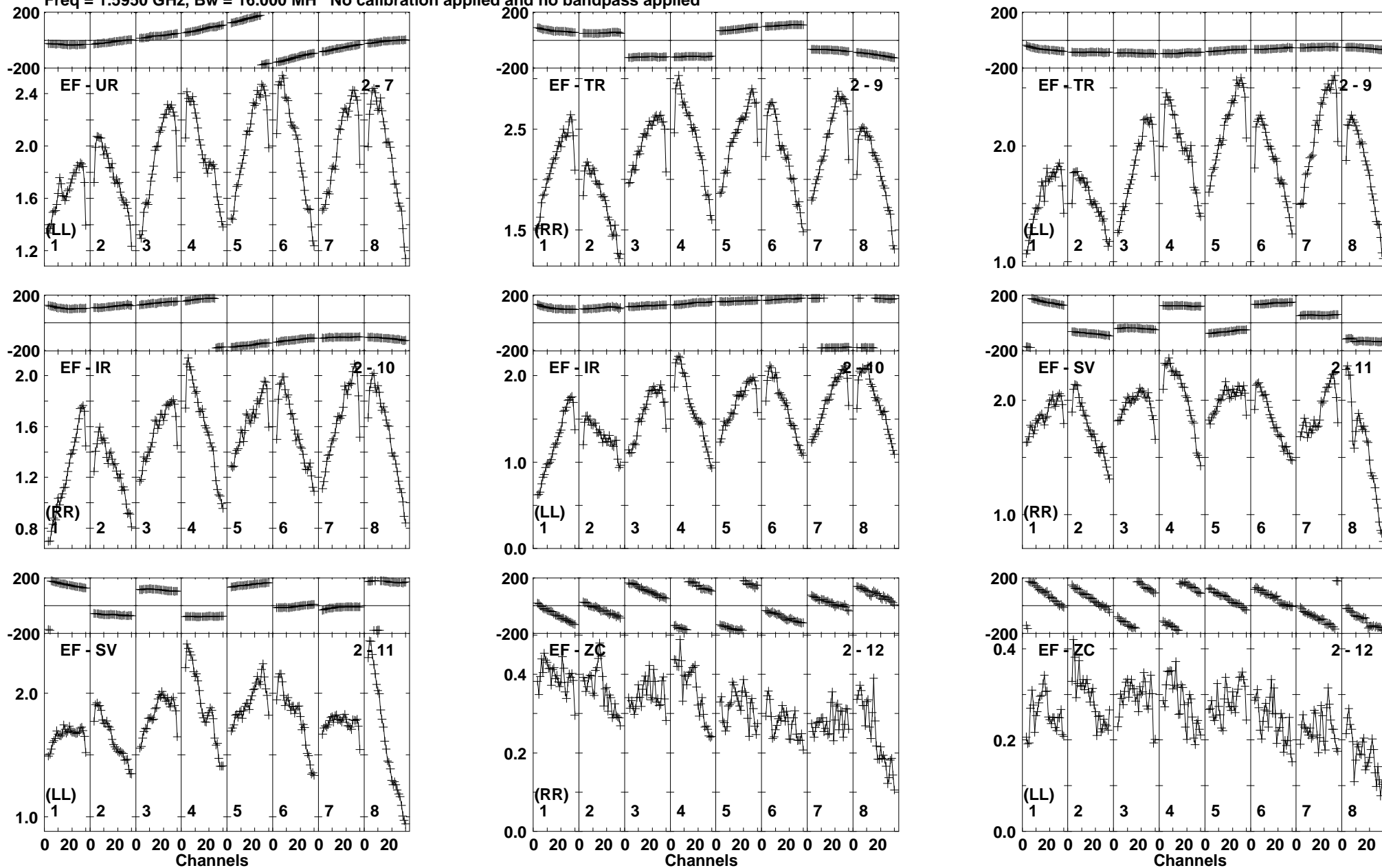
Lower frame: Milli Ampl Jy Top frame: Phas deg Vector averaged cross-power spectrum Baseline: EF (02) - UR (07) Timerange: 00/16:39:36 to 00/16:48:14
