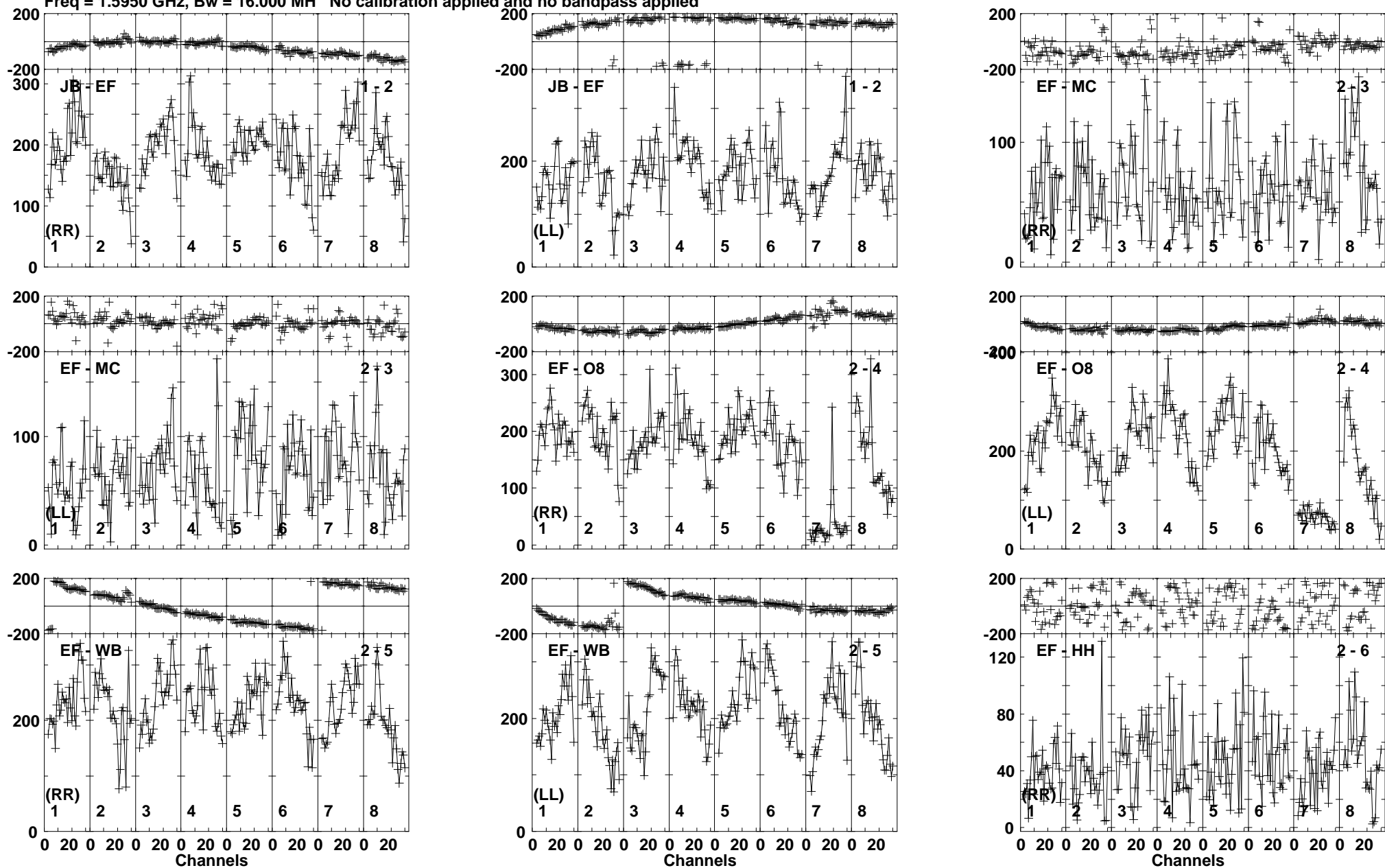
Lower frame: Micro Ampl Jy Top frame: Phas deg Vector averaged cross-power spectrum Baseline: JB (01) - EF (02) Timerange: 00:18:13:51 to 00:18:22:29
