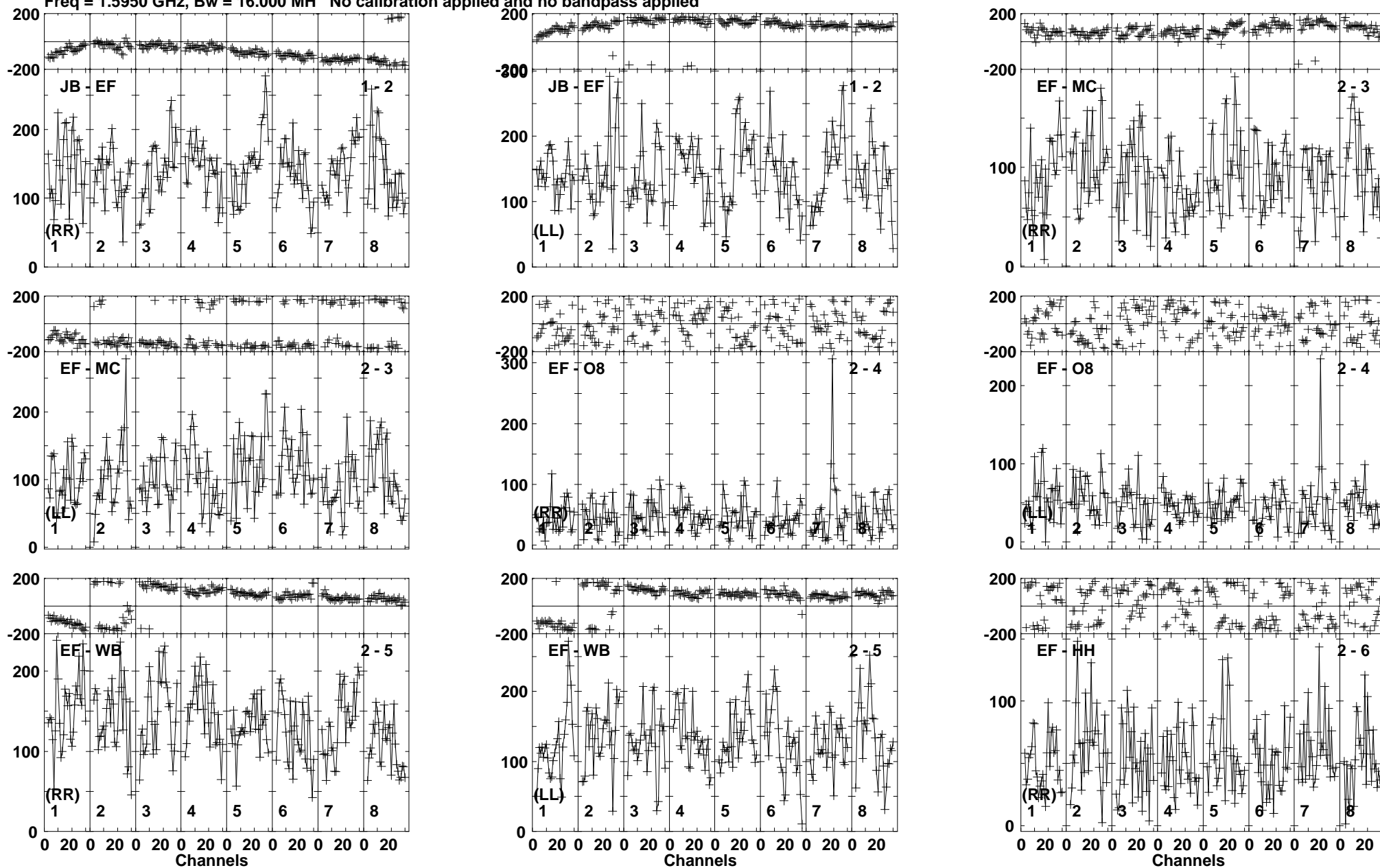
Lower frame: Micro Ampl Jy Top frame: Phas deg Vector averaged cross-power spectrum Baseline: JB (01) - EF (02) Timerange: 00/21:50:01 to 00/21:57:43
