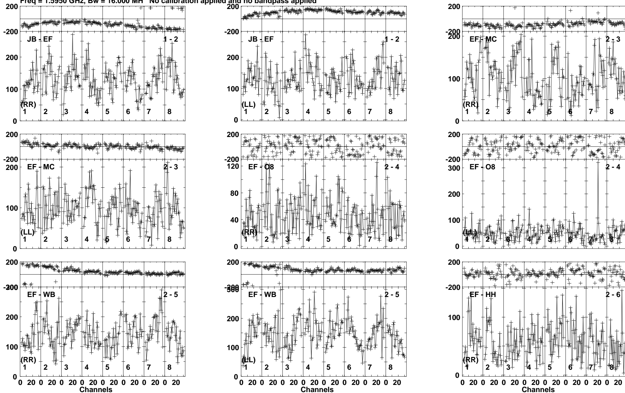
Lower frame: Micro Ampl Jy Top frame: Phas deg Vector averaged cross-power spectrum Baseline: JB (01) - EF (02) Timerange: 00/23:05:16 to 00/23:12:58
