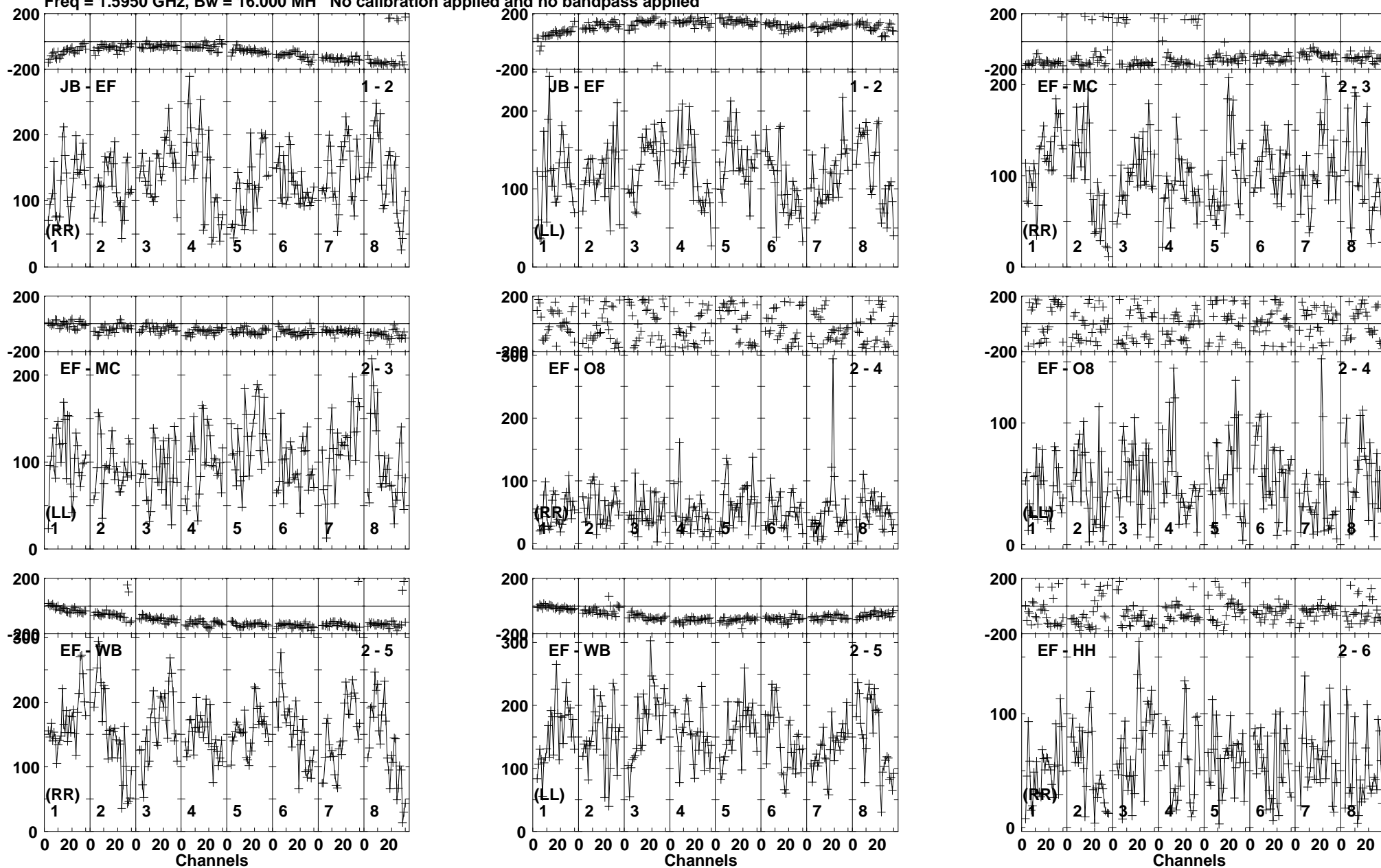
Lower frame: Micro Ampl Jy Top frame: Phas deg Vector averaged cross-power spectrum Baseline: JB (01) - EF (02) Timerange: 00/23:26:46 to 00/23:34:28
