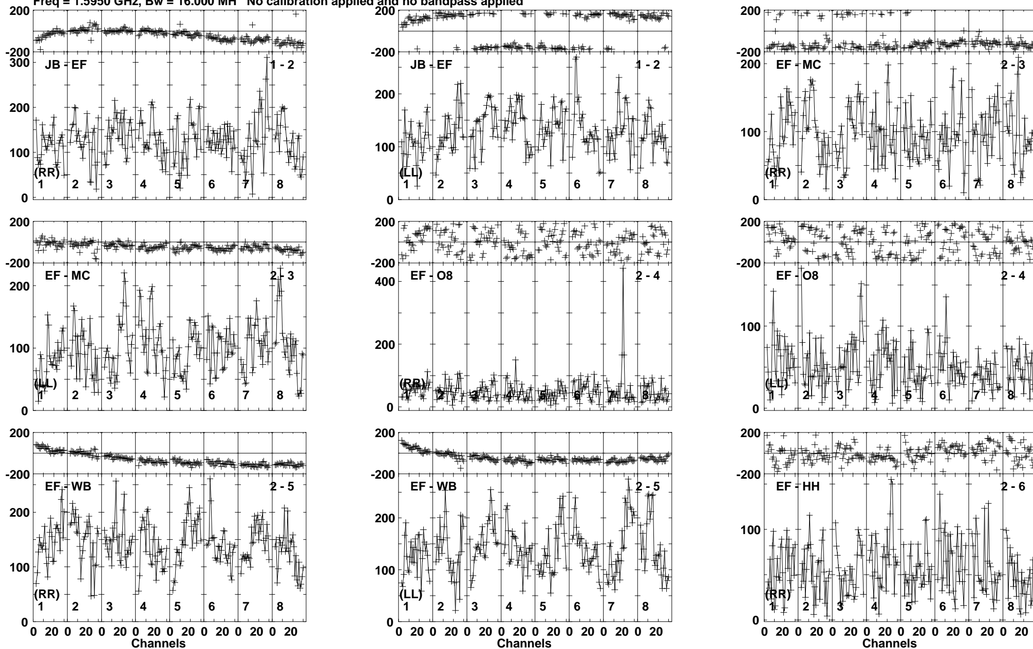
Lower frame: Micro Ampl Jy Top frame: Phas deg Vector averaged cross-power spectrum Baseline: JB (01) - EF (02) Timerange: 00/22:54:31 to 00/23:02:13
