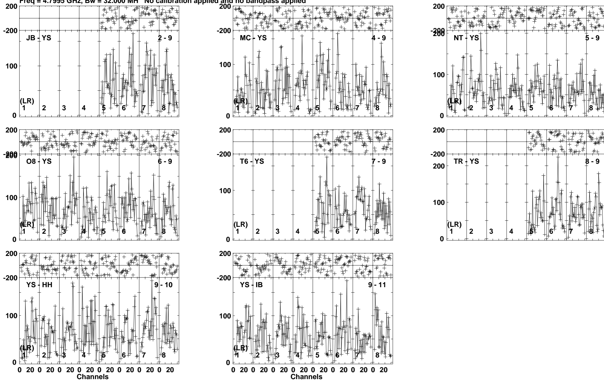
Lower frame: Micro Ampl Jy Top frame: Phas deg Vector averaged cross-power spectrum Baseline: JB (02) - YS (09) Timerange: 00/16:25:51 to 00/16:29:19
