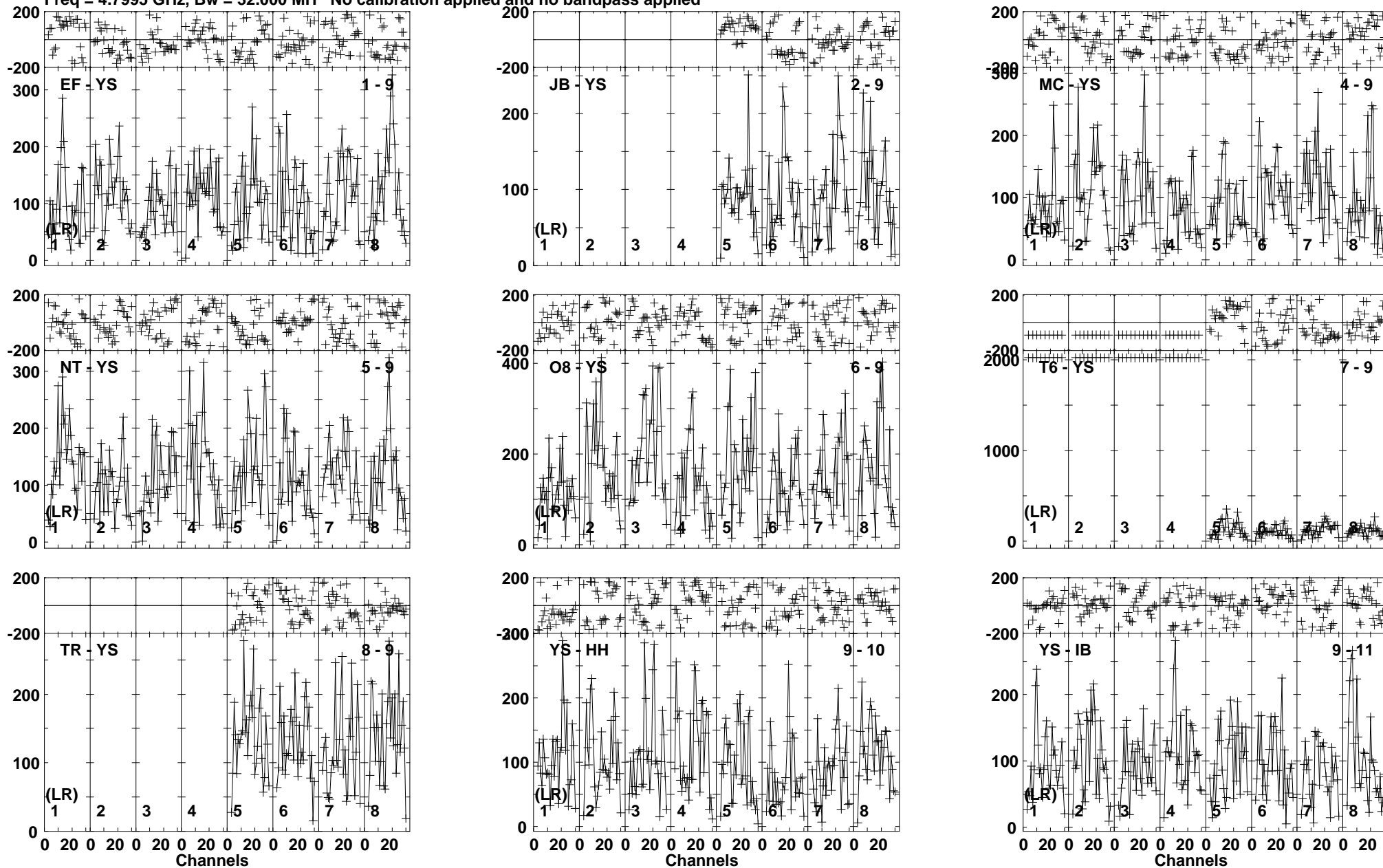
Lower frame: Micro Ampl Jy Top frame: Phas deg Vector averaged cross-power spectrum Baseline: EF (01) - YS (09) Timerange: 00/15:34:21 to 00/15:35:19
