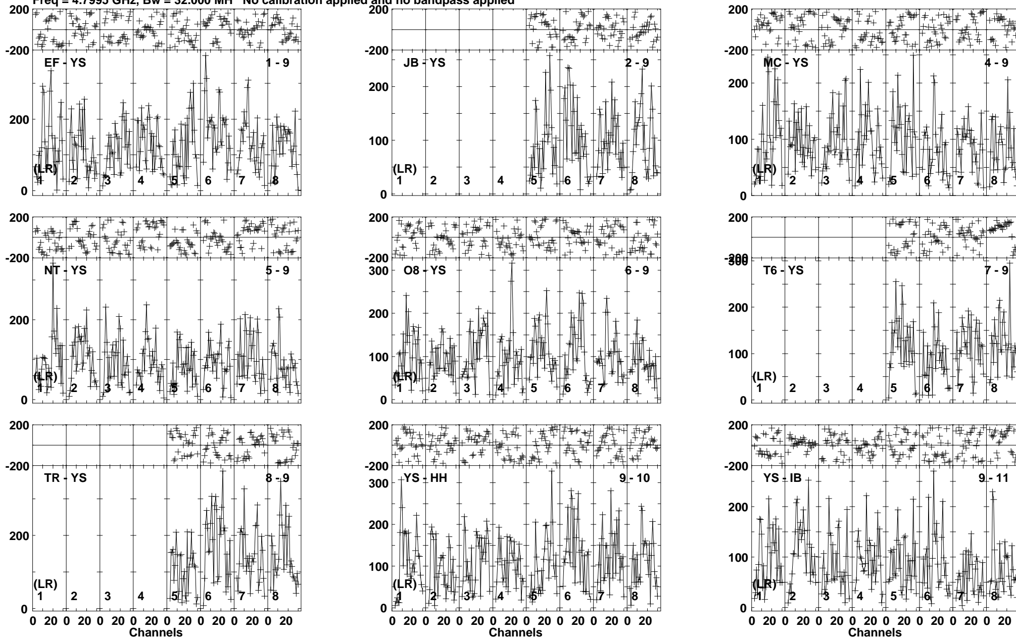
Lower frame: Micro Ampl Jy Top frame: Phas deg Vector averaged cross-power spectrum Baseline: EF (01) - YS (09) Timerange: 00/14:43:11 to 00/14:44:39
