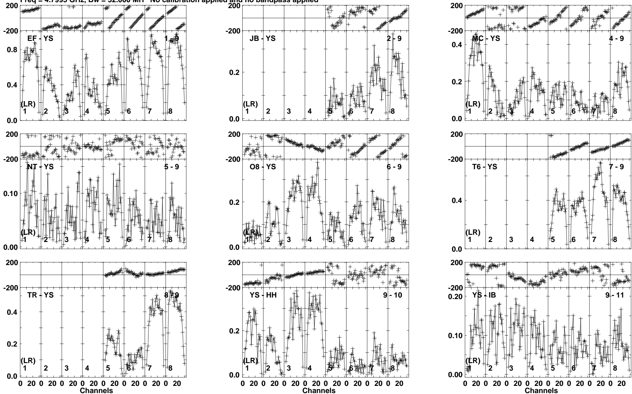
Lower frame: Milli Ampl Jy Top frame: Phas deg Vector averaged cross-power spectrum Baseline: EF (01) - YS (09) Timerange: 00/13:55:07 to 00/13:59:59
