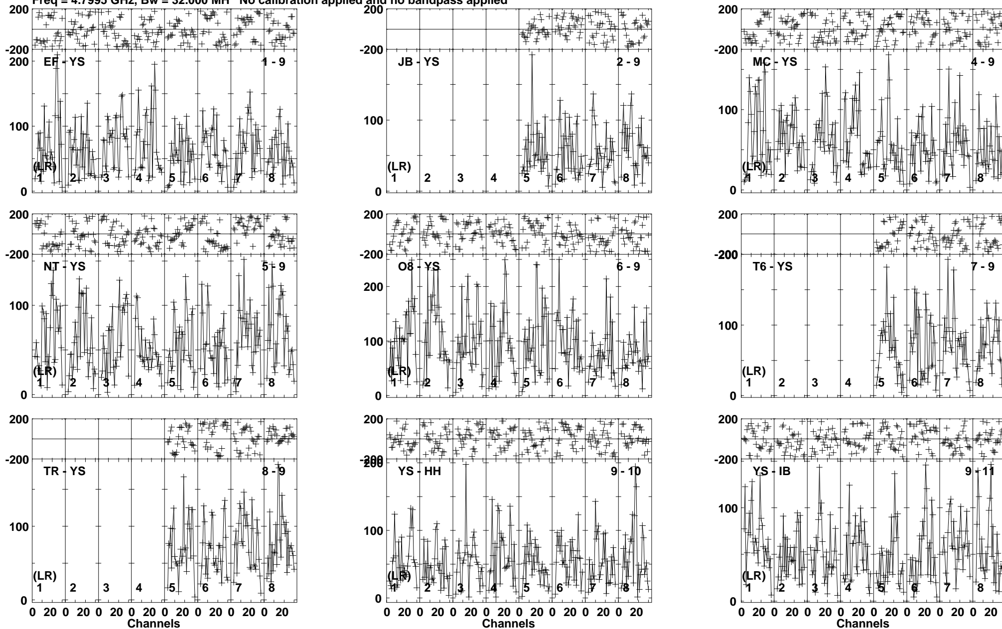
Lower frame: Micro Ampl Jy Top frame: Phas deg Vector averaged cross-power spectrum Baseline: EF (01) - YS (09) Timerange: 00/14:54:51 to 00/14:58:19
