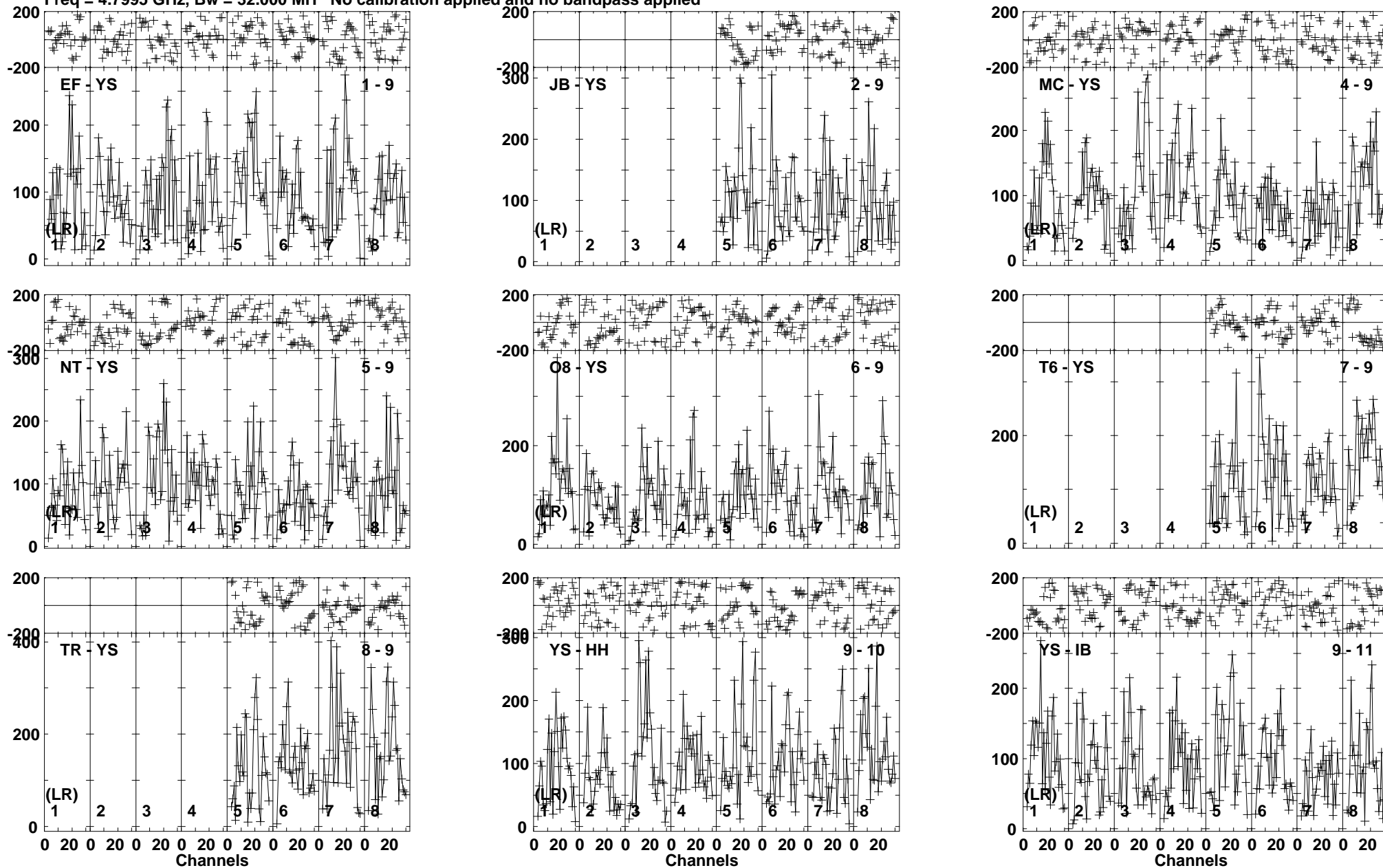
Lower frame: Micro Ampl Jy Top frame: Phas deg Vector averaged cross-power spectrum Baseline: EF (01) - YS (09) Timerange: 00/15:23:41 to 00/15:25:09
