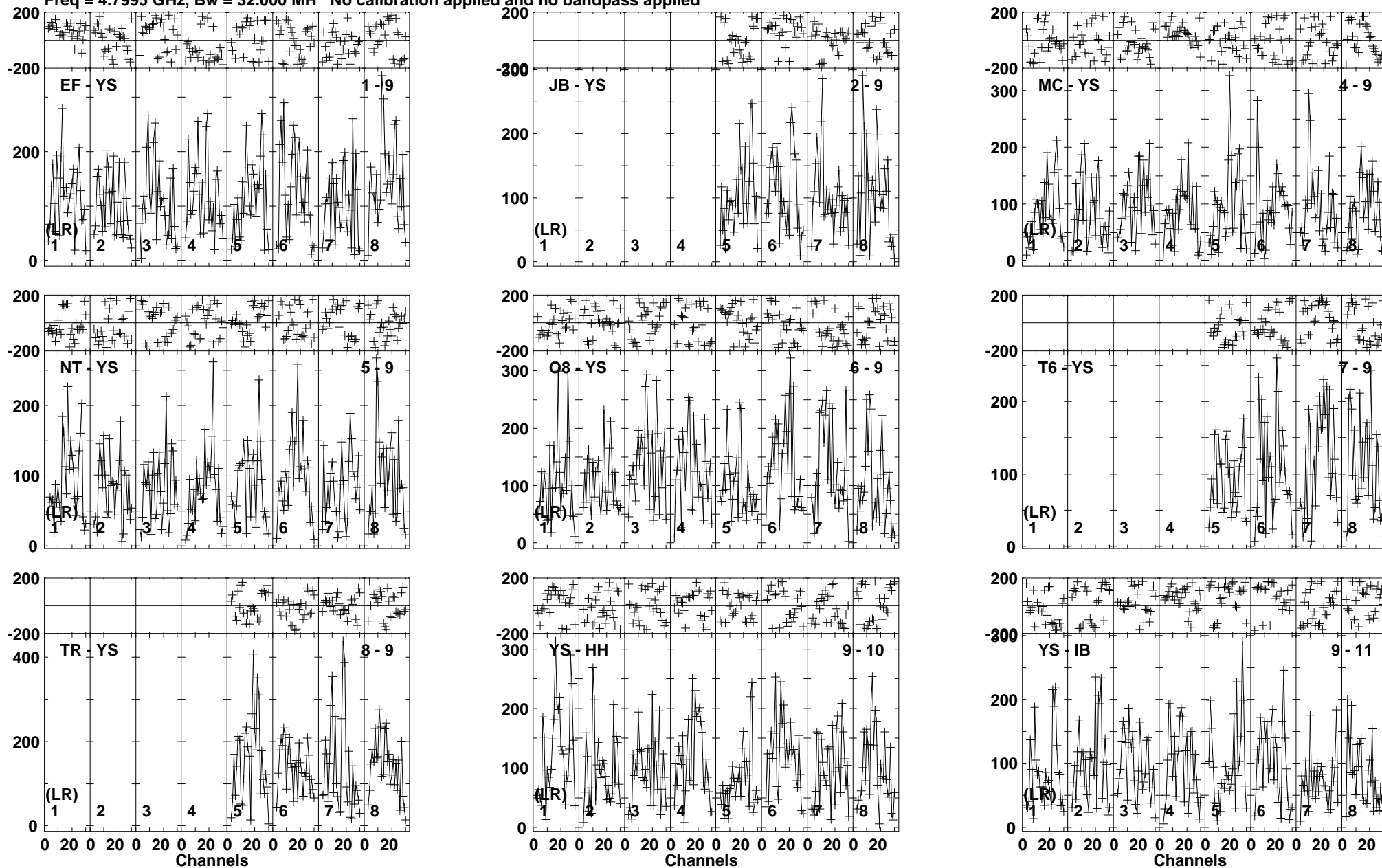
Lower frame: Micro Ampl Jy Top frame: Phas deg Vector averaged cross-power spectrum Baseline: EF (01) - YS (09) Timerange: 00/15:08:31 to 00/15:09:59
