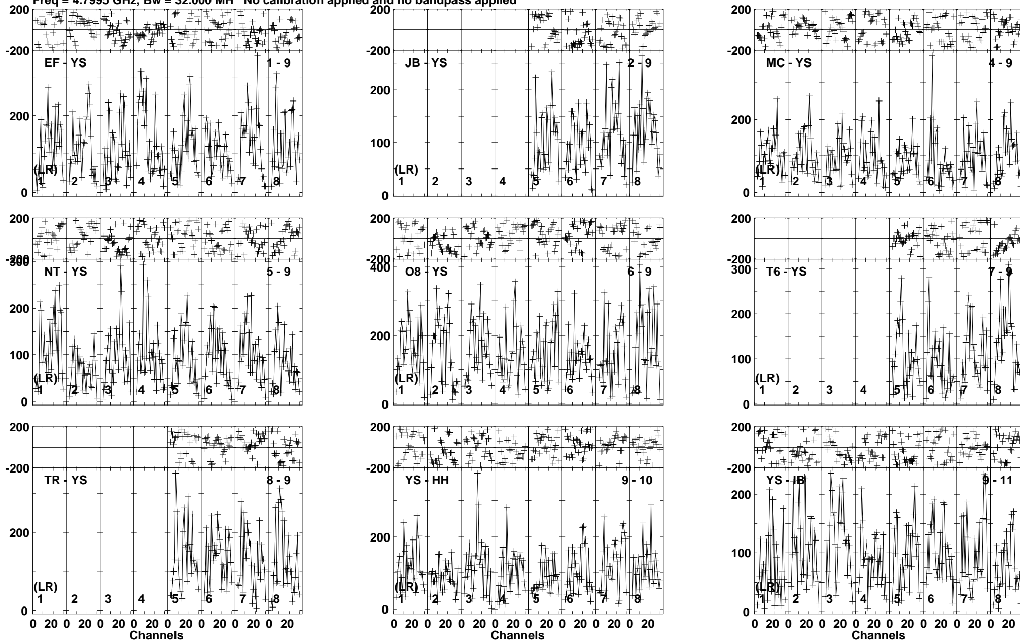
Lower frame: Micro Ampl Jy Top frame: Phas deg Vector averaged cross-power spectrum Baseline: EF (01) - YS (09) Timerange: 00/14:23:01 to 00/14:24:29
