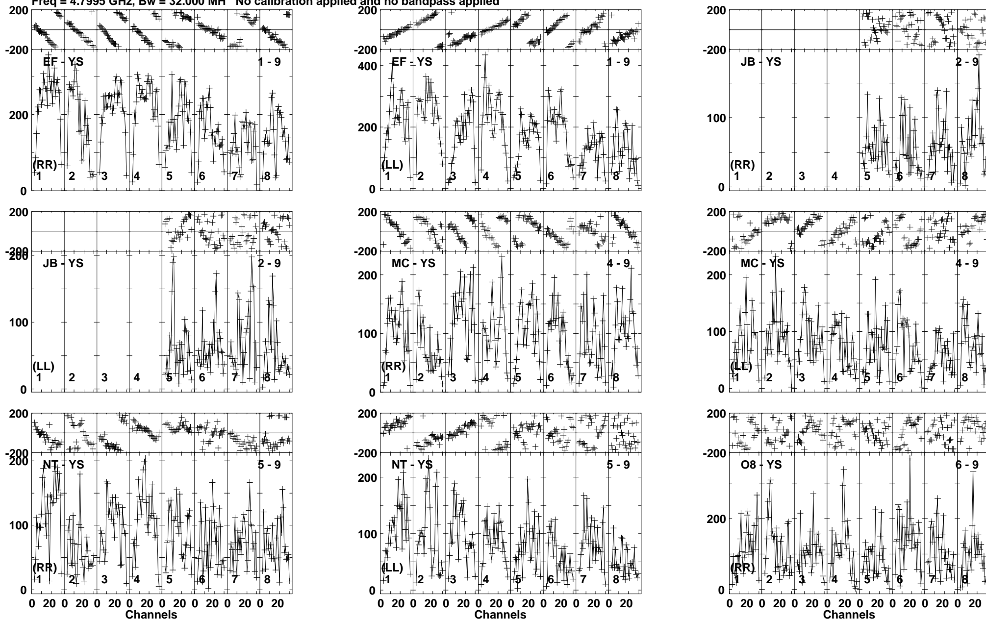
Lower frame: Micro Ampl Jy Top frame: Phas deg Vector averaged cross-power spectrum Baseline: EF (01) - YS (09) Timerange: 00/14:34:41 to 00/14:38:09
