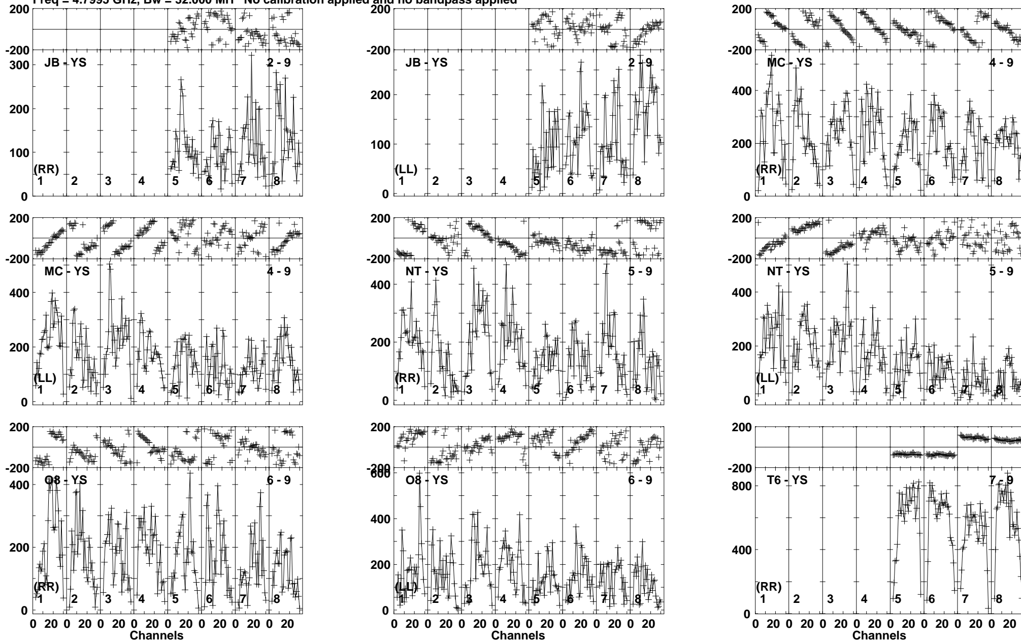
Lower frame: Micro Ampl Jy Top frame: Phas deg Vector averaged cross-power spectrum Baseline: JB (02) - YS (09) Timerange: 00/16:14:11 to 00/16:15:39
