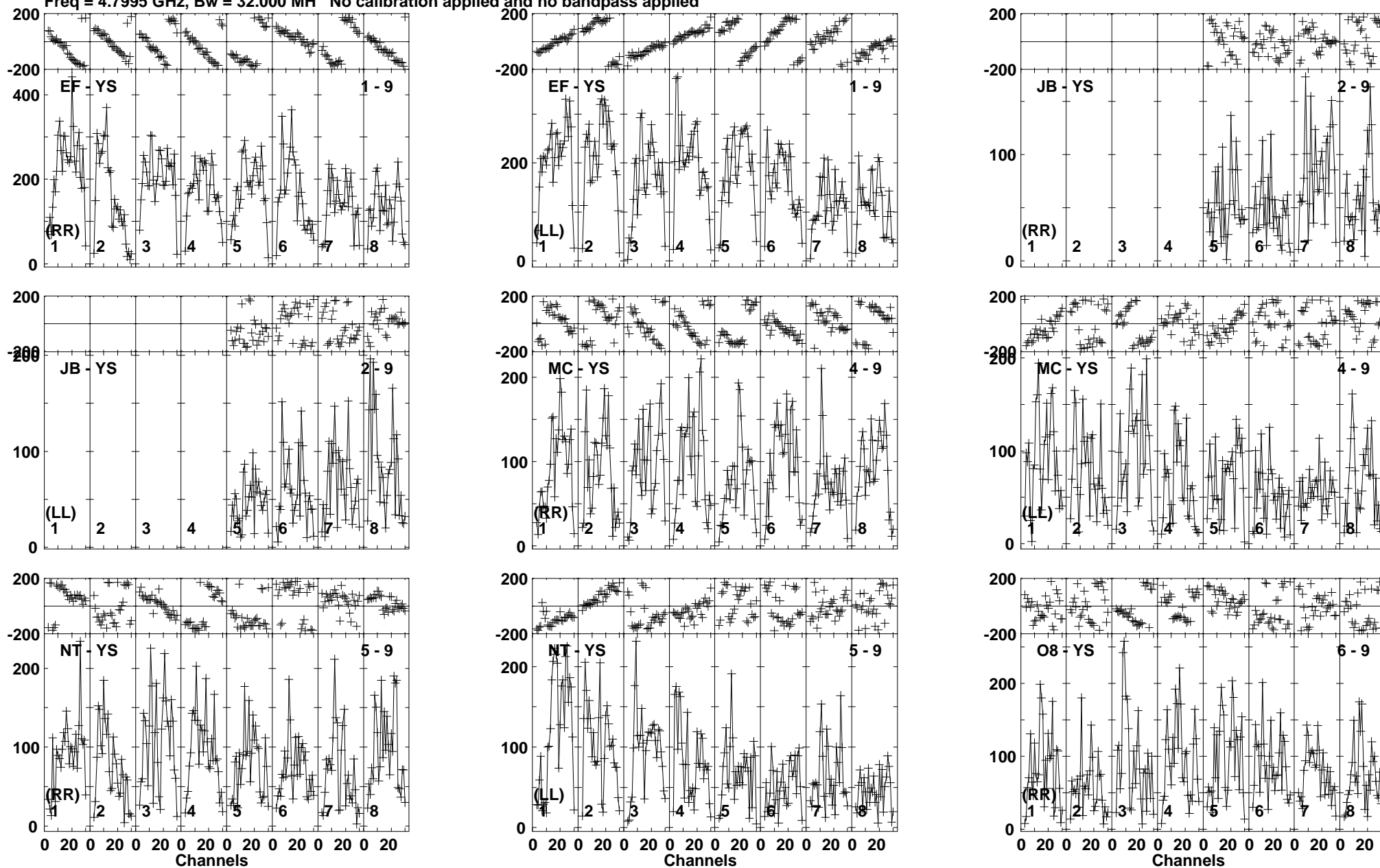
Lower frame: Micro Ampl Jy Top frame: Phas deg Vector averaged cross-power spectrum Baseline: EF (01) - YS (09) Timerange: 00/14:29:31 to 00/14:32:59
