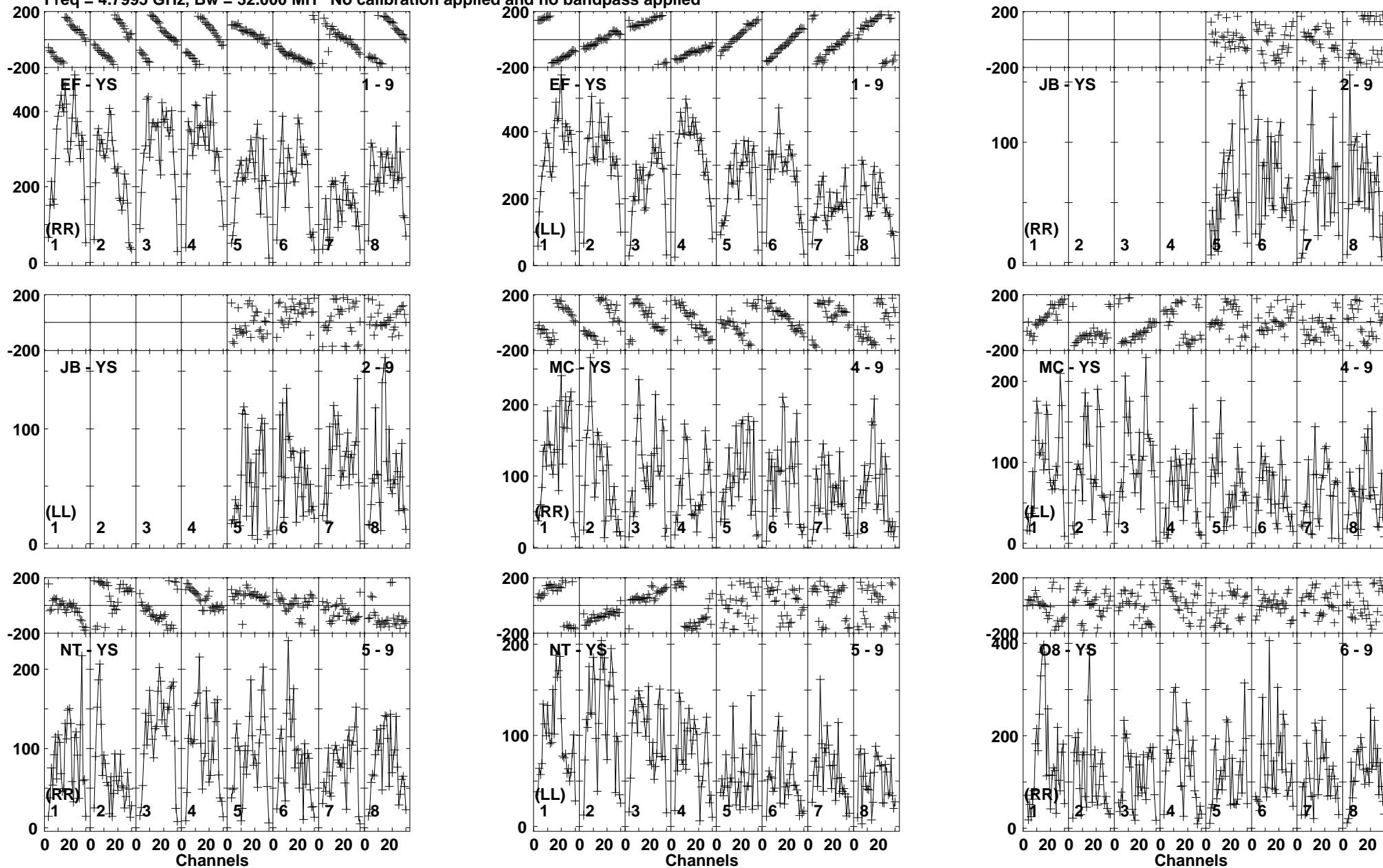
Lower frame: Micro Ampl Jy Top frame: Phas deg Vector averaged cross-power spectrum Baseline: EF (01) - YS (09) Timerange: 00/14:49:51 to 00/14:53:19
