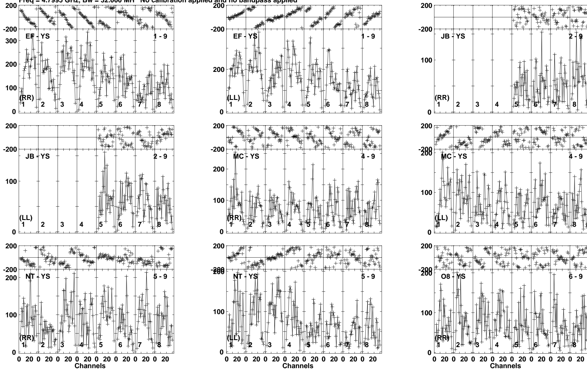
Lower frame: Micro Ampl Jy Top frame: Phas deg Vector averaged cross-power spectrum Baseline: EF (01) - YS (09) Timerange: 00/14:24:31 to 00/14:27:59
