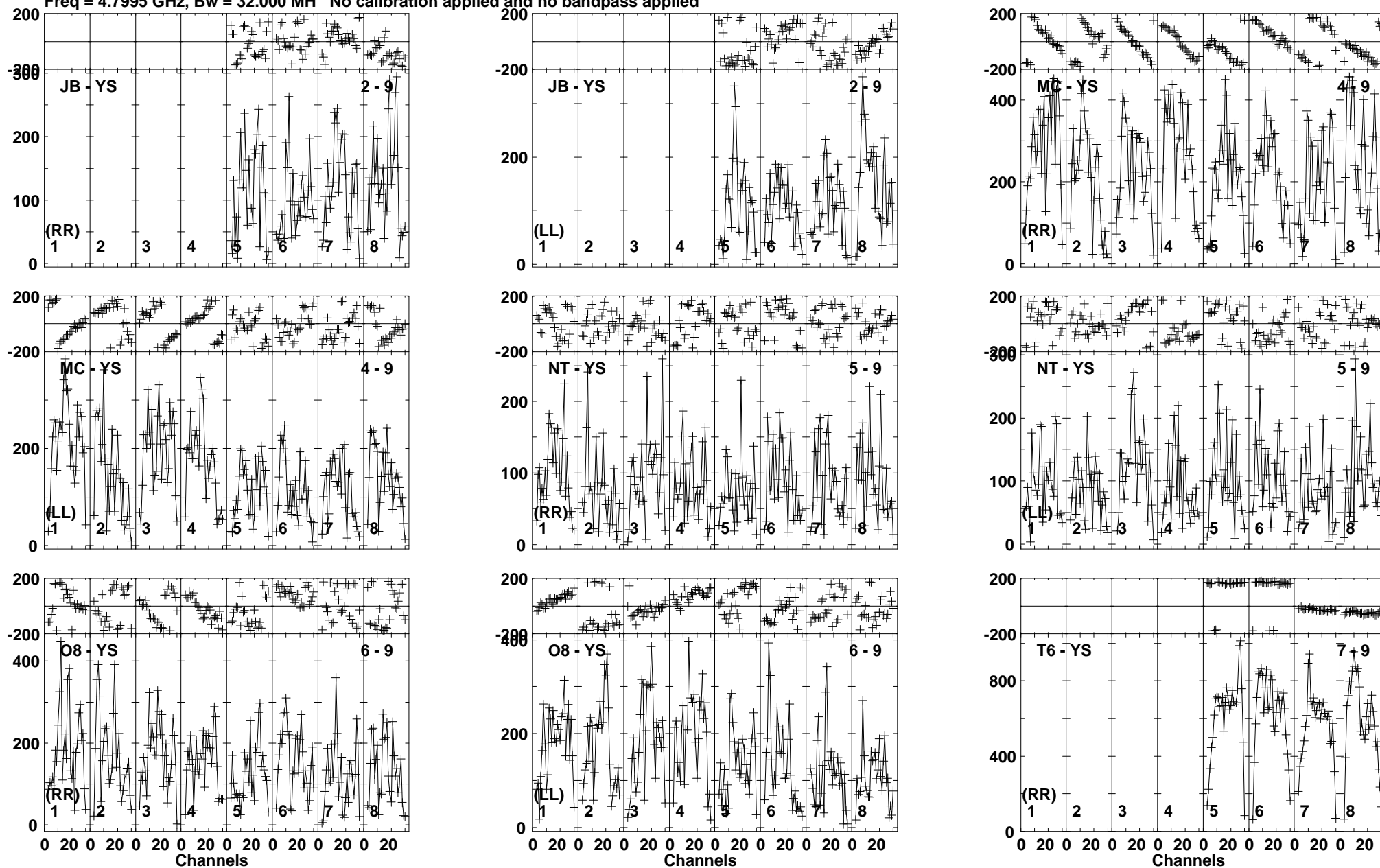
Lower frame: Micro Ampl Jy Top frame: Phas deg Vector averaged cross-power spectrum Baseline: JB (02) - YS (09) Timerange: 00/16:09:11 to 00/16:10:39
