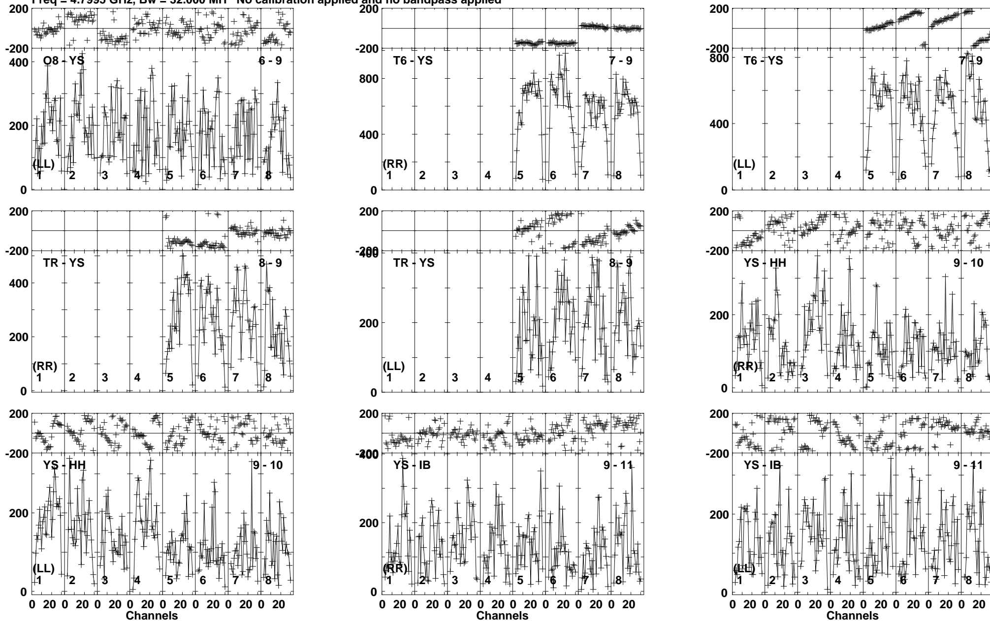
Lower frame: Micro Ampl Jy Top frame: Phas deg Vector averaged cross-power spectrum Baseline: O8 (06) - YS (09) Timerange: 00/15:04:01 to 00/15:04:59
