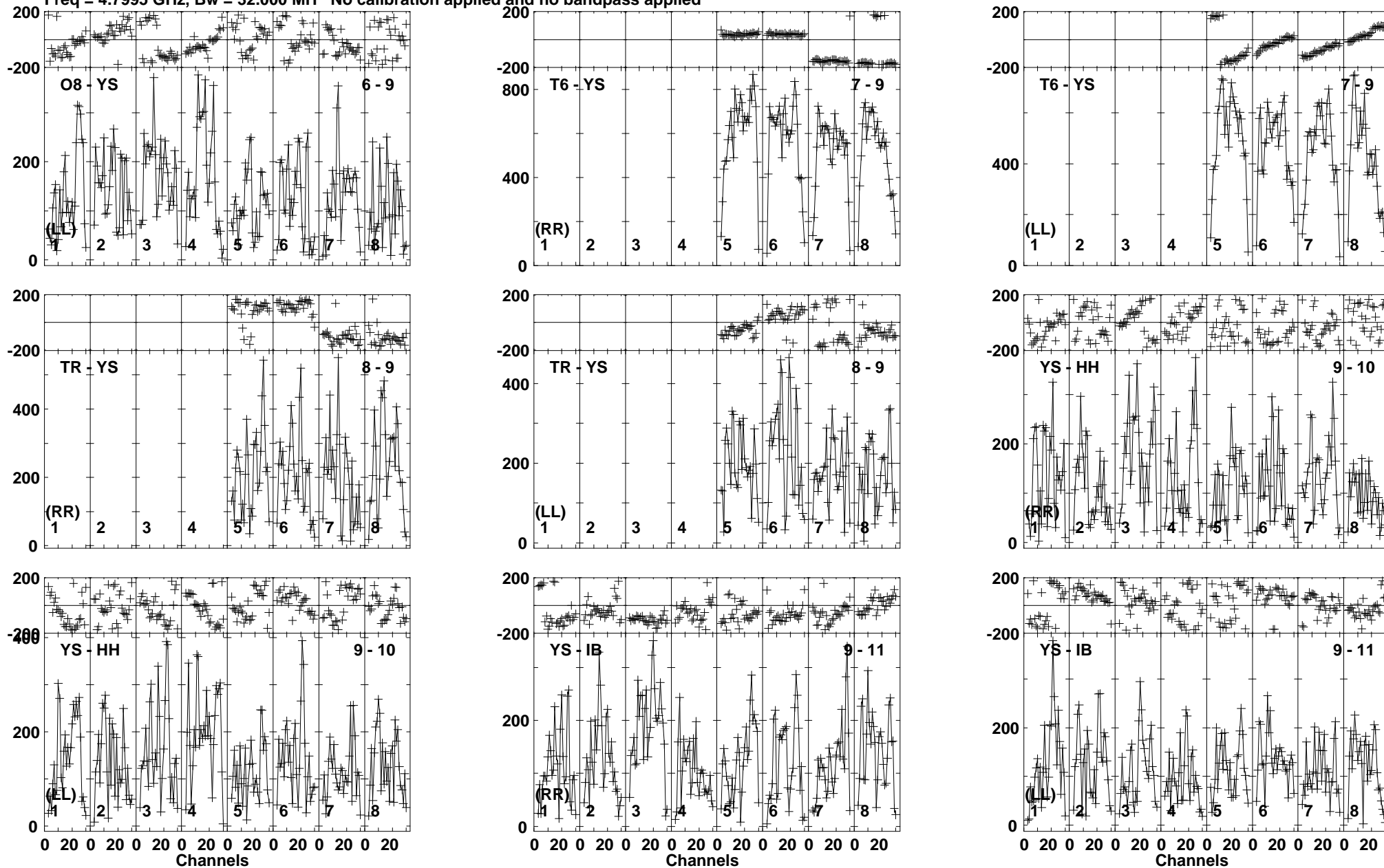
Lower frame: Micro Ampl Jy Top frame: Phas deg Vector averaged cross-power spectrum Baseline: O8 (06) - YS (09) Timerange: 00/14:58:21 to 00/14:59:49
