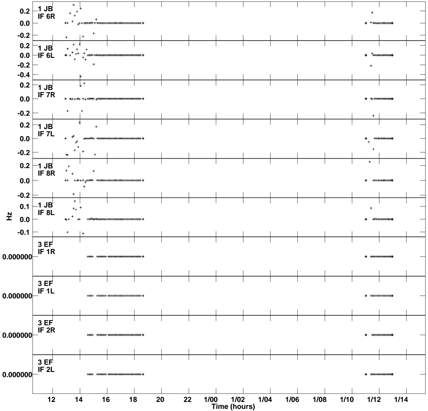
Plot file version 2 created 23-MAY-2018 15:57:18 Rate vs UTC time for EG102D.UVDATA.1 SN 2 Rpol & Lpol IF 1 - 8
