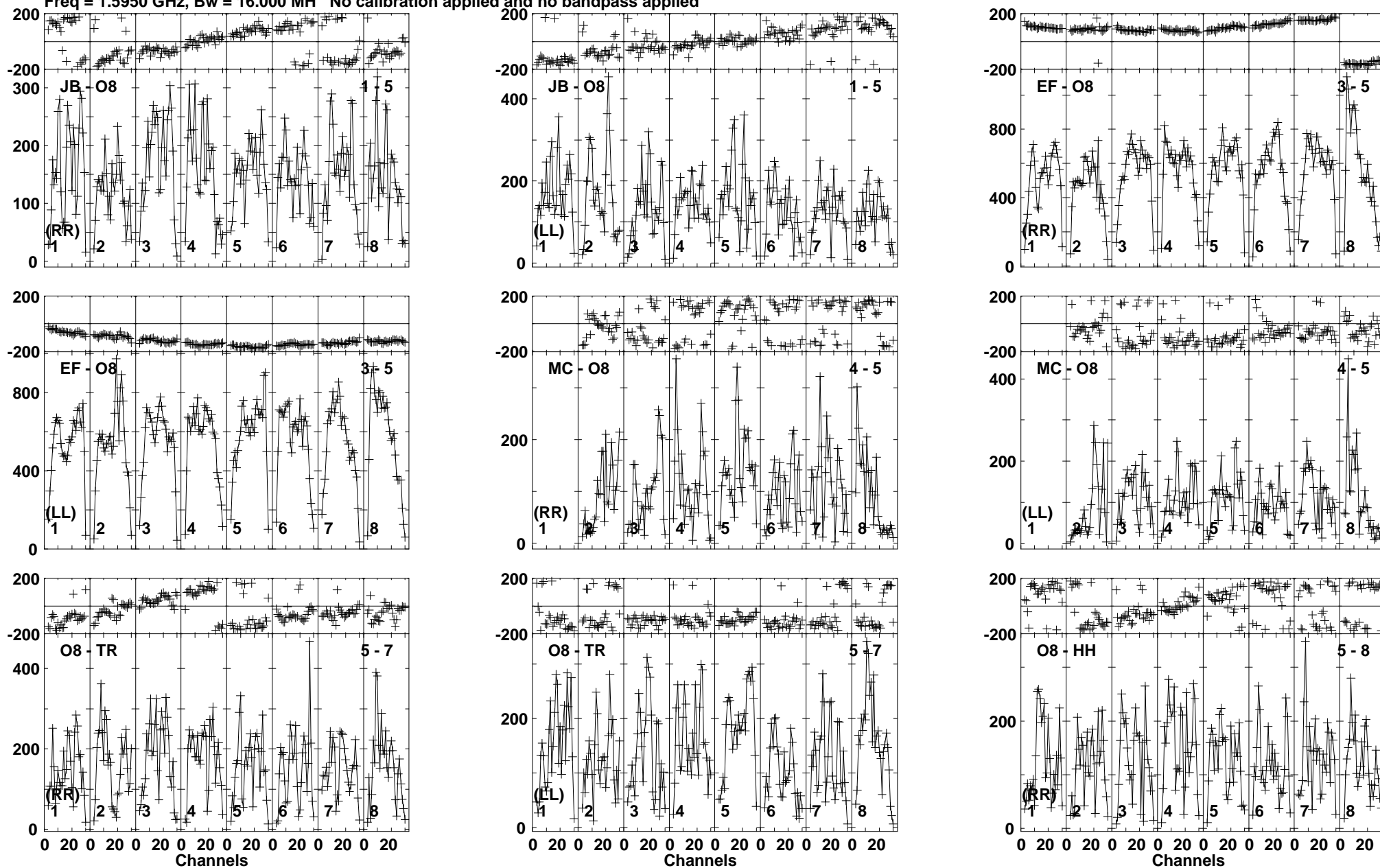
Lower frame: Micro Ampl Jy Top frame: Phas deg Vector averaged cross-power spectrum Baseline: JB (01) - O8 (05) Timerange: 00/15:44:01 to 00/15:47:29
