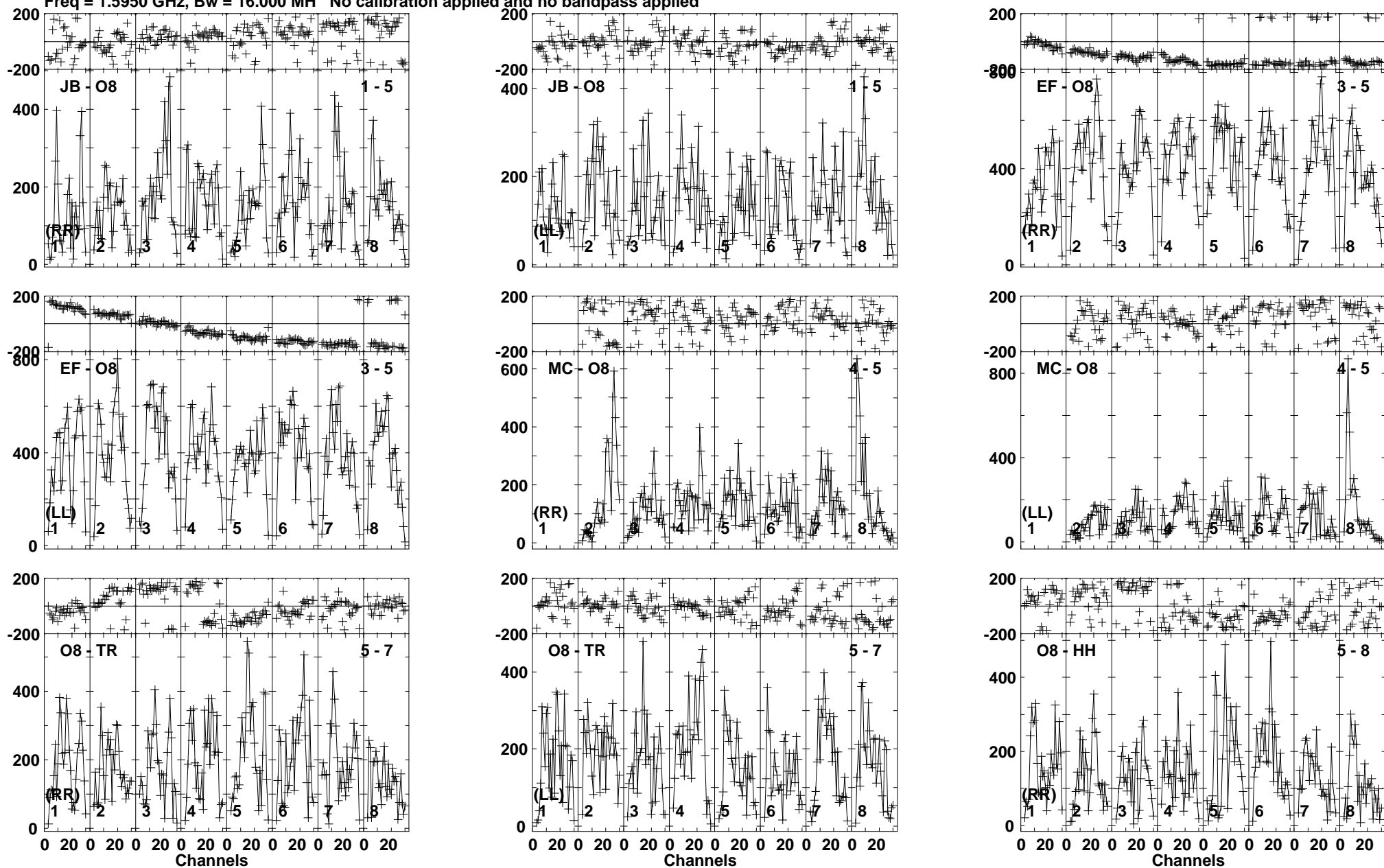
Lower frame: Micro Ampl Jy Top frame: Phas deg Vector averaged cross-power spectrum Baseline: JB (01) - O8 (05) Timerange: 01/12:26:11 to 01/12:27:39
