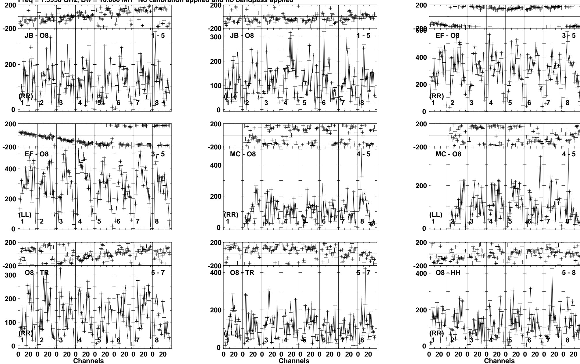
Lower frame: Micro Ampl Jy Top frame: Phas deg Vector averaged cross-power spectrum Baseline: JB (01) - O8 (05) Timerange: 01/11:50:41 to 01/11:54:09
