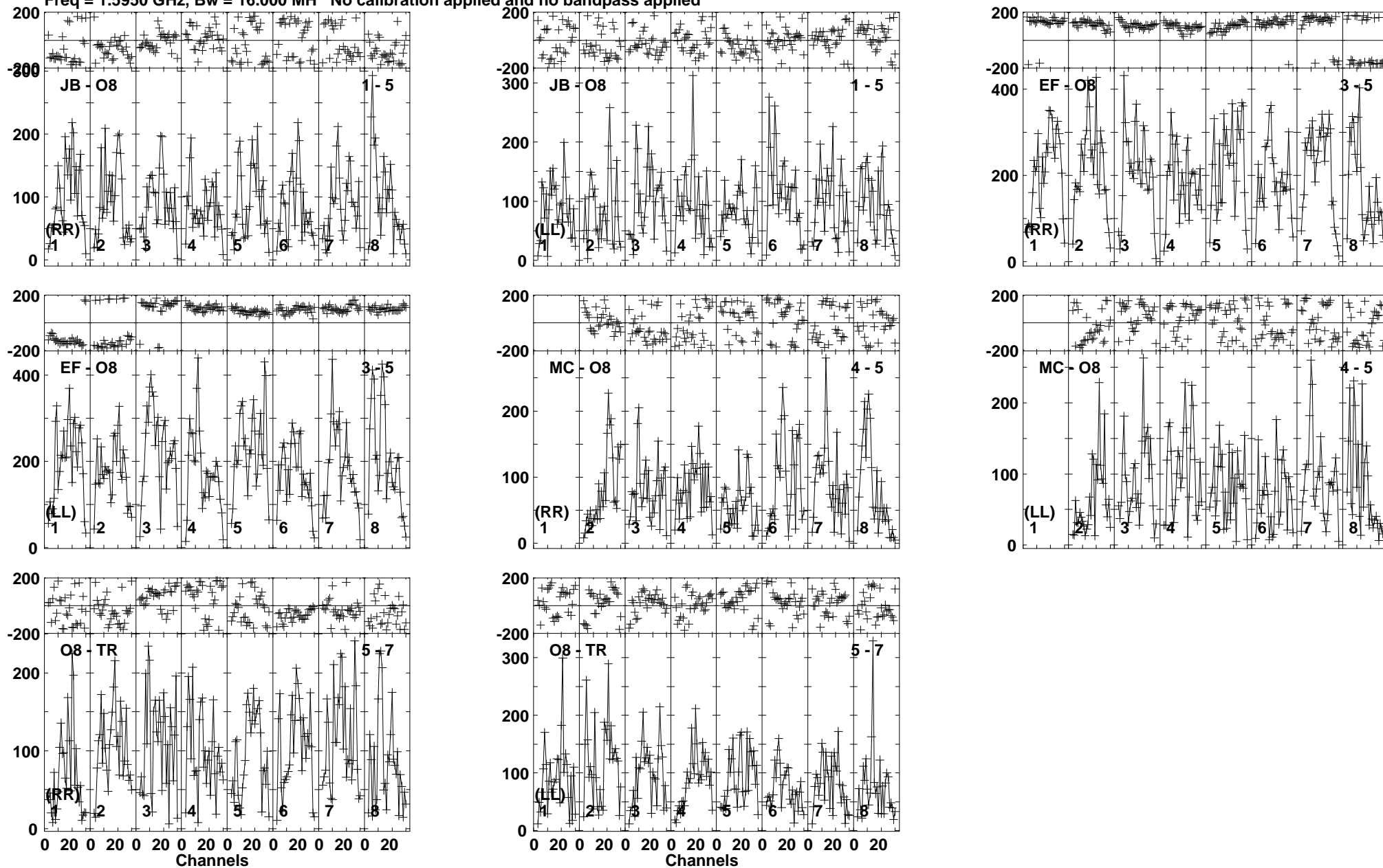
Lower frame: Micro Ampl Jy Top frame: Phas deg Vector averaged cross-power spectrum Baseline: JB (01) - O8 (05) Timerange: 00/16:43:01 to 00/16:46:29
