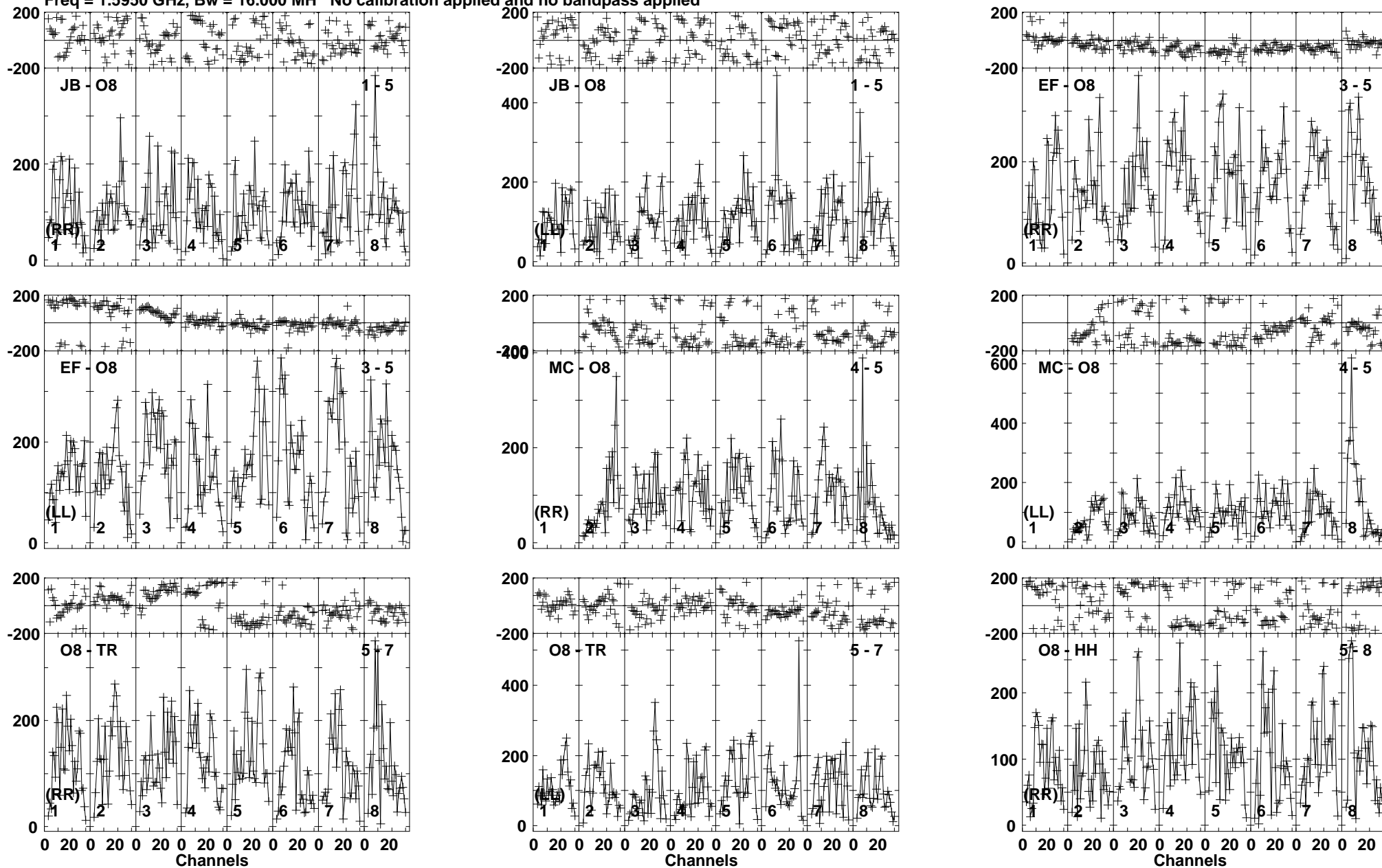
Lower frame: Micro Ampl Jy Top frame: Phas deg Vector averaged cross-power spectrum Baseline: JB (01) - O8 (05) Timerange: 01/11:29:41 to 01/11:33:09
