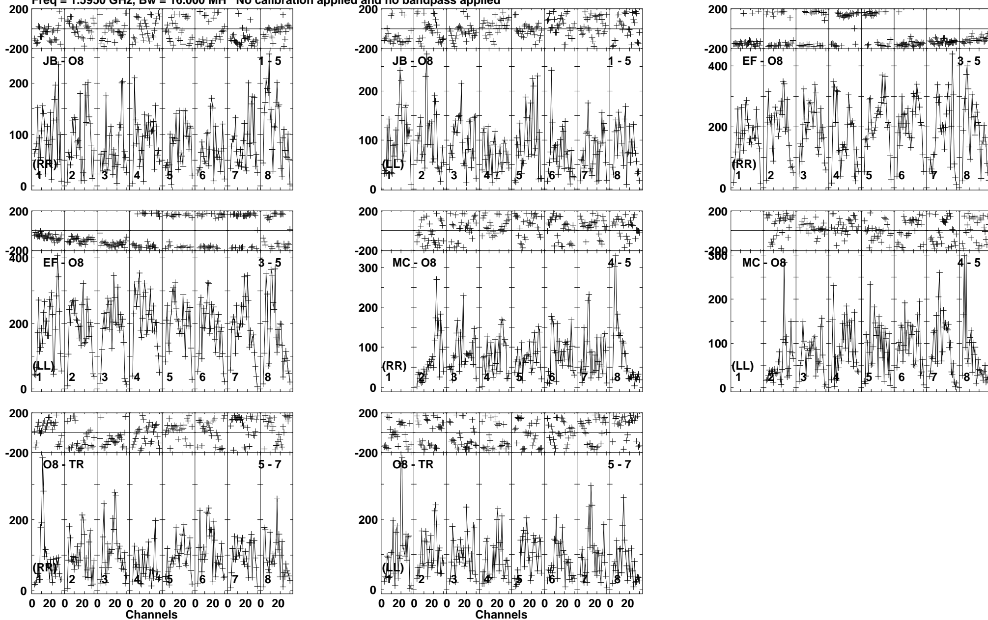
Lower frame: Micro Ampl Jy Top frame: Phas deg Vector averaged cross-power spectrum Baseline: JB (01) - O8 (05) Timerange: 00/16:22:01 to 00/16:25:29
