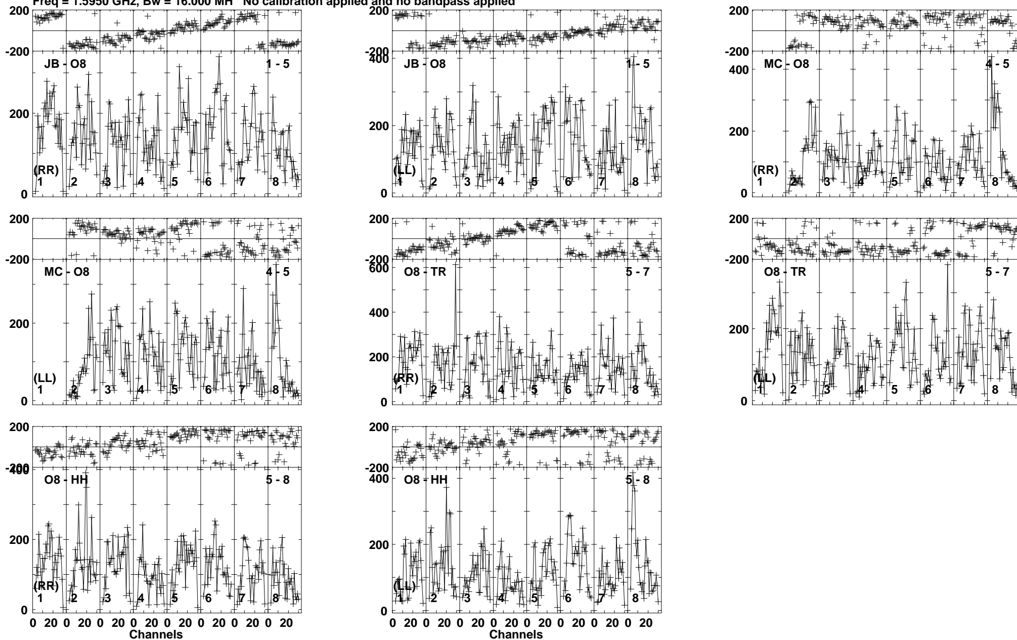
Lower frame: Micro Ampl Jy Top frame: Phas deg Vector averaged cross-power spectrum Baseline: JB (01) - O8 (05) Timerange: 00/13:27:31 to 00/13:30:59
