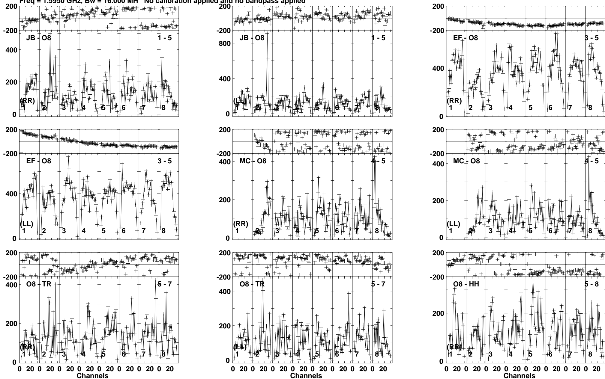
Lower frame: Micro Ampl Jy Top frame: Phas deg Vector averaged cross-power spectrum Baseline: JB (01) - O8 (05) Timerange: 01/12:06:41 to 01/12:10:09
