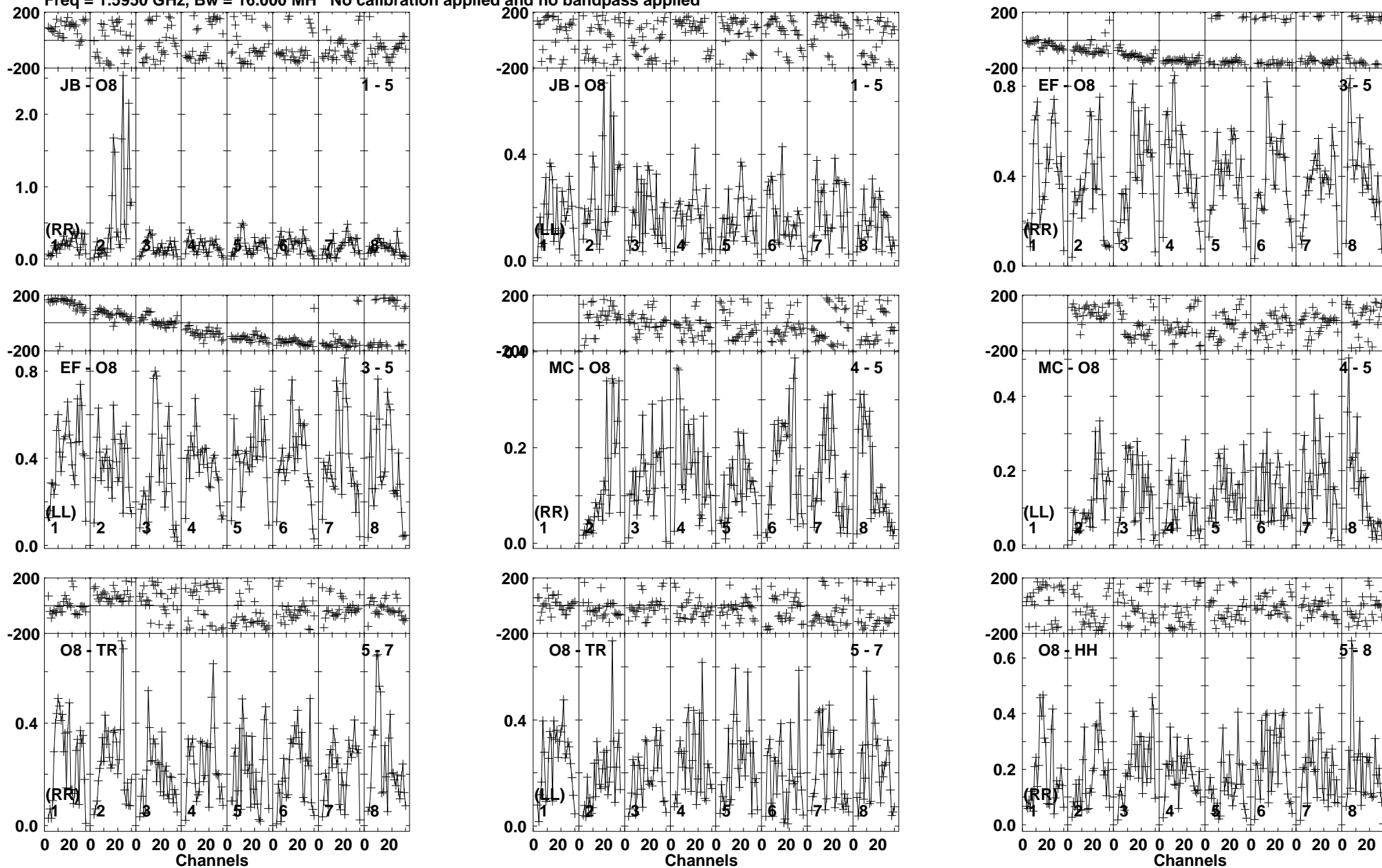
Lower frame: Milli Ampl Jy Top frame: Phas deg Vector averaged cross-power spectrum Baseline: JB (01) - O8 (05) Timerange: 01/12:10:11 to 01/12:11:39
