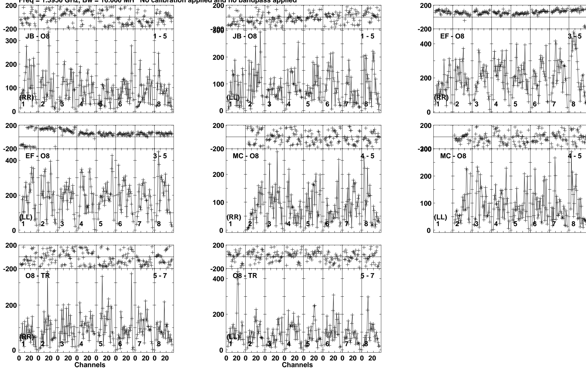
Lower frame: Micro Ampl Jy Top frame: Phas deg Vector averaged cross-power spectrum Baseline: JB (01) - O8 (05) Timerange: 00/16:59:01 to 00/17:02:29
