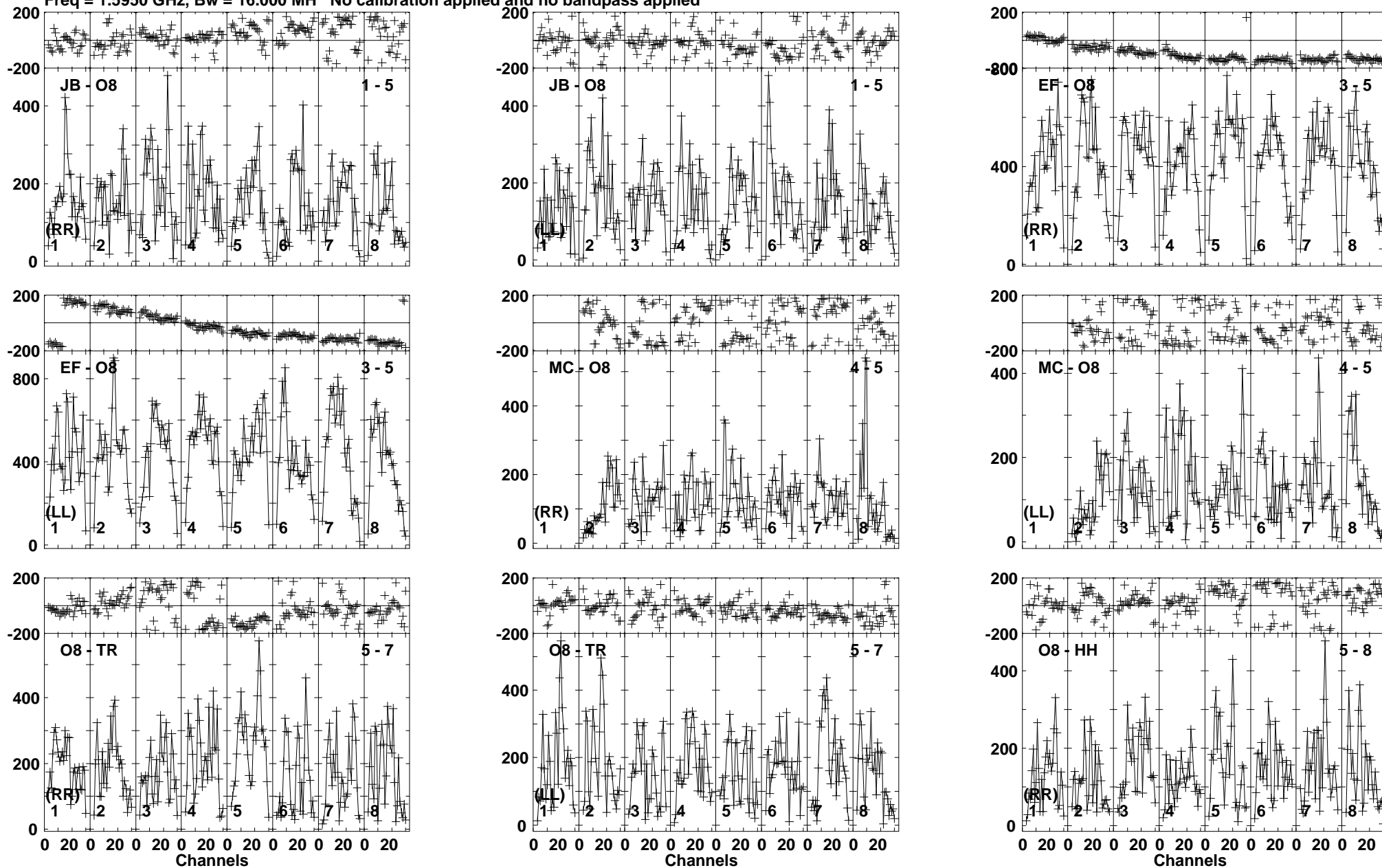
Lower frame: Micro Ampl Jy Top frame: Phas deg Vector averaged cross-power spectrum Baseline: JB (01) - O8 (05) Timerange: 01/12:47:11 to 01/12:48:39
