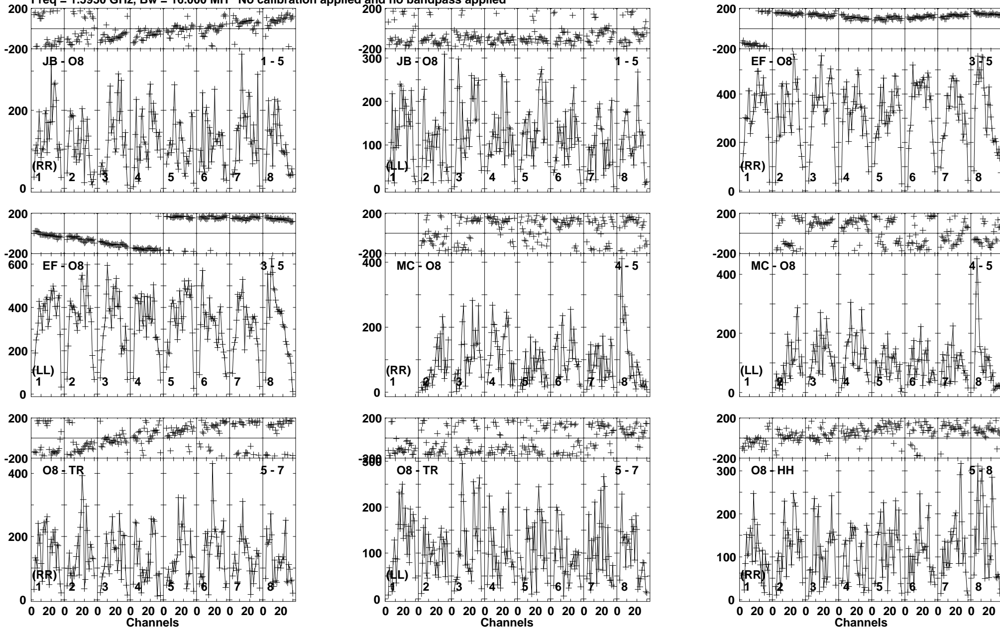
Lower frame: Micro Ampl Jy Top frame: Phas deg Vector averaged cross-power spectrum Baseline: JB (01) - O8 (05) Timerange: 01/11:56:11 to 01/11:59:39
