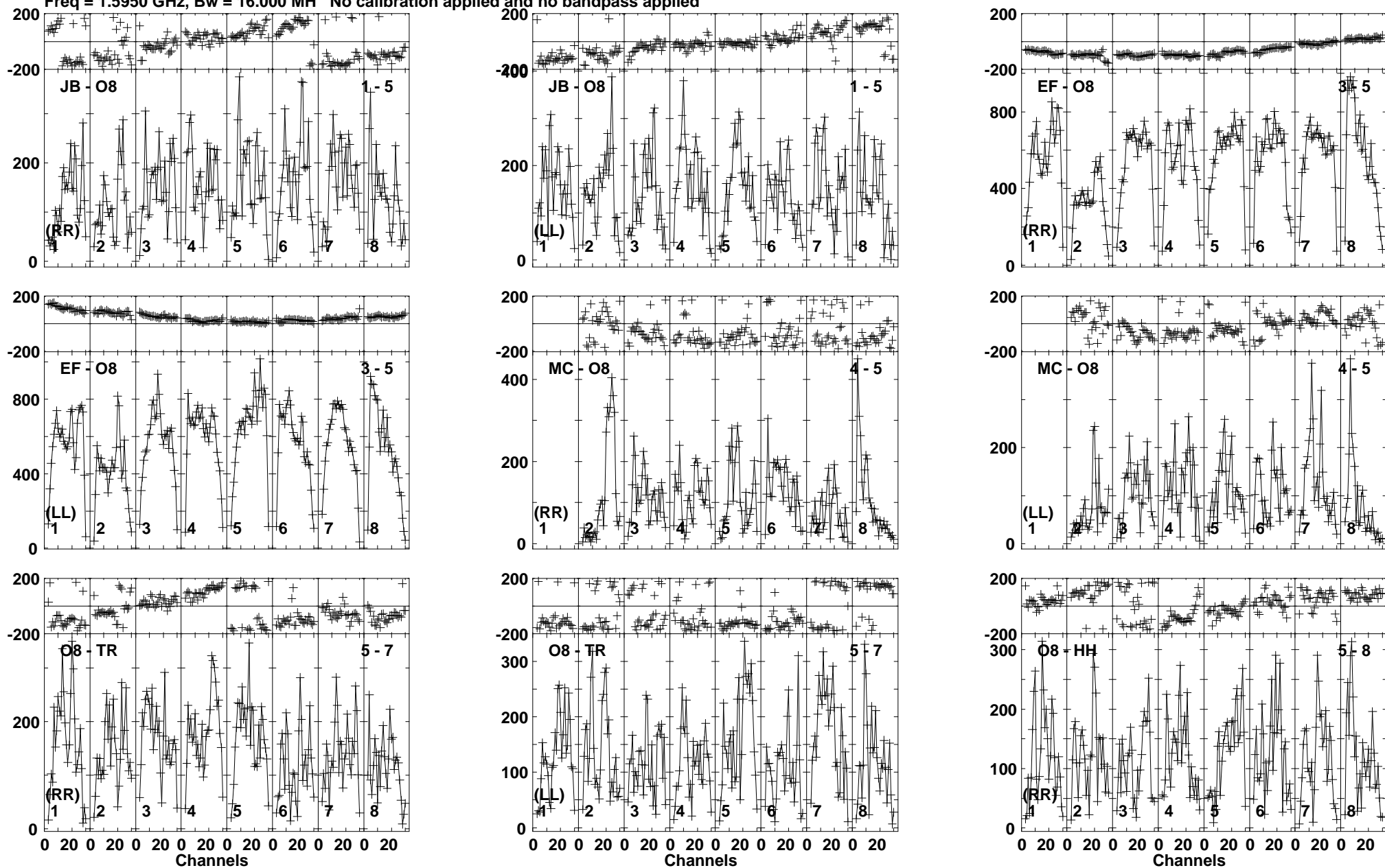
Lower frame: Micro Ampl Jy Top frame: Phas deg Vector averaged cross-power spectrum Baseline: JB (01) - O8 (05) Timerange: 00/15:28:01 to 00/15:31:29
