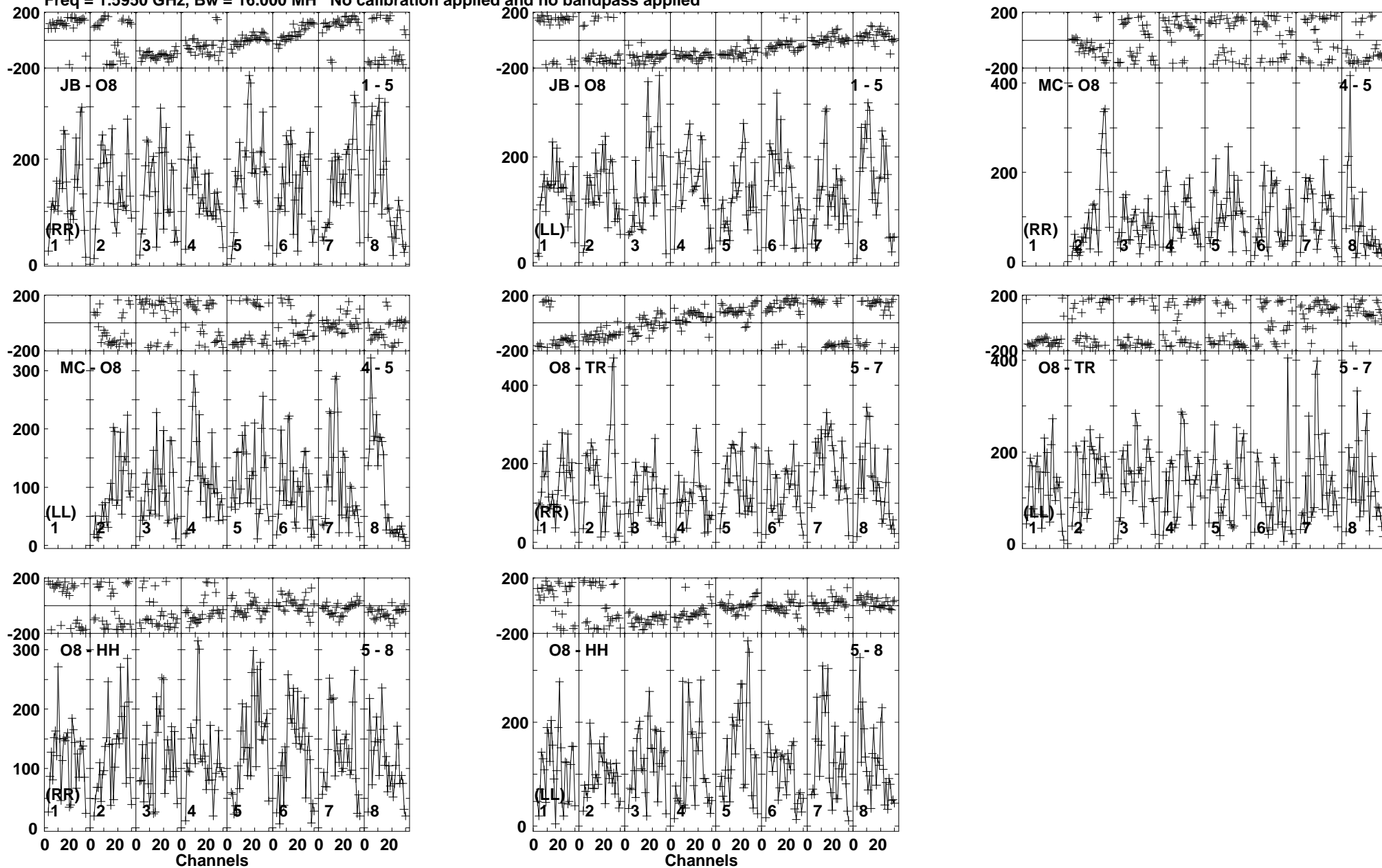
Lower frame: Micro Ampl Jy Top frame: Phas deg Vector averaged cross-power spectrum Baseline: JB (01) - O8 (05) Timerange: 00/13:22:01 to 00/13:25:29
