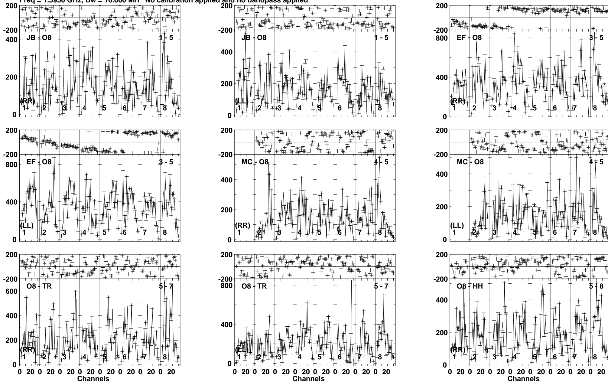
Lower frame: Micro Ampl Jy Top frame: Phas deg Vector averaged cross-power spectrum Baseline: JB (01) - O8 (05) Timerange: 01/11:49:11 to 01/11:50:39
