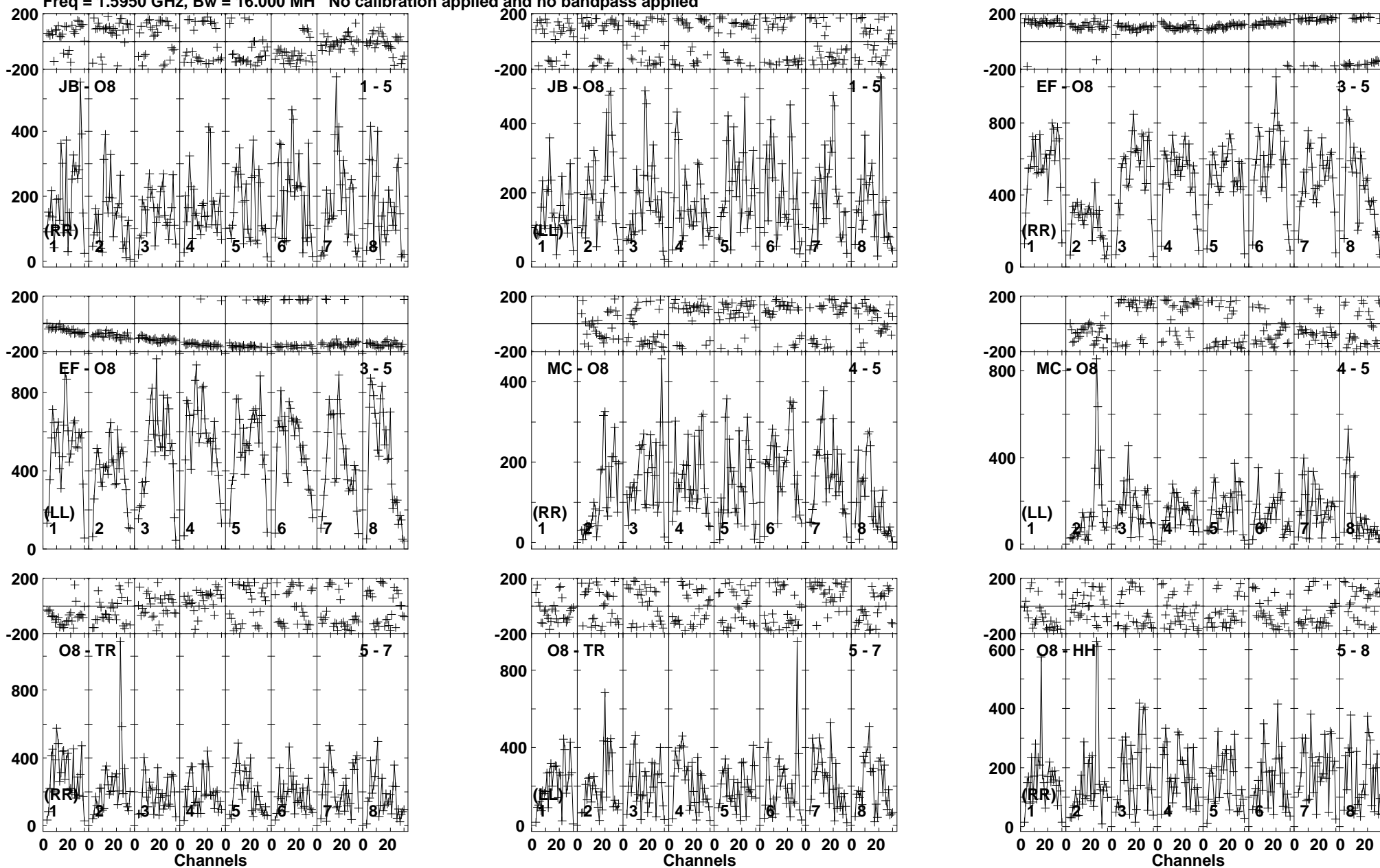
Lower frame: Micro Ampl Jy Top frame: Phas deg Vector averaged cross-power spectrum Baseline: JB (01) - O8 (05) Timerange: 00/14:44:31 to 00/14:45:59
