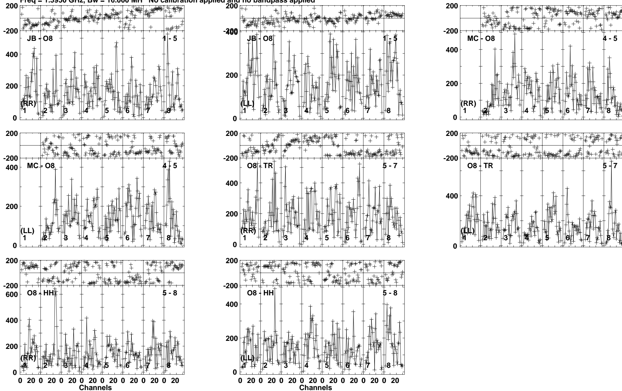
Lower frame: Micro Ampl Jy Top frame: Phas deg Vector averaged cross-power spectrum Baseline: JB (01) - O8 (05) Timerange: 00/15:11:01 to 00/15:12:29
