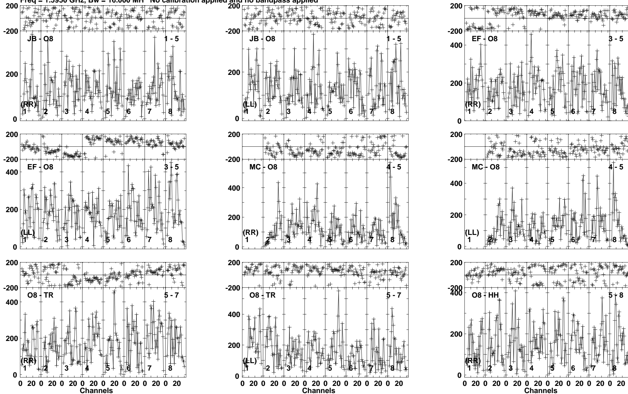
Lower frame: Micro Ampl Jy Top frame: Phas deg Vector averaged cross-power spectrum Baseline: JB (01) - O8 (05) Timerange: 01/11:23:11 to 01/11:24:39
