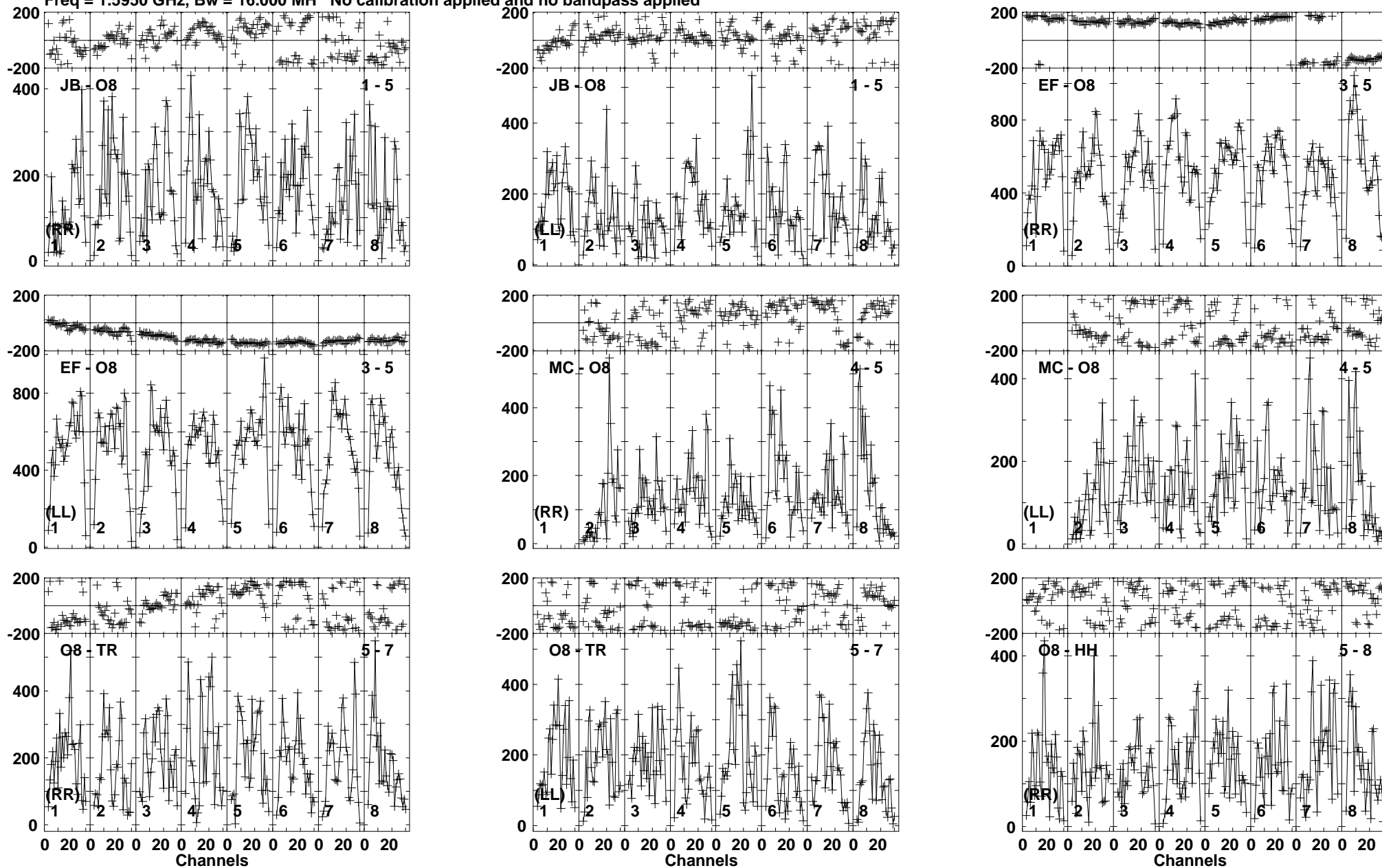
Lower frame: Micro Ampl Jy Top frame: Phas deg Vector averaged cross-power spectrum Baseline: JB (01) - O8 (05) Timerange: 00/14:39:31 to 00/14:40:59
