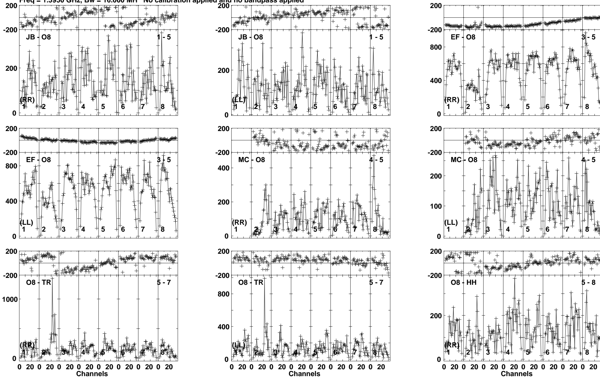
Lower frame: Micro Ampl Jy Top frame: Phas deg Vector averaged cross-power spectrum Baseline: JB (01) - O8 (05) Timerange: 00/14:51:31 to 00/14:54:59
