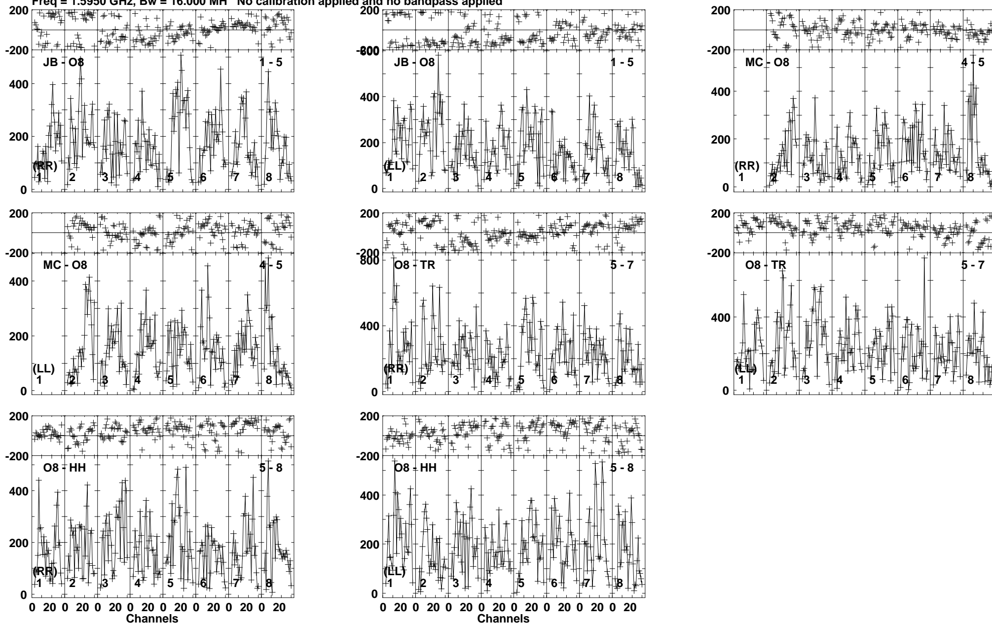
Lower frame: Micro Ampl Jy Top frame: Phas deg Vector averaged cross-power spectrum Baseline: JB (01) - O8 (05) Timerange: 00/13:20:31 to 00/13:21:59
