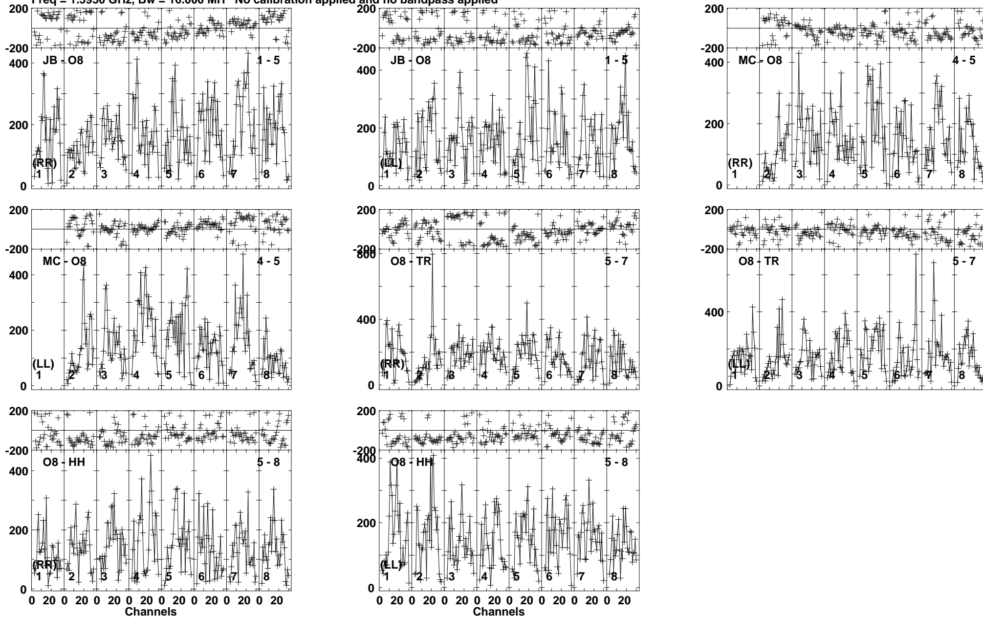
Lower frame: Micro Ampl Jy Top frame: Phas deg Vector averaged cross-power spectrum Baseline: JB (01) - O8 (05) Timerange: 00/15:00:31 to 00/15:01:59
