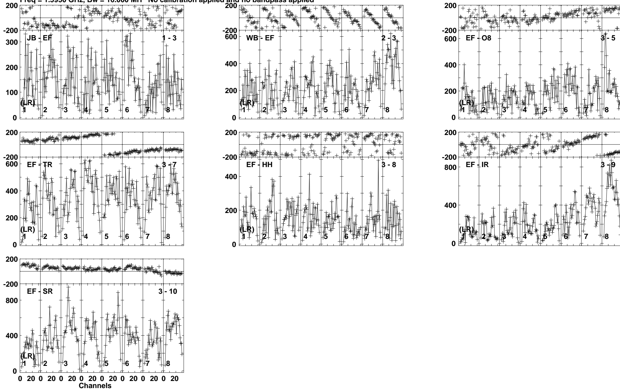
Lower frame: Micro Ampl Jy Top frame: Phas deg Vector averaged cross-power spectrum Baseline: JB (01) - EF (03) Timerange: 01/04:53:21 to 01/04:54:49
