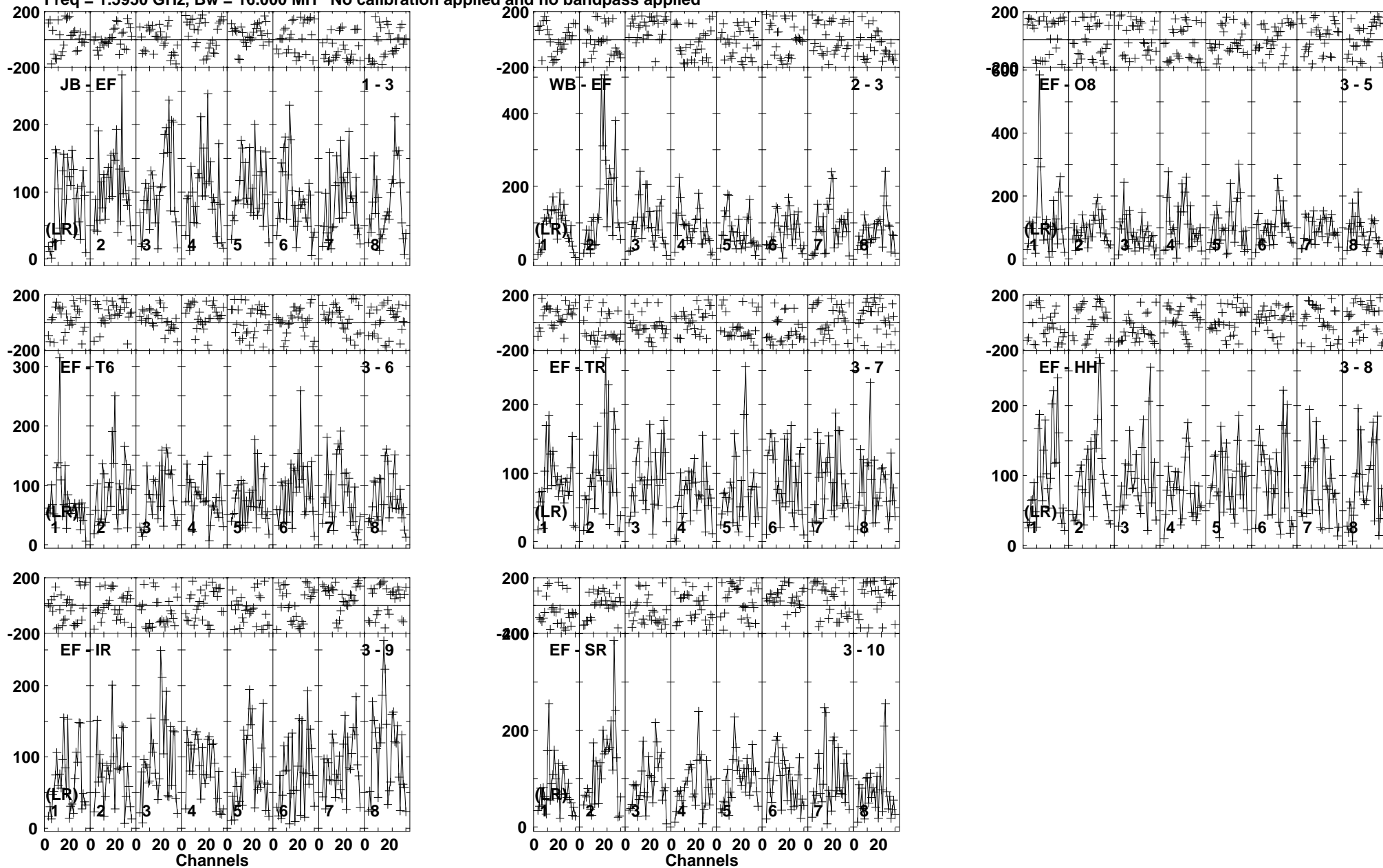
Lower frame: Micro Ampl Jy Top frame: Phas deg Vector averaged cross-power spectrum Baseline: JB (01) - EF (03) Timerange: 01/01:06:41 to 01/01:10:09
