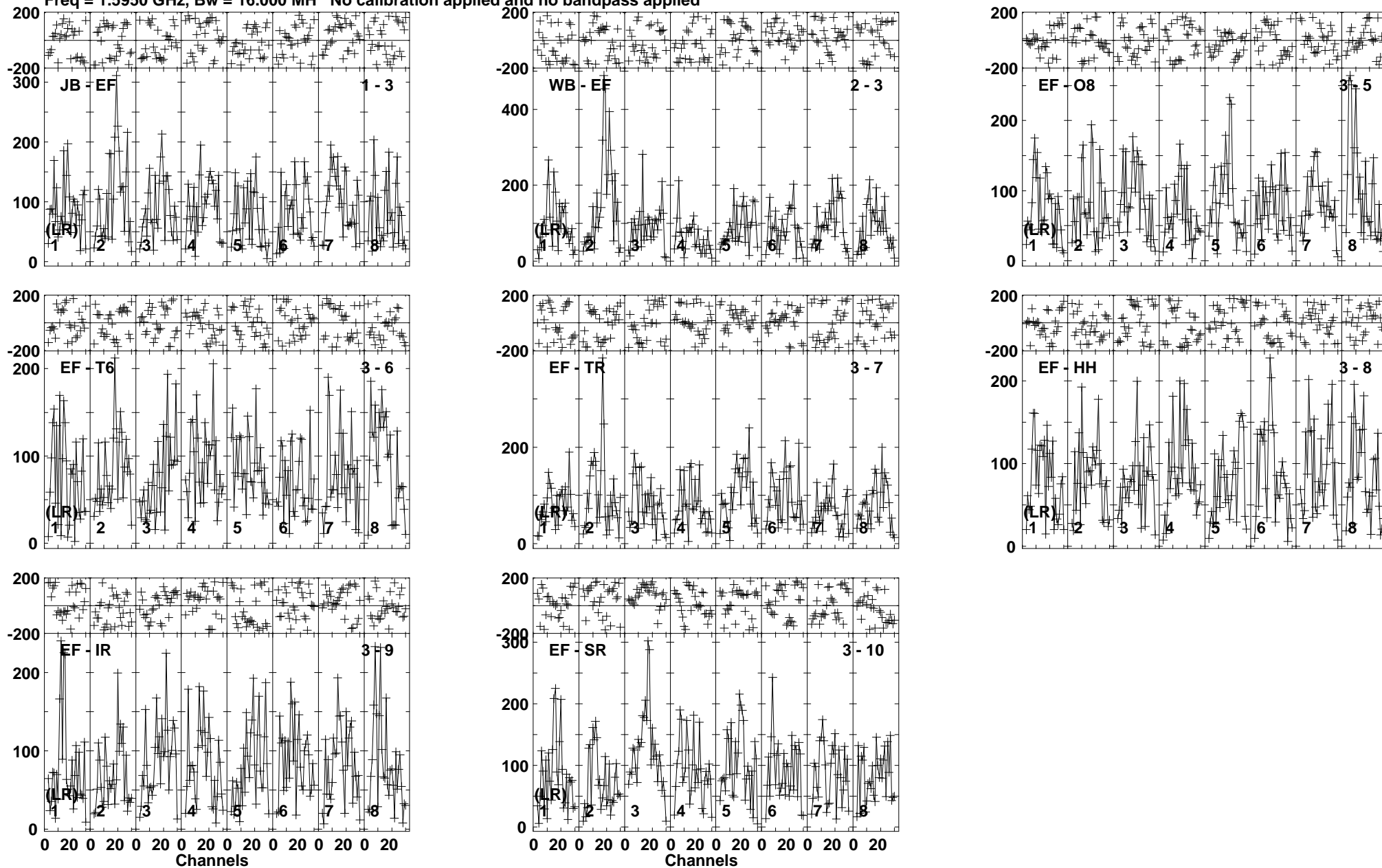
Lower frame: Micro Ampl Jy Top frame: Phas deg Vector averaged cross-power spectrum Baseline: JB (01) - EF (03) Timerange: 00/23:30:01 to 00/23:41:59
