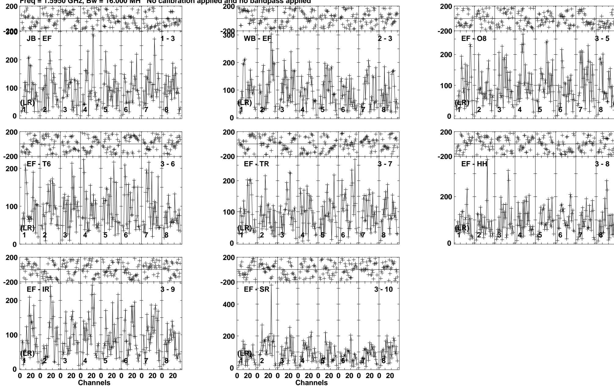
Lower frame: Micro Ampl Jy Top frame: Phas deg Vector averaged cross-power spectrum Baseline: JB (01) - EF (03) Timerange: 01/01:45:01 to 01/01:48:29
