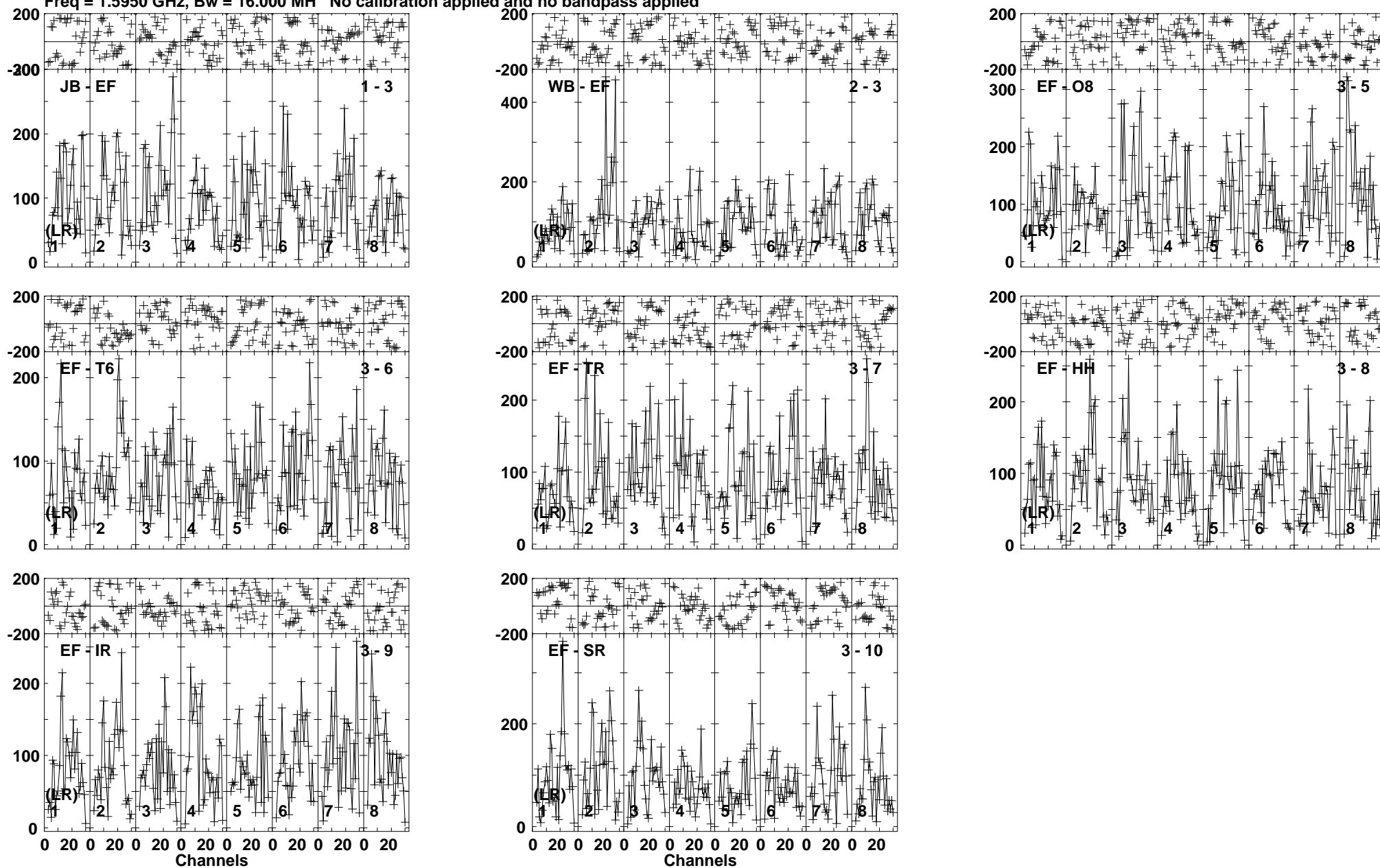
Lower frame: Micro Ampl Jy Top frame: Phas deg Vector averaged cross-power spectrum Baseline: JB (01) - EF (03) Timerange: 01/01:18:01 to 01/01:21:29
