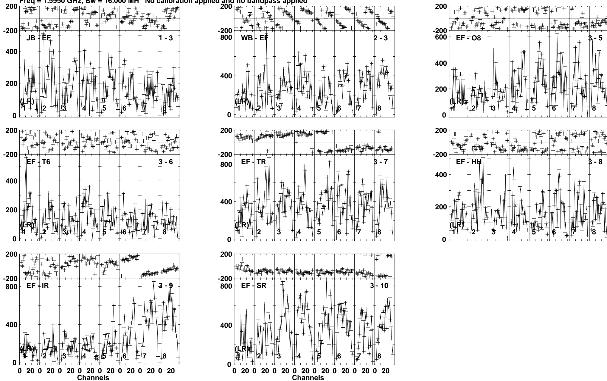
Lower frame: Micro Ampl Jy Top frame: Phas deg Vector averaged cross-power spectrum Baseline: JB (01) - EF (03) Timerange: 01/03:03:21 to 01/03:04:49
