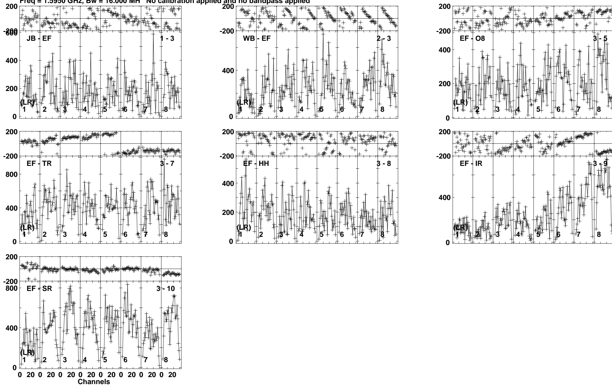
Lower frame: Micro Ampl Jy Top frame: Phas deg Vector averaged cross-power spectrum Baseline: JB (01) - EF (03) Timerange: 01/04:58:31 to 01/04:59:59
