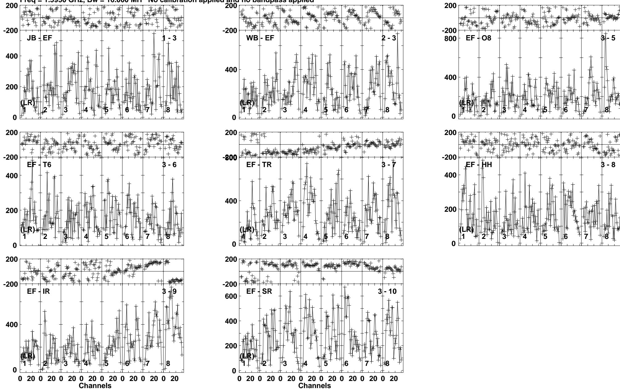
Lower frame: Micro Ampl Jy Top frame: Phas deg Vector averaged cross-power spectrum Baseline: JB (01) - EF (03) Timerange: 01/00:16:11 to 01/00:17:39
