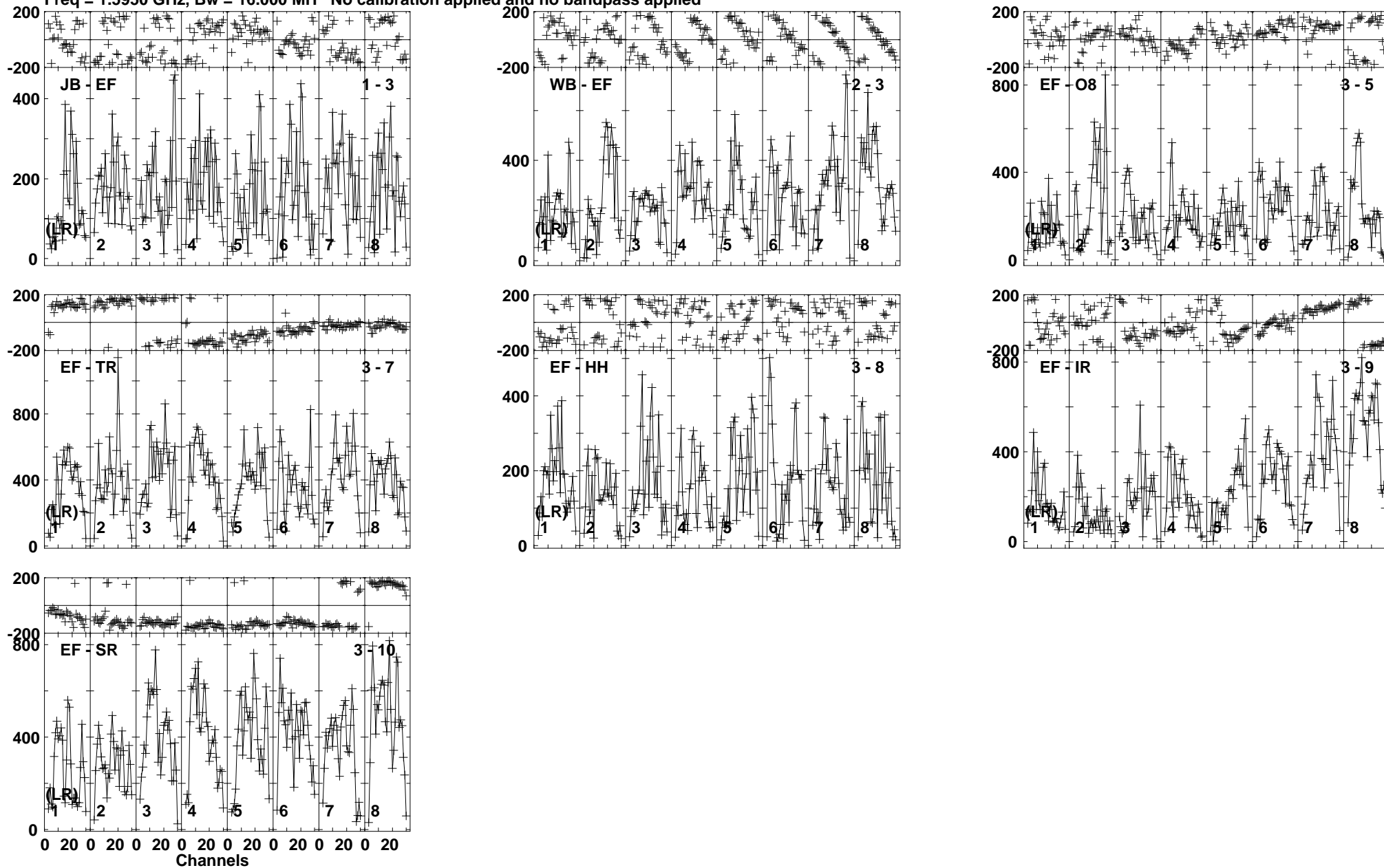
Lower frame: Micro Ampl Jy Top frame: Phas deg Vector averaged cross-power spectrum Baseline: JB (01) - EF (03) Timerange: 01/04:15:01 to 01/04:16:29
