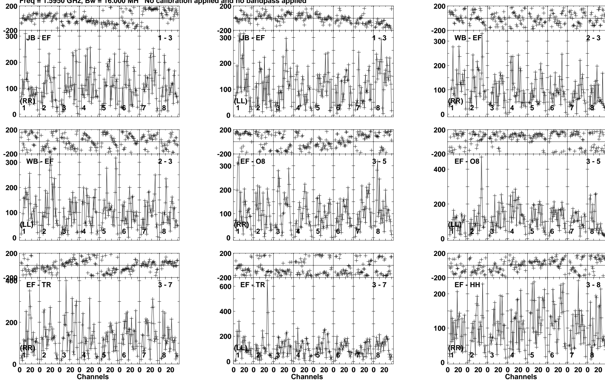
Lower frame: Micro Ampl Jy Top frame: Phas deg Vector averaged cross-power spectrum Baseline: JB (01) - EF (03) Timerange: 01/04:49:11 to 01/04:52:39
