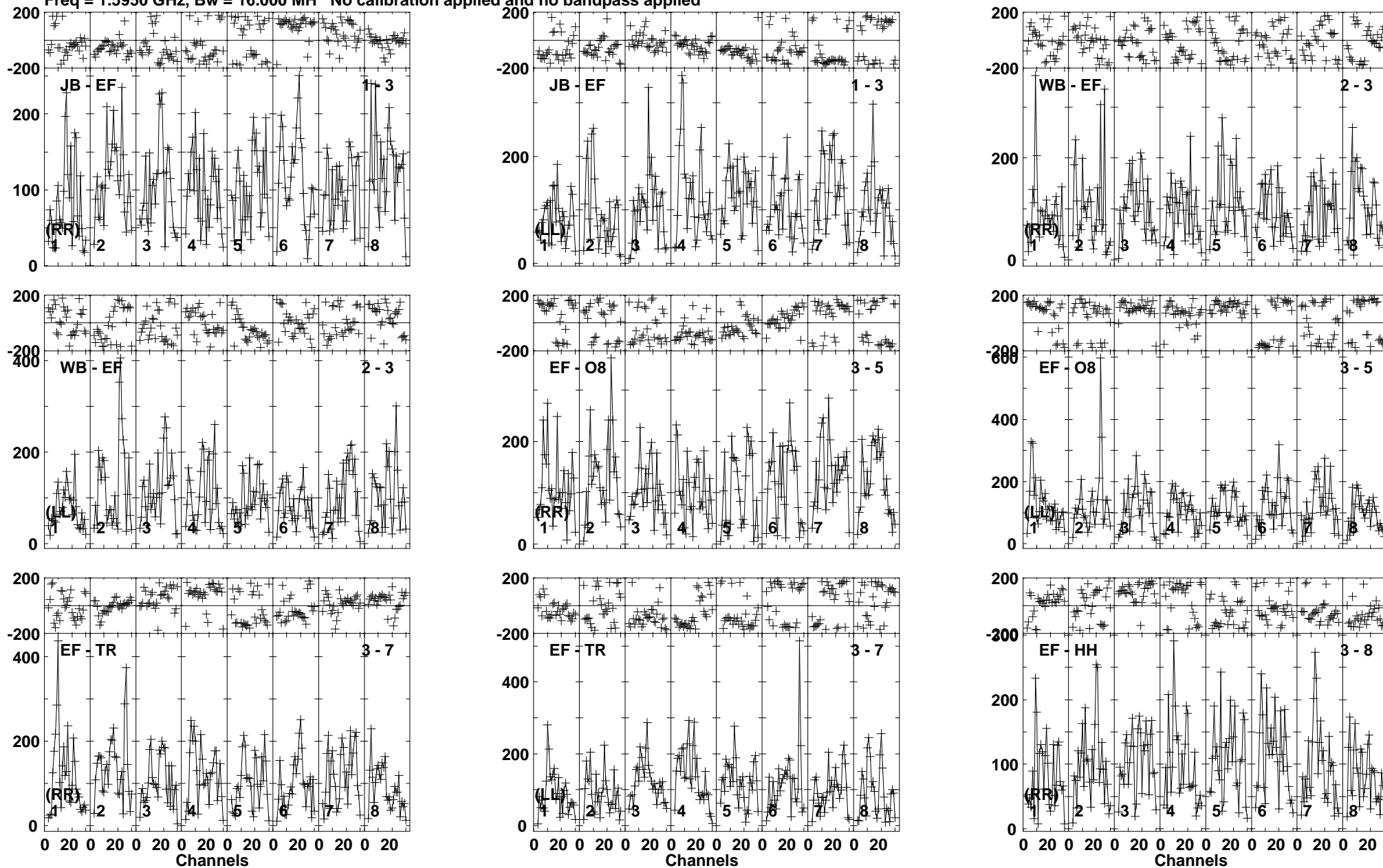
Lower frame: Micro Ampl Jy Top frame: Phas deg Vector averaged cross-power spectrum Baseline: JB (01) - EF (03) Timerange: 01/04:32:51 to 01/04:36:19
