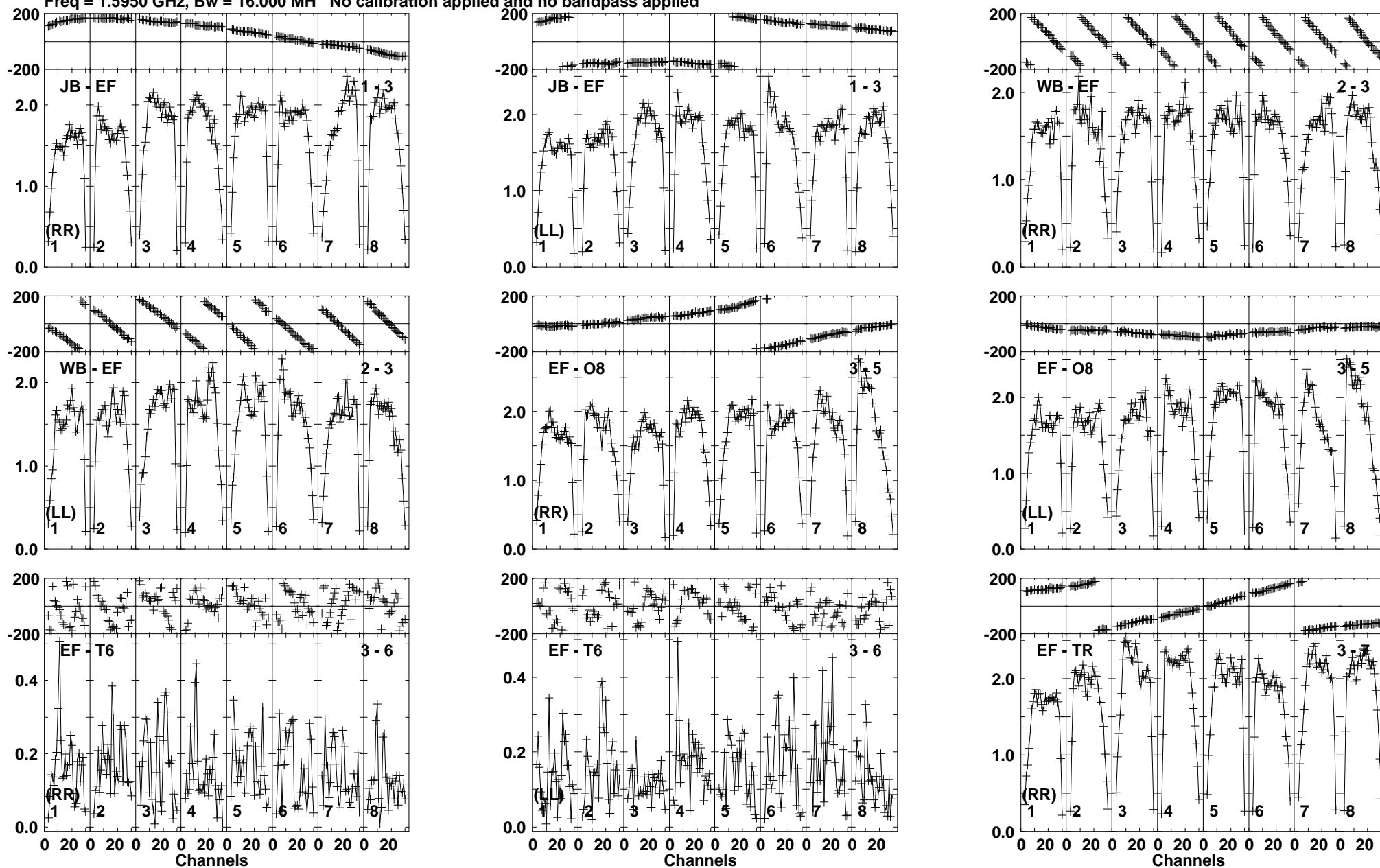
Lower frame: Milli Ampl Jy Top frame: Phas deg Vector averaged cross-power spectrum Baseline: JB (01) - EF (03) Timerange: 01/01:16:31 to 01/01:17:59
