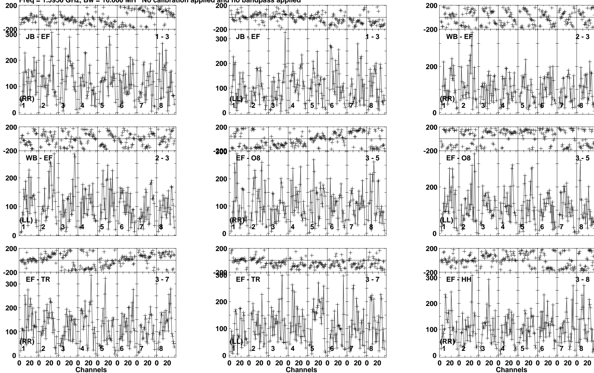
Lower frame: Micro Ampl Jy Top frame: Phas deg Vector averaged cross-power spectrum Baseline: JB (01) - EF (03) Timerange: 01/04:11:31 to 01/04:14:59
