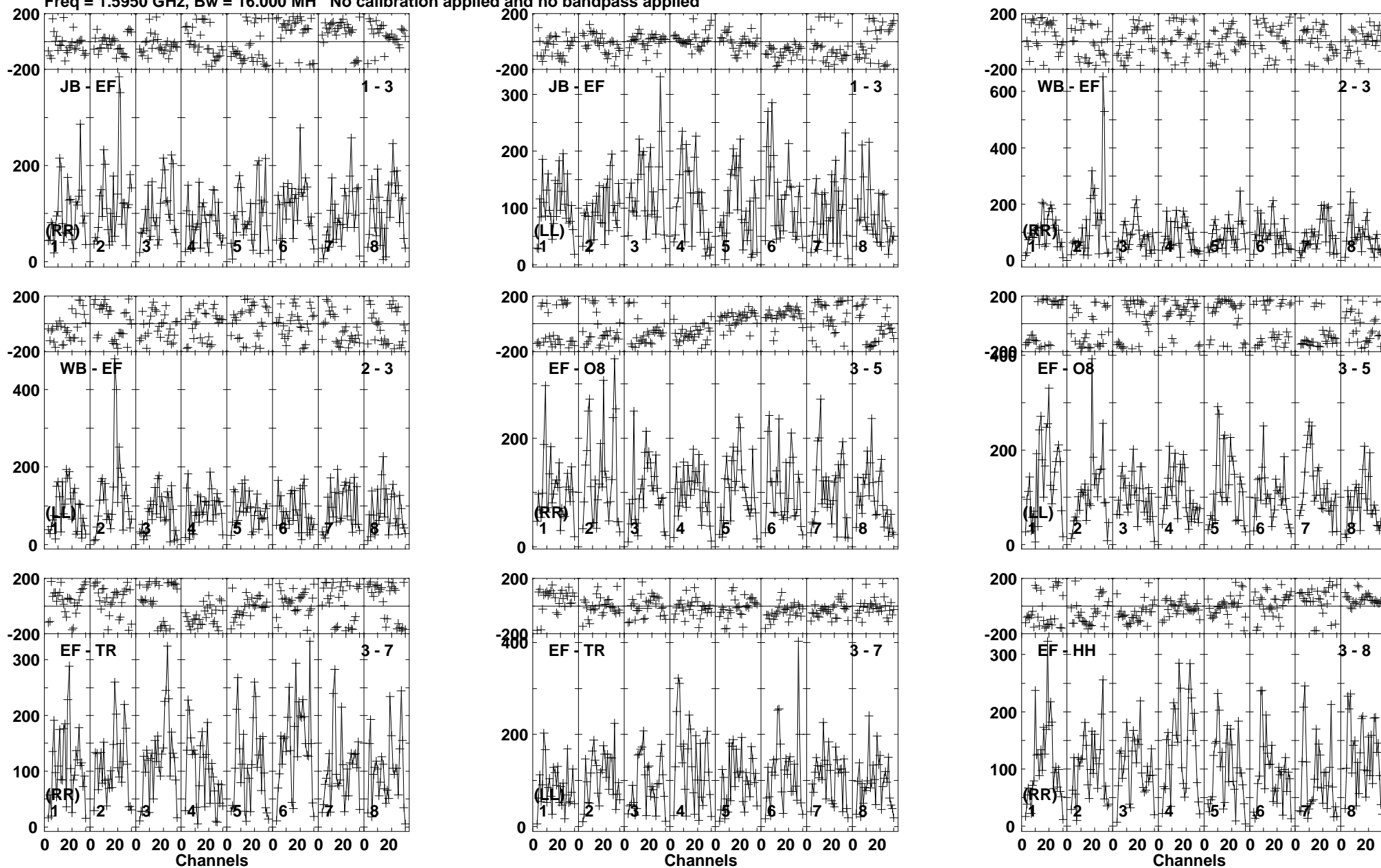
Lower frame: Micro Ampl Jy Top frame: Phas deg Vector averaged cross-power spectrum Baseline: JB (01) - EF (03) Timerange: 01/03:55:11 to 01/03:58:39
