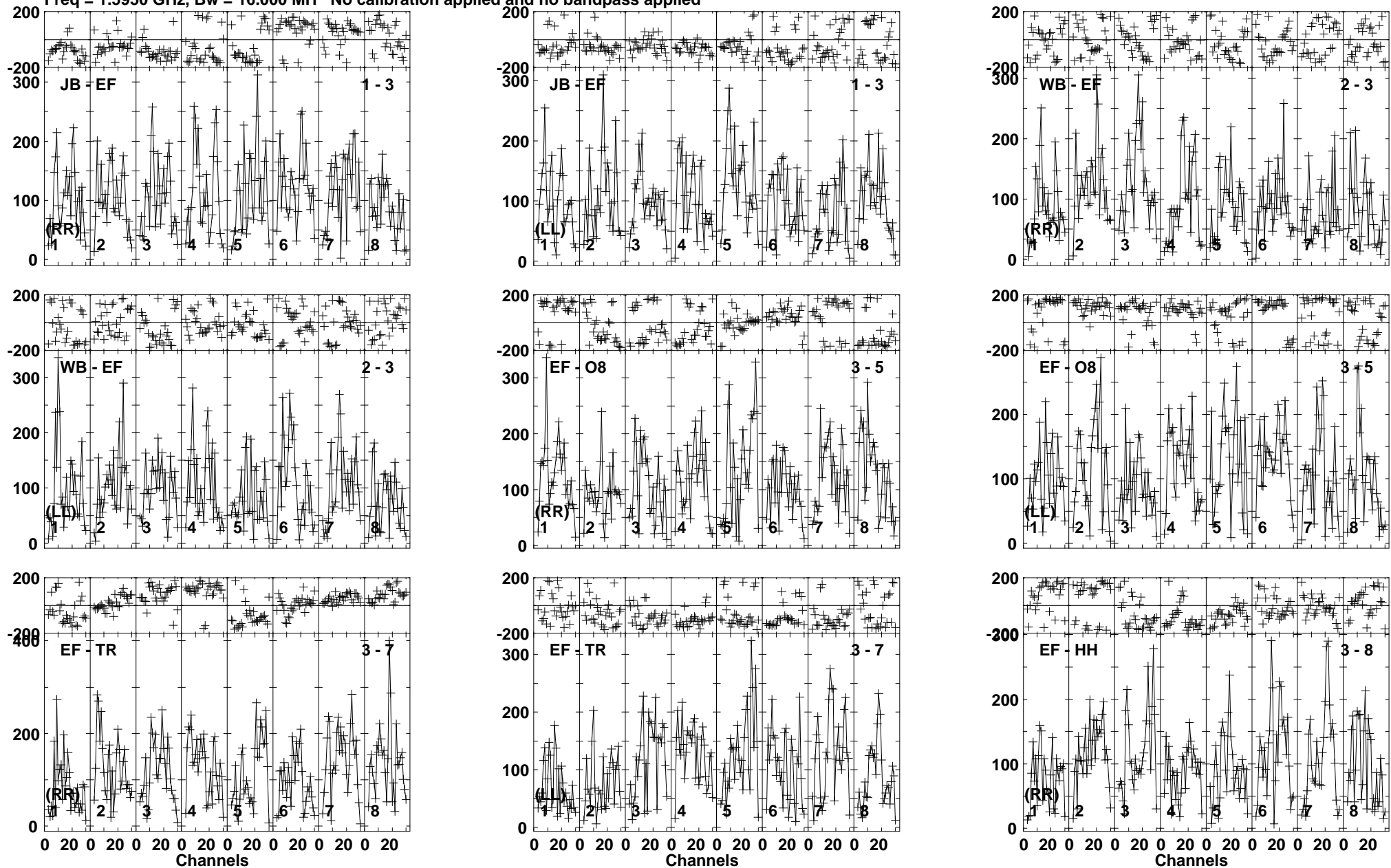
Lower frame: Micro Ampl Jy Top frame: Phas deg Vector averaged cross-power spectrum Baseline: JB (01) - EF (03) Timerange: 01/04:27:51 to 01/04:31:19
