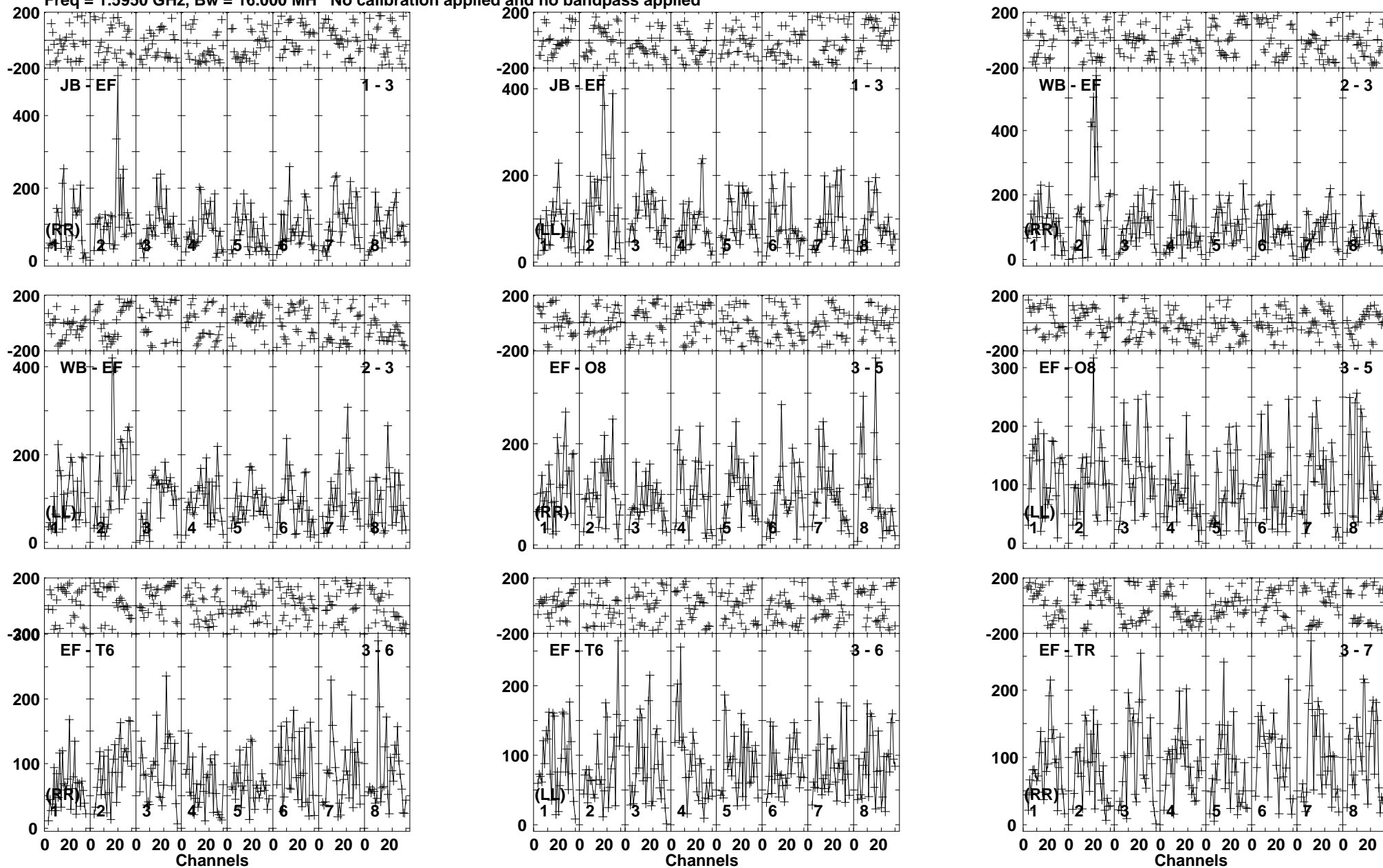
Lower frame: Micro Ampl Jy Top frame: Phas deg Vector averaged cross-power spectrum Baseline: JB (01) - EF (03) Timerange: 01/00:45:21 to 01/00:48:49
