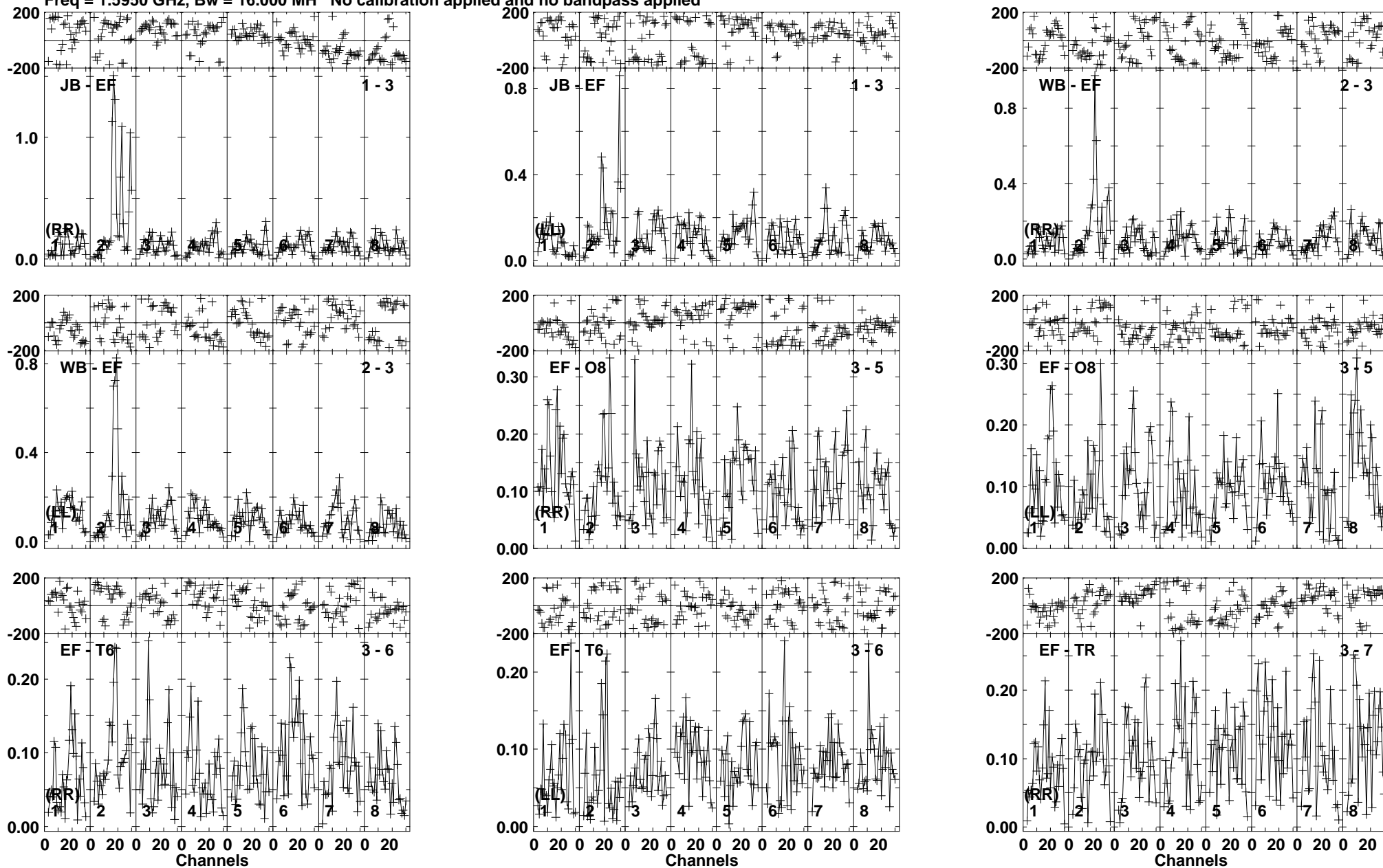
Lower frame: Milli Ampl Jy Top frame: Phas deg Vector averaged cross-power spectrum Baseline: JB (01) - EF (03) Timerange: 01/03:16:11 to 01/03:19:39
