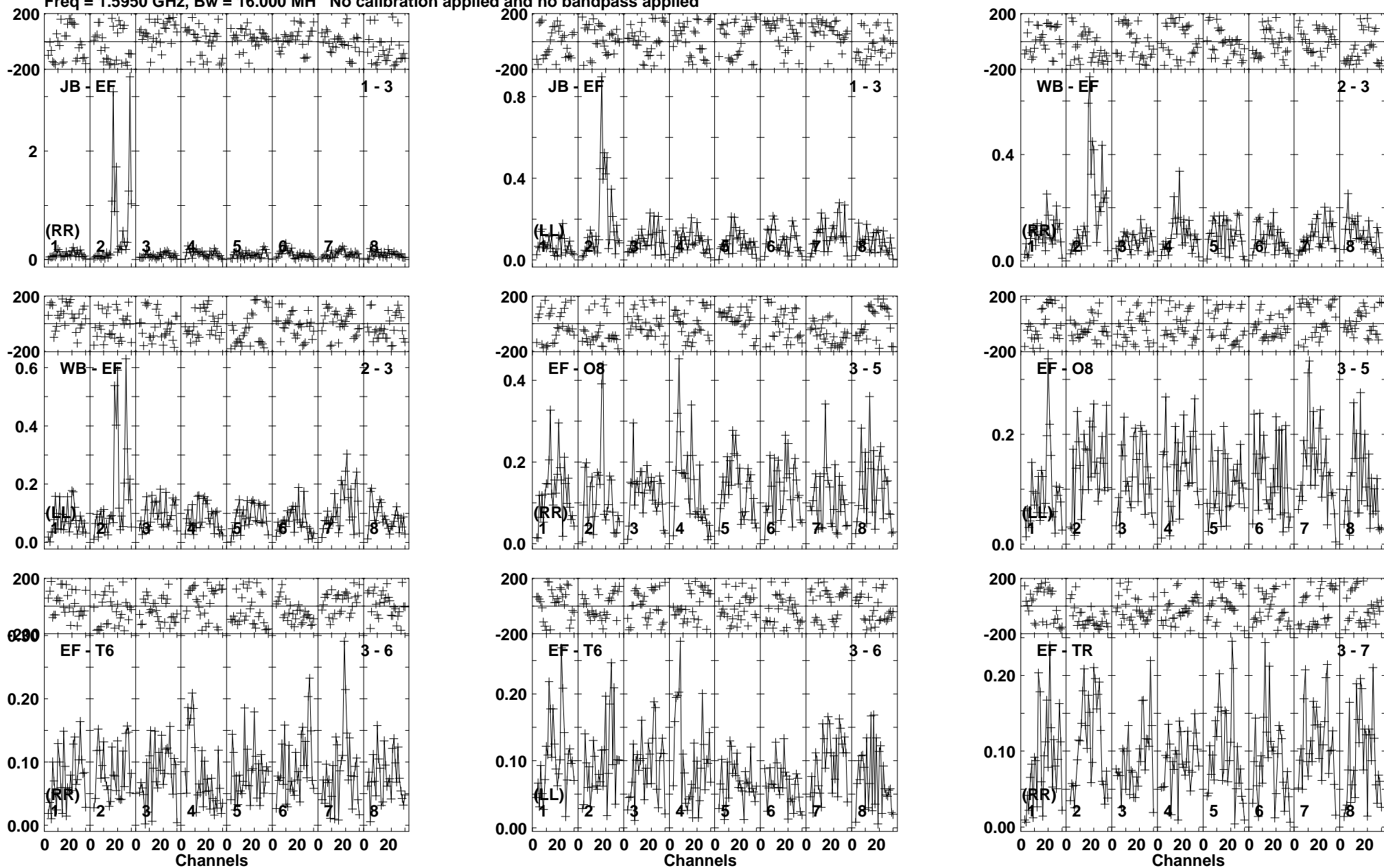
Lower frame: Milli Ampl Jy Top frame: Phas deg Vector averaged cross-power spectrum Baseline: JB (01) - EF (03) Timerange: 01/00:17:41 to 01/00:21:09
