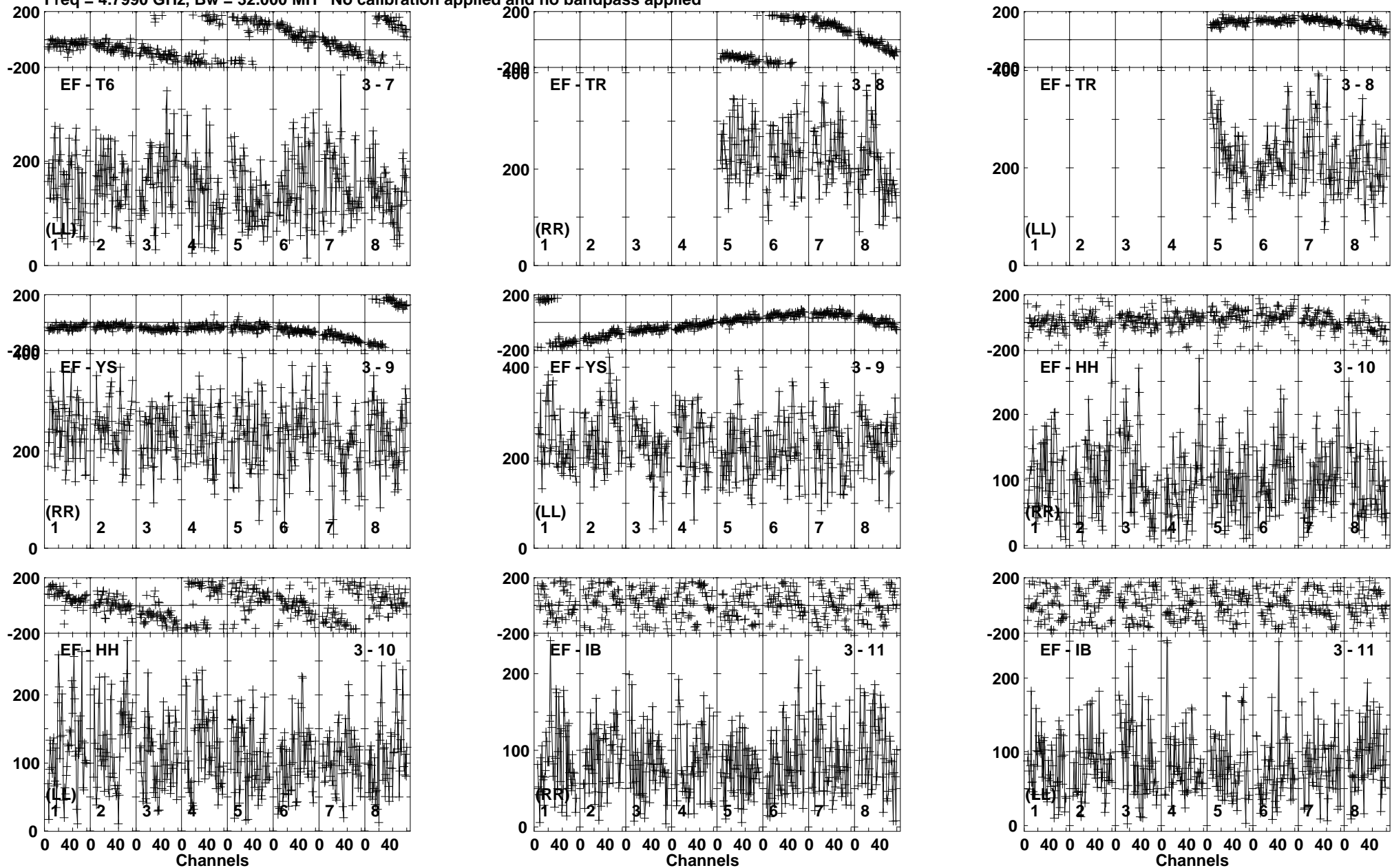
Lower frame: Micro Ampl Jy Top frame: Phas deg Vector averaged cross-power spectrum Baseline: EF (03) - T6 (07) Timerange: 00/23:21:50 to 00/23:25:19
