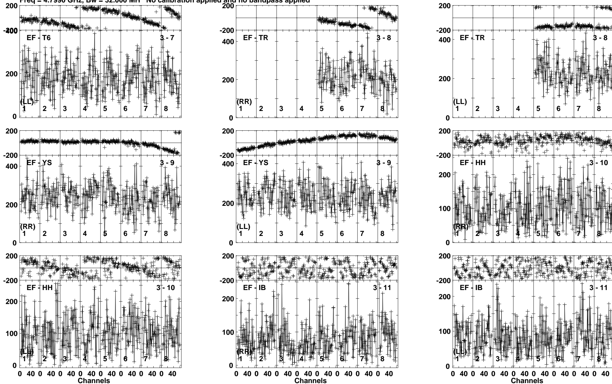
Lower frame: Micro Ampl Jy Top frame: Phas deg Vector averaged cross-power spectrum Baseline: EF (03) - T6 (07) Timerange: 00/23:06:11 to 00/23:09:40
