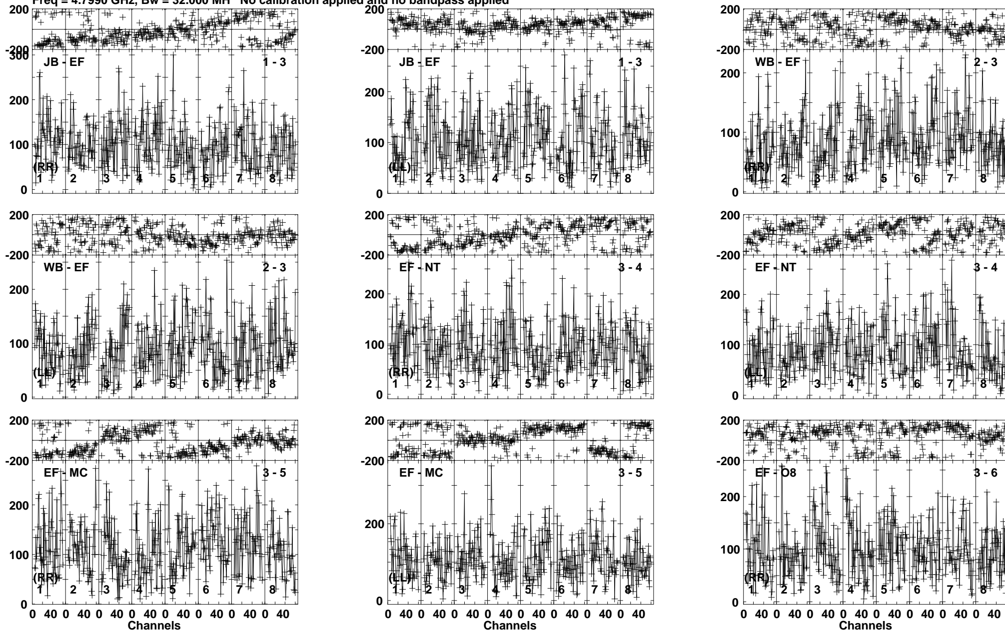
Lower frame: Micro Ampl Jy Top frame: Phas deg Vector averaged cross-power spectrum Baseline: JB (01) - EF (03) Timerange: 00/20:45:00 to 00/20:48:29
