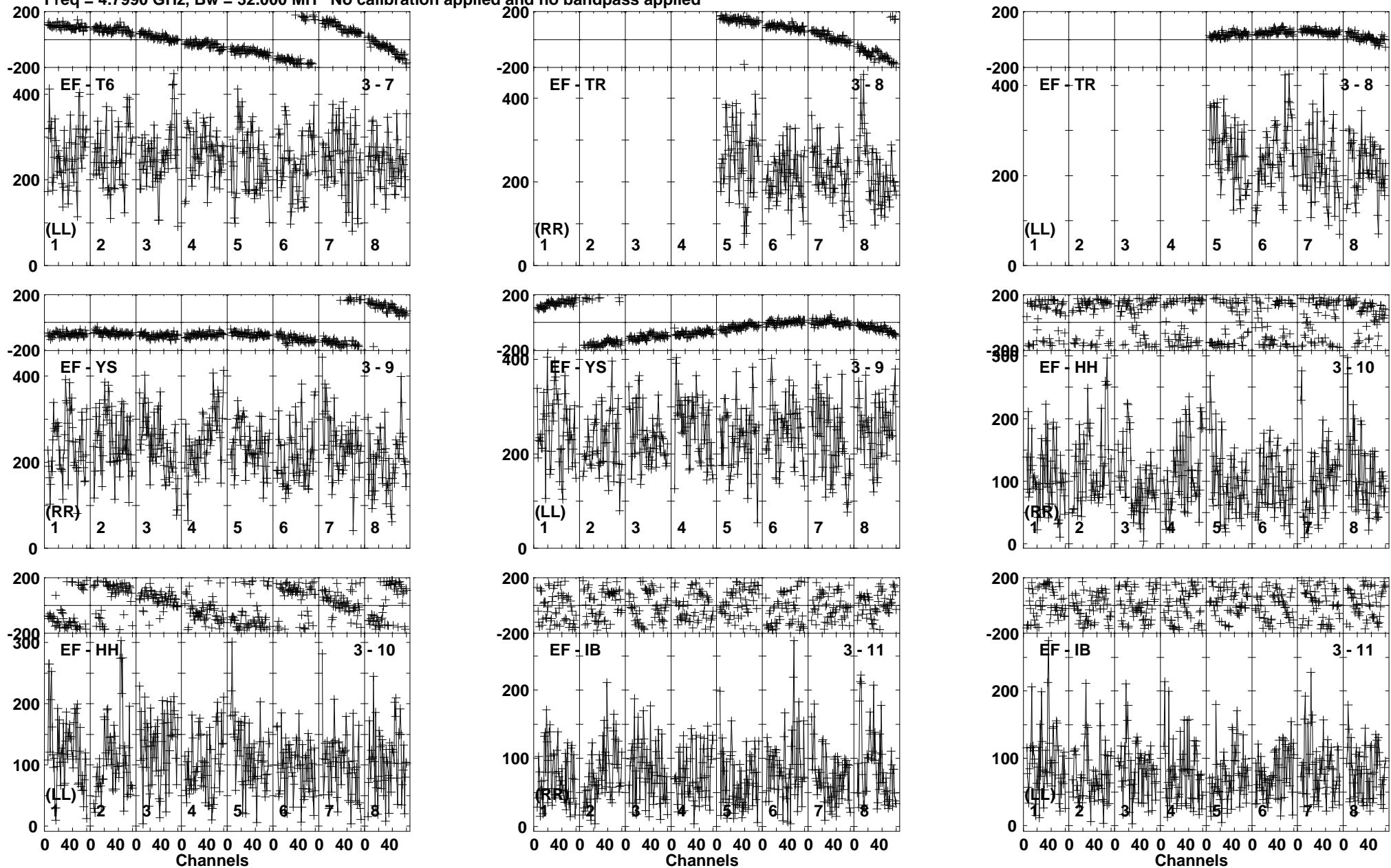
Lower frame: Micro Ampl Jy Top frame: Phas deg Vector averaged cross-power spectrum Baseline: EF (03) - T6 (07) Timerange: 00/23:32:30 to 00/23:36:00
