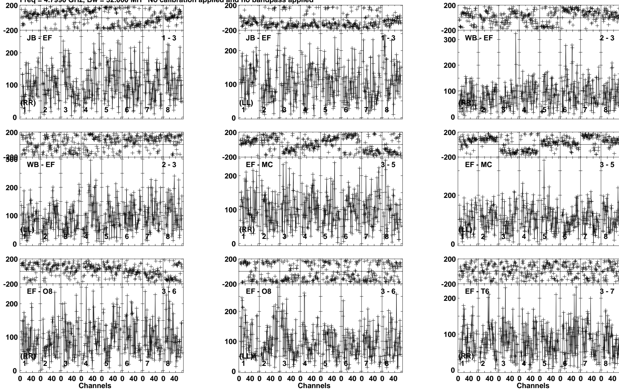
Lower frame: Micro Ampl Jy Top frame: Phas deg Vector averaged cross-power spectrum Baseline: JB (01) - EF (03) Timerange: 00/21:47:21 to 00/21:50:50
