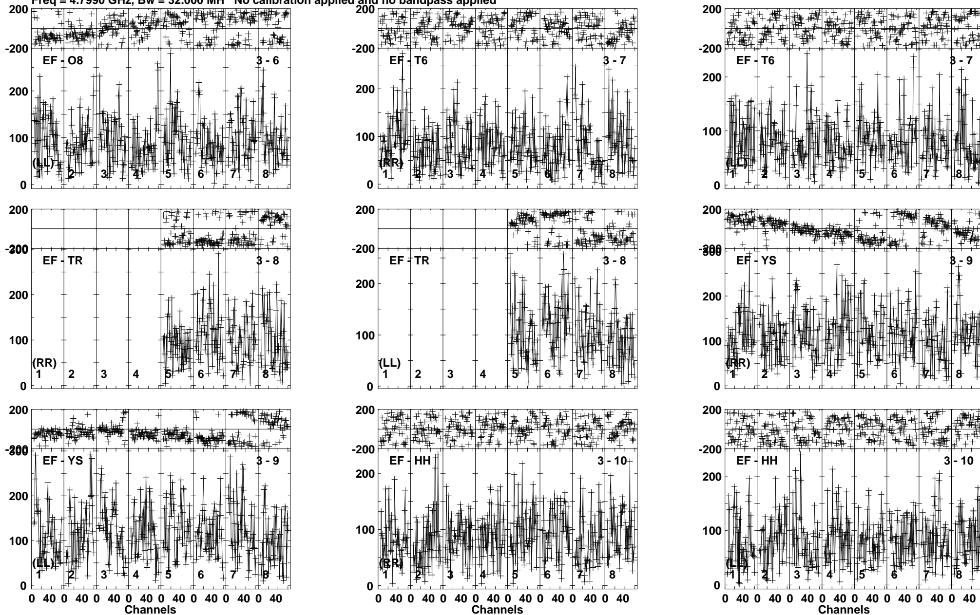
Lower frame: Micro Ampl Jy Top frame: Phas deg Vector averaged cross-power spectrum Baseline: EF (03) - O8 (06) Timerange: 00/19:56:41 to 00/20:00:10
