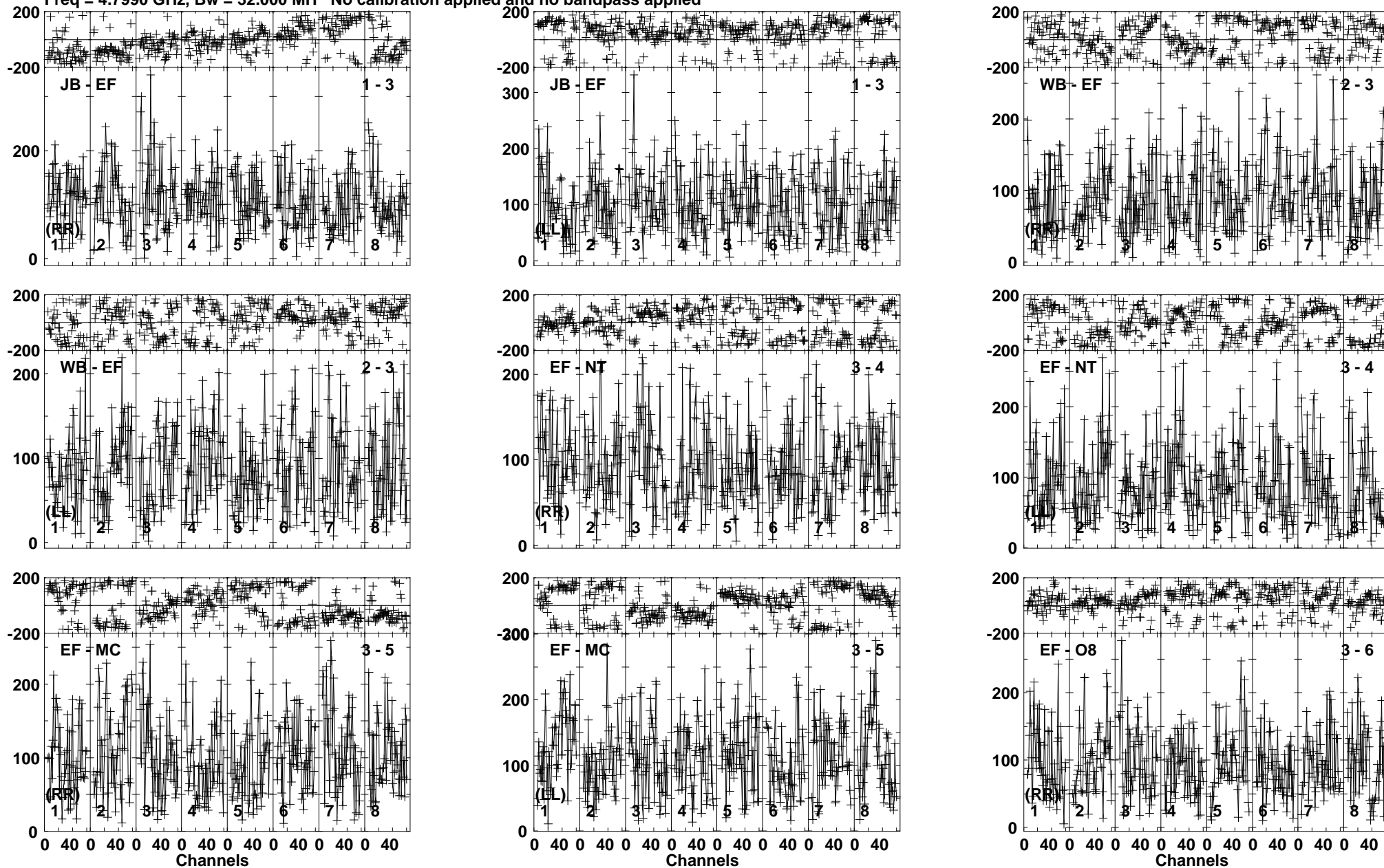
Lower frame: Micro Ampl Jy Top frame: Phas deg Vector averaged cross-power spectrum Baseline: JB (01) - EF (03) Timerange: 00/20:18:01 to 00/20:21:30
