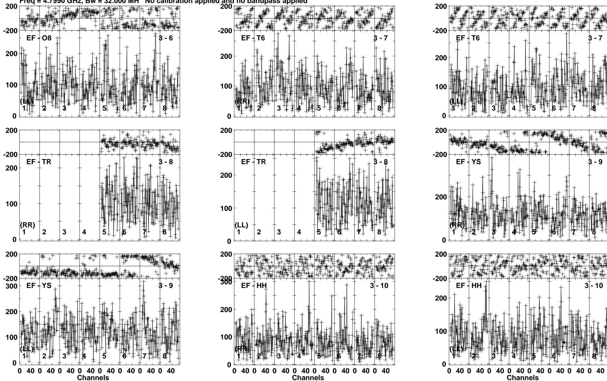
Lower frame: Micro Ampl Jy Top frame: Phas deg Vector averaged cross-power spectrum Baseline: EF (03) - O8 (06) Timerange: 00/19:35:20 to 00/19:38:49
