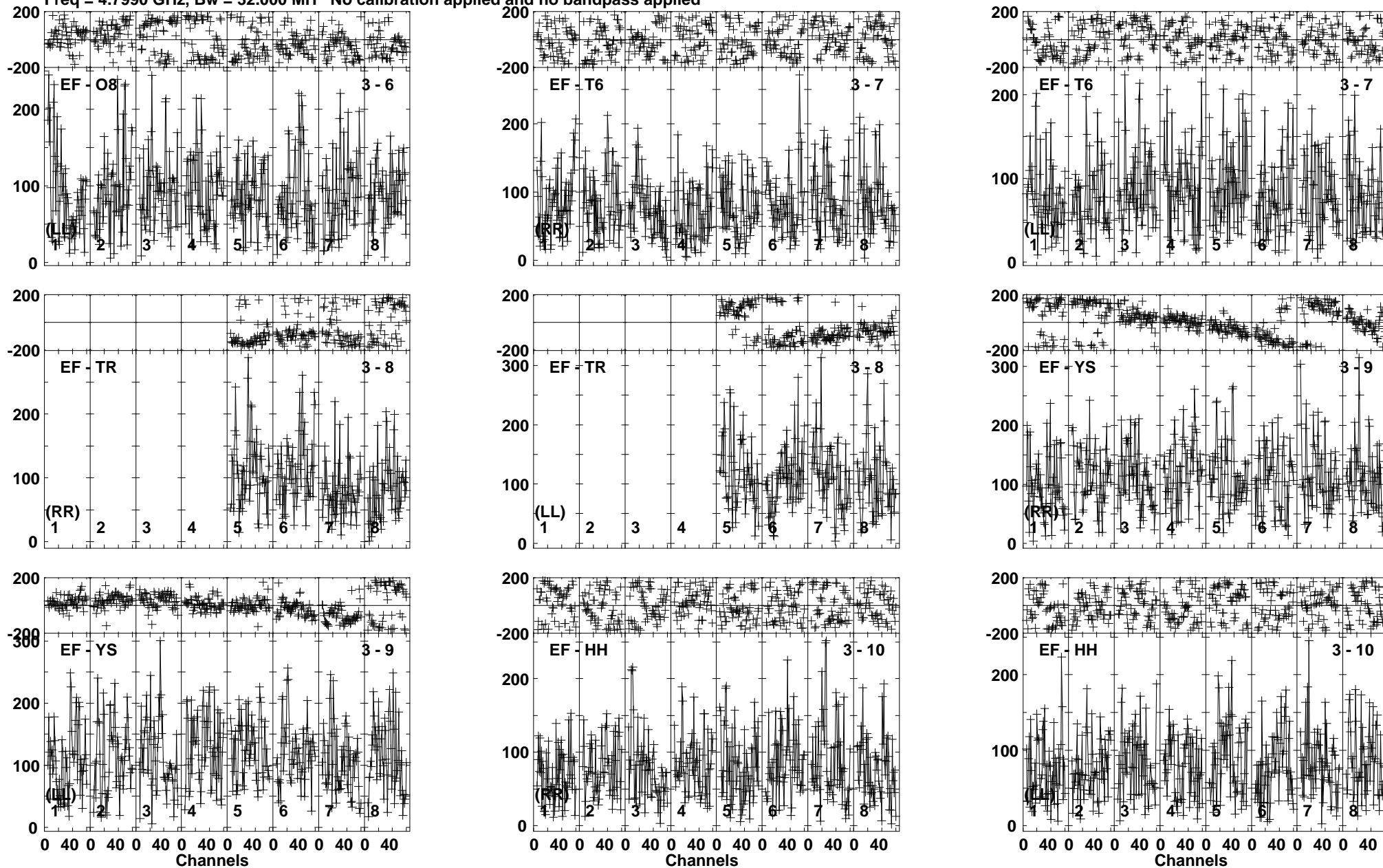
Lower frame: Micro Ampl Jy Top frame: Phas deg Vector averaged cross-power spectrum Baseline: EF (03) - O8 (06) Timerange: 00/20:07:20 to 00/20:10:49
