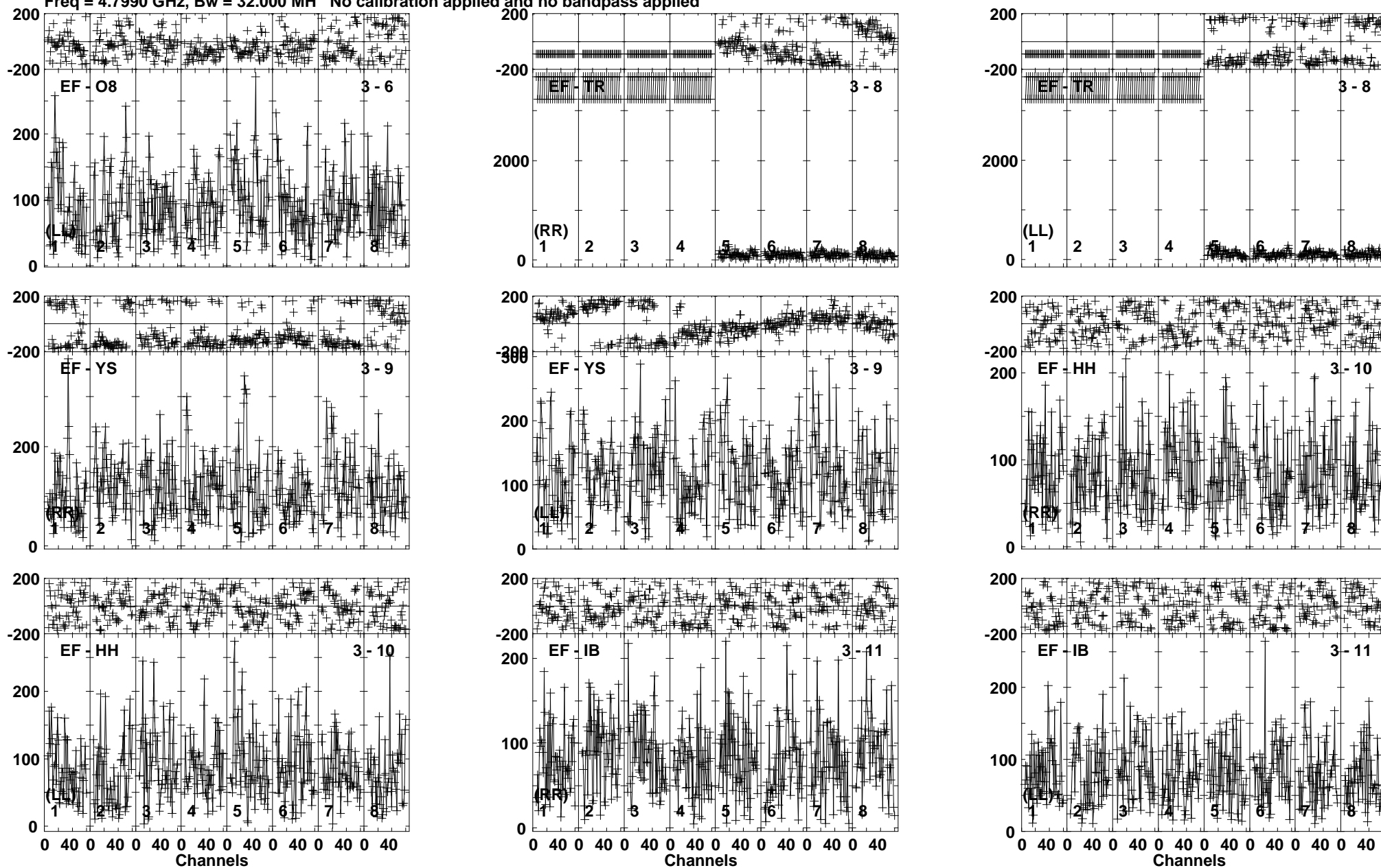
Lower frame: Micro Ampl Jy Top frame: Phas deg Vector averaged cross-power spectrum Baseline: EF (03) - O8 (06) Timerange: 01/00:24:50 to 01/00:28:19
