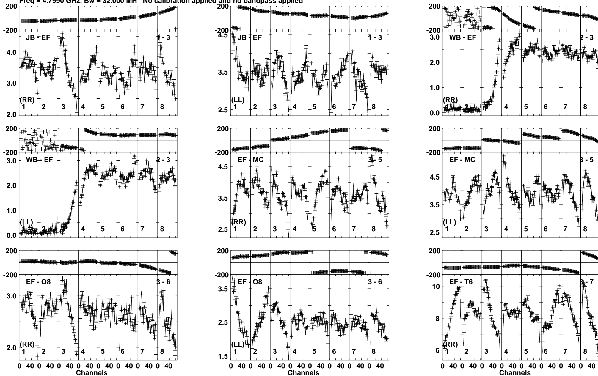
Lower frame: Milli Ampl Jy Top frame: Phas deg Vector averaged cross-power spectrum Baseline: JB (01) - EF (03) Timerange: 00/21:56:31 to 00/21:58:00
