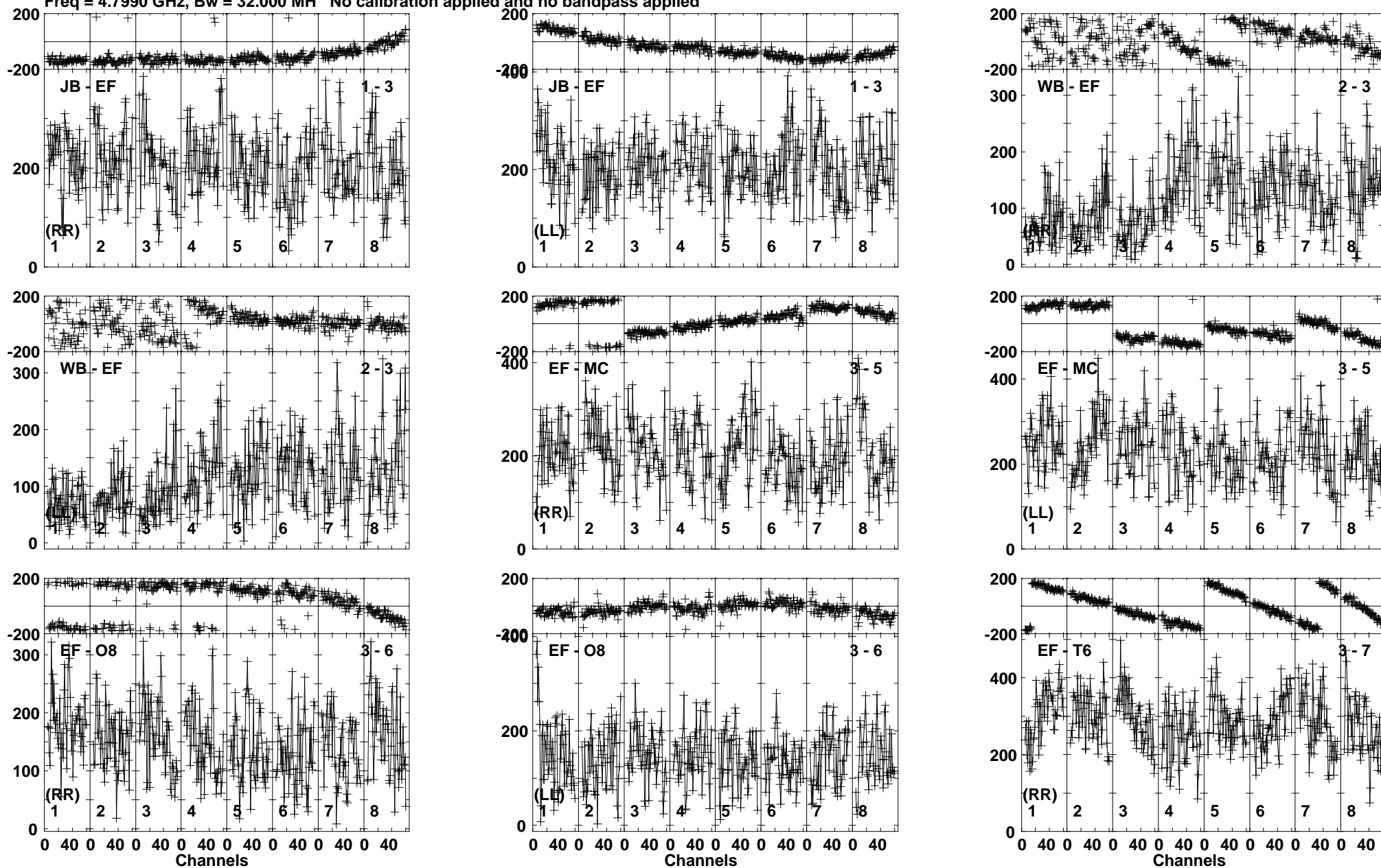
Lower frame: Micro Ampl Jy Top frame: Phas deg Vector averaged cross-power spectrum Baseline: JB (01) - EF (03) Timerange: 00/23:27:30 to 00/23:30:59
