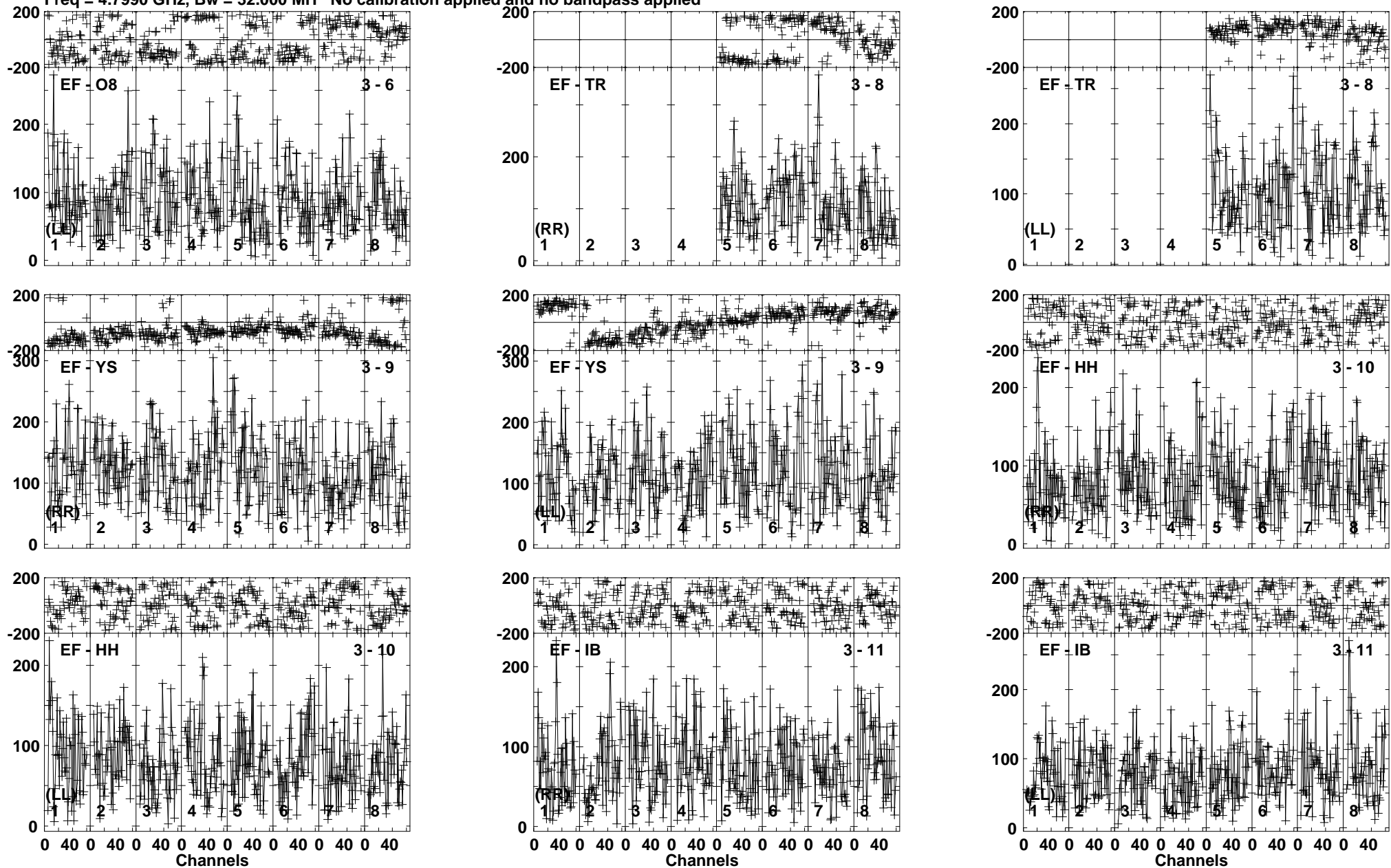
Lower frame: Micro Ampl Jy Top frame: Phas deg Vector averaged cross-power spectrum Baseline: EF (03) - O8 (06) Timerange: 01/00:29:50 to 01/00:33:19
