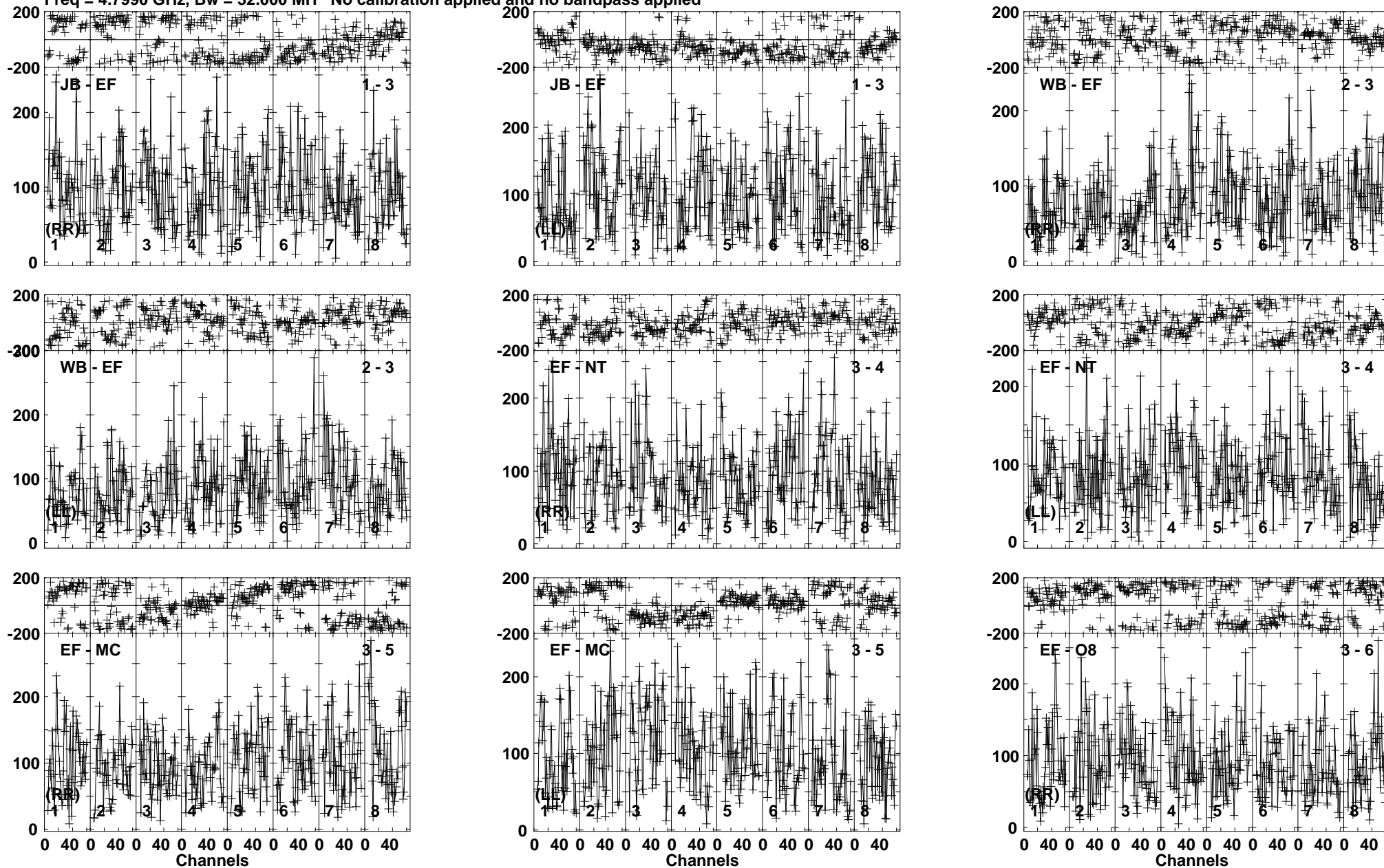
Lower frame: Micro Ampl Jy Top frame: Phas deg Vector averaged cross-power spectrum Baseline: JB (01) - EF (03) Timerange: 00:19:14:01 to 00:19:17:30
