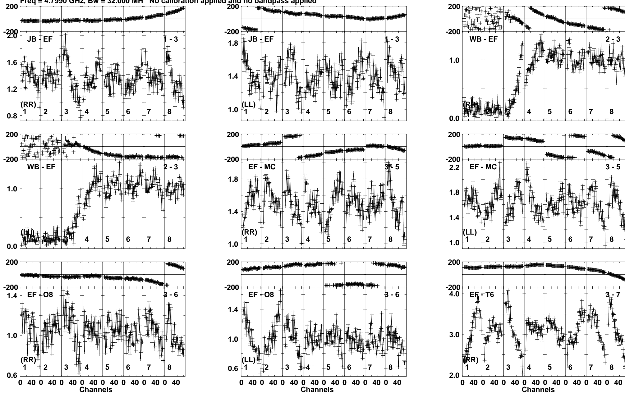
Lower frame: Milli Ampl Jy Top frame: Phas deg Vector averaged cross-power spectrum Baseline: JB (01) - EF (03) Timerange: 00/22:48:21 to 00/22:49:50
