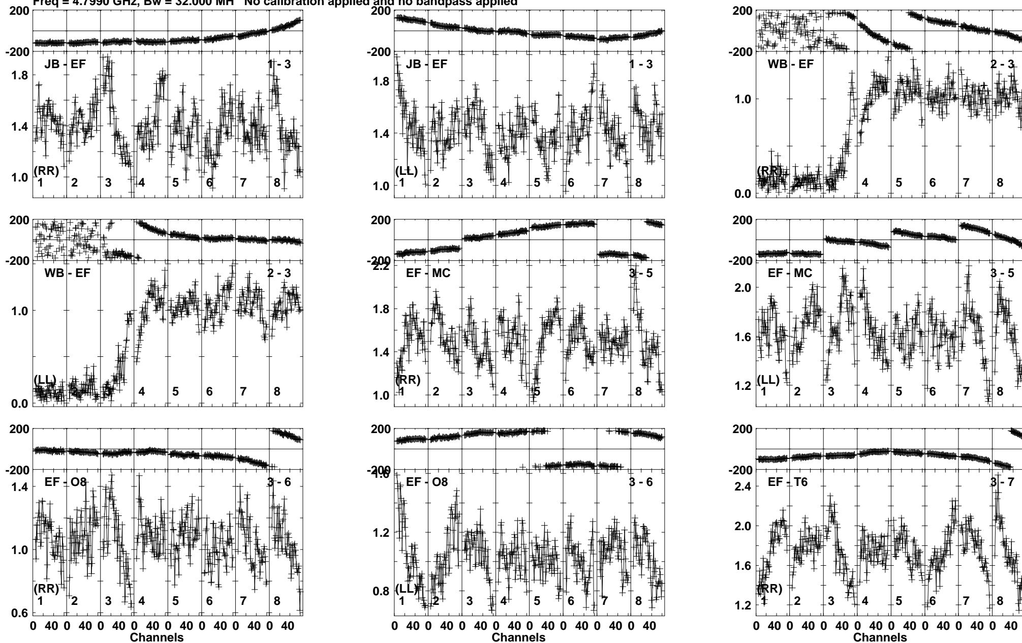
Lower frame: Milli Ampl Jy Top frame: Phas deg Vector averaged cross-power spectrum Baseline: JB (01) - EF (03) Timerange: 00/23:09:40 to 00/23:11:09
