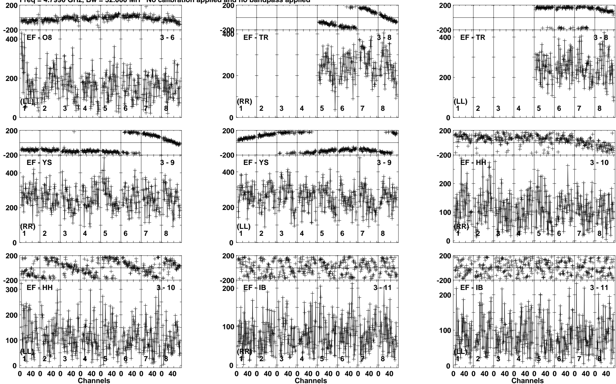
Lower frame: Micro Ampl Jy Top frame: Phas deg Vector averaged cross-power spectrum Baseline: EF (03) - O8 (06) Timerange: 01/01:44:00 to 01/01:47:29
