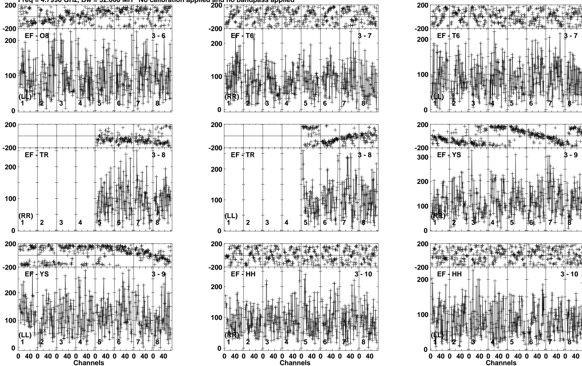
Lower frame: Micro Ampl Jy Top frame: Phas deg Vector averaged cross-power spectrum Baseline: EF (03) - O8 (06) Timerange: 00/20:28:41 to 00/20:32:10
