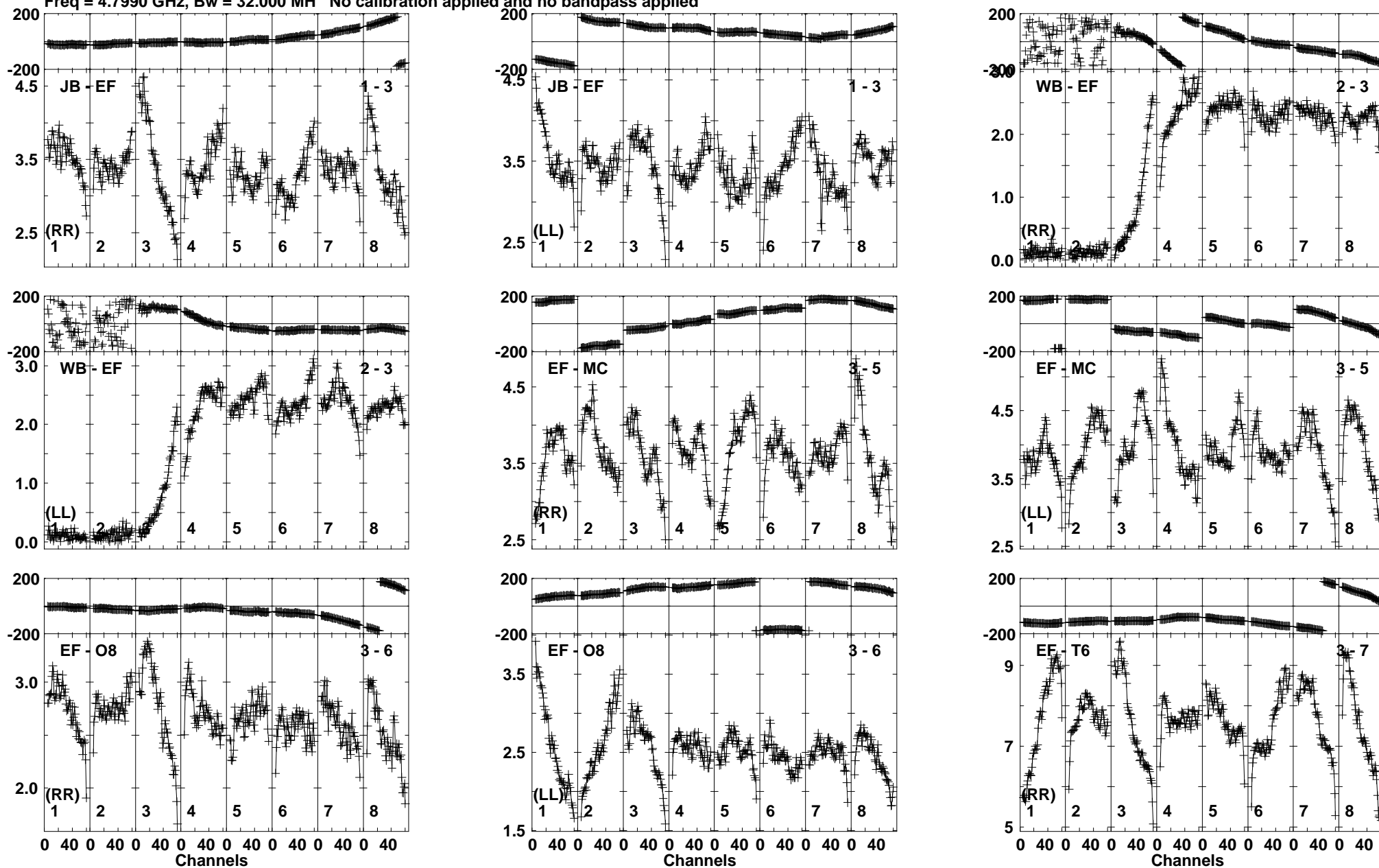
Lower frame: Milli Ampl Jy Top frame: Phas deg Vector averaged cross-power spectrum Baseline: JB (01) - EF (03) Timerange: 00/22:02:10 to 00/22:03:39
