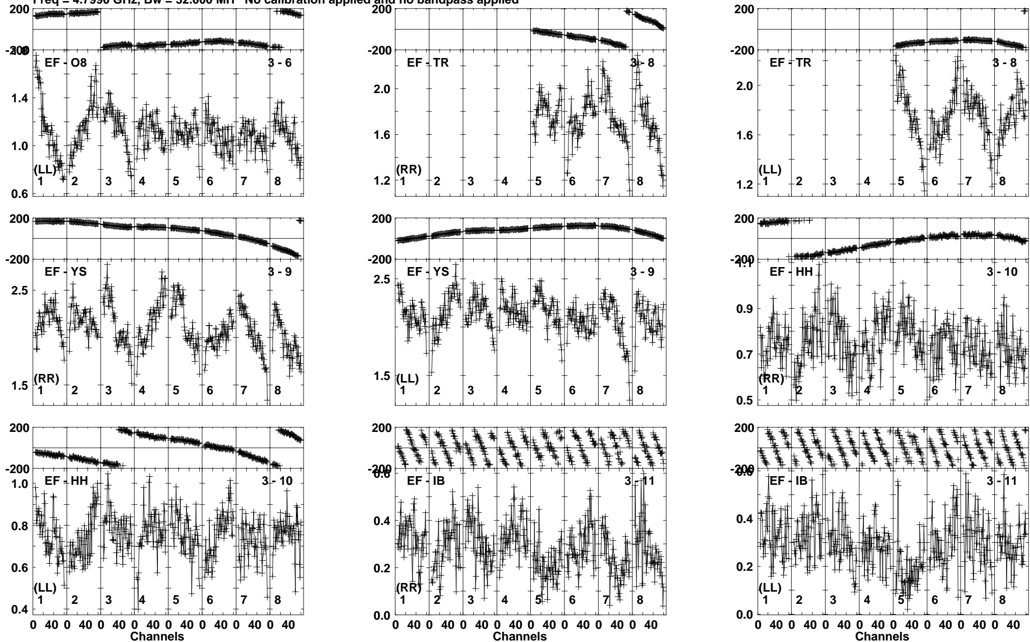
Lower frame: Milli Ampl Jy Top frame: Phas deg Vector averaged cross-power spectrum Baseline: EF (03) - O8 (06) Timerange: 01/01:31:50 to 01/01:33:20
