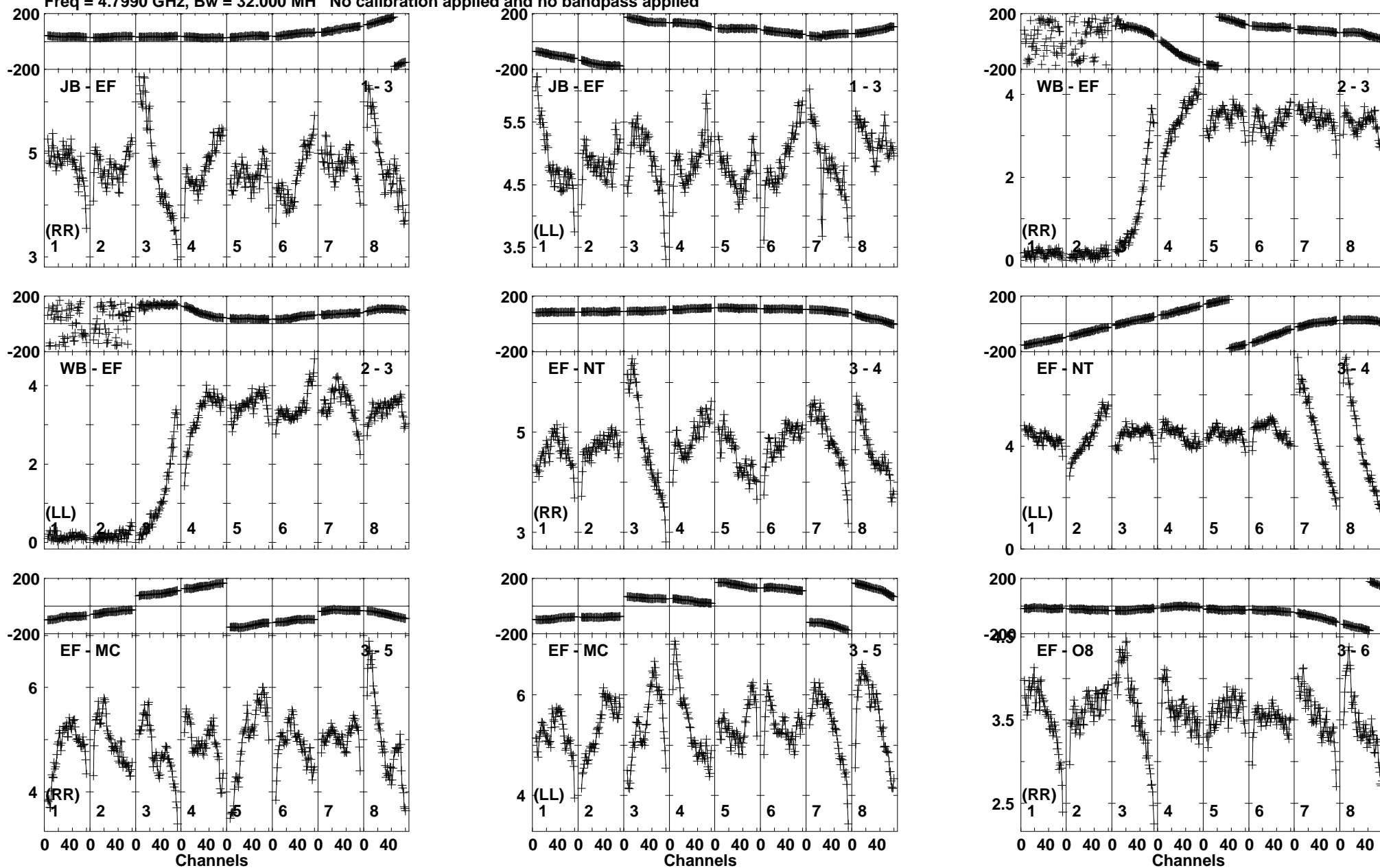
Lower frame: Milli Ampl Jy Top frame: Phas deg Vector averaged cross-power spectrum Baseline: JB (01) - EF (03) Timerange: 00/19:33:51 to 00/19:35:20
