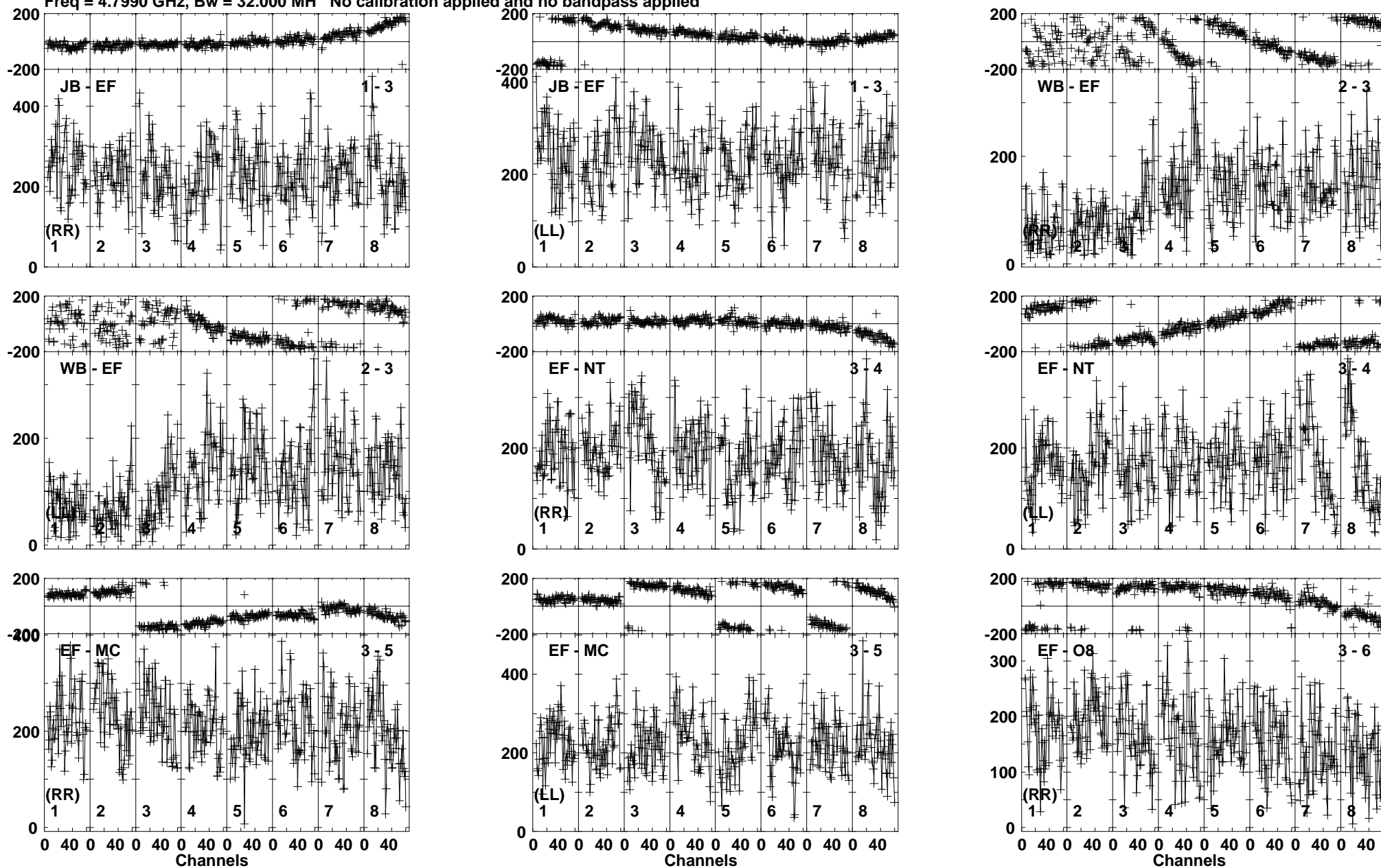
Lower frame: Micro Ampl Jy Top frame: Phas deg Vector averaged cross-power spectrum Baseline: JB (01) - EF (03) Timerange: 01/01:49:01 to 01/01:52:30
