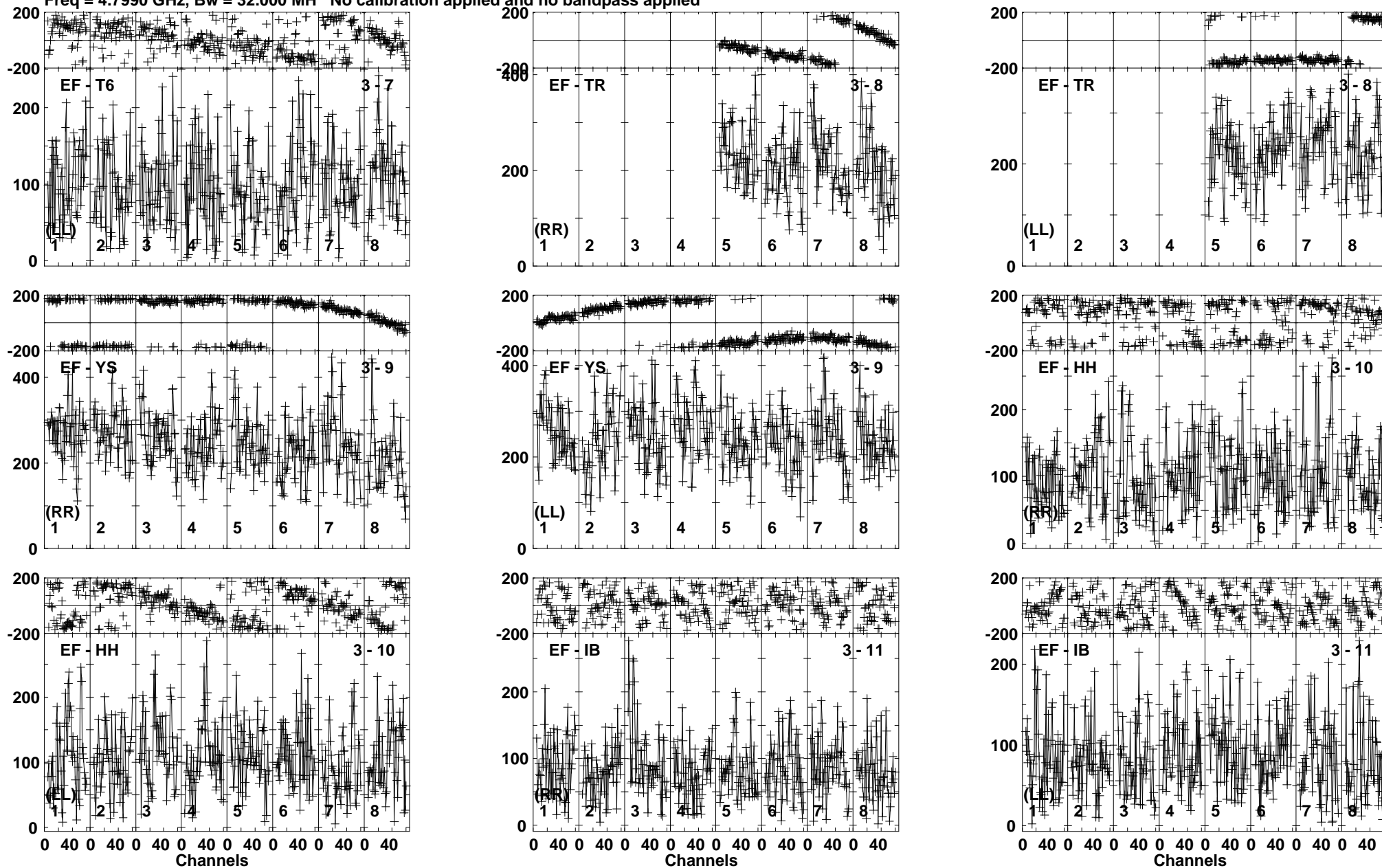
Lower frame: Micro Ampl Jy Top frame: Phas deg Vector averaged cross-power spectrum Baseline: EF (03) - T6 (07) Timerange: 00/23:48:51 to 00/23:52:20
