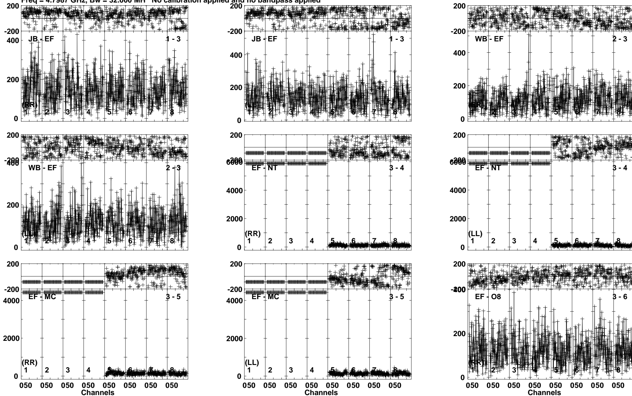
Lower frame: Micro Ampl Jy Top frame: Phas deg Vector averaged cross-power spectrum Baseline: JB (01) - EF (03) Timerange: 00/14:48:30 to 00/14:51:59
