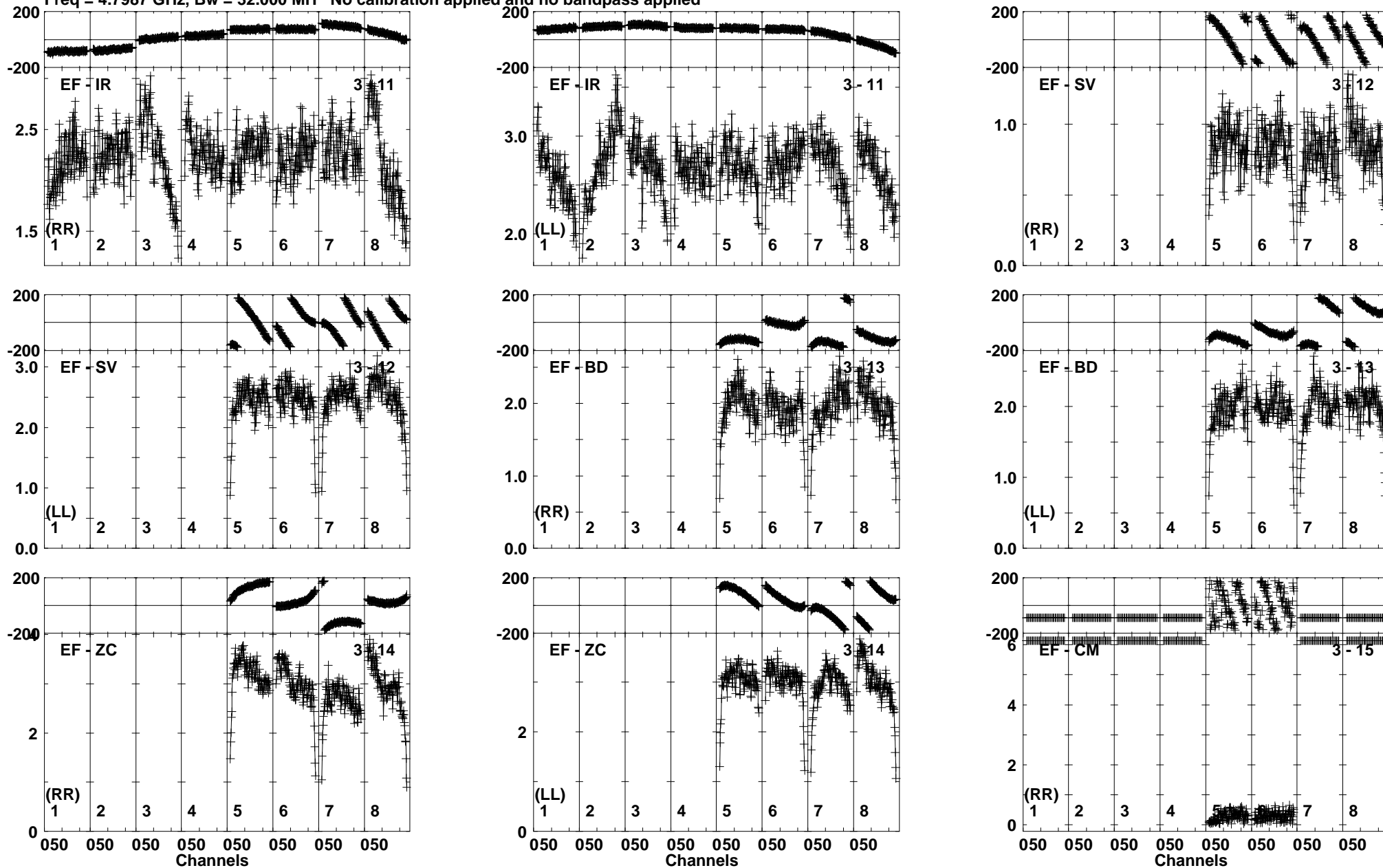
Lower frame: Milli Ampl Jy Top frame: Phas deg Vector averaged cross-power spectrum Baseline: EF (03) - IR (11) Timerange: 00/18:23:31 to 00/18:24:29
