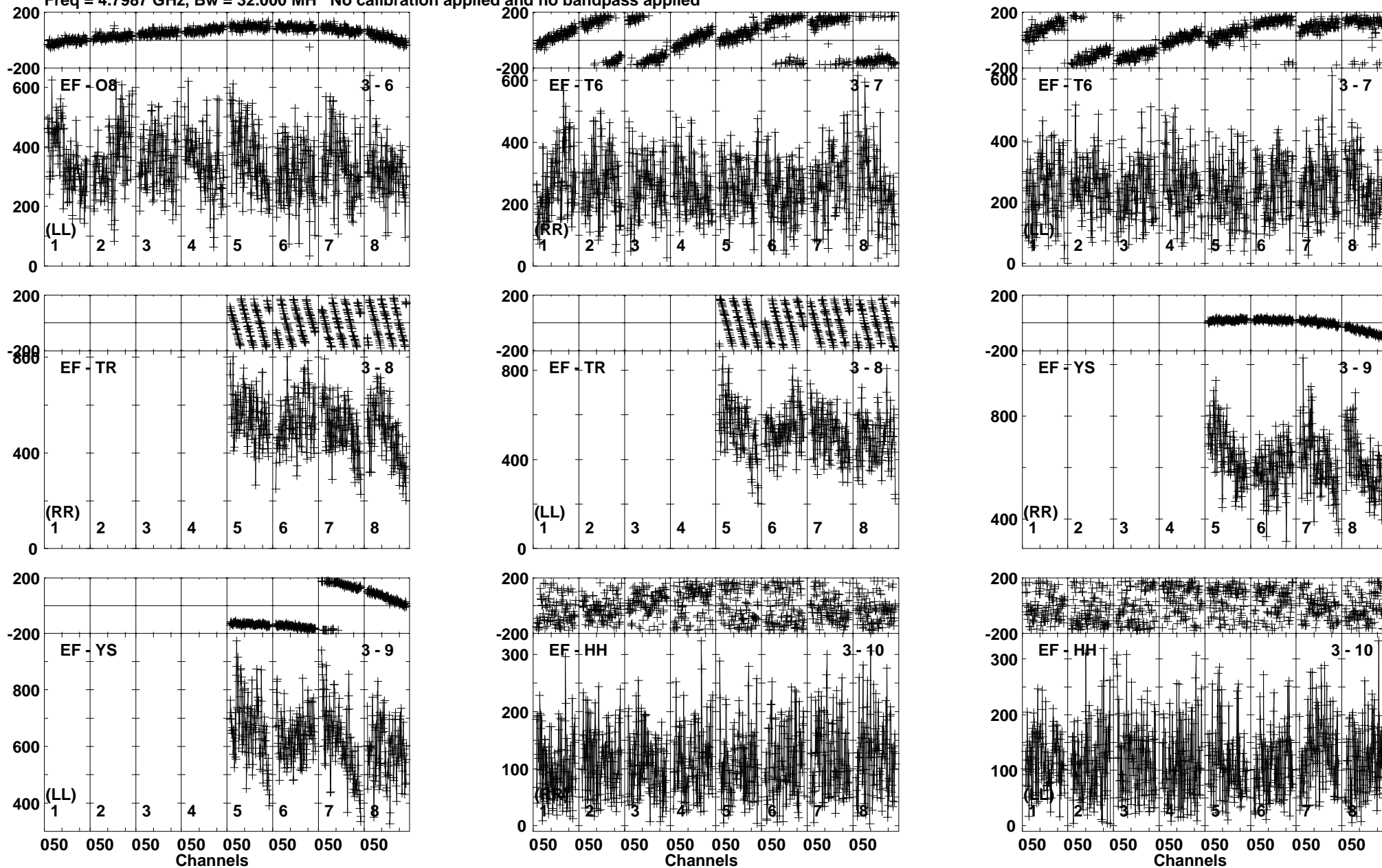
Lower frame: Micro Ampl Jy Top frame: Phas deg Vector averaged cross-power spectrum Baseline: EF (03) - O8 (06) Timerange: 00:18:34:30 to 00:18:37:59
