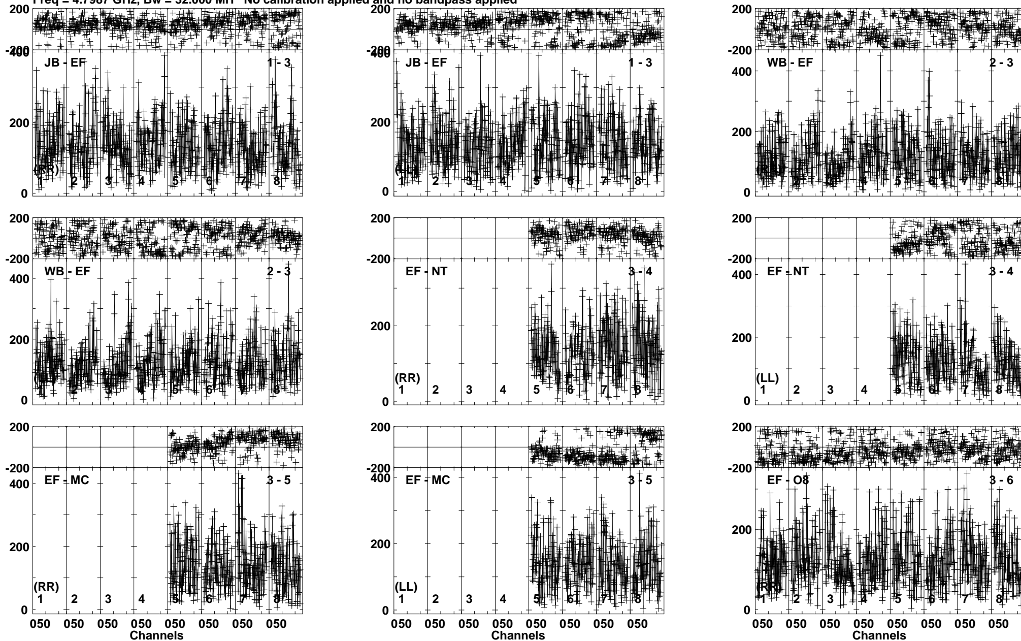
Lower frame: Micro Ampl Jy Top frame: Phas deg Vector averaged cross-power spectrum Baseline: JB (01) - EF (03) Timerange: 00/15:58:30 to 00/16:01:59
