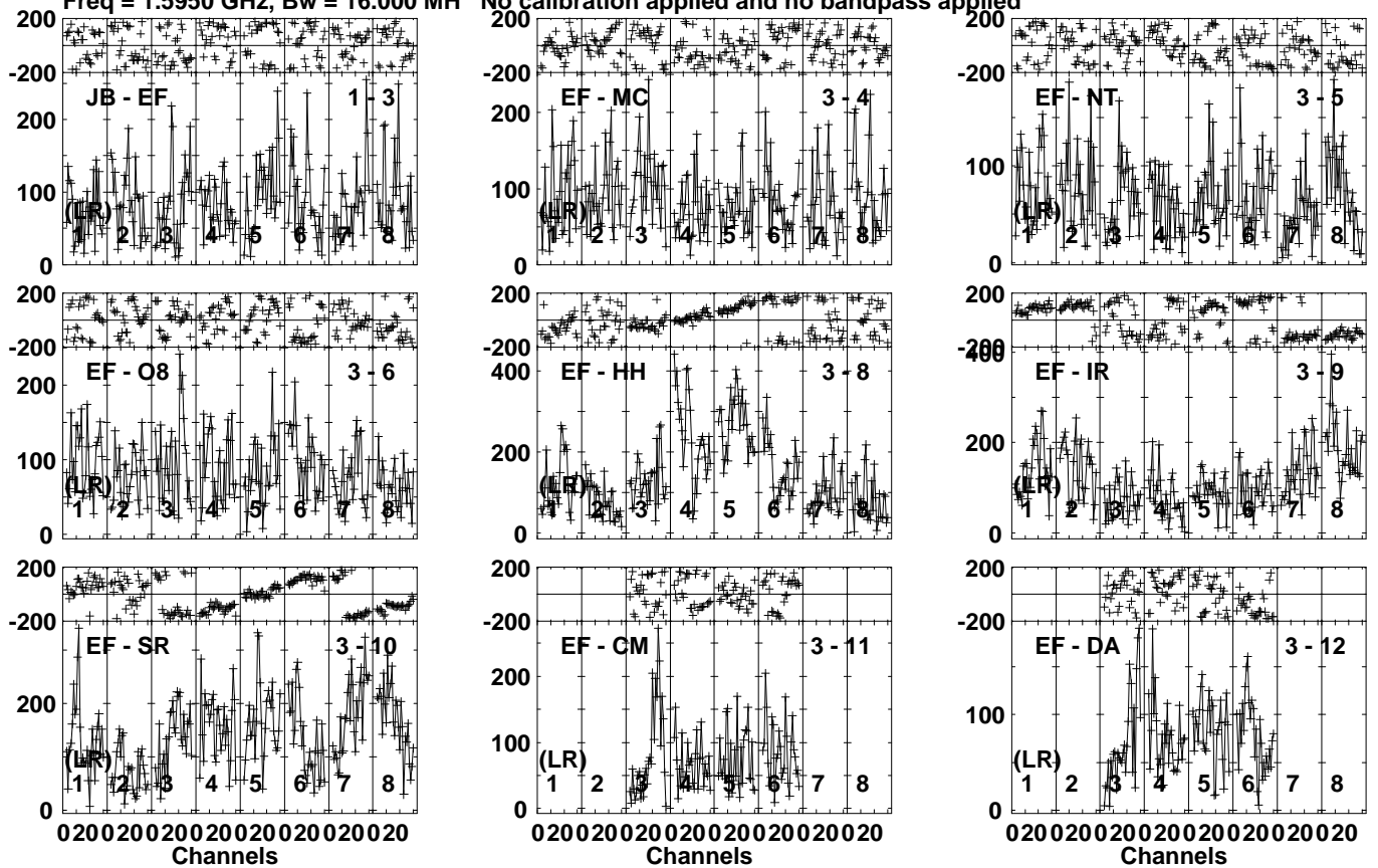
Lower frame: Micro Ampl Jy Top frame: Phas deg Vector averaged cross-power spectrum Several baselines displayed Timerange: 00/11:24:30 to 00/11:28:00
