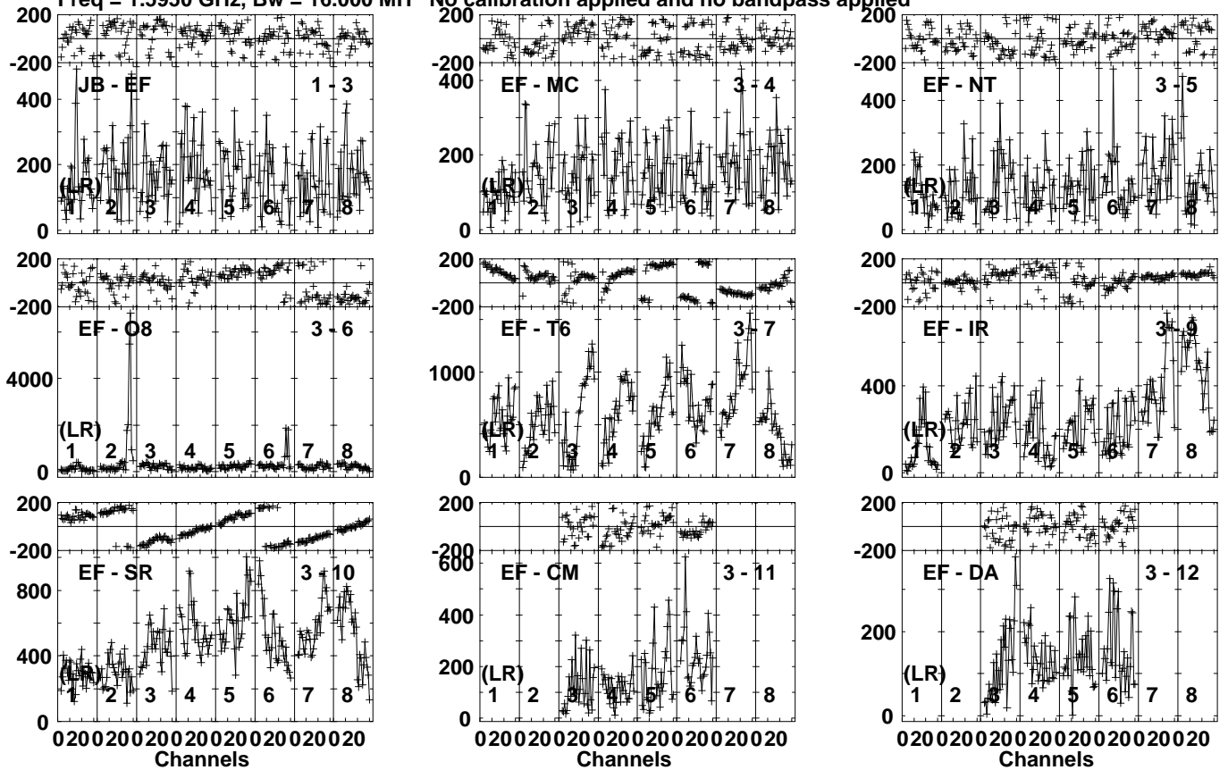
Lower frame: Micro Ampl Jy Top frame: Phas deg Vector averaged cross-power spectrum Several baselines displayed Timerange: 00/09:16:30 to 00/09:17:29
