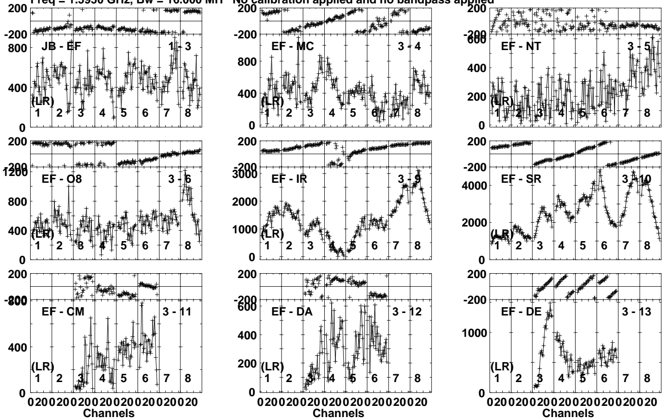
Lower frame: Micro Ampl Jy Top frame: Phas deg Vector averaged cross-power spectrum Several baselines displayed Timerange: 00/12:05:00 to 00/12:06:29
