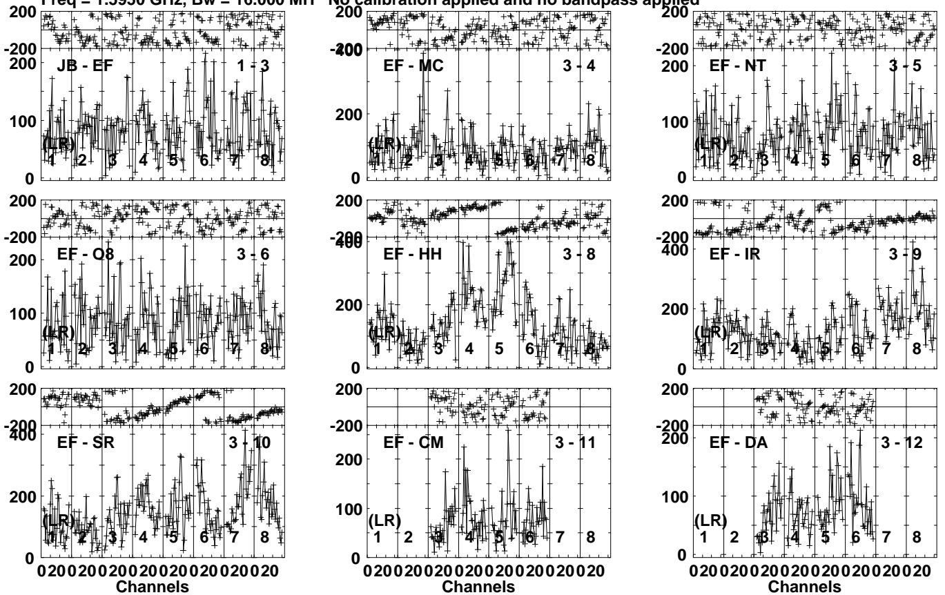
Lower frame: Micro Ampl Jy Top frame: Phas deg Vector averaged cross-power spectrum Several baselines displayed Timerange: 00/11:34:31 to 00/11:38:00
