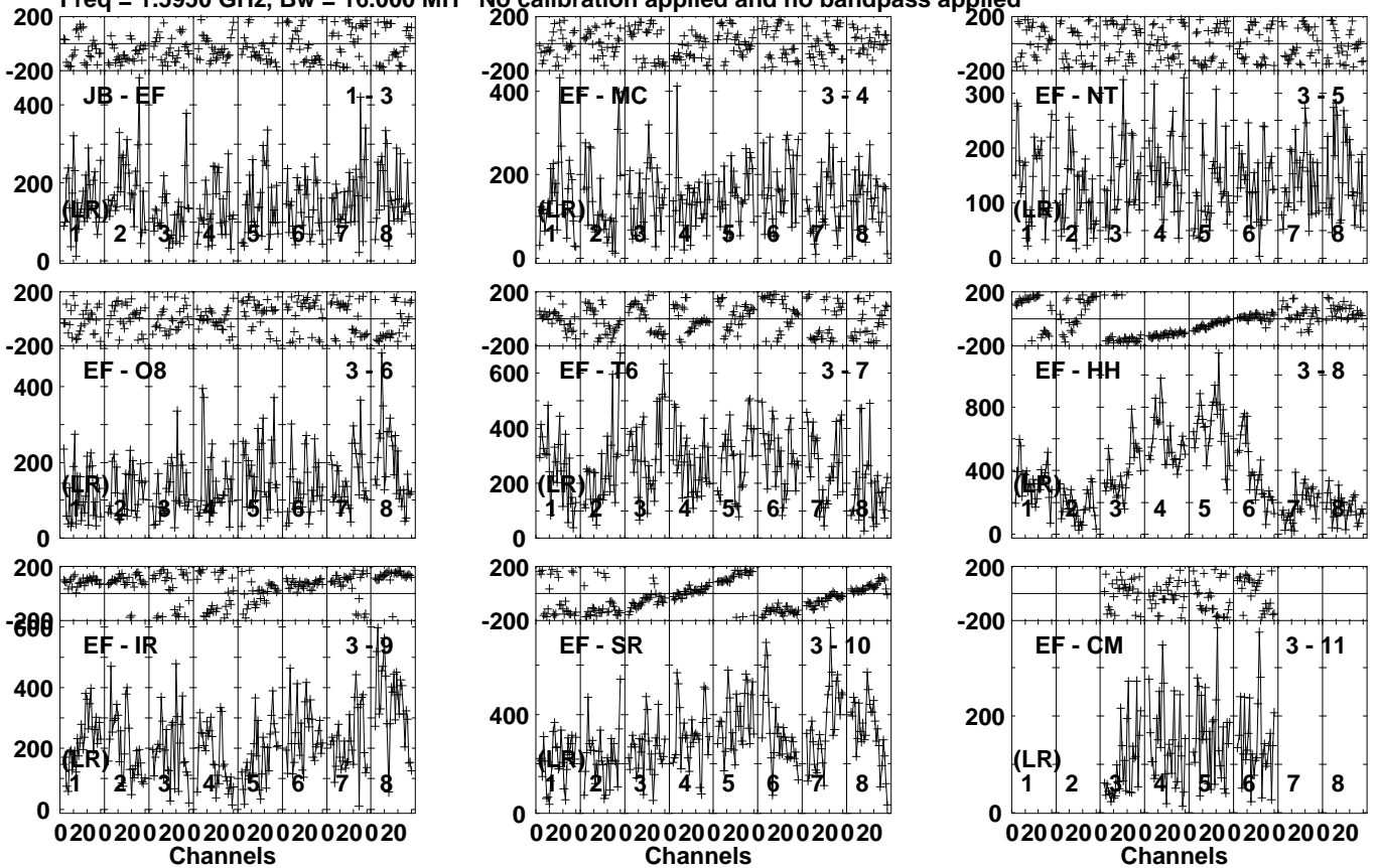
Lower frame: Micro Ampl Jy Top frame: Phas deg Vector averaged cross-power spectrum Several baselines displayed Timerange: 00/07:06:01 to 00/07:07:30
