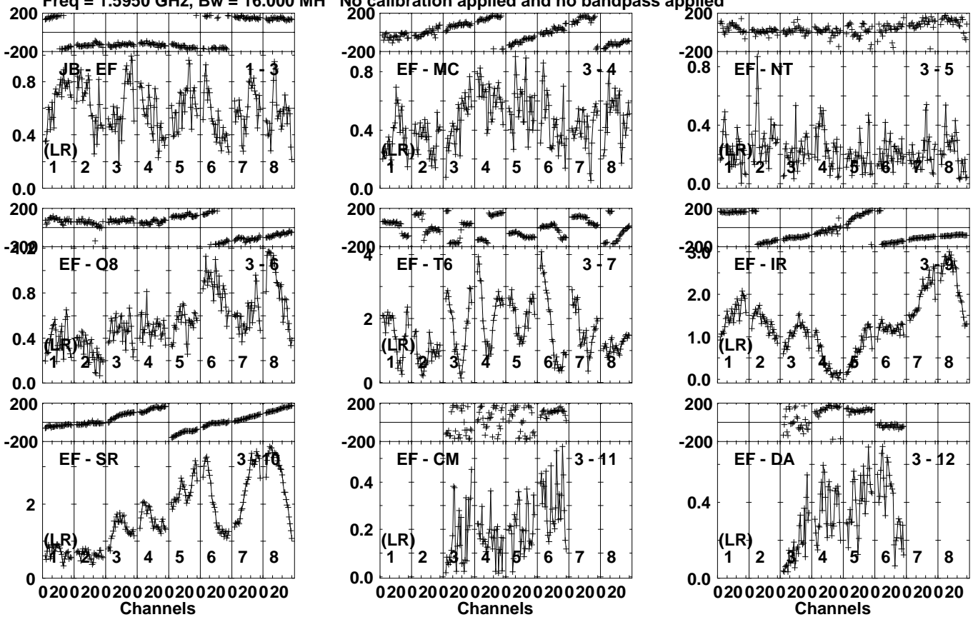
Lower frame: Milli Ampl Jy Top frame: Phas deg Vector averaged cross-power spectrum Several baselines displayed Timerange: 00/05:40:30 to 00/05:41:59
