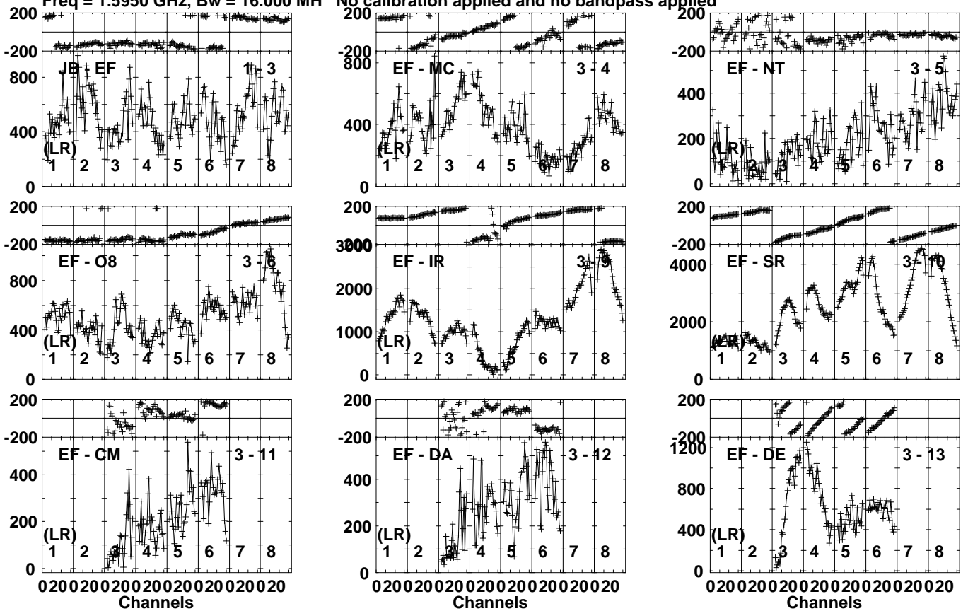
Lower frame: Micro Ampl Jy Top frame: Phas deg Vector averaged cross-power spectrum Several baselines displayed Timerange: 00/11:59:30 to 00/12:01:29
