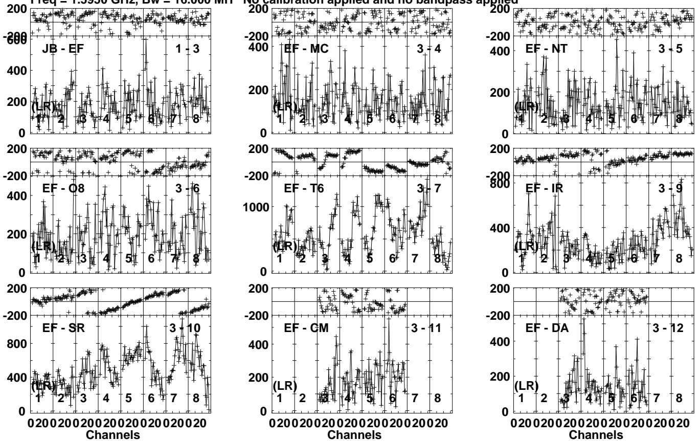
Lower frame: Micro Ampl Jy Top frame: Phas deg Vector averaged cross-power spectrum Several baselines displayed Timerange: 00/08:11:01 to 00/08:12:30
