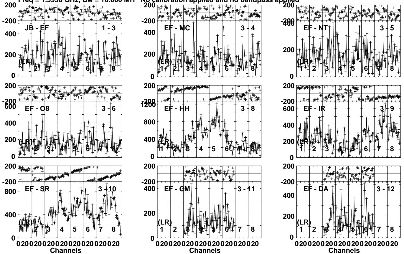
Lower frame: Micro Ampl Jy Top frame: Phas deg Vector averaged cross-power spectrum Several baselines displayed Timerange: 00/11:08:31 to 00/11:09:30
