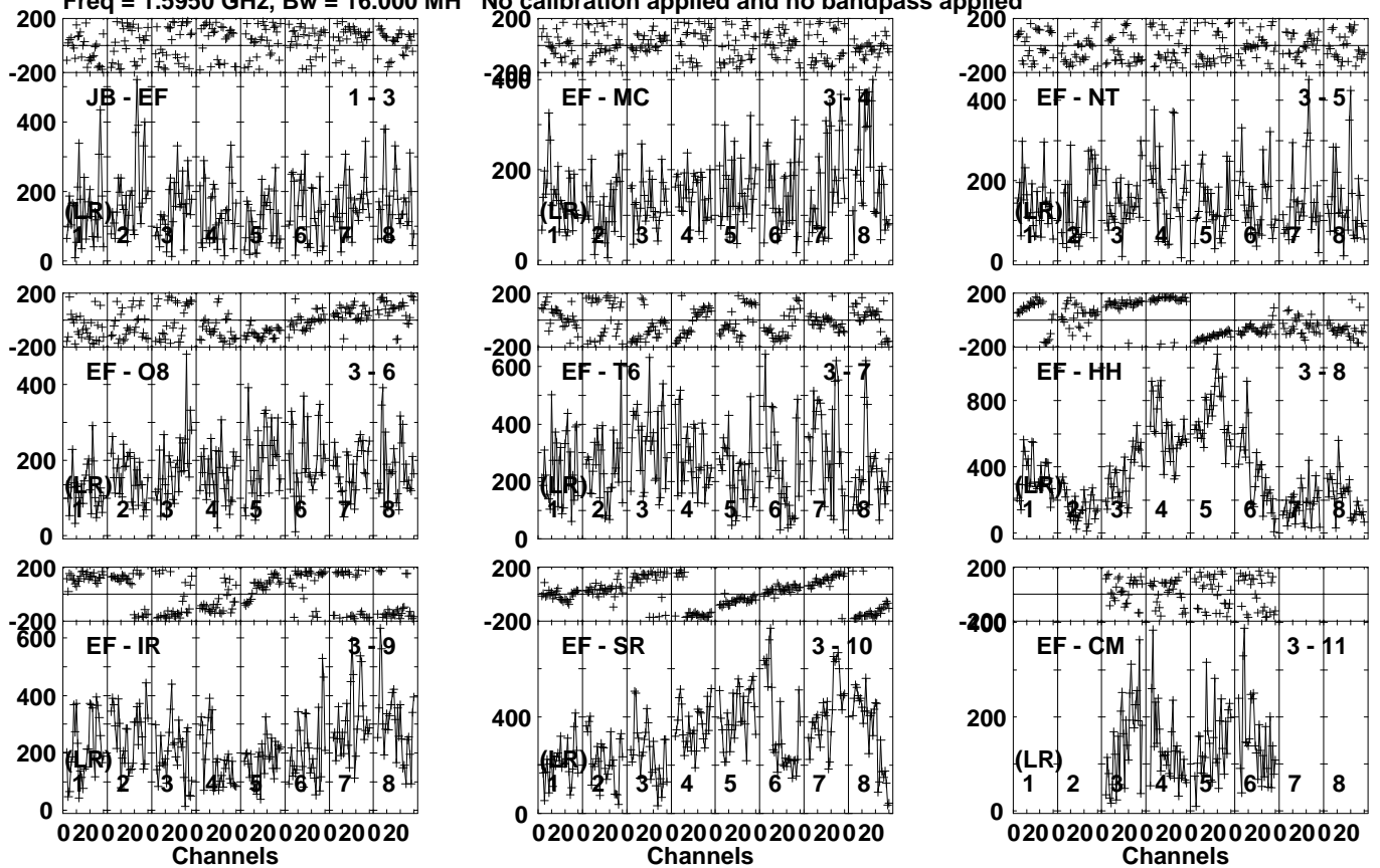
Lower frame: Micro Ampl Jy Top frame: Phas deg Vector averaged cross-power spectrum Several baselines displayed Timerange: 00/08:01:30 to 00/08:02:29
