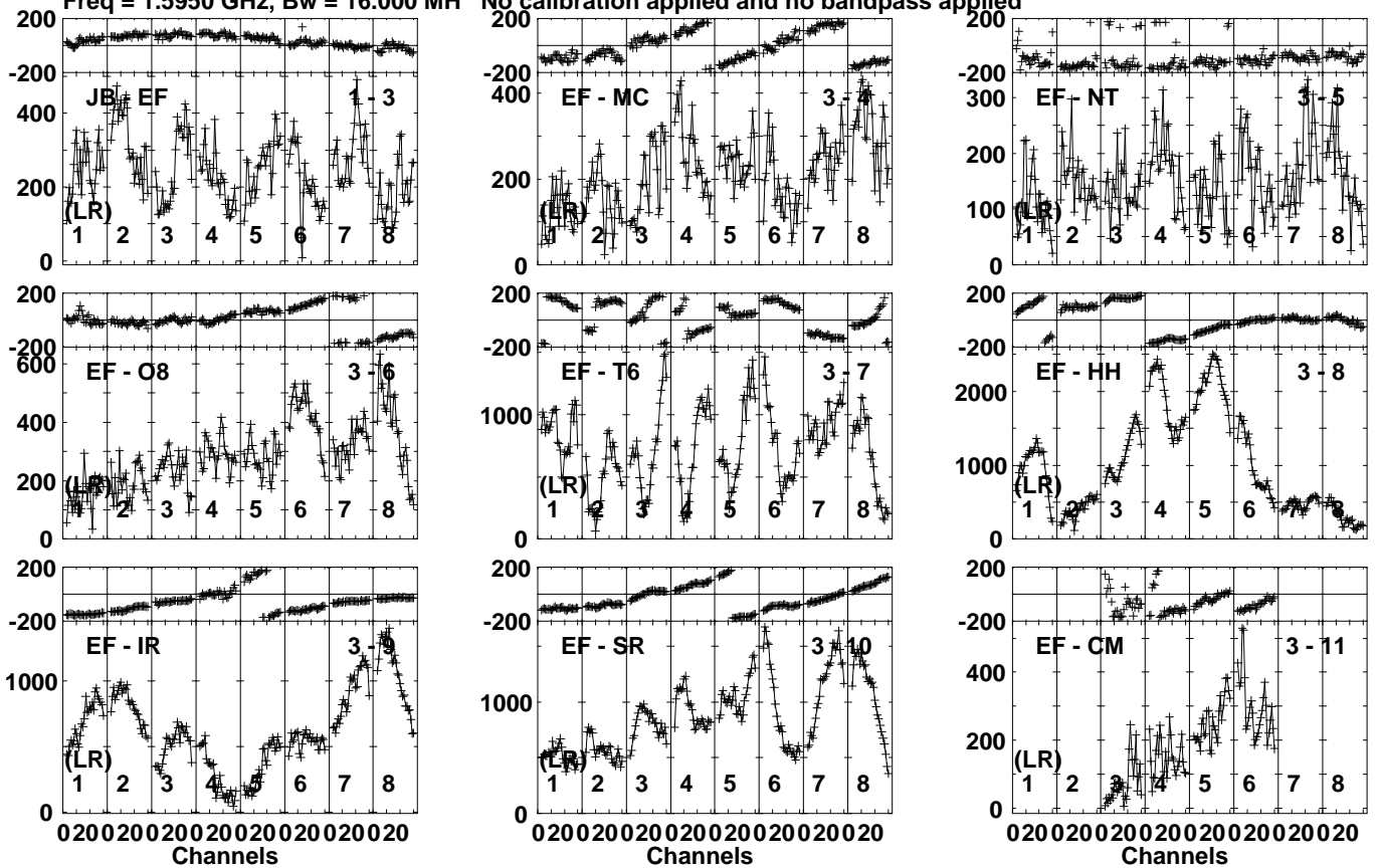
Lower frame: Micro Ampl Jy Top frame: Phas deg Vector averaged cross-power spectrum Several baselines displayed Timerange: 00/05:00:06 to 00/05:03:59
