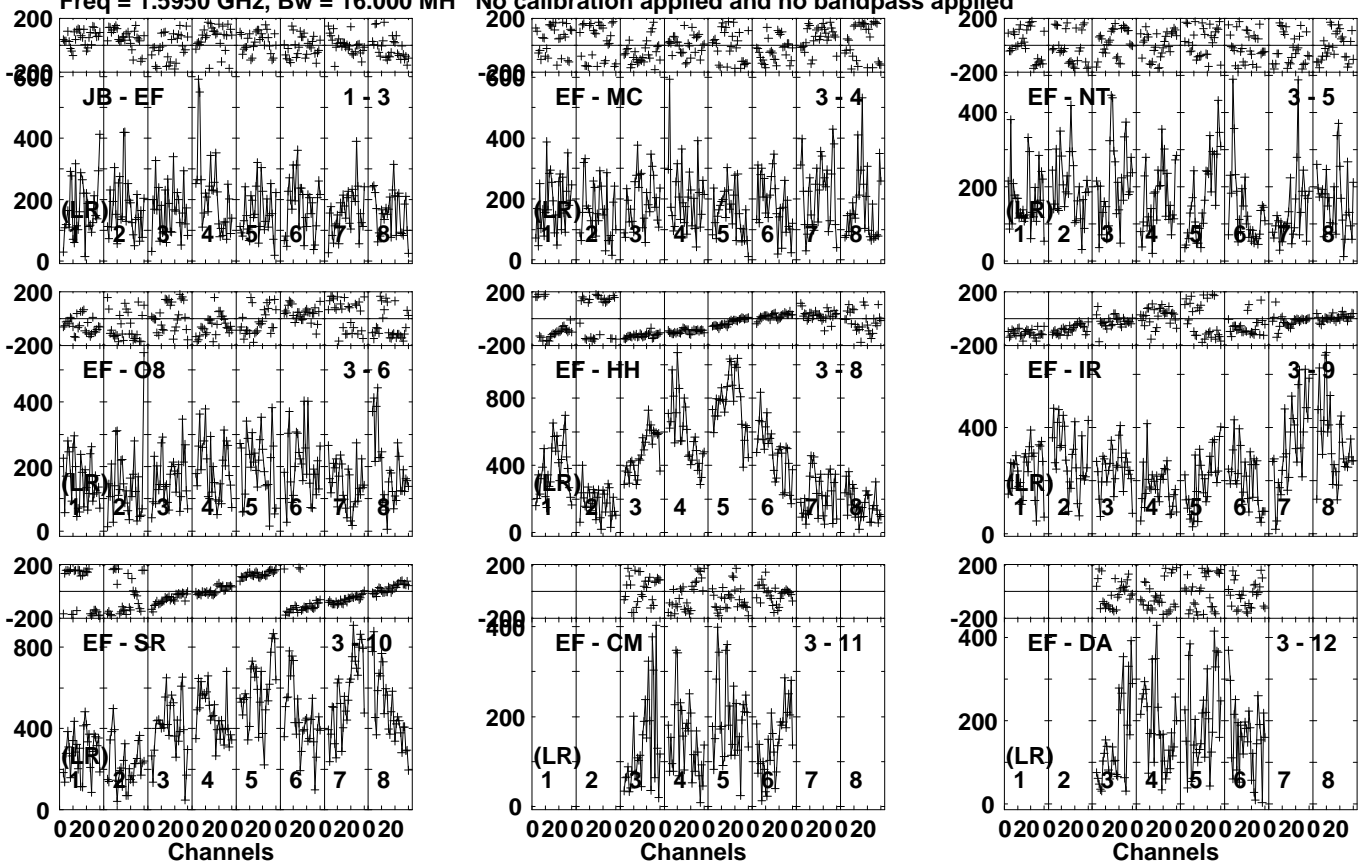
Lower frame: Micro Ampl Jy Top frame: Phas deg Vector averaged cross-power spectrum Several baselines displayed Timerange: 00/11:53:31 to 00/11:54:30
