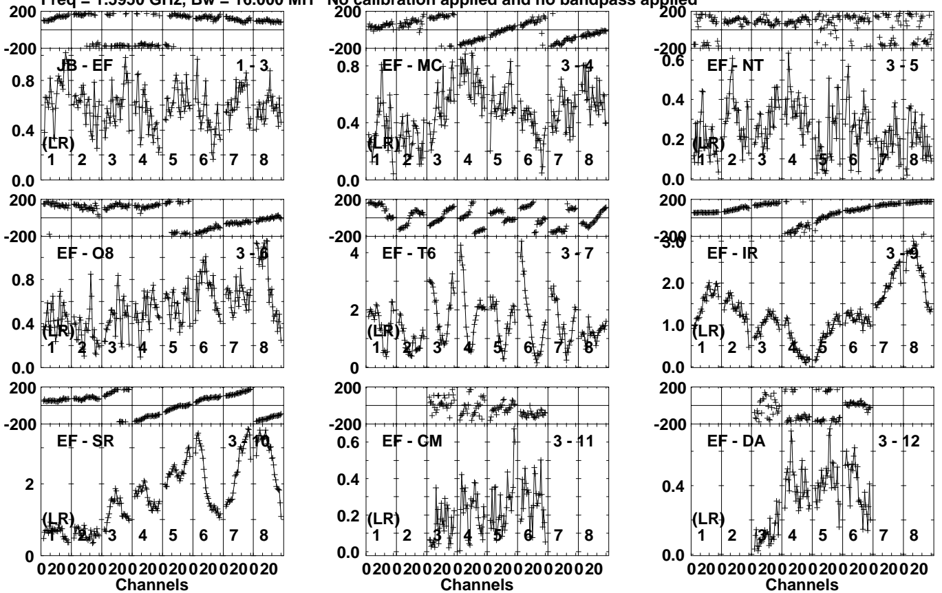
Lower frame: Milli Ampl Jy Top frame: Phas deg Vector averaged cross-power spectrum Several baselines displayed Timerange: 00/05:50:30 to 00/05:51:59
