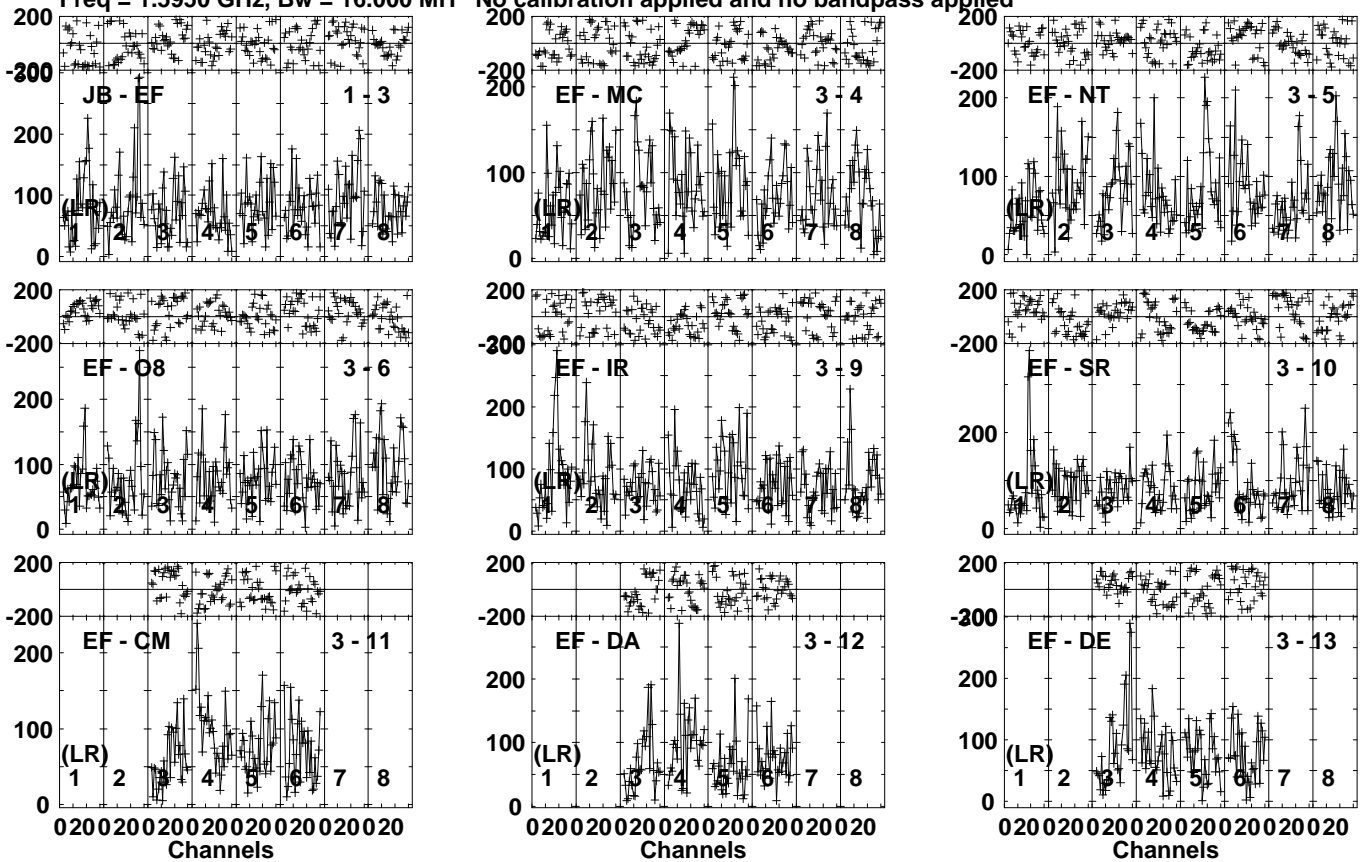
Lower frame: Micro Ampl Jy Top frame: Phas deg Vector averaged cross-power spectrum Several baselines displayed Timerange: 00/12:16:30 to 00/12:20:00
