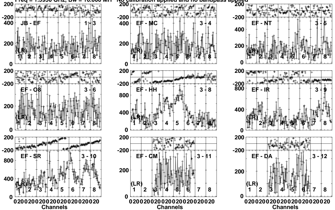
Lower frame: Micro Ampl Jy Top frame: Phas deg Vector averaged cross-power spectrum Several baselines displayed Timerange: 00/11:28:31 to 00/11:29:29
