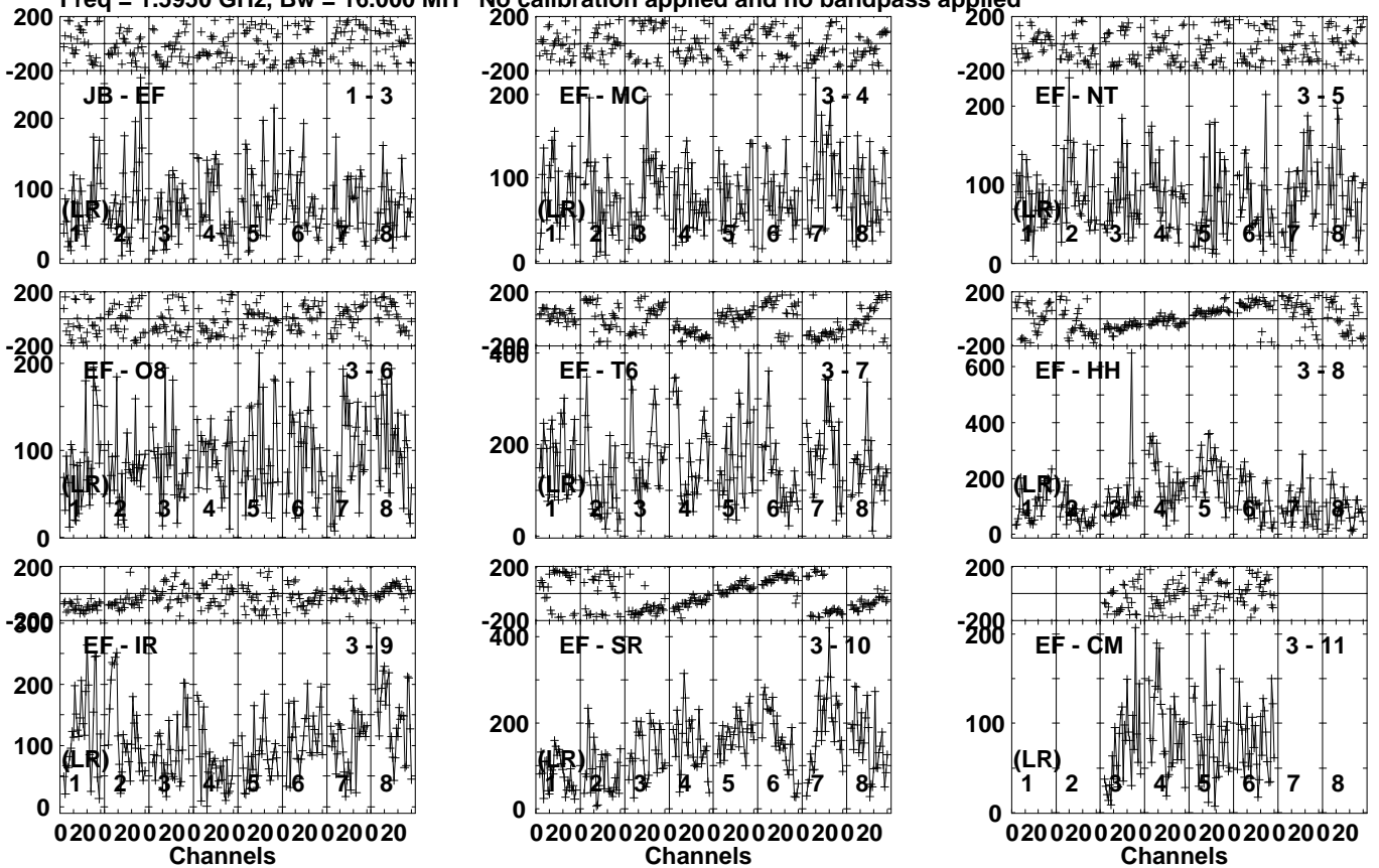
Lower frame: Micro Ampl Jy Top frame: Phas deg Vector averaged cross-power spectrum Several baselines displayed Timerange: 00/06:57:31 to 00/07:01:00
