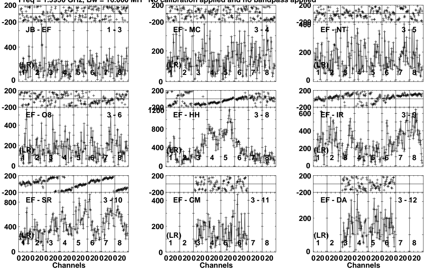
Lower frame: Micro Ampl Jy Top frame: Phas deg Vector averaged cross-power spectrum Several baselines displayed Timerange: 00/10:33:00 to 00/10:34:29
