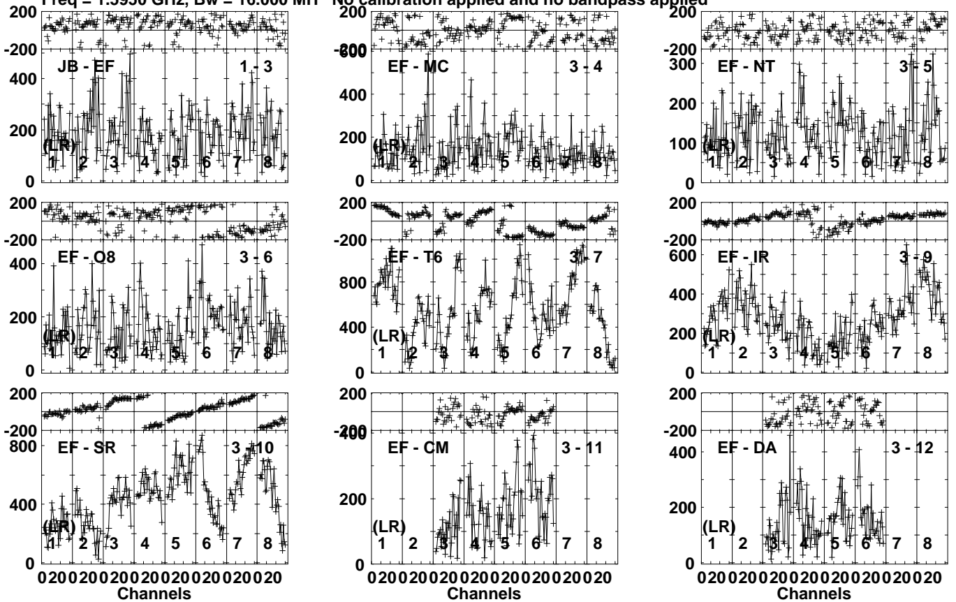
Lower frame: Micro Ampl Jy Top frame: Phas deg Vector averaged cross-power spectrum Several baselines displayed Timerange: 00/08:05:30 to 00/08:07:30
