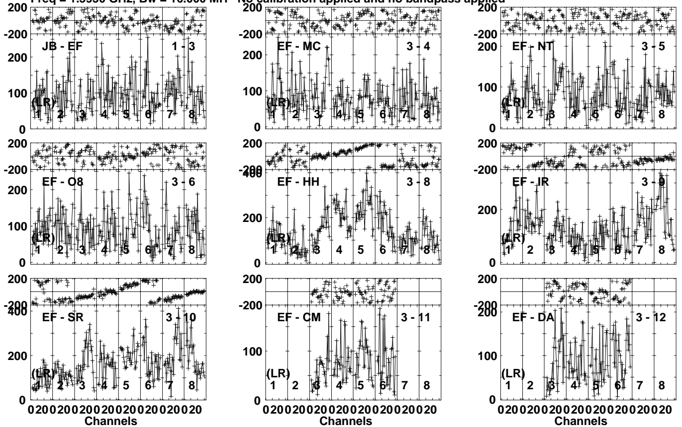
Lower frame: Micro Ampl Jy Top frame: Phas deg Vector averaged cross-power spectrum Several baselines displayed Timerange: 00/10:44:30 to 00/10:47:59
