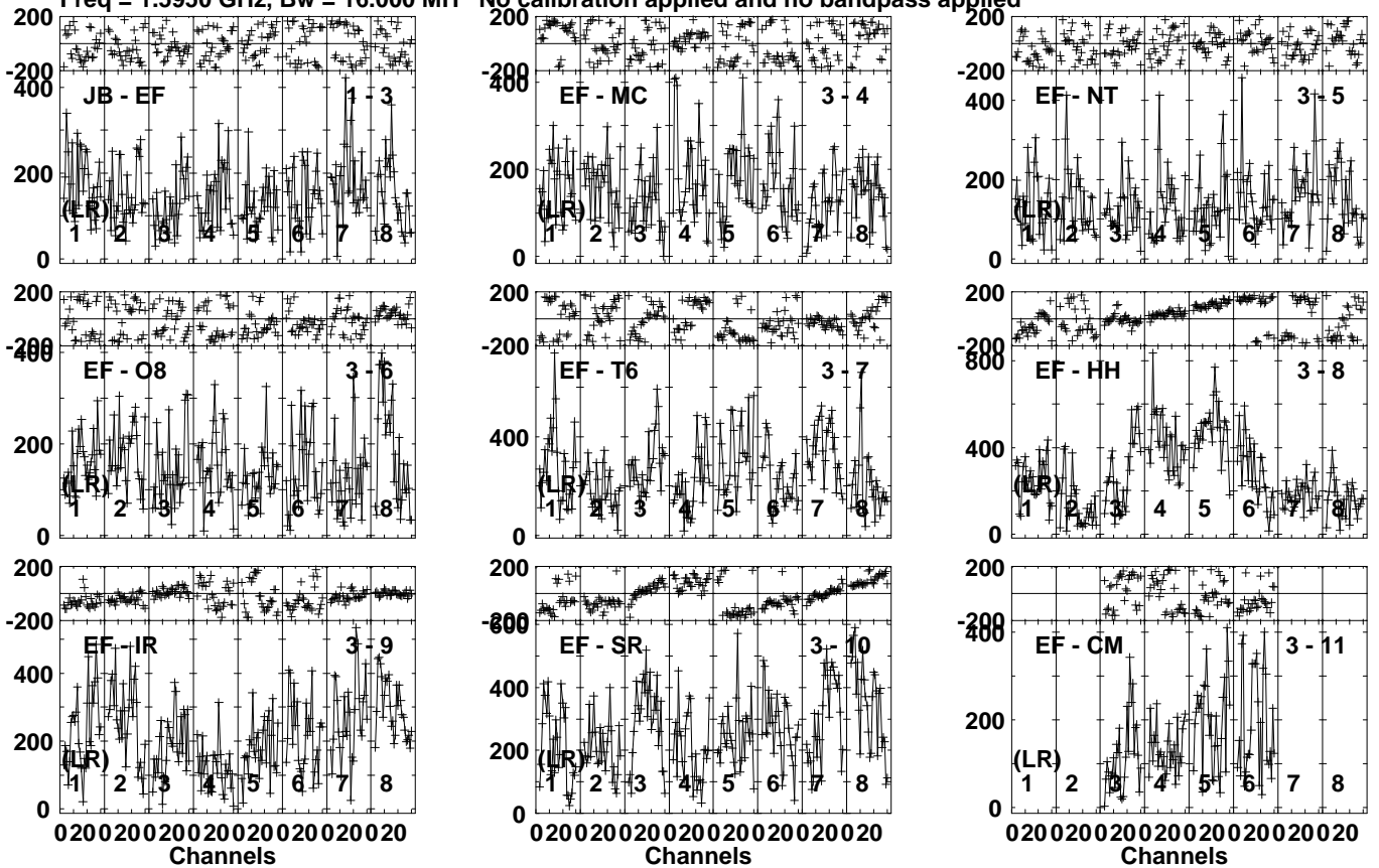
Lower frame: Micro Ampl Jy Top frame: Phas deg Vector averaged cross-power spectrum Several baselines displayed Timerange: 00/06:51:31 to 00/06:52:29
