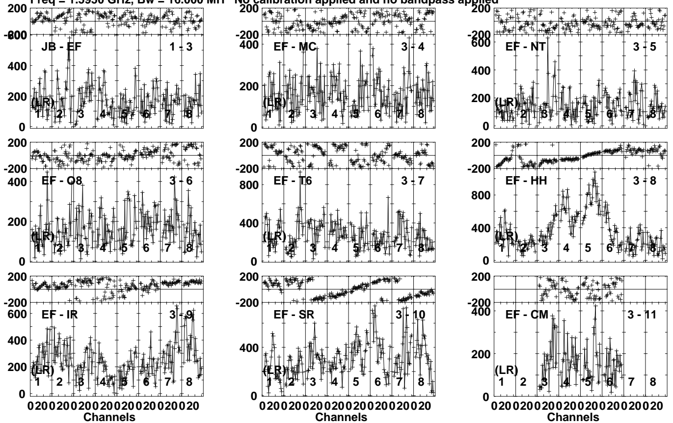
Lower frame: Micro Ampl Jy Top frame: Phas deg Vector averaged cross-power spectrum Several baselines displayed Timerange: 00/07:26:01 to 00/07:27:30
