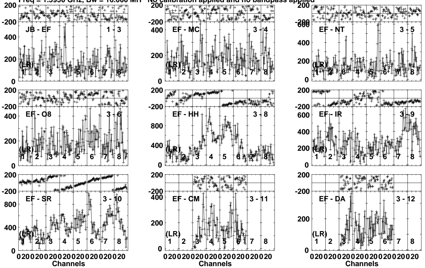
Lower frame: Micro Ampl Jy Top frame: Phas deg Vector averaged cross-power spectrum Several baselines displayed Timerange: 00/10:48:30 to 00/10:49:30
