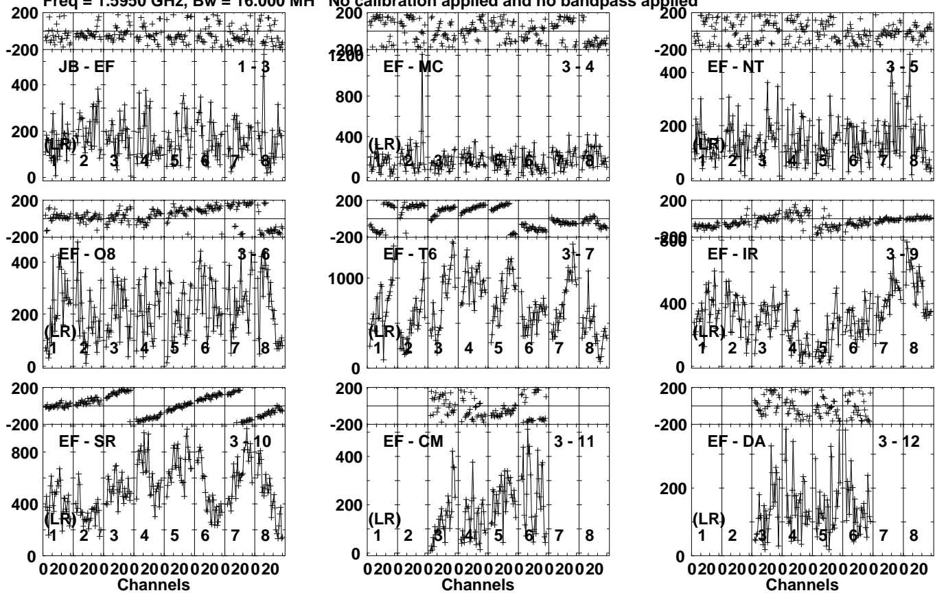
Lower frame: Micro Ampl Jy Top frame: Phas deg Vector averaged cross-power spectrum Several baselines displayed Timerange: 00/09:56:31 to 00/09:57:29
