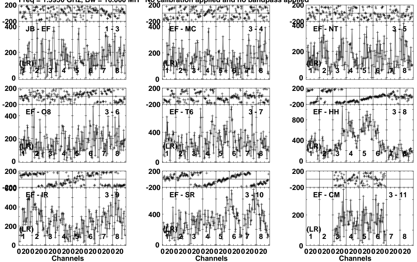
Lower frame: Micro Ampl Jy Top frame: Phas deg Vector averaged cross-power spectrum Several baselines displayed Timerange: 00/07:21:31 to 00/07:22:29
