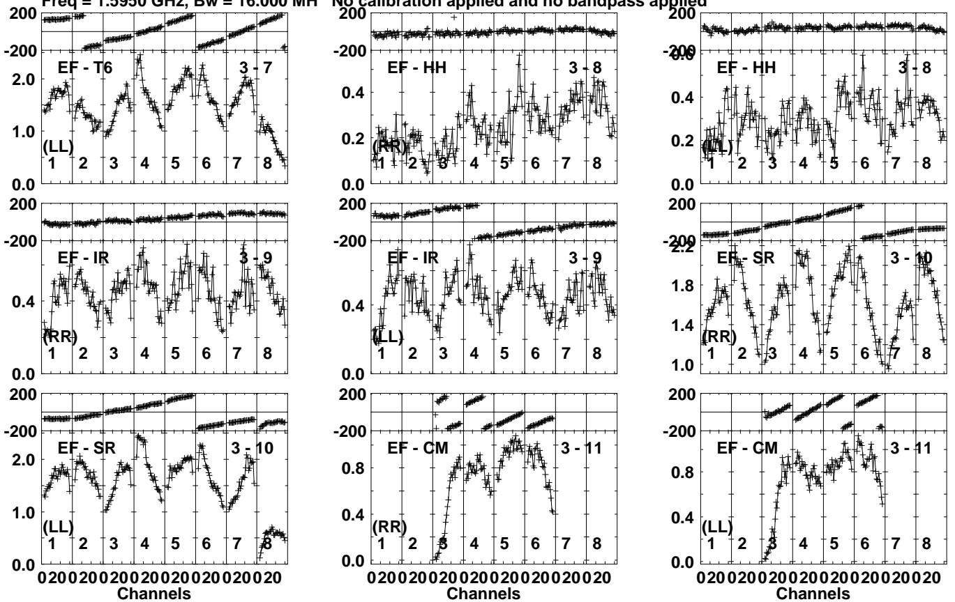
Lower frame: Milli Ampl Jy Top frame: Phas deg Vector averaged cross-power spectrum Several baselines displayed Timerange: 00/07:07:30 to 00/07:11:00
