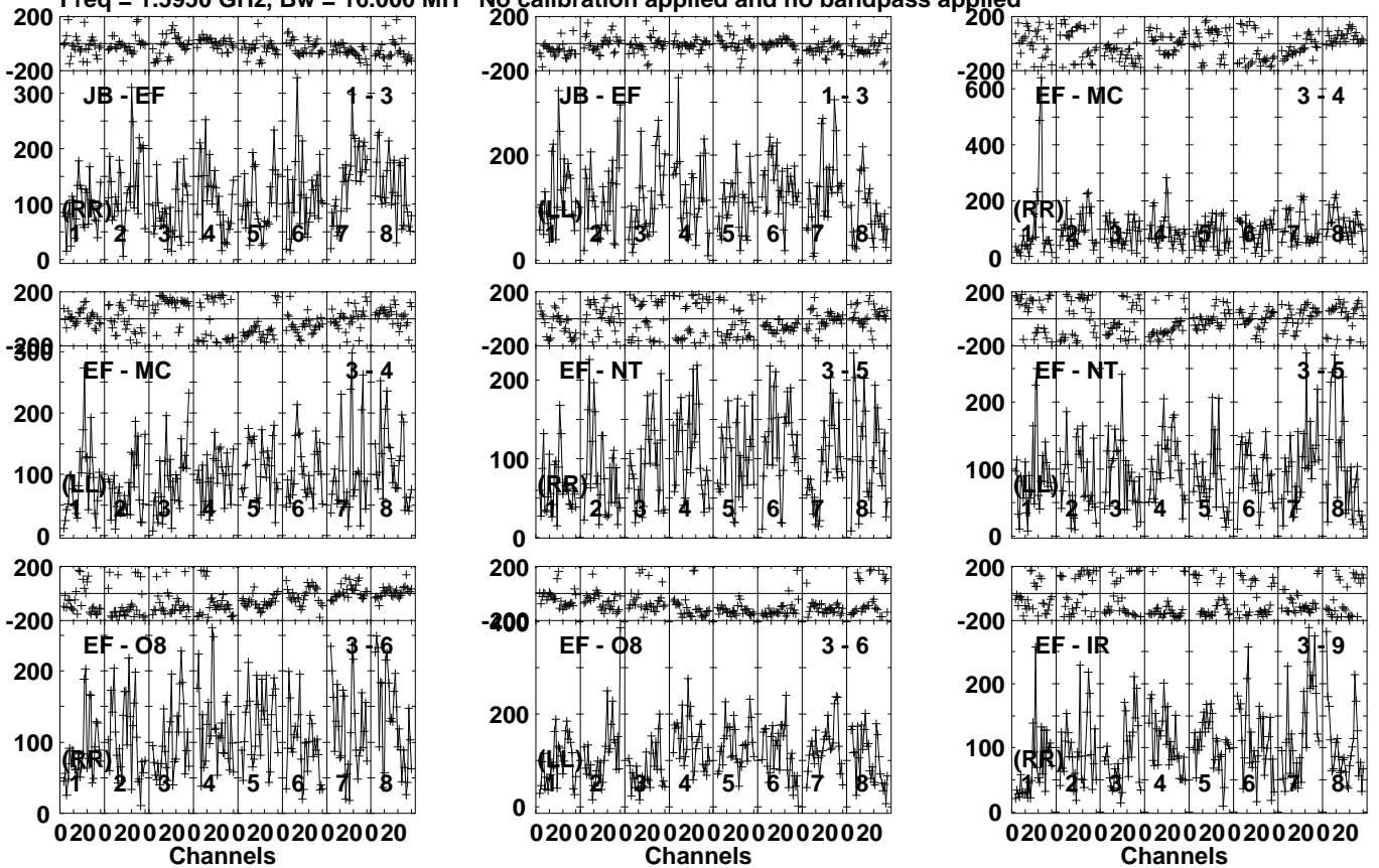
Lower frame: Micro Ampl Jy Top frame: Phas deg Vector averaged cross-power spectrum Several baselines displayed Timerange: 00/12:21:30 to 00/12:24:59
