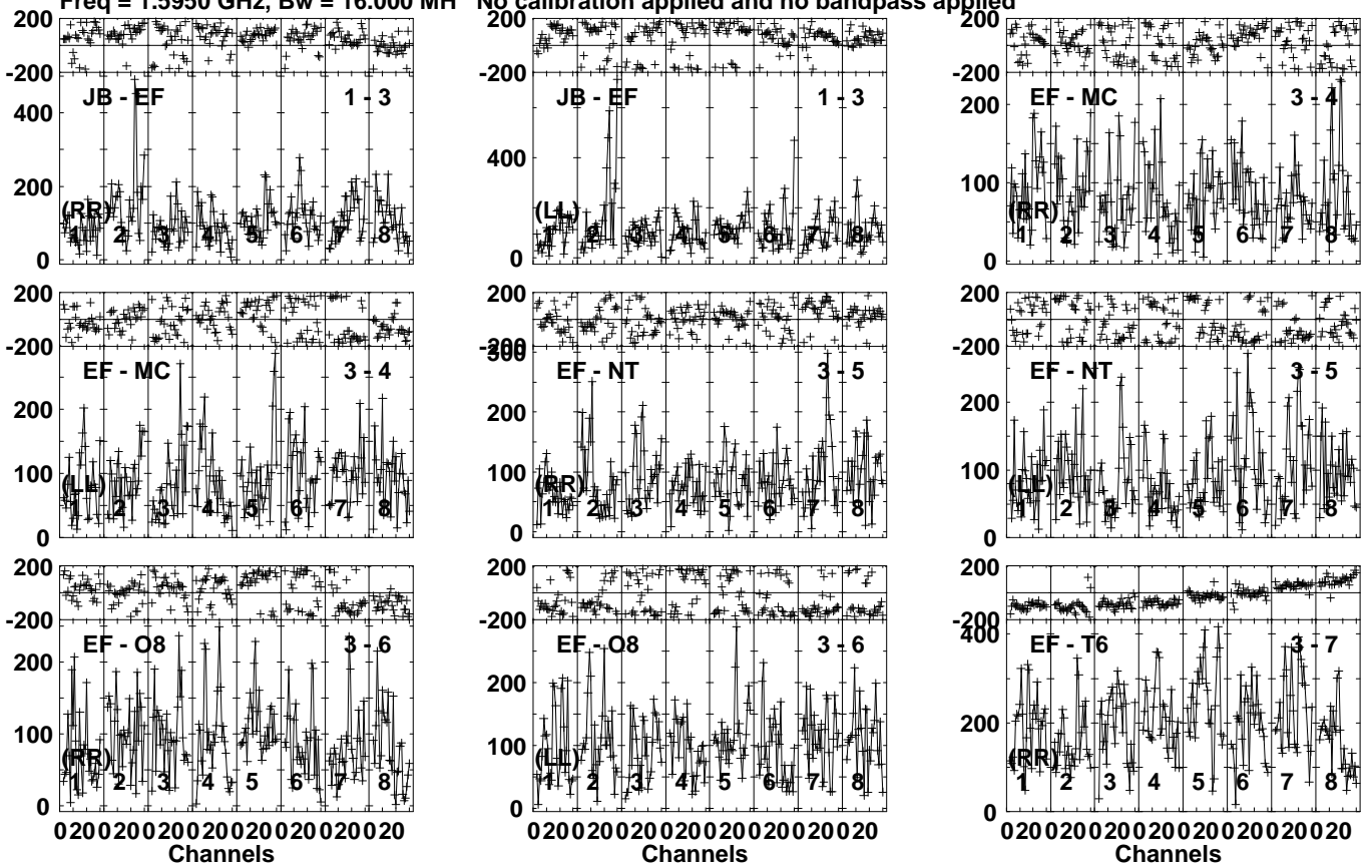
Lower frame: Micro Ampl Jy Top frame: Phas deg Vector averaged cross-power spectrum Several baselines displayed Timerange: 00/10/02:30 to 00/10/06:00
