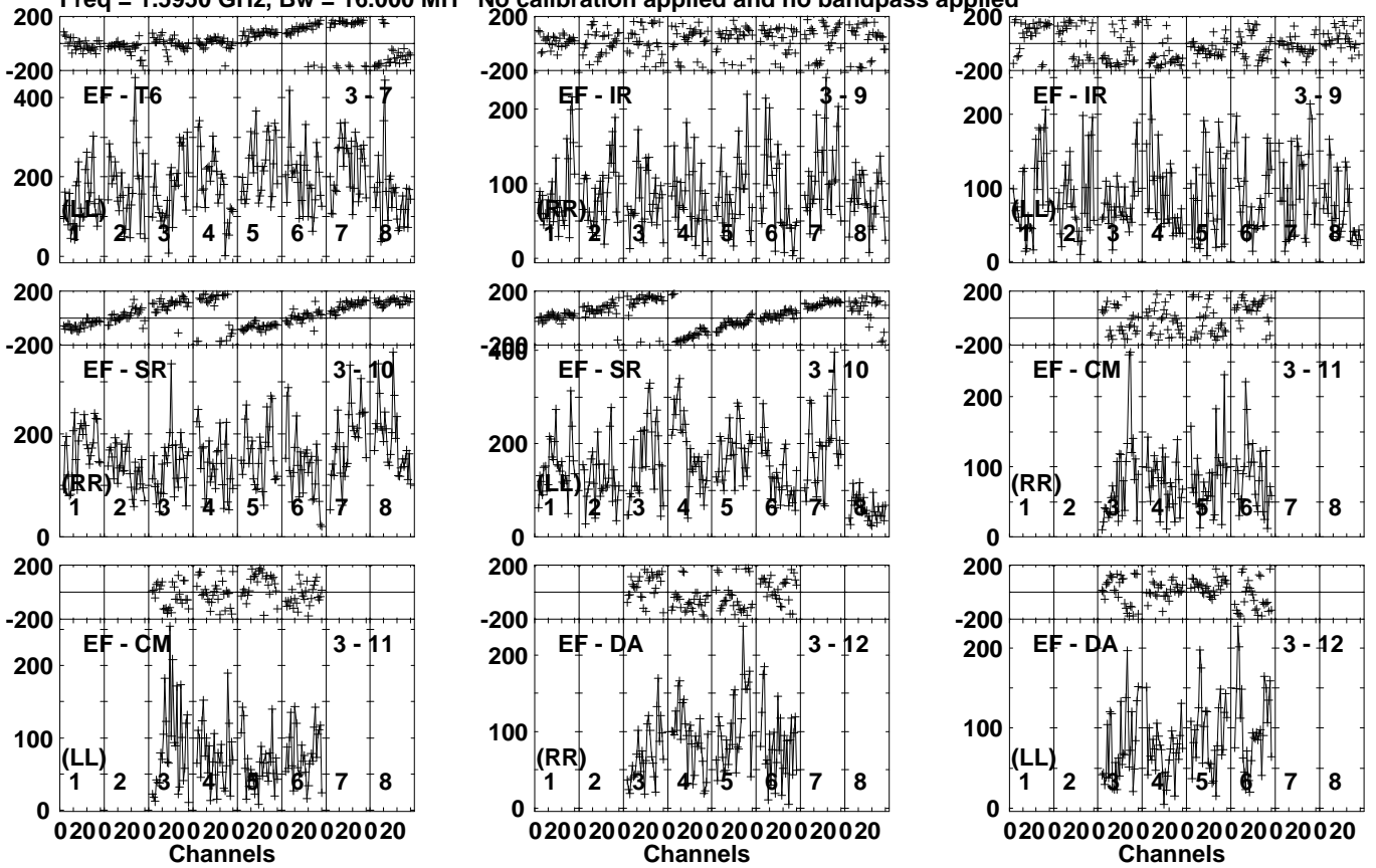
Lower frame: Micro Ampl Jy Top frame: Phas deg Vector averaged cross-power spectrum Several baselines displayed Timerange: 00/09:47:30 to 00/09:51:00
