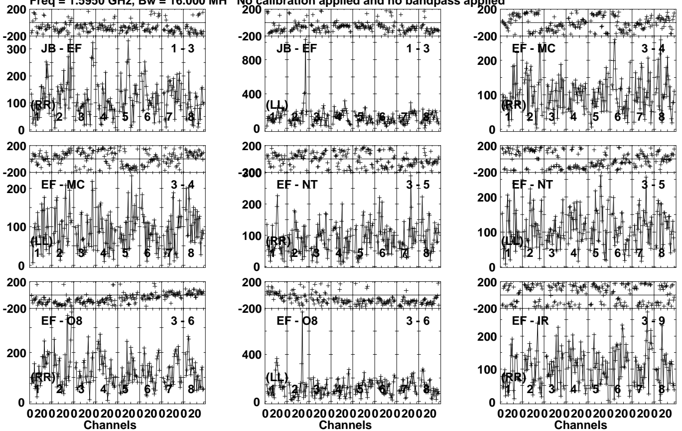
Lower frame: Micro Ampl Jy Top frame: Phas deg Vector averaged cross-power spectrum Several baselines displayed Timerange: 00/12:31:30 to 00/12:34:59
