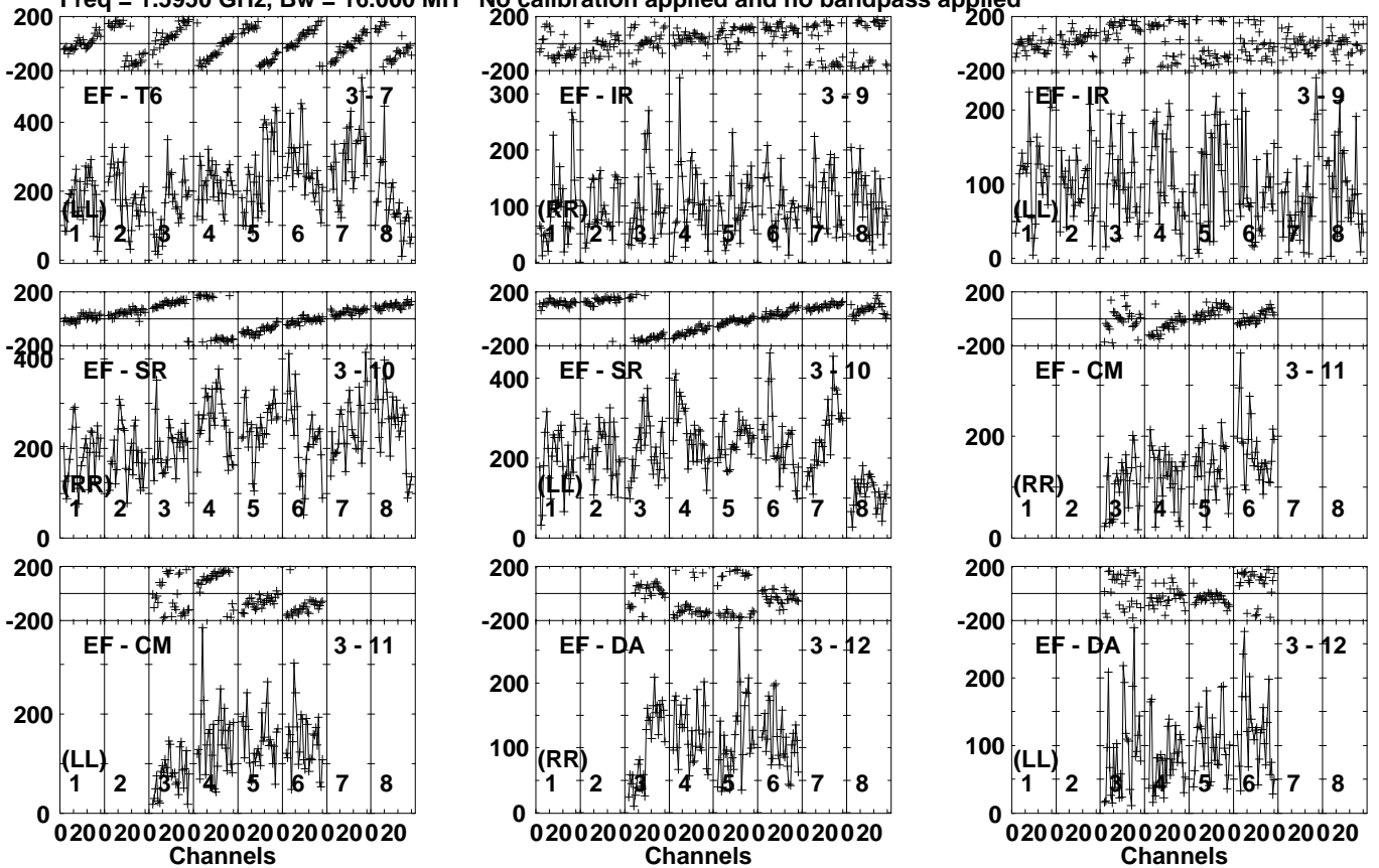
Lower frame: Micro Ampl Jy Top frame: Phas deg Vector averaged cross-power spectrum Several baselines displayed Timerange: 00/06:17:00 to 00/06:20:29
