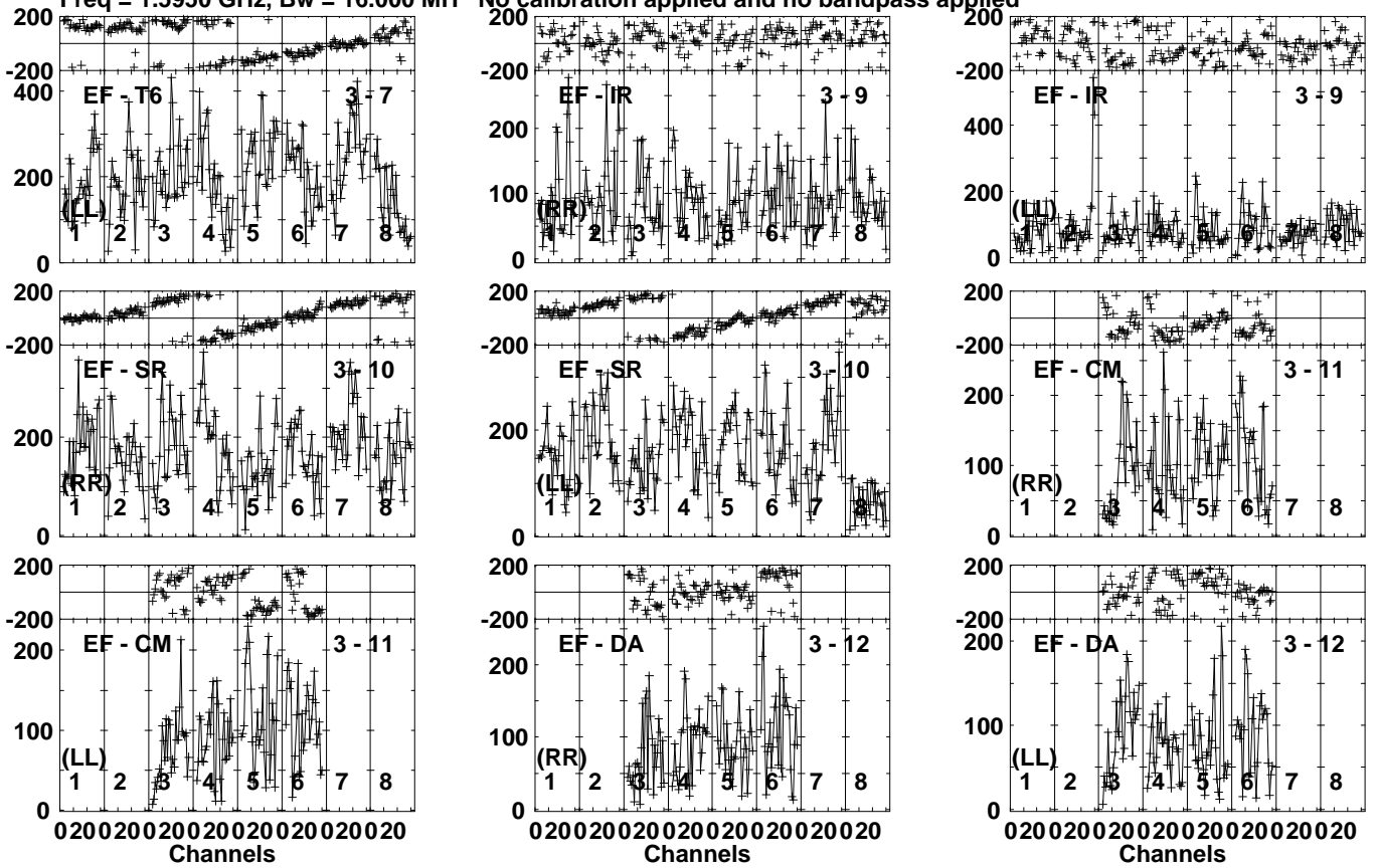
Lower frame: Micro Ampl Jy Top frame: Phas deg Vector averaged cross-power spectrum Several baselines displayed Timerange: 00/08:37:31 to 00/08:41:00
