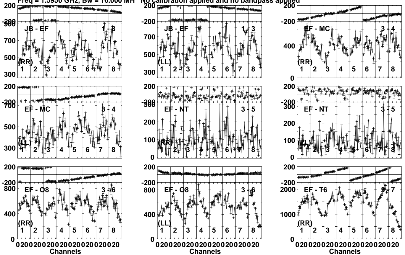
Lower frame: Micro Ampl Jy Top frame: Phas deg Vector averaged cross-power spectrum Several baselines displayed Timerange: 00/06:37:31 to 00/06:41:00
