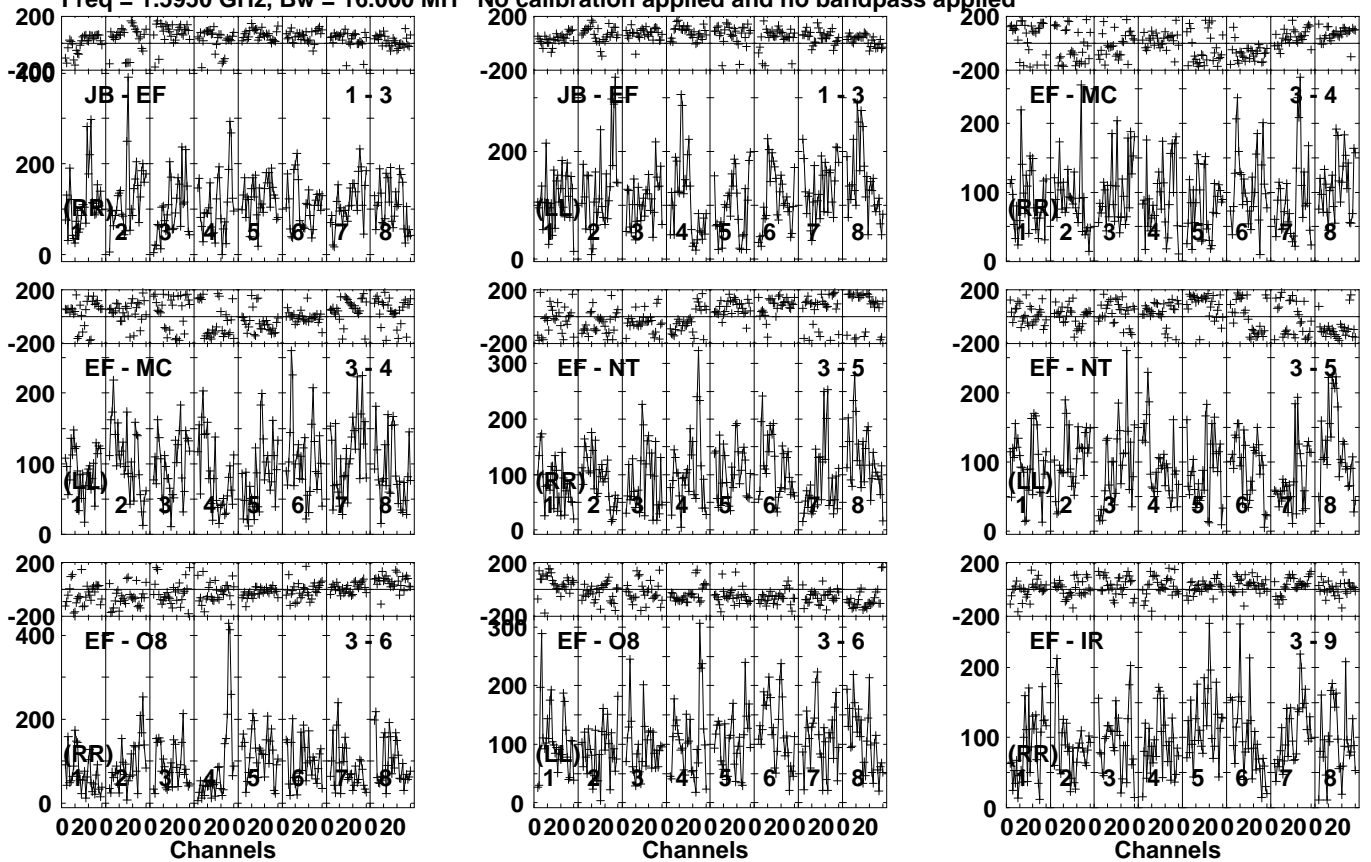
Lower frame: Micro Ampl Jy Top frame: Phas deg Vector averaged cross-power spectrum Several baselines displayed Timerange: 00:12:51:31 to 00:12:55:00
