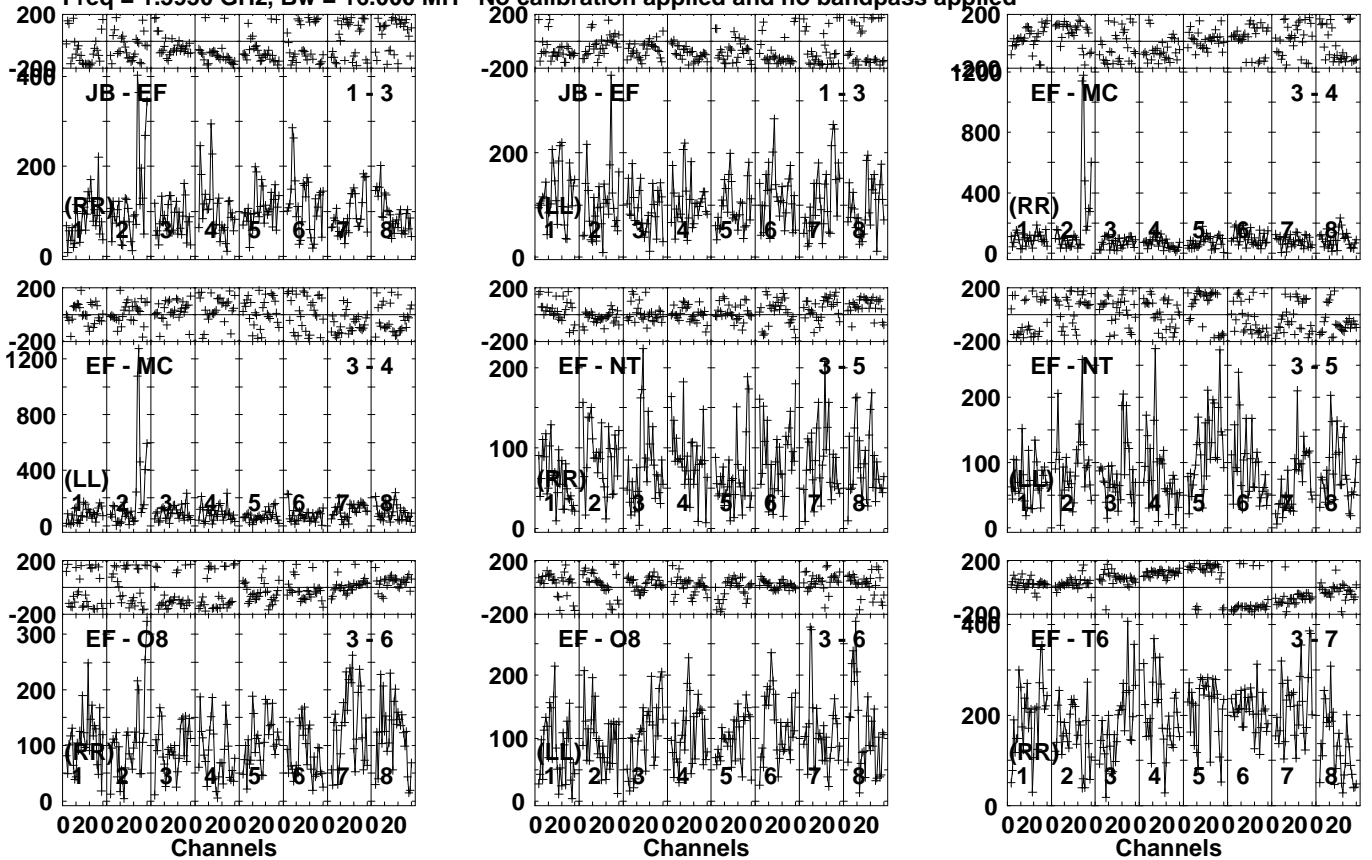
Lower frame: Micro Ampl Jy Top frame: Phas deg Vector averaged cross-power spectrum Several baselines displayed Timerange: 00/08:32:30 to 00/08:36:00
