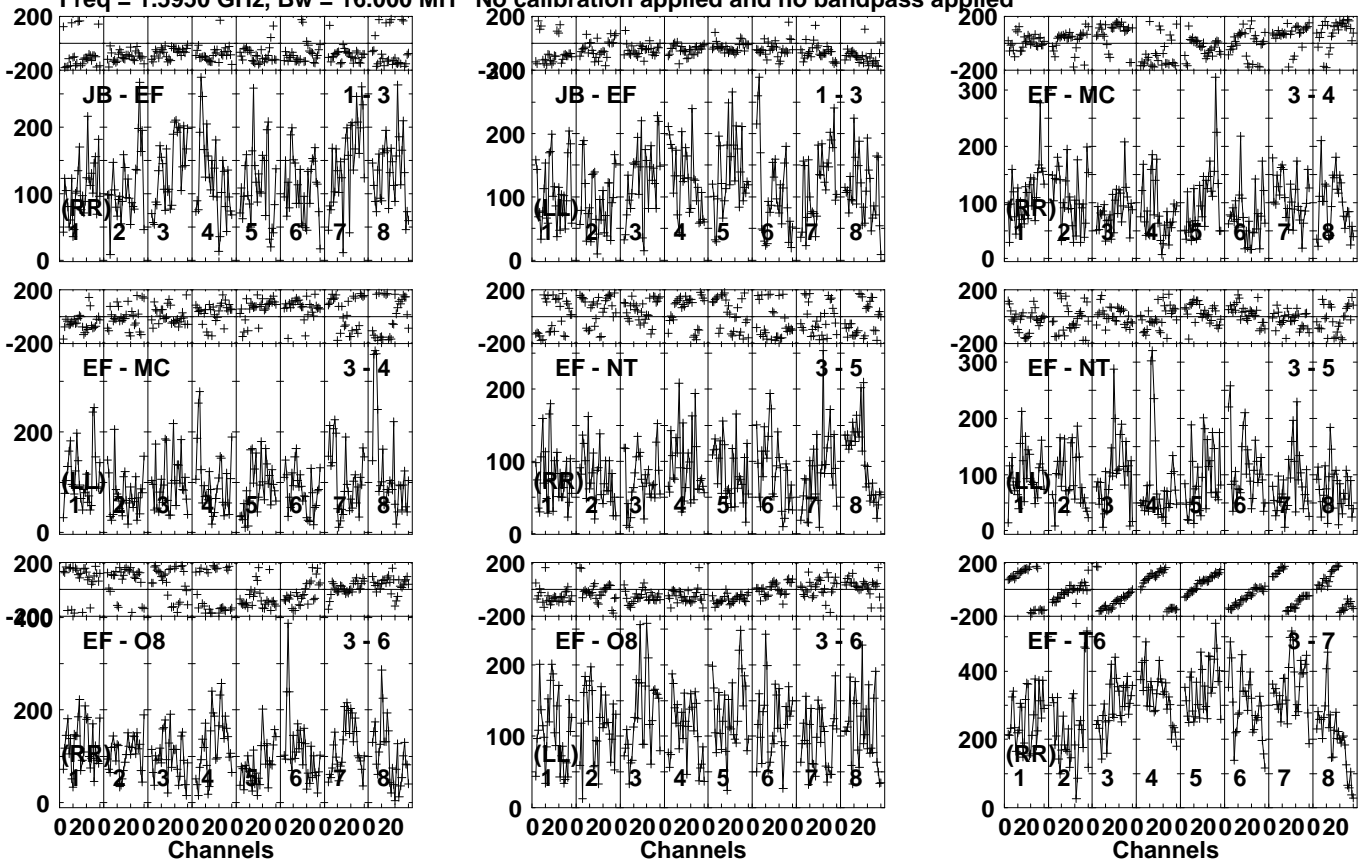
Lower frame: Micro Ampl Jy Top frame: Phas deg Vector averaged cross-power spectrum Several baselines displayed Timerange: 00/05:22:00 to 00/05:25:30
