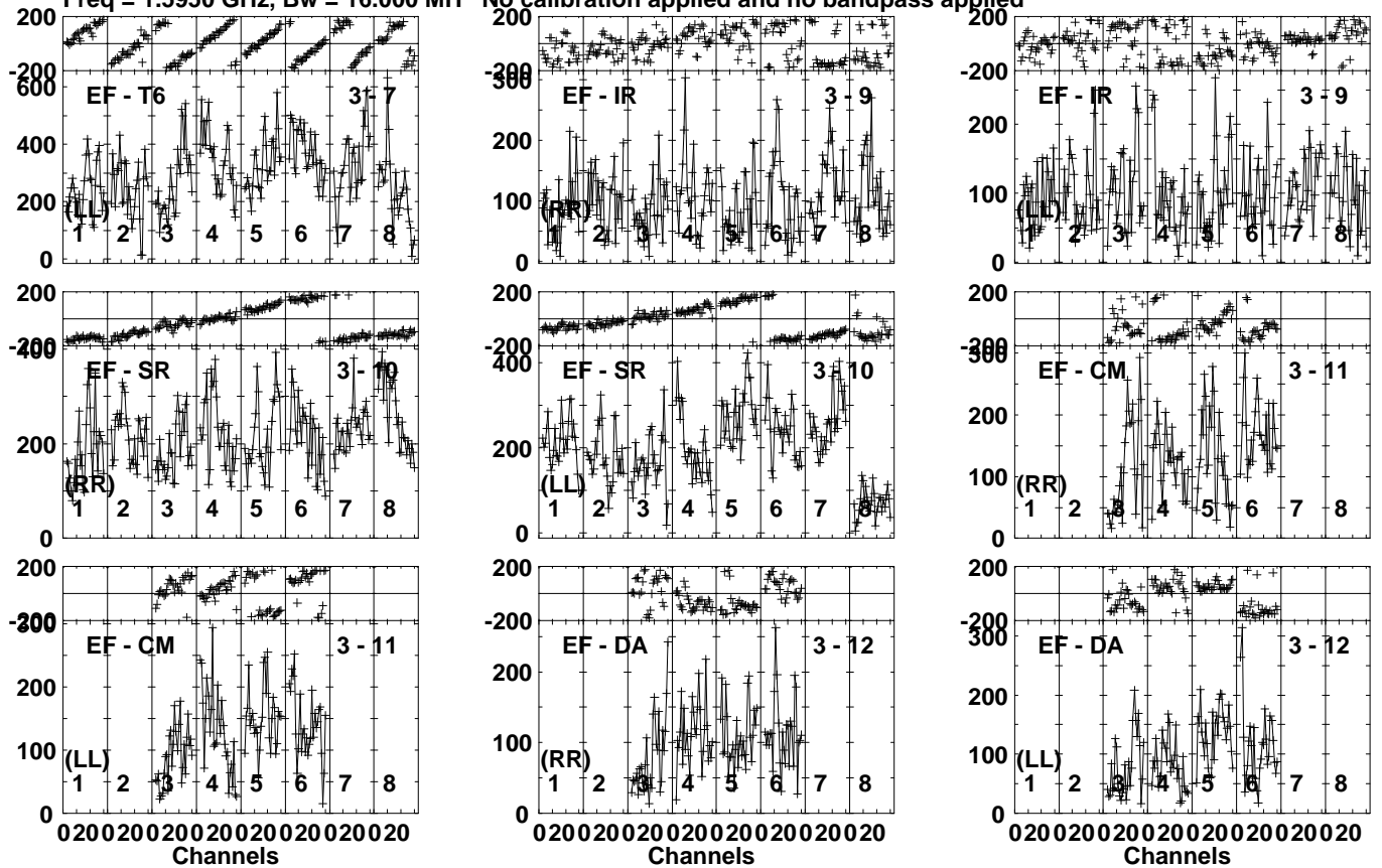
Lower frame: Micro Ampl Jy Top frame: Phas deg Vector averaged cross-power spectrum Several baselines displayed Timerange: 00/05:17:00 to 00/05:20:30
