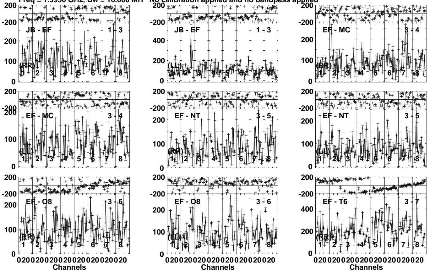
Lower frame: Micro Ampl Jy Top frame: Phas deg Vector averaged cross-power spectrum Several baselines displayed Timerange: 00/08:17:30 to 00/08:21:00
