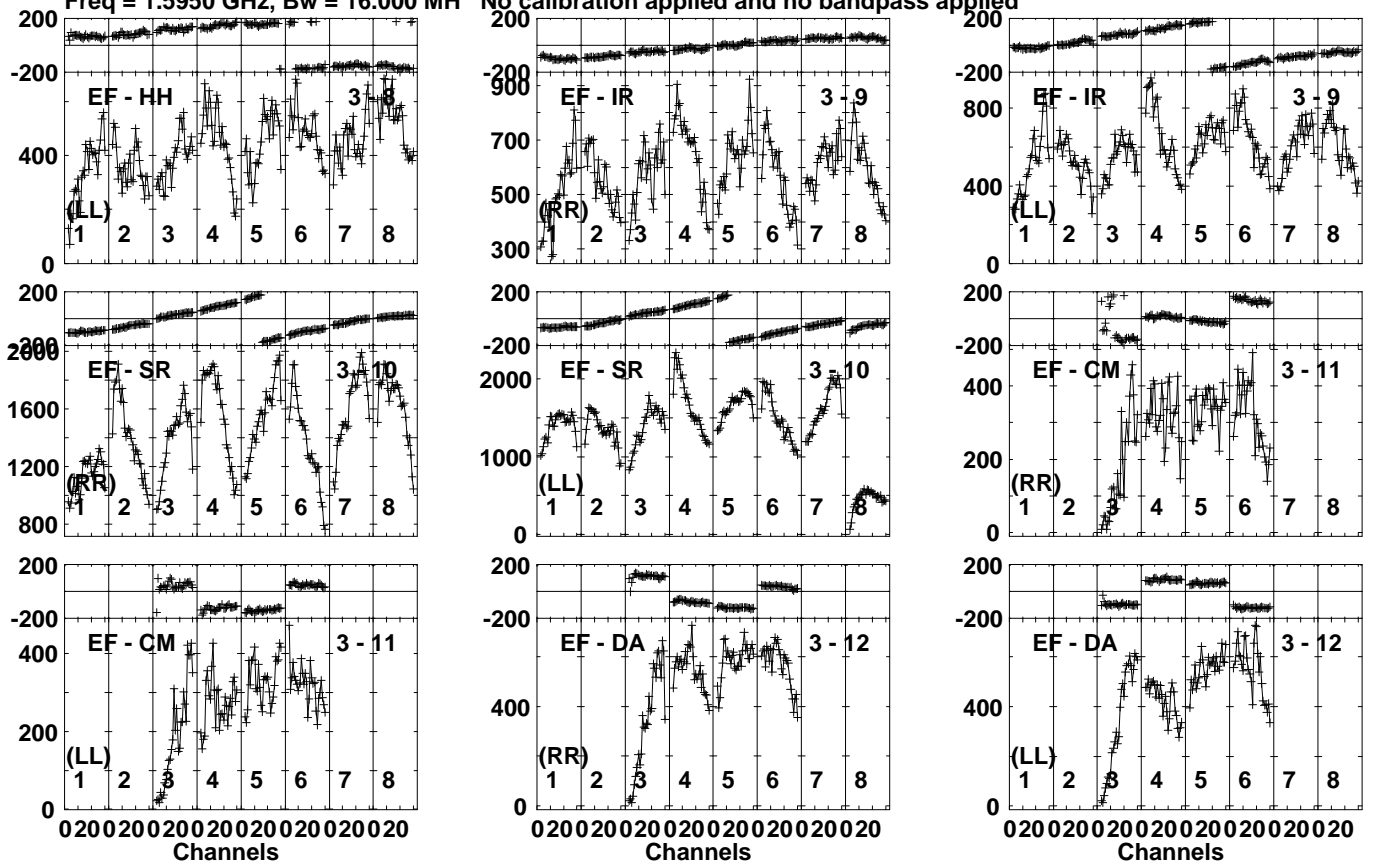
Lower frame: Micro Ampl Jy Top frame: Phas deg Vector averaged cross-power spectrum Several baselines displayed Timerange: 00/11:44:31 to 00/11:48:00
