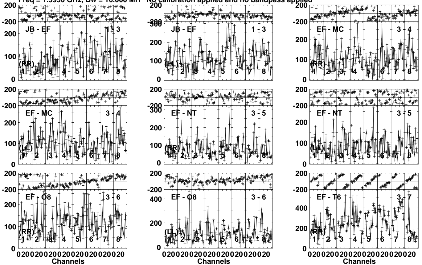
Lower frame: Micro Ampl Jy Top frame: Phas deg Vector averaged cross-power spectrum Several baselines displayed Timerange: 00/05:07:00 to 00/05:10:29
