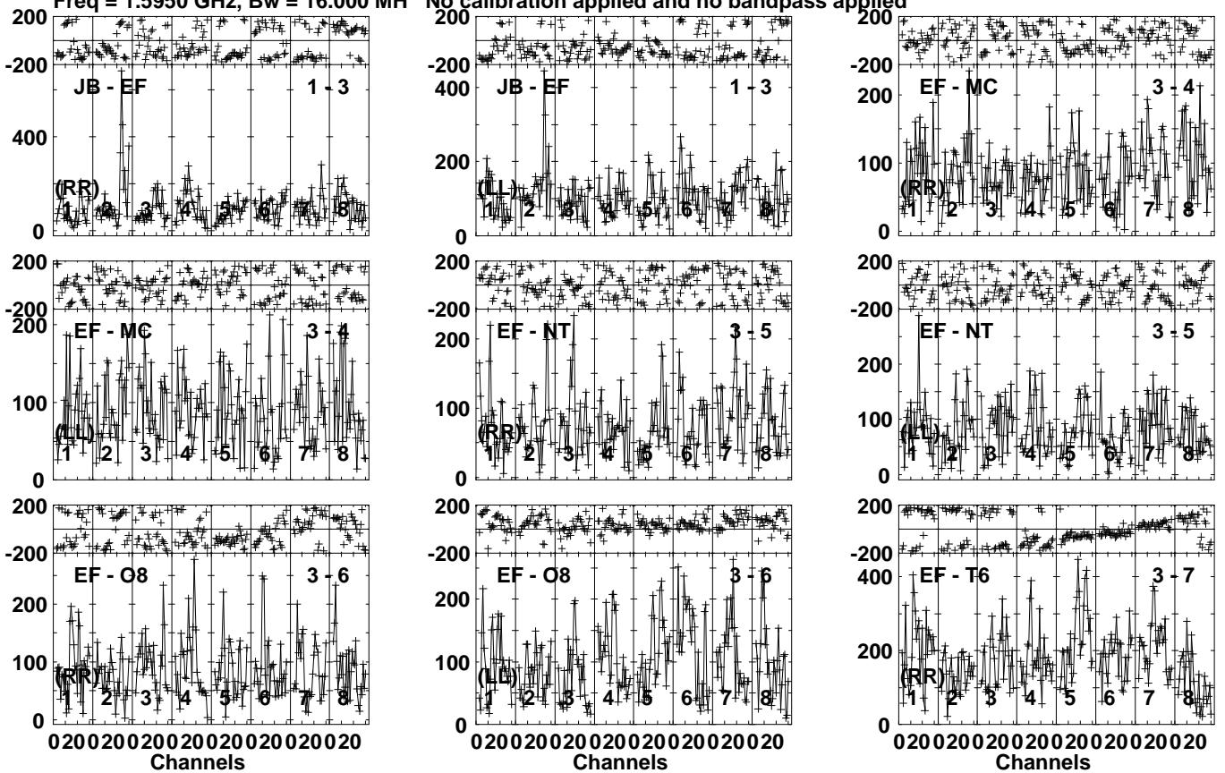
Lower frame: Micro Ampl Jy Top frame: Phas deg Vector averaged cross-power spectrum Several baselines displayed Timerange: 00/08:12:31 to 00/08:16:00
