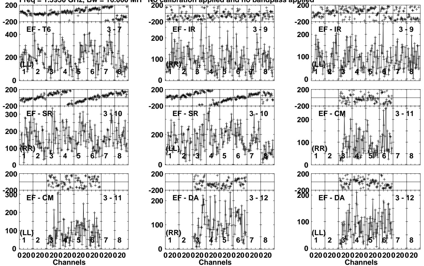
Lower frame: Micro Ampl Jy Top frame: Phas deg Vector averaged cross-power spectrum Several baselines displayed Timerange: 00/09:42:31 to 00/09:46:00
