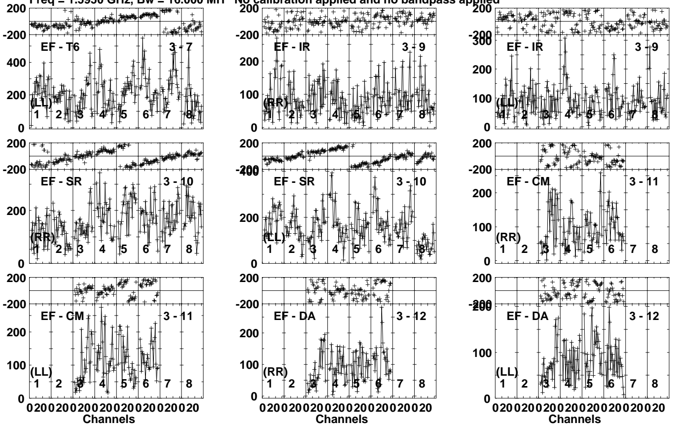
Lower frame: Micro Ampl Jy Top frame: Phas deg Vector averaged cross-power spectrum Several baselines displayed Timerange: 00/08:07:31 to 00/08:11:00
