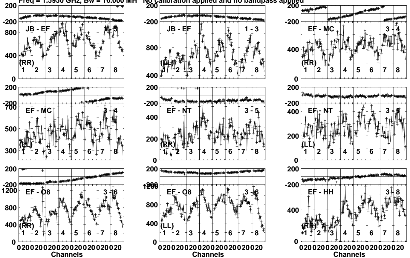
Lower frame: Micro Ampl Jy Top frame: Phas deg Vector averaged cross-power spectrum Several baselines displayed Timerange: 00/10:29:30 to 00/10:32:59
