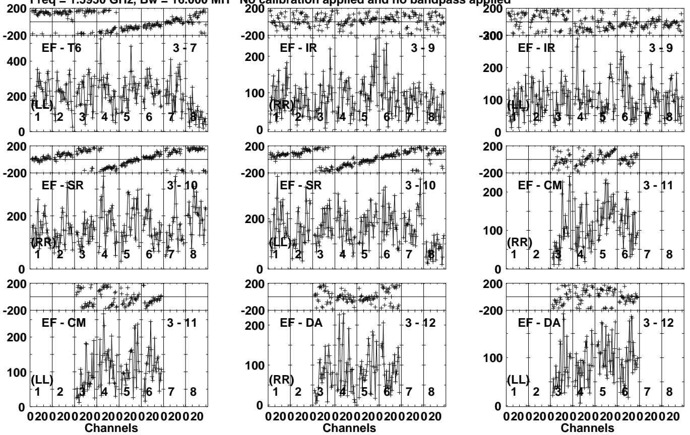
Lower frame: Micro Ampl Jy Top frame: Phas deg Vector averaged cross-power spectrum Several baselines displayed Timerange: 00/08:42:30 to 00/08:45:59
