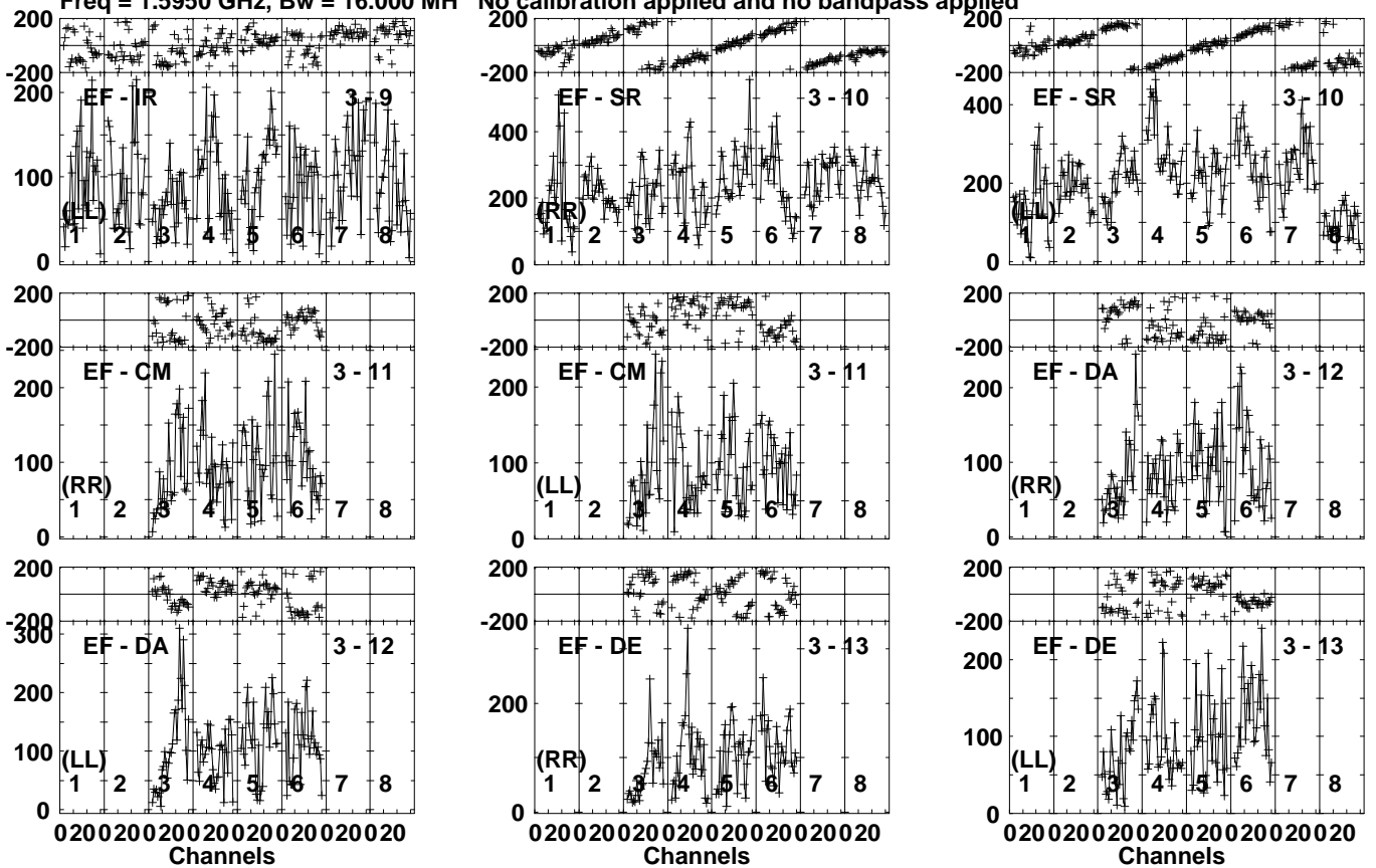
Lower frame: Micro Ampl Jy Top frame: Phas deg Vector averaged cross-power spectrum Several baselines displayed Timerange: 00/12:26:30 to 00/12:29:59
