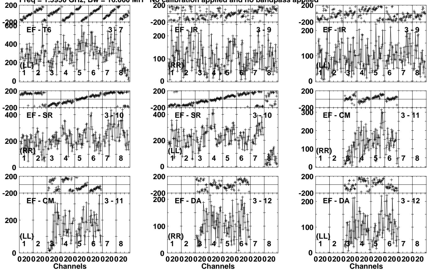
Lower frame: Micro Ampl Jy Top frame: Phas deg Vector averaged cross-power spectrum Several baselines displayed Timerange: 00/05:37:00 to 00/05:40:29
