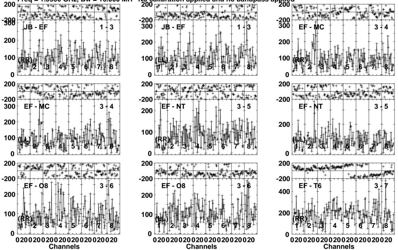
Lower frame: Micro Ampl Jy Top frame: Phas deg Vector averaged cross-power spectrum Several baselines displayed Timerange: 00/09:17:30 to 00/09:21:00
