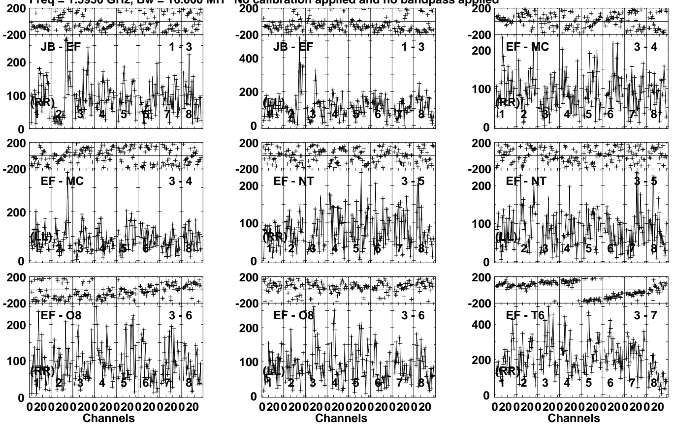
Lower frame: Micro Ampl Jy Top frame: Phas deg Vector averaged cross-power spectrum Several baselines displayed Timerange: 00/08:22:30 to 00/08:25:59
