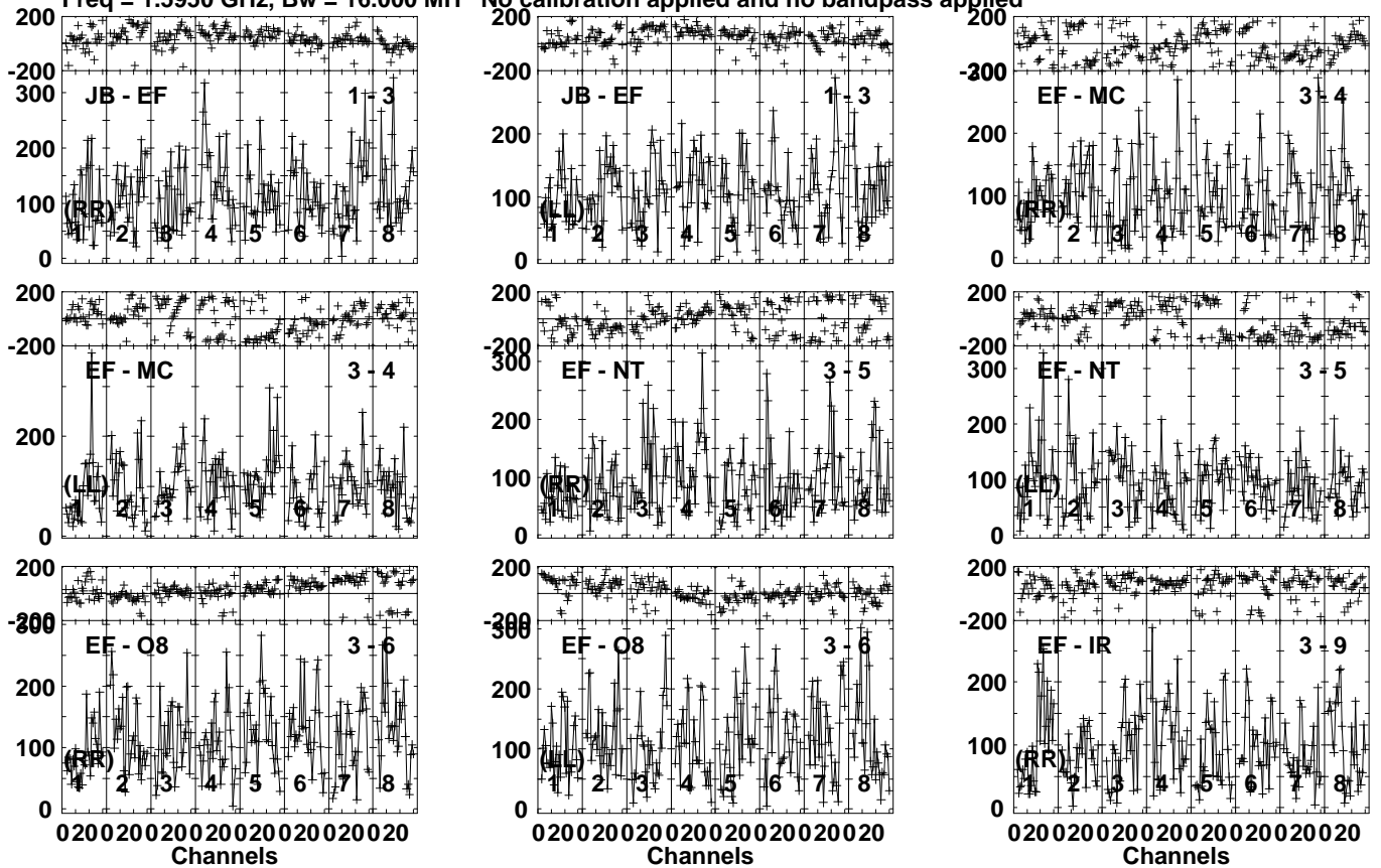
Lower frame: Micro Ampl Jy Top frame: Phas deg Vector averaged cross-power spectrum Several baselines displayed Timerange: 00/12:01:30 to 00/12:05:00
