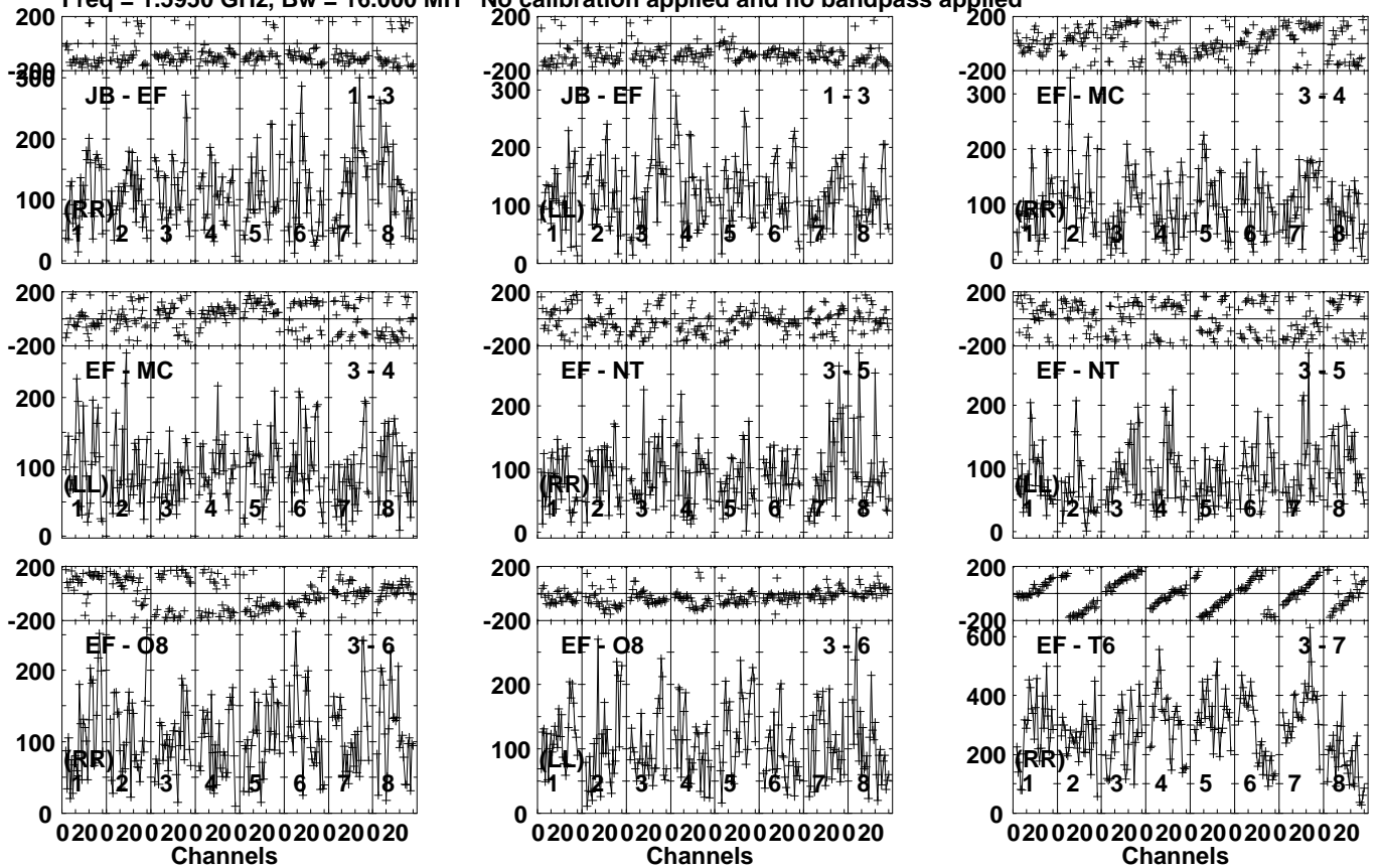
Lower frame: Micro Ampl Jy Top frame: Phas deg Vector averaged cross-power spectrum Several baselines displayed Timerange: 00/05:52:00 to 00/05:55:29
