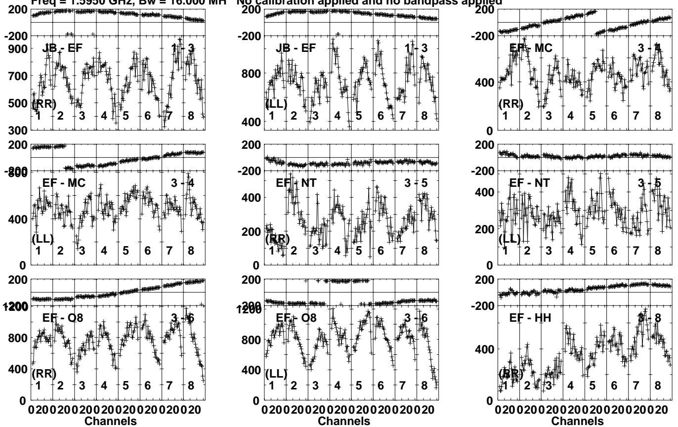
Lower frame: Micro Ampl Jy Top frame: Phas deg Vector averaged cross-power spectrum Several baselines displayed Timerange: 00/11:04:30 to 00/11:07:59
