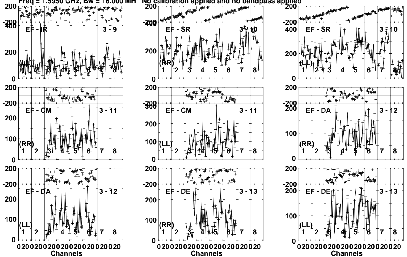
Lower frame: Micro Ampl Jy Top frame: Phas deg Vector averaged cross-power spectrum Several baselines displayed Timerange: 00/12:46:30 to 00/12:50:00
