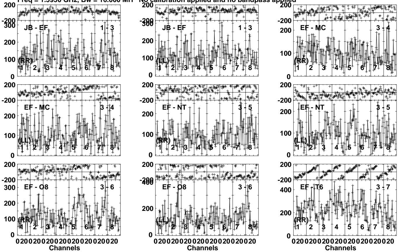
Lower frame: Micro Ampl Jy Top frame: Phas deg Vector averaged cross-power spectrum Several baselines displayed Timerange: 00/06:22:00 to 00/06:25:29
