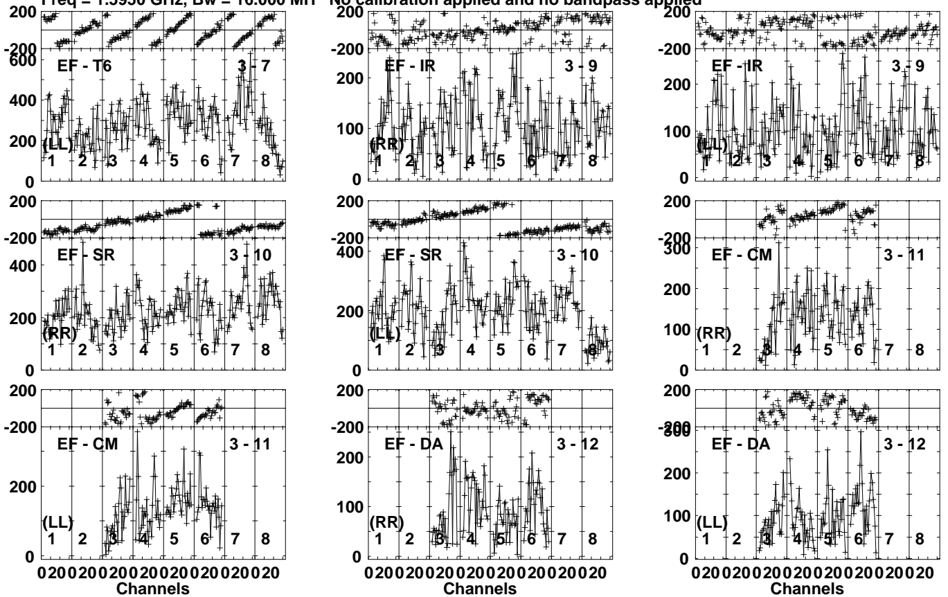
Lower frame: Micro Ampl Jy Top frame: Phas deg Vector averaged cross-power spectrum Several baselines displayed Timerange: 00/05:42:01 to 00/05:45:30
