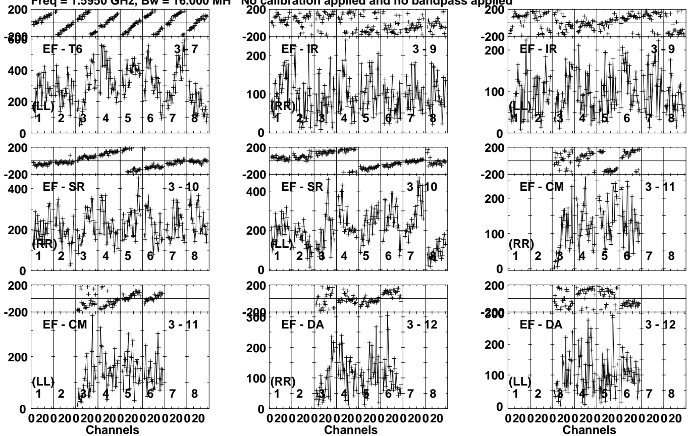
Lower frame: Micro Ampl Jy Top frame: Phas deg Vector averaged cross-power spectrum Several baselines displayed Timerange: 00/05:47:00 to 00/05:50:30
