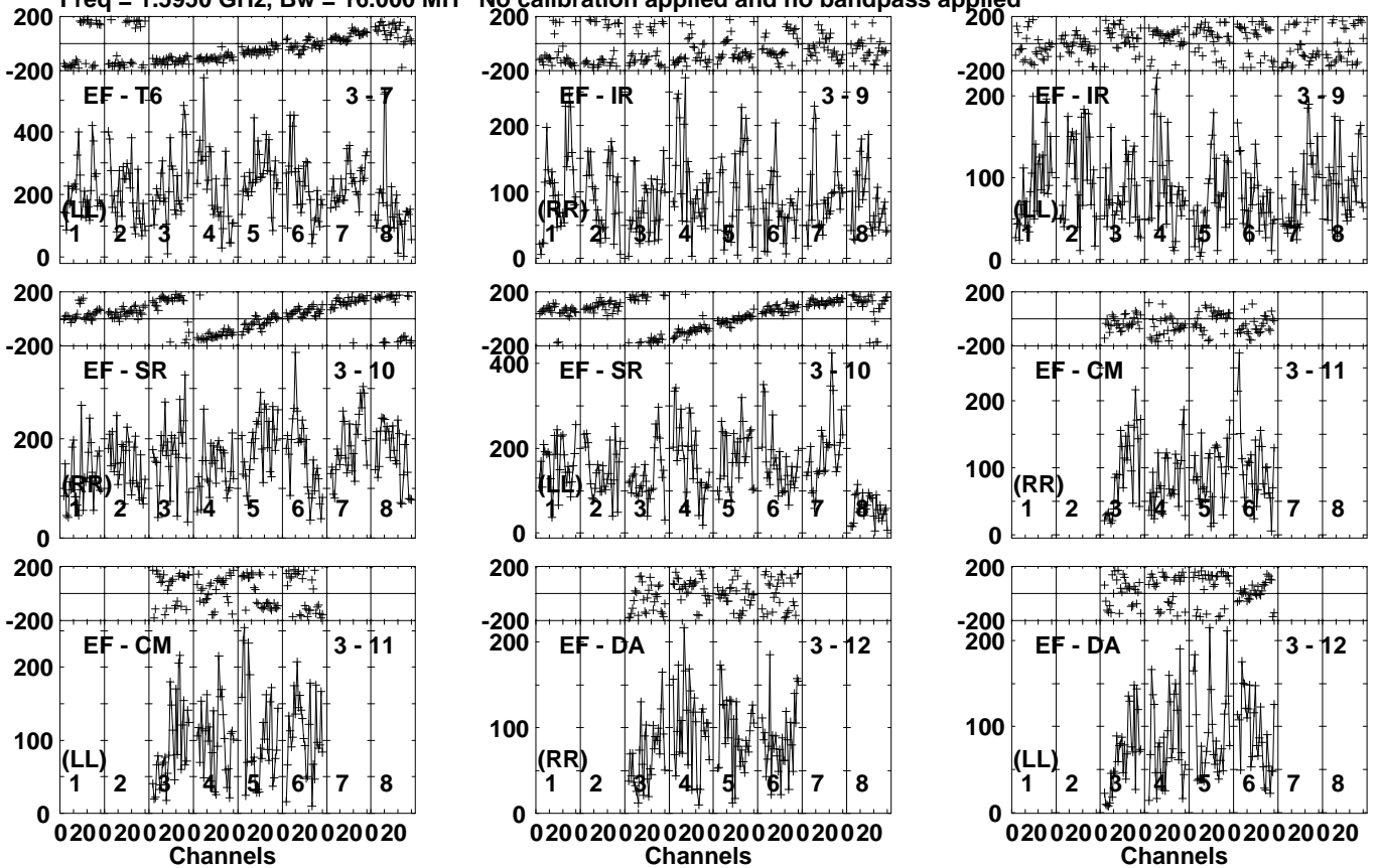
Lower frame: Micro Ampl Jy Top frame: Phas deg Vector averaged cross-power spectrum Several baselines displayed Timerange: 00/08:52:31 to 00/08:56:00
