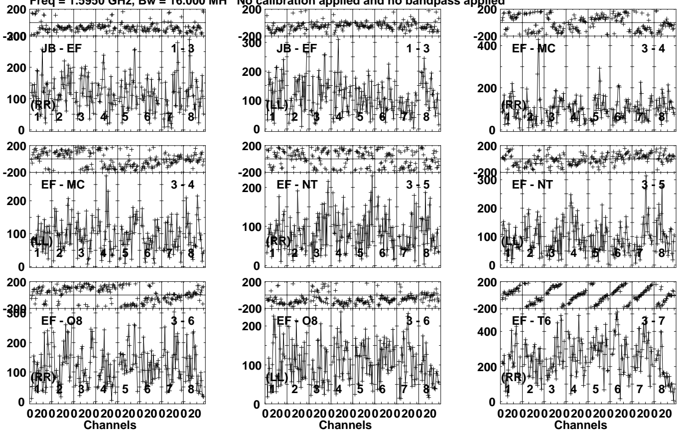
Lower frame: Micro Ampl Jy Top frame: Phas deg Vector averaged cross-power spectrum Several baselines displayed Timerange: 00/06:02:01 to 00/06:05:30
