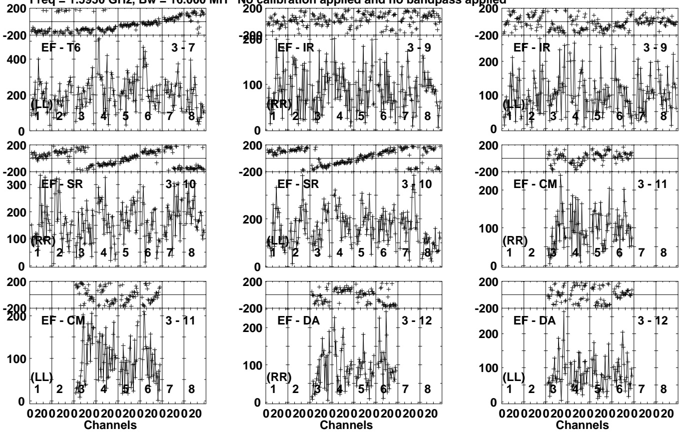
Lower frame: Micro Ampl Jy Top frame: Phas deg Vector averaged cross-power spectrum Several baselines displayed Timerange: 00/08:57:31 to 00/09:01:00
