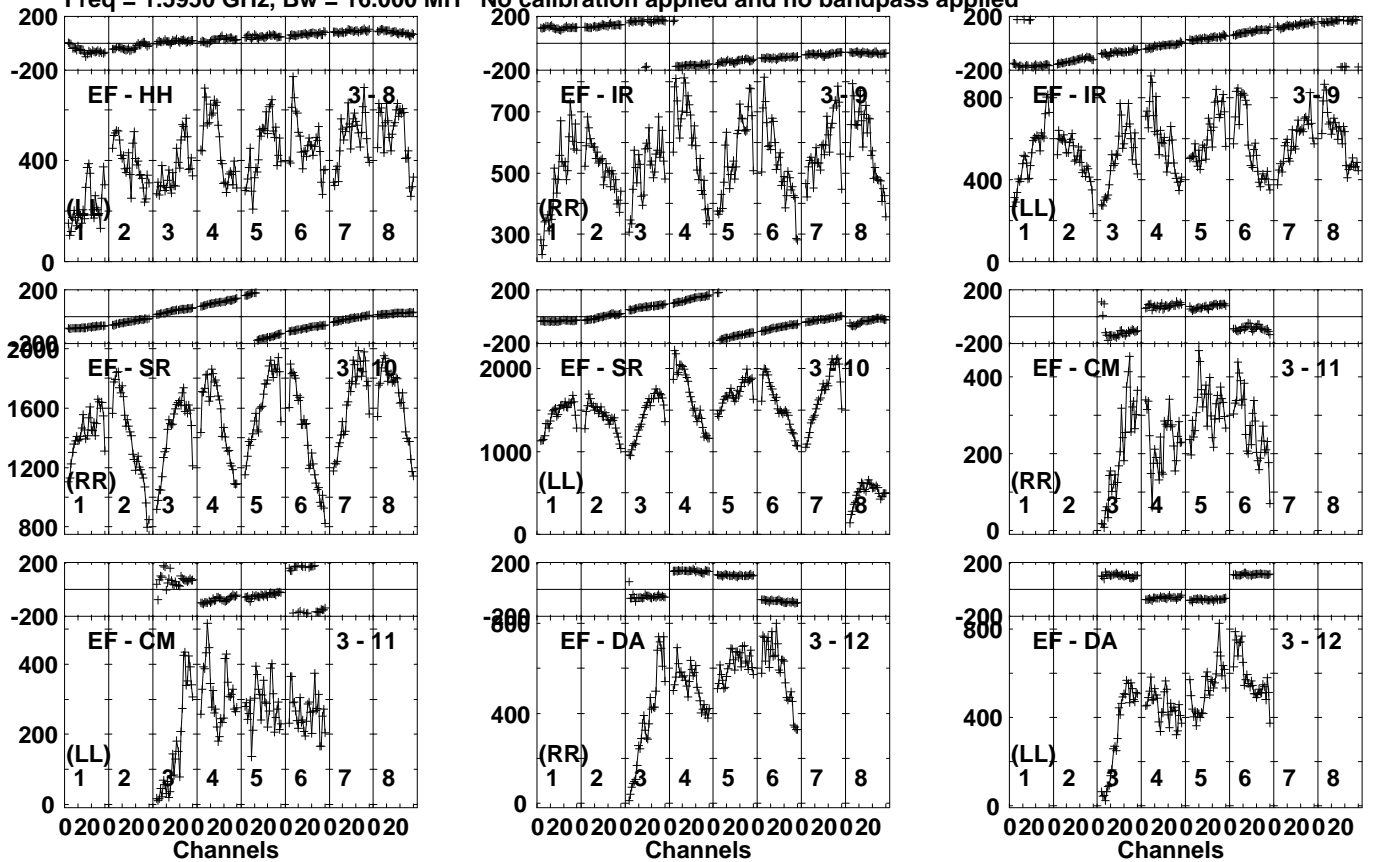
Lower frame: Micro Ampl Jy Top frame: Phas deg Vector averaged cross-power spectrum Several baselines displayed Timerange: 00/10:59:31 to 00/11:03:00
