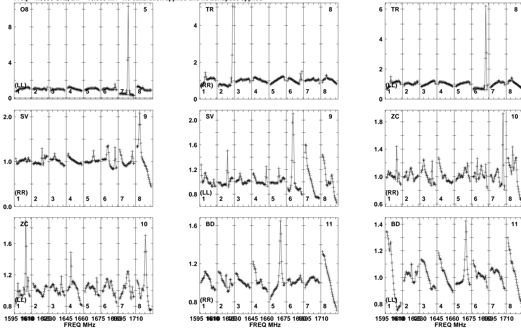
Lower frame: Real Jy Total-power spectrum Antenna: O8 (05) Timerange: 00/23:29:31 to 00/23:39:29
