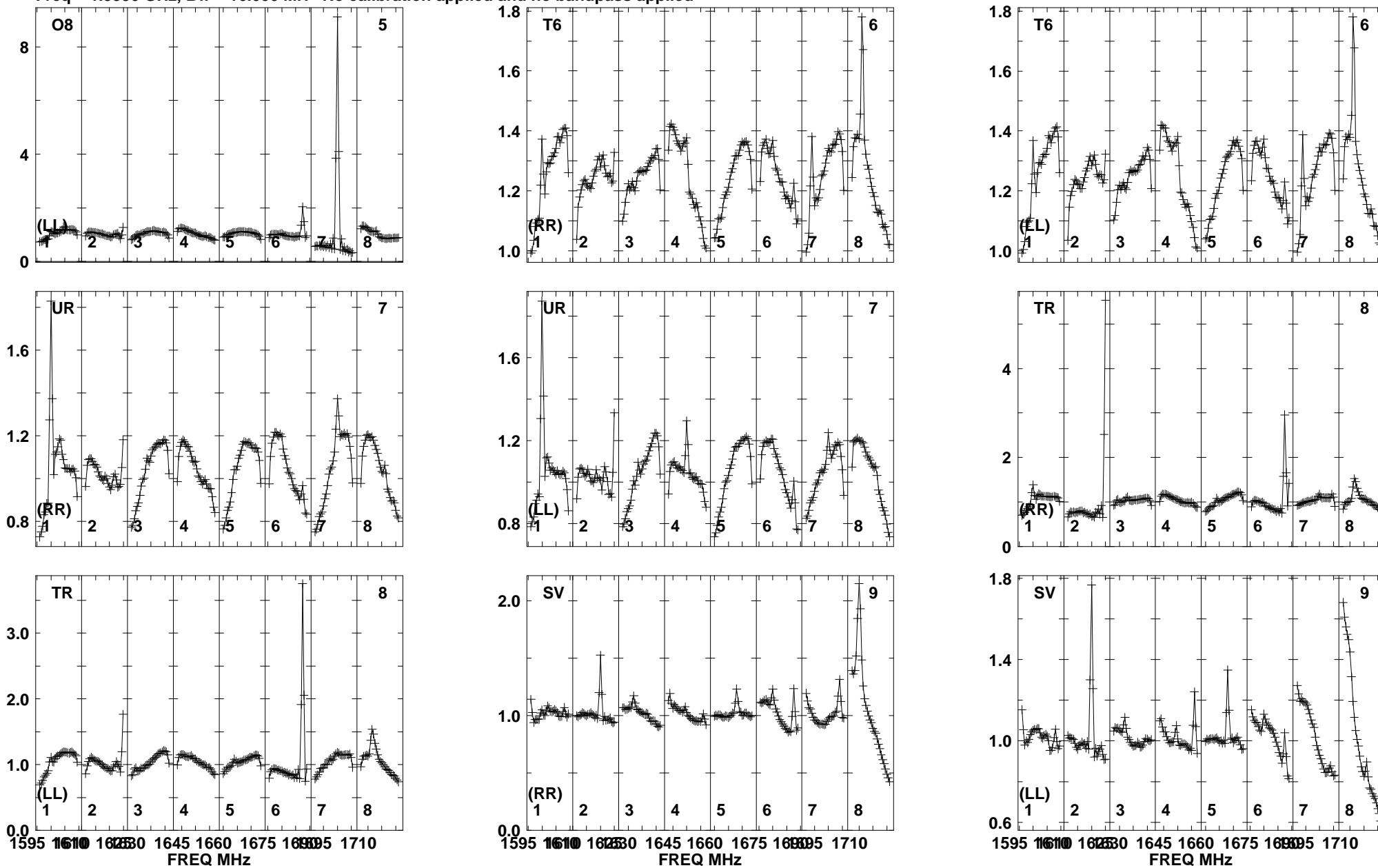
Lower frame: Real Jy Total-power spectrum Antenna: O8 (05) Timerange: 00/21:00:31 to 00/21:10:29
