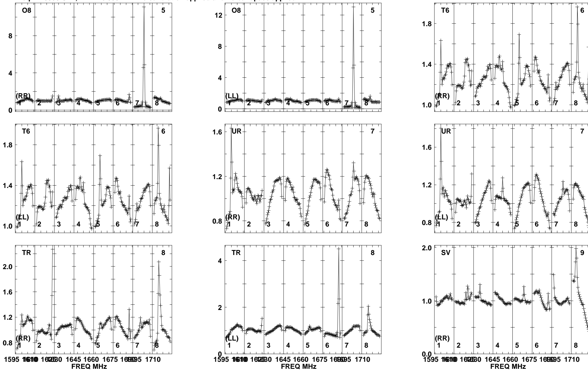
Lower frame: Real Jy Total-power spectrum Antenna: O8 (05) Timerange: 00/17:24:01 to 00/17:33:59
