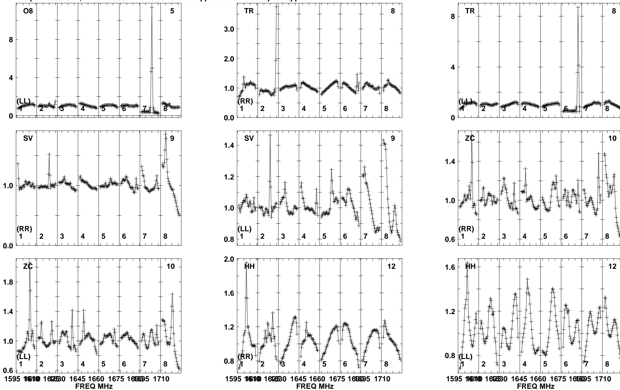
Lower frame: Real Jy Total-power spectrum Antenna: O8 (05) Timerange: 01/01:41:31 to 01/01:51:29
