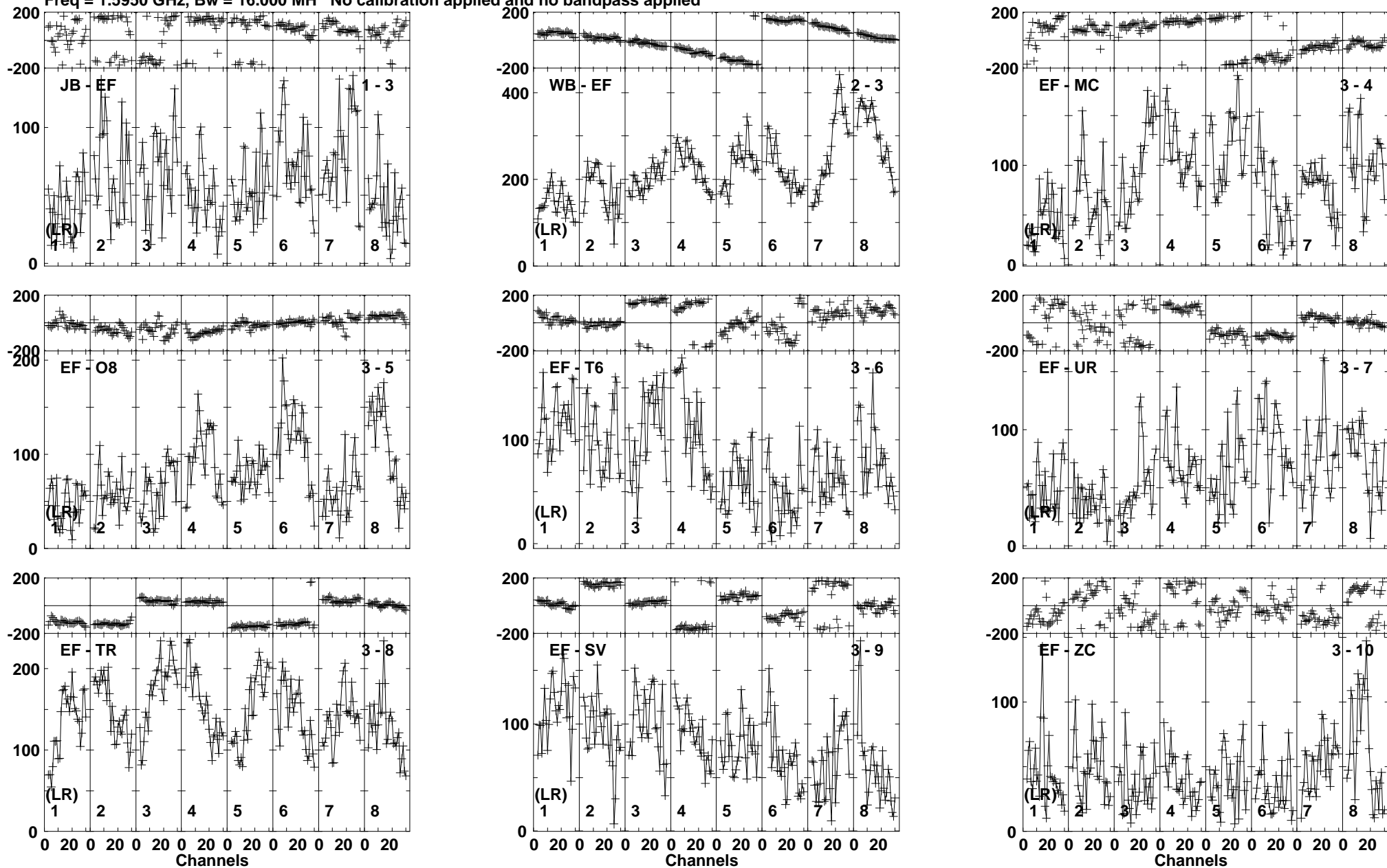
Lower frame: Micro Ampl Jy Top frame: Phas deg Vector averaged cross-power spectrum Baseline: JB (01) - EF (03) Timerange: 00/20:27:31 to 00/20:37:29
