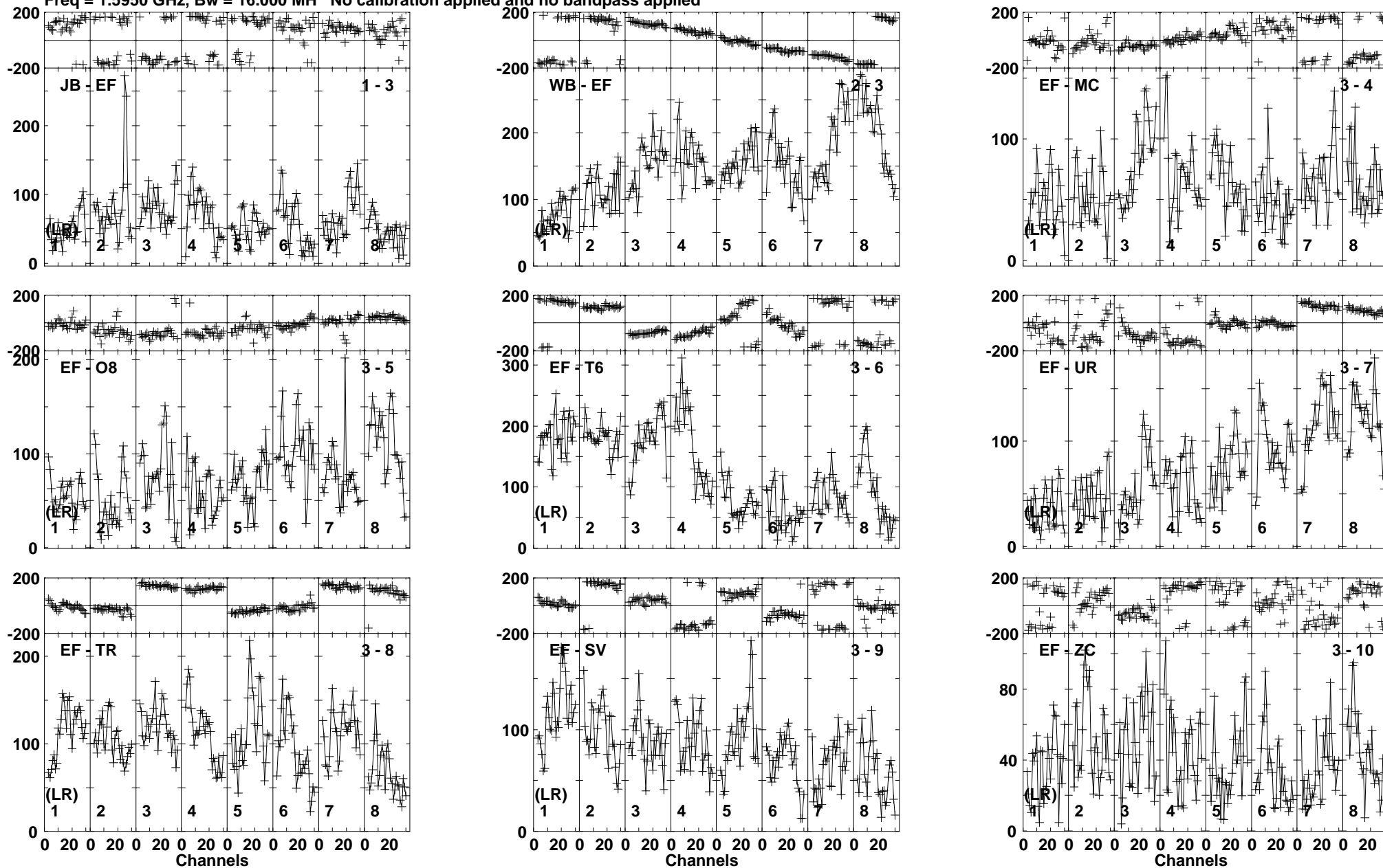
Lower frame: Micro Ampl Jy Top frame: Phas deg Vector averaged cross-power spectrum Baseline: JB (01) - EF (03) Timerange: 00/20:15:31 to 00/20:25:29
