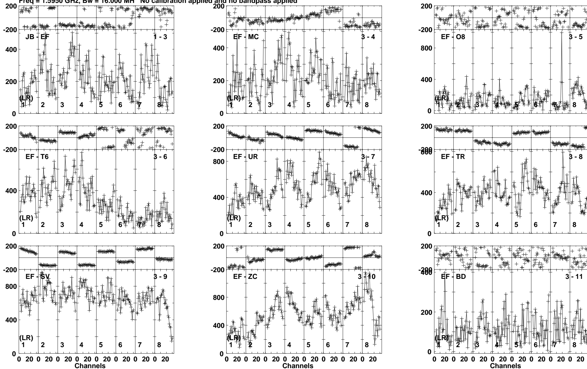
Lower frame: Micro Ampl Jy Top frame: Phas deg Vector averaged cross-power spectrum Baseline: JB (01) - EF (03) Timerange: 00/18:47:01 to 00/18:47:59
