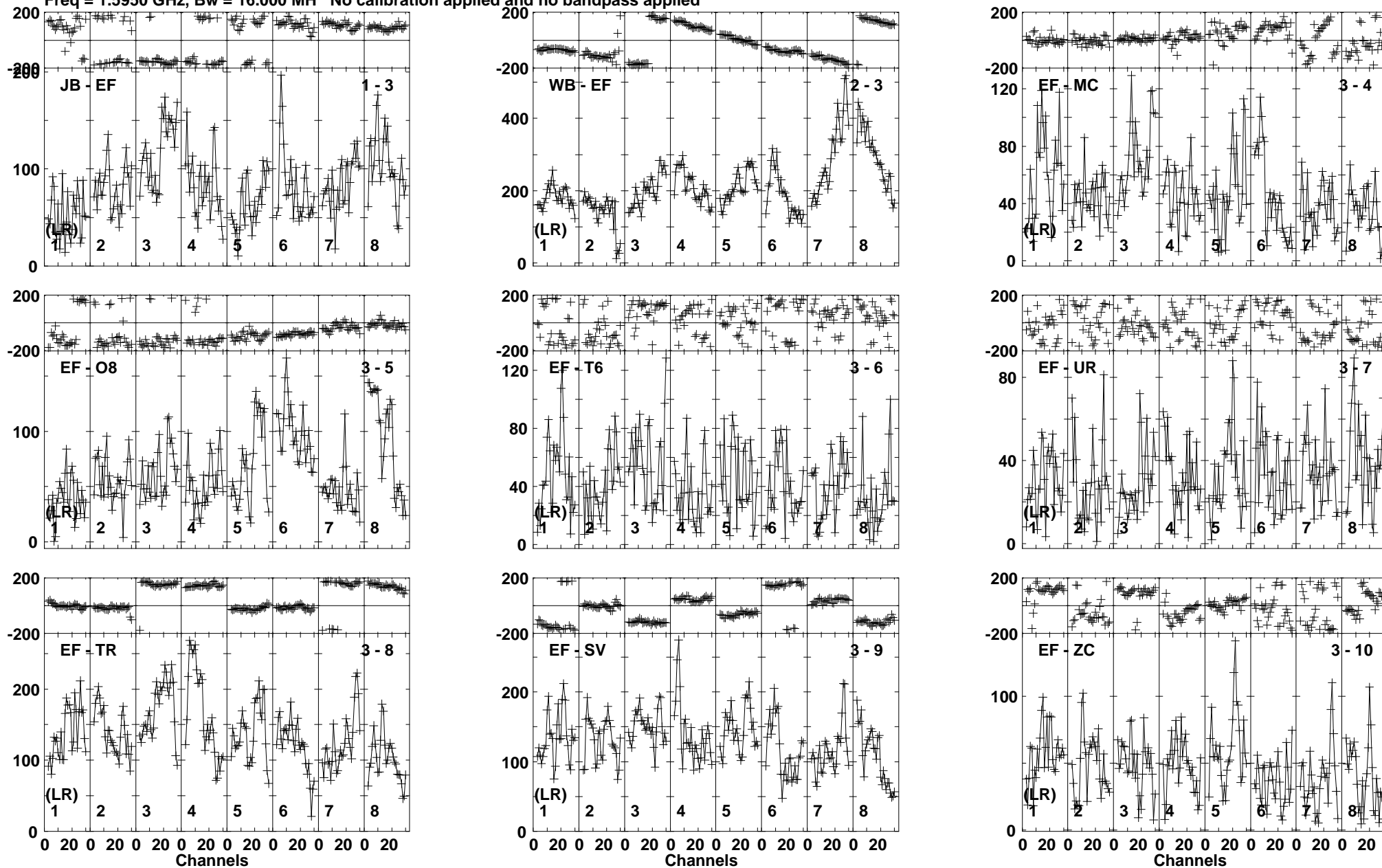
Lower frame: Micro Ampl Jy Top frame: Phas deg Vector averaged cross-power spectrum Baseline: JB (01) - EF (03) Timerange: 00/22:27:31 to 00/22:37:29
