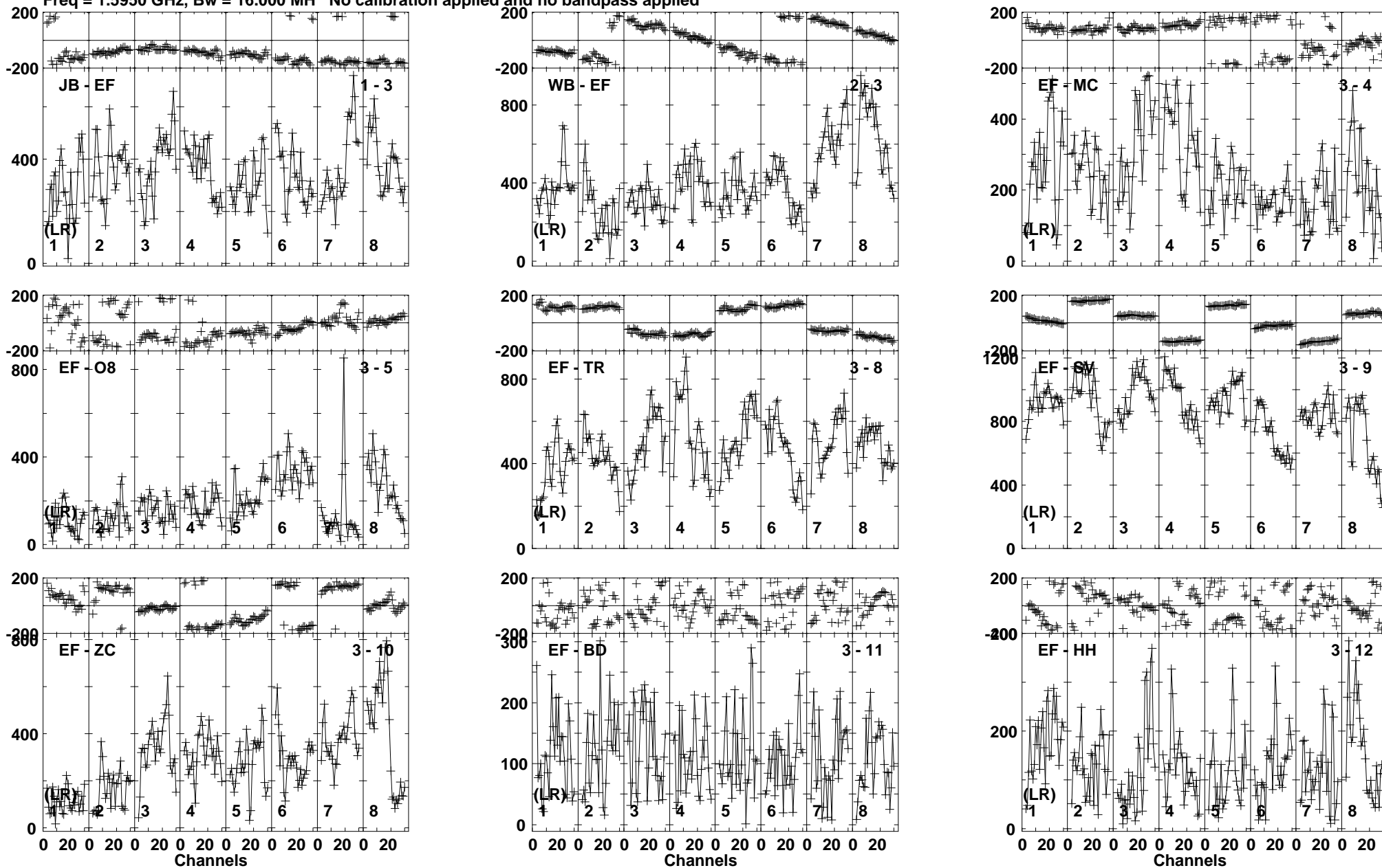
Lower frame: Micro Ampl Jy Top frame: Phas deg Vector averaged cross-power spectrum Baseline: JB (01) - EF (03) Timerange: 00/23:50:31 to 00/23:51:29
