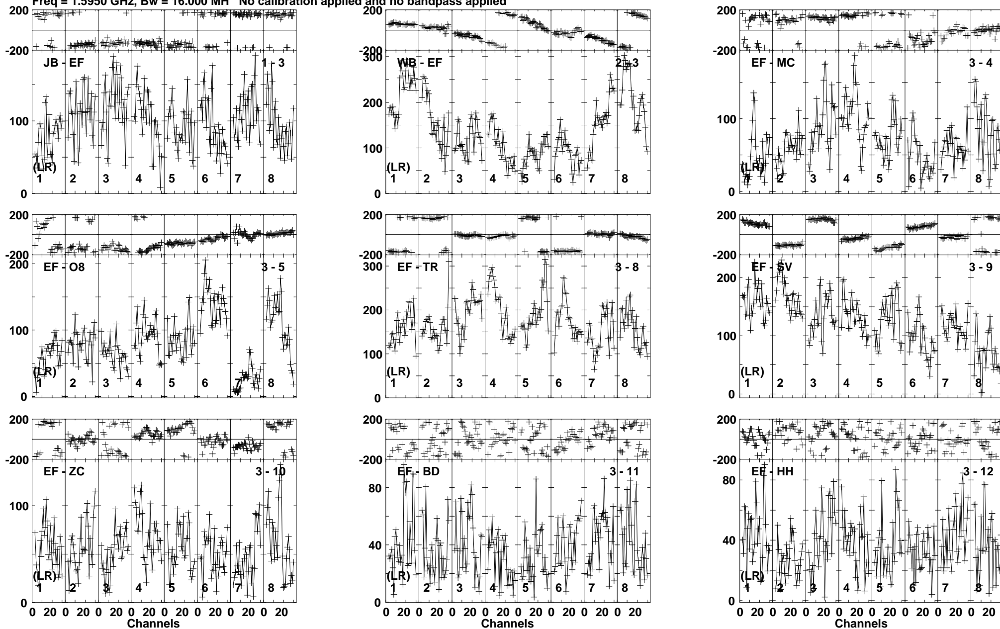
Lower frame: Micro Ampl Jy Top frame: Phas deg Vector averaged cross-power spectrum Baseline: JB (01) - EF (03) Timerange: 01/00:13:01 to 01/00:22:59
