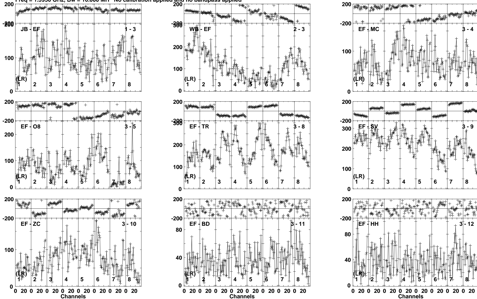
Lower frame: Micro Ampl Jy Top frame: Phas deg Vector averaged cross-power spectrum Baseline: JB (01) - EF (03) Timerange: 01/00:46:01 to 01/00:55:59
