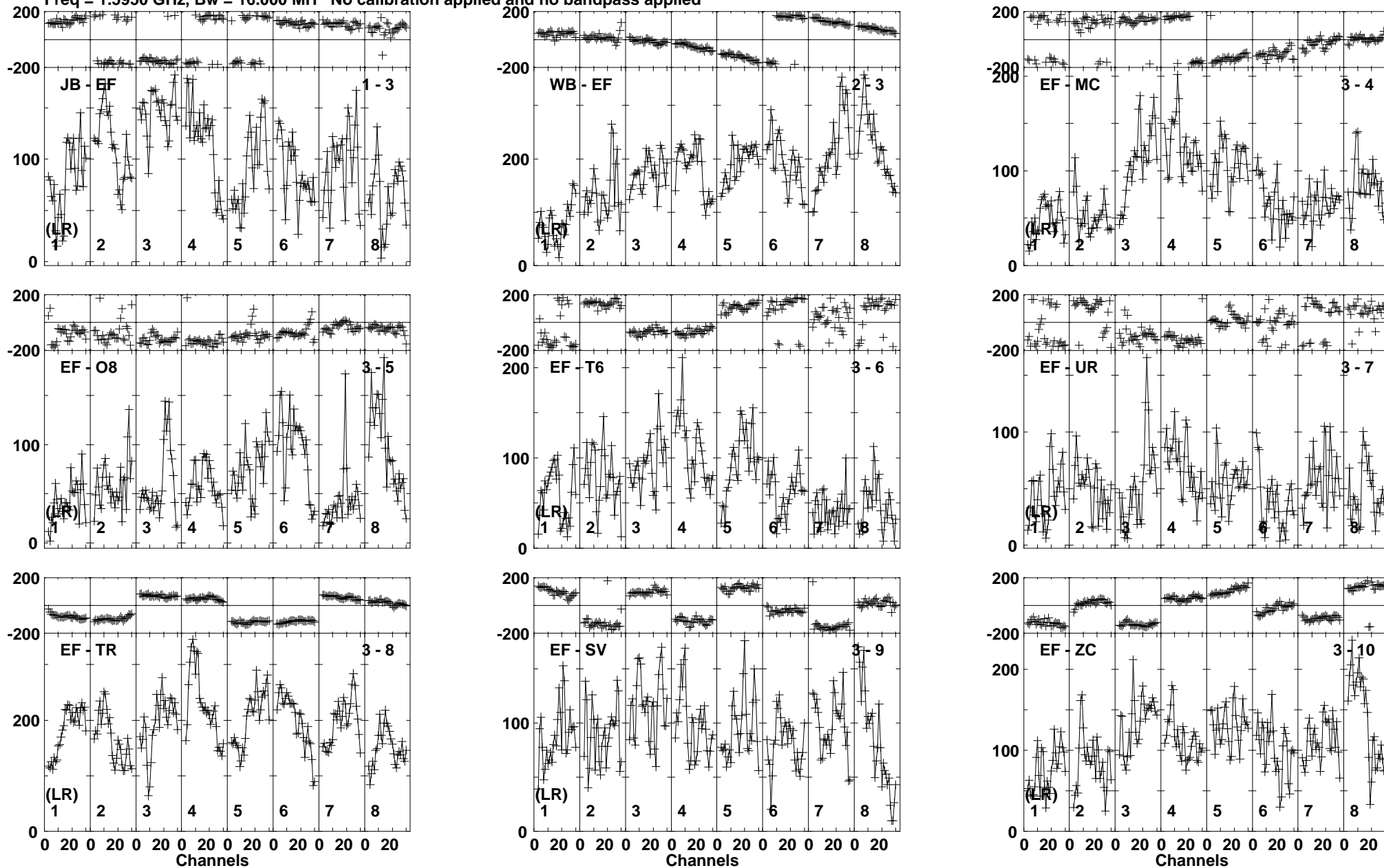
Lower frame: Micro Ampl Jy Top frame: Phas deg Vector averaged cross-power spectrum Baseline: JB (01) - EF (03) Timerange: 00:19:21:31 to 00:19:31:29
