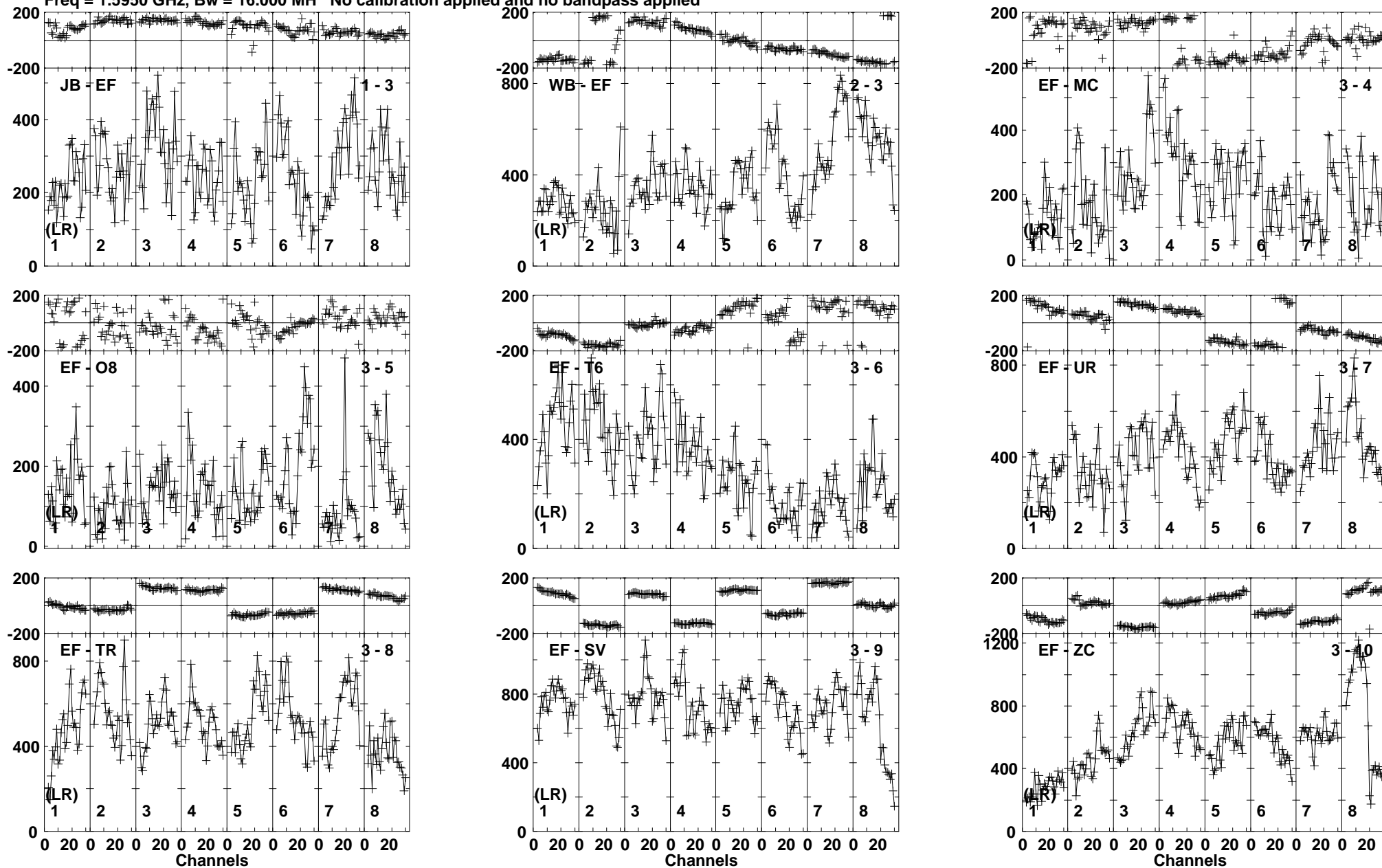
Lower frame: Micro Ampl Jy Top frame: Phas deg Vector averaged cross-power spectrum Baseline: JB (01) - EF (03) Timerange: 00/19:20:01 to 00/19:20:59
