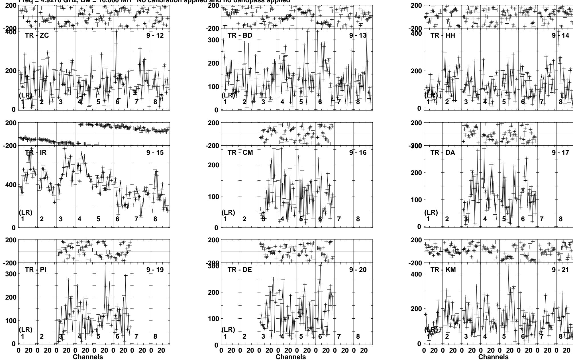
Lower frame: Micro Ampl Jy Top frame: Phas deg Vector averaged cross-power spectrum Baseline: TR (09) - ZC (12) Timerange: 00/22:05:01 to 00/22:05:59
