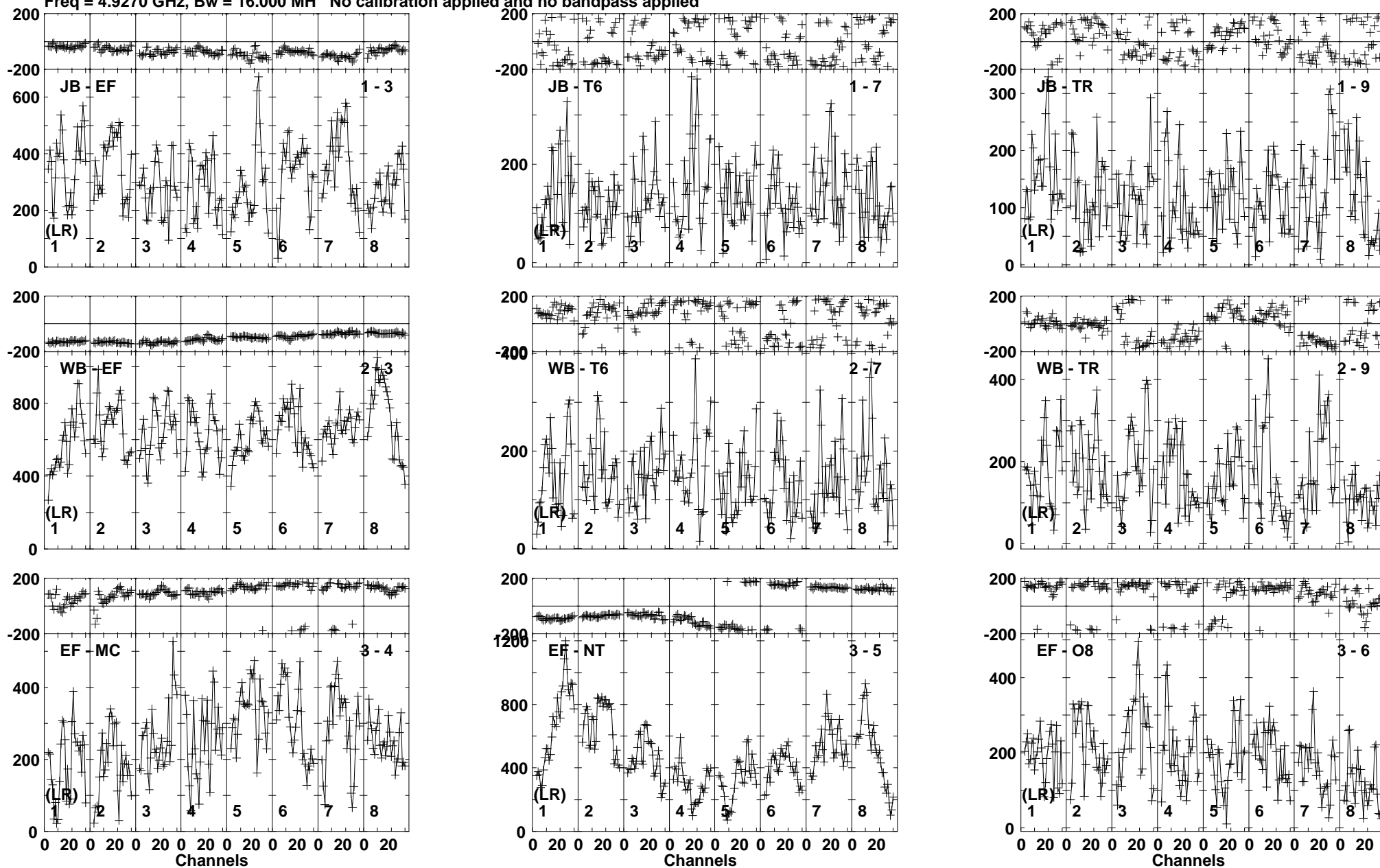
Lower frame: Micro Ampl Jy Top frame: Phas deg Vector averaged cross-power spectrum Baseline: JB (01) - EF (03) Timerange: 00/20:26:01 to 00/20:26:59
