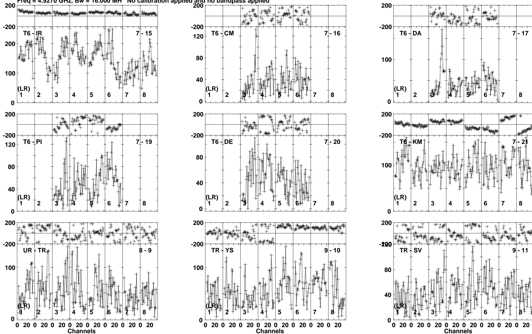
Lower frame: Micro Ampl Jy Top frame: Phas deg Vector averaged cross-power spectrum Baseline: T6 (07) - IR (15) Timerange: 00/19:32:01 to 00/19:41:59
