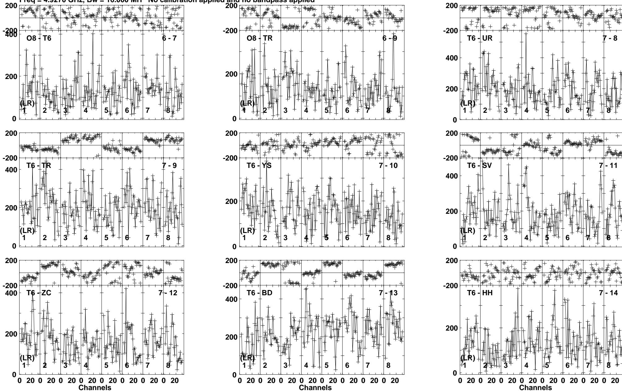
Lower frame: Micro Ampl Jy Top frame: Phas deg Vector averaged cross-power spectrum Baseline: O8 (06) - T6 (07) Timerange: 00/18:47:01 to 00/18:47:59
