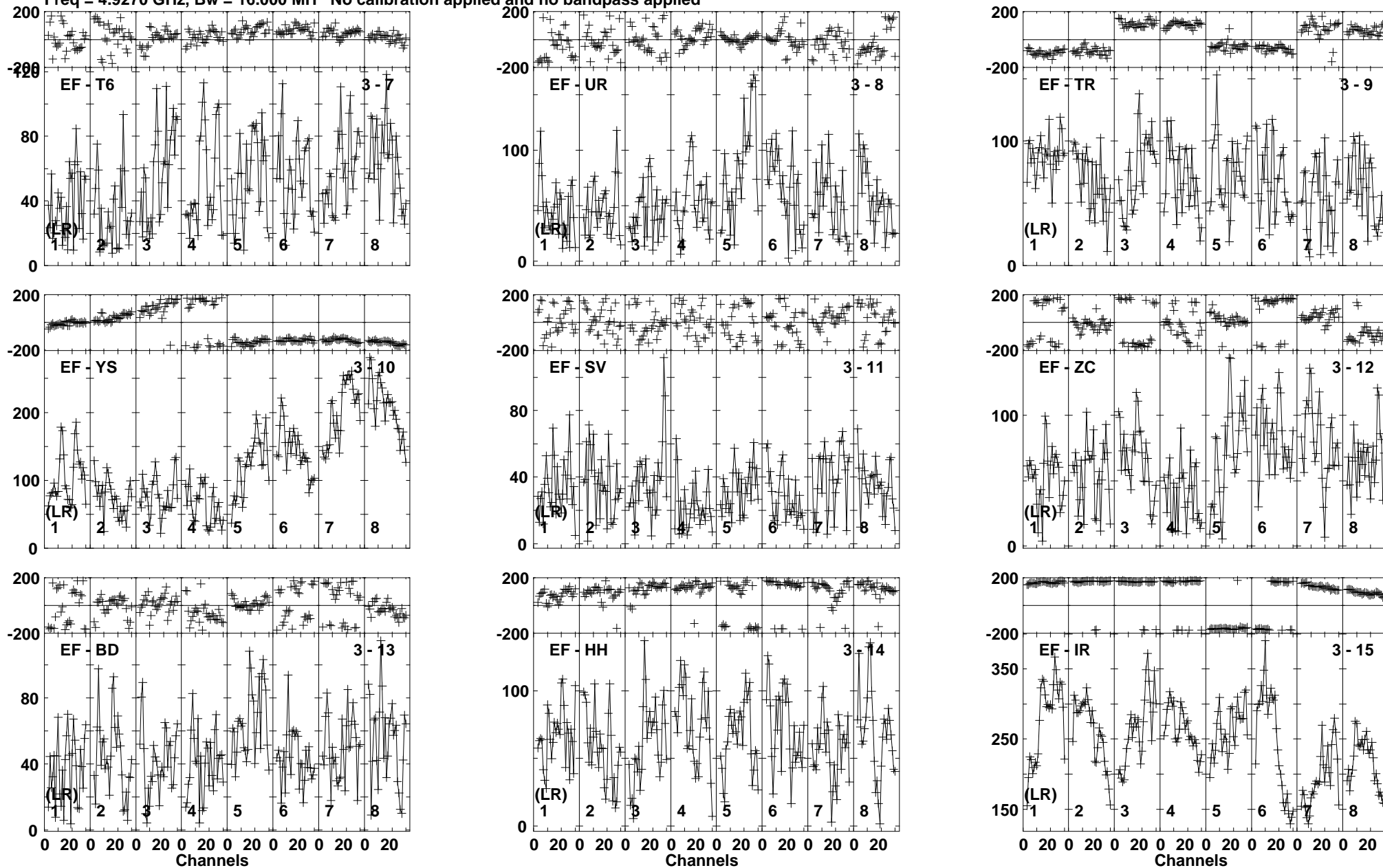
Lower frame: Micro Ampl Jy Top frame: Phas deg Vector averaged cross-power spectrum Baseline: EF (03) - T6 (07) Timerange: 00/21:33:31 to 00/21:43:29
