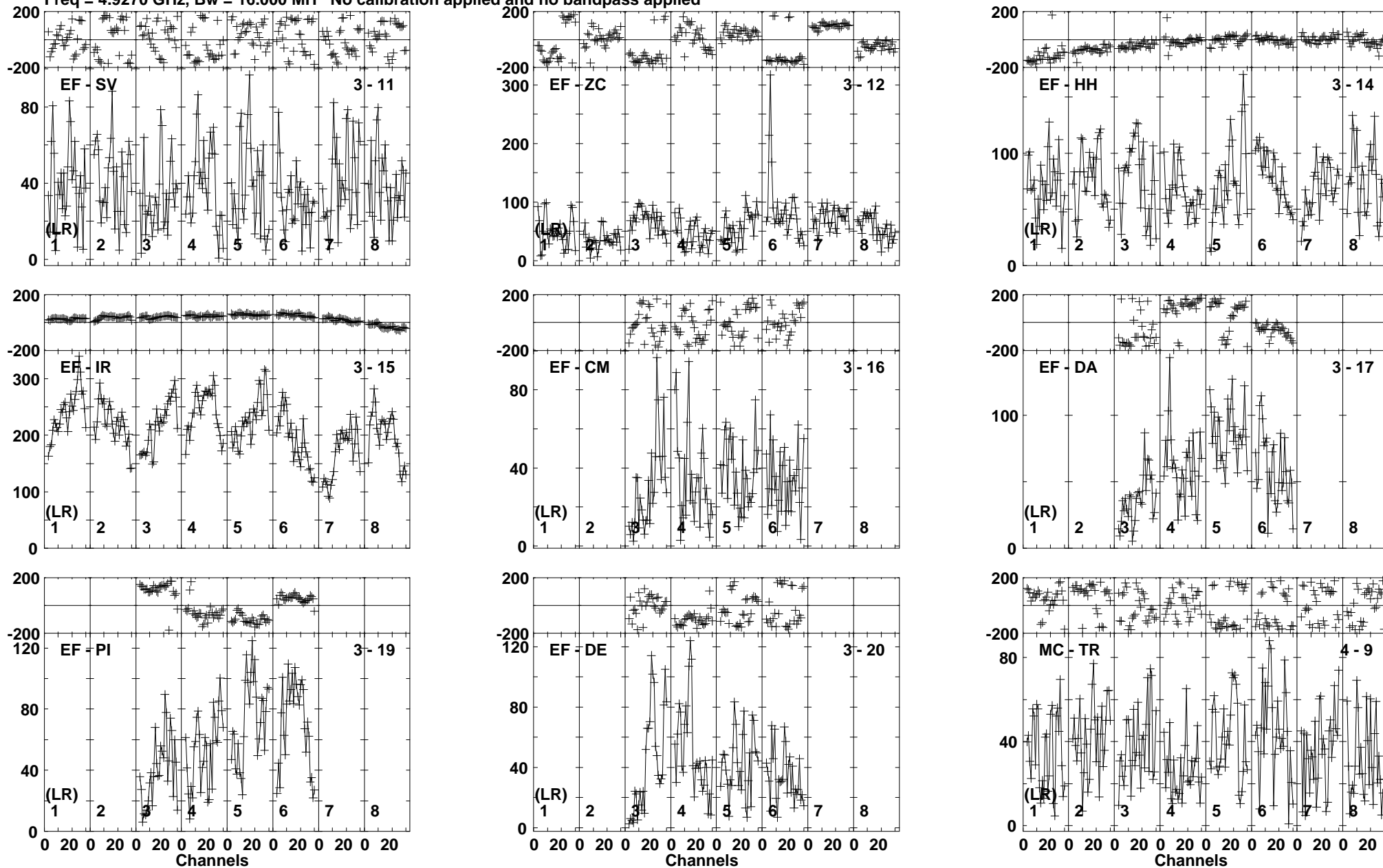
Lower frame: Micro Ampl Jy Top frame: Phas deg Vector averaged cross-power spectrum Baseline: EF (03) - SV (11) Timerange: 01/00:25:01 to 01/00:34:59
