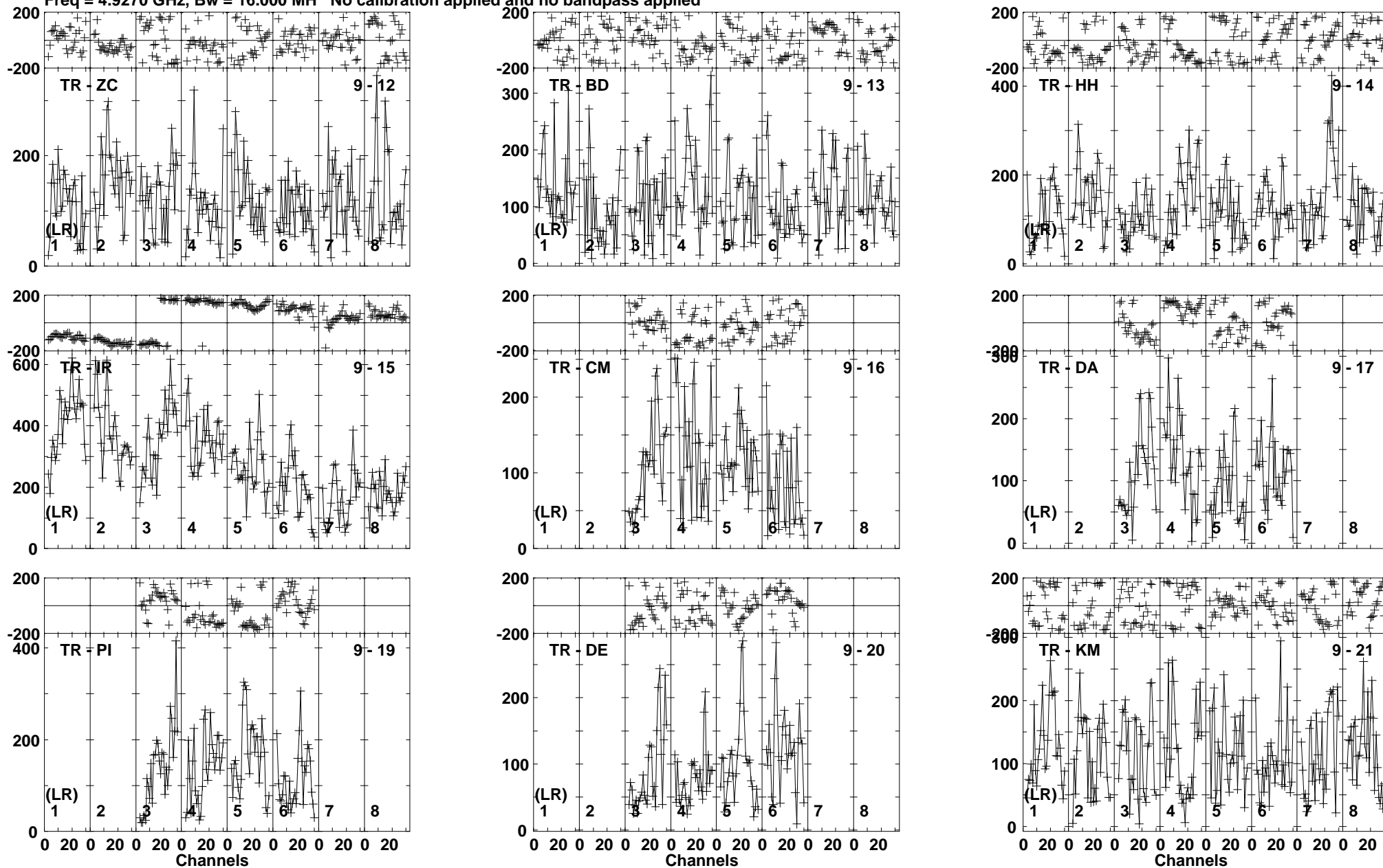
Lower frame: Micro Ampl Jy Top frame: Phas deg Vector averaged cross-power spectrum Baseline: TR (09) - ZC (12) Timerange: 00/19:53:01 to 00/19:53:59
