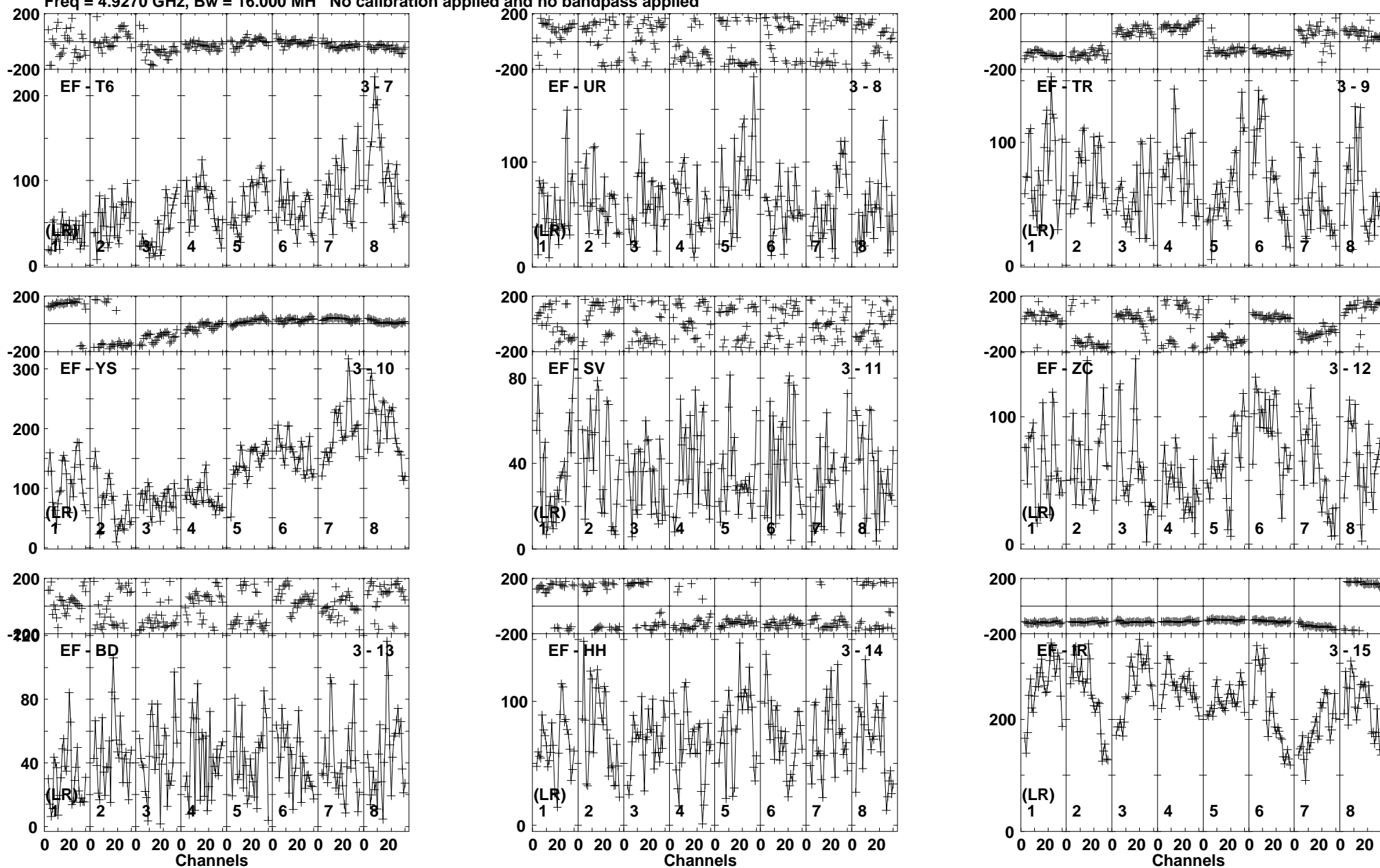
Lower frame: Micro Ampl Jy Top frame: Phas deg Vector averaged cross-power spectrum Baseline: EF (03) - T6 (07) Timerange: 00/22:06:31 to 00/22:16:29
