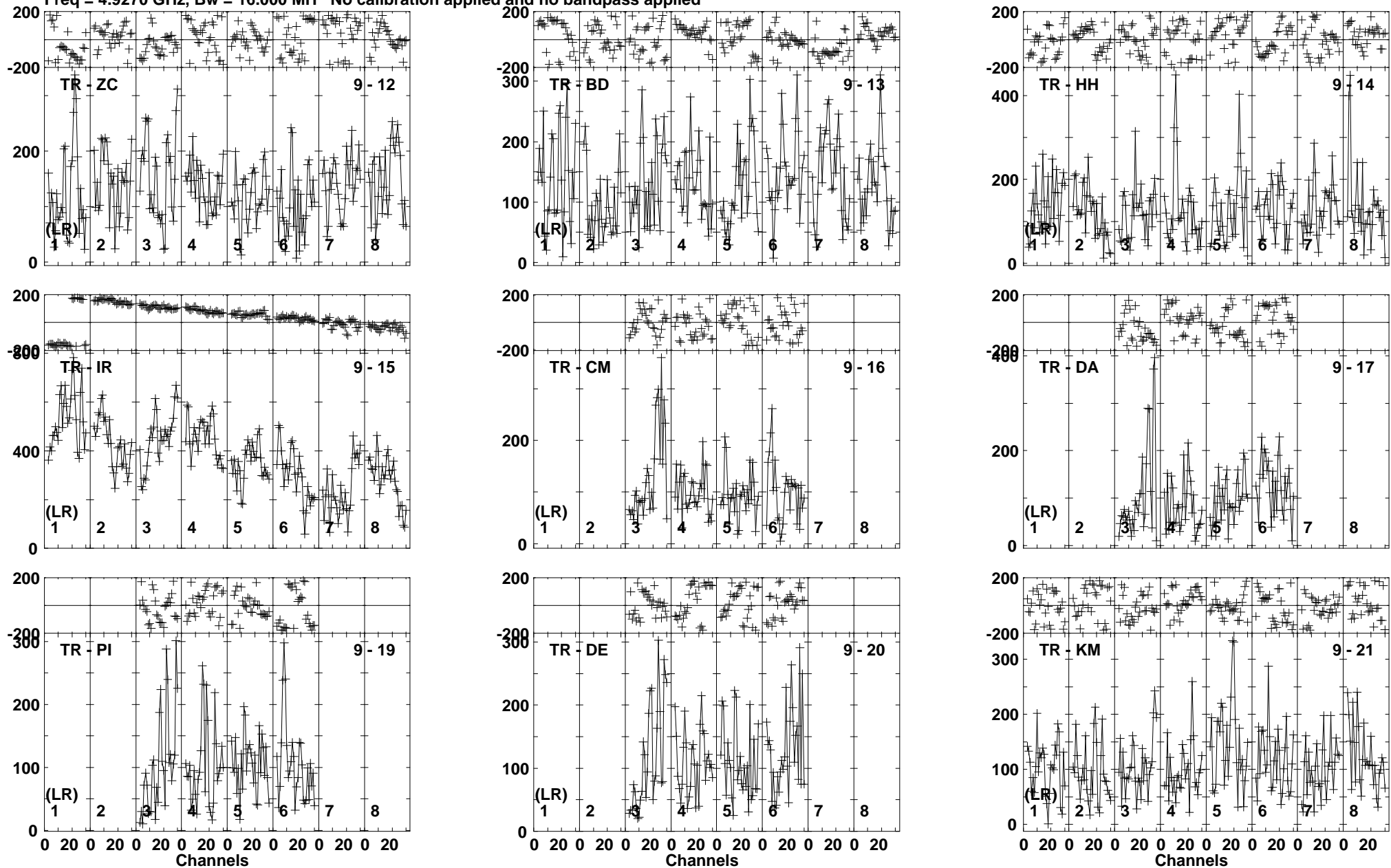
Lower frame: Micro Ampl Jy Top frame: Phas deg Vector averaged cross-power spectrum Baseline: TR (09) - ZC (12) Timerange: 00:21:32:01 to 00:21:32:59
