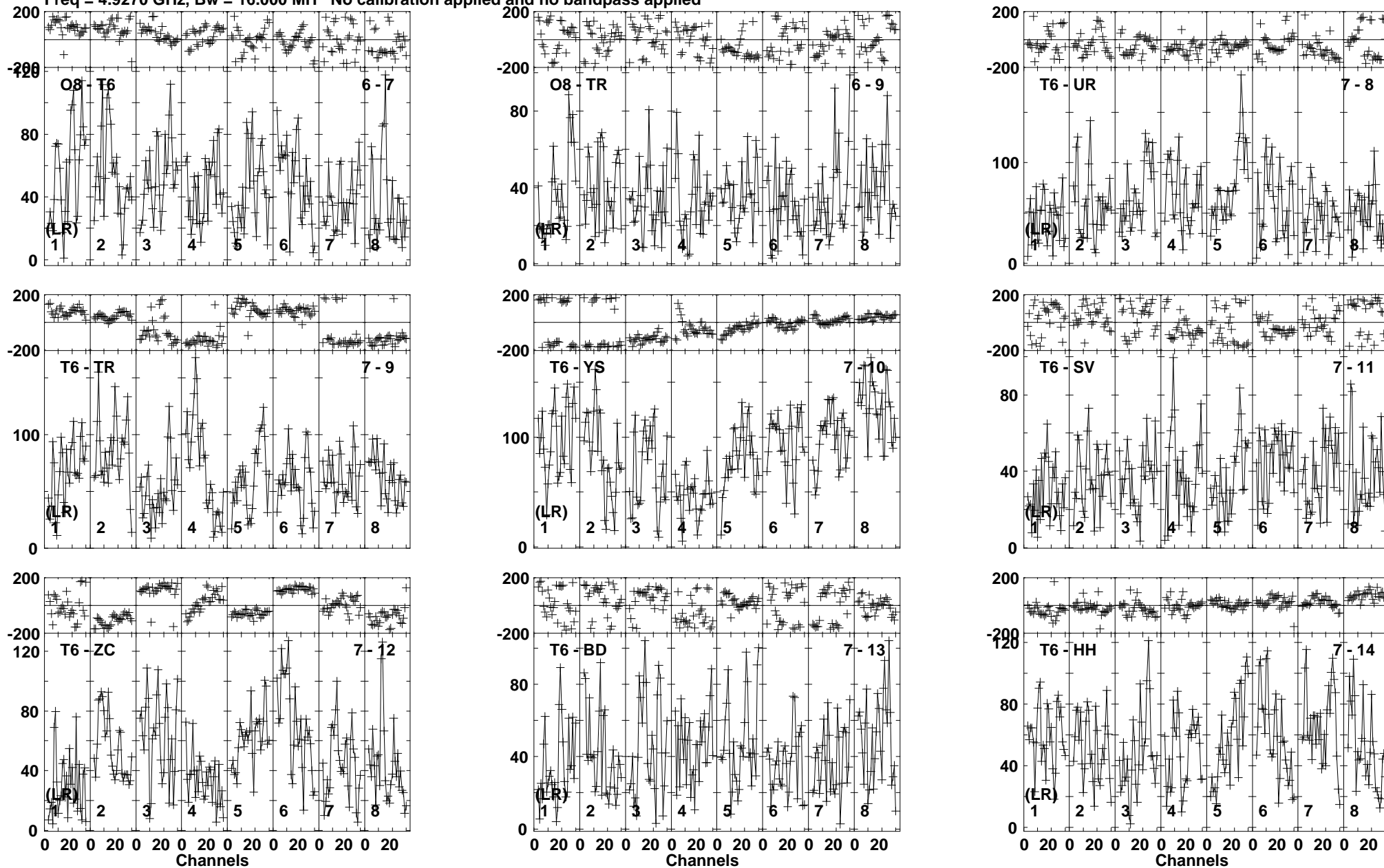
Lower frame: Micro Ampl Jy Top frame: Phas deg Vector averaged cross-power spectrum Baseline: O8 (06) - T6 (07) Timerange: 00/20:38:01 to 00/20:47:59
