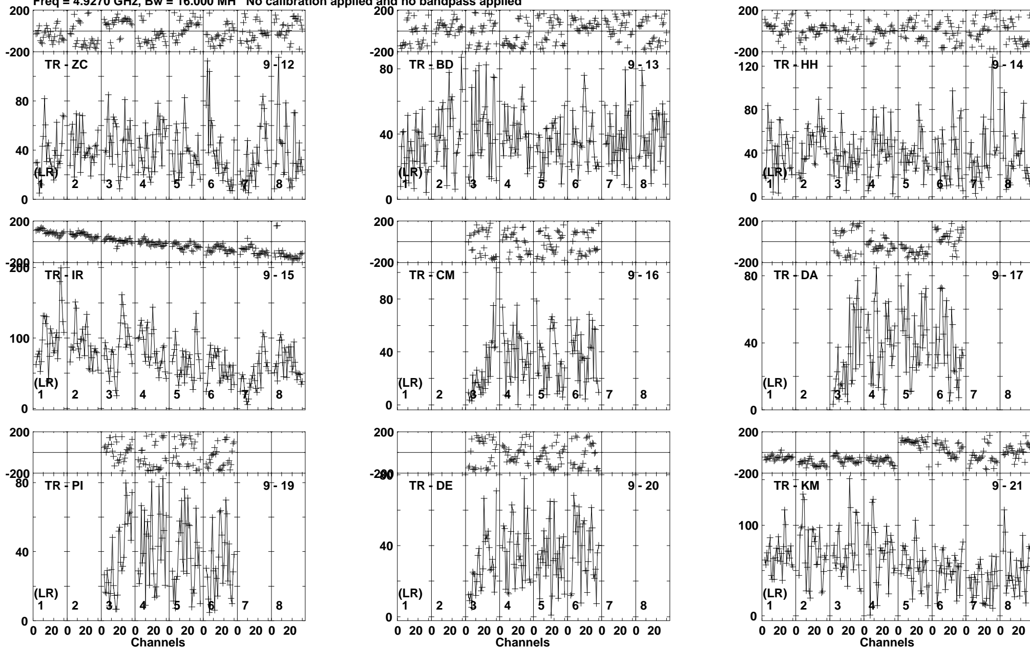
Lower frame: Micro Ampl Jy Top frame: Phas deg Vector averaged cross-power spectrum Baseline: TR (09) - ZC (12) Timerange: 00/21:11:01 to 00/21:20:59
