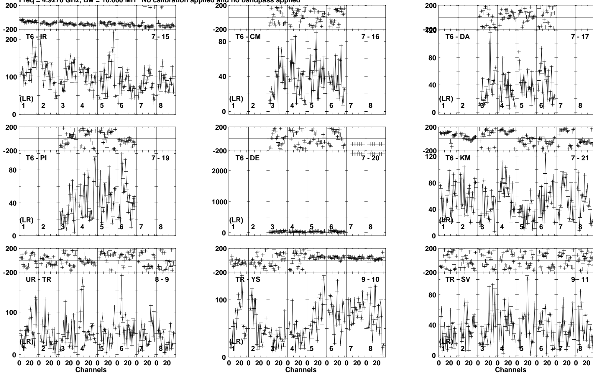
Lower frame: Micro Ampl Jy Top frame: Phas deg Vector averaged cross-power spectrum Baseline: T6 (07) - IR (15) Timerange: 00/21:21:31 to 00/21:31:29
