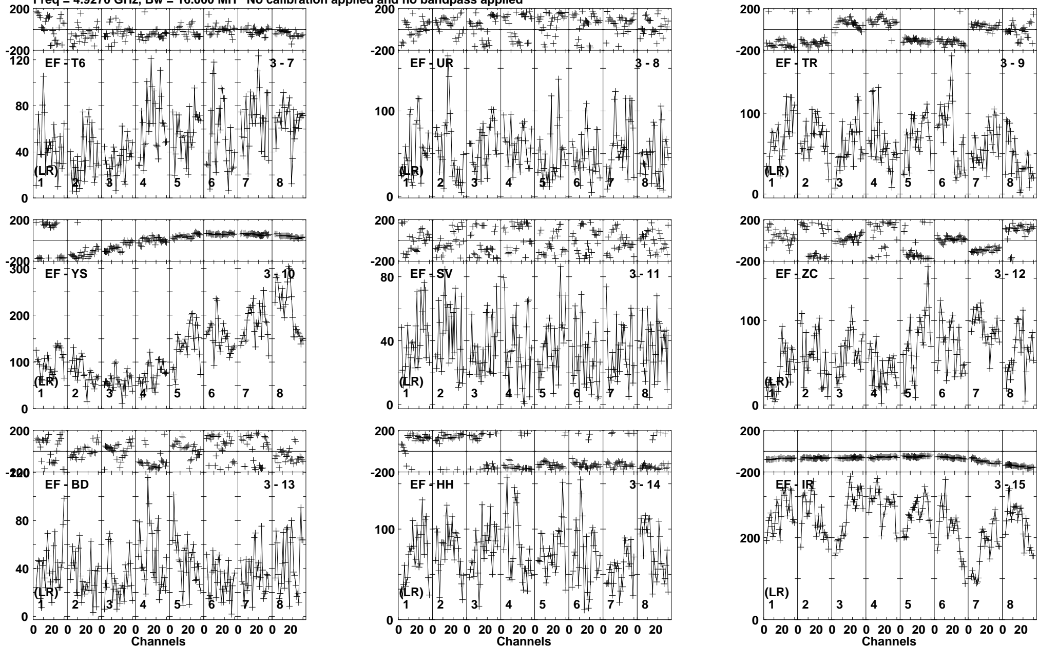
Lower frame: Micro Ampl Jy Top frame: Phas deg Vector averaged cross-power spectrum Baseline: EF (03) - T6 (07) Timerange: 00/22:17:01 to 00/22:26:59
