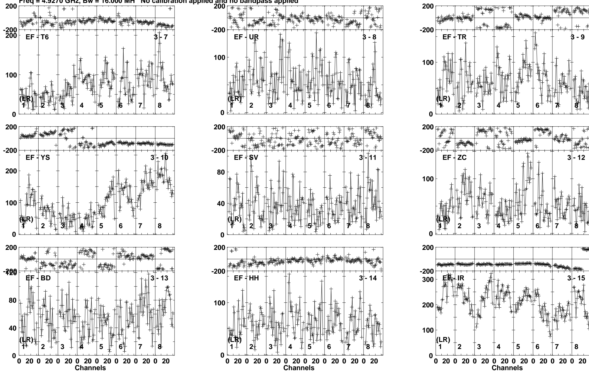
Lower frame: Micro Ampl Jy Top frame: Phas deg Vector averaged cross-power spectrum Baseline: EF (03) - T6 (07) Timerange: 00:18:48:31 to 00:18:58:29
