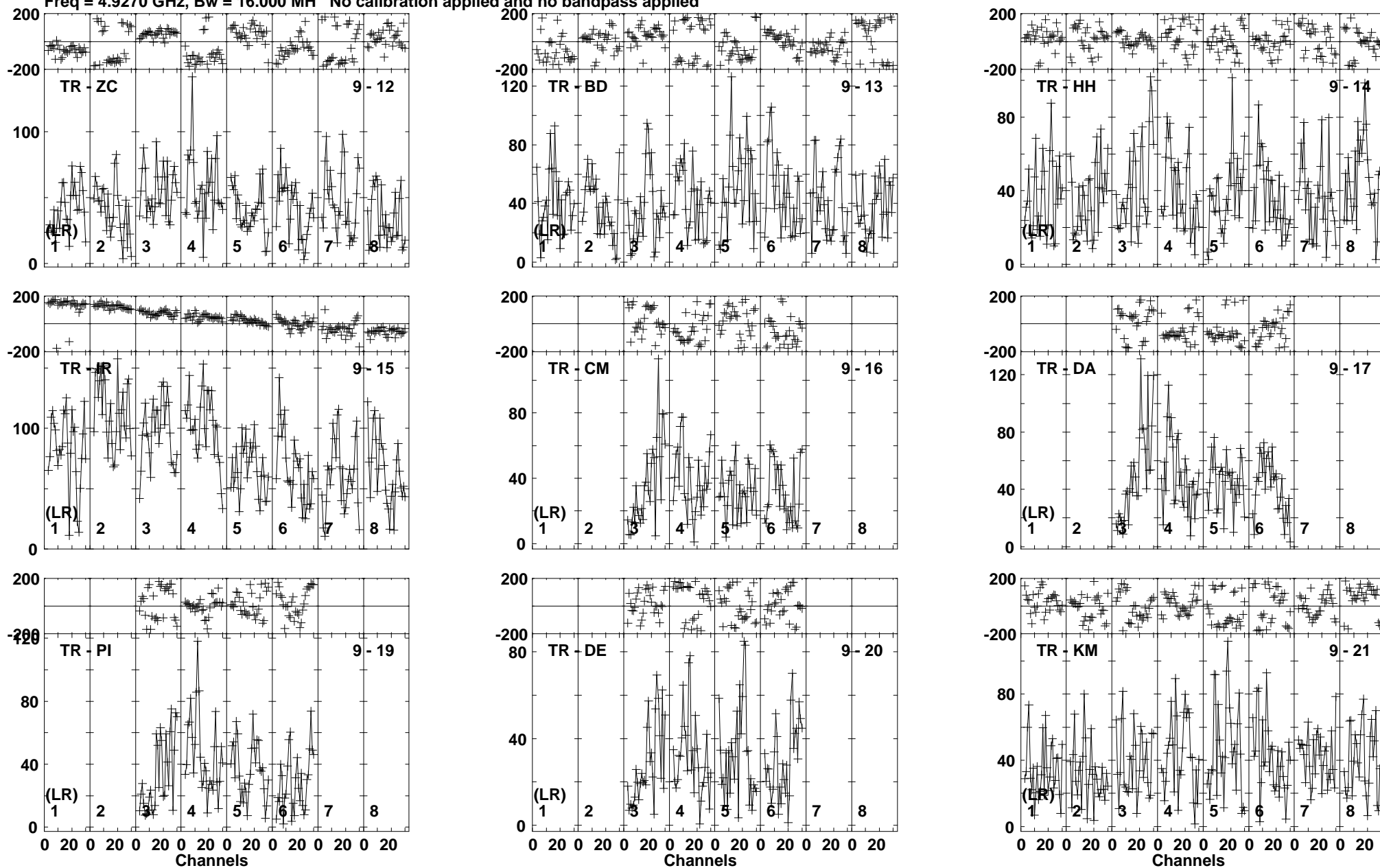
Lower frame: Micro Ampl Jy Top frame: Phas deg Vector averaged cross-power spectrum Baseline: TR (09) - ZC (12) Timerange: 00/21:33:31 to 00/21:43:29
