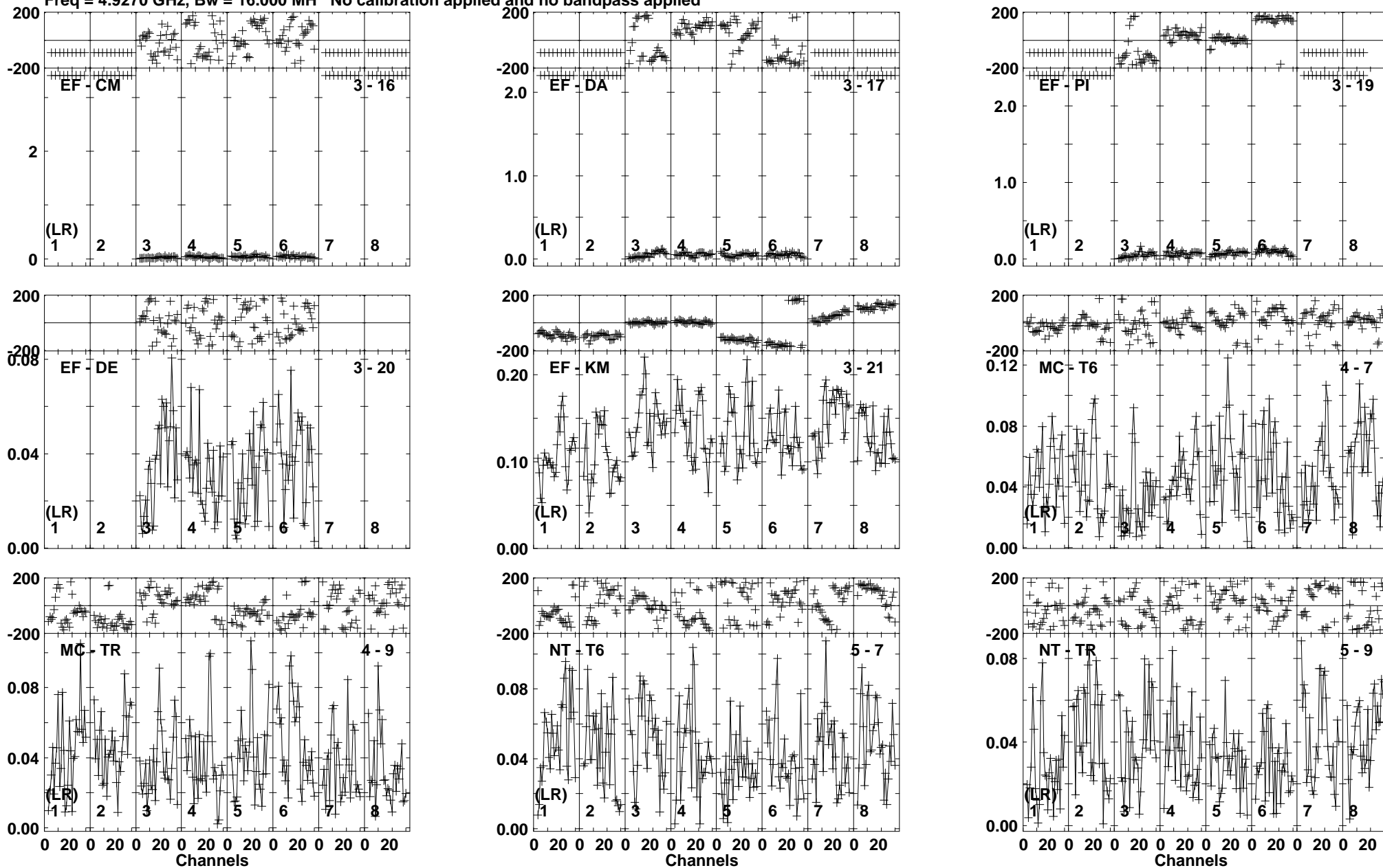
Lower frame: Milli Ampl Jy Top frame: Phas deg Vector averaged cross-power spectrum Baseline: EF (03) - CM (16) Timerange: 00/20:15:31 to 00/20:25:29
