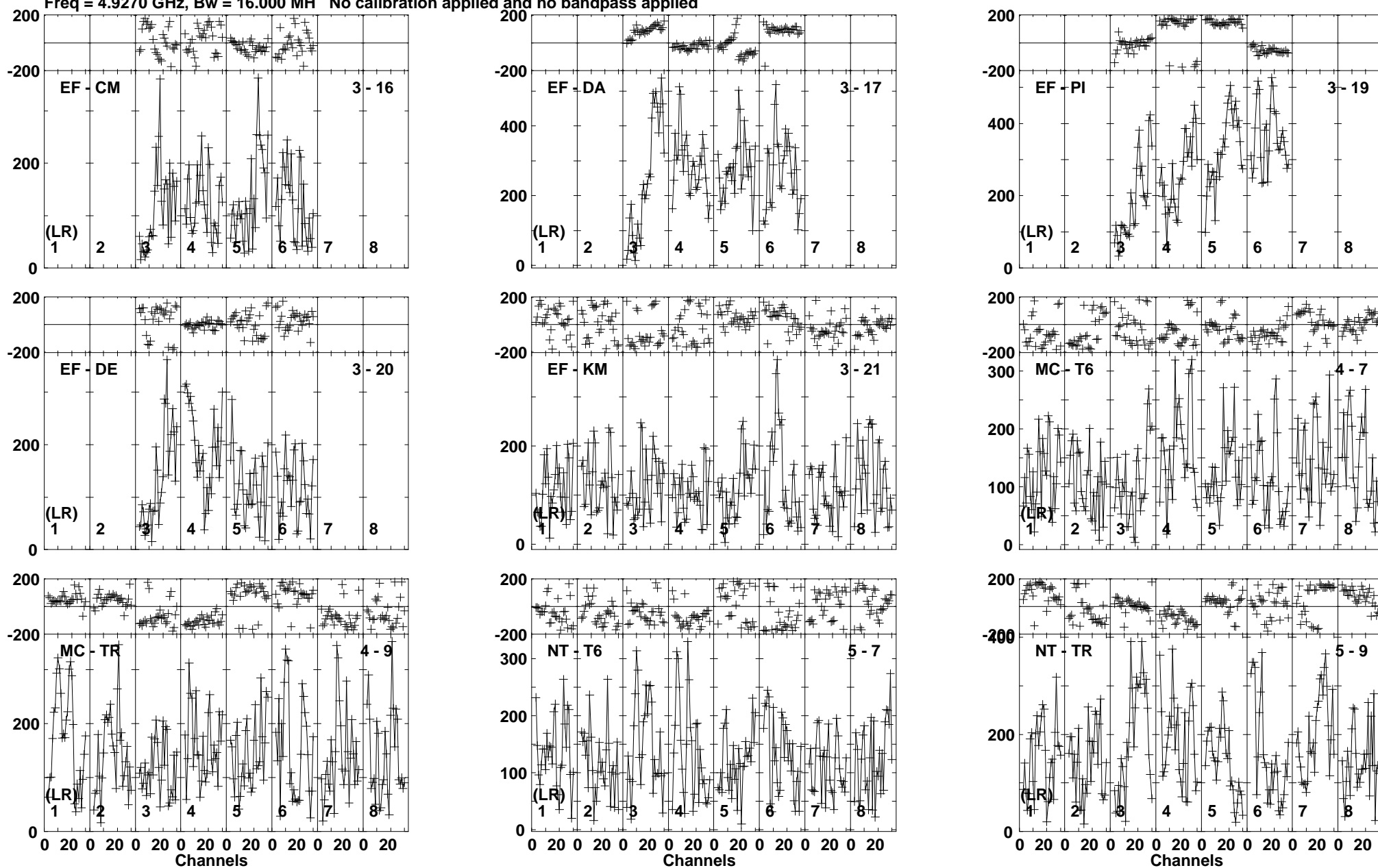
Lower frame: Micro Ampl Jy Top frame: Phas deg Vector averaged cross-power spectrum Baseline: EF (03) - CM (16) Timerange: 00/22:05:01 to 00/22:05:59
