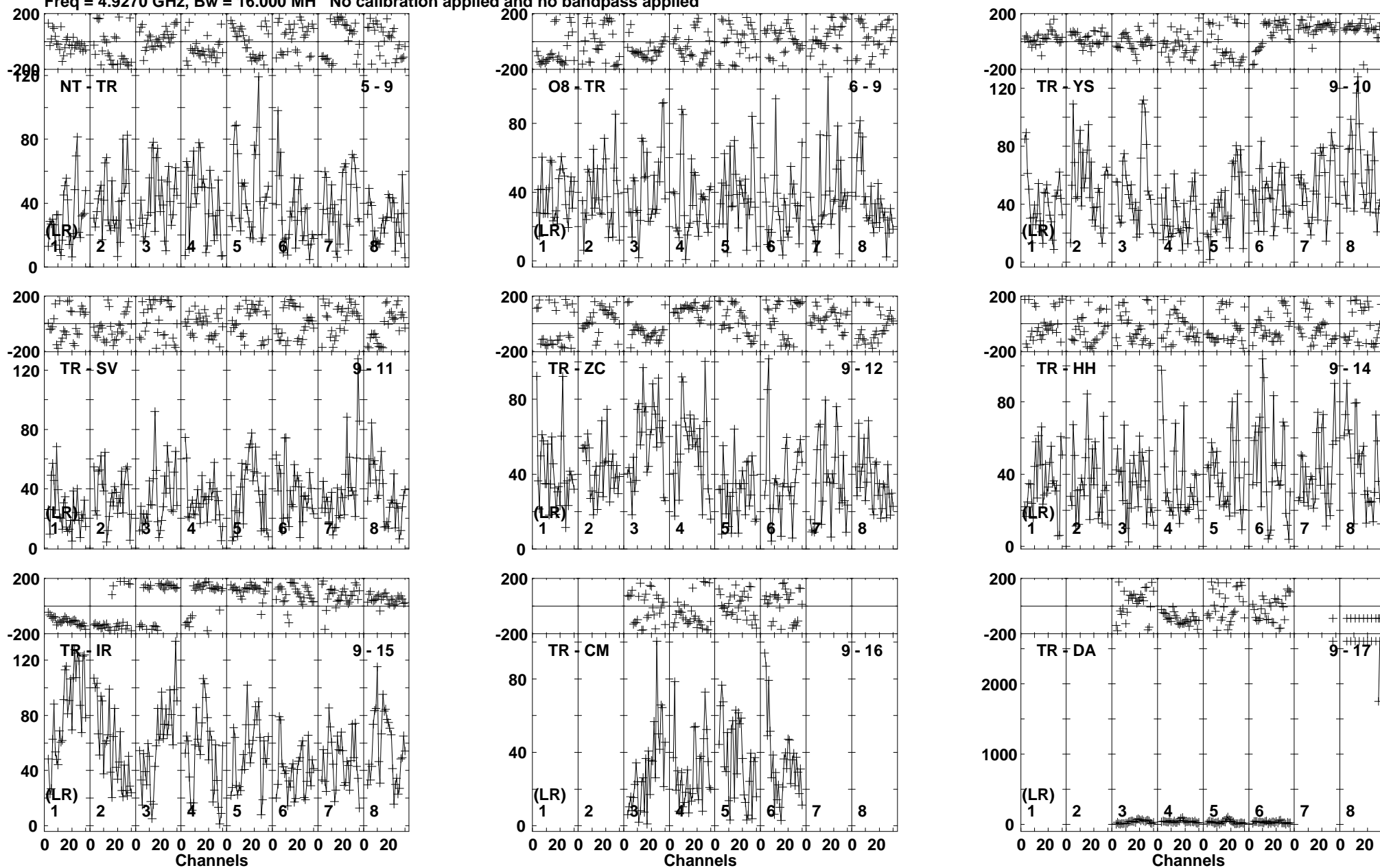
Lower frame: Micro Ampl Jy Top frame: Phas deg Vector averaged cross-power spectrum Baseline: NT (05) - TR (09) Timerange: 01/01:19:01 to 01/01:28:59
