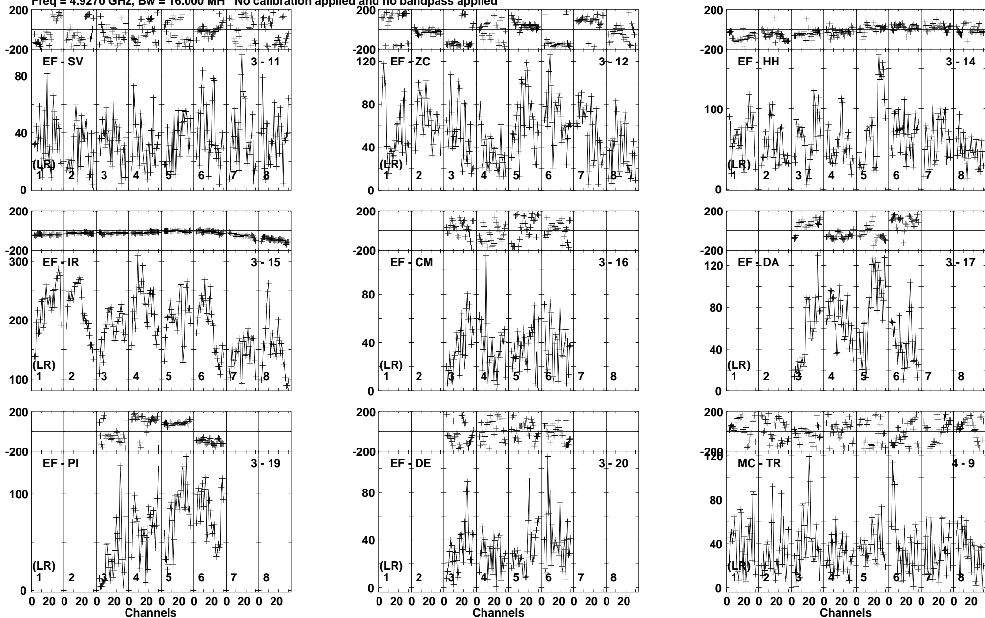
Lower frame: Micro Ampl Jy Top frame: Phas deg Vector averaged cross-power spectrum Baseline: EF (03) - SV (11) Timerange: 01/02:14:31 to 01/02:24:29
