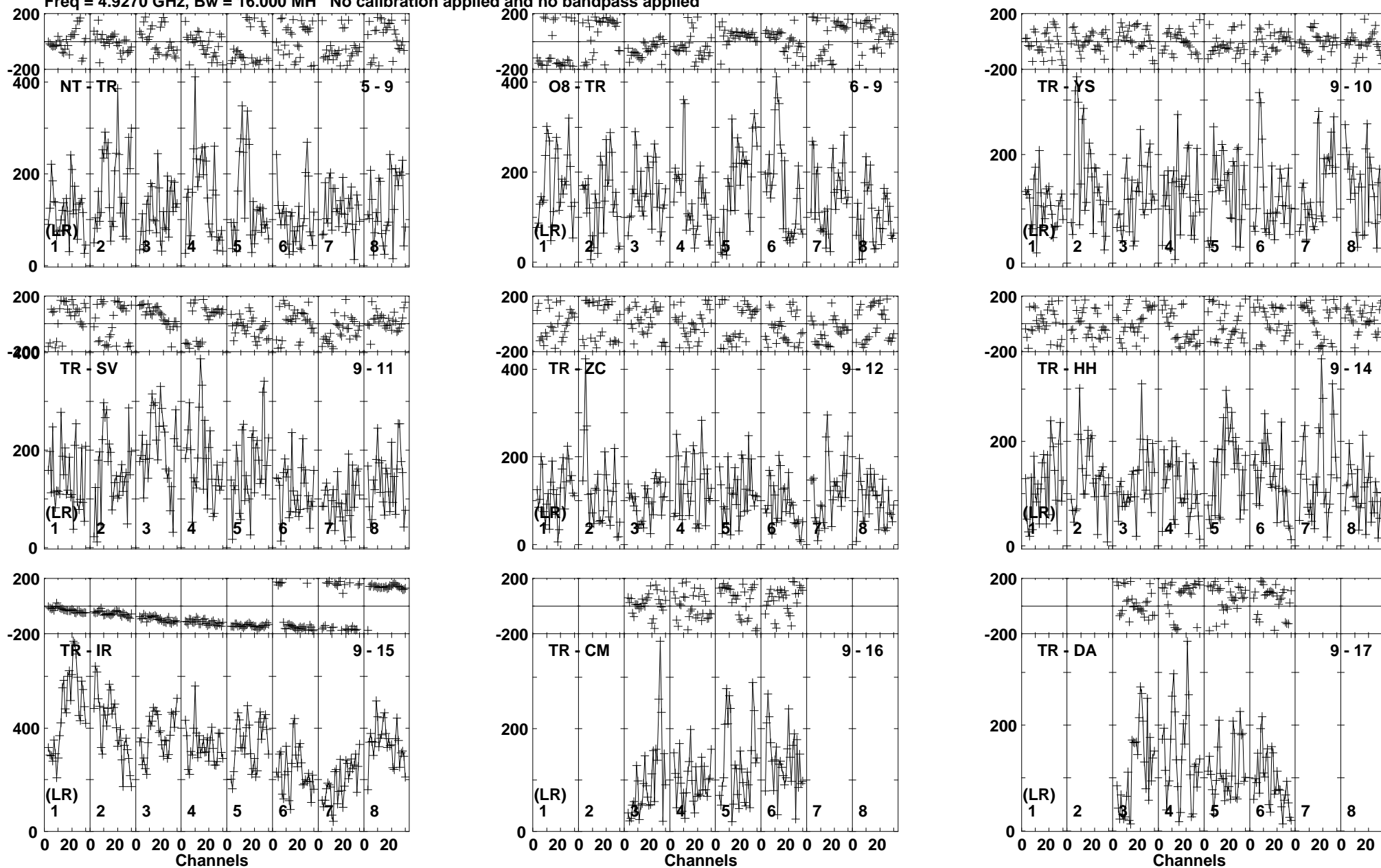
Lower frame: Micro Ampl Jy Top frame: Phas deg Vector averaged cross-power spectrum Baseline: NT (05) - TR (09) Timerange: 01/00:56:31 to 01/00:57:29
