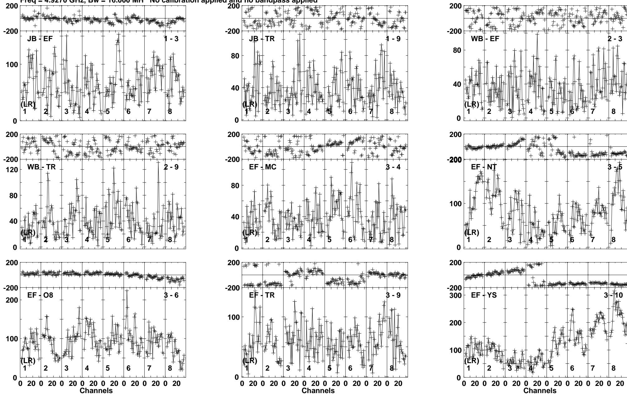
Lower frame: Micro Ampl Jy Top frame: Phas deg Vector averaged cross-power spectrum Baseline: JB (01) - EF (03) Timerange: 01/00:35:31 to 01/00:45:29
