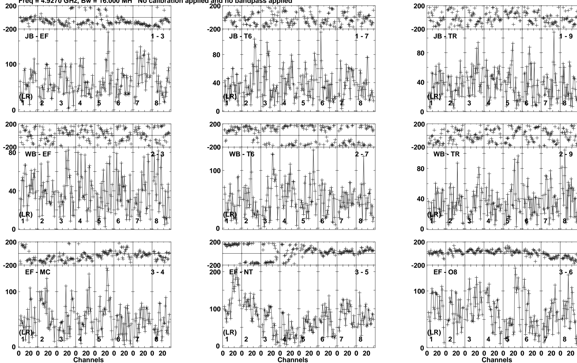
Lower frame: Micro Ampl Jy Top frame: Phas deg Vector averaged cross-power spectrum Baseline: JB (01) - EF (03) Timerange: 00/21:44:01 to 00/21:53:59
