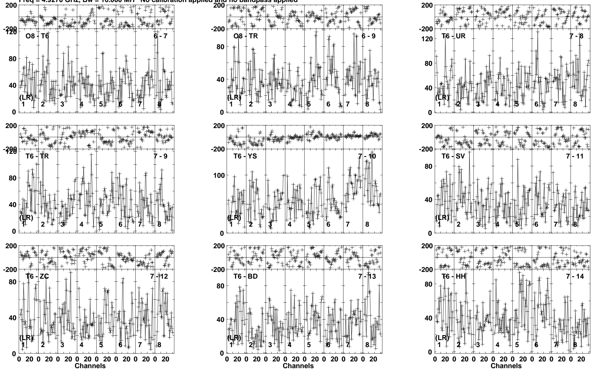
Lower frame: Micro Ampl Jy Top frame: Phas deg Vector averaged cross-power spectrum Baseline: O8 (06) - T6 (07) Timerange: 00/22:17:01 to 00/22:26:59
