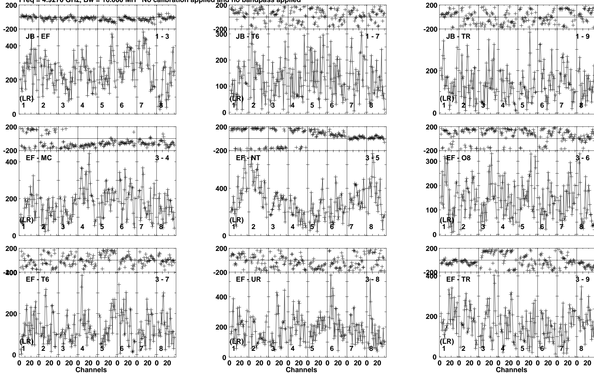
Lower frame: Micro Ampl Jy Top frame: Phas deg Vector averaged cross-power spectrum Baseline: JB (01) - EF (03) Timerange: 00:18:14:01 to 00:18:14:59
