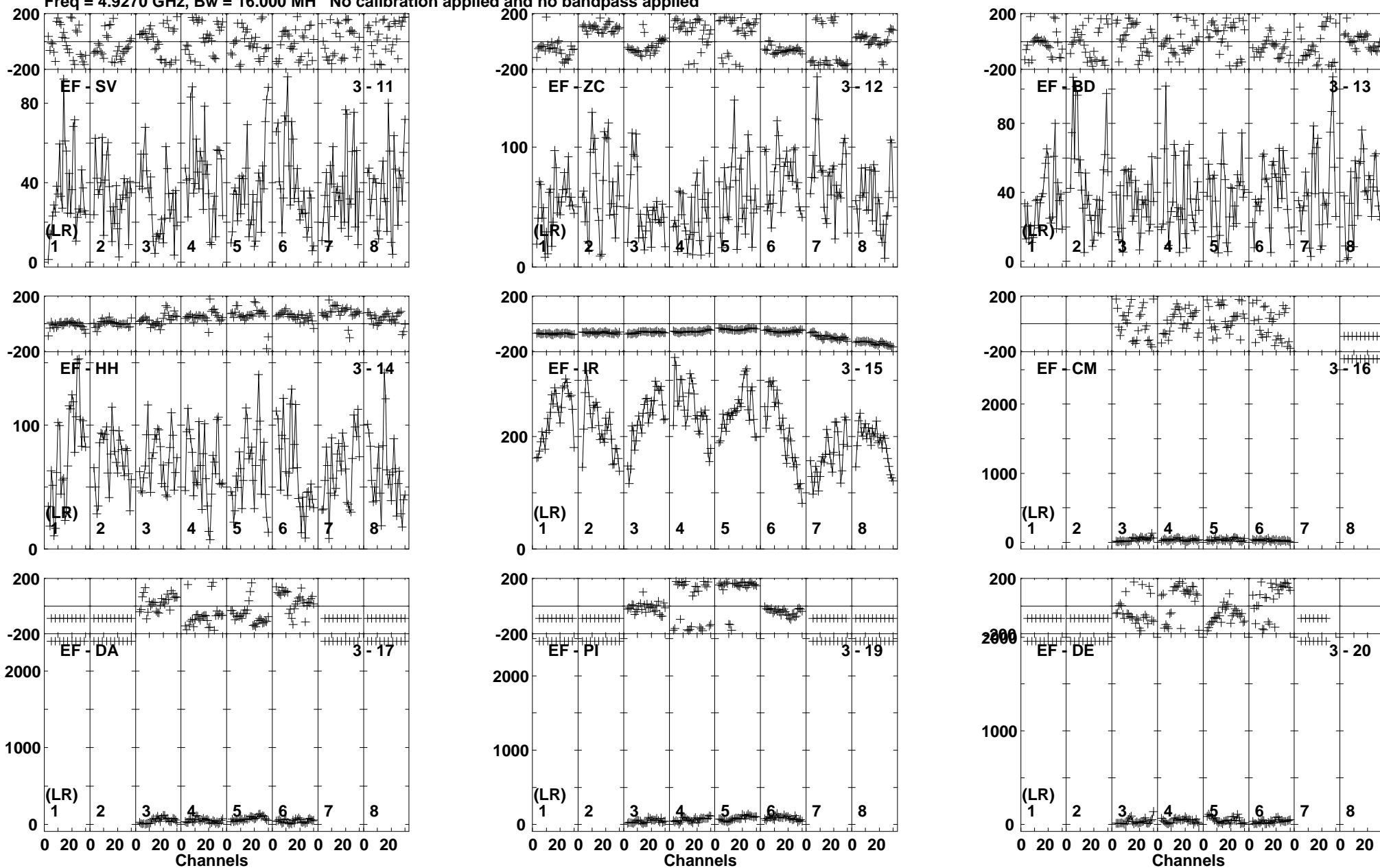
Lower frame: Micro Ampl Jy Top frame: Phas deg Vector averaged cross-power spectrum Baseline: EF (03) - SV (11) Timerange: 01/00:02:31 to 01/00:12:29
