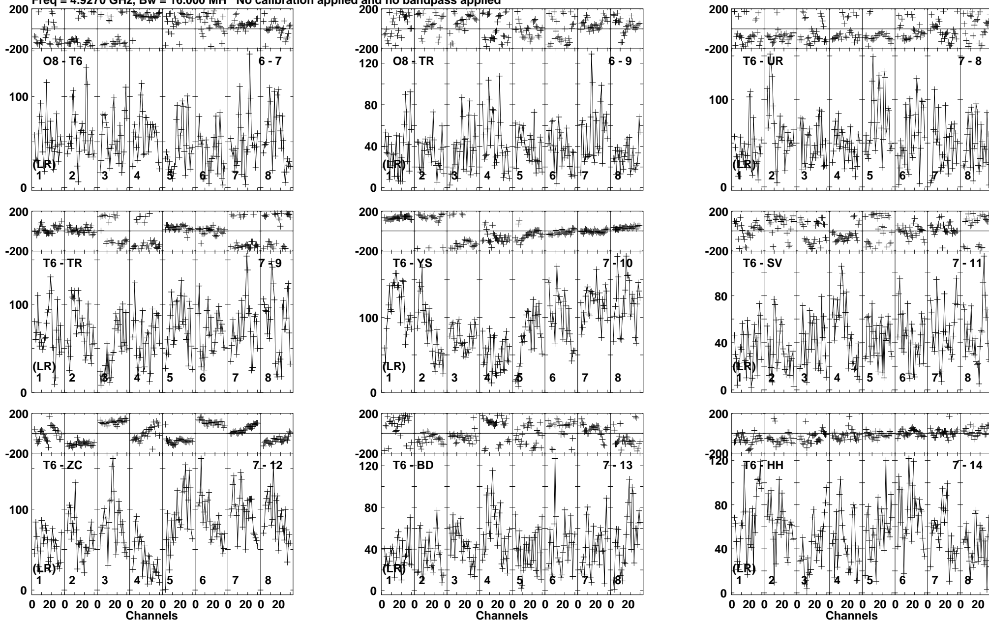
Lower frame: Micro Ampl Jy Top frame: Phas deg Vector averaged cross-power spectrum Baseline: O8 (06) - T6 (07) Timerange: 00:19:32:01 to 00:19:41:59
