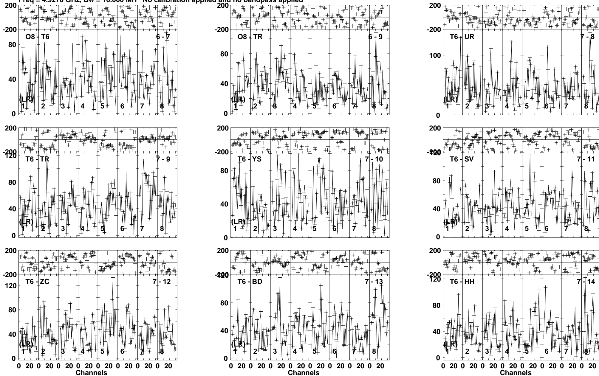
Lower frame: Micro Ampl Jy Top frame: Phas deg Vector averaged cross-power spectrum Baseline: O8 (06) - T6 (07) Timerange: 00/21:33:31 to 00/21:43:29
