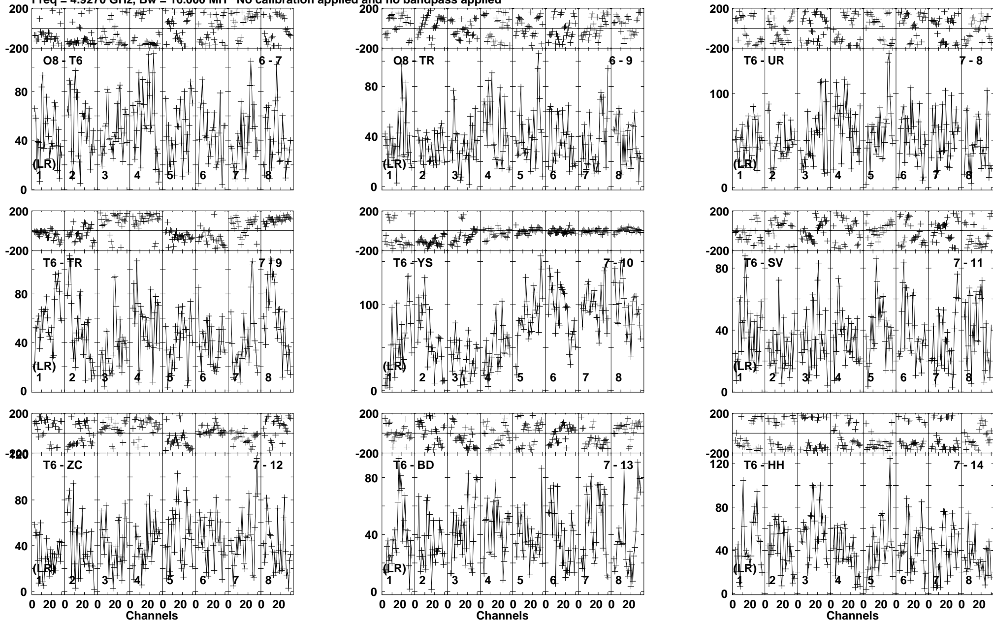
Lower frame: Micro Ampl Jy Top frame: Phas deg Vector averaged cross-power spectrum Baseline: O8 (06) - T6 (07) Timerange: 00/22:06:31 to 00/22:16:29
