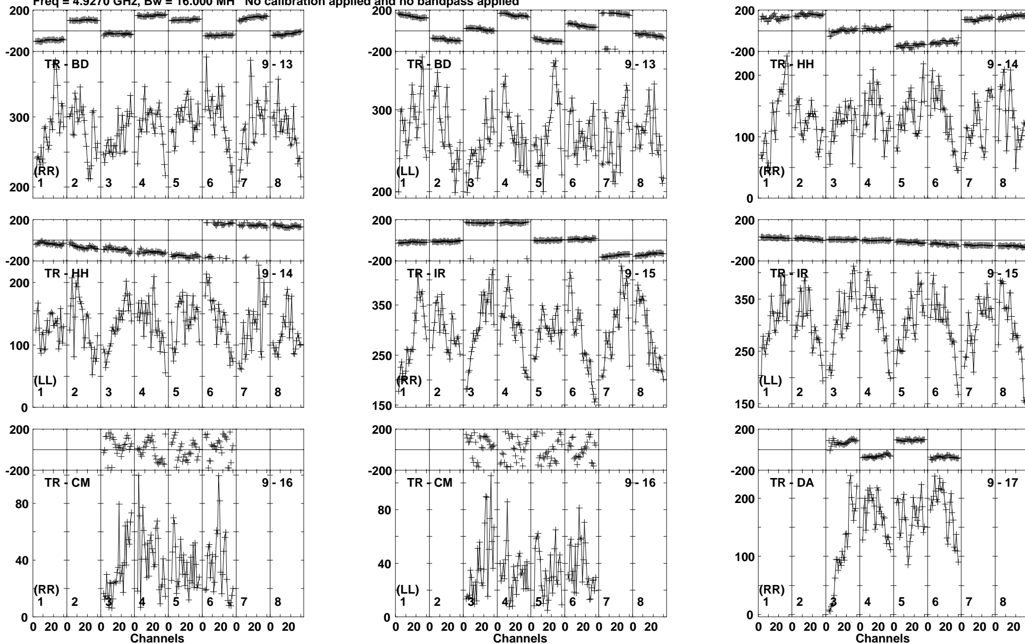
Lower frame: Micro Ampl Jy Top frame: Phas deg Vector averaged cross-power spectrum Baseline: TR (09) - BD (13) Timerange: 00/23:40:01 to 00/23:49:59
