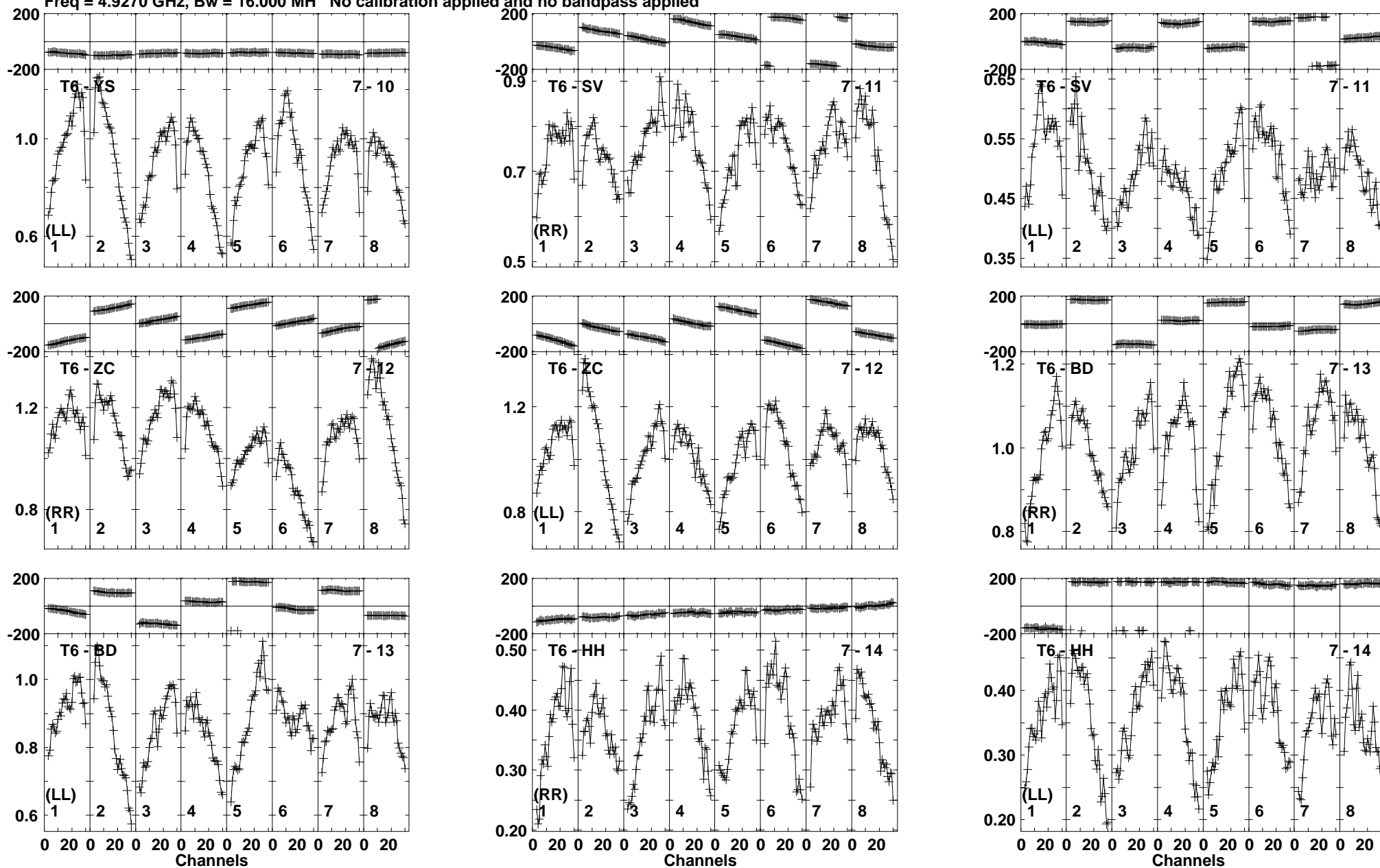
Lower frame: Milli Ampl Jy Top frame: Phas deg Vector averaged cross-power spectrum Baseline: T6 (07) - YS (10) Timerange: 00/20:38:01 to 00/20:47:59
