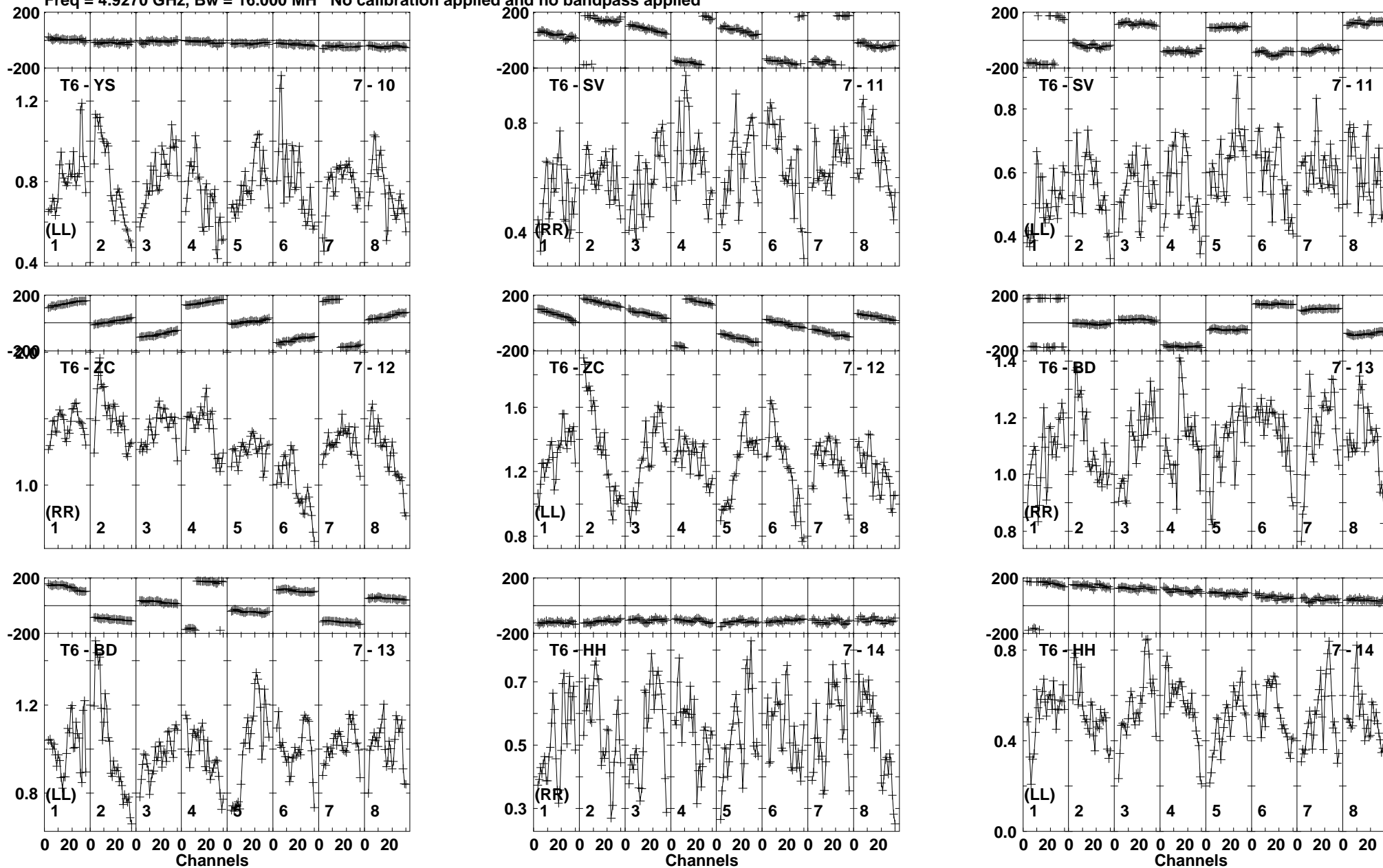
Lower frame: Milli Ampl Jy Top frame: Phas deg Vector averaged cross-power spectrum Baseline: T6 (07) - YS (10) Timerange: 00/22:05:01 to 00/22:05:59
