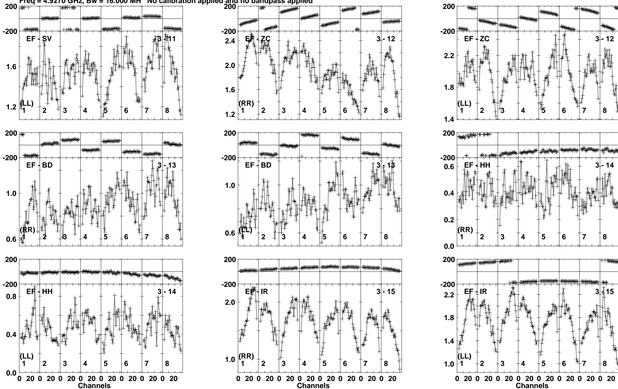
Lower frame: Milli Ampl Jy Top frame: Phas deg Vector averaged cross-power spectrum Baseline: EF (03) - SV (11) Timerange: 00/20:59:01 to 00/20:59:59
