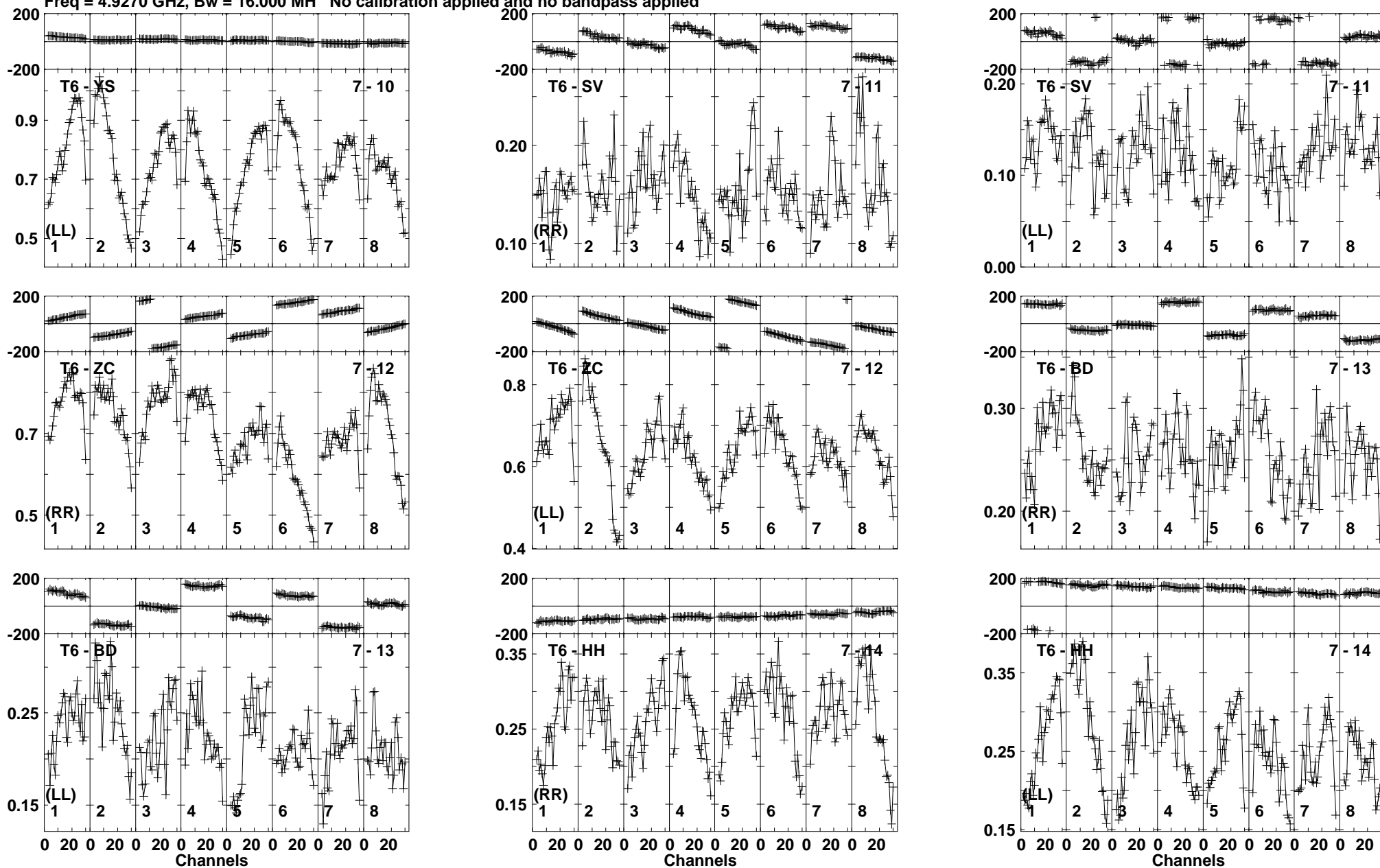
Lower frame: Milli Ampl Jy Top frame: Phas deg Vector averaged cross-power spectrum Baseline: T6 (07) - YS (10) Timerange: 00/21:54:31 to 00/22:04:29
