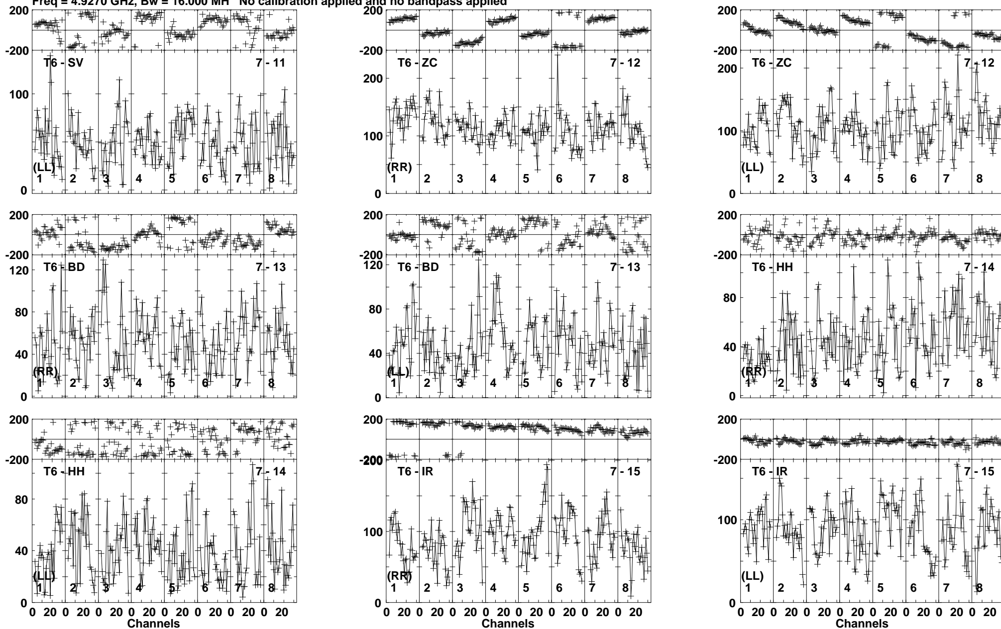
Lower frame: Micro Ampl Jy Top frame: Phas deg Vector averaged cross-power spectrum Baseline: T6 (07) - SV (11) Timerange: 00/22:27:31 to 00/22:37:29
