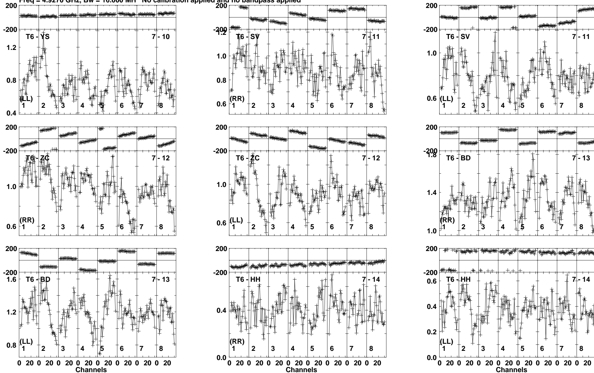
Lower frame: Milli Ampl Jy Top frame: Phas deg Vector averaged cross-power spectrum Baseline: T6 (07) - YS (10) Timerange: 00/18:47:01 to 00/18:47:59
