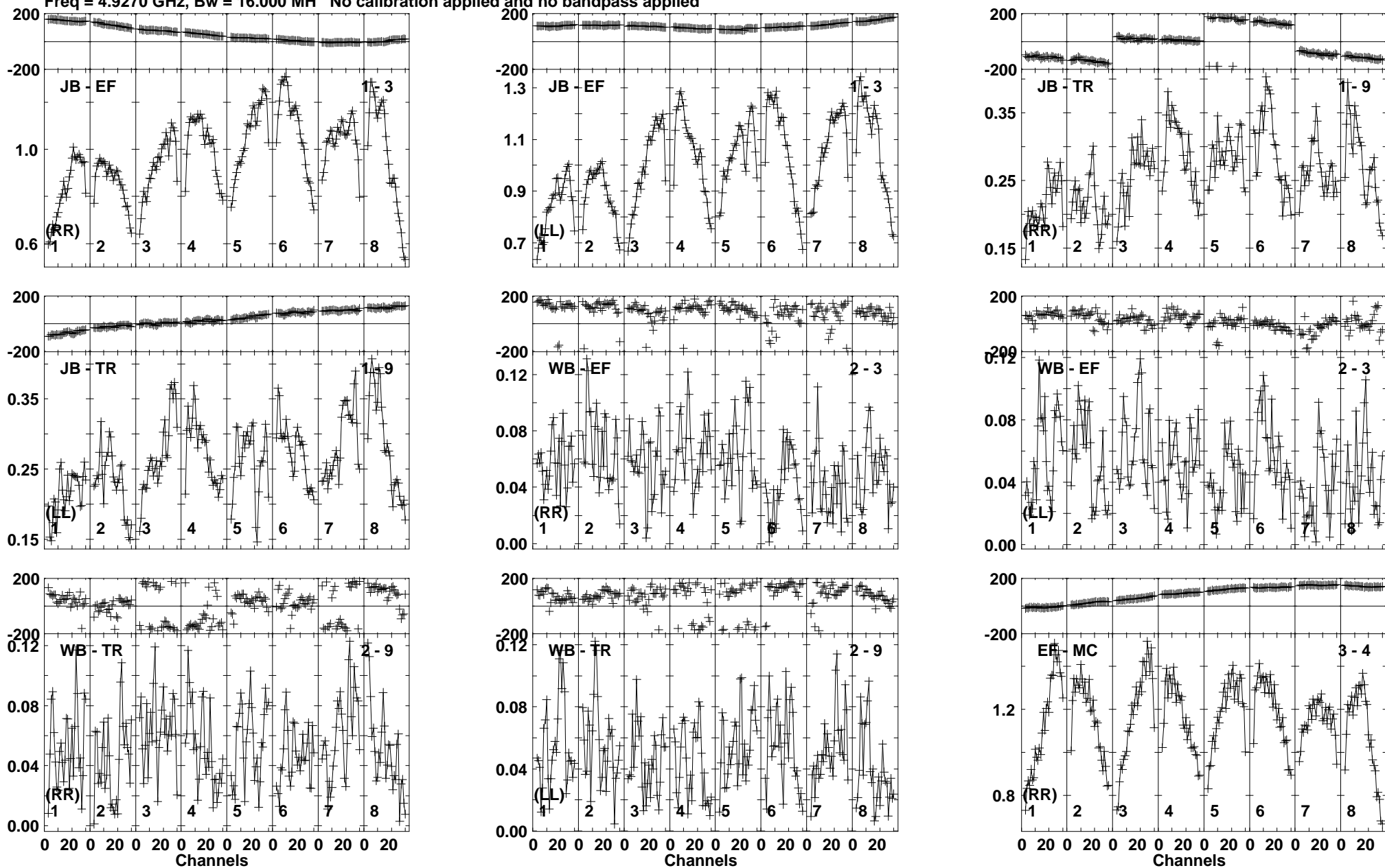
Lower frame: Milli Ampl Jy Top frame: Phas deg Vector averaged cross-power spectrum Baseline: JB (01) - EF (03) Timerange: 01/01:19:01 to 01/01:28:59
