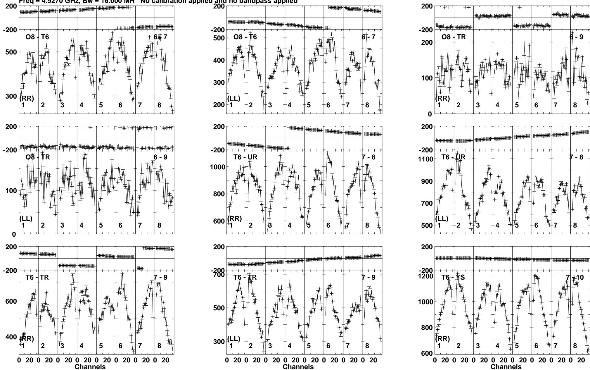
Lower frame: Micro Ampl Jy Top frame: Phas deg Vector averaged cross-power spectrum Baseline: O8 (06) - T6 (07) Timerange: 00/21:00:31 to 00/21:10:29
