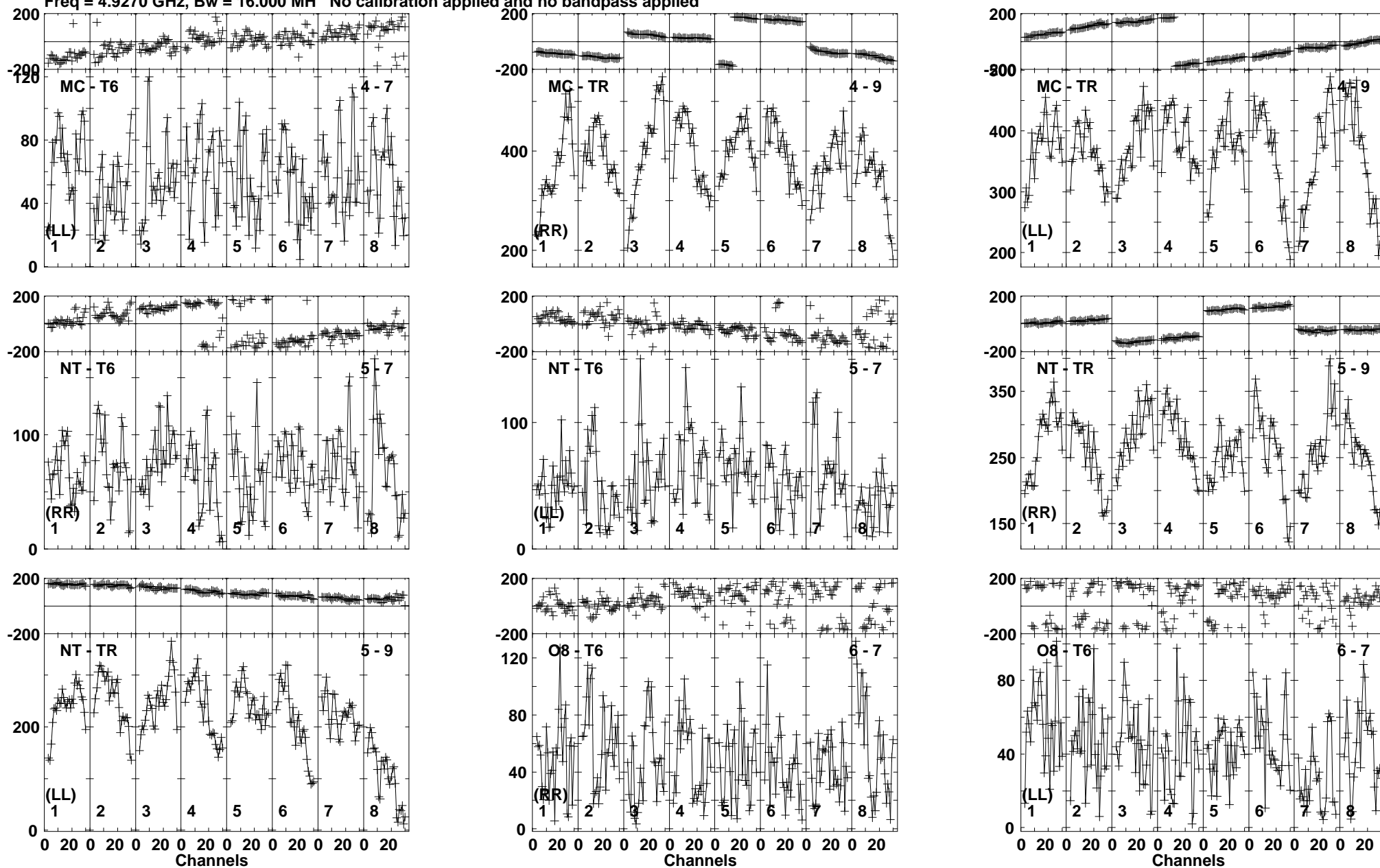
Lower frame: Micro Ampl Jy Top frame: Phas deg Vector averaged cross-power spectrum Baseline: MC (04) - T6 (07) Timerange: 00:22:27:31 to 00:22:37:29
