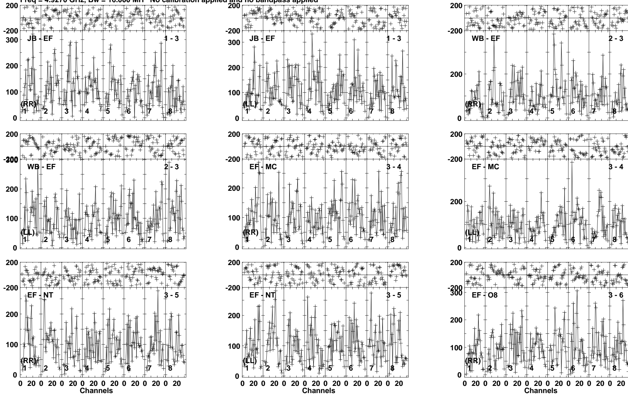
Lower frame: Micro Ampl Jy Top frame: Phas deg Vector averaged cross-power spectrum Baseline: JB (01) - EF (03) Timerange: 00/09:38:57 to 00/09:42:05
