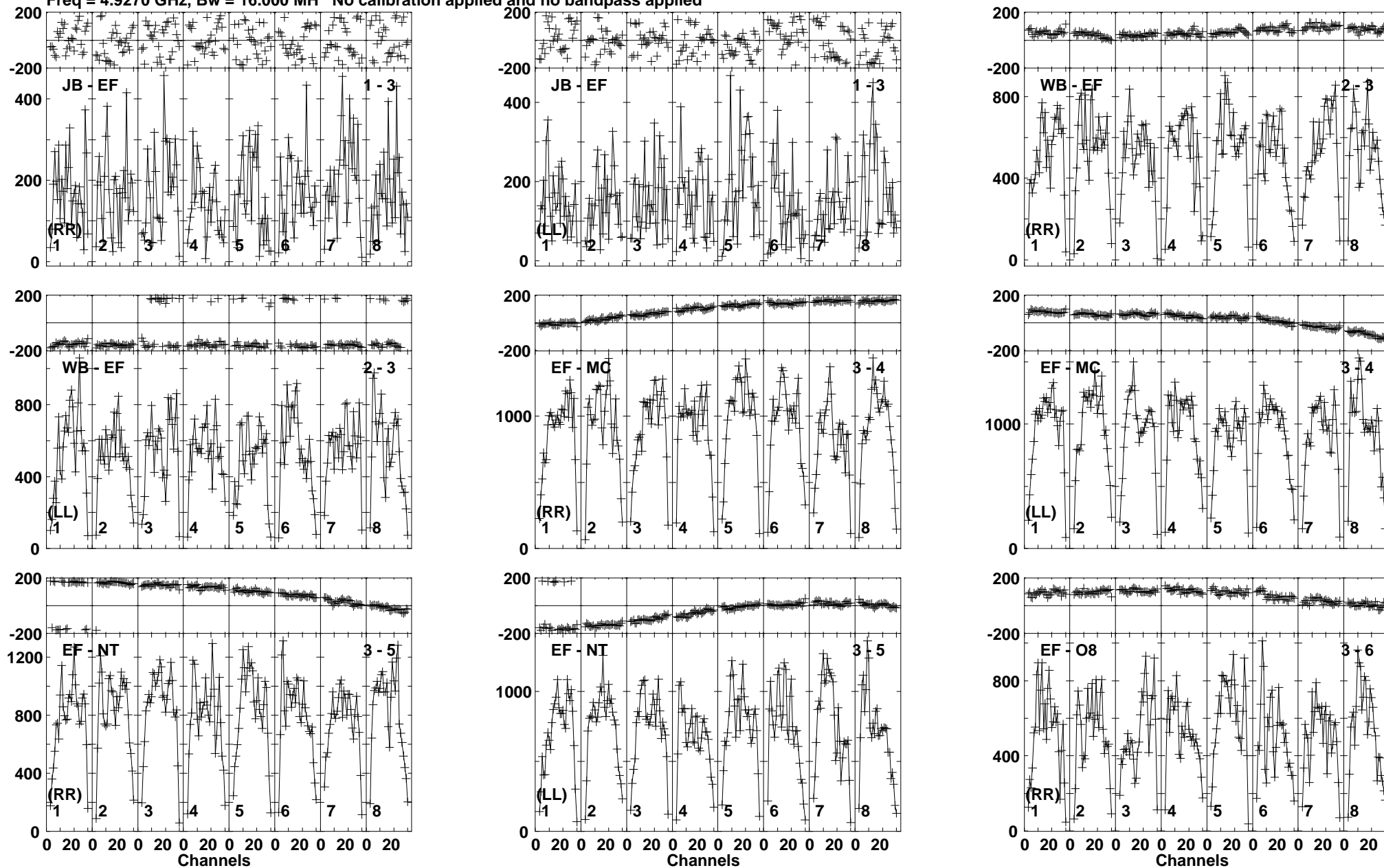
Lower frame: Micro Ampl Jy Top frame: Phas deg Vector averaged cross-power spectrum Baseline: JB (01) - EF (03) Timerange: 00/12:07:47 to 00/12:09:05
