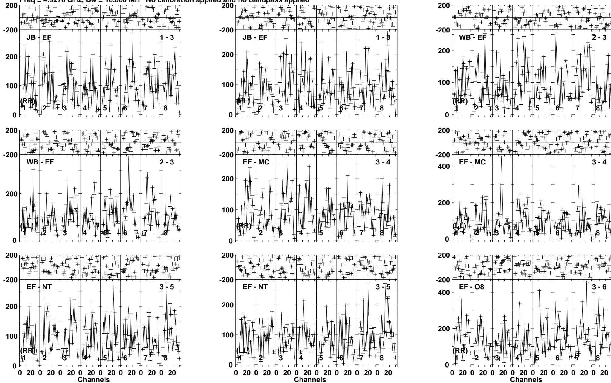
Lower frame: Micro Ampl Jy Top frame: Phas deg Vector averaged cross-power spectrum Baseline: JB (01) - EF (03) Timerange: 00/08:41:07 to 00/08:44:15
