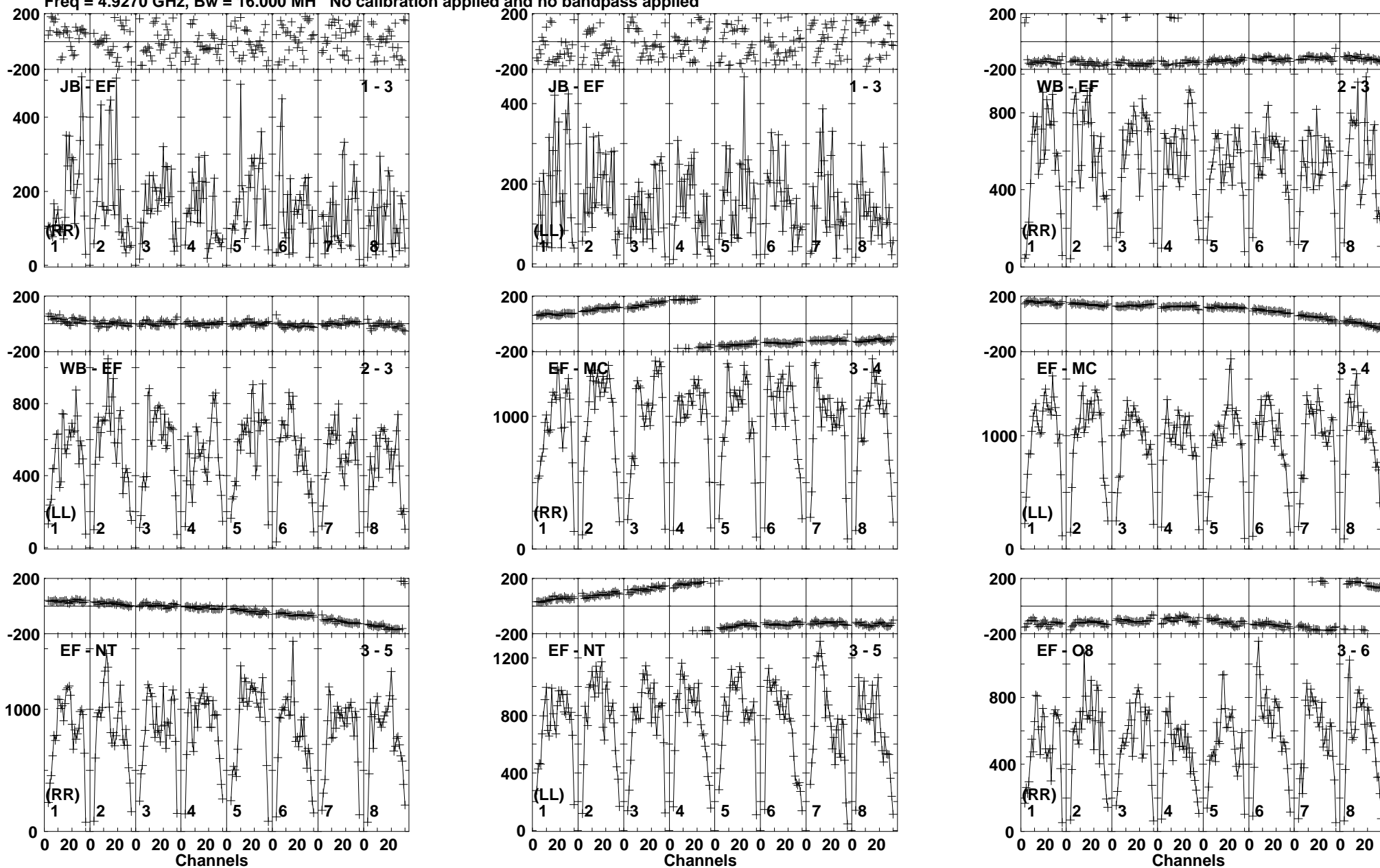
Lower frame: Micro Ampl Jy Top frame: Phas deg Vector averaged cross-power spectrum Baseline: JB (01) - EF (03) Timerange: 00/11:29:47 to 00/11:31:05
