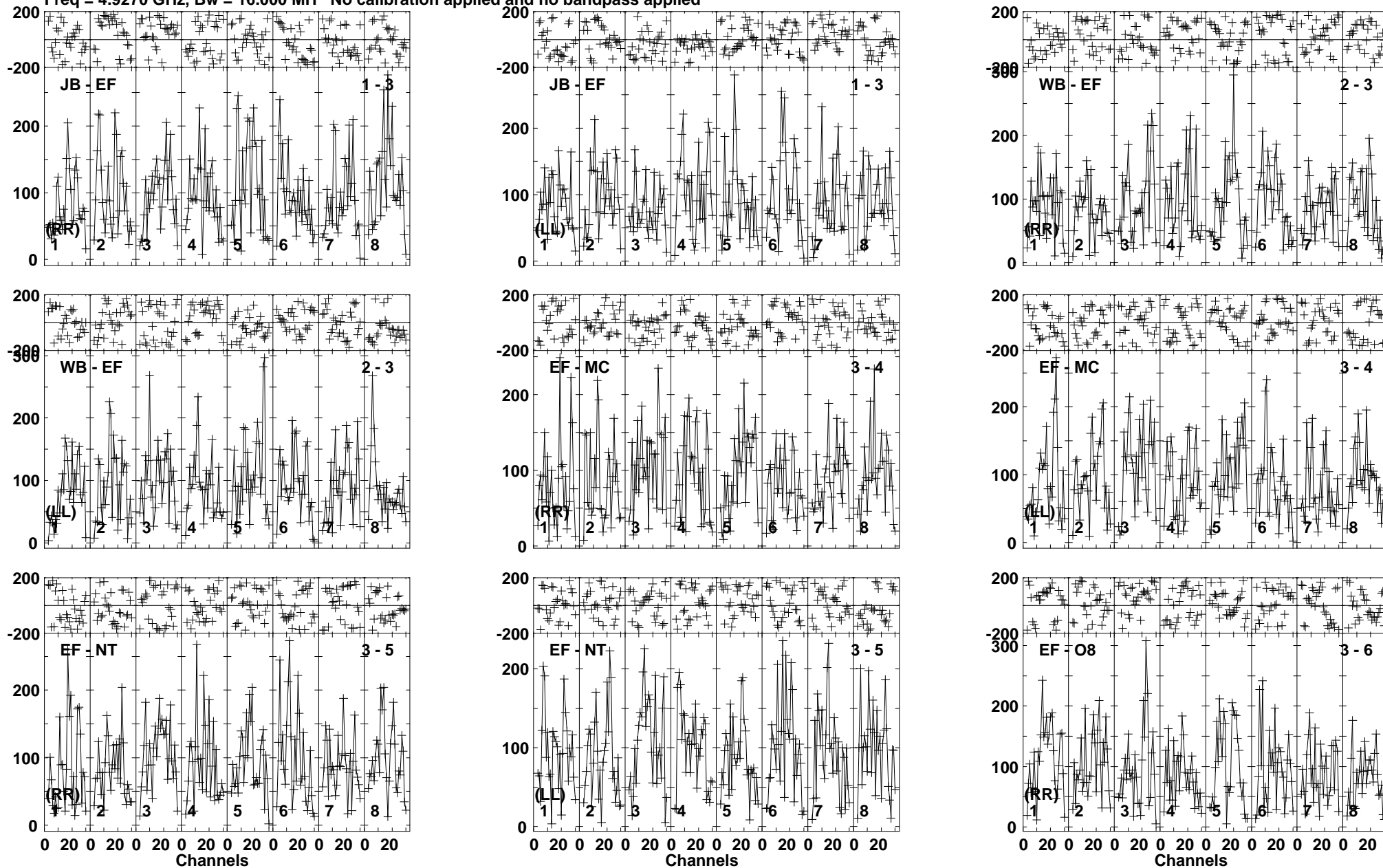
Lower frame: Micro Ampl Jy Top frame: Phas deg Vector averaged cross-power spectrum Baseline: JB (01) - EF (03) Timerange: 00/12:23:37 to 00/12:26:45
