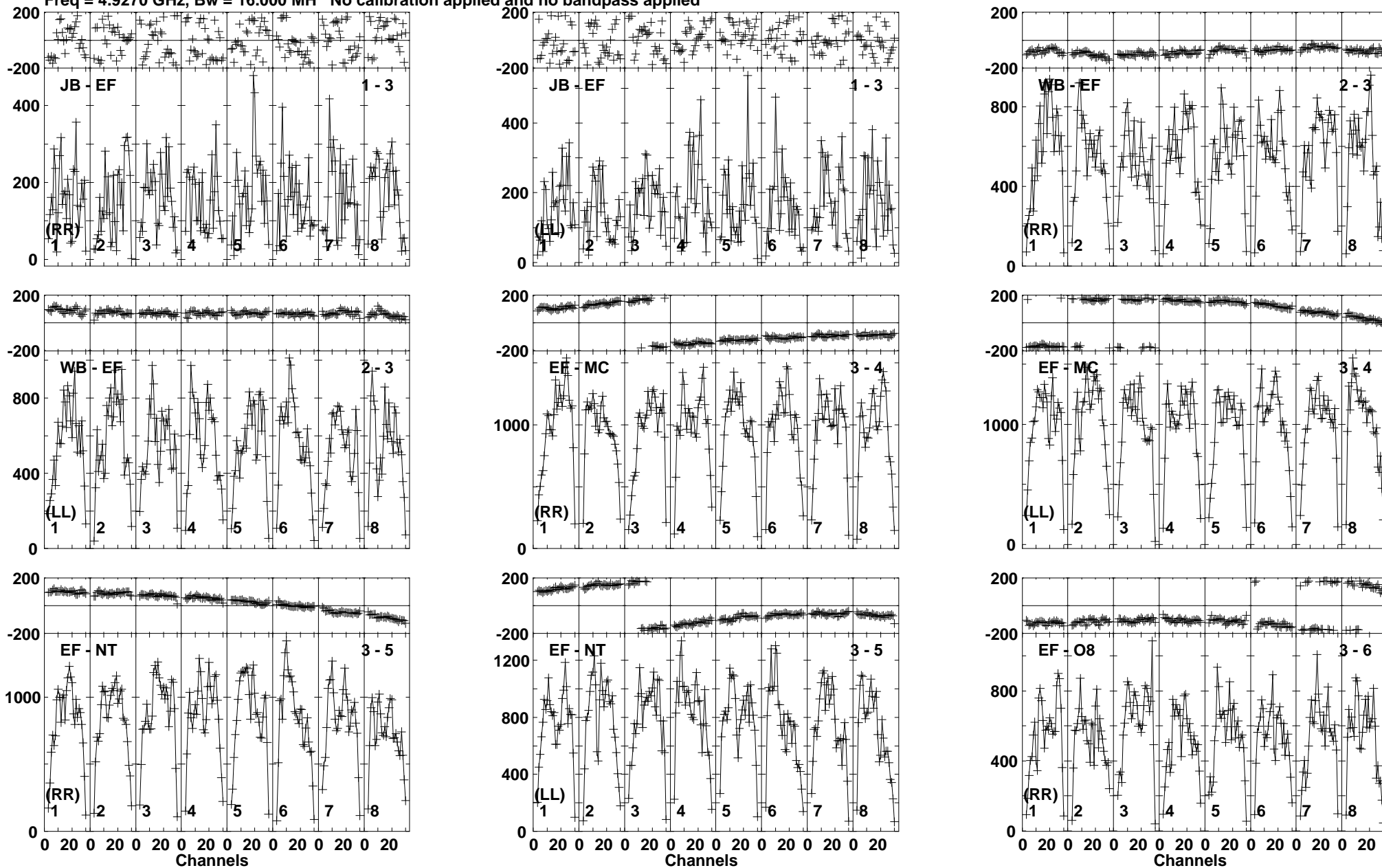
Lower frame: Micro Ampl Jy Top frame: Phas deg Vector averaged cross-power spectrum Baseline: JB (01) - EF (03) Timerange: 00/11:04:27 to 00/11:05:45
