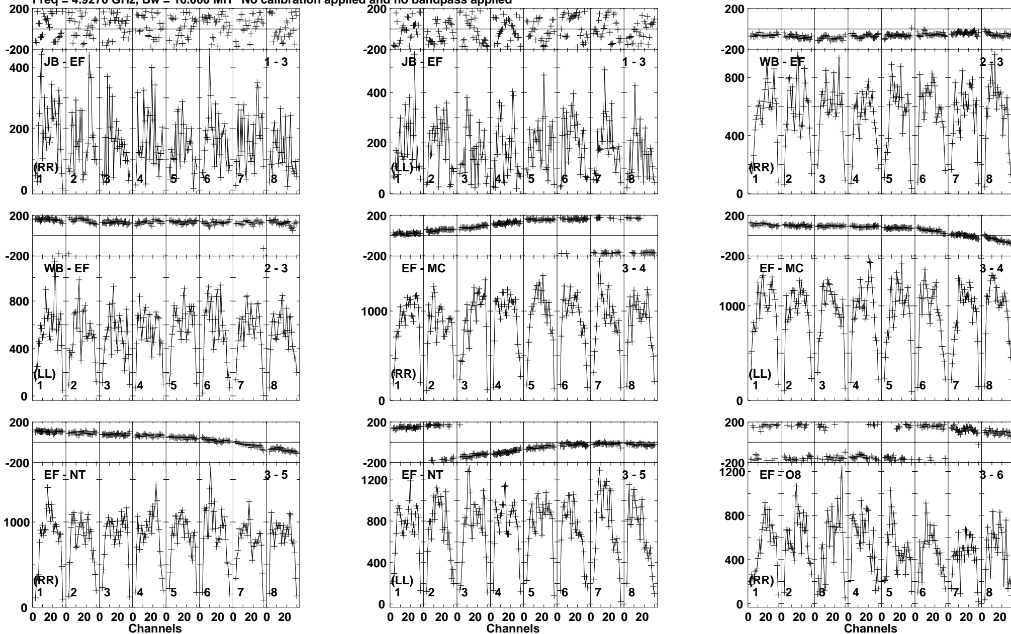
Lower frame: Micro Ampl Jy Top frame: Phas deg Vector averaged cross-power spectrum Baseline: JB (01) - EF (03) Timerange: 00/08:44:17 to 00/08:45:35
