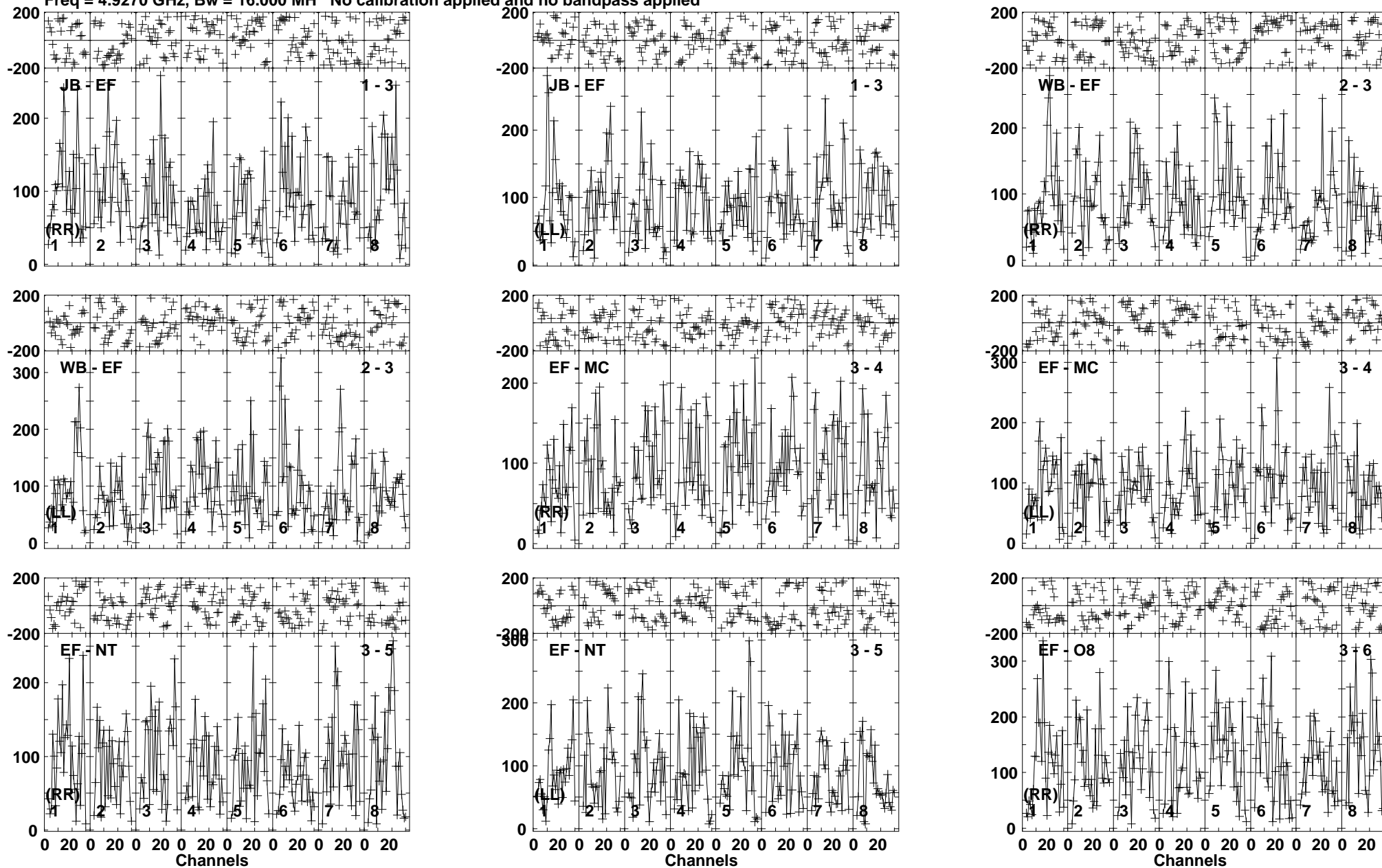
Lower frame: Micro Ampl Jy Top frame: Phas deg Vector averaged cross-power spectrum Baseline: JB (01) - EF (03) Timerange: 00/07:39:56 to 00/07:43:04
