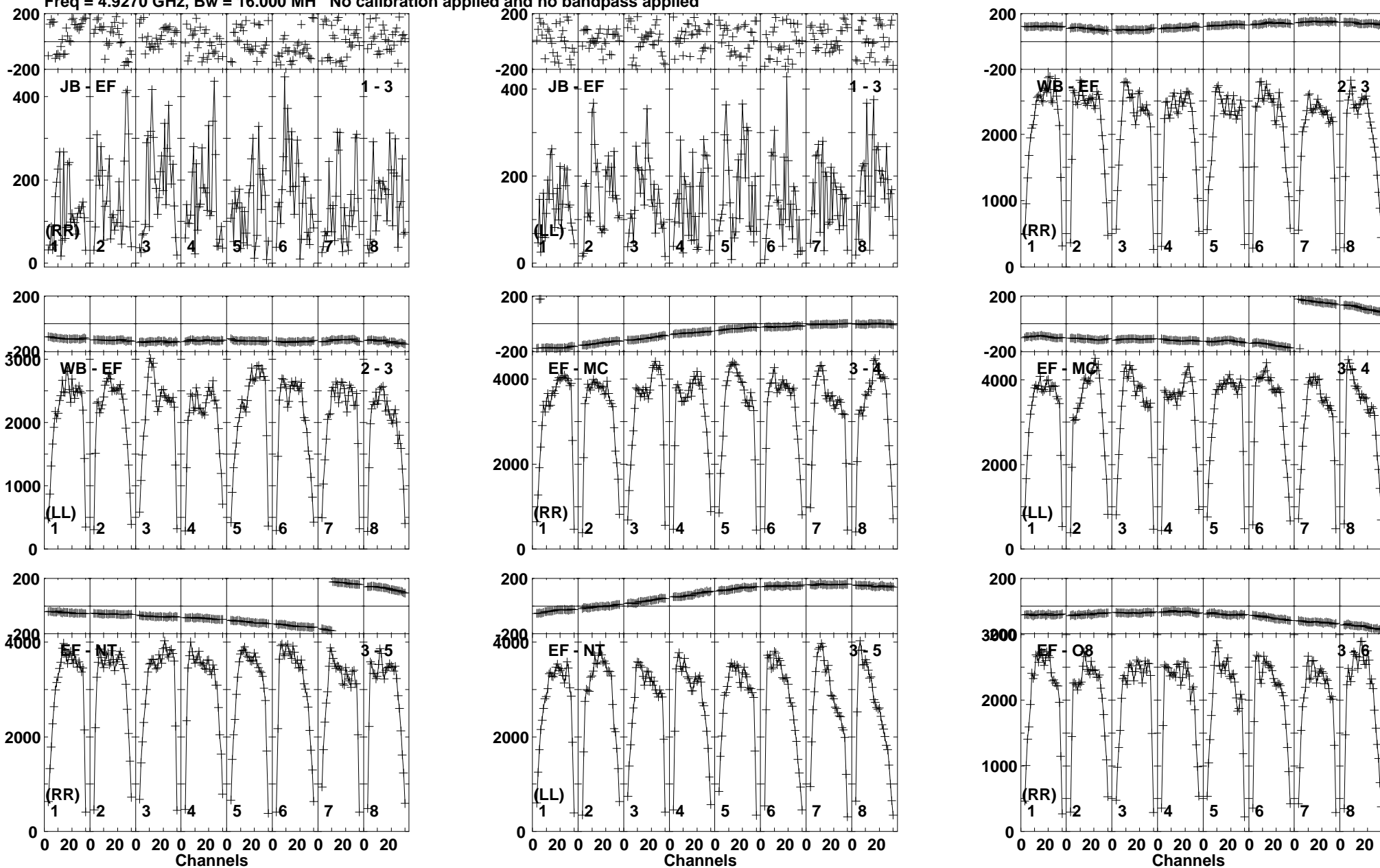
Lower frame: Micro Ampl Jy Top frame: Phas deg Vector averaged cross-power spectrum Baseline: JB (01) - EF (03) Timerange: 00/12:47:47 to 00/12:48:55
