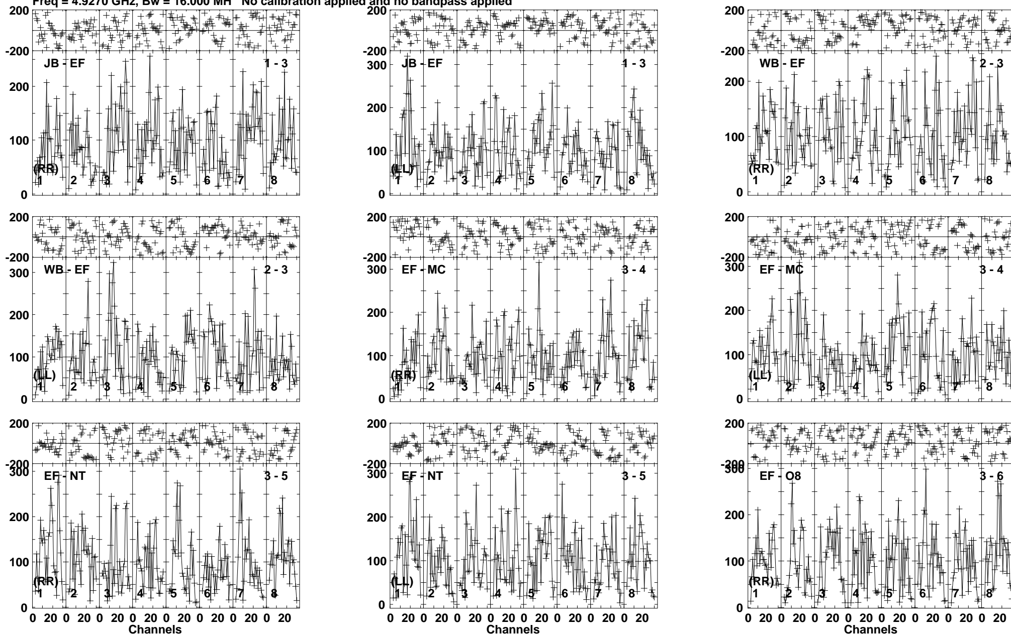
Lower frame: Micro Ampl Jy Top frame: Phas deg Vector averaged cross-power spectrum Baseline: JB (01) - EF (03) Timerange: 00/11:32:57 to 00/11:36:05
