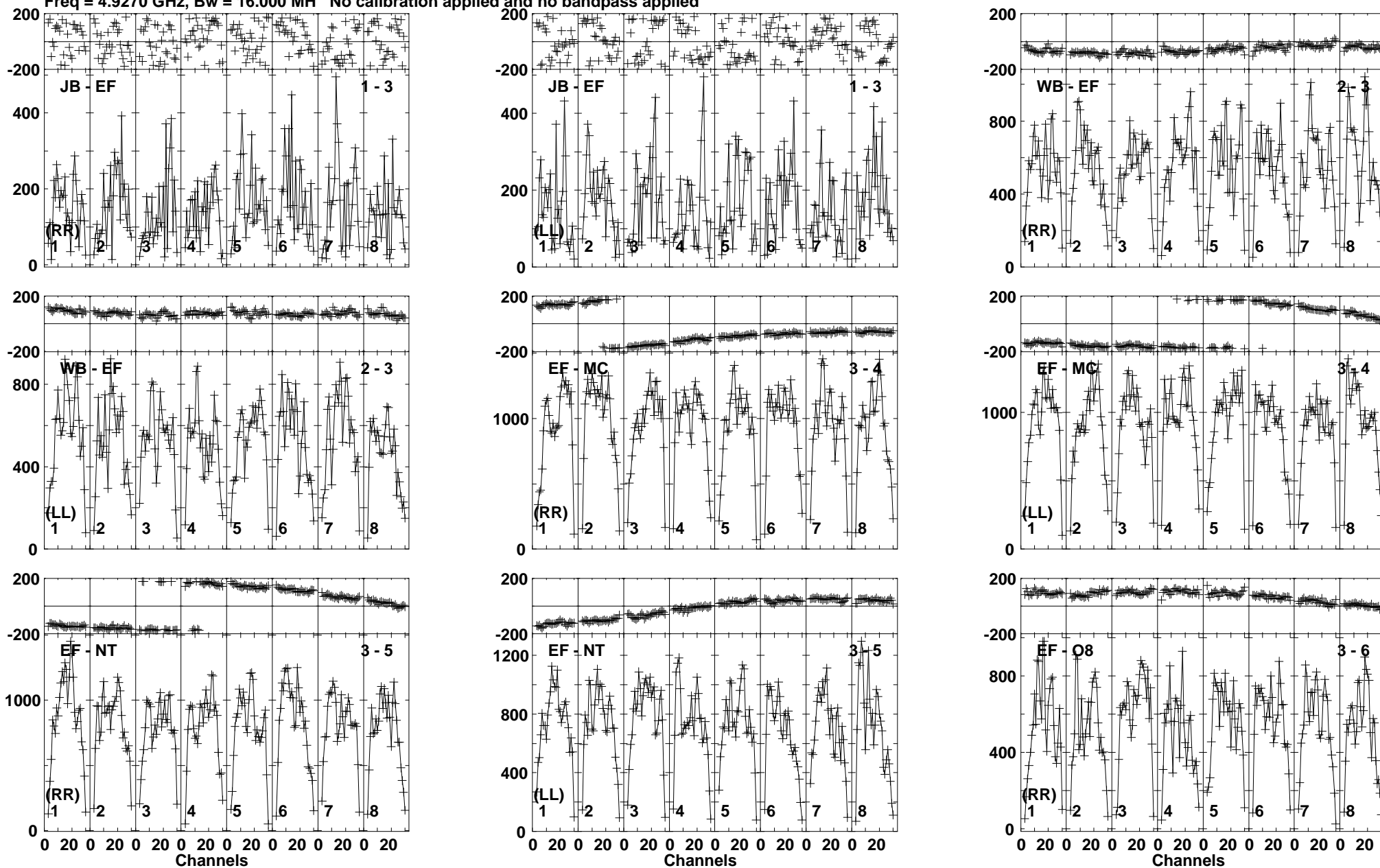
Lower frame: Micro Ampl Jy Top frame: Phas deg Vector averaged cross-power spectrum Baseline: JB (01) - EF (03) Timerange: 00/12:14:07 to 00/12:15:25
