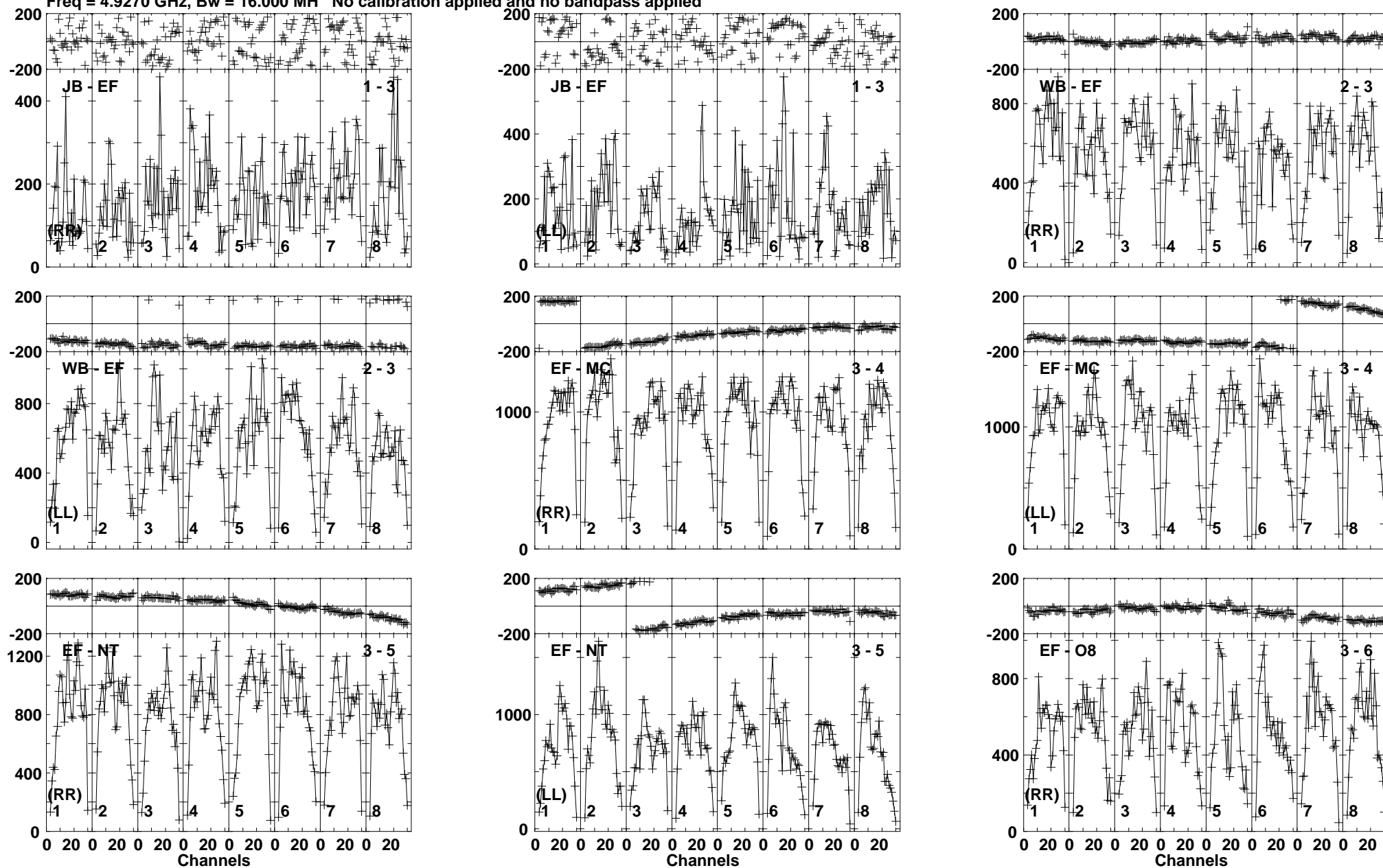
Lower frame: Micro Ampl Jy Top frame: Phas deg Vector averaged cross-power spectrum Baseline: JB (01) - EF (03) Timerange: 00/09:23:07 to 00/09:24:25
