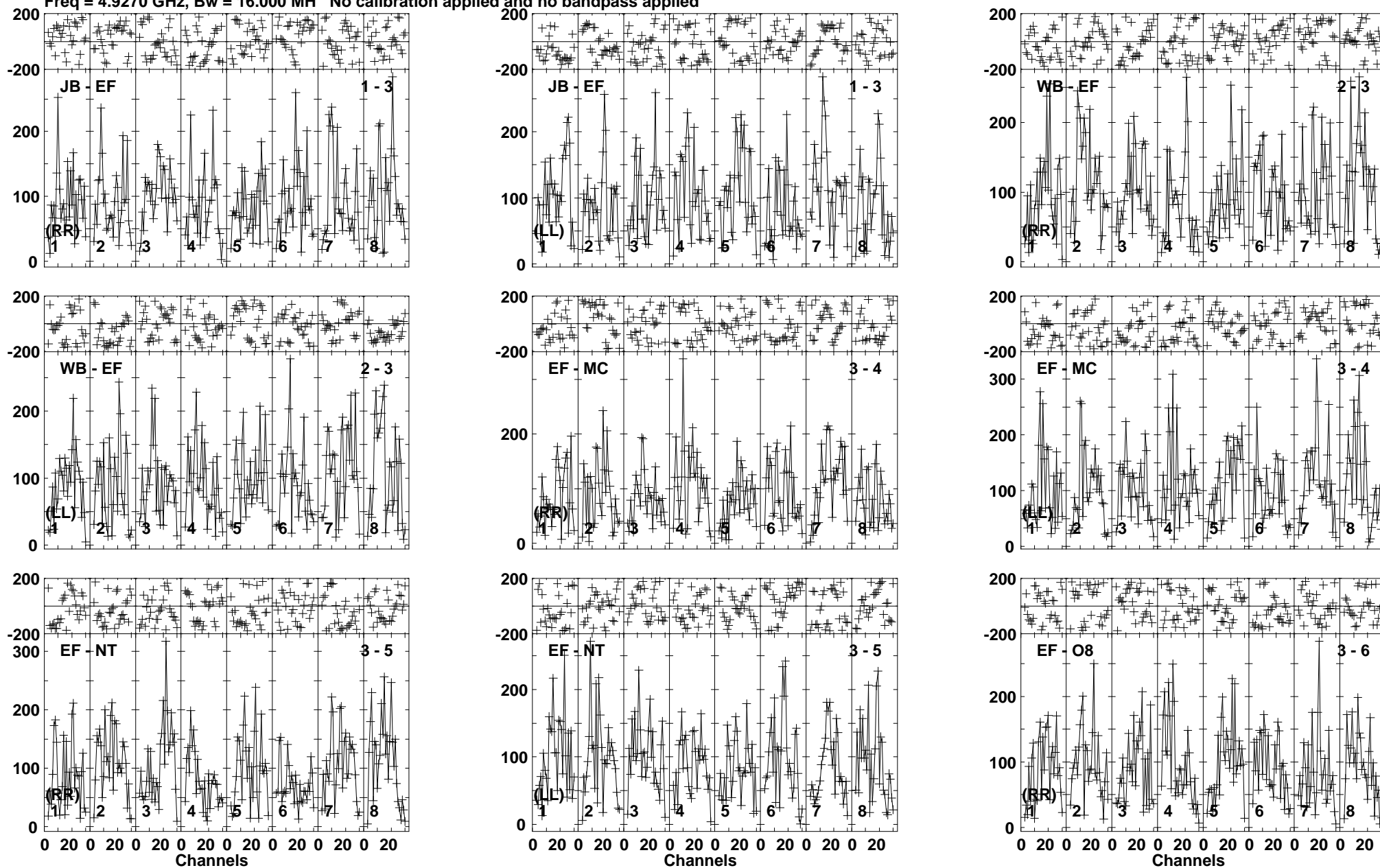
Lower frame: Micro Ampl Jy Top frame: Phas deg Vector averaged cross-power spectrum Baseline: JB (01) - EF (03) Timerange: 00/11:58:17 to 00/12:01:25
