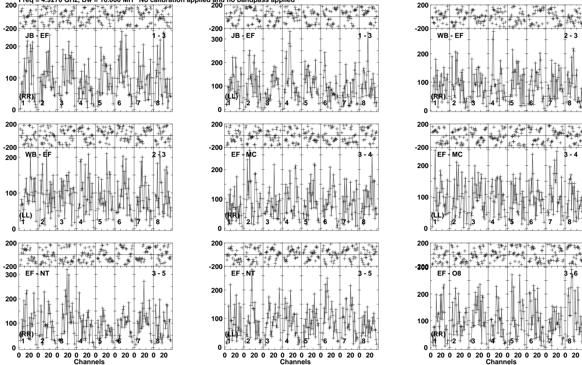
Lower frame: Micro Ampl Jy Top frame: Phas deg Vector averaged cross-power spectrum Baseline: JB (01) - EF (03) Timerange: 00/10:35:57 to 00/10:39:05
