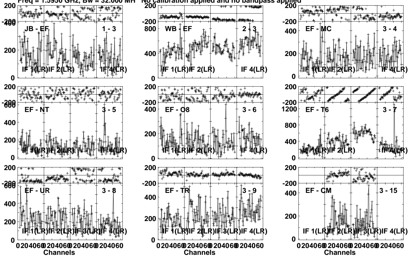
Lower frame: Micro Ampl Jy Top frame: Phas deg Vector averaged cross-power spectrum Several baselines displayed Timerange: 01/04:58:51 to 01/04:59:59
