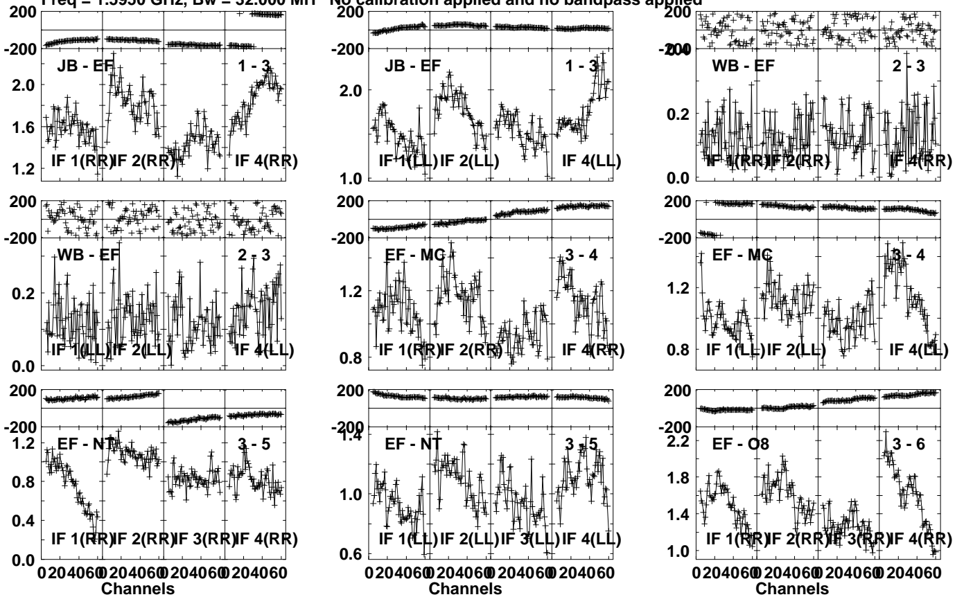
Lower frame: Milli Ampl Jy Top frame: Phas deg Vector averaged cross-power spectrum Several baselines displayed Timerange: 01/01:59:11 to 01/02:00:19
