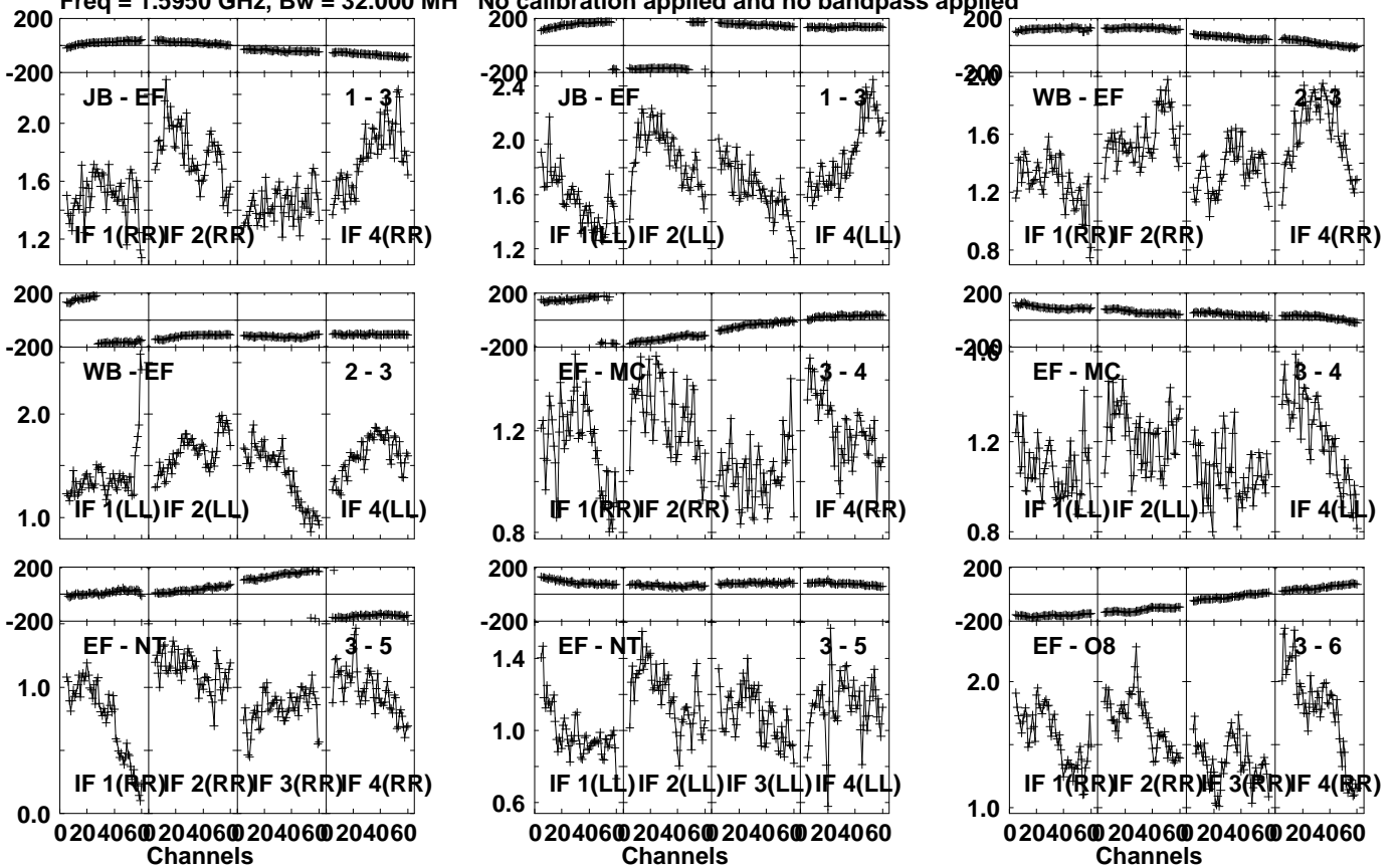
Lower frame: Milli Ampl Jy Top frame: Phas deg Vector averaged cross-power spectrum Several baselines displayed Timerange: 01/04:58:51 to 01/04:59:59
