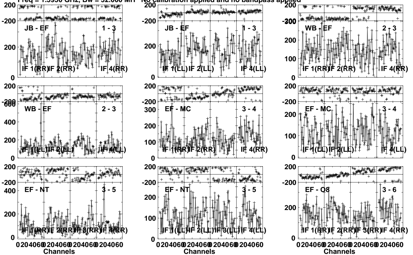
Lower frame: Micro Ampl Jy Top frame: Phas deg Vector averaged cross-power spectrum Several baselines displayed Timerange: 01/04:07:21 to 01/04:10:49
