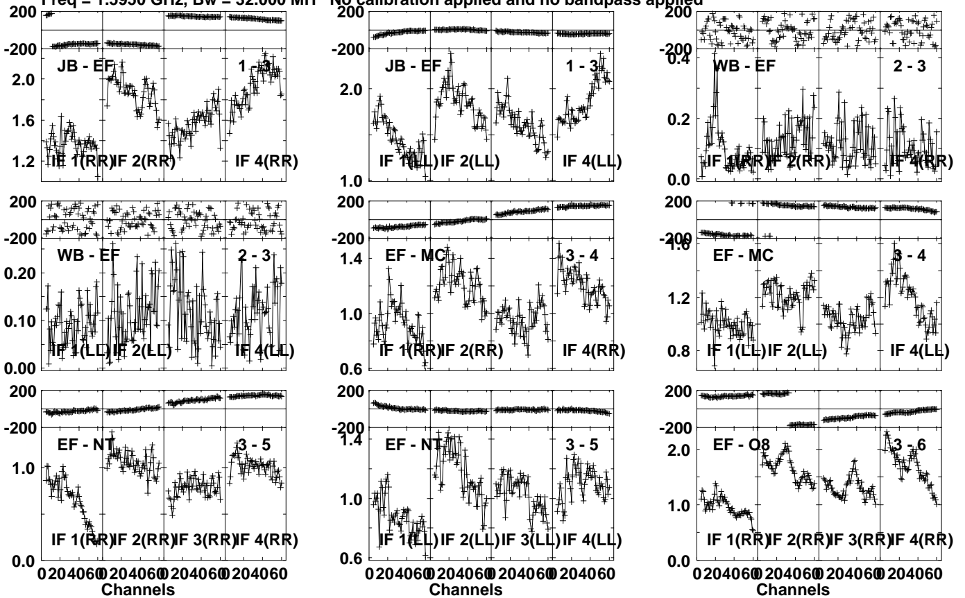
Lower frame: Milli Ampl Jy Top frame: Phas deg Vector averaged cross-power spectrum Several baselines displayed Timerange: 01/03:11:16 to 01/03:12:44
