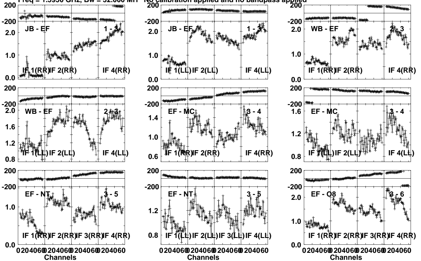
Lower frame: Milli Ampl Jy Top frame: Phas deg Vector averaged cross-power spectrum Several baselines displayed Timerange: 01/04:27:41 to 01/04:29:09
