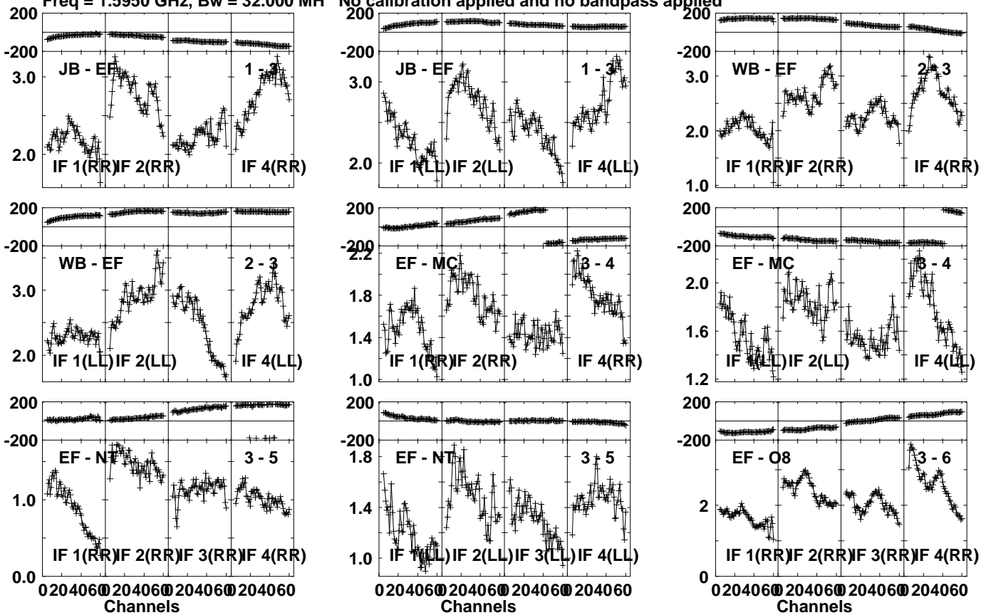
Lower frame: Milli Ampl Jy Top frame: Phas deg Vector averaged cross-power spectrum Several baselines displayed Timerange: 01/00:24:51 to 01/00:26:19
