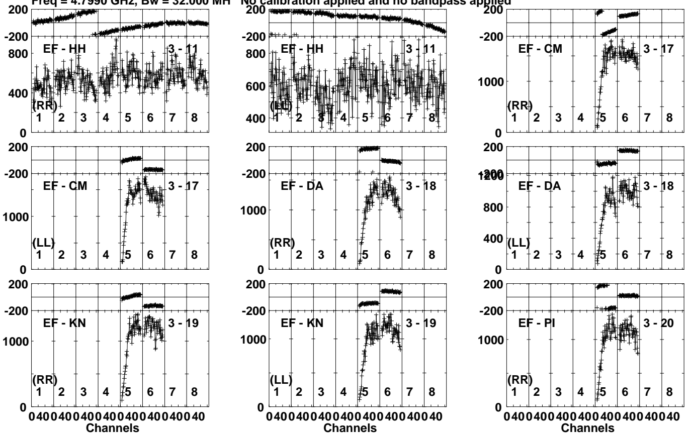
Lower frame: Micro Ampl Jy Top frame: Phas deg Vector averaged cross-power spectrum Several baselines displayed Timerange: 00/23:33:11 to 00/23:35:09
