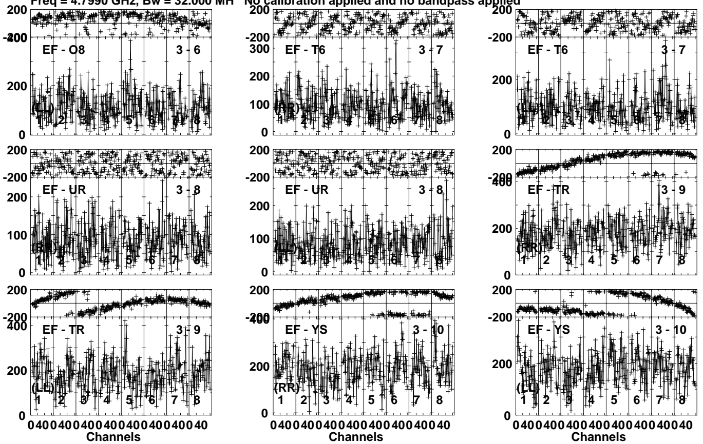
Lower frame: Micro Ampl Jy Top frame: Phas deg Vector averaged cross-power spectrum Several baselines displayed Timerange: 01/04:10:06 to 01/04:13:34
