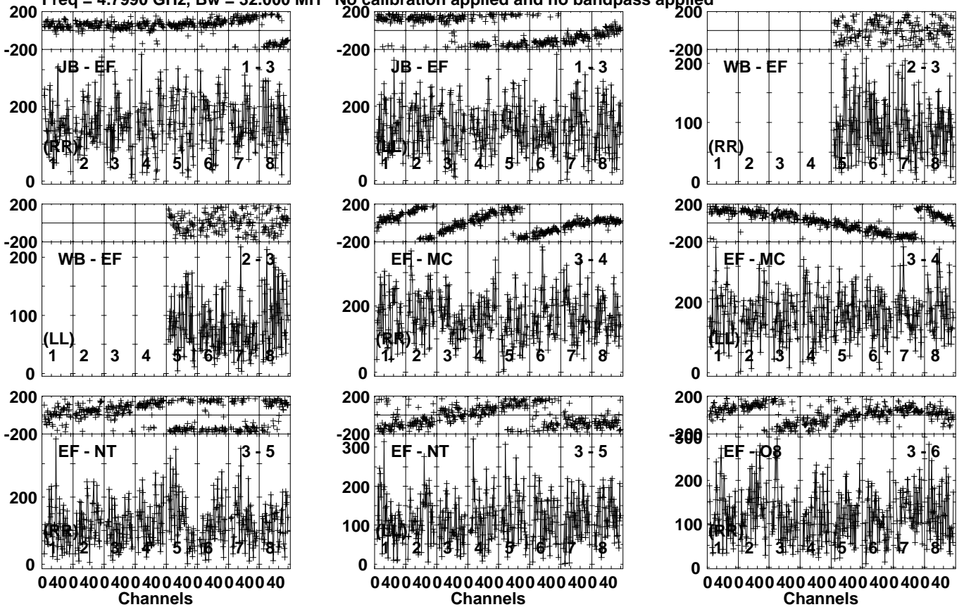
Lower frame: Micro Ampl Jy Top frame: Phas deg Vector averaged cross-power spectrum Several baselines displayed Timerange: 01/02:25:56 to 01/02:29:24
