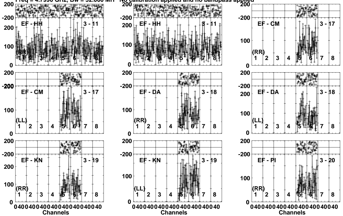
Lower frame: Micro Ampl Jy Top frame: Phas deg Vector averaged cross-power spectrum Several baselines displayed Timerange: 00/23:24:11 to 00/23:27:39
