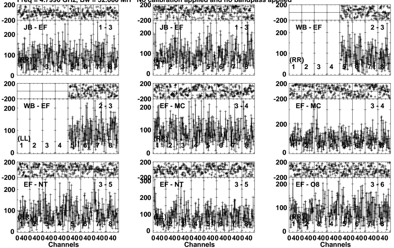
Lower frame: Micro Ampl Jy Top frame: Phas deg Vector averaged cross-power spectrum Several baselines displayed Timerange: 01/00:03:11 to 01/00:06:39
