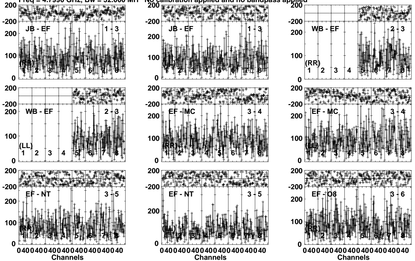
Lower frame: Micro Ampl Jy Top frame: Phas deg Vector averaged cross-power spectrum Several baselines displayed Timerange: 01/00:24:11 to 01/00:27:39
