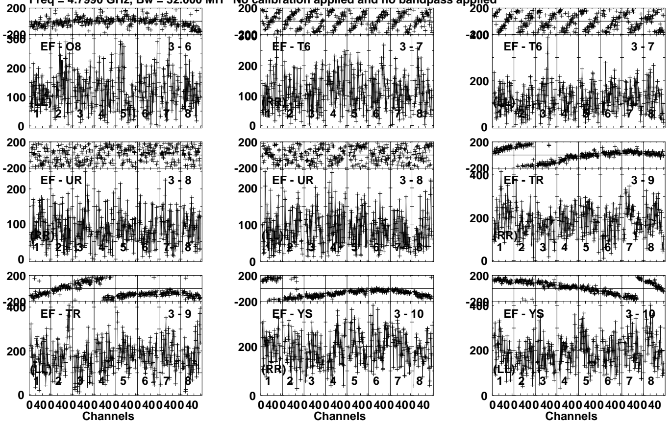
Lower frame: Micro Ampl Jy Top frame: Phas deg Vector averaged cross-power spectrum Several baselines displayed Timerange: 01/03:04:36 to 01/03:08:04
