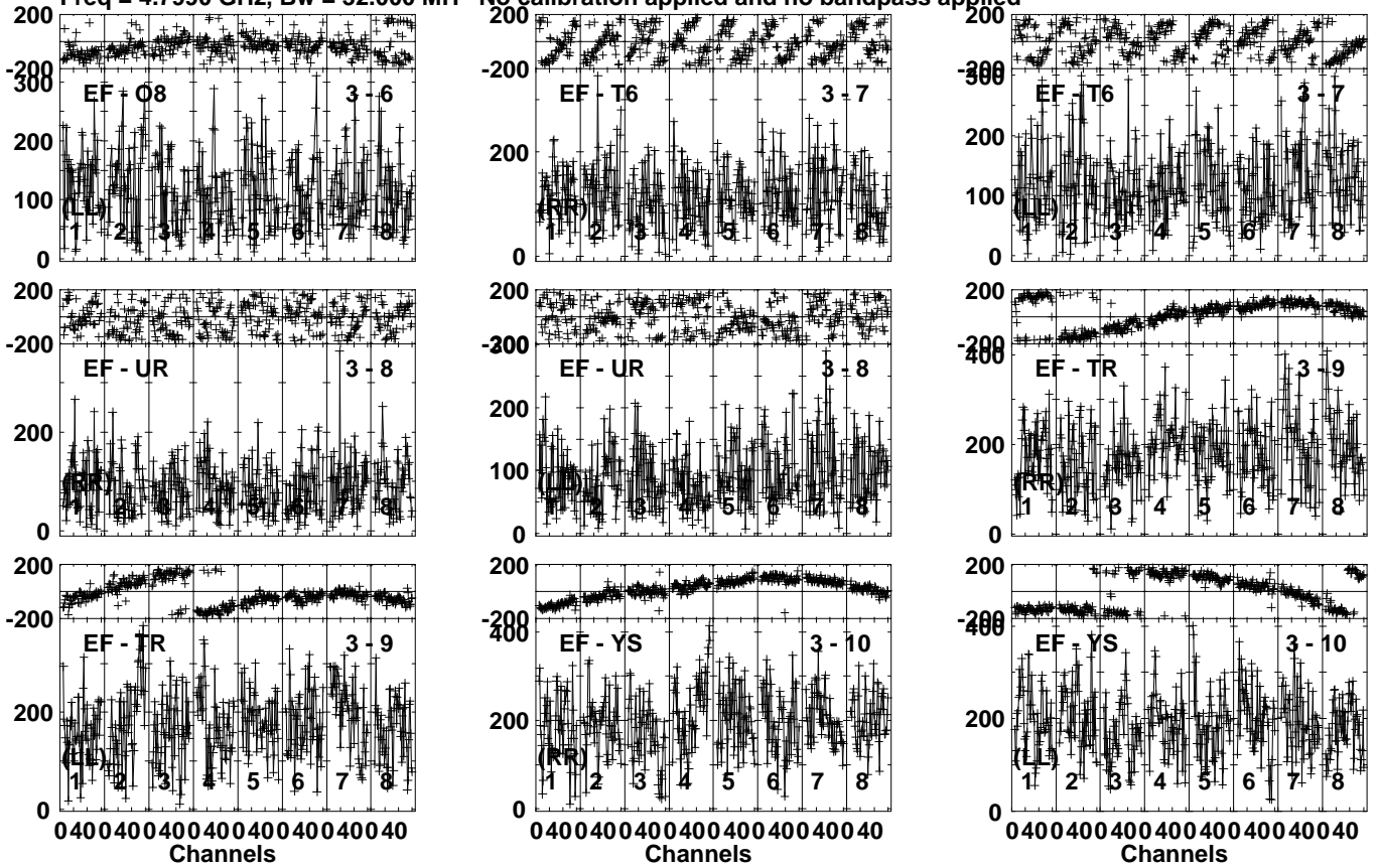
Lower frame: Micro Ampl Jy Top frame: Phas deg Vector averaged cross-power spectrum Several baselines displayed Timerange: 01/03:26:26 to 01/03:29:54
