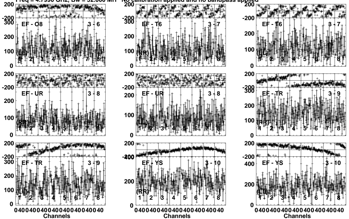
Lower frame: Micro Ampl Jy Top frame: Phas deg Vector averaged cross-power spectrum Several baselines displayed Timerange: 01/03:53:16 to 01/03:56:44
