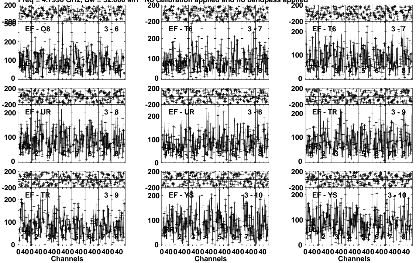
Lower frame: Micro Ampl Jy Top frame: Phas deg Vector averaged cross-power spectrum Several baselines displayed Timerange: 00/22:42:11 to 00/22:45:39
