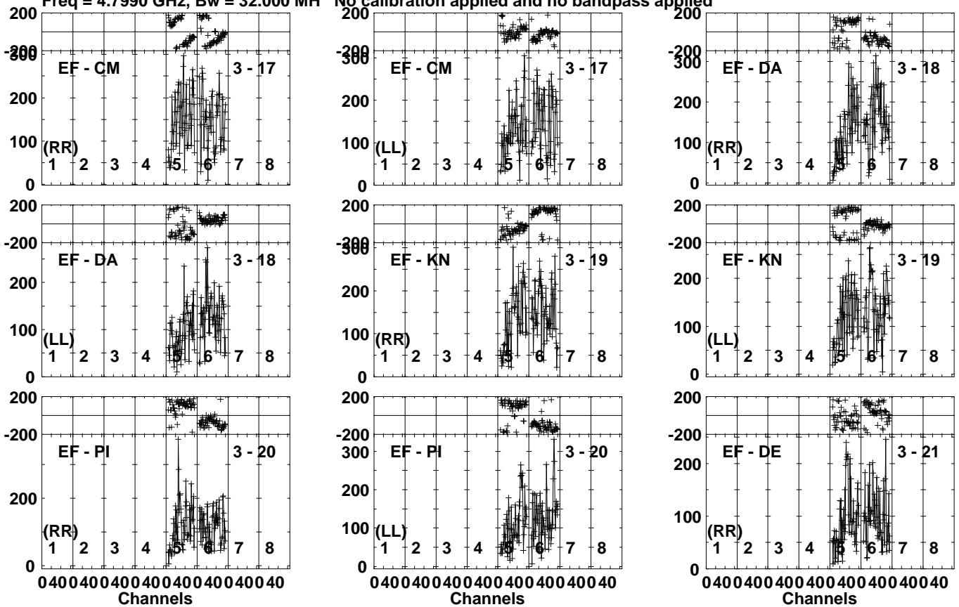
Lower frame: Micro Ampl Jy Top frame: Phas deg Vector averaged cross-power spectrum Several baselines displayed Timerange: 01/04:04:11 to 01/04:07:39
