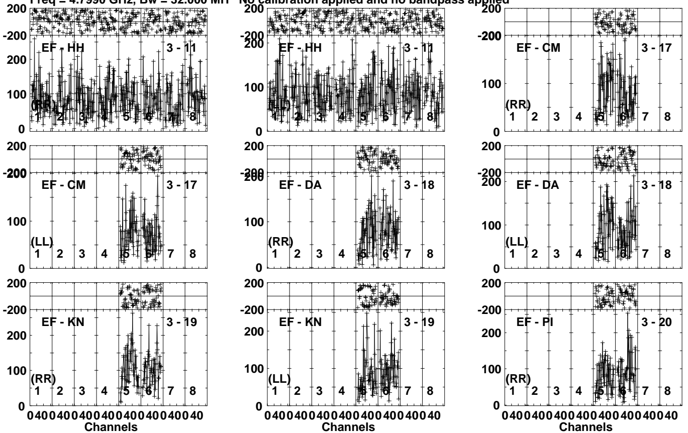
Lower frame: Micro Ampl Jy Top frame: Phas deg Vector averaged cross-power spectrum Several baselines displayed Timerange: 00/23:46:51 to 00/23:50:19
