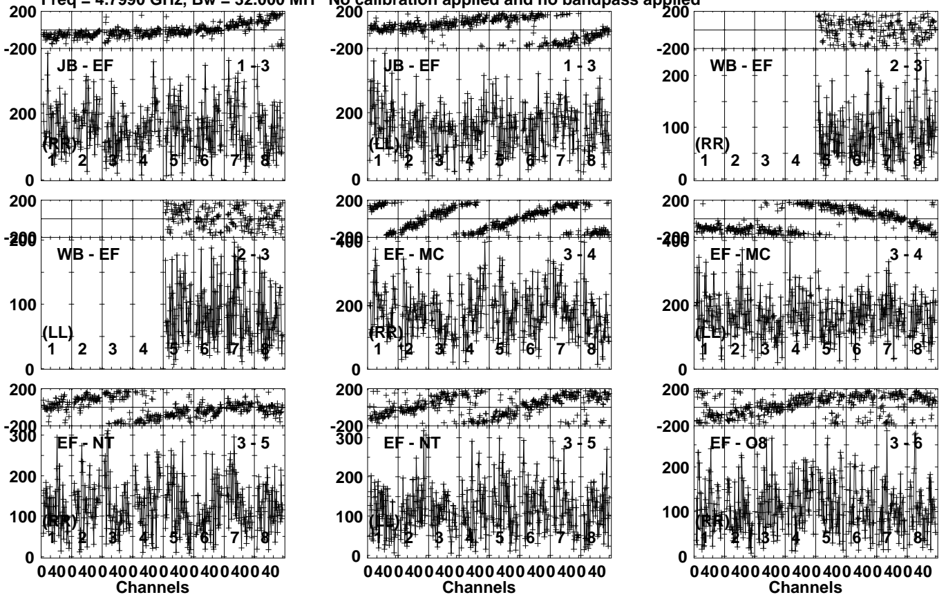
Lower frame: Micro Ampl Jy Top frame: Phas deg Vector averaged cross-power spectrum Several baselines displayed Timerange: 01/04:24:41 to 01/04:27:53
