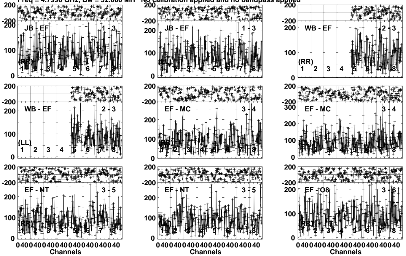
Lower frame: Micro Ampl Jy Top frame: Phas deg Vector averaged cross-power spectrum Several baselines displayed Timerange: 00/23:13:41 to 00/23:17:09
