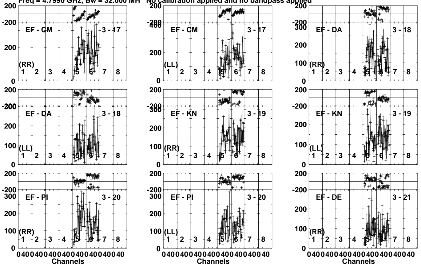
Lower frame: Micro Ampl Jy Top frame: Phas deg Vector averaged cross-power spectrum Several baselines displayed Timerange: 01/04:15:06 to 01/04:18:14
