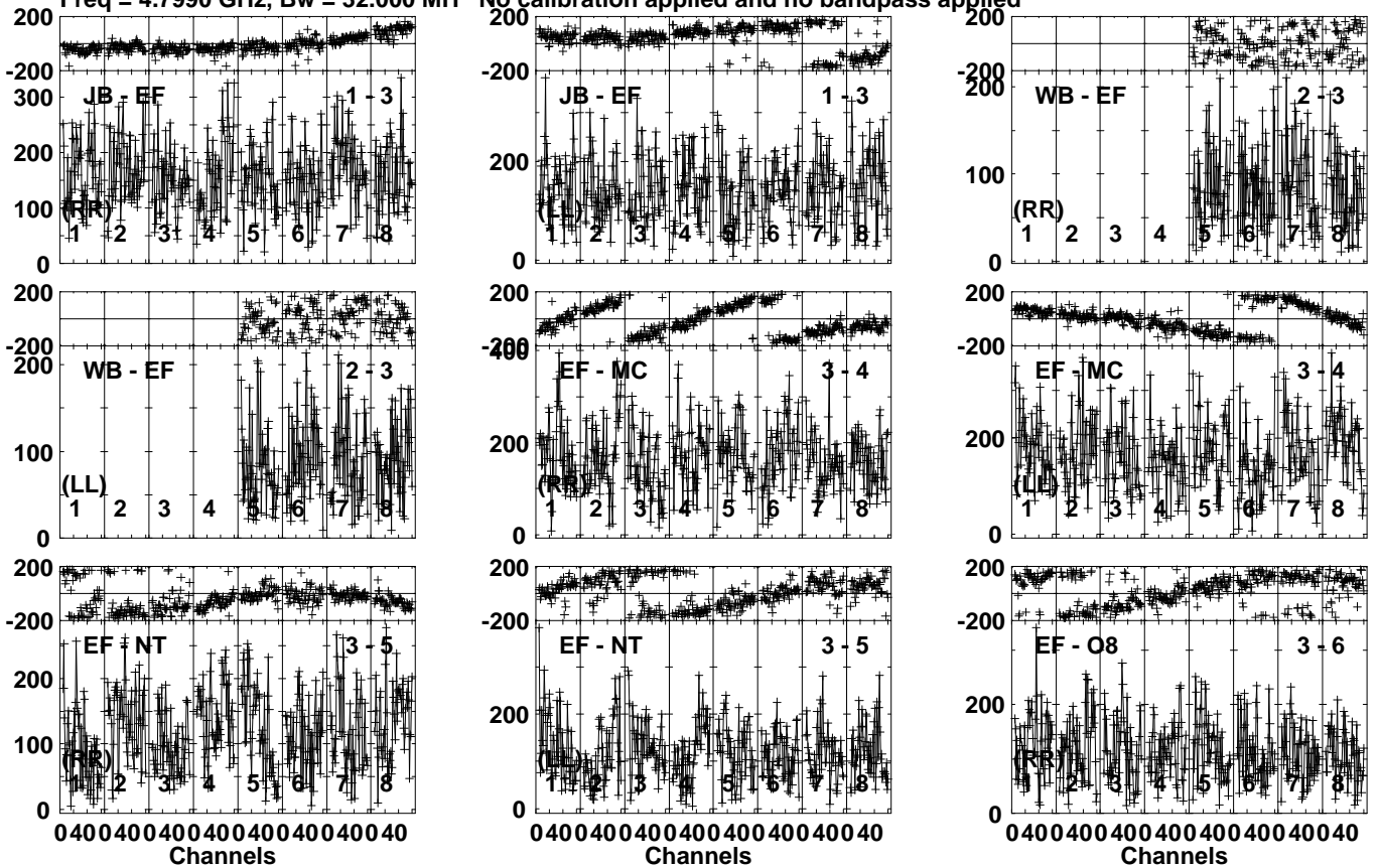
Lower frame: Micro Ampl Jy Top frame: Phas deg Vector averaged cross-power spectrum Several baselines displayed Timerange: 01/02:20:56 to 01/02:24:24
