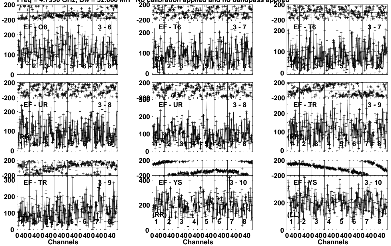
Lower frame: Micro Ampl Jy Top frame: Phas deg Vector averaged cross-power spectrum Several baselines displayed Timerange: 01/02:10:01 to 01/02:13:29
