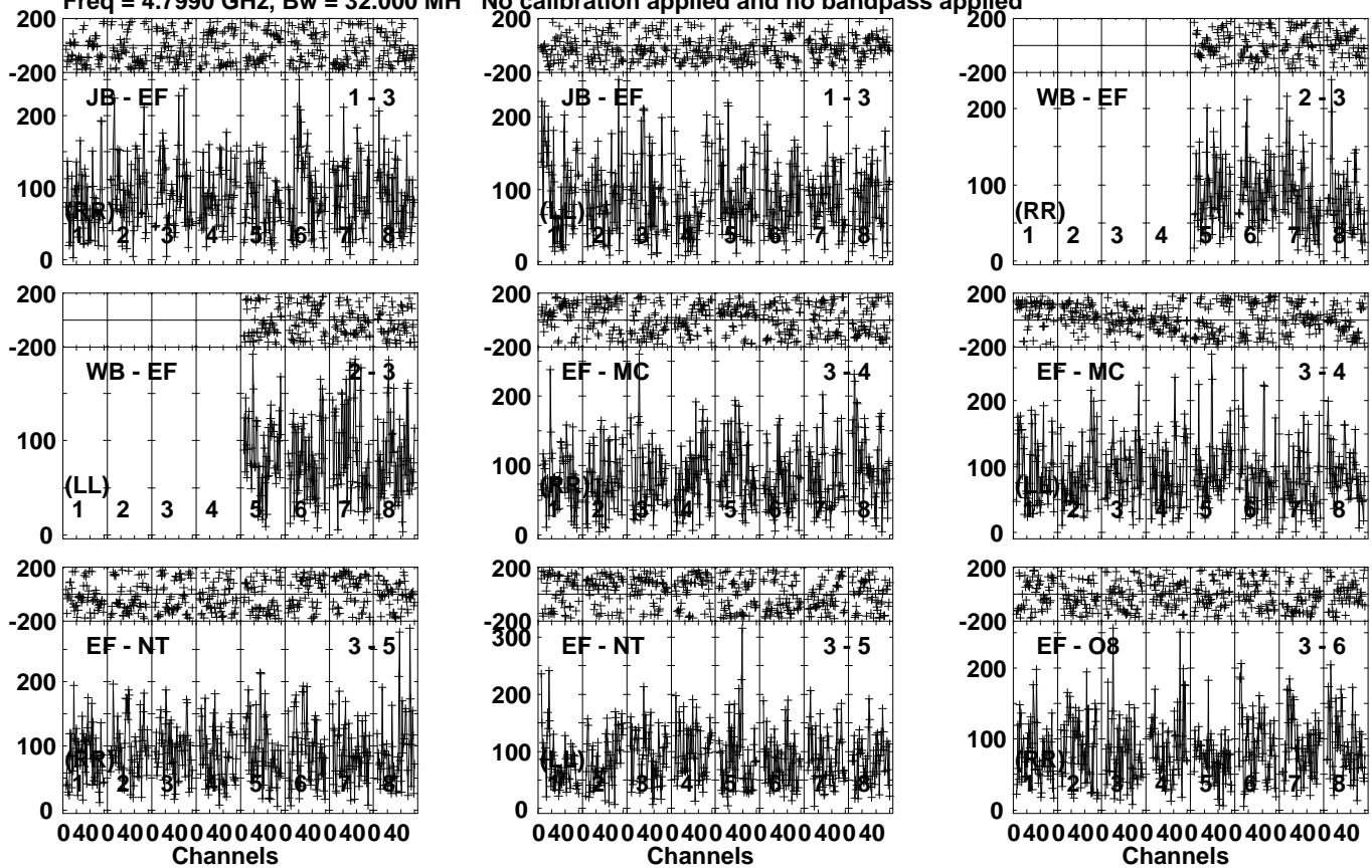
Lower frame: Micro Ampl Jy Top frame: Phas deg Vector averaged cross-power spectrum Several baselines displayed Timerange: 00/23:57:21 to 01/00:00:49
