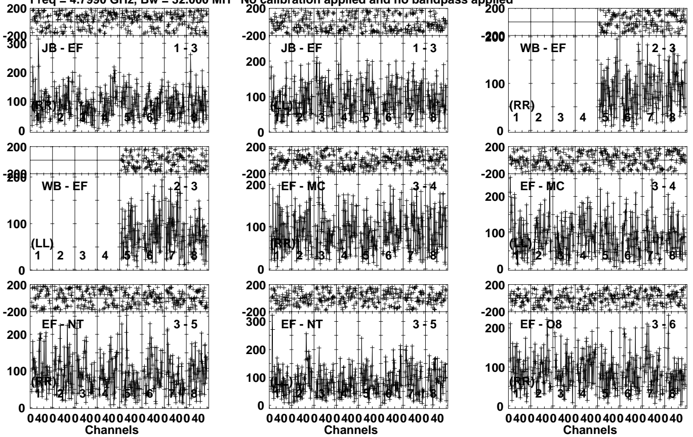
Lower frame: Micro Ampl Jy Top frame: Phas deg Vector averaged cross-power spectrum Several baselines displayed Timerange: 00/23:03:11 to 00/23:06:39
