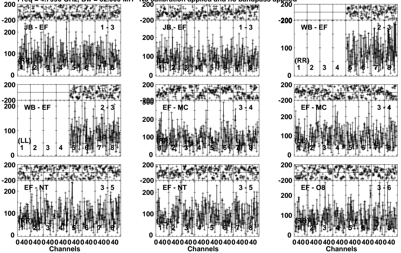
Lower frame: Micro Ampl Jy Top frame: Phas deg Vector averaged cross-power spectrum Several baselines displayed Timerange: 01/00:39:21 to 01/00:42:49
