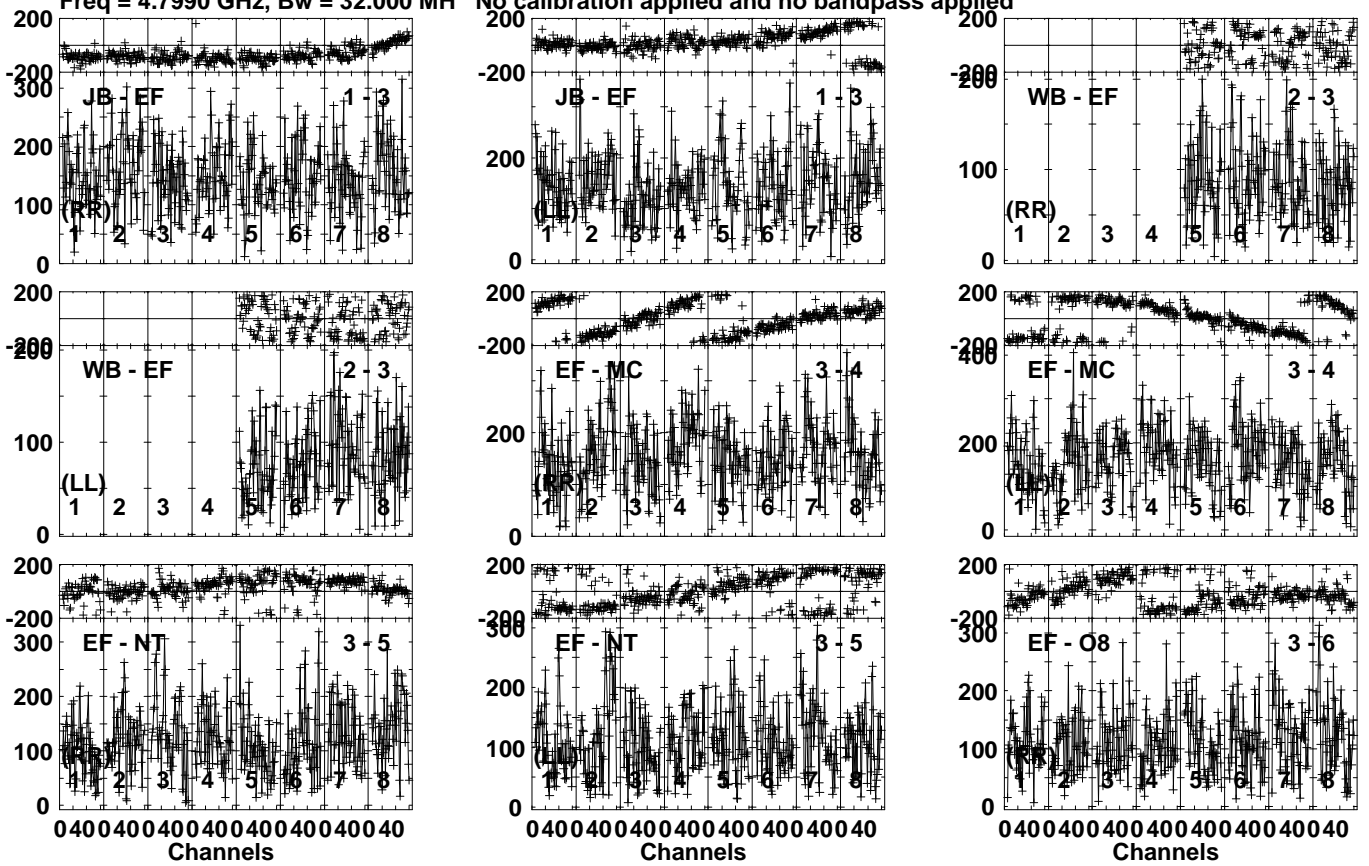
Lower frame: Micro Ampl Jy Top frame: Phas deg Vector averaged cross-power spectrum Several baselines displayed Timerange: 01/01:40:36 to 01/01:44:04
