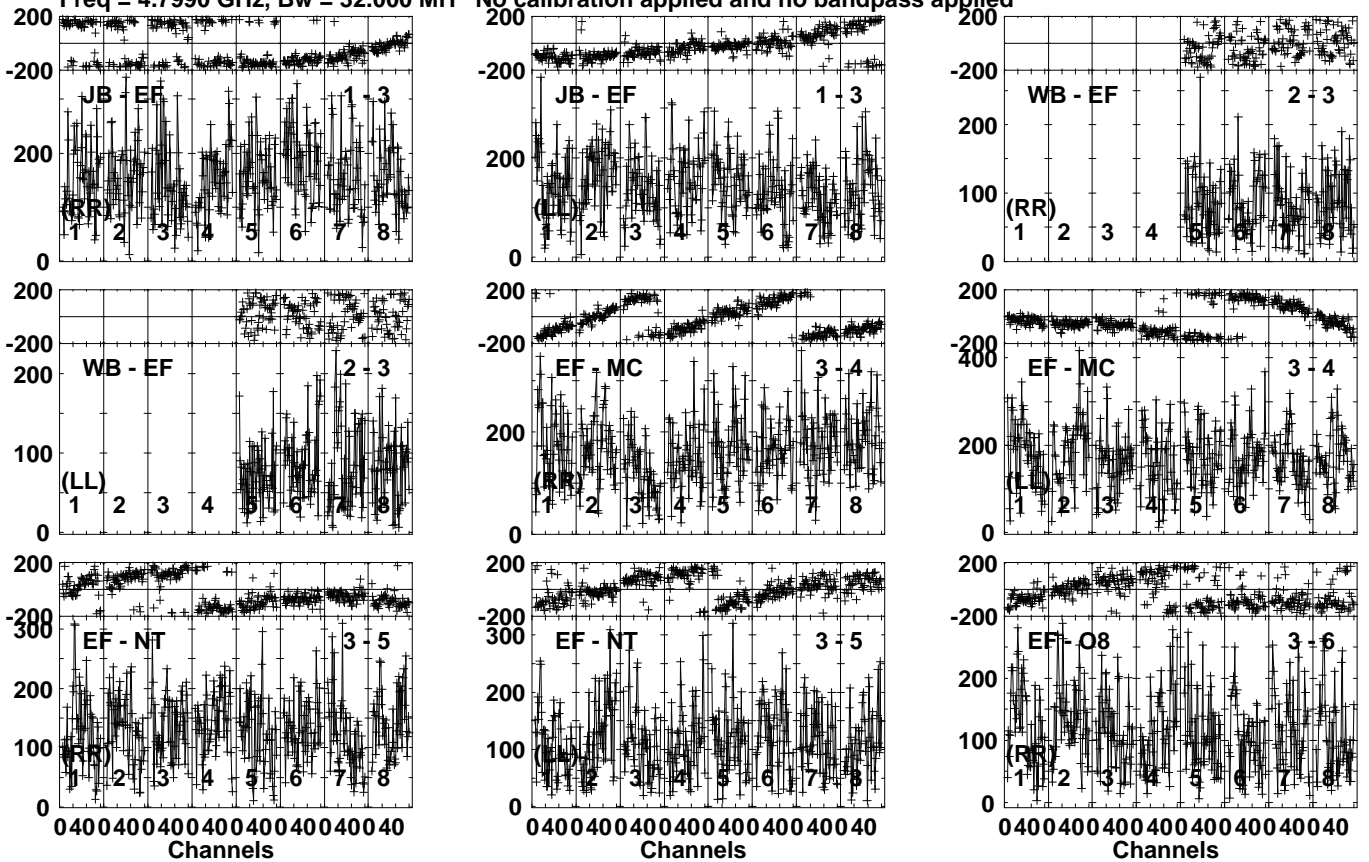
Lower frame: Micro Ampl Jy Top frame: Phas deg Vector averaged cross-power spectrum Several baselines displayed Timerange: 01/03:31:26 to 01/03:34:54
