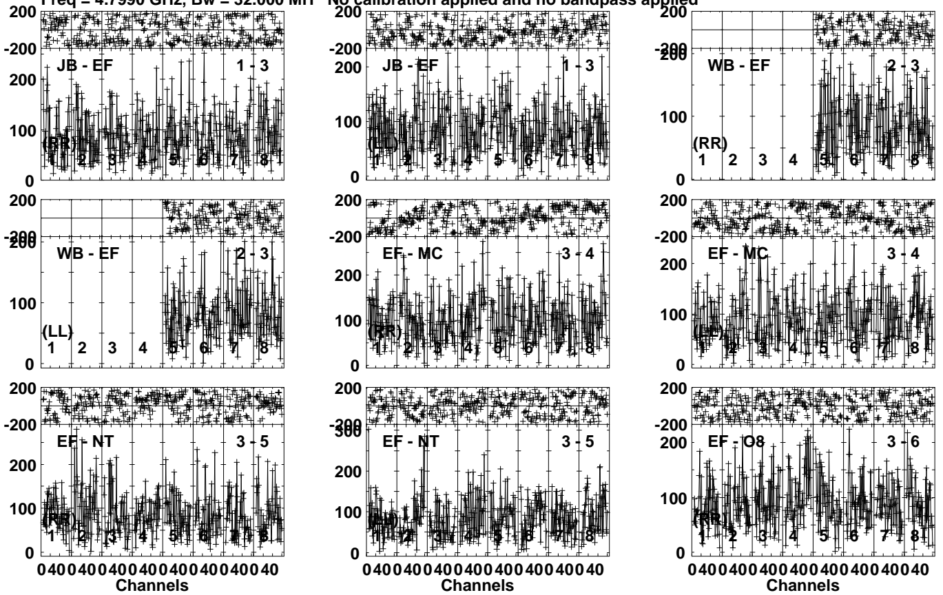
Lower frame: Micro Ampl Jy Top frame: Phas deg Vector averaged cross-power spectrum Several baselines displayed Timerange: 01/00:55:41 to 01/00:59:09
