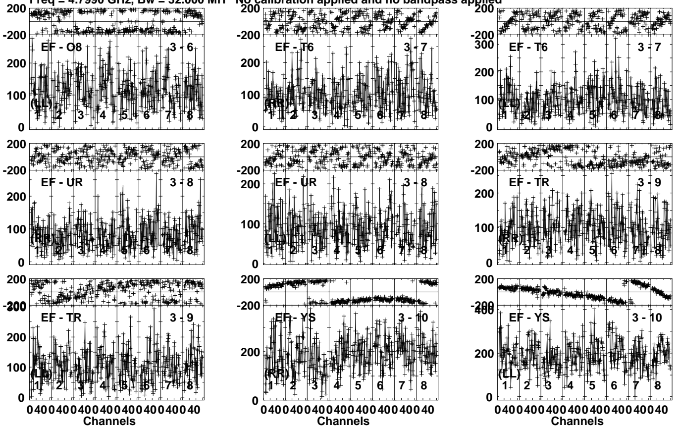
Lower frame: Micro Ampl Jy Top frame: Phas deg Vector averaged cross-power spectrum Several baselines displayed Timerange: 01/02:36:51 to 01/02:40:19
