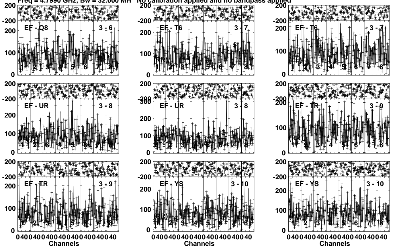
Lower frame: Micro Ampl Jy Top frame: Phas deg Vector averaged cross-power spectrum Several baselines displayed Timerange: 00/23:52:41 to 00/23:56:09
