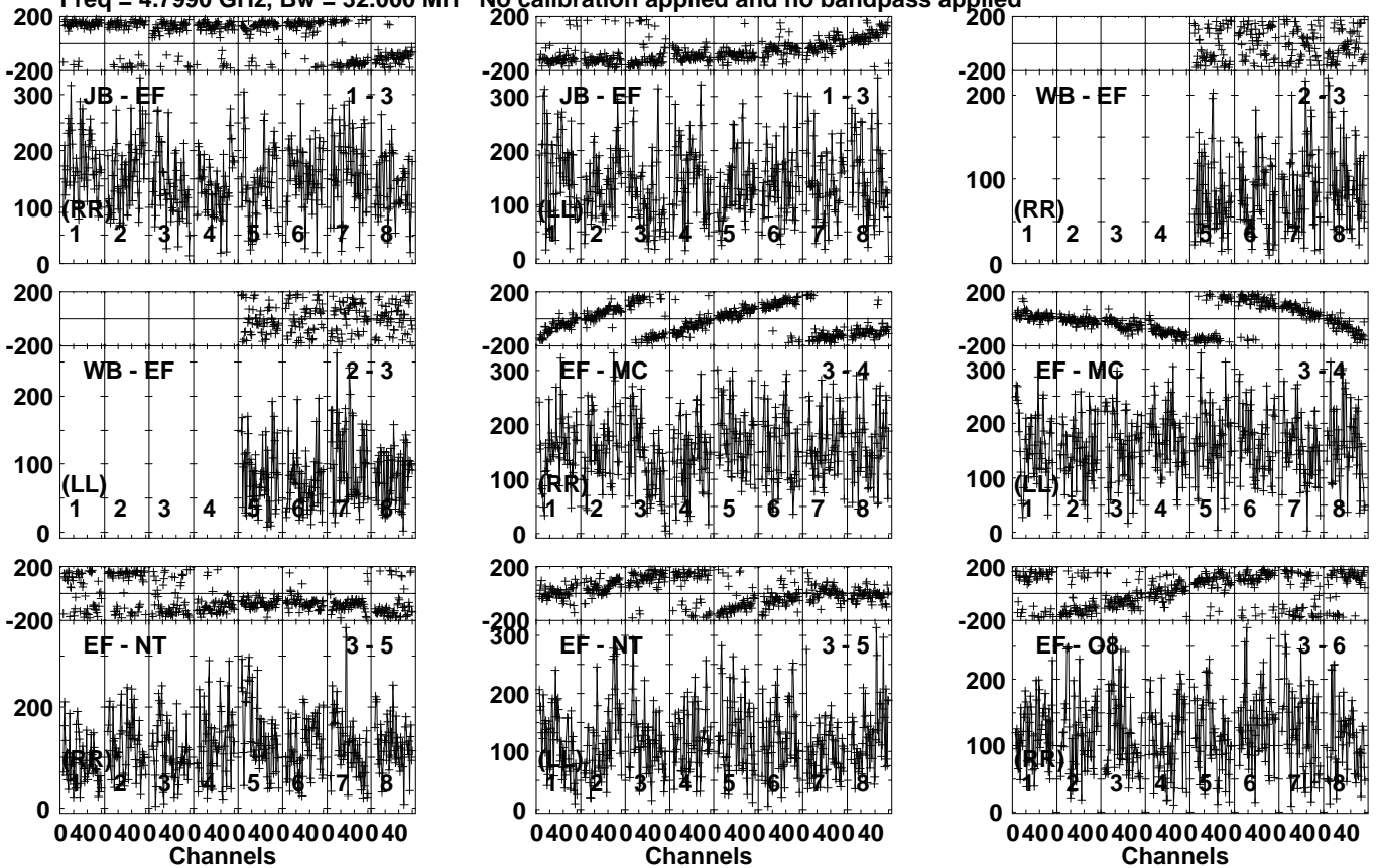
Lower frame: Micro Ampl Jy Top frame: Phas deg Vector averaged cross-power spectrum Several baselines displayed Timerange: 01/01:53:11 to 01/01:56:39
