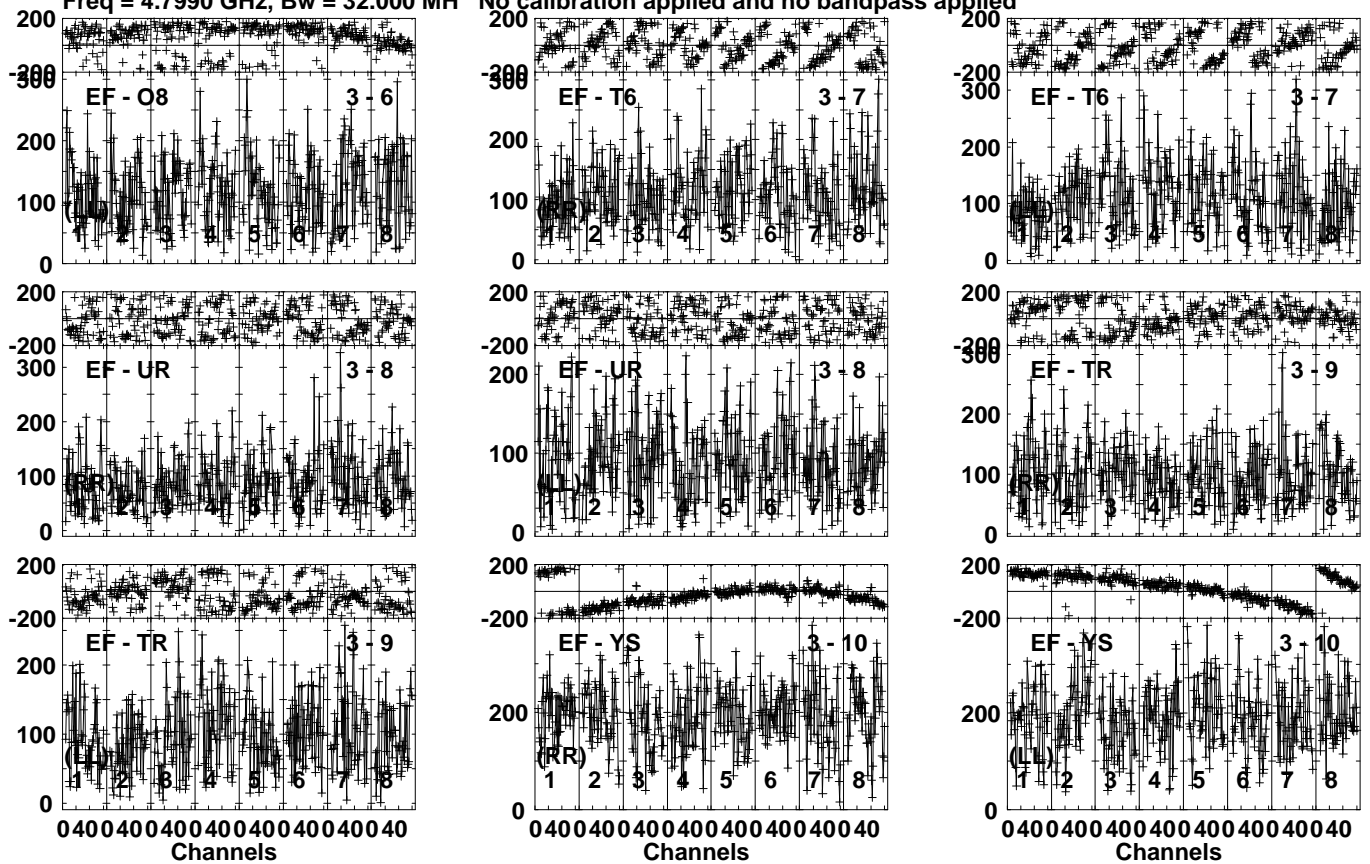
Lower frame: Micro Ampl Jy Top frame: Phas deg Vector averaged cross-power spectrum Several baselines displayed Timerange: 01/03:37:21 to 01/03:40:49
