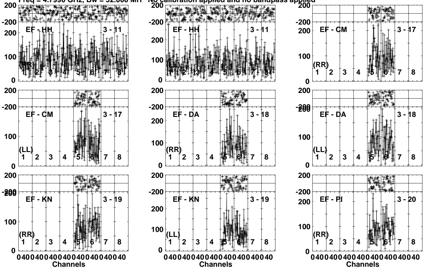
Lower frame: Micro Ampl Jy Top frame: Phas deg Vector averaged cross-power spectrum Several baselines displayed Timerange: 00/23:07:51 to 00/23:11:19
