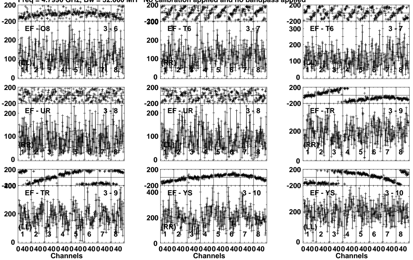
Lower frame: Micro Ampl Jy Top frame: Phas deg Vector averaged cross-power spectrum Several baselines displayed Timerange: 01/02:47:46 to 01/02:51:14
