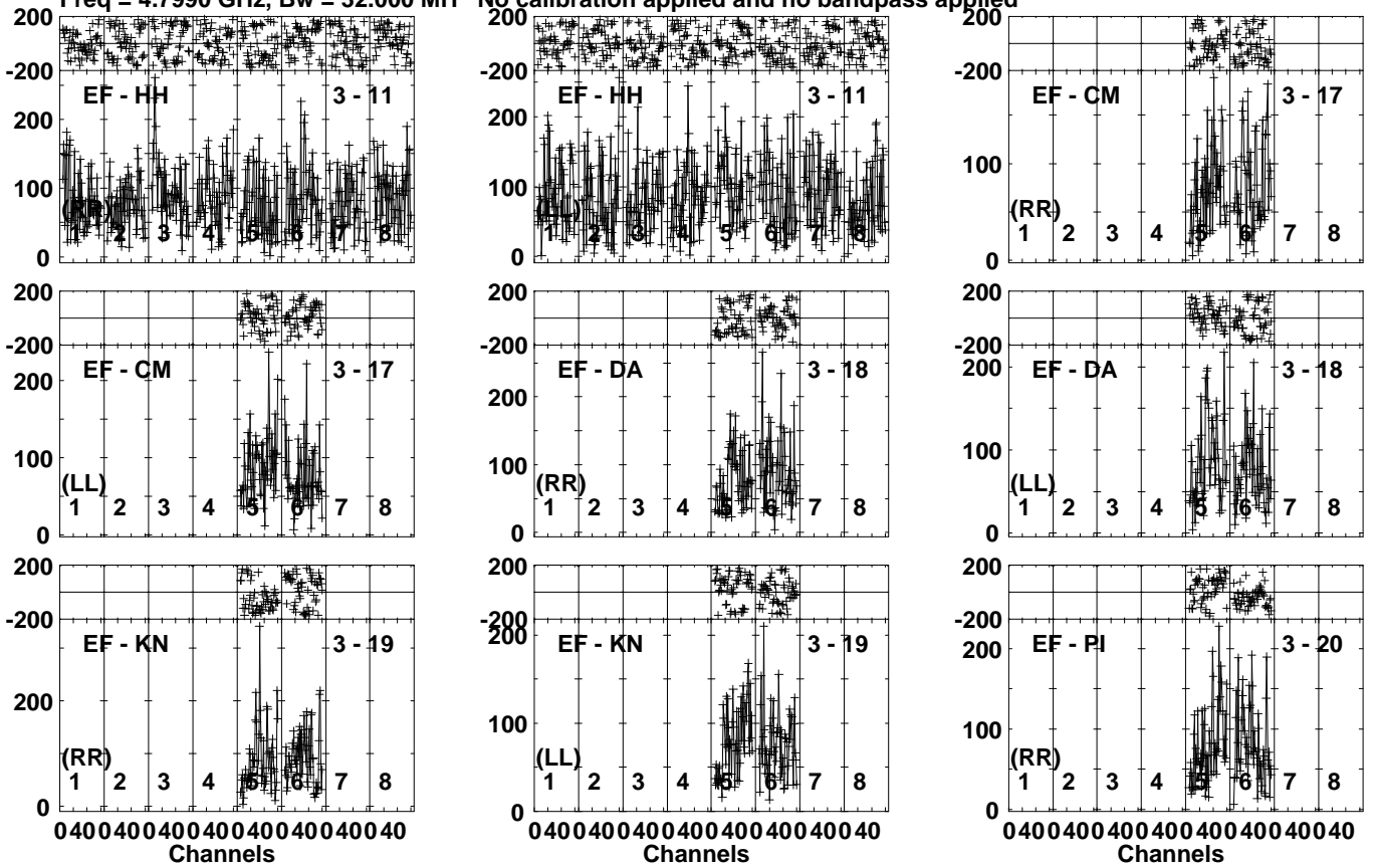
Lower frame: Micro Ampl Jy Top frame: Phas deg Vector averaged cross-power spectrum Several baselines displayed Timerange: 01/00:28:51 to 01/00:32:19
