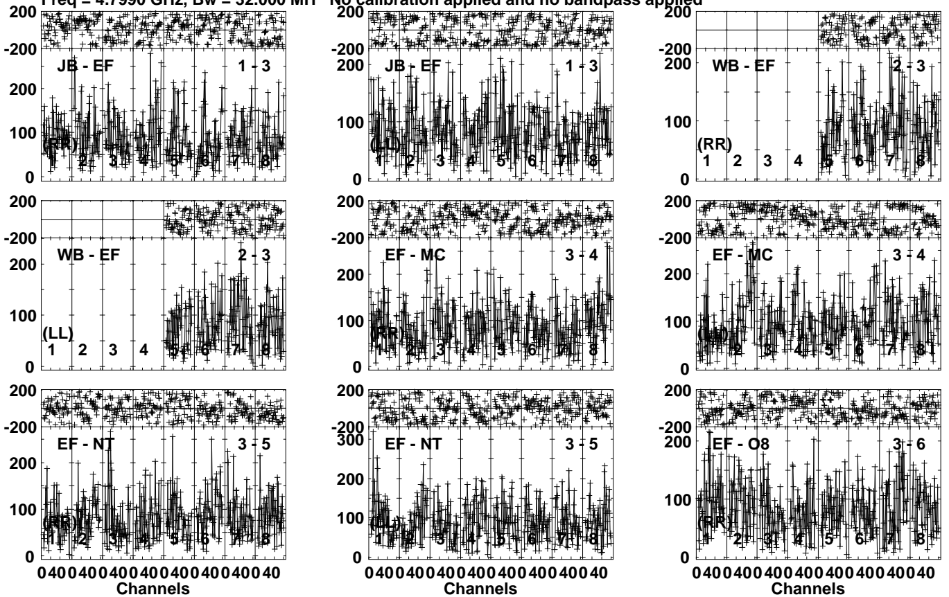
Lower frame: Micro Ampl Jy Top frame: Phas deg Vector averaged cross-power spectrum Several baselines displayed Timerange: 01/01:10:51 to 01/01:14:19
