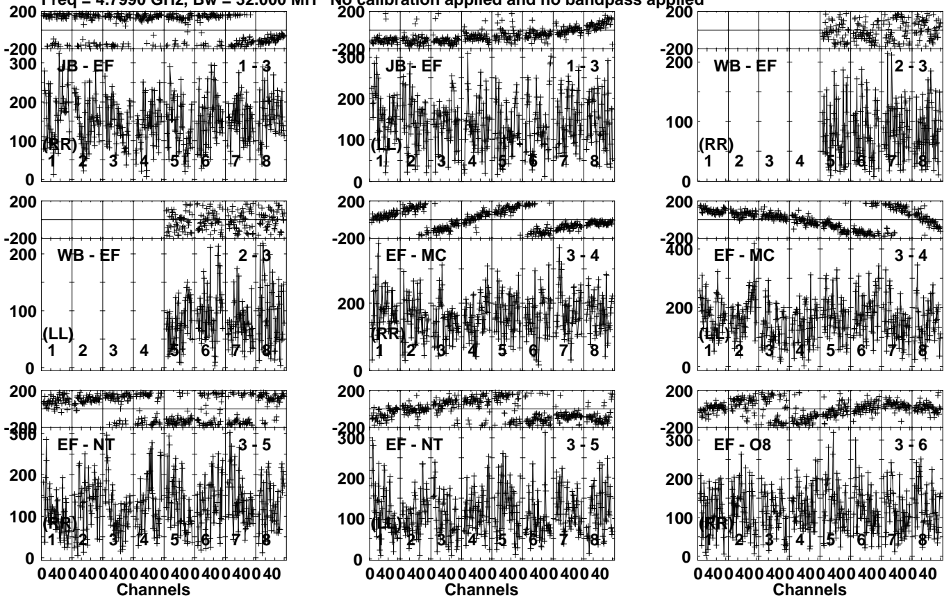
Lower frame: Micro Ampl Jy Top frame: Phas deg Vector averaged cross-power spectrum Several baselines displayed Timerange: 01/01:35:01 to 01/01:38:29
