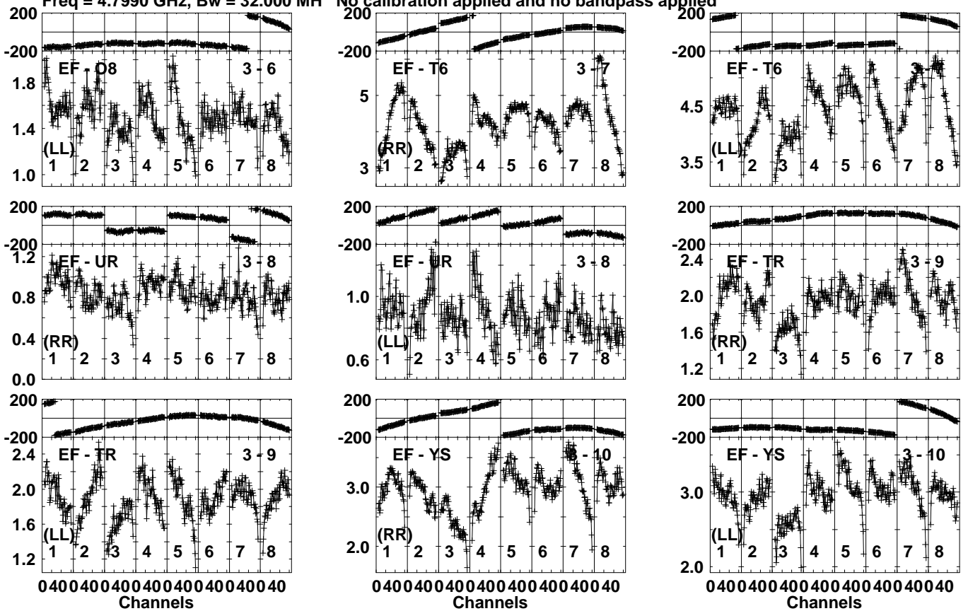
Lower frame: Milli Ampl Jy Top frame: Phas deg Vector averaged cross-power spectrum Several baselines displayed Timerange: 01/02:30:21 to 01/02:31:49
