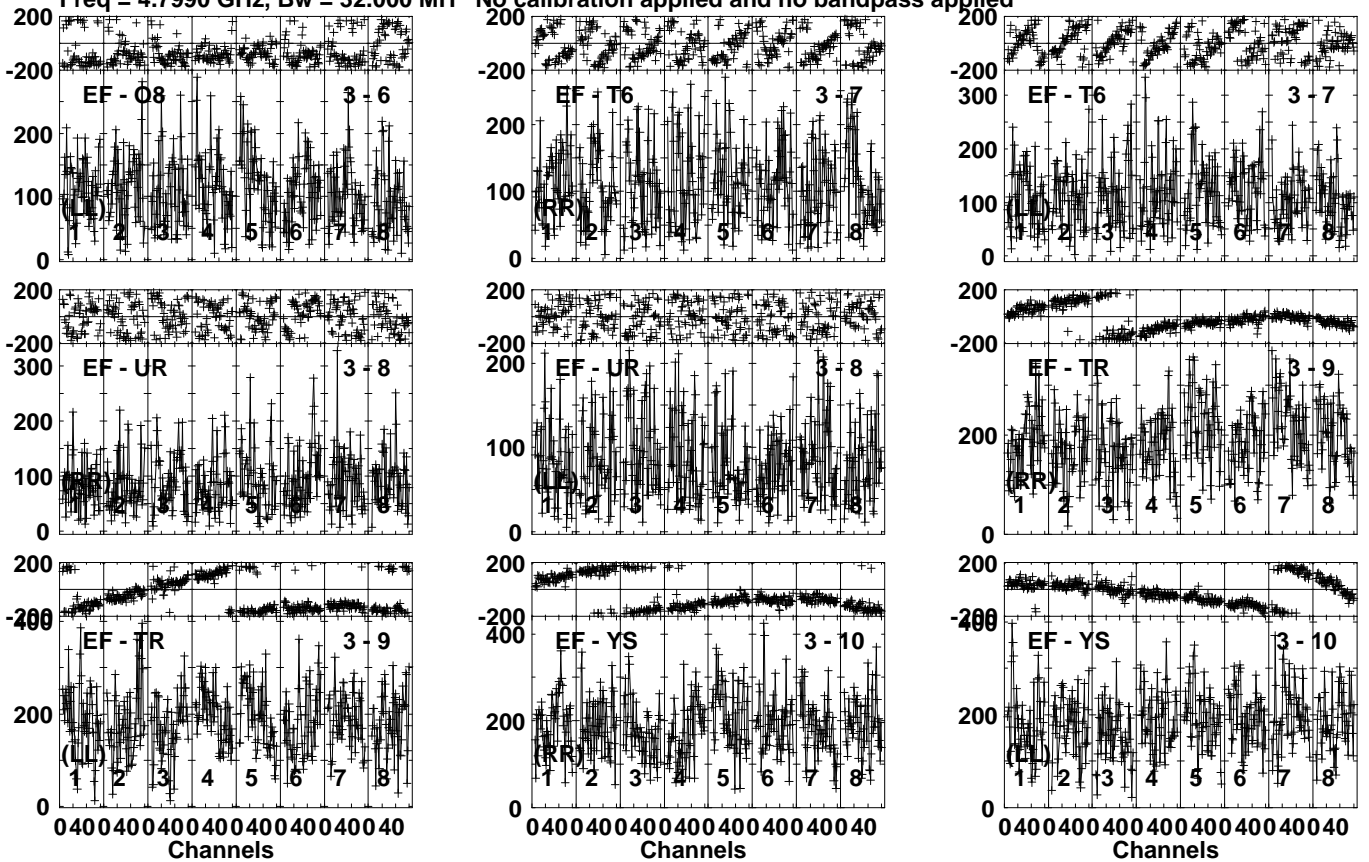
Lower frame: Micro Ampl Jy Top frame: Phas deg Vector averaged cross-power spectrum Several baselines displayed Timerange: 01/03:48:16 to 01/03:51:44
