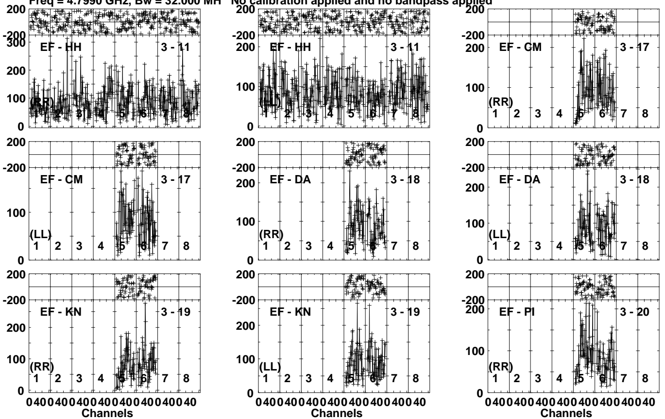
Lower frame: Micro Ampl Jy Top frame: Phas deg Vector averaged cross-power spectrum Several baselines displayed Timerange: 00/23:36:21 to 00/23:39:49
