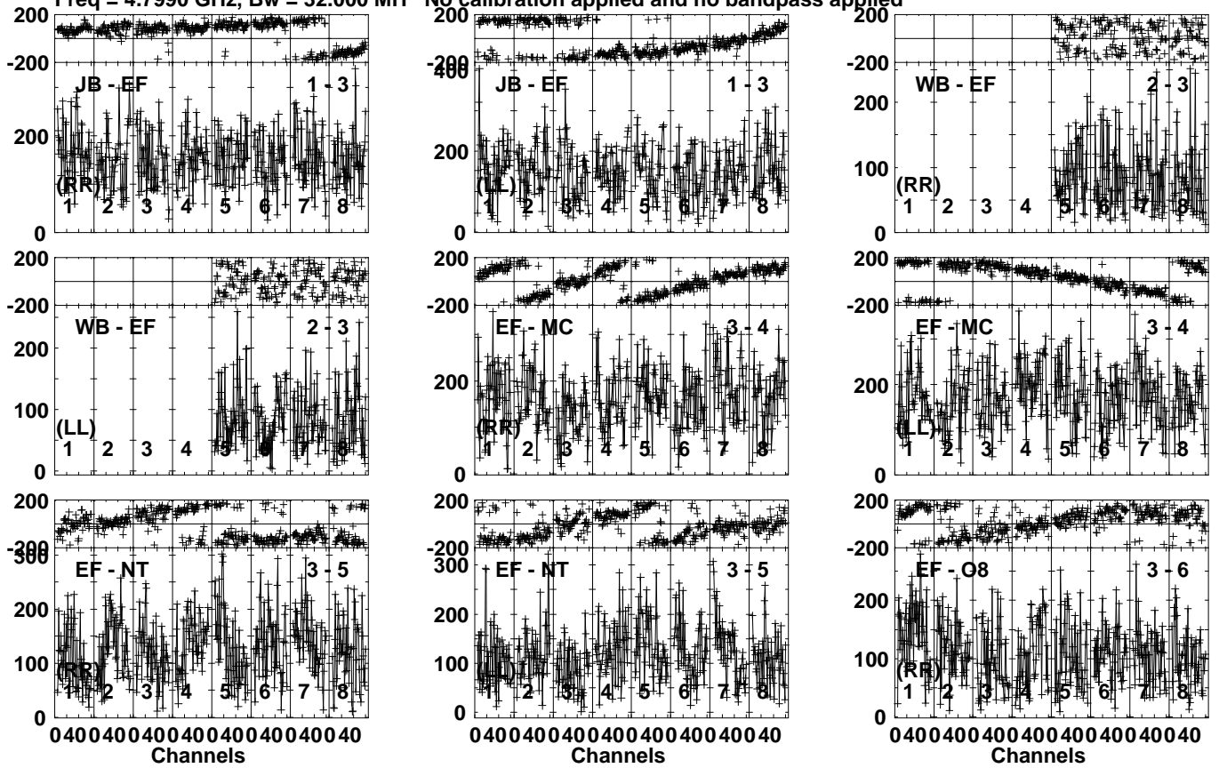
Lower frame: Micro Ampl Jy Top frame: Phas deg Vector averaged cross-power spectrum Several baselines displayed Timerange: 01/03:20:31 to 01/03:23:59
