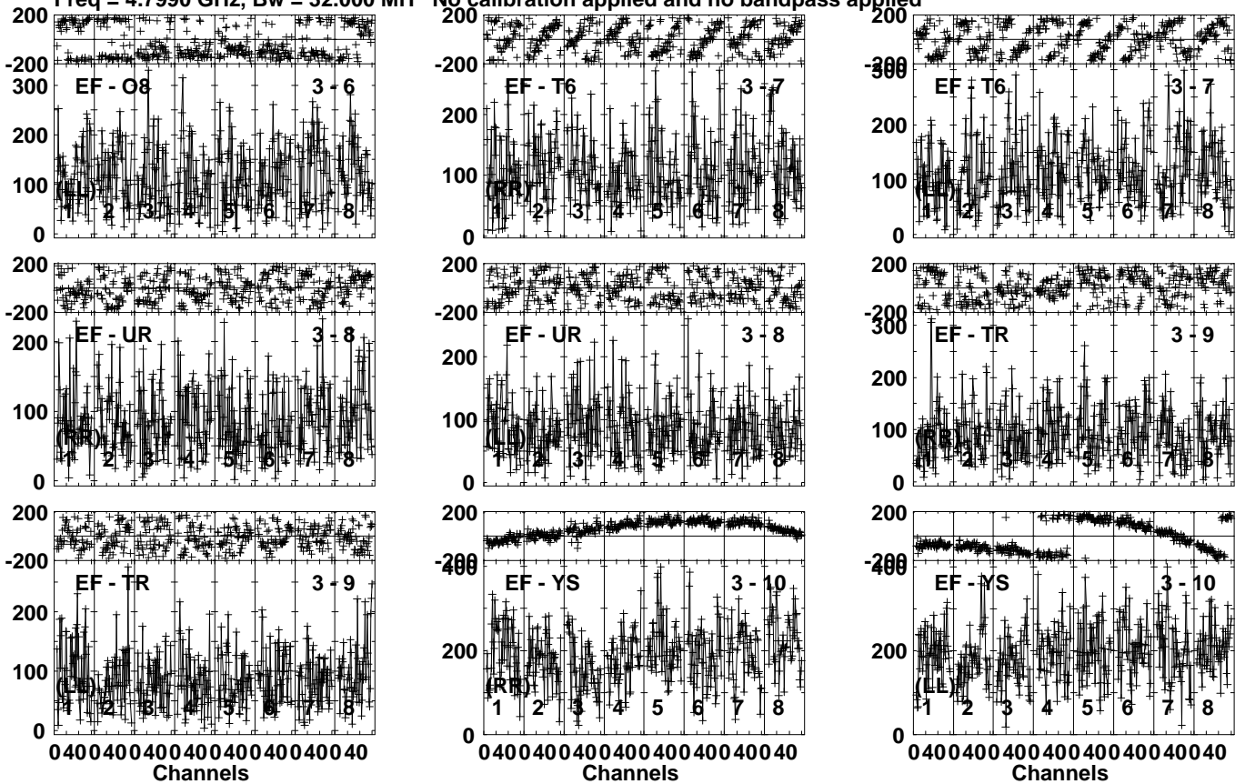
Lower frame: Micro Ampl Jy Top frame: Phas deg Vector averaged cross-power spectrum Several baselines displayed Timerange: 01/02:53:41 to 01/02:57:09
