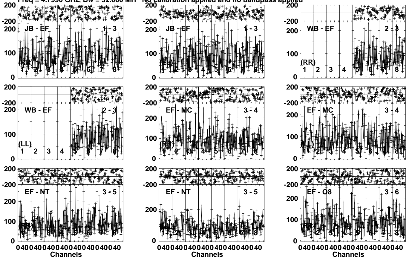
Lower frame: Micro Ampl Jy Top frame: Phas deg Vector averaged cross-power spectrum Several baselines displayed Timerange: 00/22:52:21 to 00/22:55:49
