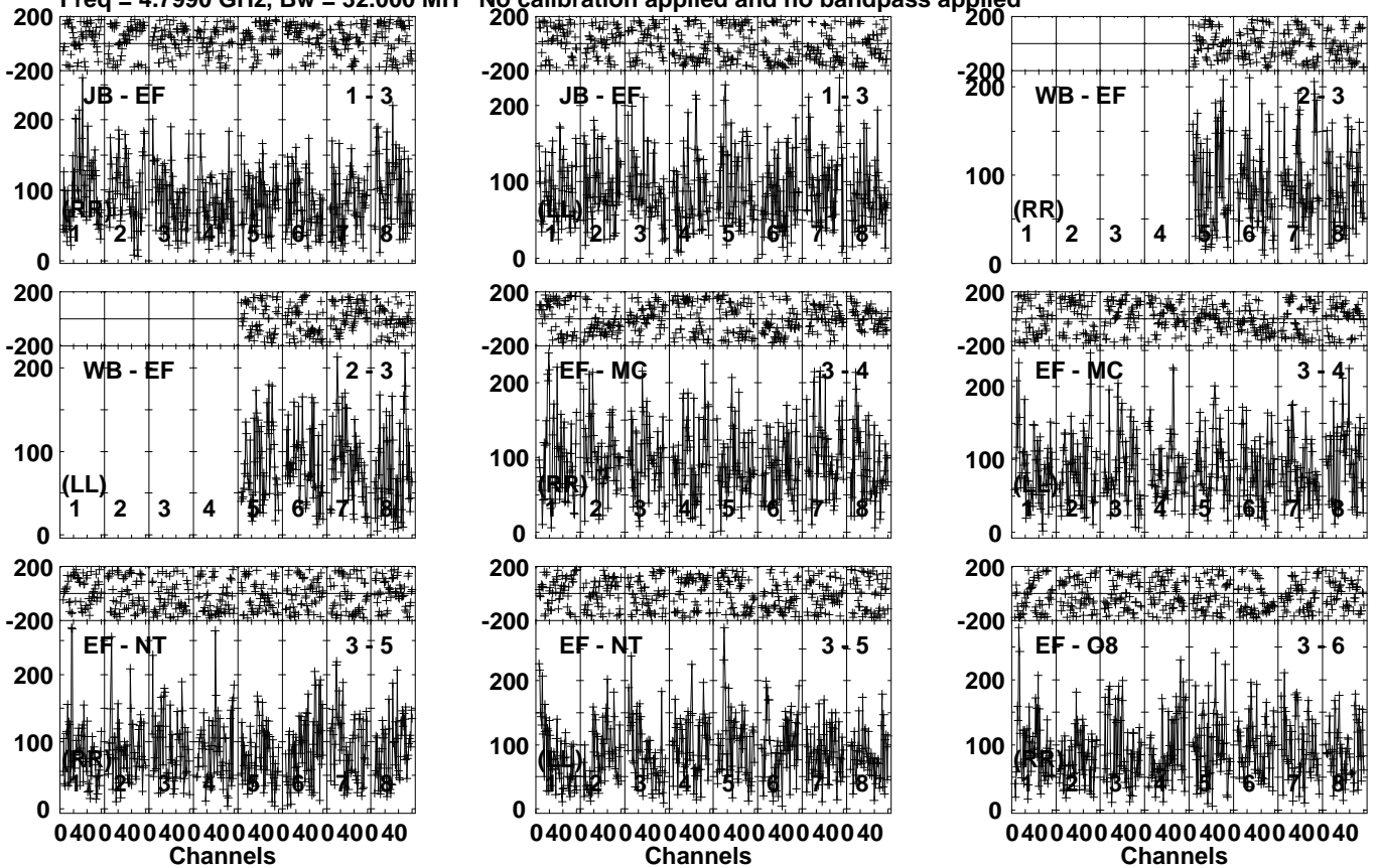
Lower frame: Micro Ampl Jy Top frame: Phas deg Vector averaged cross-power spectrum Several baselines displayed Timerange: 01/00:49:51 to 01/00:53:19
