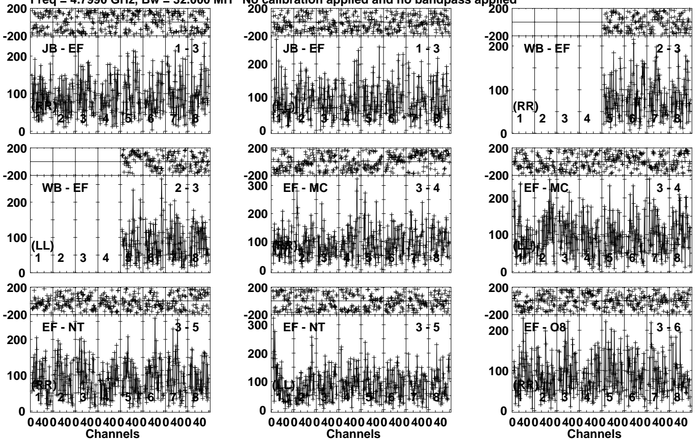
Lower frame: Micro Ampl Jy Top frame: Phas deg Vector averaged cross-power spectrum Several baselines displayed Timerange: 01/00:34:41 to 01/00:38:09
