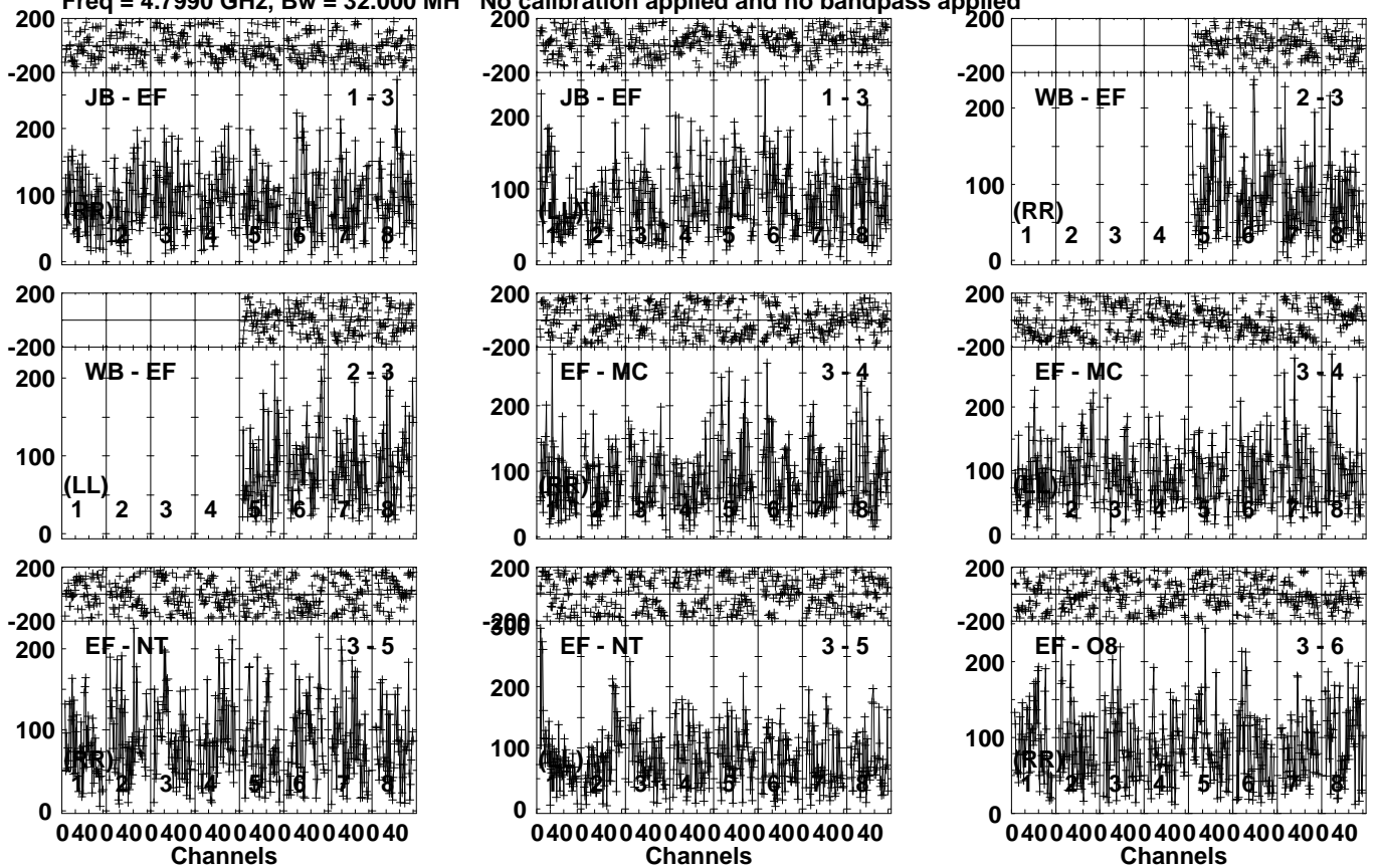
Lower frame: Micro Ampl Jy Top frame: Phas deg Vector averaged cross-power spectrum Several baselines displayed Timerange: 00/23:42:11 to 00/23:45:39
