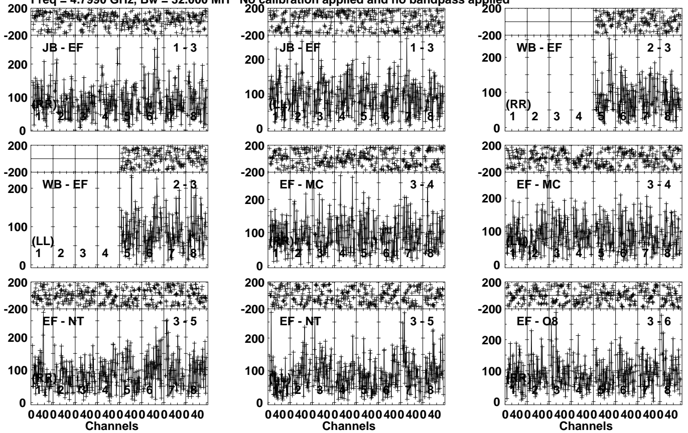
Lower frame: Micro Ampl Jy Top frame: Phas deg Vector averaged cross-power spectrum Several baselines displayed Timerange: 00/22:46:51 to 00/22:50:19
