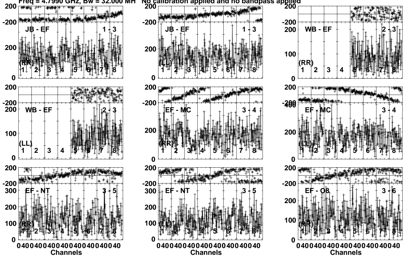
Lower frame: Micro Ampl Jy Top frame: Phas deg Vector averaged cross-power spectrum Several baselines displayed Timerange: 01/02:58:41 to 01/03:02:09
