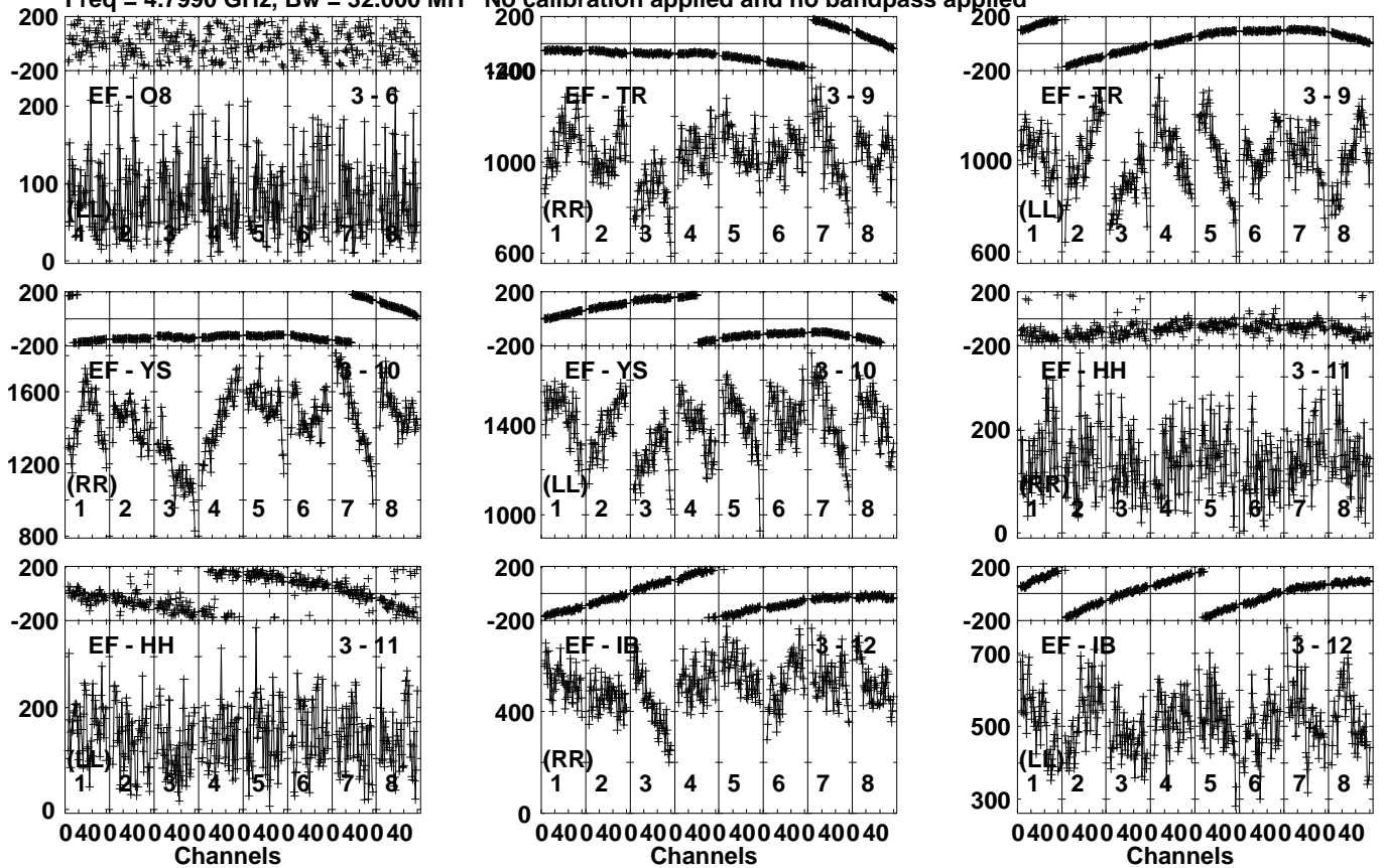
Lower frame: Micro Ampl Jy Top frame: Phas deg Vector averaged cross-power spectrum Several baselines displayed Timerange: 00/17:28:01 to 00/17:31:29
