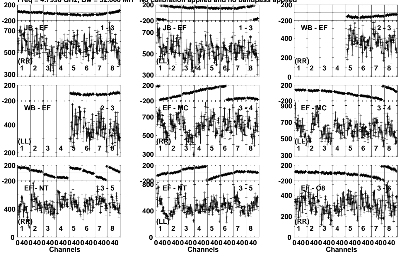
Lower frame: Micro Ampl Jy Top frame: Phas deg Vector averaged cross-power spectrum Several baselines displayed Timerange: 00/13:55:31 to 00/13:58:59
