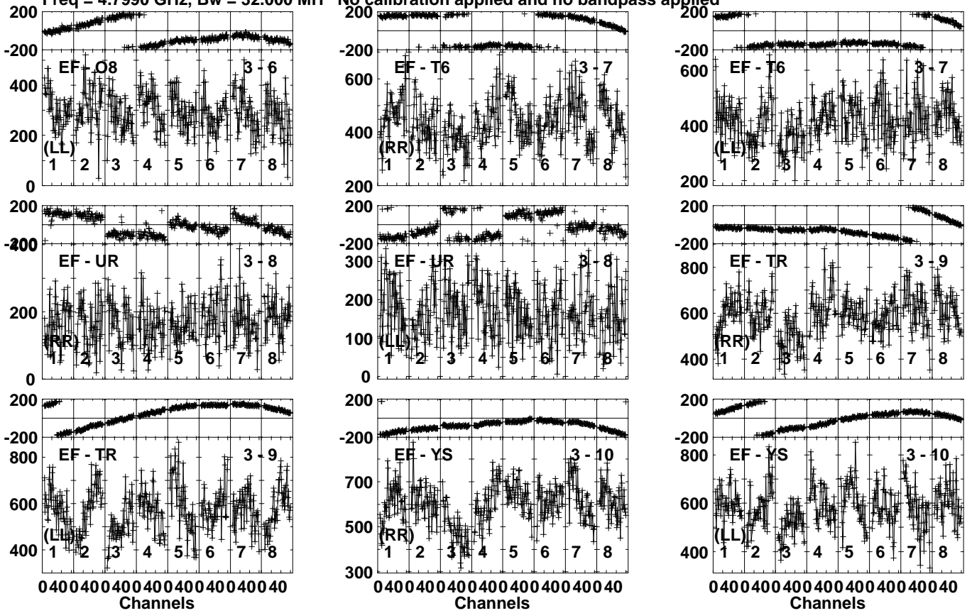
Lower frame: Micro Ampl Jy Top frame: Phas deg Vector averaged cross-power spectrum Several baselines displayed Timerange: 00/13:40:31 to 00/13:43:59
