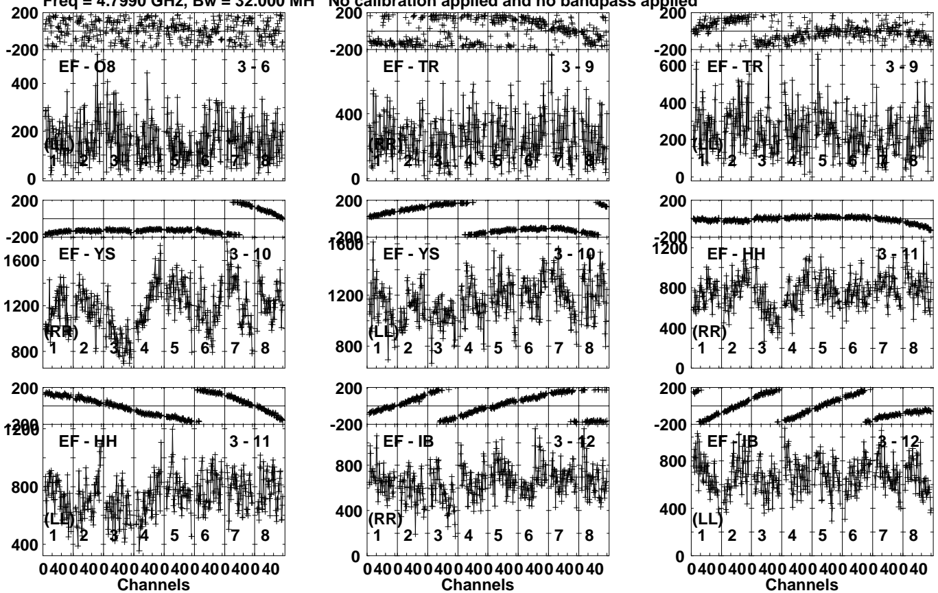
Lower frame: Micro Ampl Jy Top frame: Phas deg Vector averaged cross-power spectrum Several baselines displayed Timerange: 00/18:20:03 to 00/18:21:29
