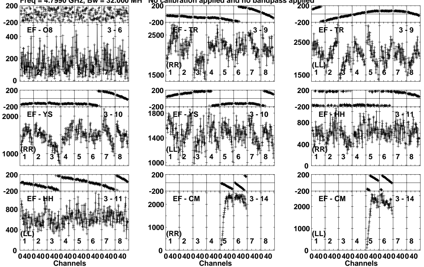
Lower frame: Micro Ampl Jy Top frame: Phas deg Vector averaged cross-power spectrum Several baselines displayed Timerange: 00/19:53:33 to 00/19:54:59
