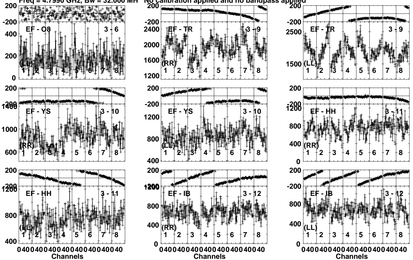
Lower frame: Micro Ampl Jy Top frame: Phas deg Vector averaged cross-power spectrum Several baselines displayed Timerange: 00/18:25:31 to 00/18:26:29
