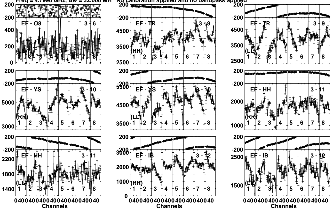
Lower frame: Micro Ampl Jy Top frame: Phas deg Vector averaged cross-power spectrum Several baselines displayed Timerange: 00/17:36:31 to 00/17:37:59
