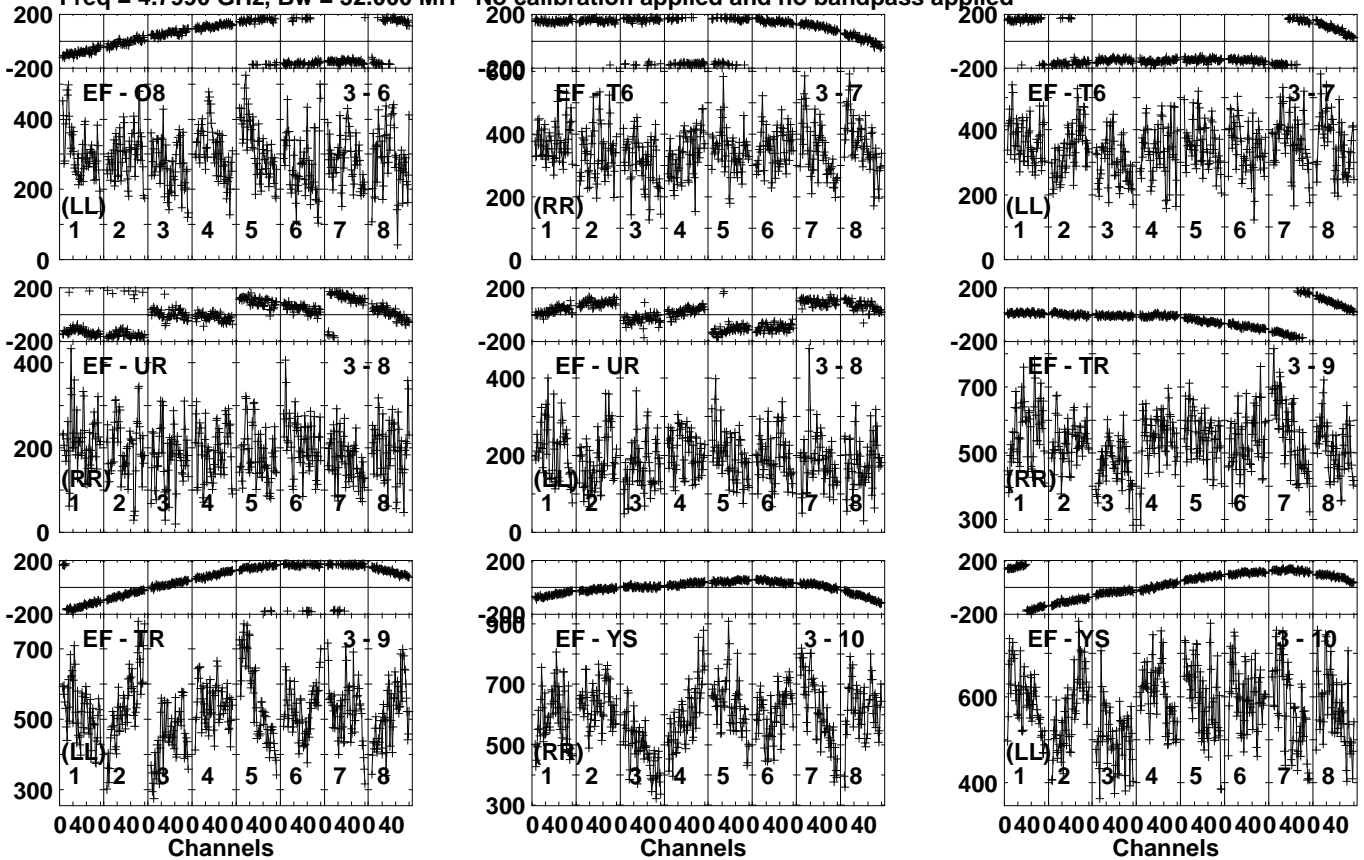
Lower frame: Micro Ampl Jy Top frame: Phas deg Vector averaged cross-power spectrum Several baselines displayed Timerange: 00/14:35:31 to 00/14:38:59
