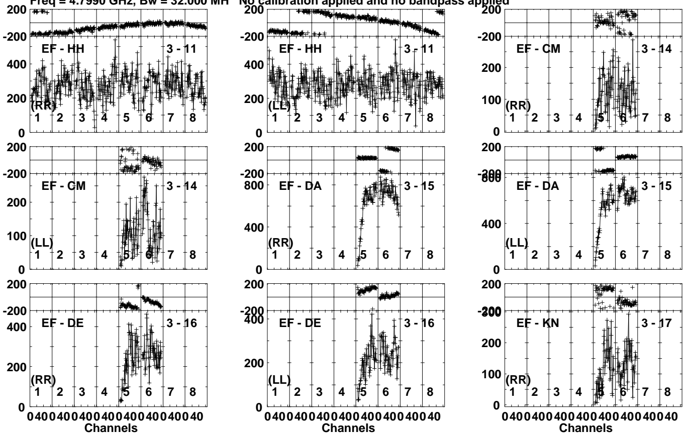
Lower frame: Micro Ampl Jy Top frame: Phas deg Vector averaged cross-power spectrum Several baselines displayed Timerange: 00/12:25:01 to 00/12:28:29
