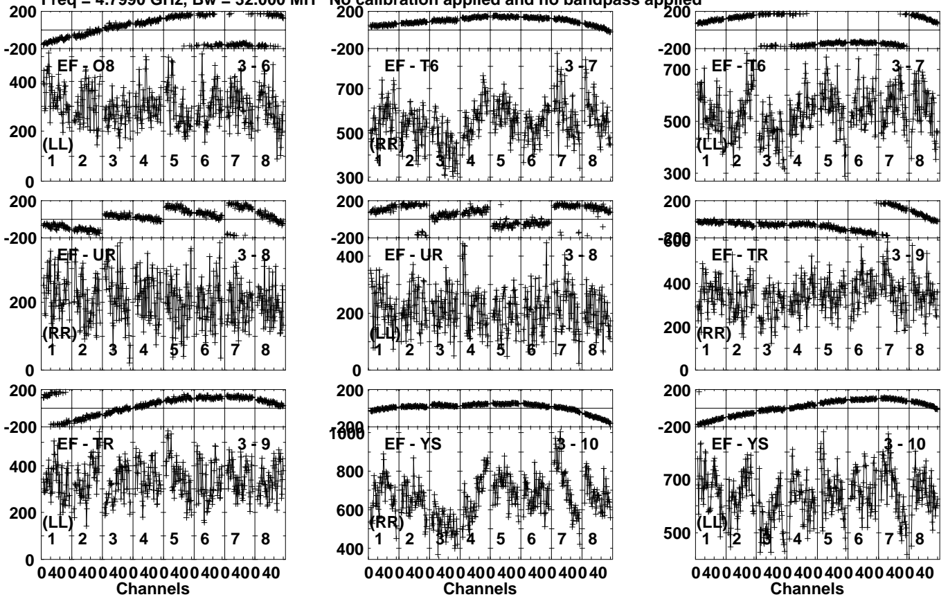
Lower frame: Micro Ampl Jy Top frame: Phas deg Vector averaged cross-power spectrum Several baselines displayed Timerange: 00/15:28:01 to 00/15:31:29
