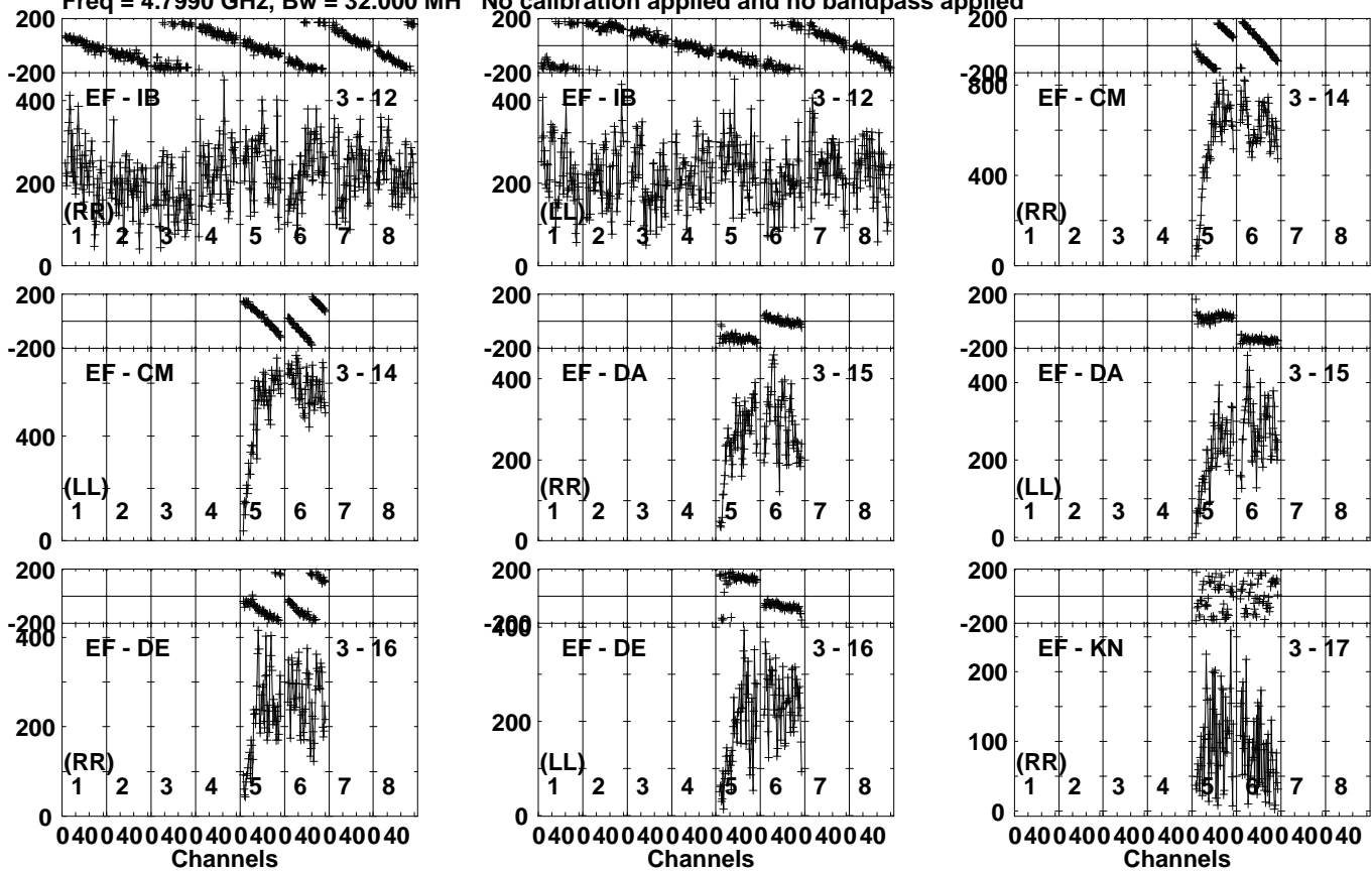
Lower frame: Micro Ampl Jy Top frame: Phas deg Vector averaged cross-power spectrum Several baselines displayed Timerange: 00:16:43:01 to 00:16:46:29
