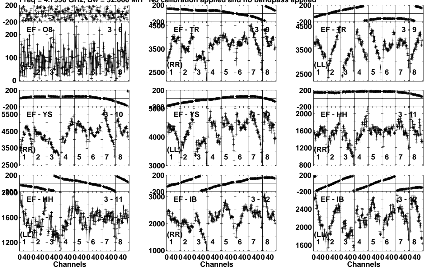
Lower frame: Micro Ampl Jy Top frame: Phas deg Vector averaged cross-power spectrum Several baselines displayed Timerange: 00/18:56:31 to 00/18:59:59
