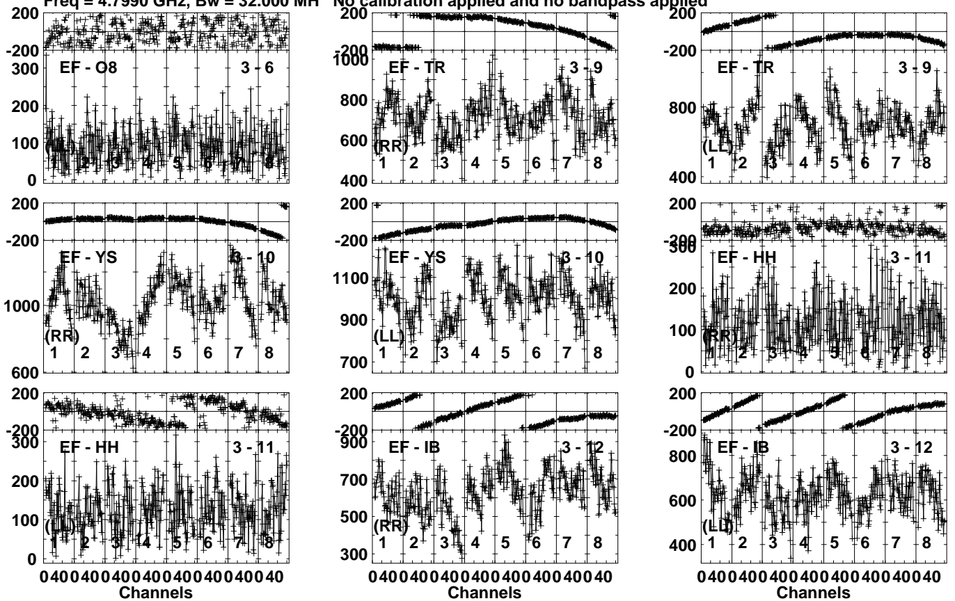
Lower frame: Micro Ampl Jy Top frame: Phas deg Vector averaged cross-power spectrum Several baselines displayed Timerange: 00/19:00:03 to 00/19:03:29
