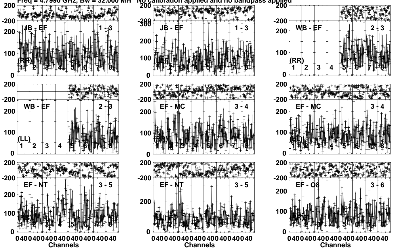
Lower frame: Micro Ampl Jy Top frame: Phas deg Vector averaged cross-power spectrum Several baselines displayed Timerange: 00/18:51:31 to 00/18:54:59
