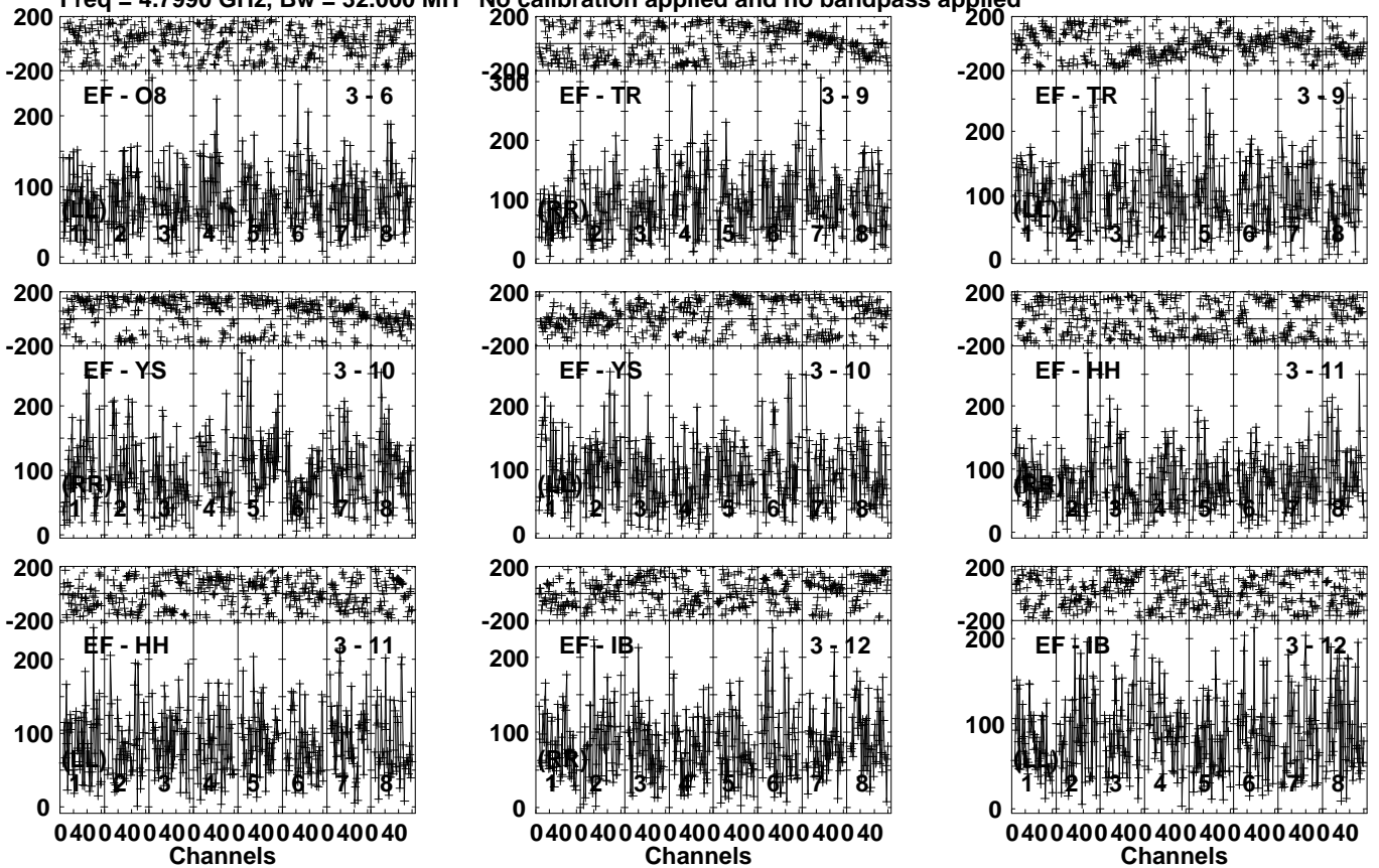
Lower frame: Micro Ampl Jy Top frame: Phas deg Vector averaged cross-power spectrum Several baselines displayed Timerange: 00/18:21:31 to 00/18:24:59
