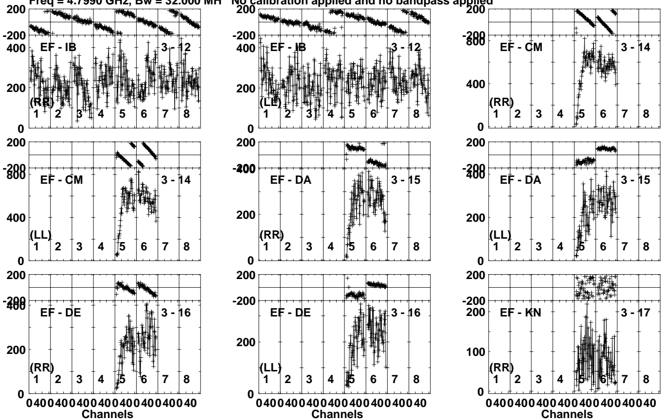
Lower frame: Micro Ampl Jy Top frame: Phas deg Vector averaged cross-power spectrum Several baselines displayed Timerange: 00/16:18:01 to 00/16:21:29
