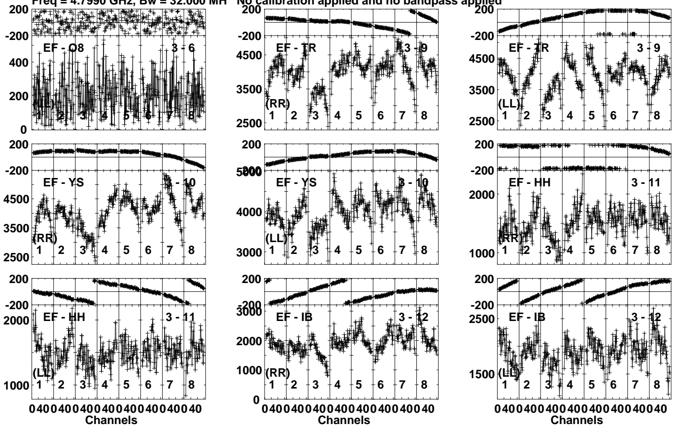
Lower frame: Micro Ampl Jy Top frame: Phas deg Vector averaged cross-power spectrum Several baselines displayed Timerange: 00/19:39:01 to 00/19:39:59
