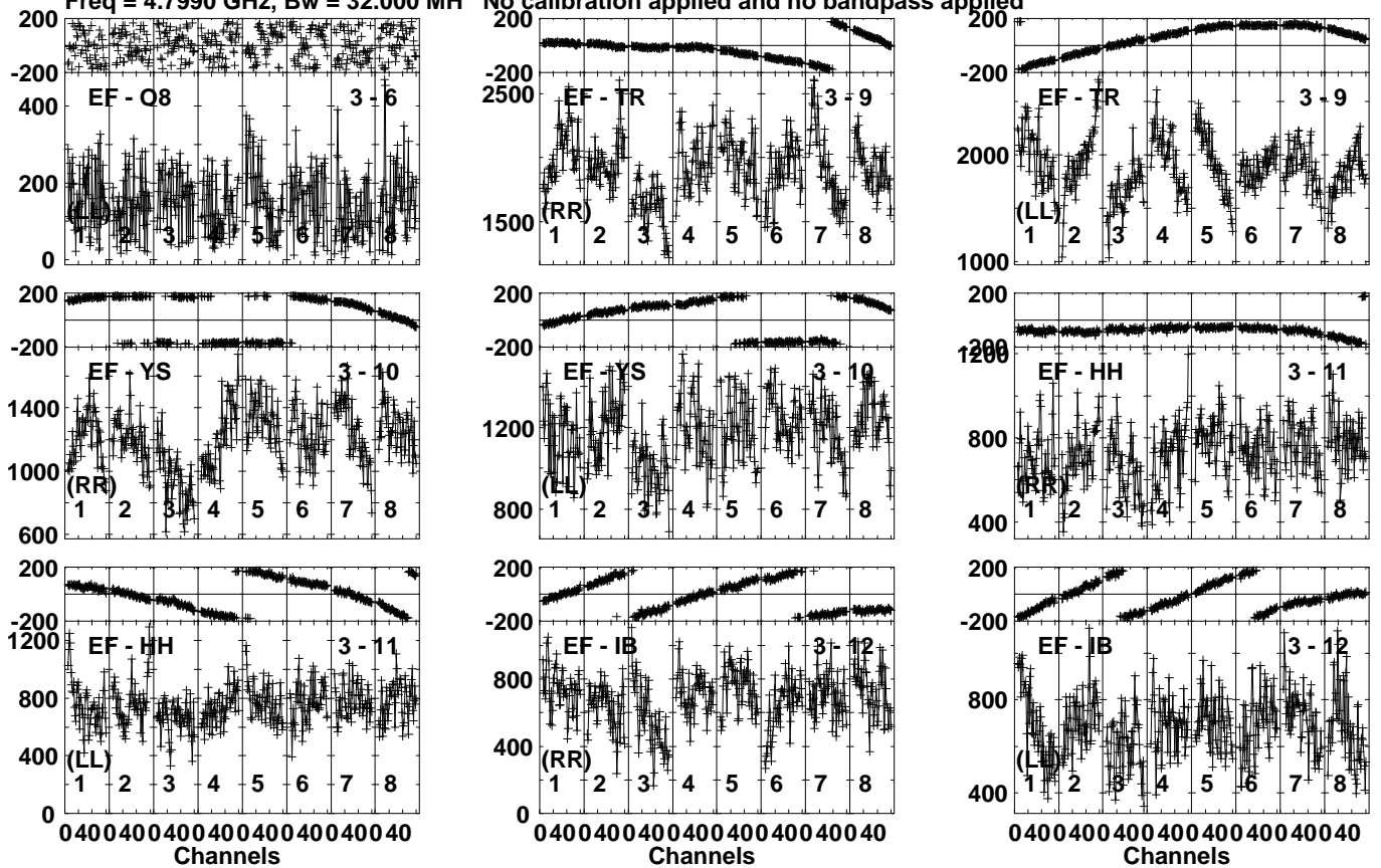
Lower frame: Micro Ampl Jy Top frame: Phas deg Vector averaged cross-power spectrum Several baselines displayed Timerange: 00:18:30:01 to 00:18:31:29
