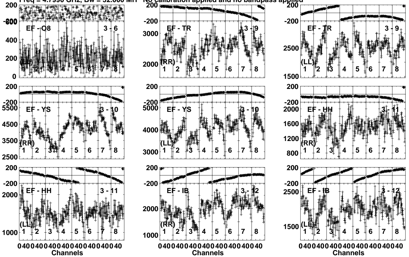
Lower frame: Micro Ampl Jy Top frame: Phas deg Vector averaged cross-power spectrum Several baselines displayed Timerange: 00/19:29:01 to 00/19:29:59
