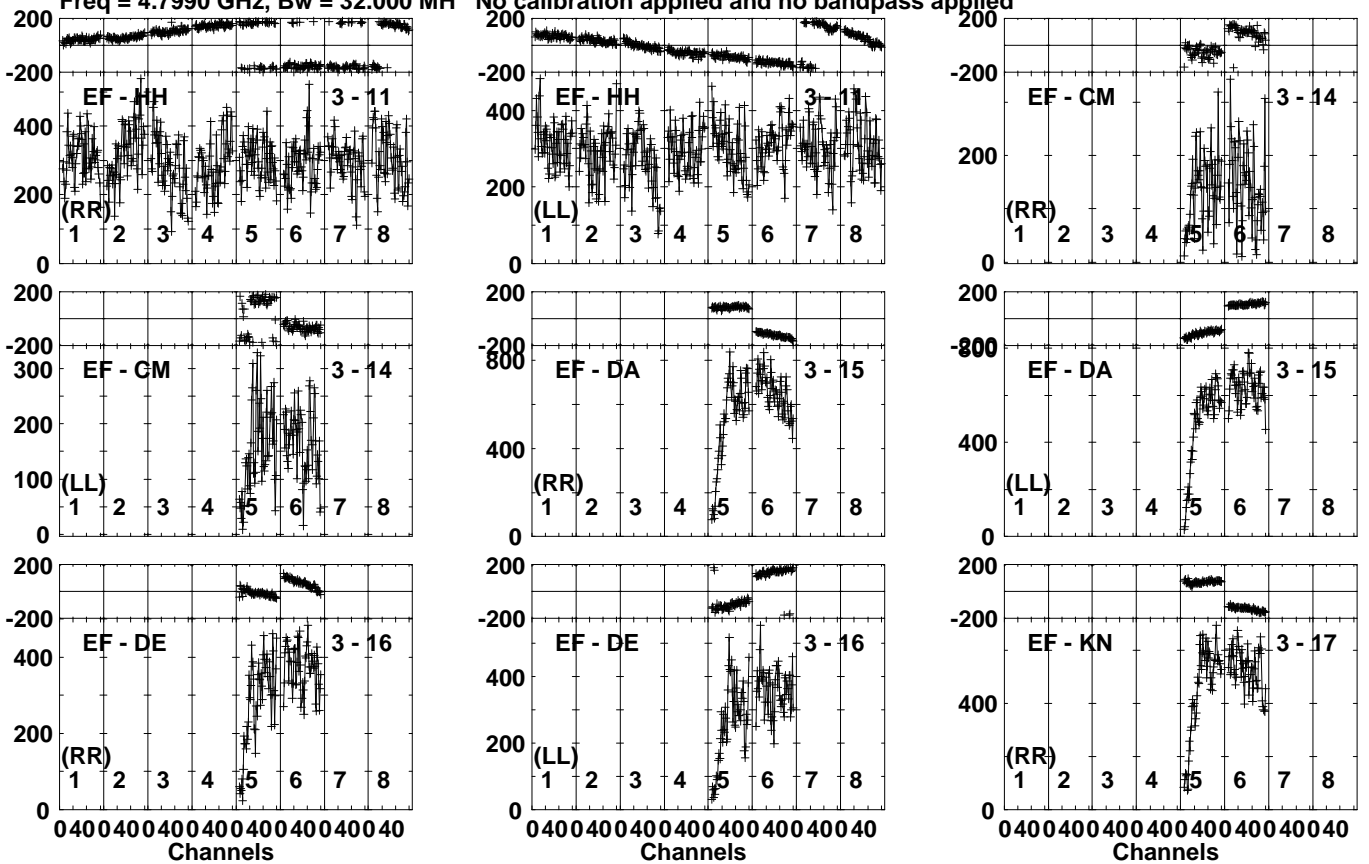
Lower frame: Micro Ampl Jy Top frame: Phas deg Vector averaged cross-power spectrum Several baselines displayed Timerange: 00/12:20:01 to 00/12:23:29
