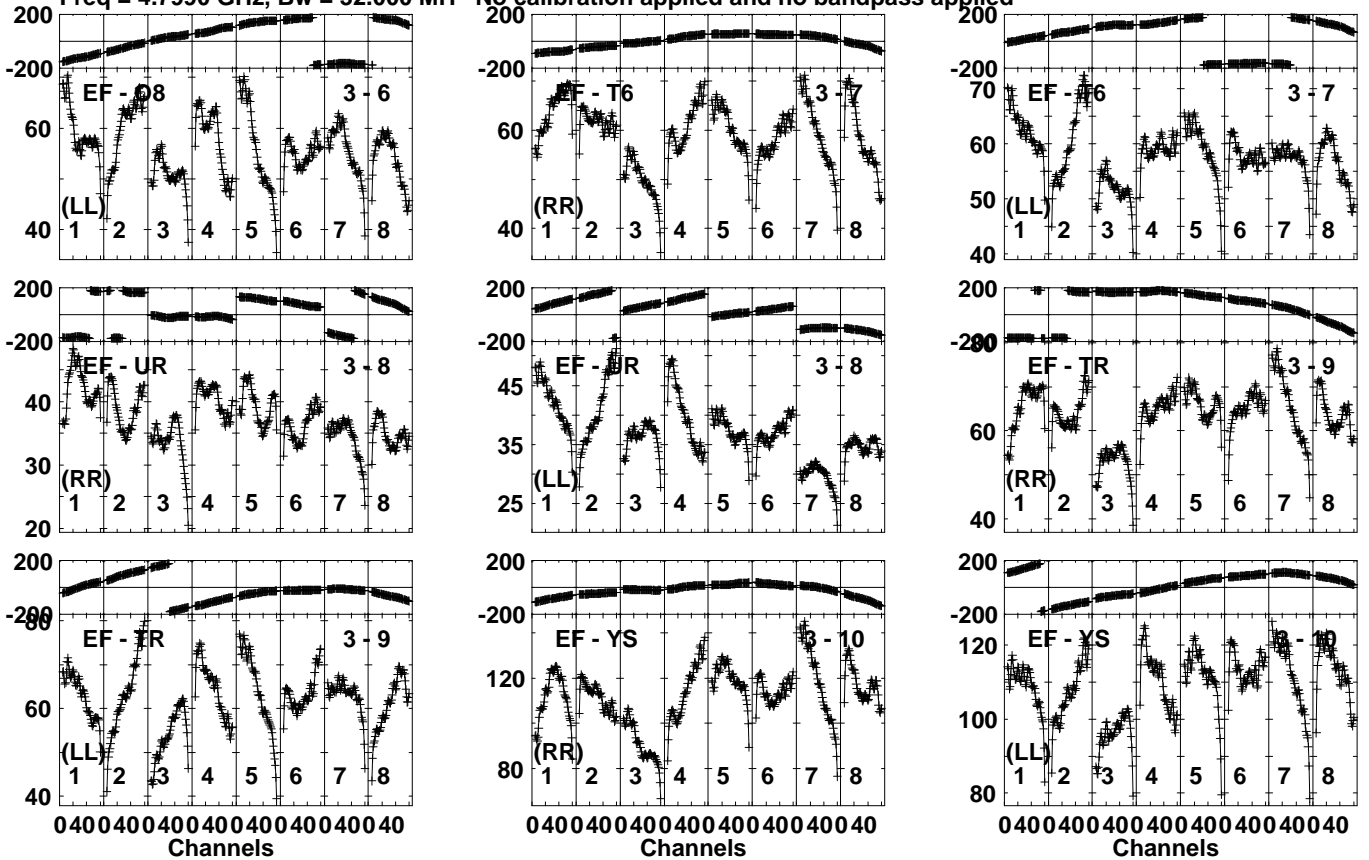
Lower frame: Milli Ampl Jy Top frame: Phas deg Vector averaged cross-power spectrum Several baselines displayed Timerange: 00/13:16:01 to 00/13:20:59
