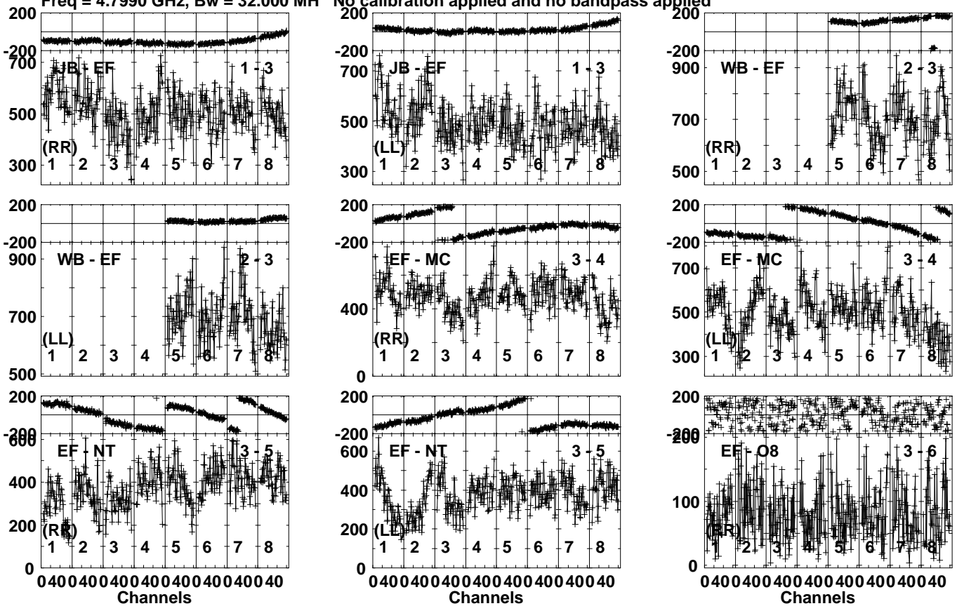
Lower frame: Micro Ampl Jy Top frame: Phas deg Vector averaged cross-power spectrum Several baselines displayed Timerange: 00/17:33:01 to 00/17:36:29
