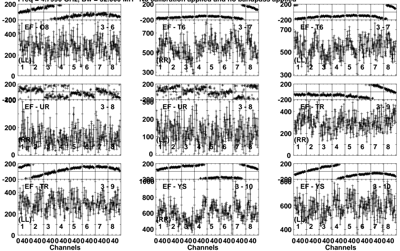
Lower frame: Micro Ampl Jy Top frame: Phas deg Vector averaged cross-power spectrum Several baselines displayed Timerange: 00:12:44:31 to 00:12:47:59
