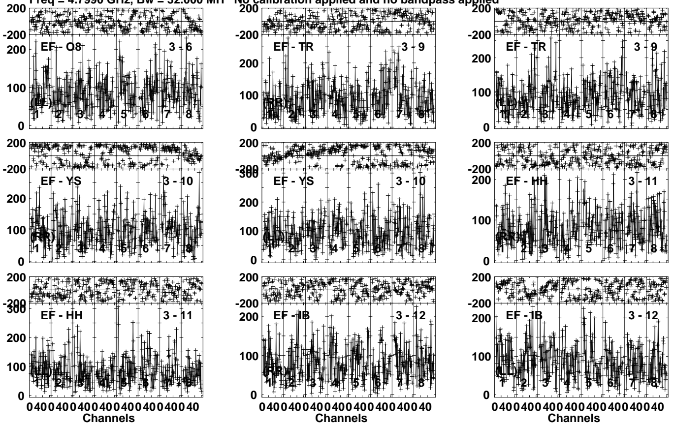
Lower frame: Micro Ampl Jy Top frame: Phas deg Vector averaged cross-power spectrum Several baselines displayed Timerange: 00/18:11:31 to 00/18:14:59
