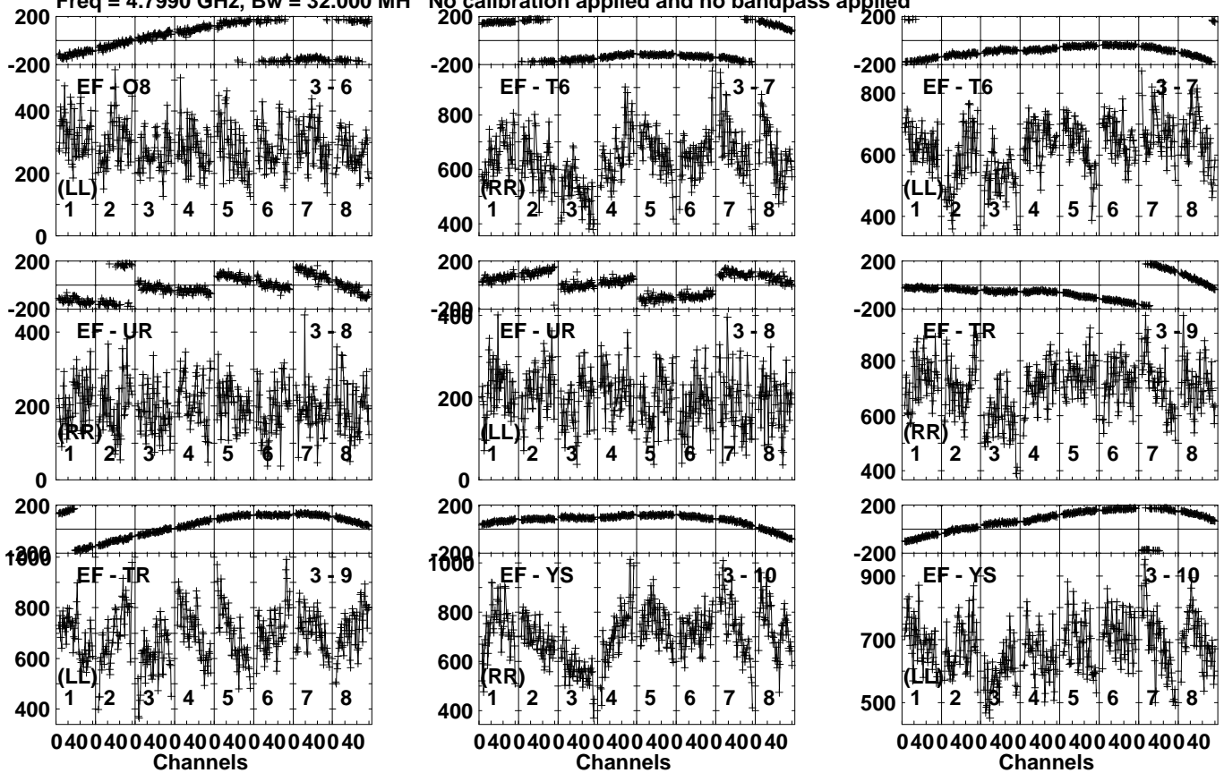
Lower frame: Micro Ampl Jy Top frame: Phas deg Vector averaged cross-power spectrum Several baselines displayed Timerange: 00/15:23:01 to 00/15:26:29
