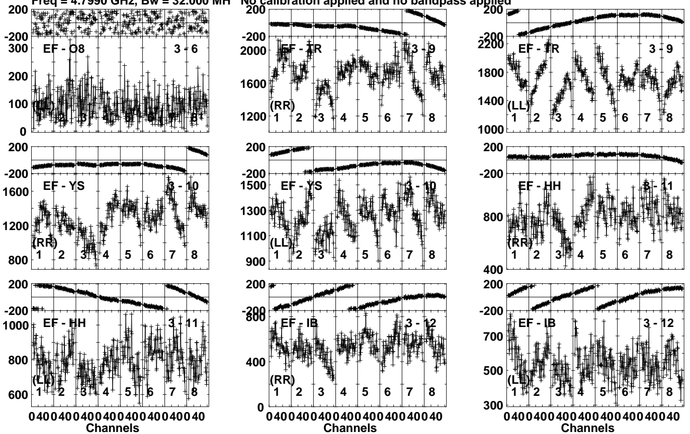
Lower frame: Micro Ampl Jy Top frame: Phas deg Vector averaged cross-power spectrum Several baselines displayed Timerange: 00/17:53:01 to 00/17:56:29
