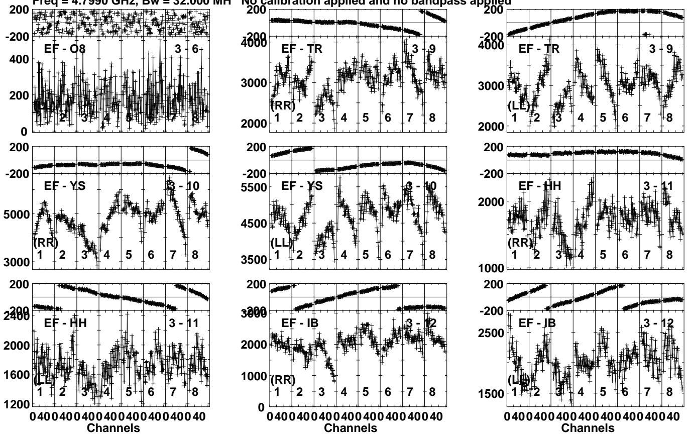
Lower frame: Micro Ampl Jy Top frame: Phas deg Vector averaged cross-power spectrum Several baselines displayed Timerange: 00/17:52:01 to 00/17:52:59
