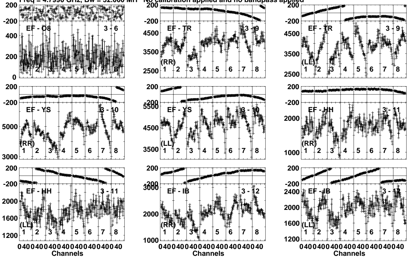
Lower frame: Micro Ampl Jy Top frame: Phas deg Vector averaged cross-power spectrum Several baselines displayed Timerange: 00/17:42:01 to 00/17:42:59
