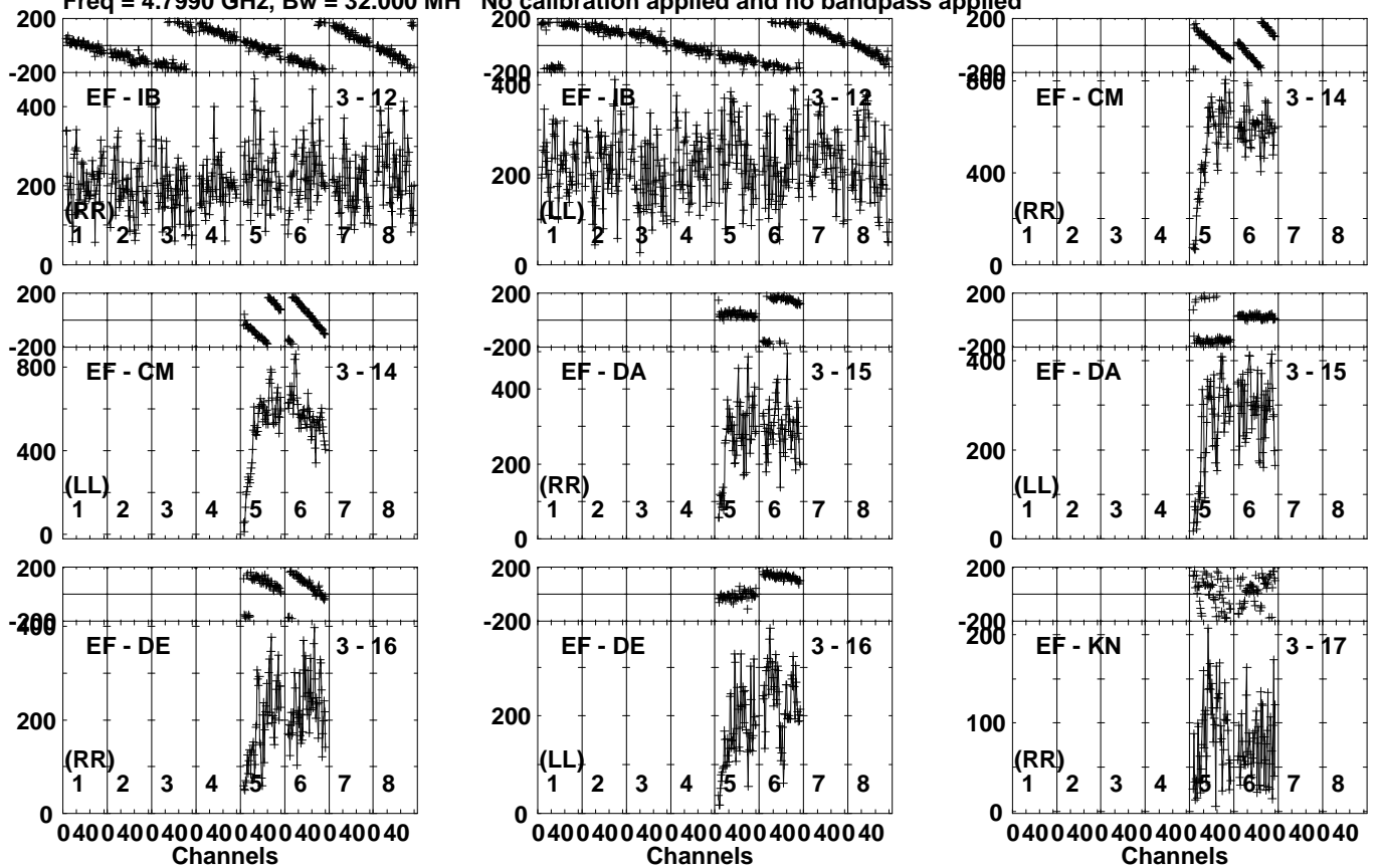
Lower frame: Micro Ampl Jy Top frame: Phas deg Vector averaged cross-power spectrum Several baselines displayed Timerange: 00/16:58:01 to 00/17:01:29
