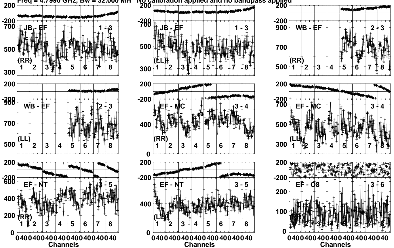
Lower frame: Micro Ampl Jy Top frame: Phas deg Vector averaged cross-power spectrum Several baselines displayed Timerange: 00/17:38:01 to 00/17:41:29
