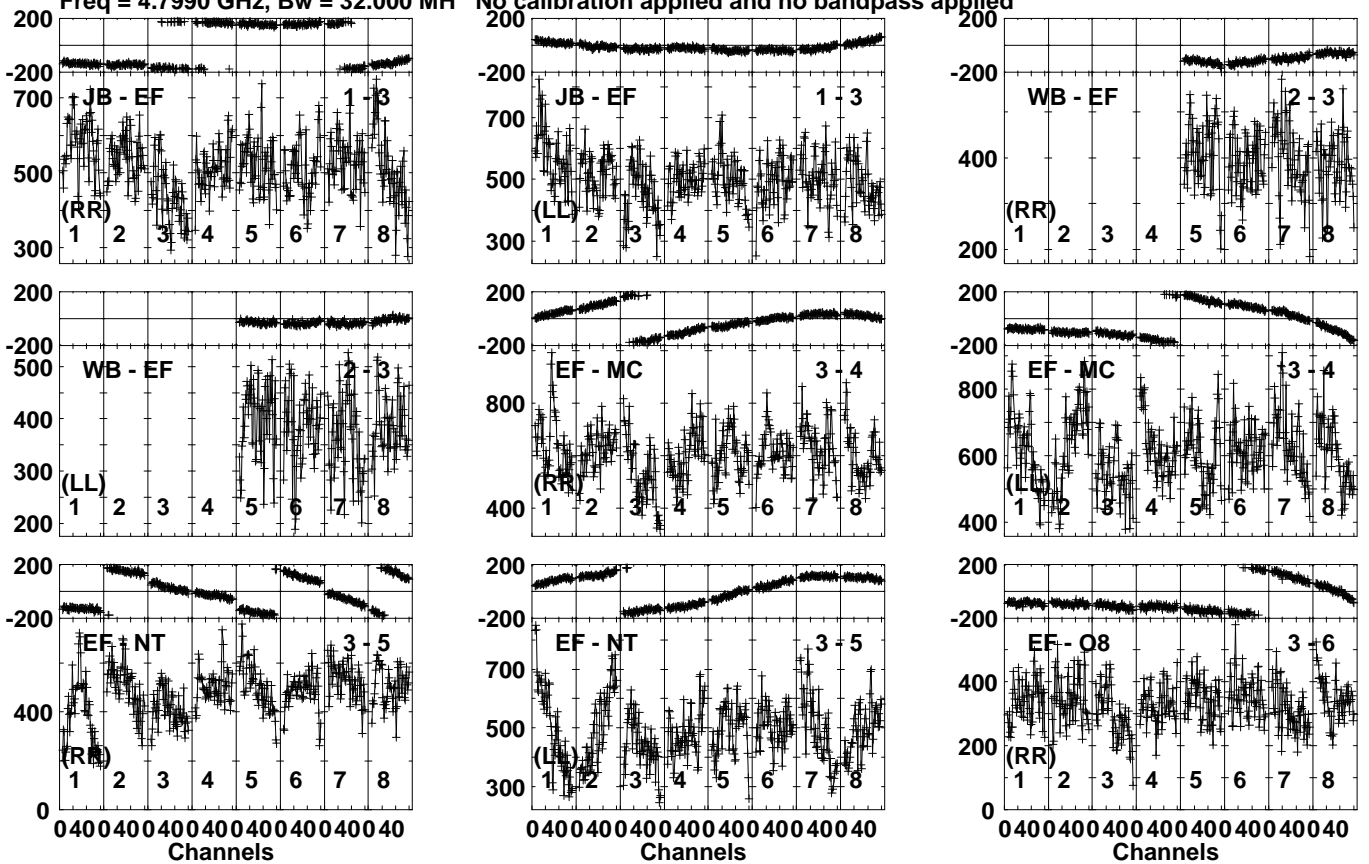
Lower frame: Micro Ampl Jy Top frame: Phas deg Vector averaged cross-power spectrum Several baselines displayed Timerange: 00/14:50:31 to 00/14:53:59
