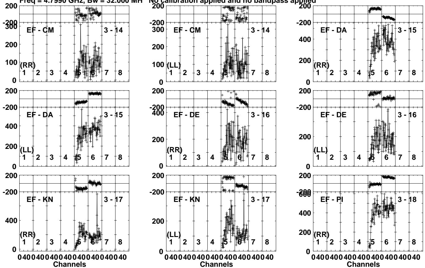
Lower frame: Micro Ampl Jy Top frame: Phas deg Vector averaged cross-power spectrum Several baselines displayed Timerange: 00:12:54:31 to 00:12:57:59
