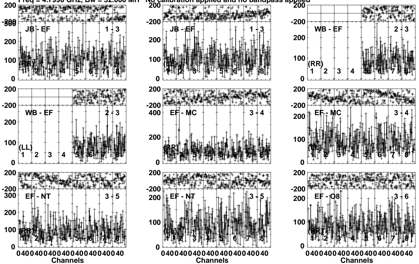
Lower frame: Micro Ampl Jy Top frame: Phas deg Vector averaged cross-power spectrum Several baselines displayed Timerange: 00/19:40:01 to 00/19:43:29
