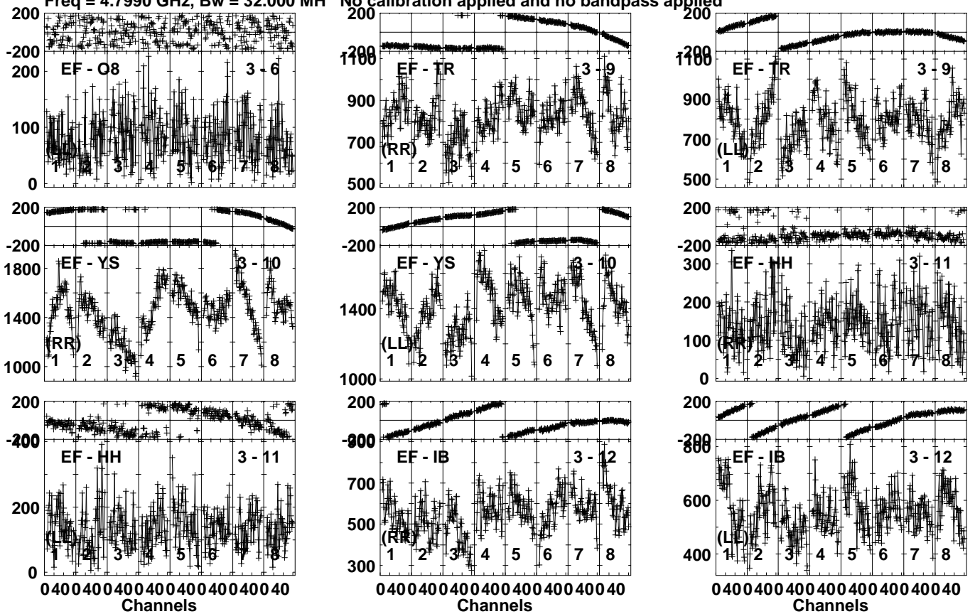
Lower frame: Micro Ampl Jy Top frame: Phas deg Vector averaged cross-power spectrum Several baselines displayed Timerange: 00/17:43:01 to 00/17:46:29
