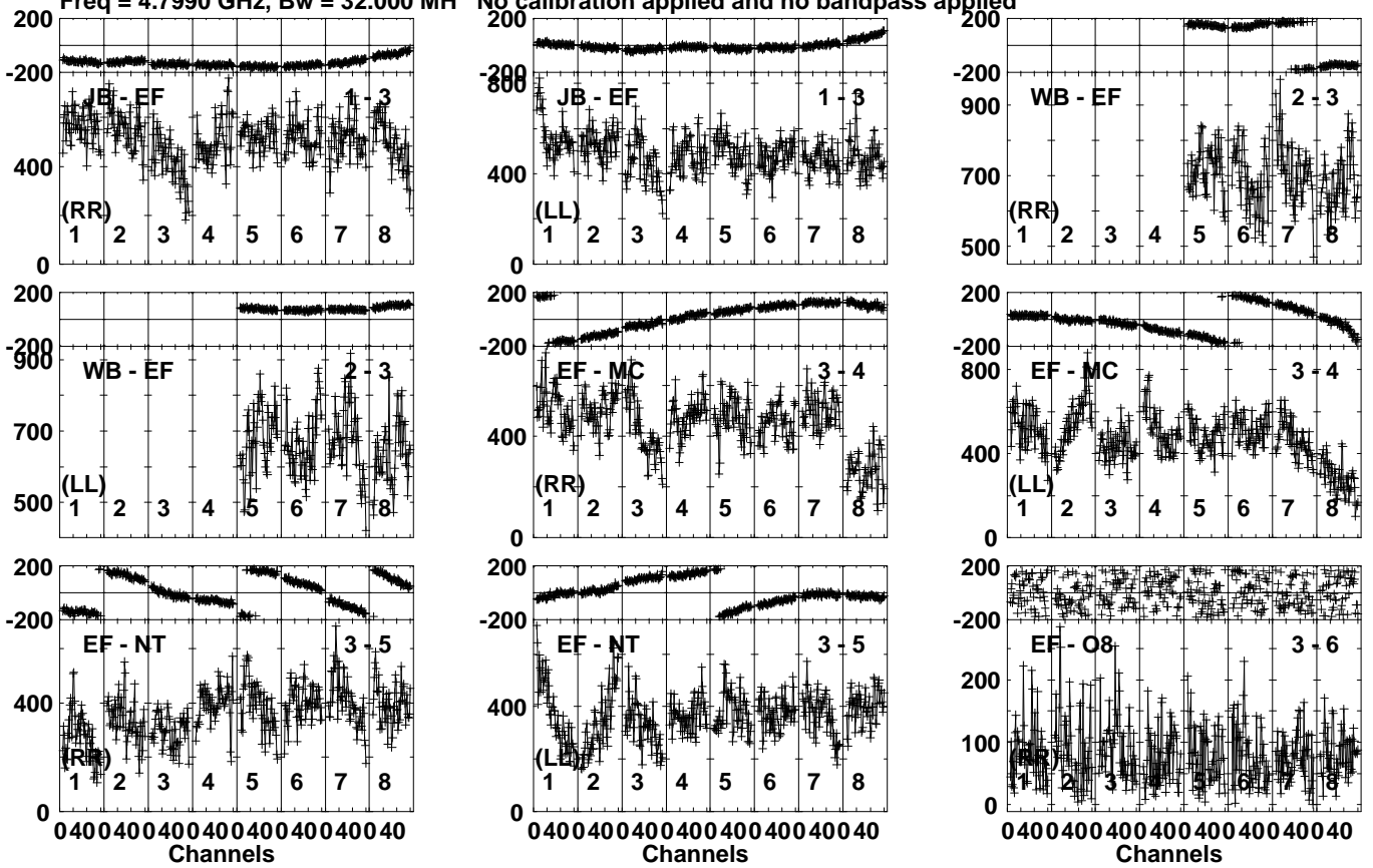
Lower frame: Micro Ampl Jy Top frame: Phas deg Vector averaged cross-power spectrum Several baselines displayed Timerange: 00/17:23:01 to 00/17:26:29
