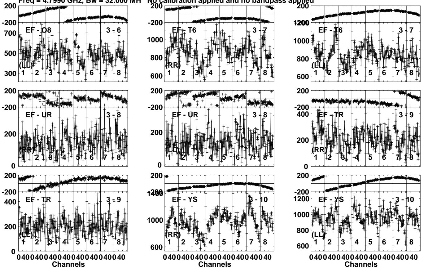
Lower frame: Micro Ampl Jy Top frame: Phas deg Vector averaged cross-power spectrum Several baselines displayed Timerange: 00/12:35:01 to 00/12:38:29
