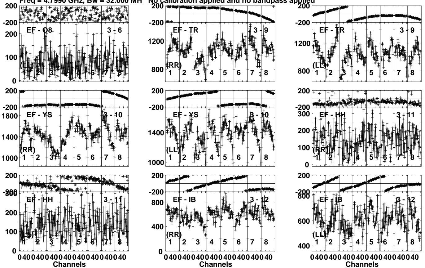
Lower frame: Micro Ampl Jy Top frame: Phas deg Vector averaged cross-power spectrum Several baselines displayed Timerange: 00/17:48:01 to 00/17:51:29
