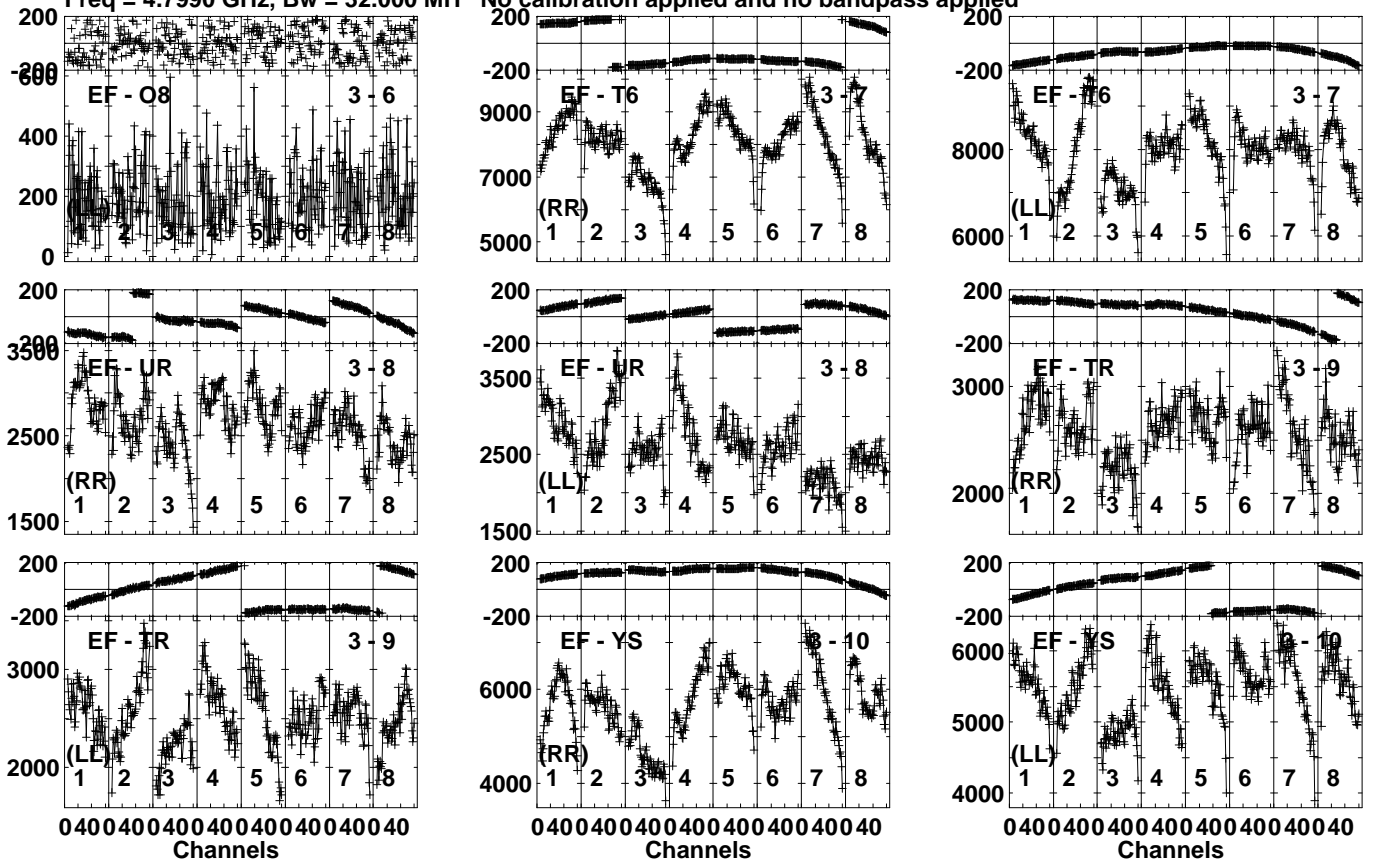
Lower frame: Micro Ampl Jy Top frame: Phas deg Vector averaged cross-power spectrum Several baselines displayed Timerange: 00/17:11:33 to 00/17:12:59
