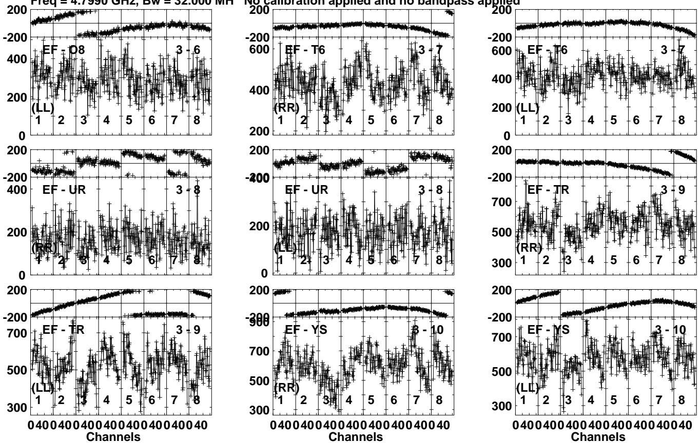
Lower frame: Micro Ampl Jy Top frame: Phas deg Vector averaged cross-power spectrum Several baselines displayed Timerange: 00/13:35:31 to 00/13:38:59
