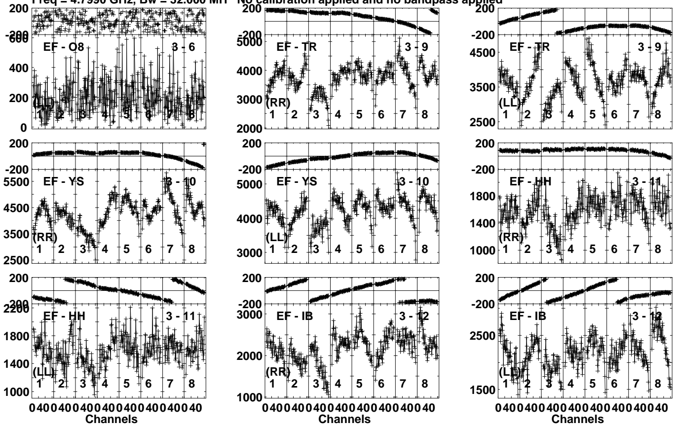
Lower frame: Micro Ampl Jy Top frame: Phas deg Vector averaged cross-power spectrum Several baselines displayed Timerange: 00/19:03:31 to 00/19:04:59
