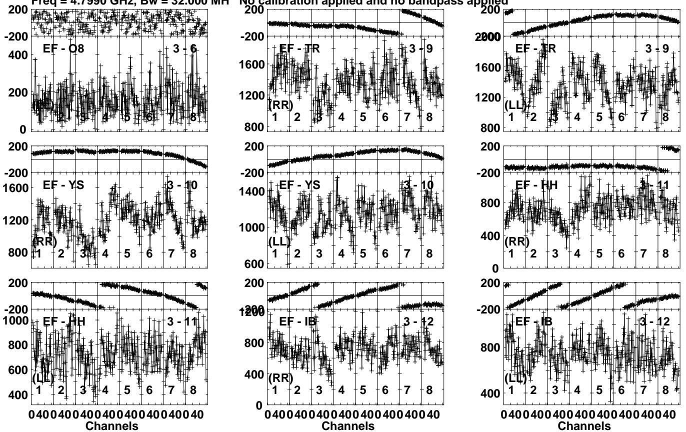
Lower frame: Micro Ampl Jy Top frame: Phas deg Vector averaged cross-power spectrum Several baselines displayed Timerange: 00/18:40:01 to 00/18:41:29
