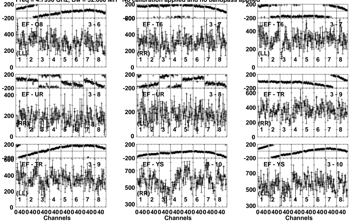
Lower frame: Micro Ampl Jy Top frame: Phas deg Vector averaged cross-power spectrum Several baselines displayed Timerange: 00:14:10:31 to 00:14:13:59
