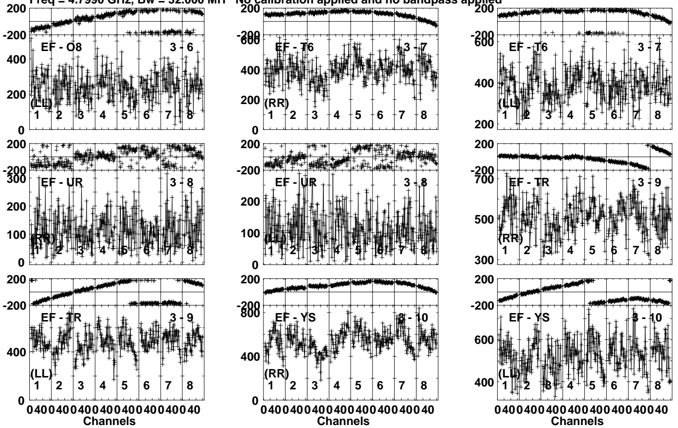
Lower frame: Micro Ampl Jy Top frame: Phas deg Vector averaged cross-power spectrum Several baselines displayed Timerange: 00:12:59:31 to 00:13:02:59
