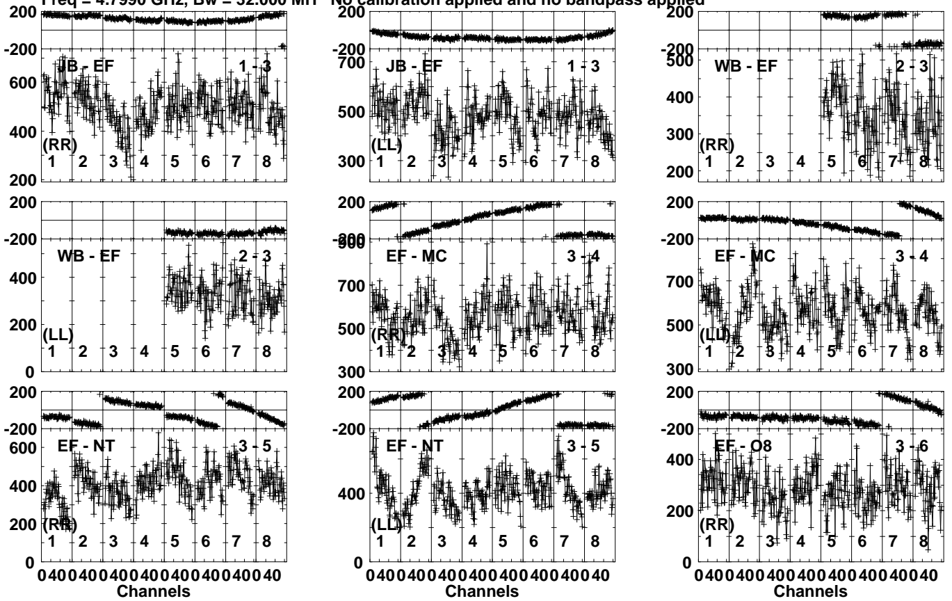
Lower frame: Micro Ampl Jy Top frame: Phas deg Vector averaged cross-power spectrum Several baselines displayed Timerange: 00/13:04:31 to 00/13:07:59
