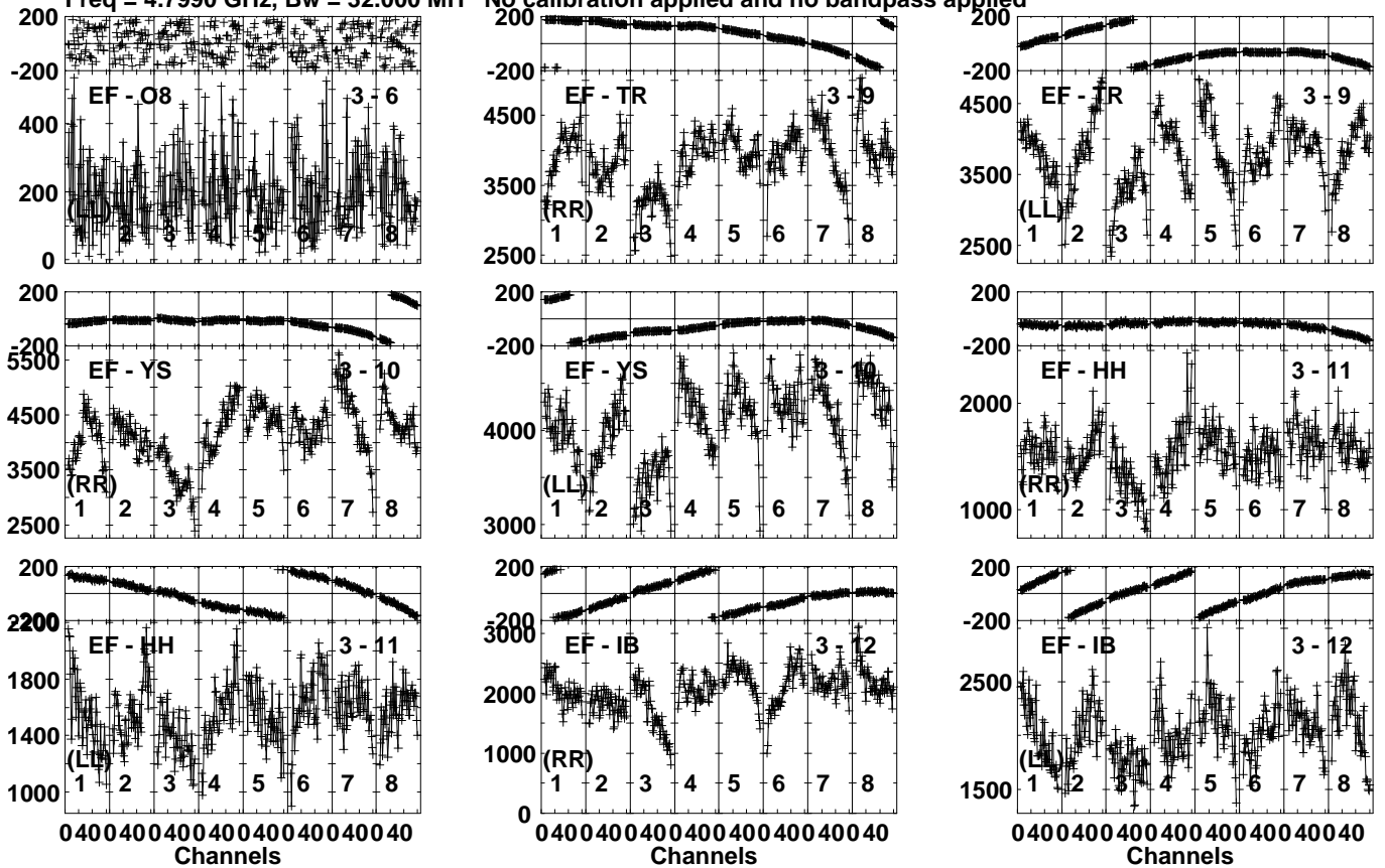
Lower frame: Micro Ampl Jy Top frame: Phas deg Vector averaged cross-power spectrum Several baselines displayed Timerange: 00/19:23:31 to 00/19:24:59
