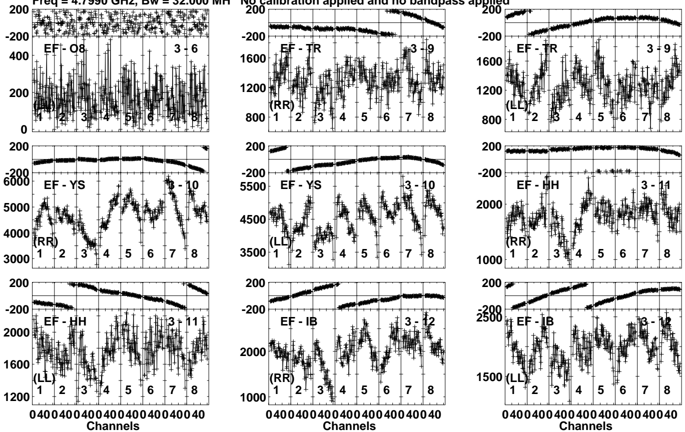
Lower frame: Micro Ampl Jy Top frame: Phas deg Vector averaged cross-power spectrum Several baselines displayed Timerange: 00/17:32:01 to 00/17:32:59
