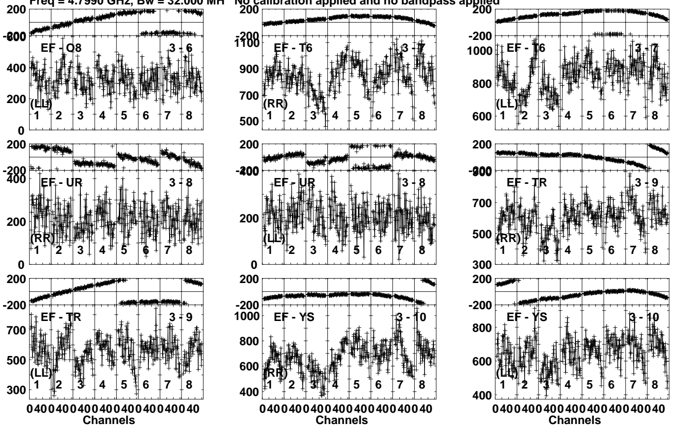
Lower frame: Micro Ampl Jy Top frame: Phas deg Vector averaged cross-power spectrum Several baselines displayed Timerange: 00/15:43:03 to 00/15:46:29
