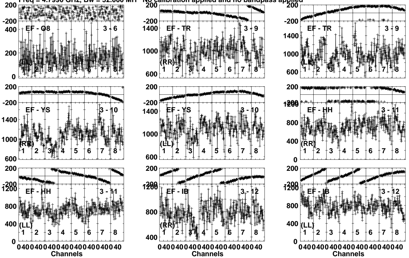
Lower frame: Micro Ampl Jy Top frame: Phas deg Vector averaged cross-power spectrum Several baselines displayed Timerange: 00/18:55:31 to 00/18:56:29
