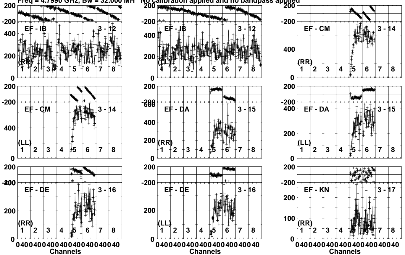
Lower frame: Micro Ampl Jy Top frame: Phas deg Vector averaged cross-power spectrum Several baselines displayed Timerange: 00/16:53:01 to 00/16:56:29
