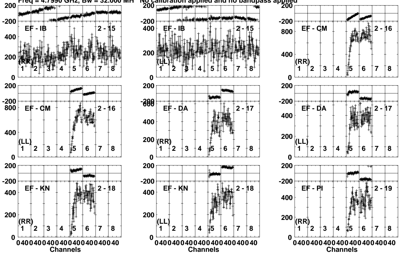
Lower frame: Micro Ampl Jy Top frame: Phas deg Vector averaged cross-power spectrum Several baselines displayed Timerange: 00/19:45:31 to 00/19:48:29
