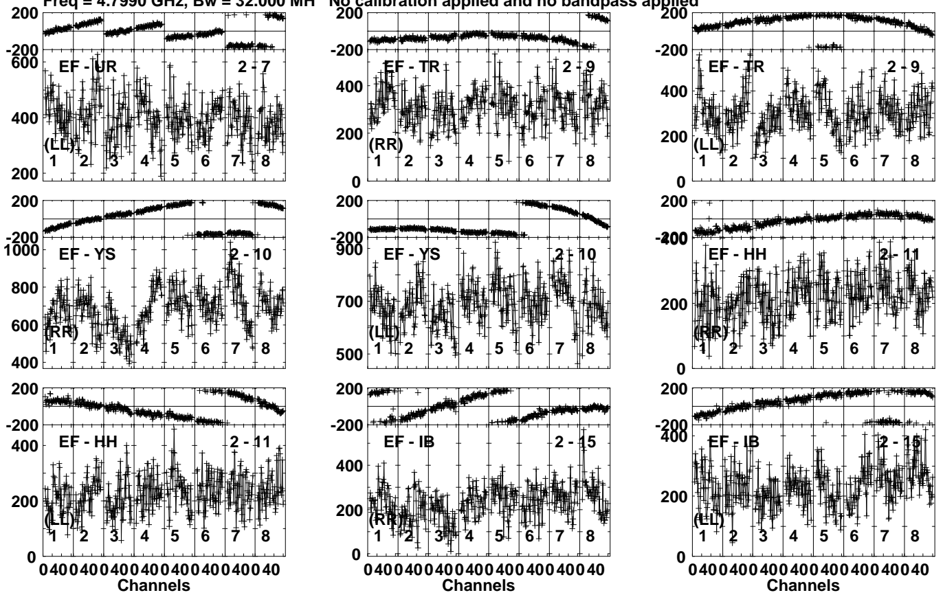
Lower frame: Micro Ampl Jy Top frame: Phas deg Vector averaged cross-power spectrum Several baselines displayed Timerange: 00/21:06:11 to 00/21:09:09
