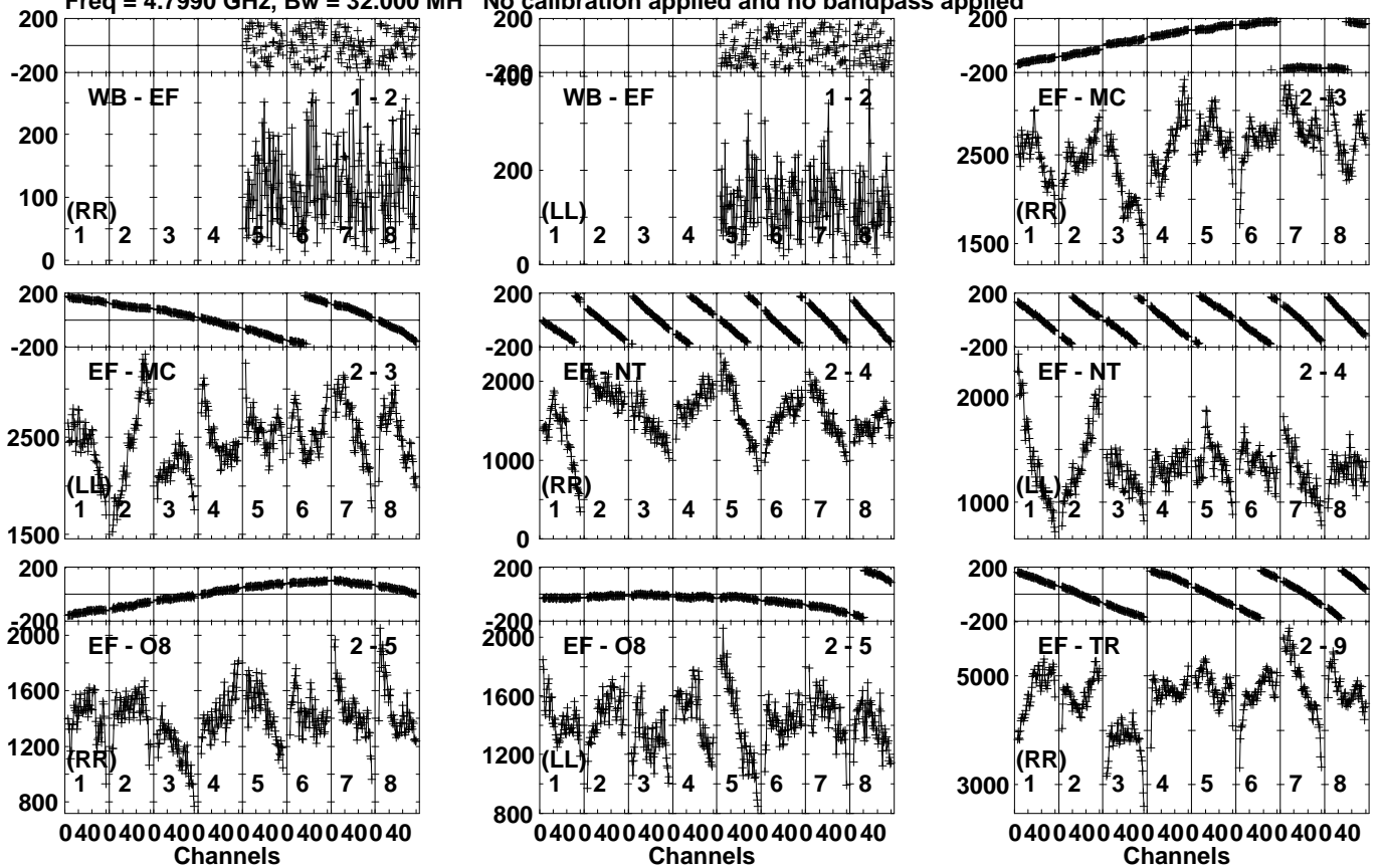
Lower frame: Micro Ampl Jy Top frame: Phas deg Vector averaged cross-power spectrum Several baselines displayed Timerange: 01/02:24:01 to 01/02:25:19
