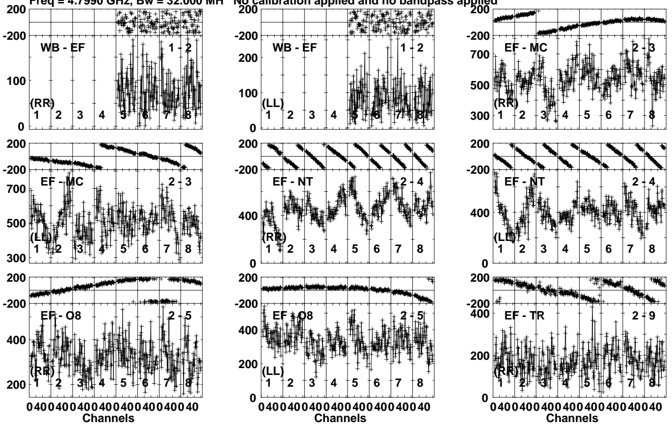
Lower frame: Micro Ampl Jy Top frame: Phas deg Vector averaged cross-power spectrum Several baselines displayed Timerange: 01/00:23:11 to 01/00:26:09
