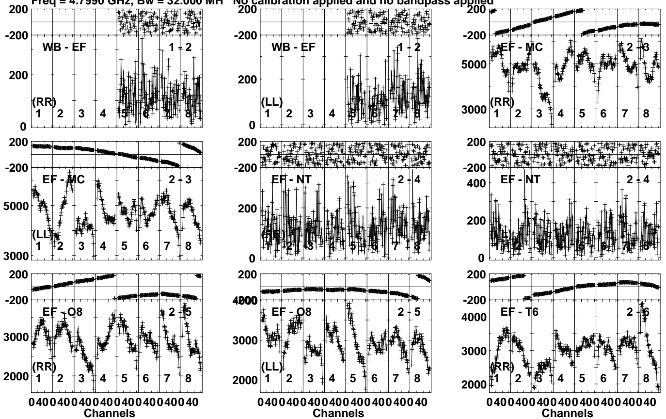
Lower frame: Micro Ampl Jy Top frame: Phas deg Vector averaged cross-power spectrum Several baselines displayed Timerange: 00/18:16:51 to 00/18:18:09
