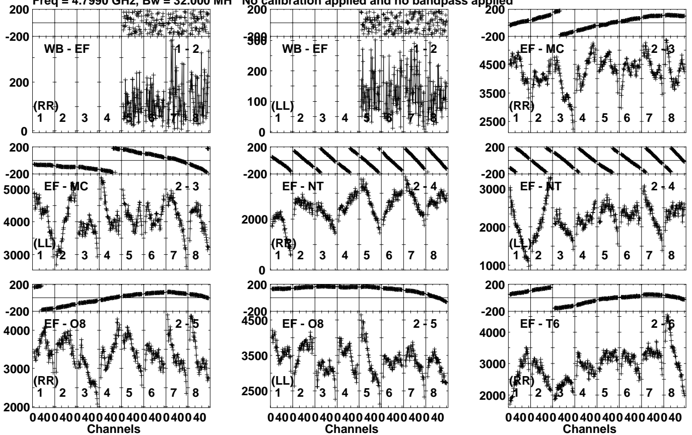
Lower frame: Micro Ampl Jy Top frame: Phas deg Vector averaged cross-power spectrum Several baselines displayed Timerange: 00/19:11:41 to 00/19:12:59
