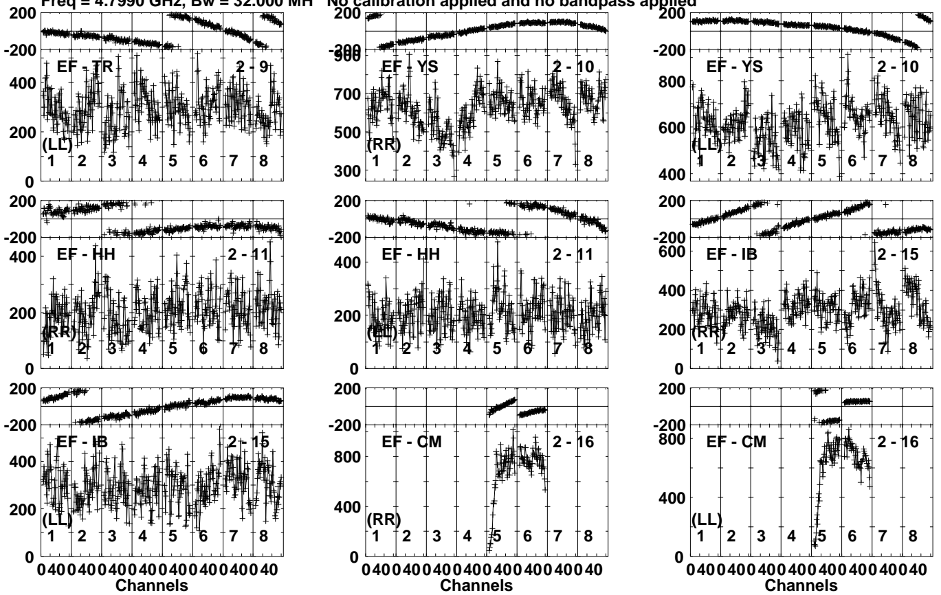
Lower frame: Micro Ampl Jy Top frame: Phas deg Vector averaged cross-power spectrum Several baselines displayed Timerange: 01/00:01:51 to 01/00:04:49
