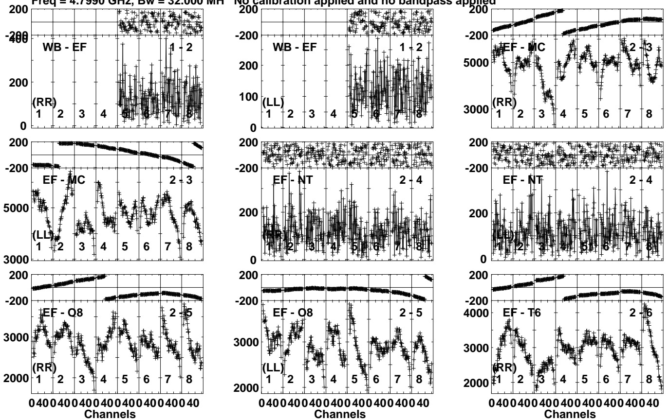
Lower frame: Micro Ampl Jy Top frame: Phas deg Vector averaged cross-power spectrum Several baselines displayed Timerange: 00/18:11:31 to 00/18:12:49
