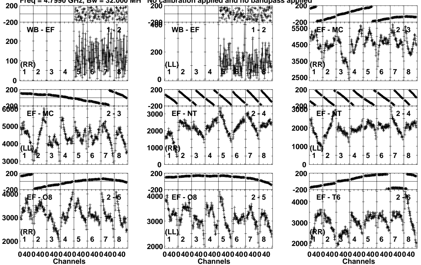
Lower frame: Micro Ampl Jy Top frame: Phas deg Vector averaged cross-power spectrum Several baselines displayed Timerange: 00:18:50:21 to 00:18:51:39
