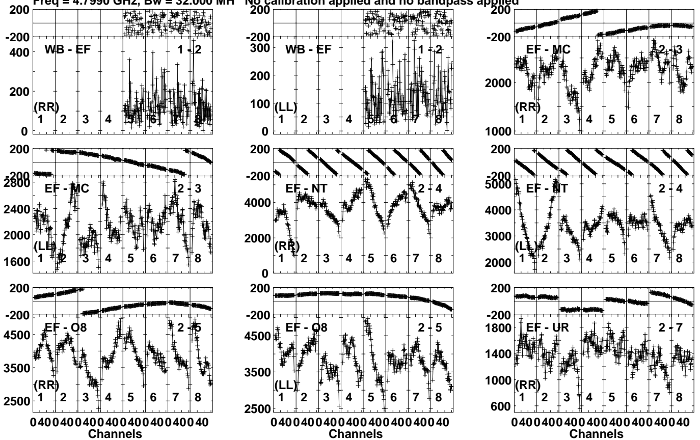
Lower frame: Micro Ampl Jy Top frame: Phas deg Vector averaged cross-power spectrum Several baselines displayed Timerange: 00/21:47:01 to 00/21:48:19
