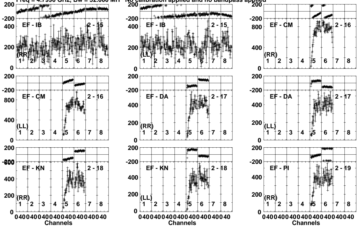
Lower frame: Micro Ampl Jy Top frame: Phas deg Vector averaged cross-power spectrum Several baselines displayed Timerange: 00/20:06:51 to 00/20:09:49
