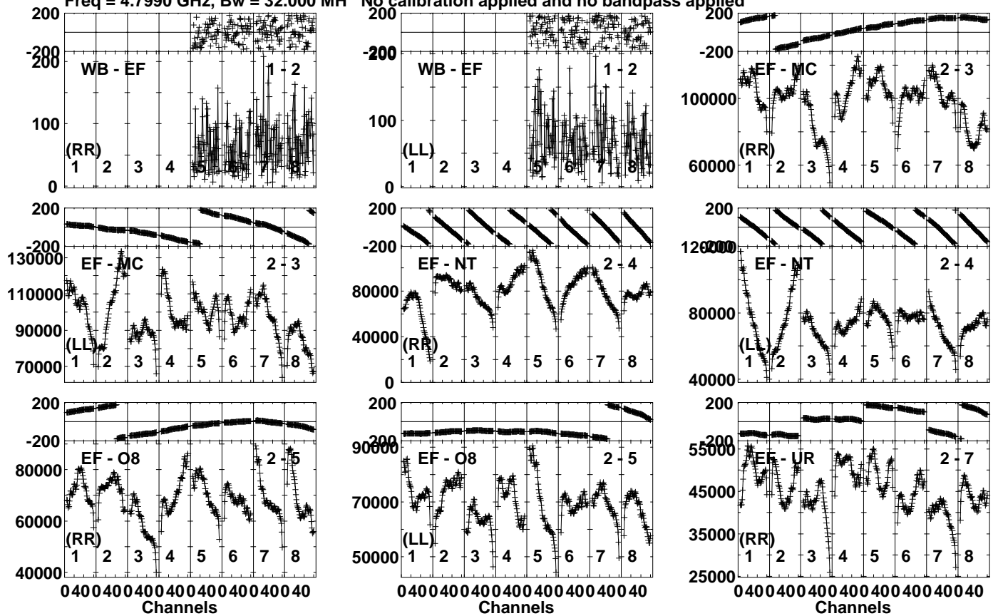
Lower frame: Micro Ampl Jy Top frame: Phas deg Vector averaged cross-power spectrum Several baselines displayed Timerange: 00/23:15:41 to 00/23:19:39
