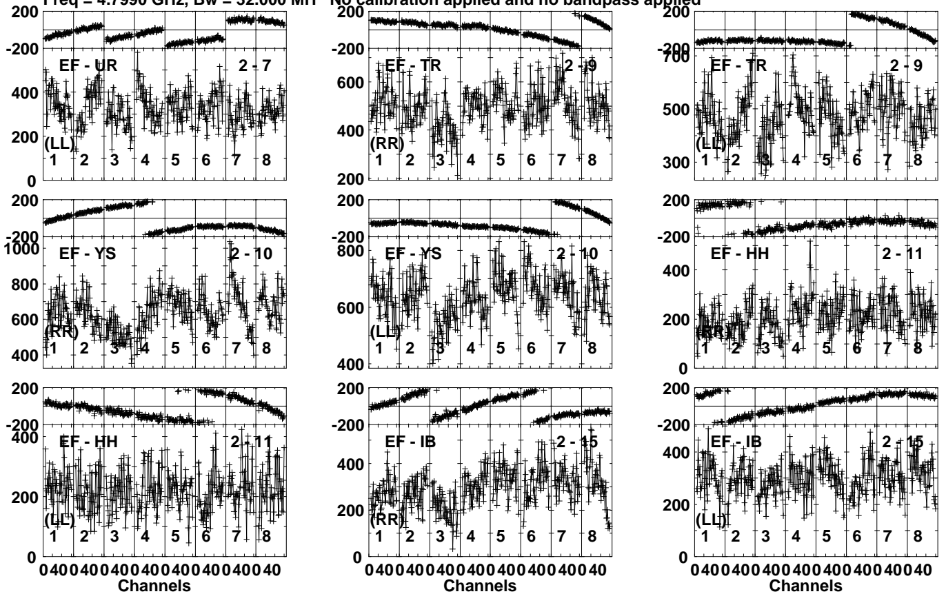
Lower frame: Micro Ampl Jy Top frame: Phas deg Vector averaged cross-power spectrum Several baselines displayed Timerange: 00/22:36:51 to 00/22:39:49
