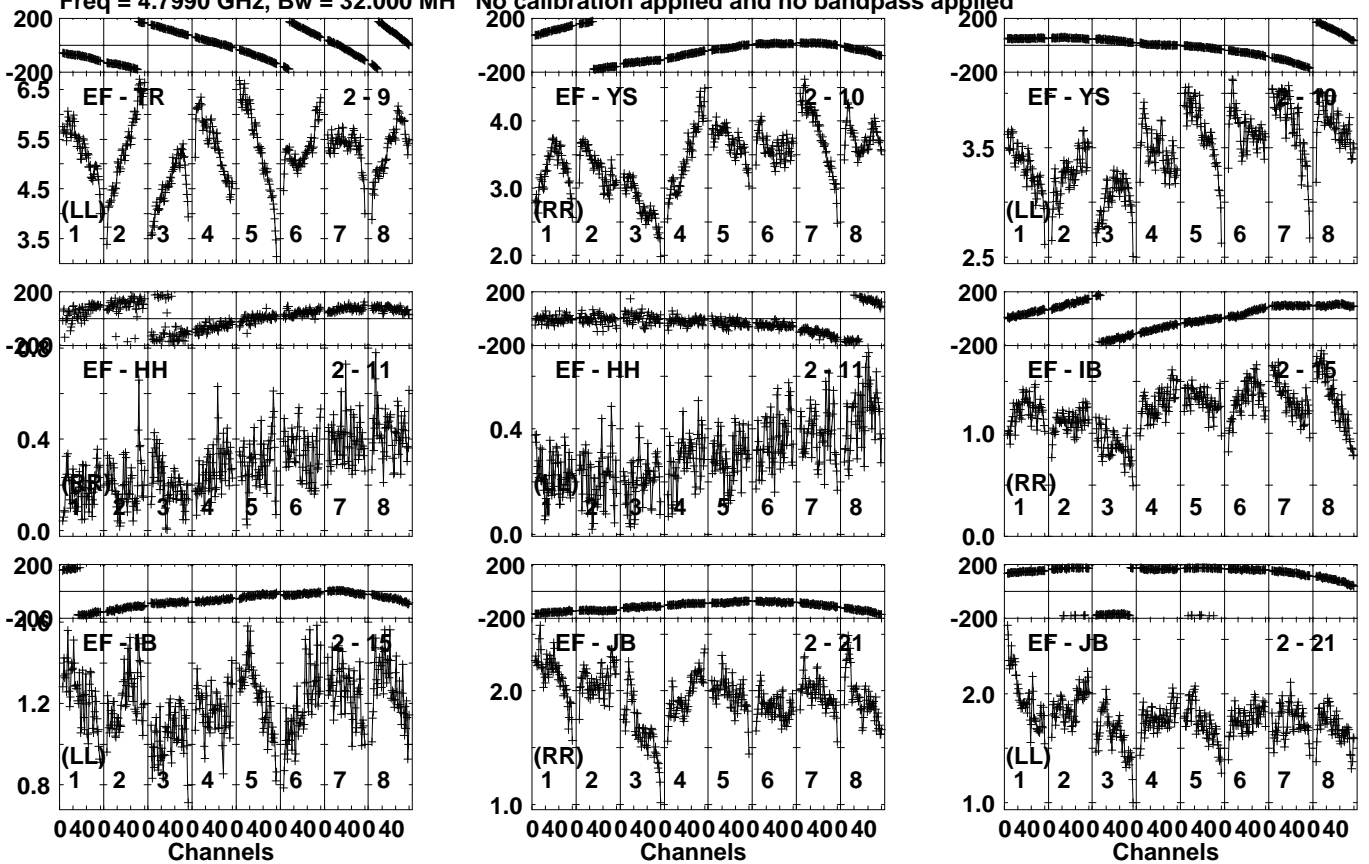
Lower frame: Milli Ampl Jy Top frame: Phas deg Vector averaged cross-power spectrum Several baselines displayed Timerange: 01/01:52:01 to 01/01:53:19
