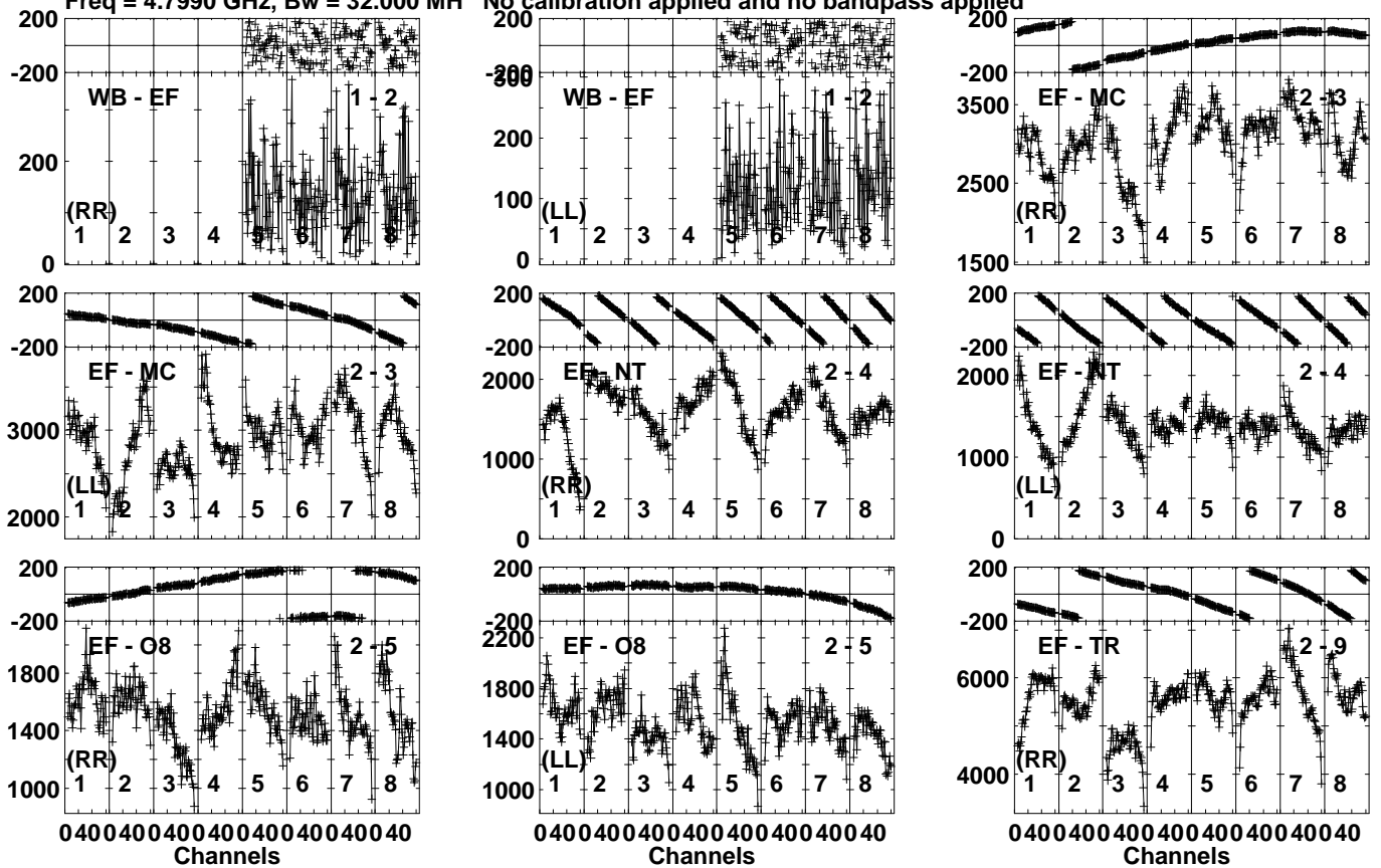
Lower frame: Micro Ampl Jy Top frame: Phas deg Vector averaged cross-power spectrum Several baselines displayed Timerange: 01/00:53:21 to 01/00:54:39
