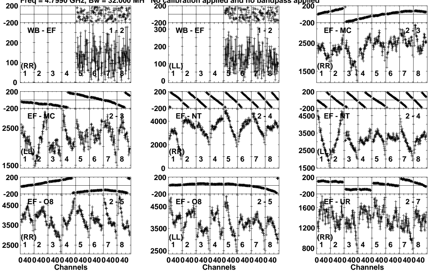
Lower frame: Micro Ampl Jy Top frame: Phas deg Vector averaged cross-power spectrum Several baselines displayed Timerange: 00/22:08:21 to 00/22:09:39
