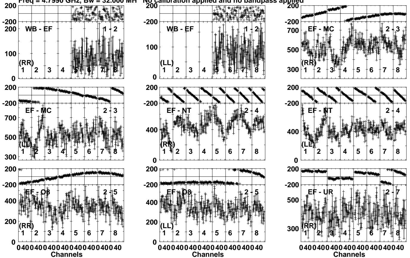
Lower frame: Micro Ampl Jy Top frame: Phas deg Vector averaged cross-power spectrum Several baselines displayed Timerange: 00/21:11:31 to 00/21:14:29
