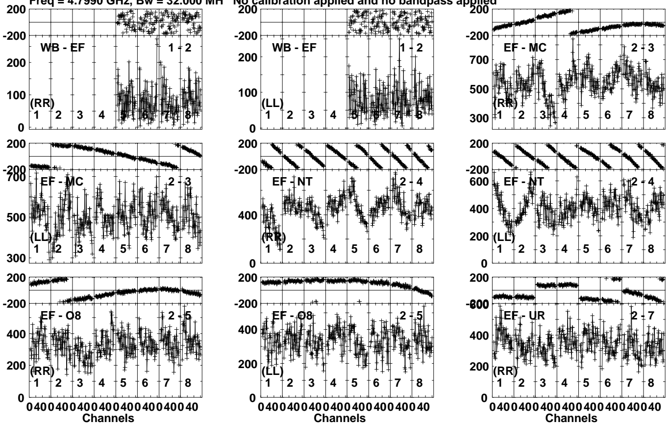
Lower frame: Micro Ampl Jy Top frame: Phas deg Vector averaged cross-power spectrum Several baselines displayed Timerange: 00/21:48:51 to 00/21:51:49
