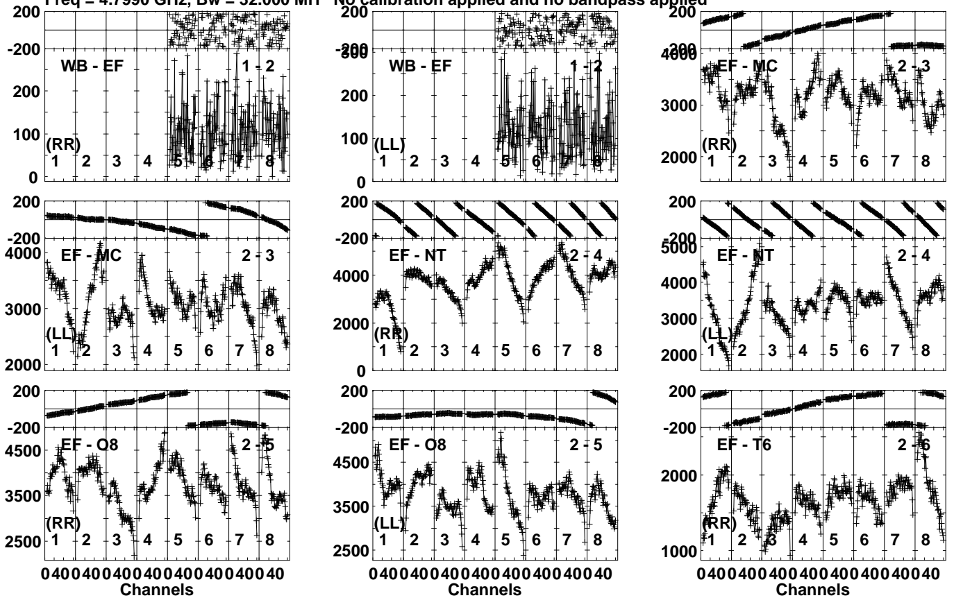
Lower frame: Micro Ampl Jy Top frame: Phas deg Vector averaged cross-power spectrum Several baselines displayed Timerange: 00/20:10:21 to 00/20:11:39
