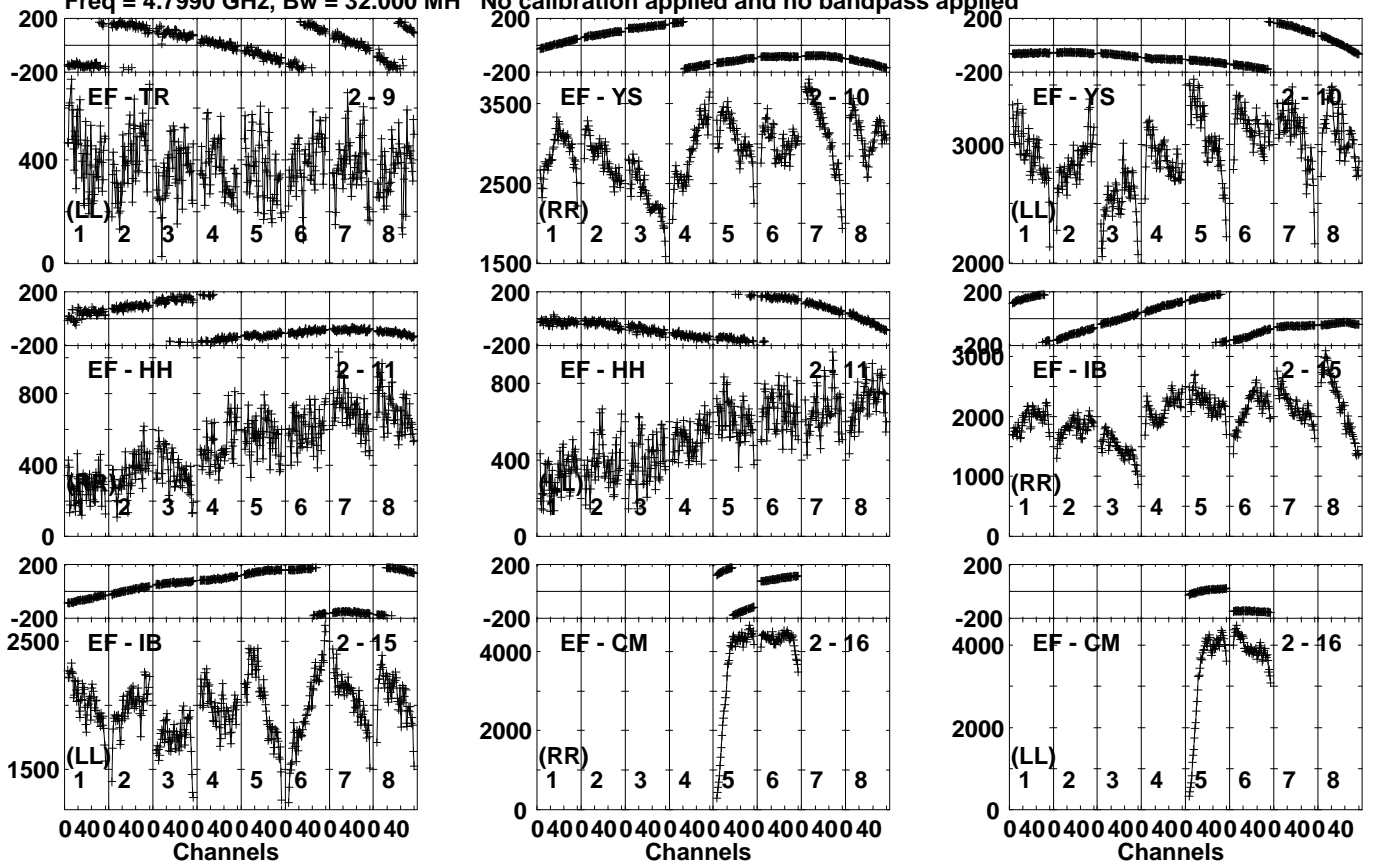
Lower frame: Micro Ampl Jy Top frame: Phas deg Vector averaged cross-power spectrum Several baselines displayed Timerange: 01/01:14:41 to 01/01:15:59
