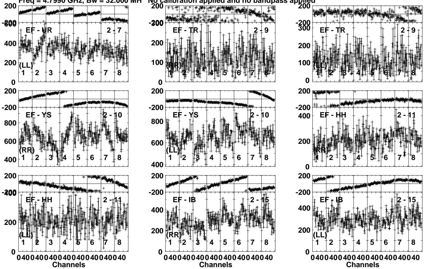
Lower frame: Micro Ampl Jy Top frame: Phas deg Vector averaged cross-power spectrum Several baselines displayed Timerange: 00/22:31:31 to 00/22:34:29
