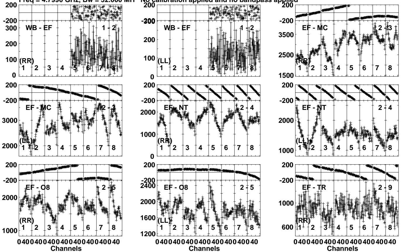
Lower frame: Micro Ampl Jy Top frame: Phas deg Vector averaged cross-power spectrum Several baselines displayed Timerange: 01/00:32:01 to 01/00:33:19
