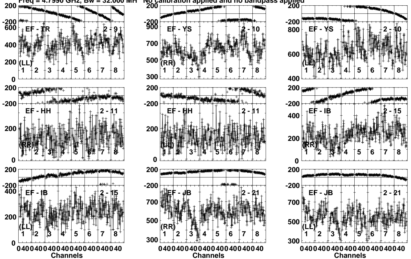
Lower frame: Micro Ampl Jy Top frame: Phas deg Vector averaged cross-power spectrum Several baselines displayed Timerange: 01/01:27:11 to 01/01:30:09
