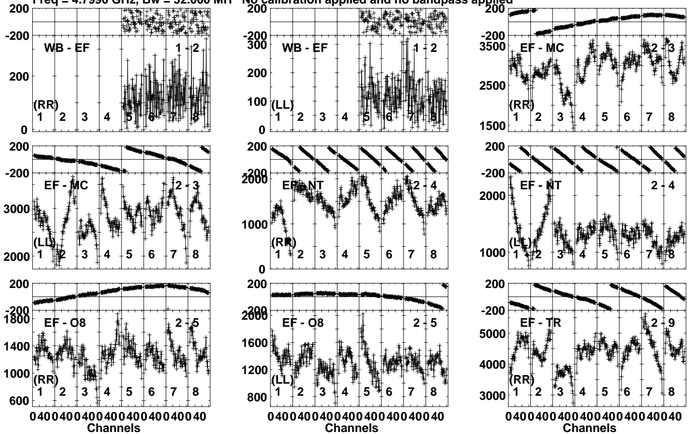
Lower frame: Micro Ampl Jy Top frame: Phas deg Vector averaged cross-power spectrum Several baselines displayed Timerange: 01/01:30:41 to 01/01:31:59
