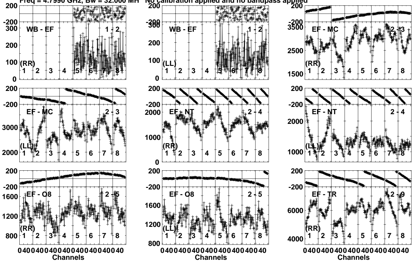
Lower frame: Micro Ampl Jy Top frame: Phas deg Vector averaged cross-power spectrum Several baselines displayed Timerange: 01/01:36:01 to 01/01:37:19
