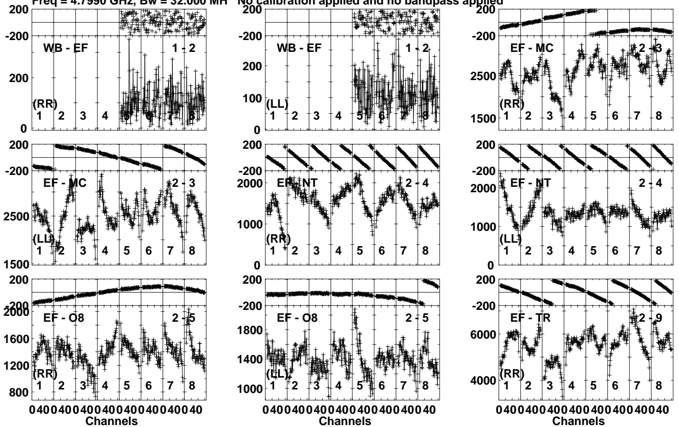
Lower frame: Micro Ampl Jy Top frame: Phas deg Vector averaged cross-power spectrum Several baselines displayed Timerange: 01/02:18:41 to 01/02:19:59
