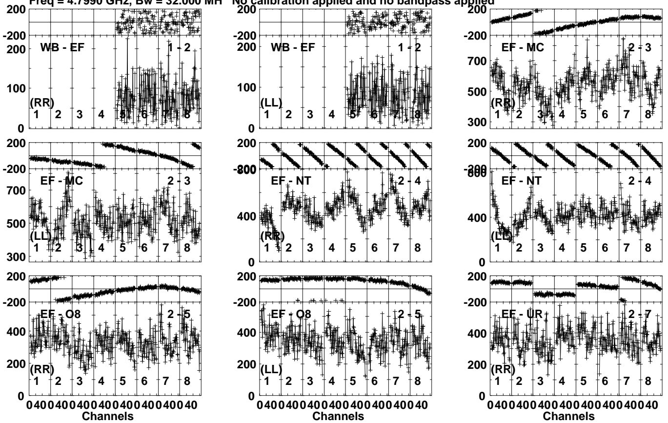
Lower frame: Micro Ampl Jy Top frame: Phas deg Vector averaged cross-power spectrum Several baselines displayed Timerange: 00/21:38:11 to 00/21:41:09
