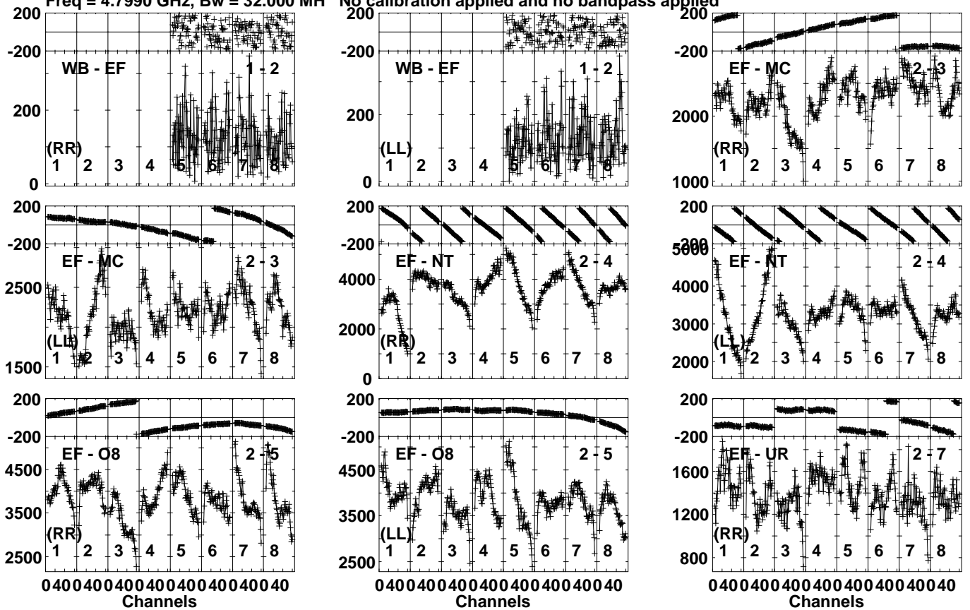
Lower frame: Micro Ampl Jy Top frame: Phas deg Vector averaged cross-power spectrum Several baselines displayed Timerange: 00/21:57:41 to 00/21:58:59
