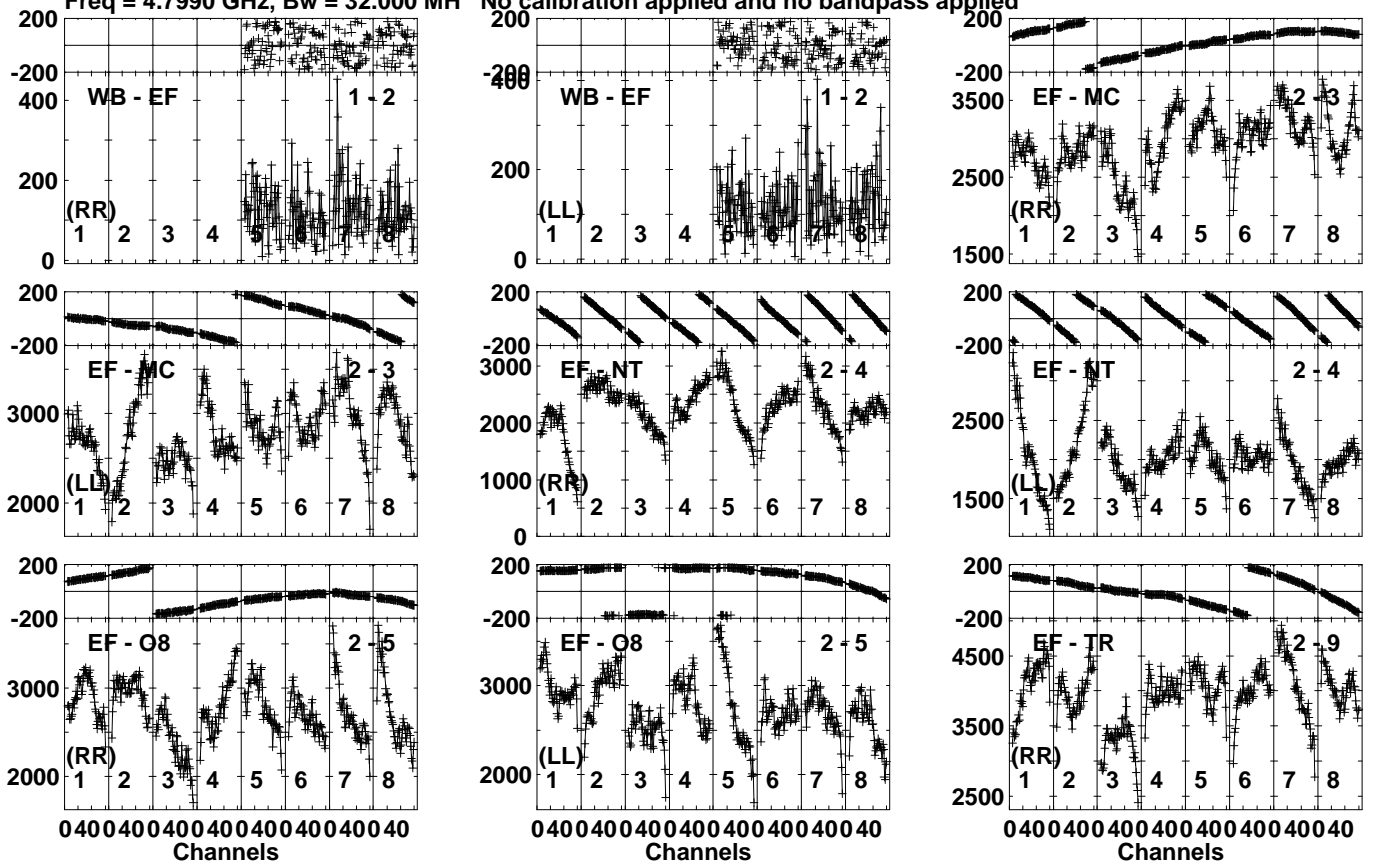
Lower frame: Micro Ampl Jy Top frame: Phas deg Vector averaged cross-power spectrum Several baselines displayed Timerange: 00/23:33:21 to 00/23:34:39
