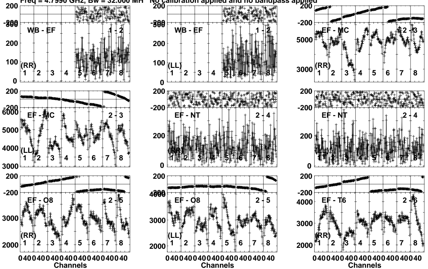
Lower frame: Micro Ampl Jy Top frame: Phas deg Vector averaged cross-power spectrum Several baselines displayed Timerange: 00/18:22:11 to 00/18:23:29
