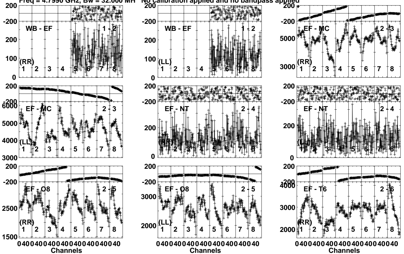
Lower frame: Micro Ampl Jy Top frame: Phas deg Vector averaged cross-power spectrum Several baselines displayed Timerange: 00/17:39:31 to 00/17:40:49
