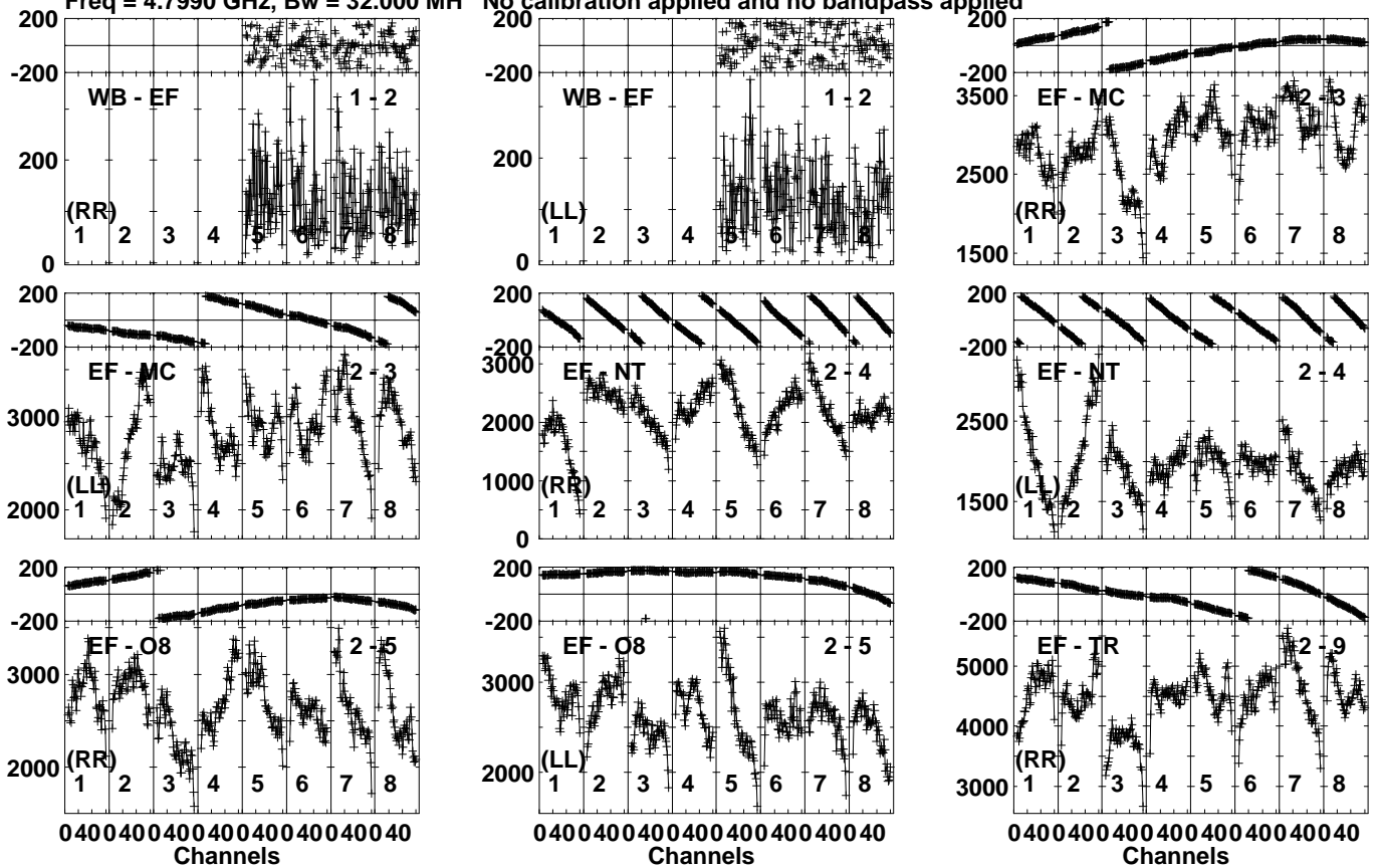
Lower frame: Micro Ampl Jy Top frame: Phas deg Vector averaged cross-power spectrum Several baselines displayed Timerange: 00/23:38:41 to 00/23:39:59
