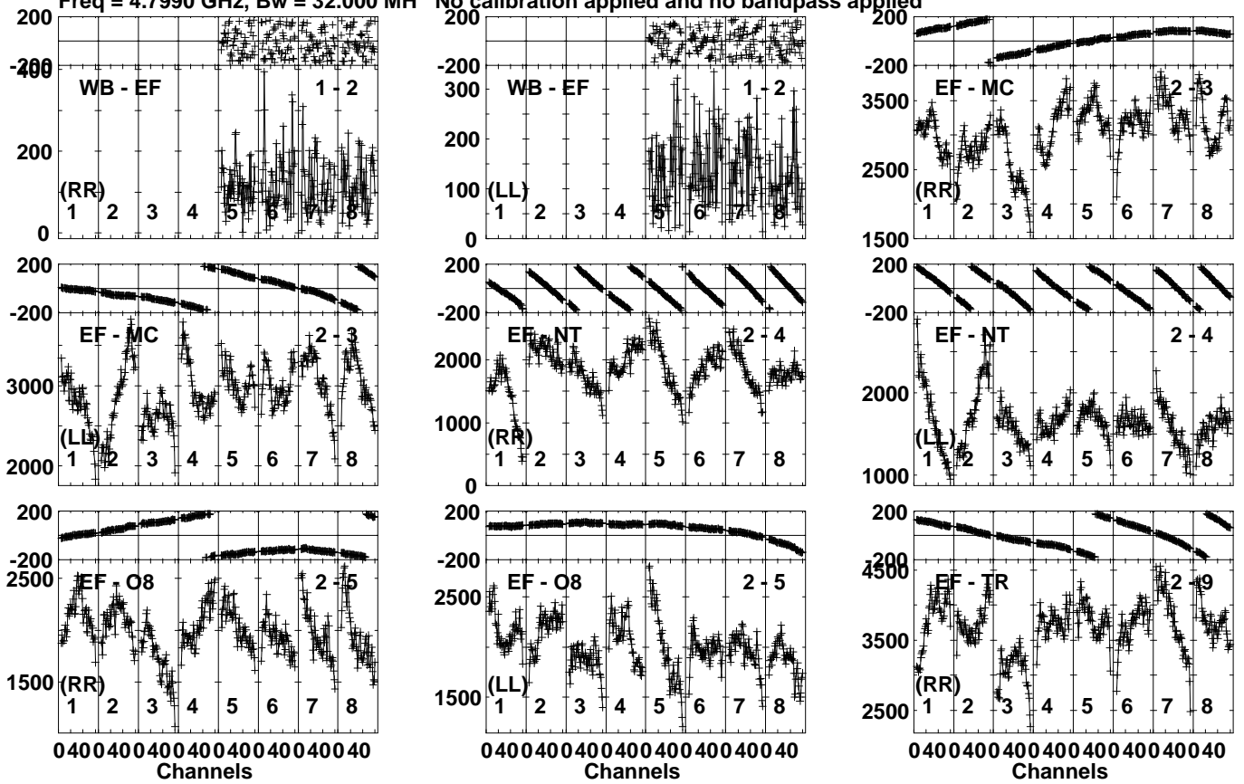
Lower frame: Micro Ampl Jy Top frame: Phas deg Vector averaged cross-power spectrum Several baselines displayed Timerange: 01/00:16:01 to 01/00:17:19
