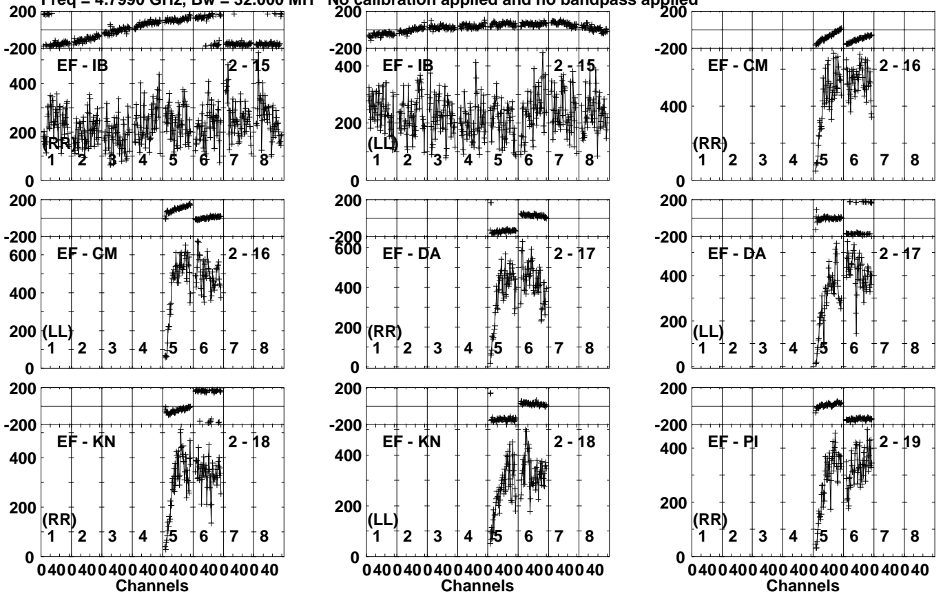
Lower frame: Micro Ampl Jy Top frame: Phas deg Vector averaged cross-power spectrum Several baselines displayed Timerange: 00/19:29:31 to 00/19:32:29
