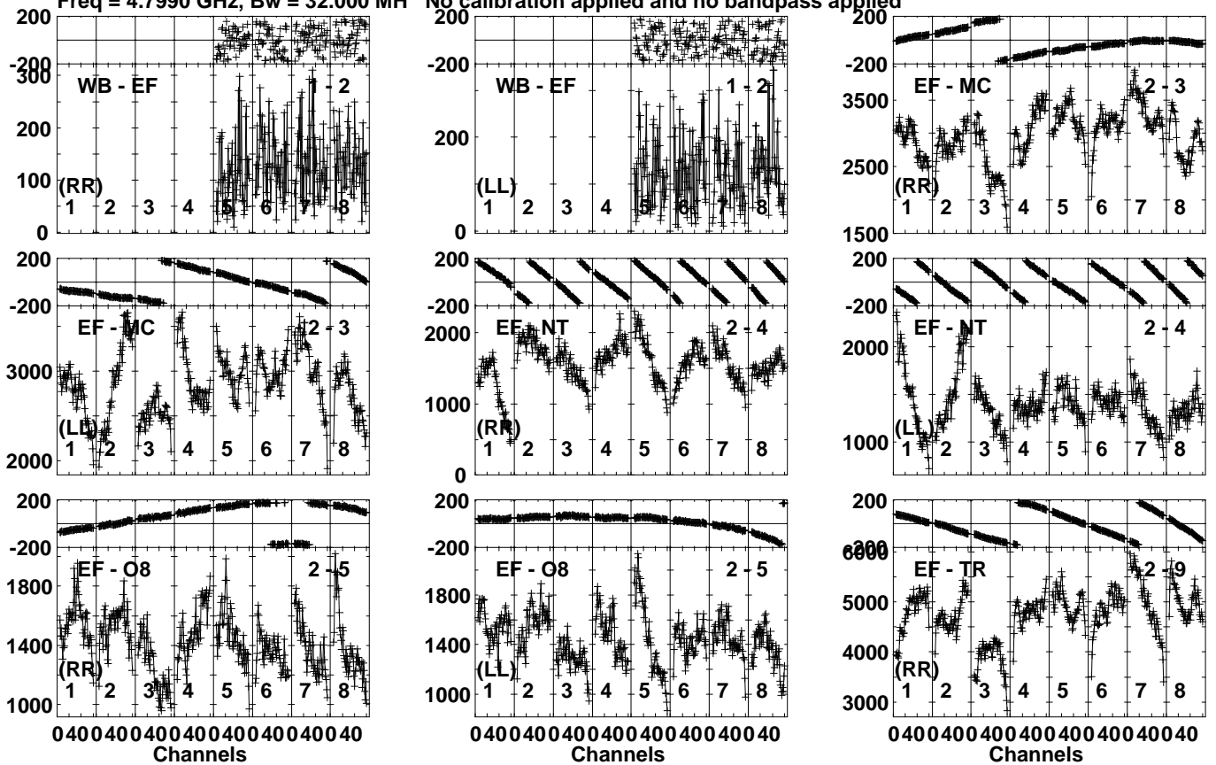
Lower frame: Micro Ampl Jy Top frame: Phas deg Vector averaged cross-power spectrum Several baselines displayed Timerange: 01/01:04:01 to 01/01:05:19
