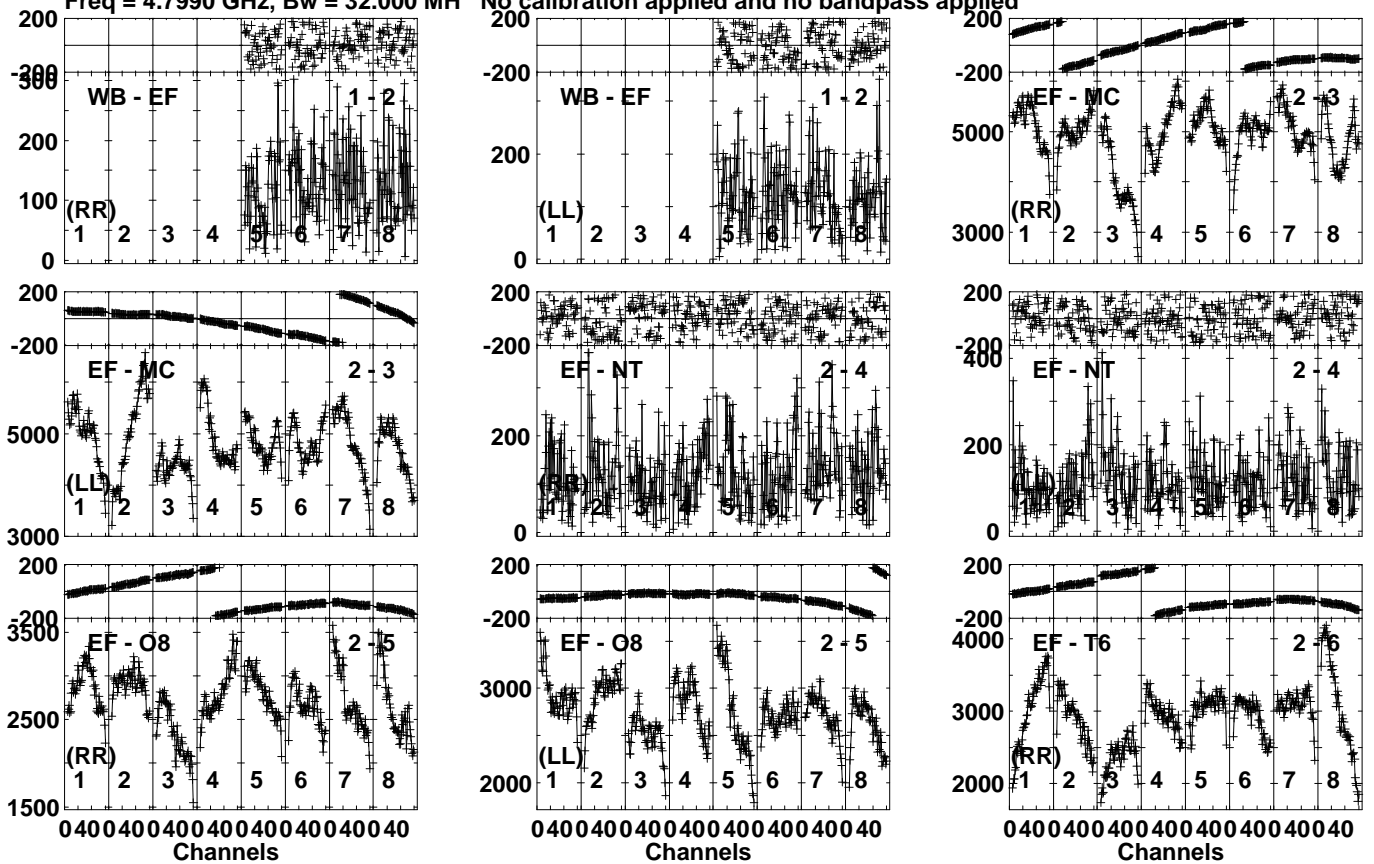
Lower frame: Micro Ampl Jy Top frame: Phas deg Vector averaged cross-power spectrum Several baselines displayed Timerange: 00/17:50:11 to 00/17:51:29
