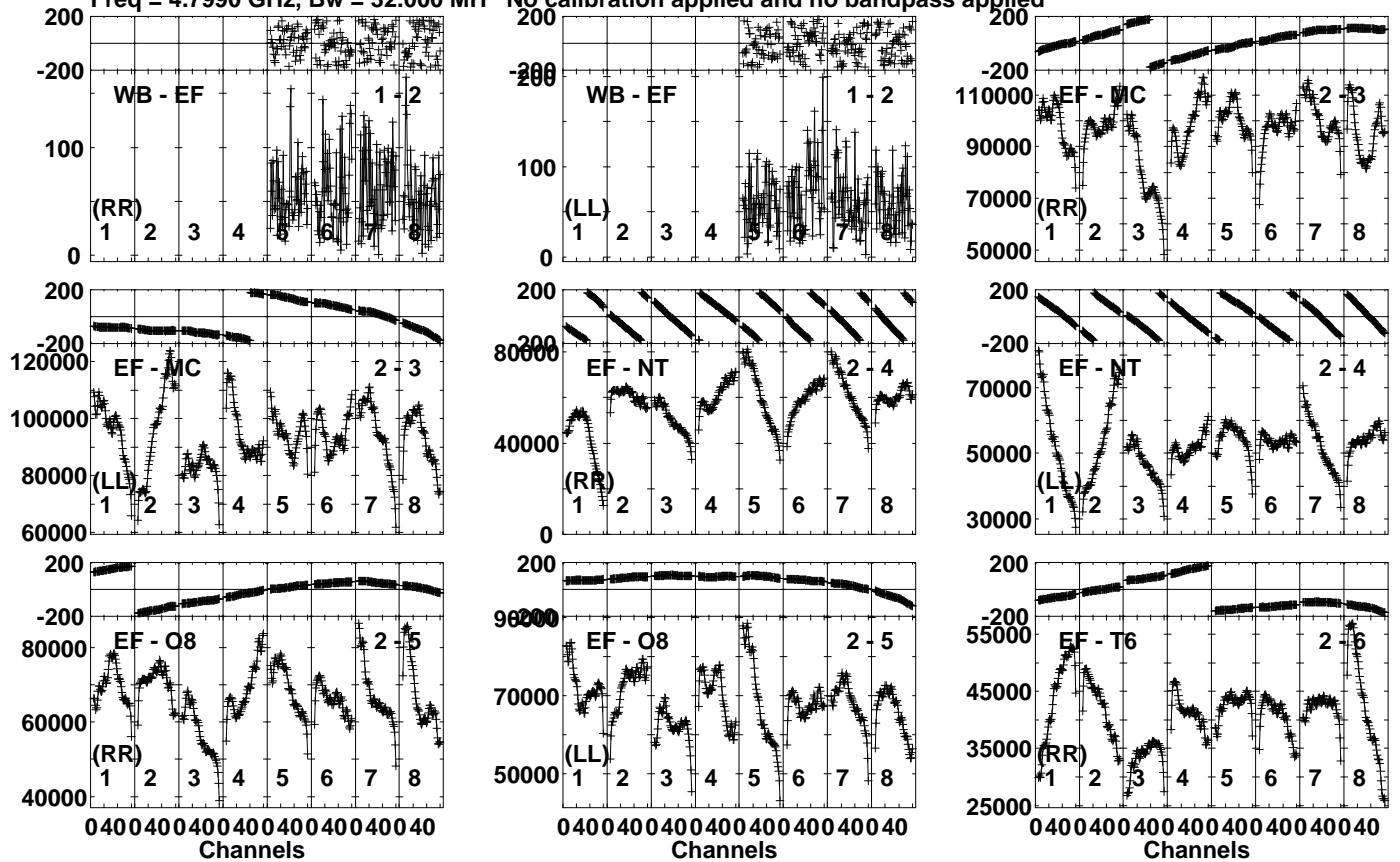
Lower frame: Micro Ampl Jy Top frame: Phas deg Vector averaged cross-power spectrum Several baselines displayed Timerange: 00/18:26:21 to 00/18:31:19
