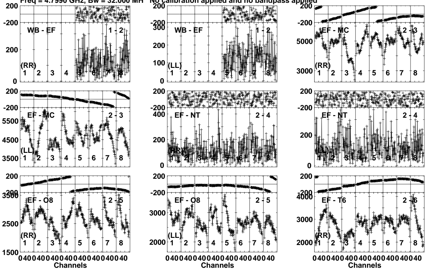
Lower frame: Micro Ampl Jy Top frame: Phas deg Vector averaged cross-power spectrum Several baselines displayed Timerange: 00/17:44:51 to 00/17:46:09
