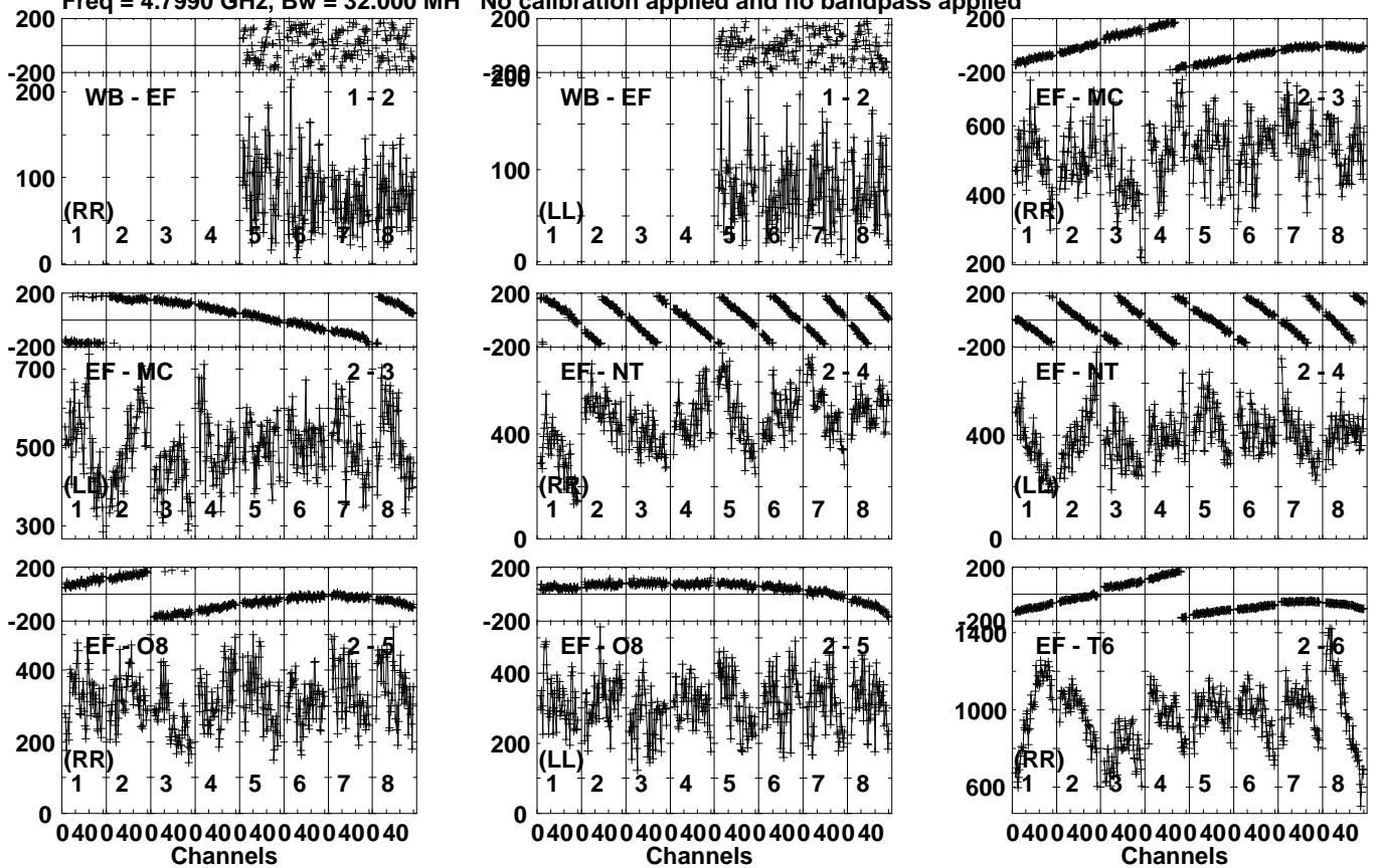
Lower frame: Micro Ampl Jy Top frame: Phas deg Vector averaged cross-power spectrum Several baselines displayed Timerange: 00/19:56:11 to 00/19:59:09
