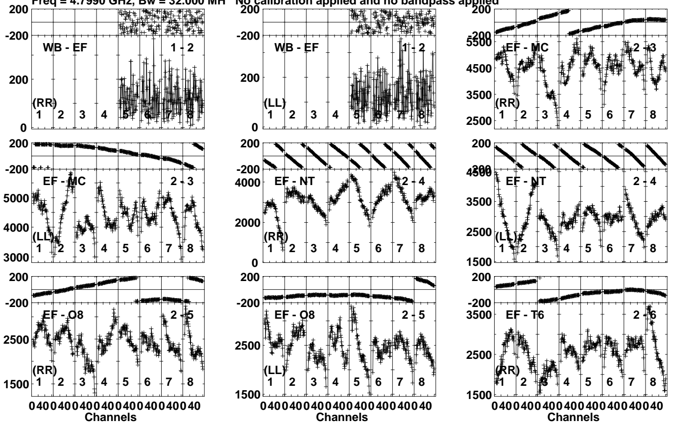
Lower frame: Micro Ampl Jy Top frame: Phas deg Vector averaged cross-power spectrum Several baselines displayed Timerange: 00/17:28:51 to 00/17:30:09
