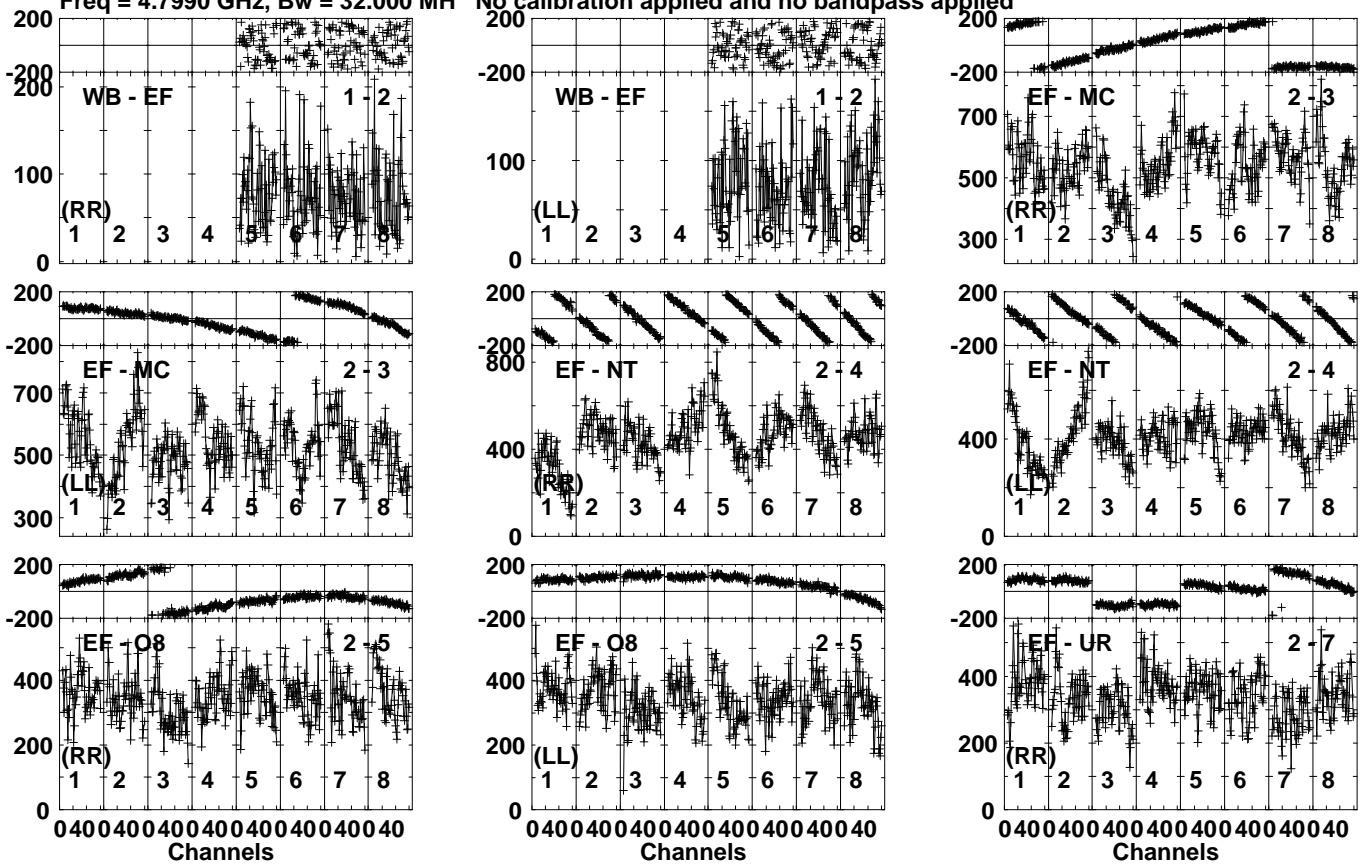
Lower frame: Micro Ampl Jy Top frame: Phas deg Vector averaged cross-power spectrum Several baselines displayed Timerange: 00/21:59:31 to 00/22:02:29
