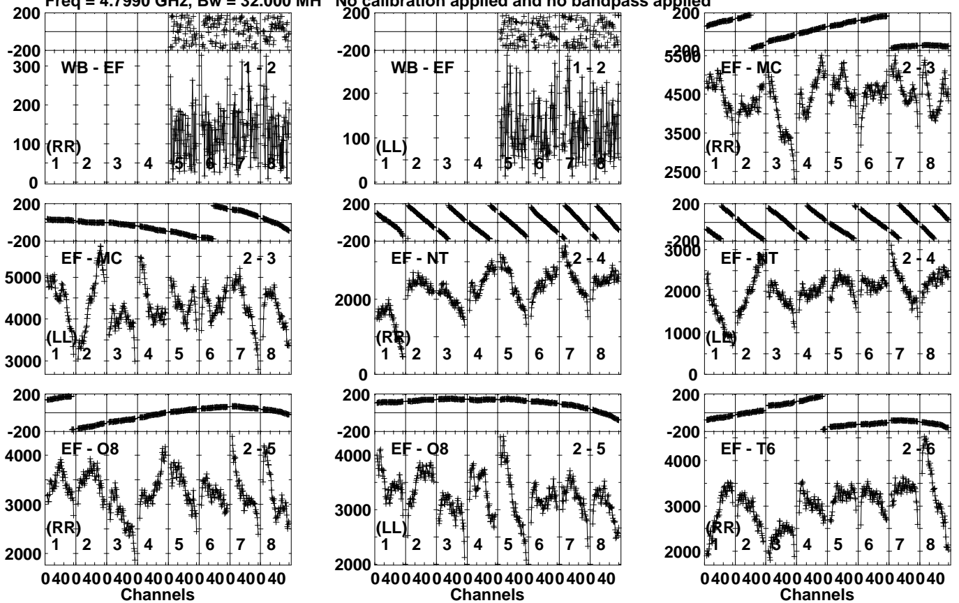
Lower frame: Micro Ampl Jy Top frame: Phas deg Vector averaged cross-power spectrum Several baselines displayed Timerange: 00/19:01:01 to 00/19:02:19
