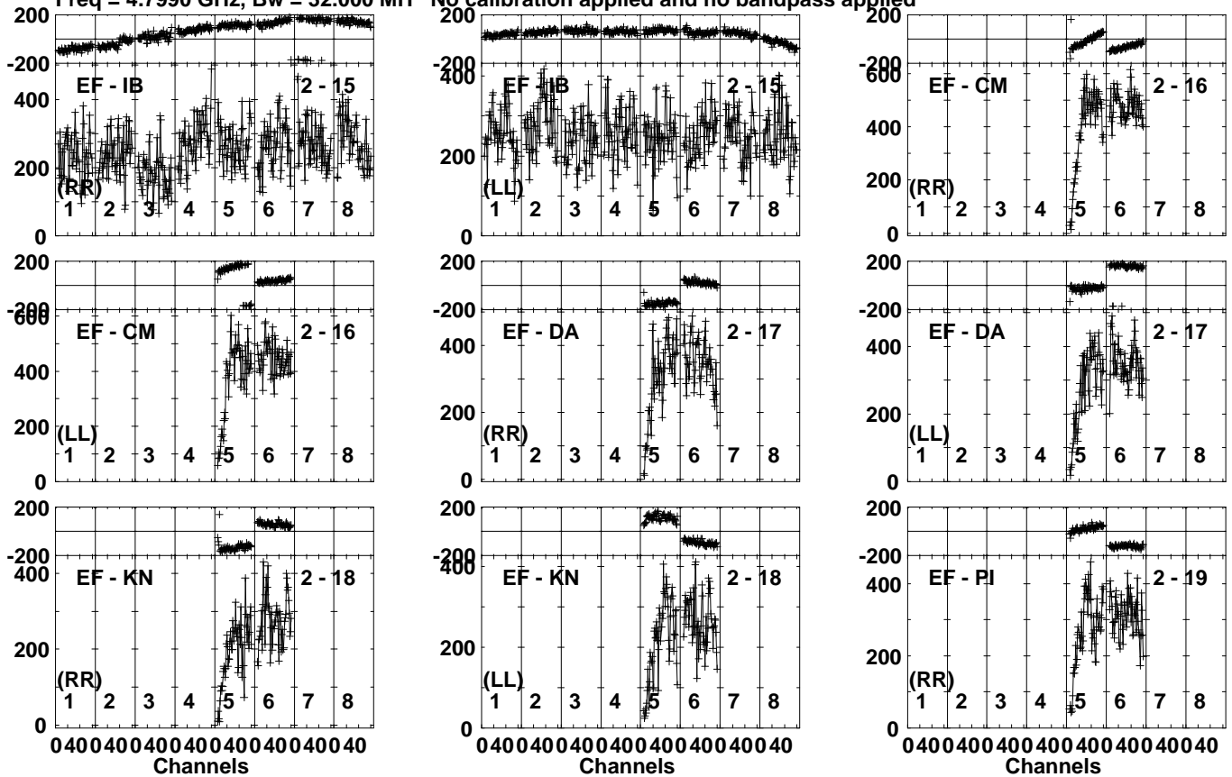
Lower frame: Micro Ampl Jy Top frame: Phas deg Vector averaged cross-power spectrum Several baselines displayed Timerange: 00/17:57:21 to 00/18:00:19
