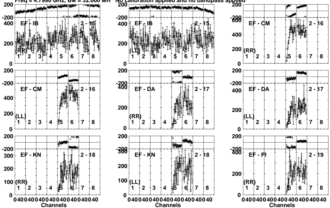
Lower frame: Micro Ampl Jy Top frame: Phas deg Vector averaged cross-power spectrum Several baselines displayed Timerange: 00/17:14:41 to 00/17:17:39
