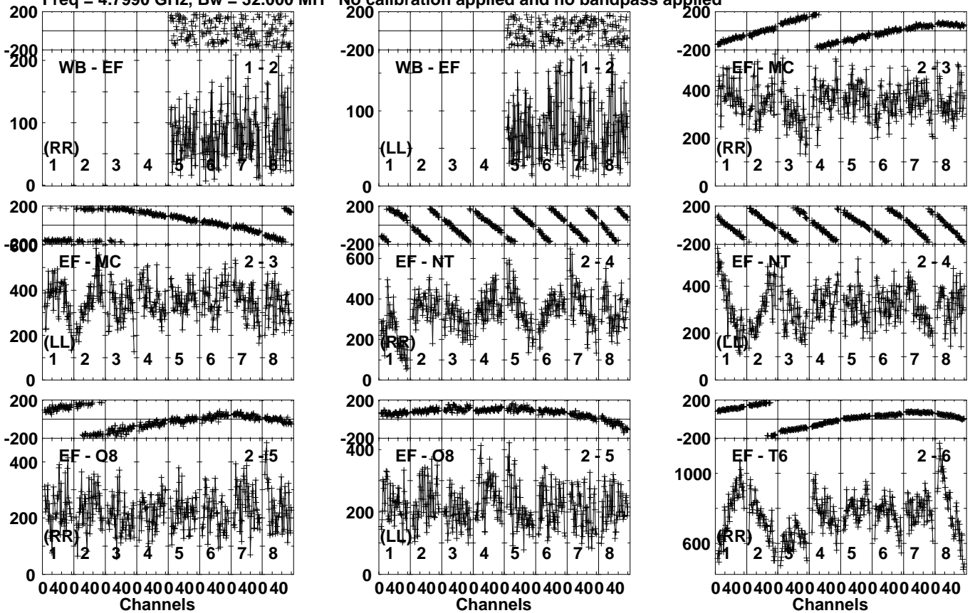
Lower frame: Micro Ampl Jy Top frame: Phas deg Vector averaged cross-power spectrum Several baselines displayed Timerange: 00/17:20:01 to 00/17:22:59
