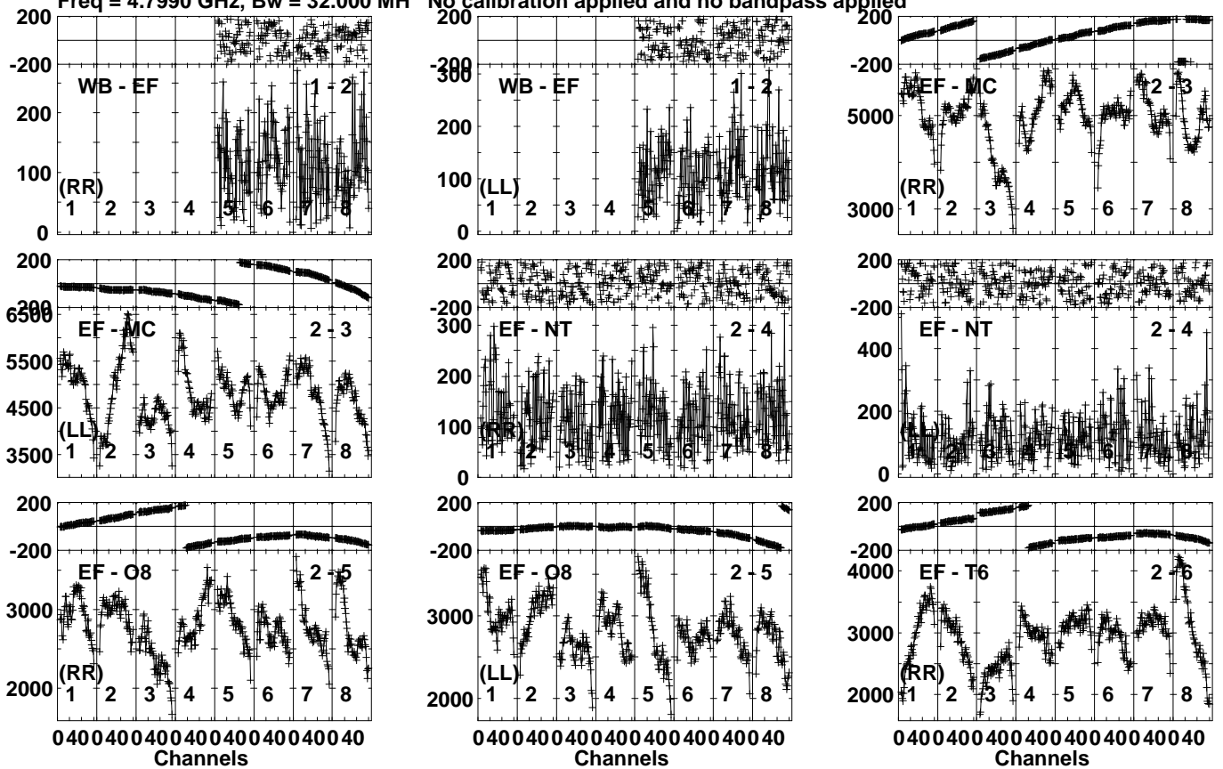
Lower frame: Micro Ampl Jy Top frame: Phas deg Vector averaged cross-power spectrum Several baselines displayed Timerange: 00/18:00:51 to 00/18:02:09
