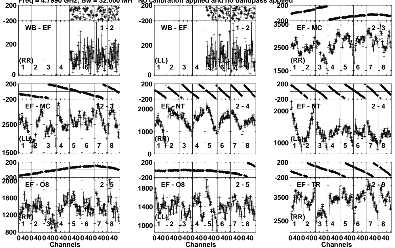
Lower frame: Micro Ampl Jy Top frame: Phas deg Vector averaged cross-power spectrum Several baselines displayed Timerange: 01/02:13:21 to 01/02:14:39
