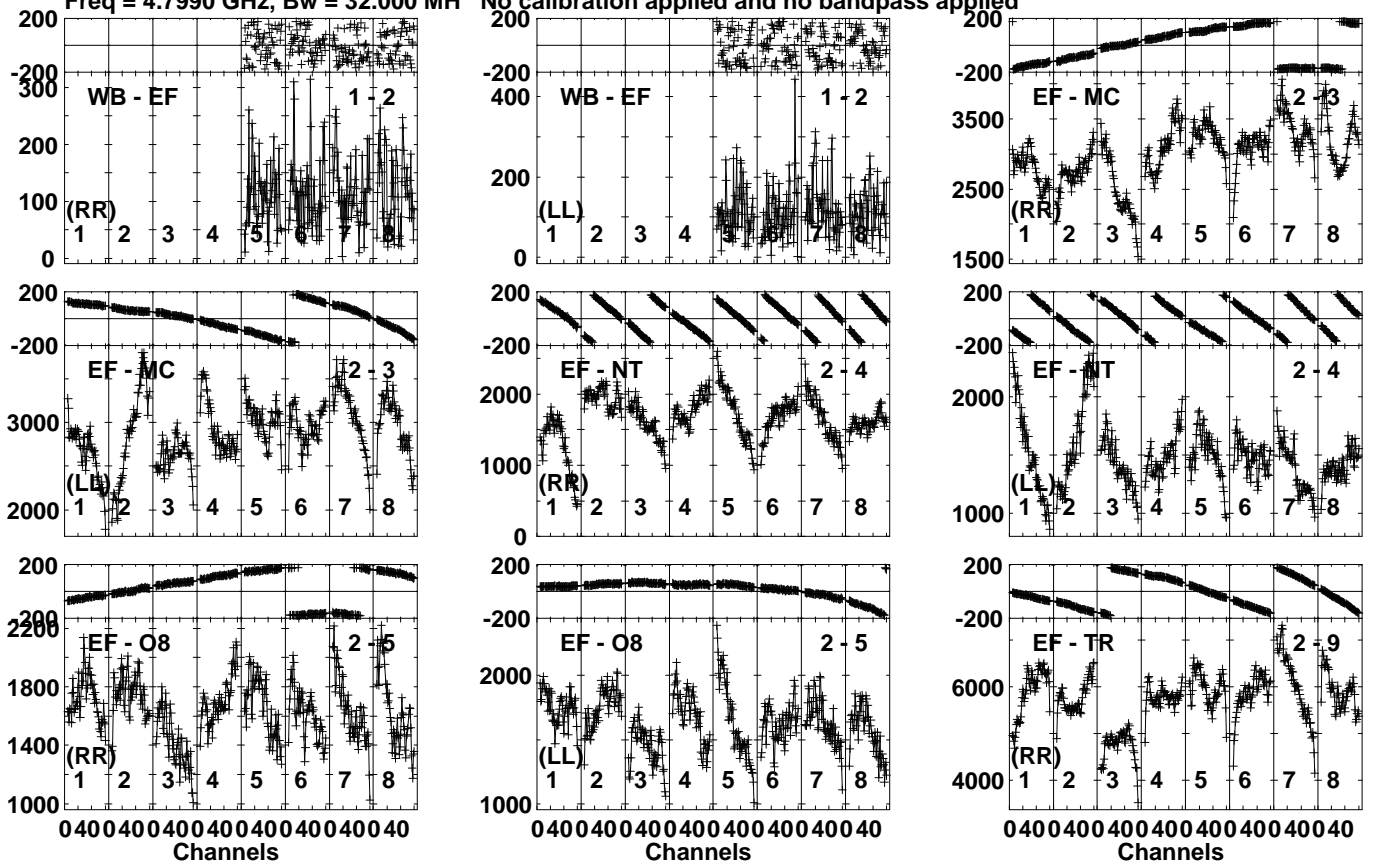
Lower frame: Micro Ampl Jy Top frame: Phas deg Vector averaged cross-power spectrum Several baselines displayed Timerange: 01/00:42:41 to 01/00:43:59
