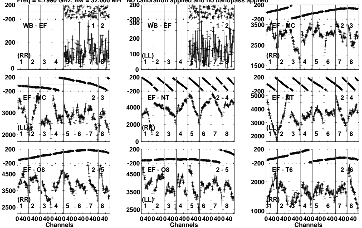
Lower frame: Micro Ampl Jy Top frame: Phas deg Vector averaged cross-power spectrum Several baselines displayed Timerange: 00/20:21:01 to 00/20:22:19
