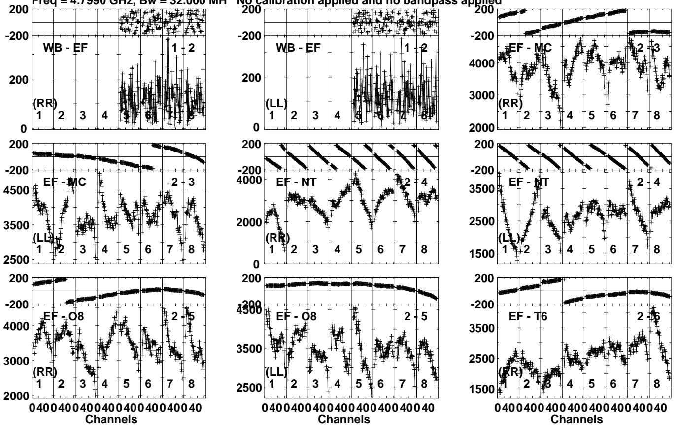
Lower frame: Micro Ampl Jy Top frame: Phas deg Vector averaged cross-power spectrum Several baselines displayed Timerange: 00:19:33:01 to 00:19:34:19
