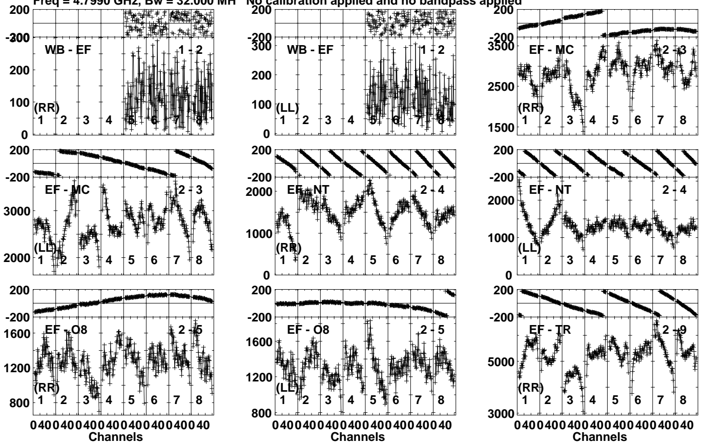
Lower frame: Micro Ampl Jy Top frame: Phas deg Vector averaged cross-power spectrum Several baselines displayed Timerange: 01/01:46:41 to 01/01:47:59
