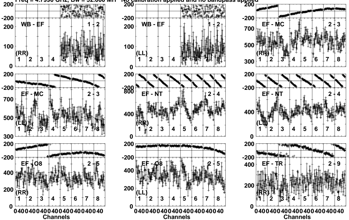
Lower frame: Micro Ampl Jy Top frame: Phas deg Vector averaged cross-power spectrum Several baselines displayed Timerange: 00/23:40:31 to 00/23:43:29
