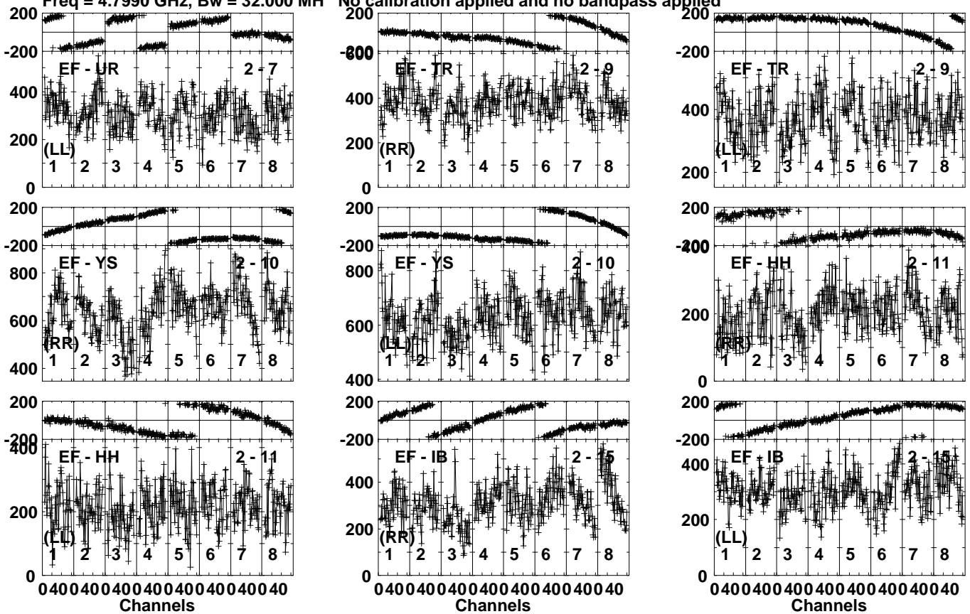
Lower frame: Micro Ampl Jy Top frame: Phas deg Vector averaged cross-power spectrum Several baselines displayed Timerange: 00/22:42:11 to 00/22:45:09
