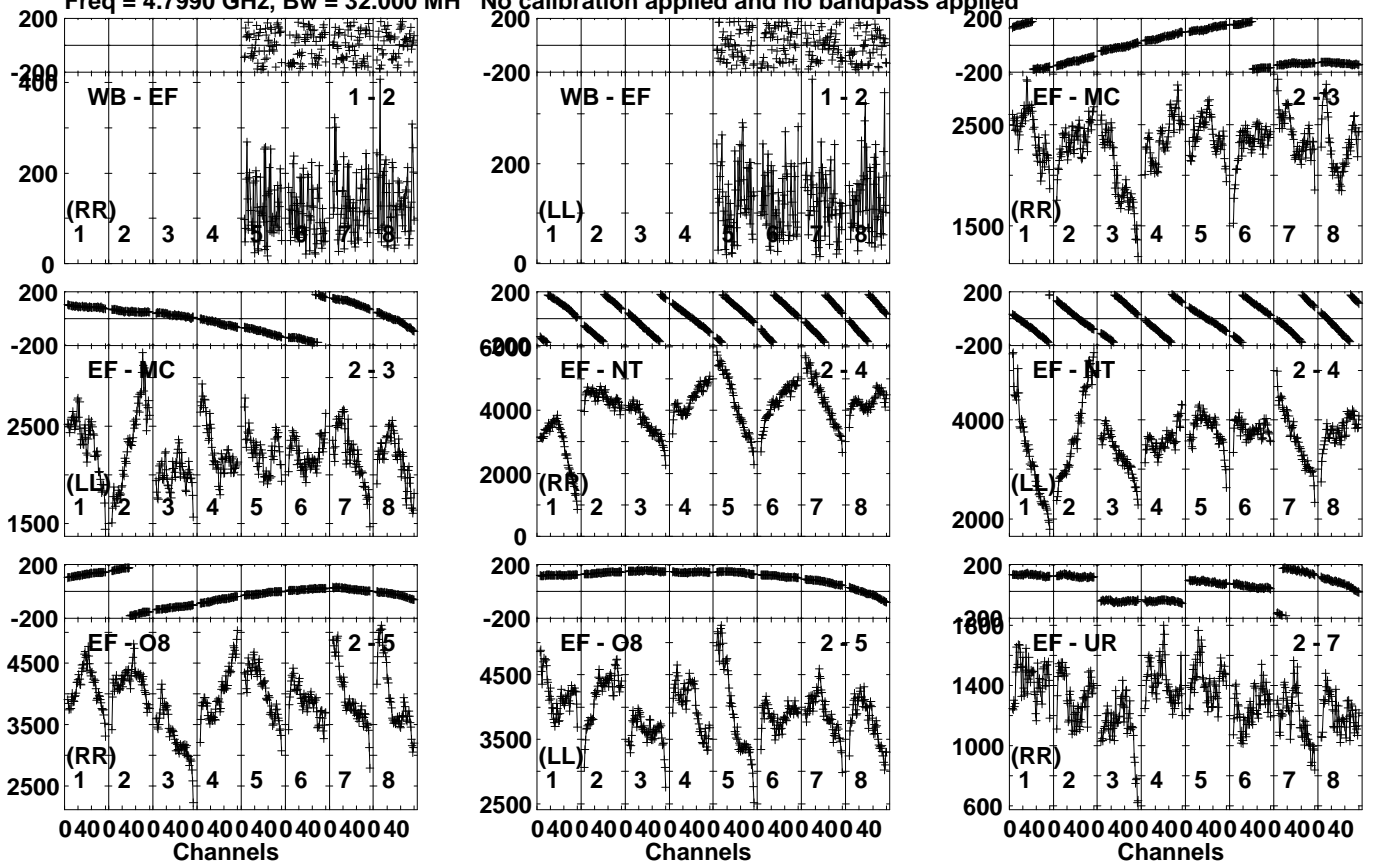
Lower frame: Micro Ampl Jy Top frame: Phas deg Vector averaged cross-power spectrum Several baselines displayed Timerange: 00/21:20:21 to 00/21:21:39
