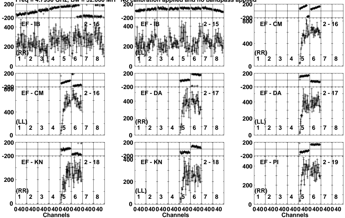
Lower frame: Micro Ampl Jy Top frame: Phas deg Vector averaged cross-power spectrum Several baselines displayed Timerange: 00/18:46:51 to 00/18:49:49
