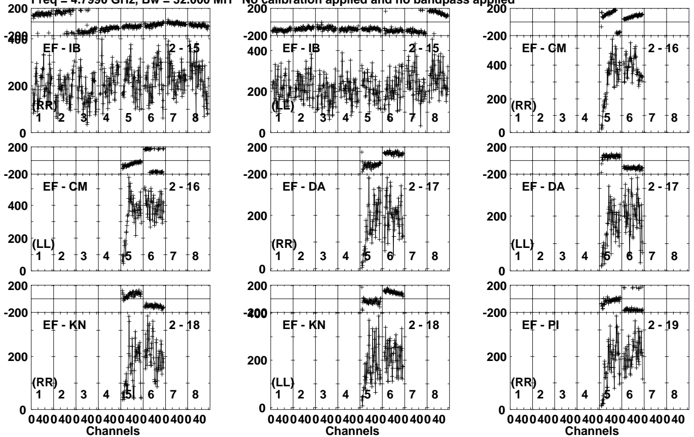
Lower frame: Micro Ampl Jy Top frame: Phas deg Vector averaged cross-power spectrum Several baselines displayed Timerange: 00/17:04:01 to 00/17:06:59
