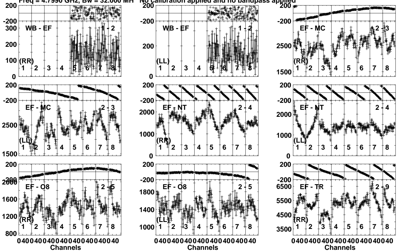
Lower frame: Micro Ampl Jy Top frame: Phas deg Vector averaged cross-power spectrum Several baselines displayed Timerange: 01/02:29:01 to 01/02:29:59
