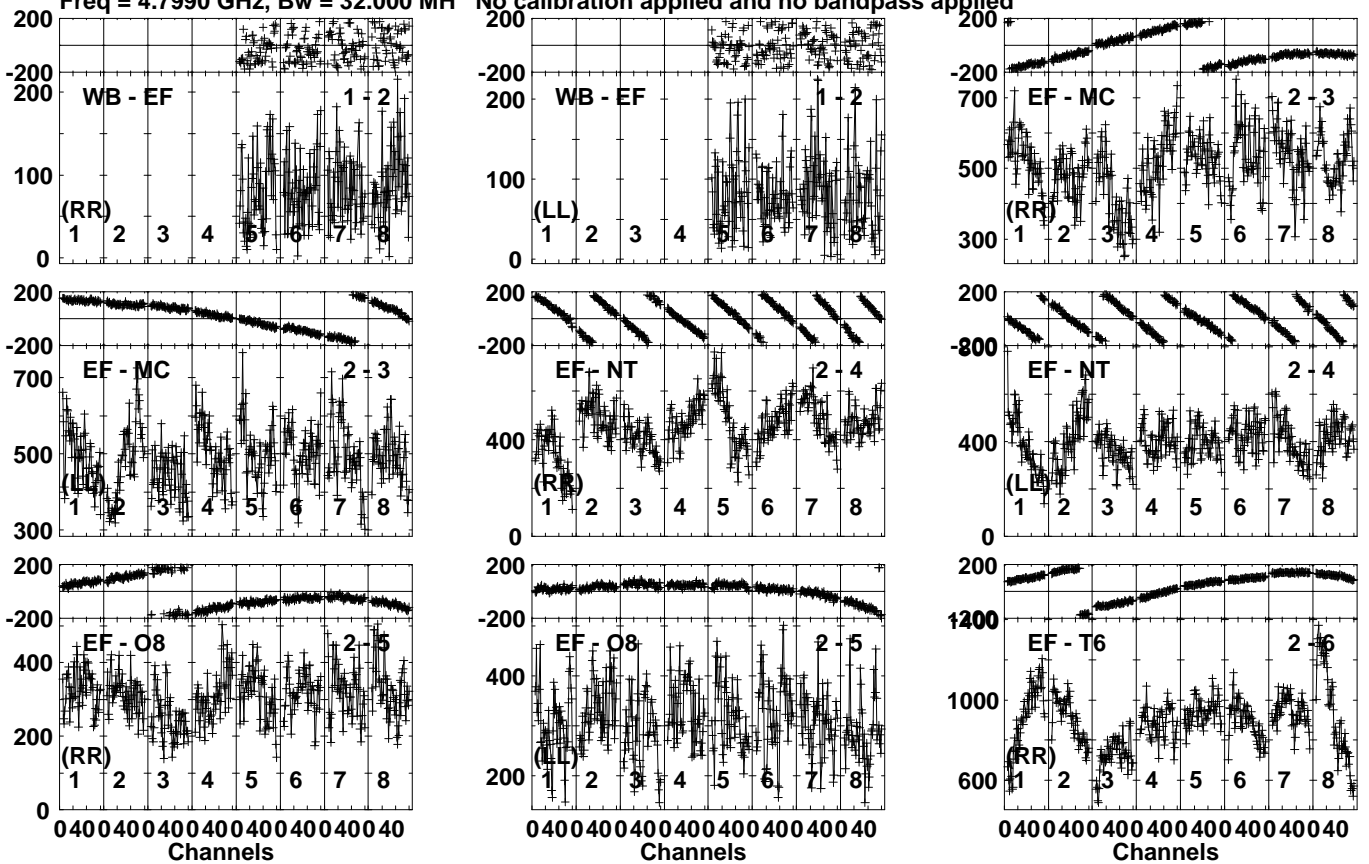
Lower frame: Micro Ampl Jy Top frame: Phas deg Vector averaged cross-power spectrum Several baselines displayed Timerange: 00/20:01:31 to 00/20:04:29
