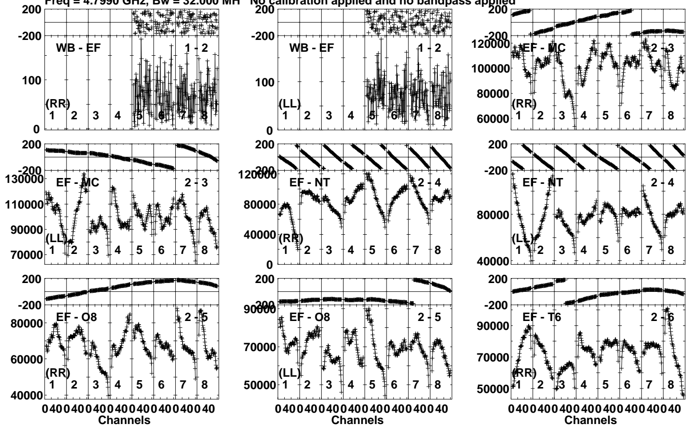
Lower frame: Micro Ampl Jy Top frame: Phas deg Vector averaged cross-power spectrum Several baselines displayed Timerange: 00/20:30:41 to 00/20:34:39
