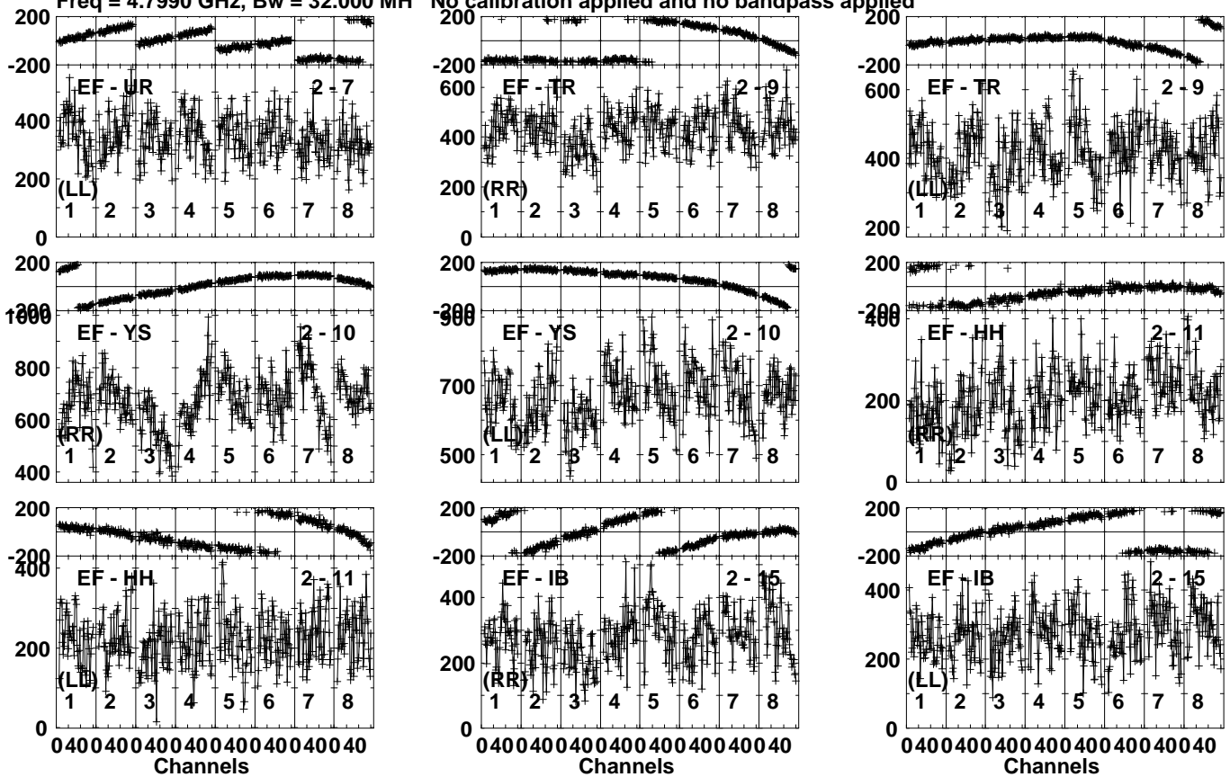
Lower frame: Micro Ampl Jy Top frame: Phas deg Vector averaged cross-power spectrum Several baselines displayed Timerange: 00/21:54:11 to 00/21:57:09
