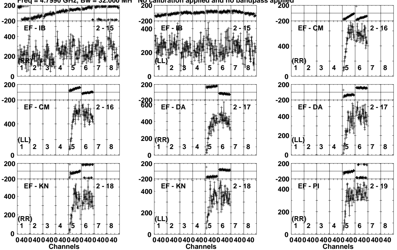
Lower frame: Micro Ampl Jy Top frame: Phas deg Vector averaged cross-power spectrum Several baselines displayed Timerange: 00/19:18:51 to 00/19:21:49
