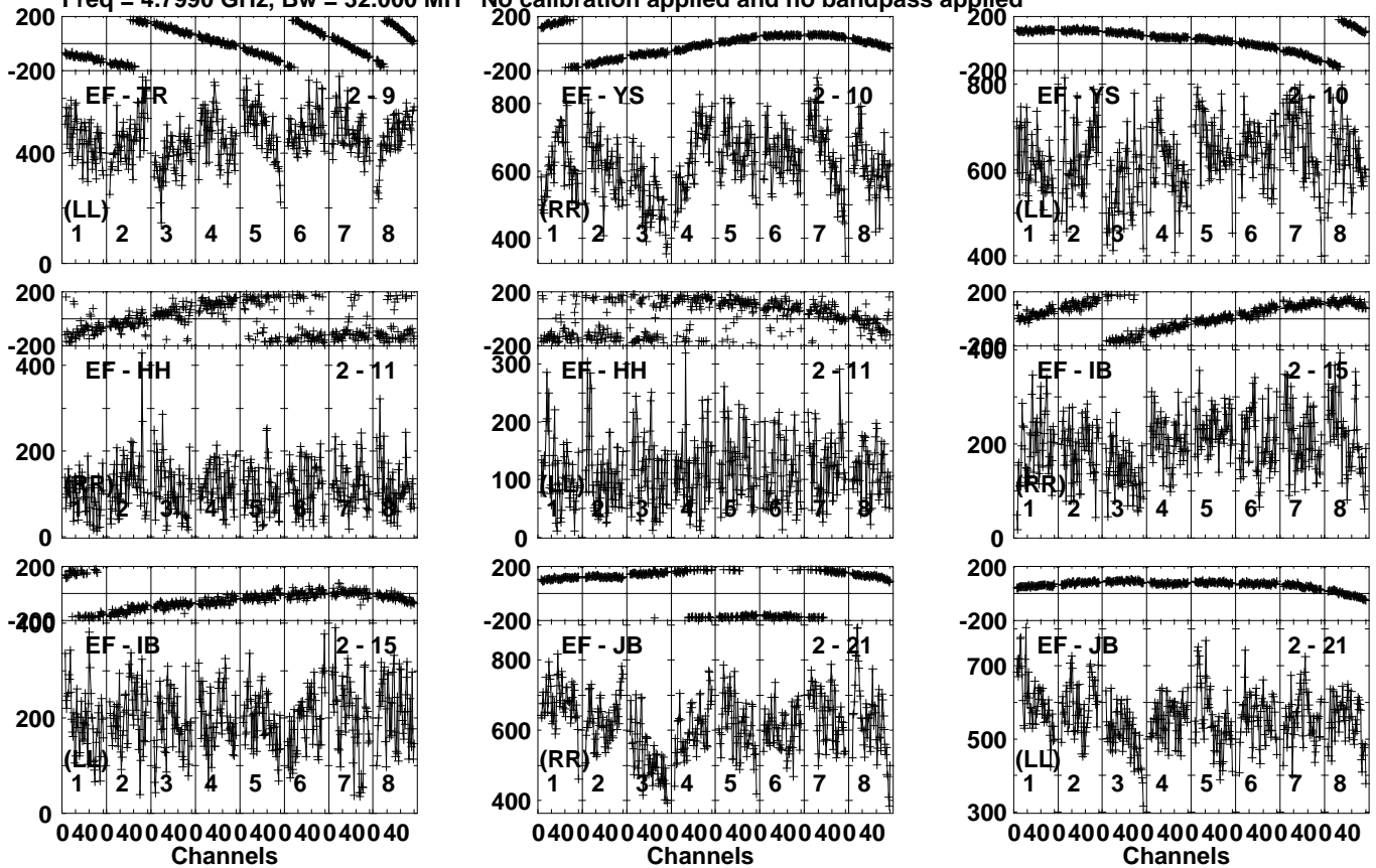
Lower frame: Micro Ampl Jy Top frame: Phas deg Vector averaged cross-power spectrum Several baselines displayed Timerange: 01/01:43:11 to 01/01:46:09
