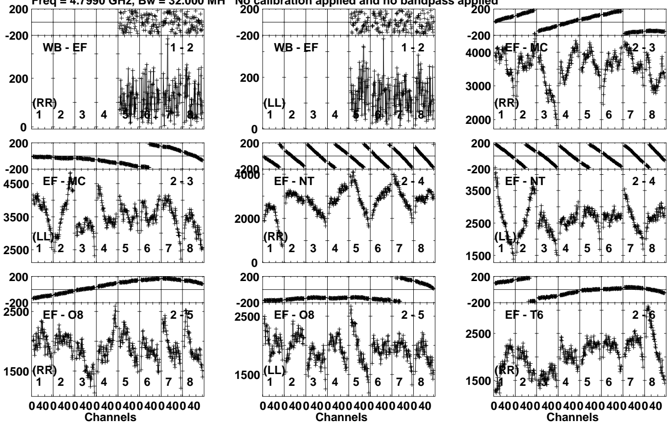
Lower frame: Micro Ampl Jy Top frame: Phas deg Vector averaged cross-power spectrum Several baselines displayed Timerange: 00/17:02:11 to 00/17:03:29
