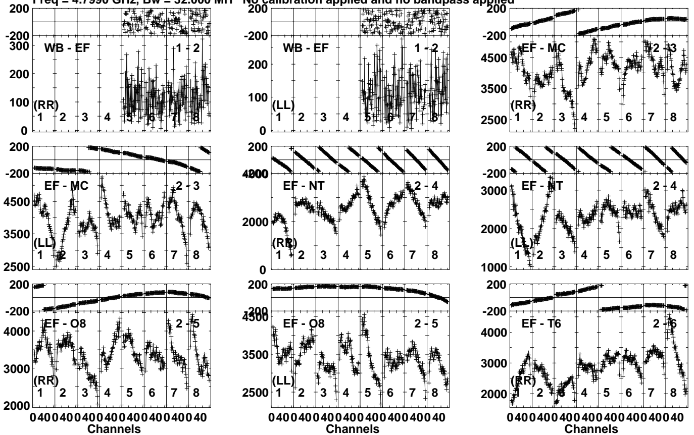
Lower frame: Micro Ampl Jy Top frame: Phas deg Vector averaged cross-power spectrum Several baselines displayed Timerange: 00/19:17:01 to 00/19:18:19
