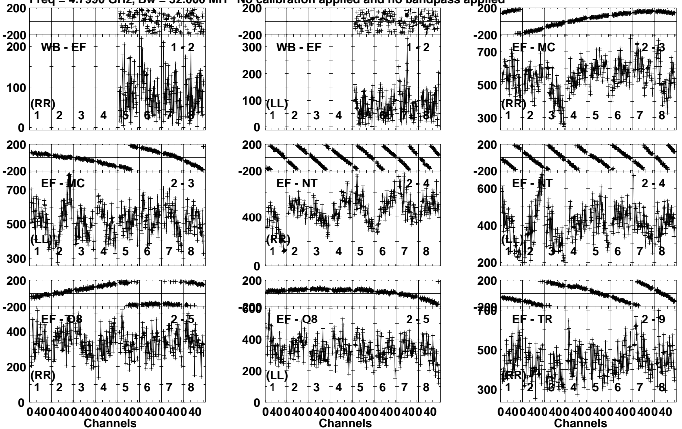
Lower frame: Micro Ampl Jy Top frame: Phas deg Vector averaged cross-power spectrum Several baselines displayed Timerange: 01/00:12:31 to 01/00:15:29
