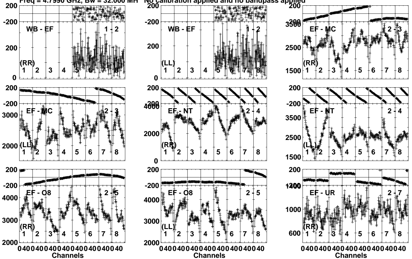
Lower frame: Micro Ampl Jy Top frame: Phas deg Vector averaged cross-power spectrum Several baselines displayed Timerange: 00/22:51:01 to 00/22:52:19
