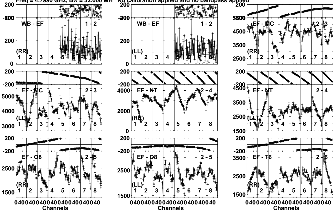
Lower frame: Micro Ampl Jy Top frame: Phas deg Vector averaged cross-power spectrum Several baselines displayed Timerange: 00/17:23:31 to 00/17:24:49
