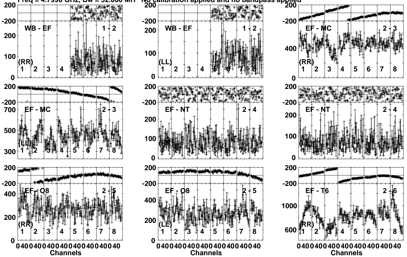
Lower frame: Micro Ampl Jy Top frame: Phas deg Vector averaged cross-power spectrum Several baselines displayed Timerange: 00:18:13:21 to 00:18:16:19
