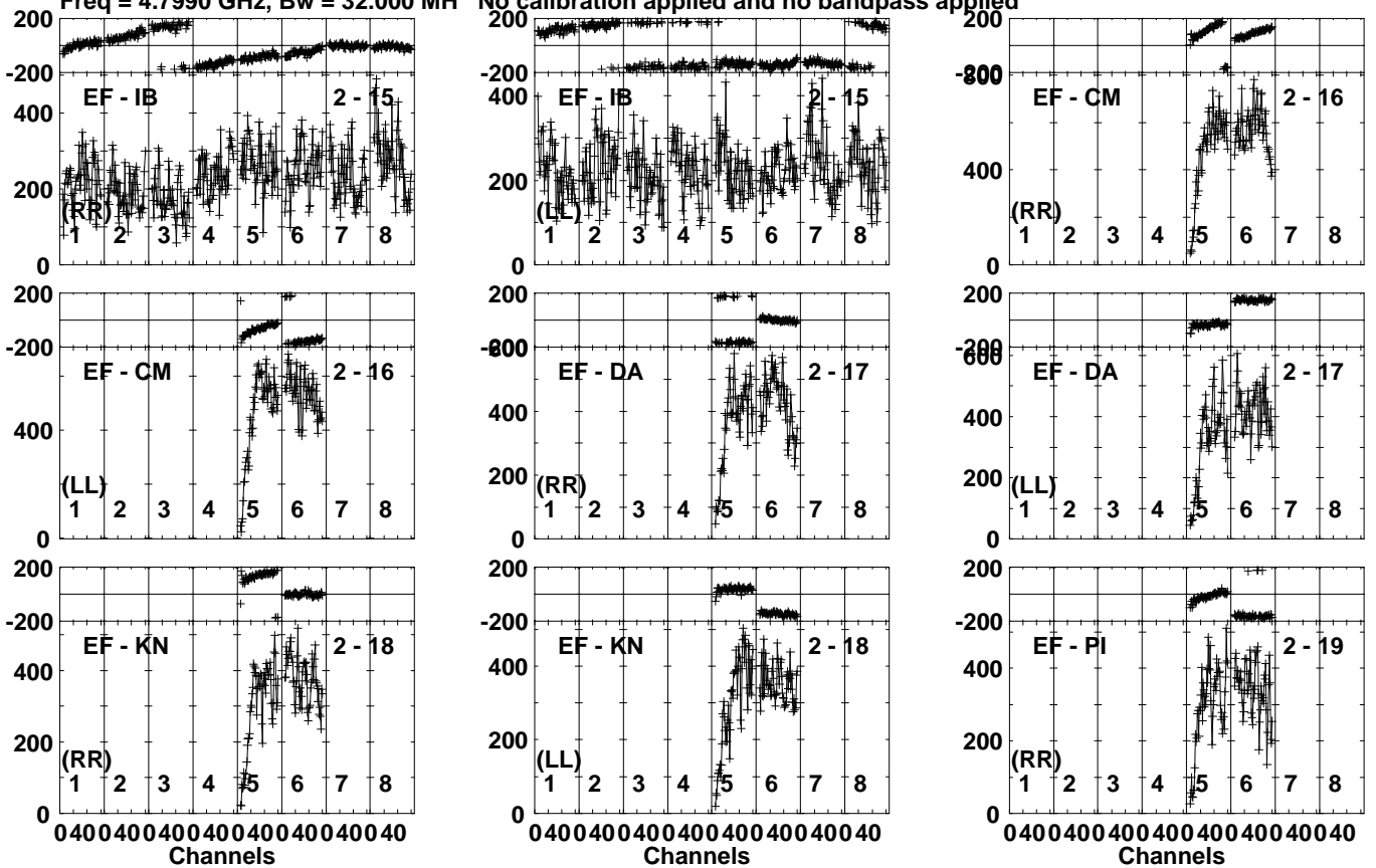
Lower frame: Micro Ampl Jy Top frame: Phas deg Vector averaged cross-power spectrum Several baselines displayed Timerange: 00/19:24:11 to 00/19:27:09
