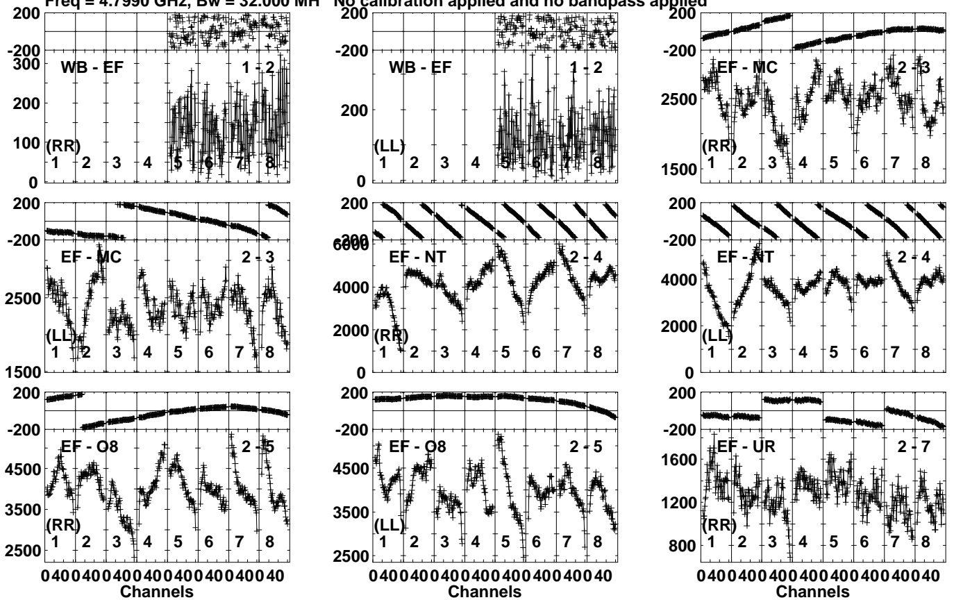
Lower frame: Micro Ampl Jy Top frame: Phas deg Vector averaged cross-power spectrum Several baselines displayed Timerange: 00/21:04:21 to 00/21:05:39
