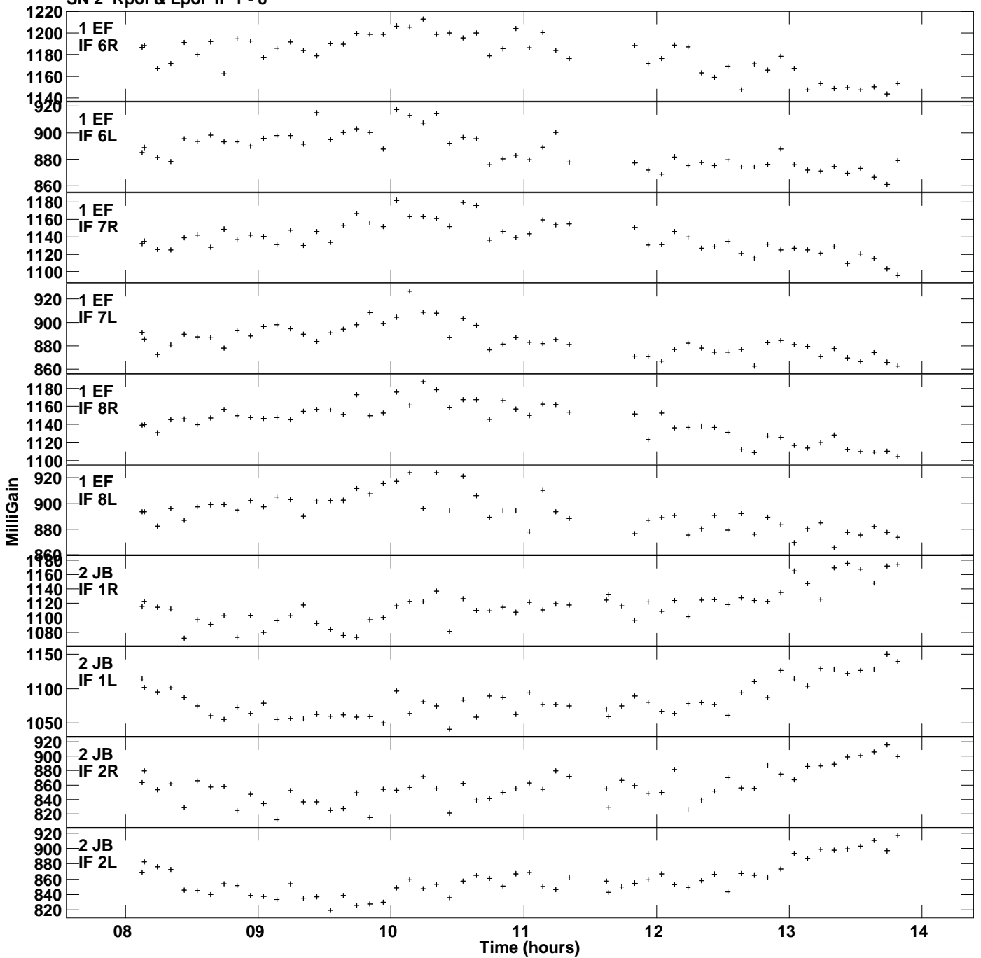
Plot file version 2 created 17-DEC-2021 12:53:57 Gain amp vs UTC time for J1300+2830.MULTI.1 SN 2 Rpol & Lpol IF 1 - 8
