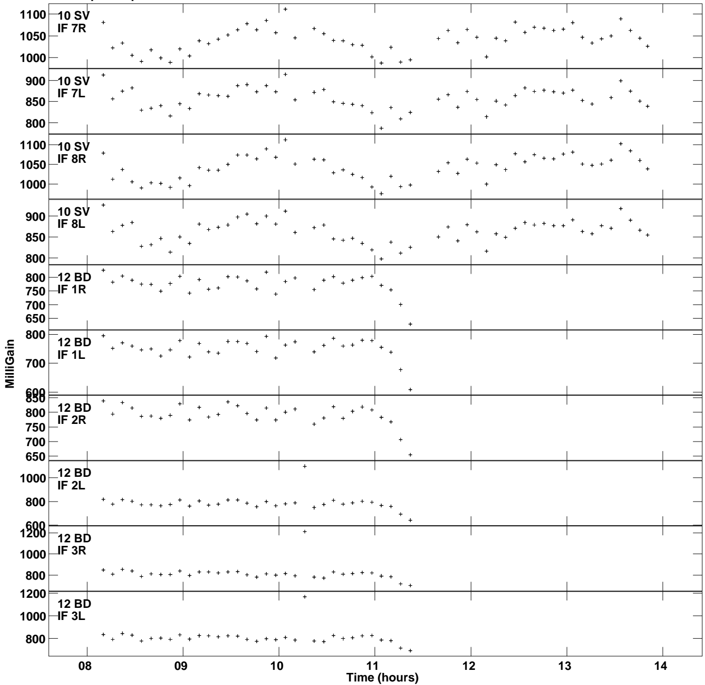
Plot file version 15 created 17-DEC-2021 12:53:42 Gain amp vs UTC time for J1310+3220.MULTI.1 SN 2 Rpol & Lpol IF 1 - 8
