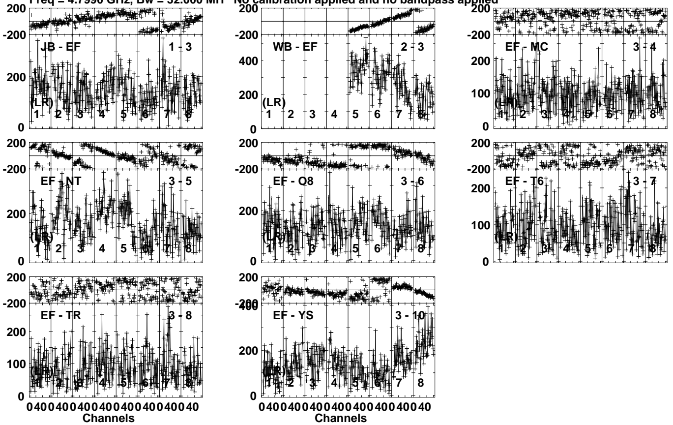
Lower frame: Micro Ampl Jy Top frame: Phas deg Vector averaged cross-power spectrum Several baselines displayed Timerange: 00/08:24:11 to 00/08:28:09
