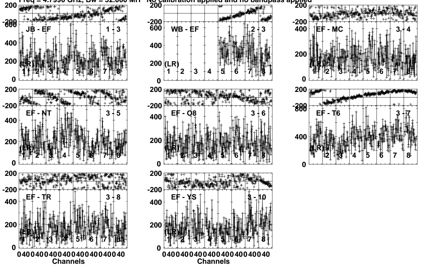
Lower frame: Micro Ampl Jy Top frame: Phas deg Vector averaged cross-power spectrum Several baselines displayed Timerange: 00/07:33:21 to 00/07:34:19
