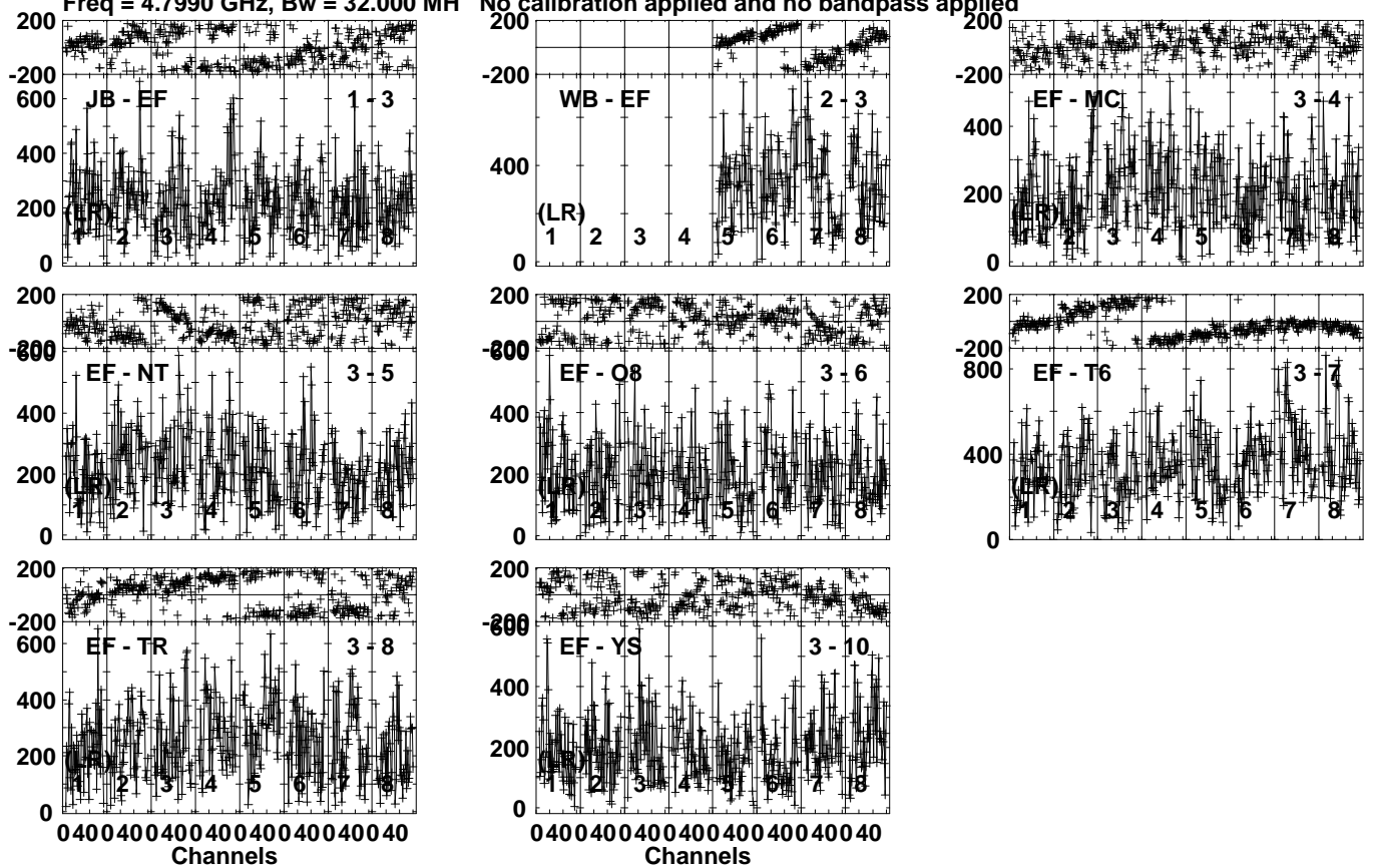
Lower frame: Micro Ampl Jy Top frame: Phas deg Vector averaged cross-power spectrum Several baselines displayed Timerange: 00/09:12:31 to 00/09:13:59
