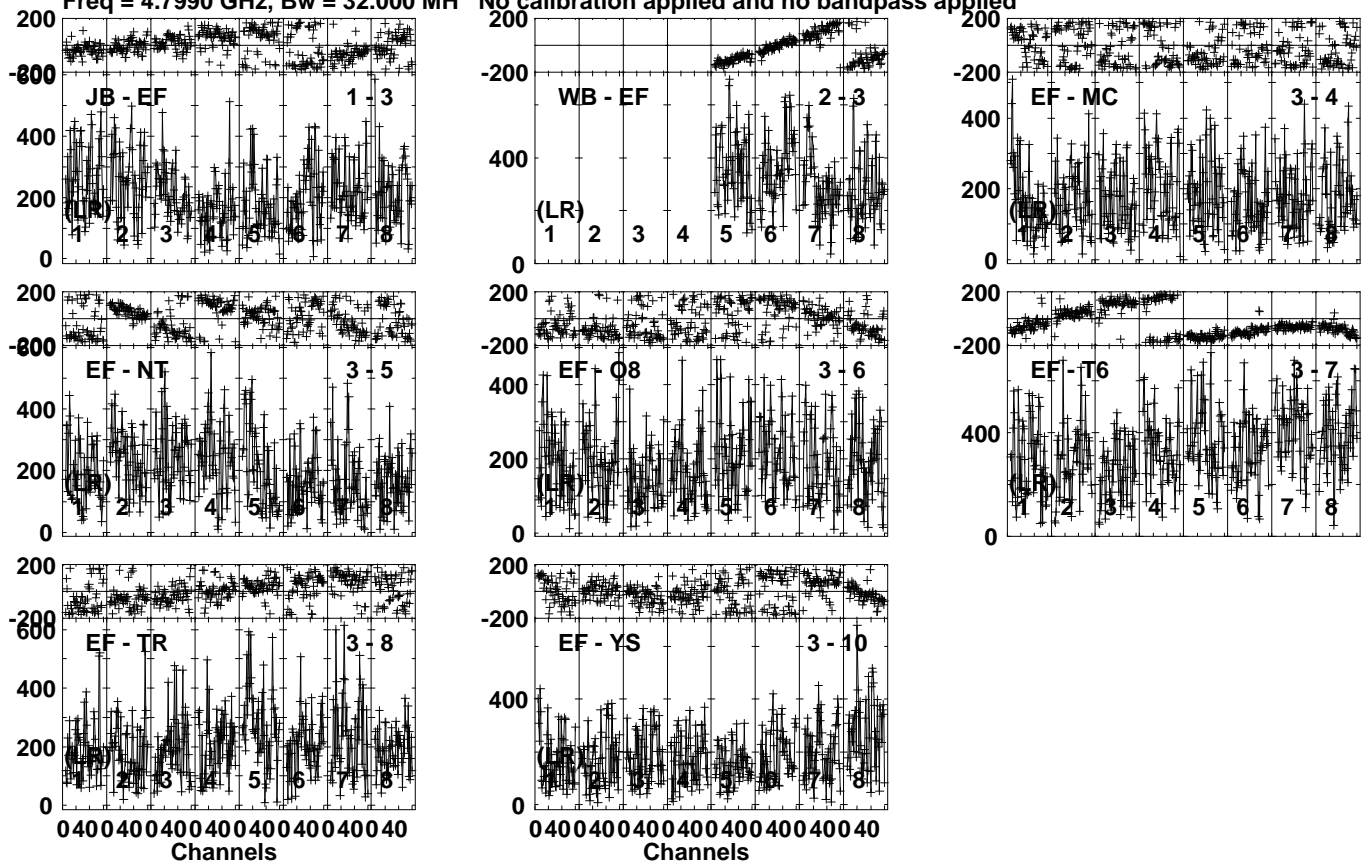
Lower frame: Micro Ampl Jy Top frame: Phas deg Vector averaged cross-power spectrum Several baselines displayed Timerange: 00/08:56:01 to 00/08:57:29
