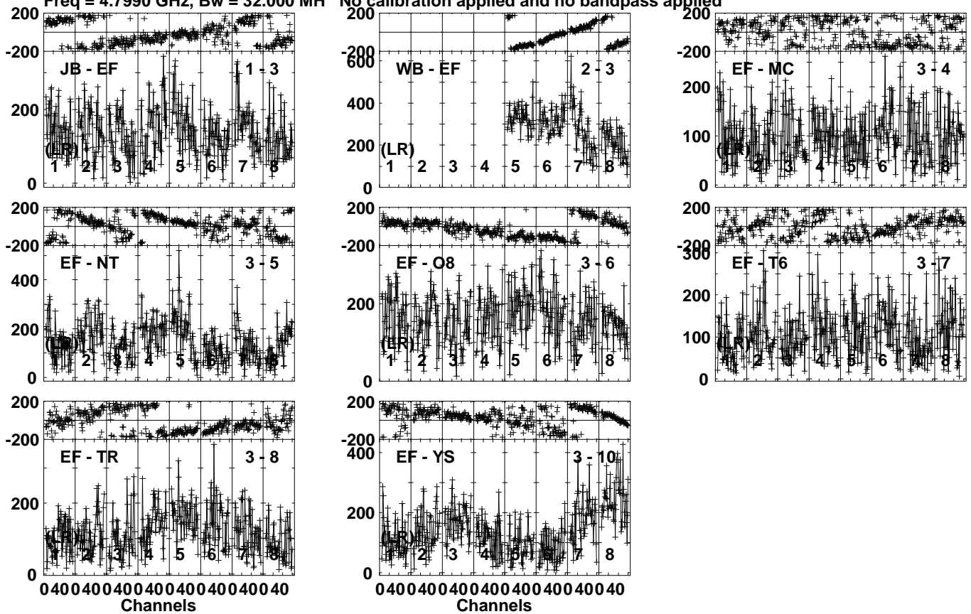
Lower frame: Micro Ampl Jy Top frame: Phas deg Vector averaged cross-power spectrum Several baselines displayed Timerange: 00/09:41:51 to 00/09:45:49
