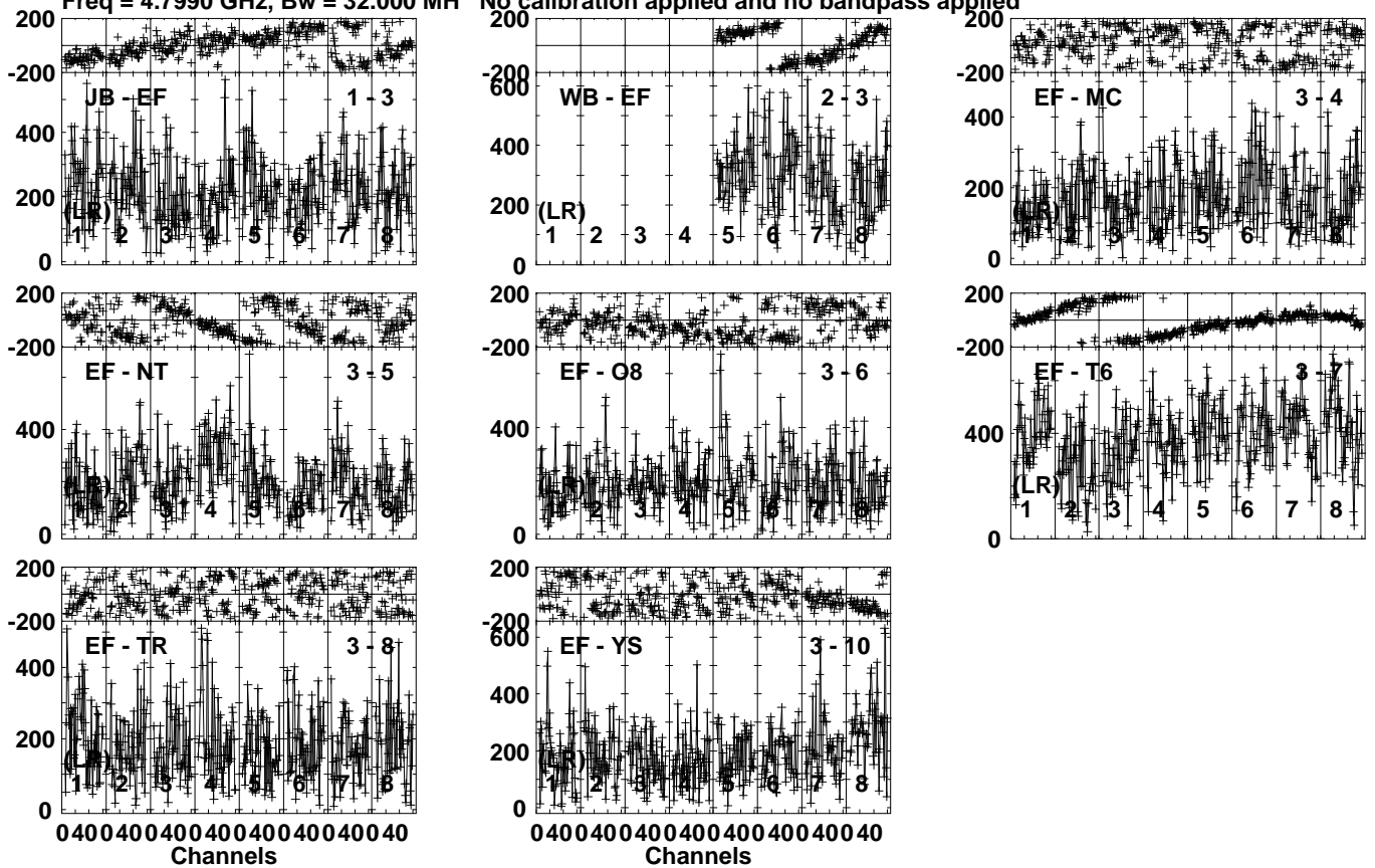
Lower frame: Micro Ampl Jy Top frame: Phas deg Vector averaged cross-power spectrum Several baselines displayed Timerange: 00/07:54:51 to 00/07:56:19
