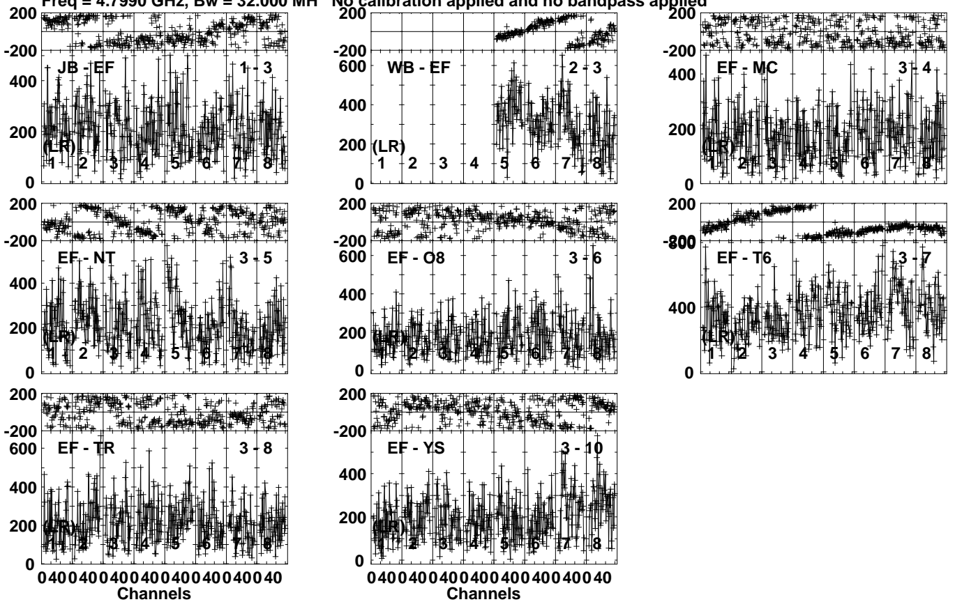
Lower frame: Micro Ampl Jy Top frame: Phas deg Vector averaged cross-power spectrum Several baselines displayed Timerange: 00/08:23:11 to 00/08:24:09
