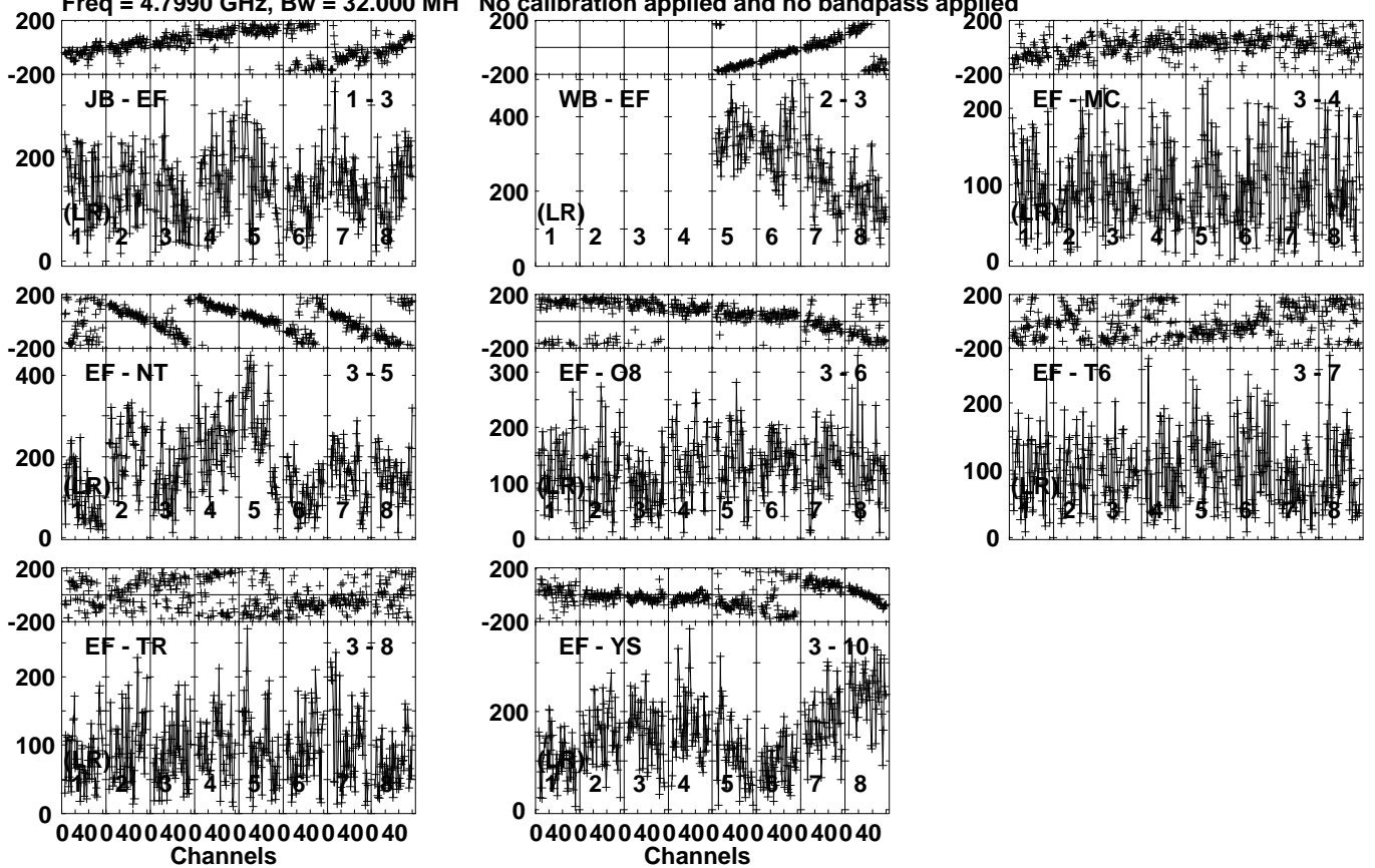
Lower frame: Micro Ampl Jy Top frame: Phas deg Vector averaged cross-power spectrum Several baselines displayed Timerange: 00/07:06:31 to 00/07:10:29
