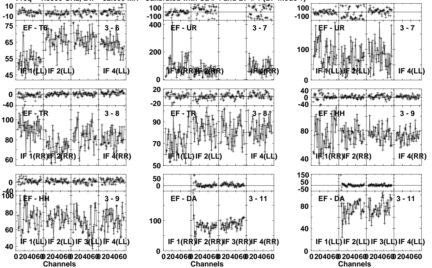
Lower frame: Milli Ampl Jy Top frame: Phas deg Vector averaged cross-power spectrum Several baselines displayed Timerange: 00/01:34:01 to 00/01:35:29
