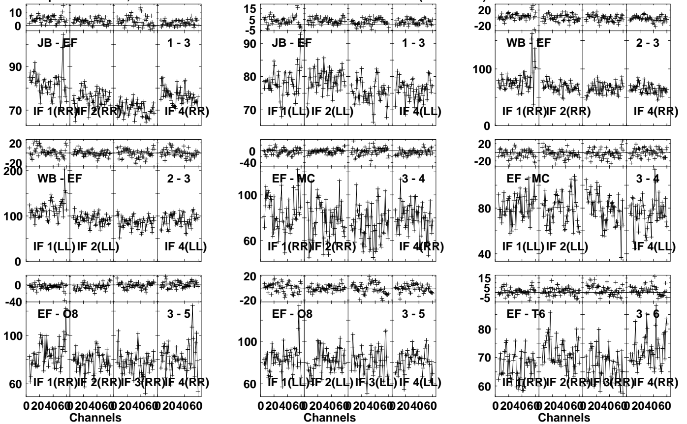
Lower frame: Milli Ampl Jy Top frame: Phas deg Vector averaged cross-power spectrum Several baselines displayed Timerange: 00/00:50:01 to 00/00:51:29
