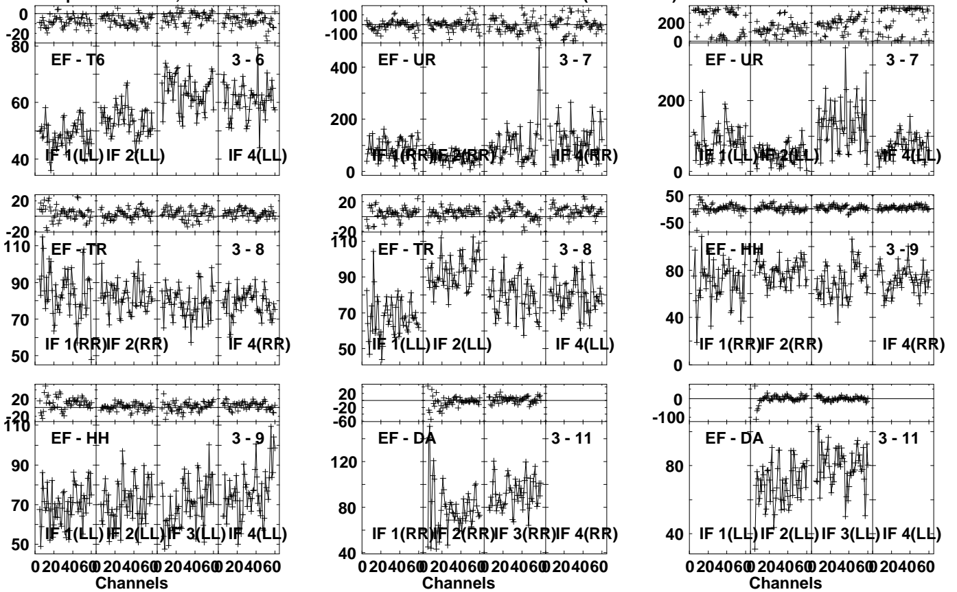
Lower frame: Milli Ampl Jy Top frame: Phas deg Vector averaged cross-power spectrum Several baselines displayed Timerange: 00/02:18:01 to 00/02:19:29
