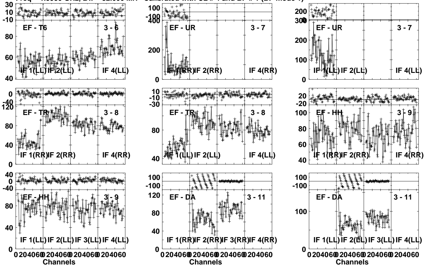
Lower frame: Milli Ampl Jy Top frame: Phas deg Vector averaged cross-power spectrum Several baselines displayed Timerange: 00/02:42:36 to 00/02:43:58
