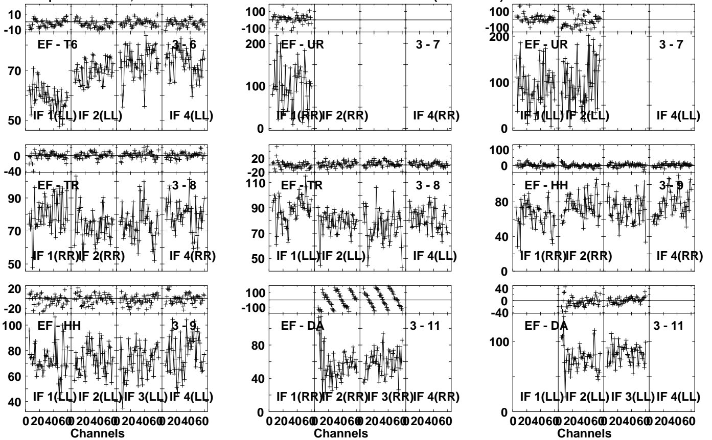
Lower frame: Milli Ampl Jy Top frame: Phas deg Vector averaged cross-power spectrum Several baselines displayed Timerange: 00/00:17:01 to 00/00:18:29
