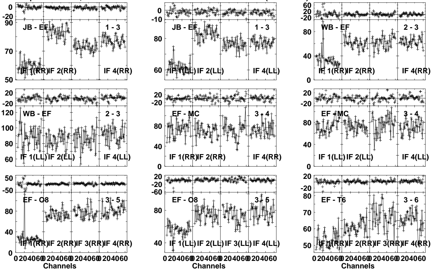
Lower frame: Milli Ampl Jy Top frame: Phas deg Vector averaged cross-power spectrum Several baselines displayed Timerange: 00/01:45:01 to 00/01:46:29
