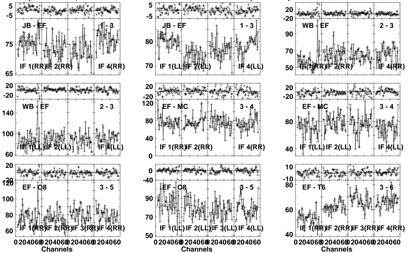
Lower frame: Milli Ampl Jy Top frame: Phas deg Vector averaged cross-power spectrum Several baselines displayed Timerange: 00/01:23:01 to 00/01:24:29
