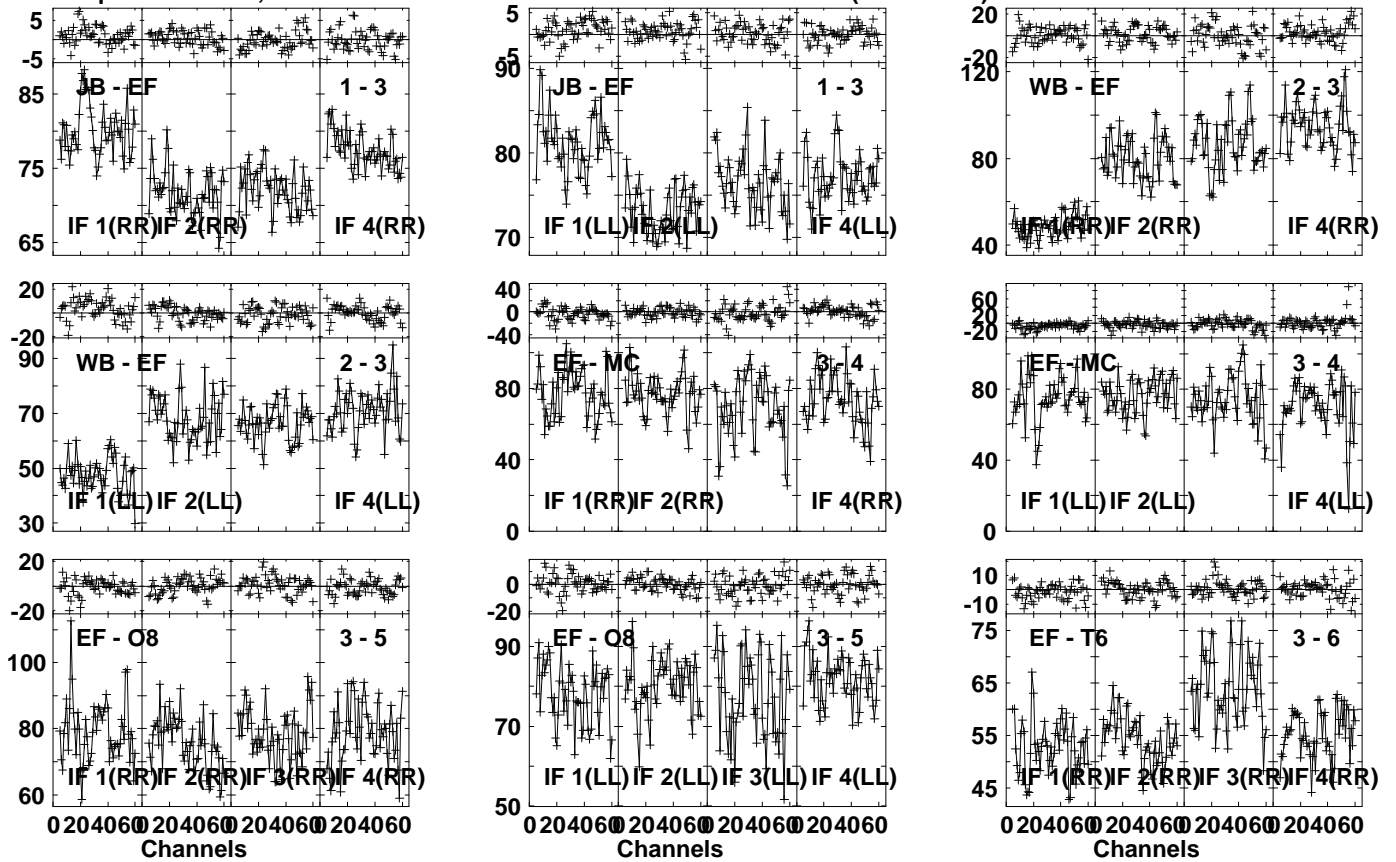
Lower frame: Milli Ampl Jy Top frame: Phas deg Vector averaged cross-power spectrum Several baselines displayed Timerange: 00/02:34:31 to 00/02:35:59
