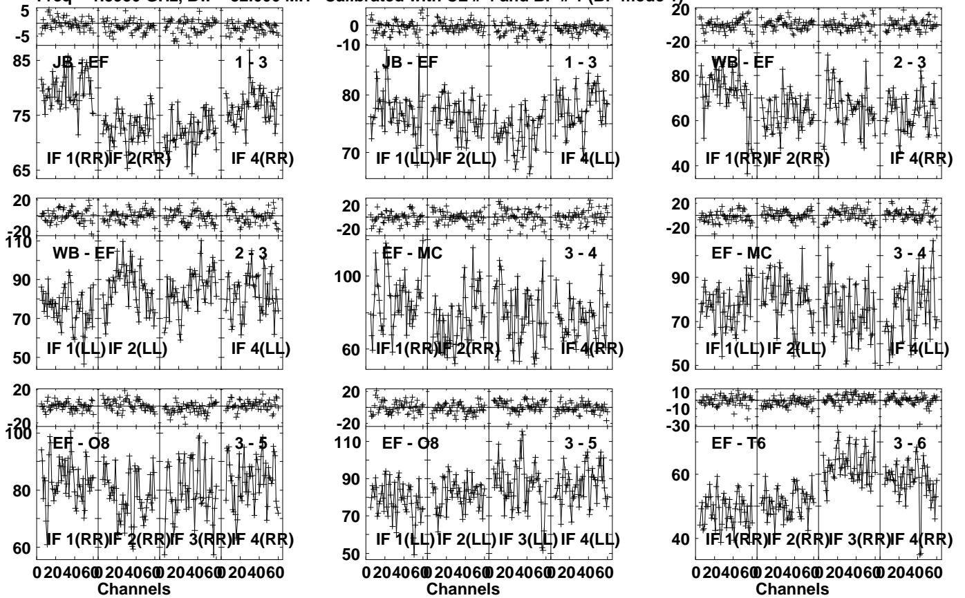
Lower frame: Milli Ampl Jy Top frame: Phas deg Vector averaged cross-power spectrum Several baselines displayed Timerange: 00/02:07:01 to 00/02:08:29
