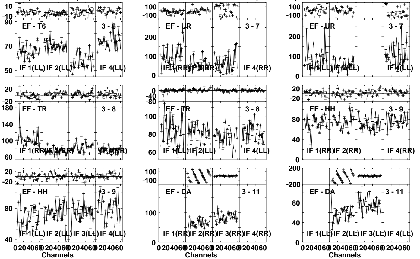
Lower frame: Milli Ampl Jy Top frame: Phas deg Vector averaged cross-power spectrum Several baselines displayed Timerange: 00/00:39:01 to 00/00:40:29
