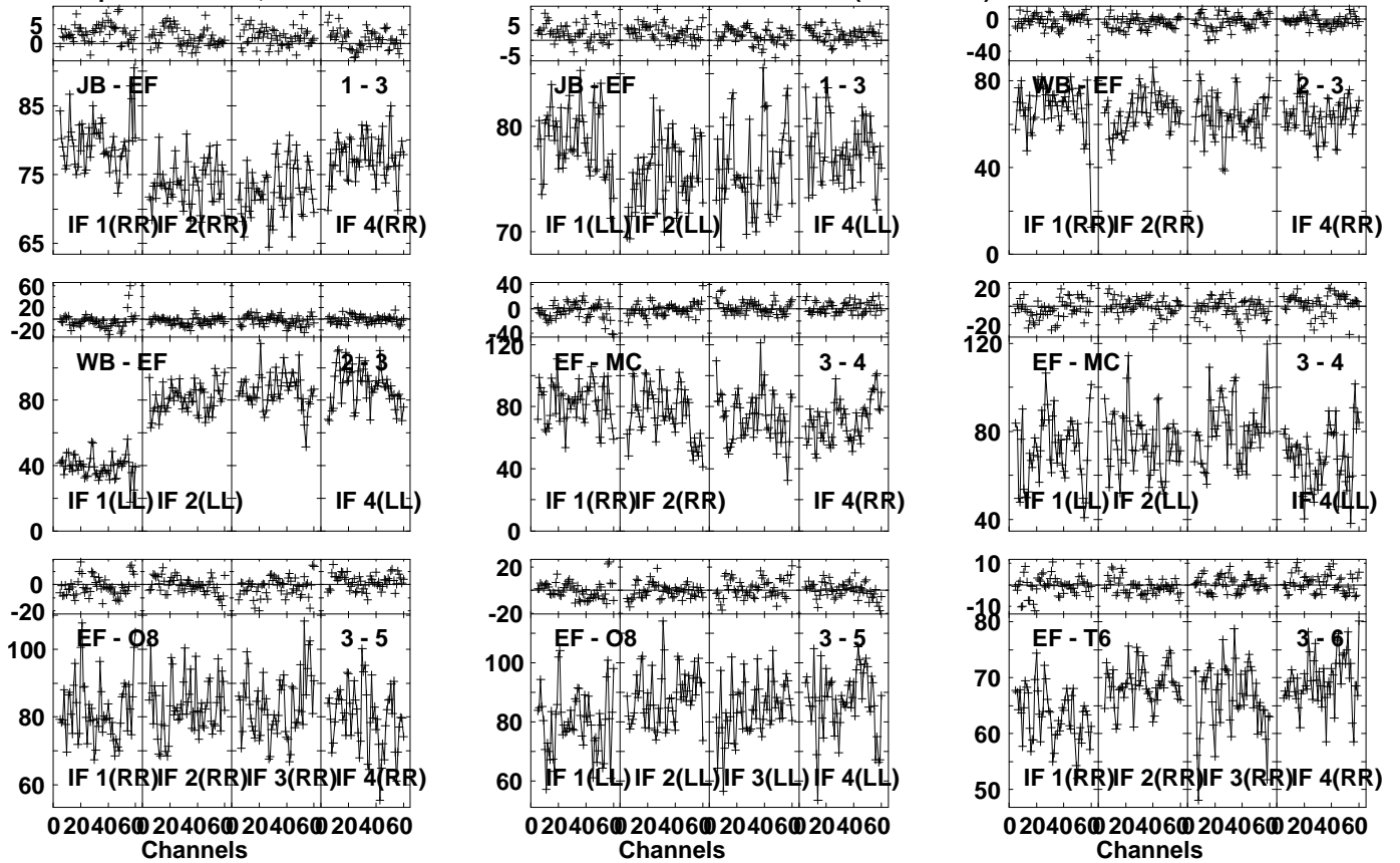
Lower frame: Milli Ampl Jy Top frame: Phas deg Vector averaged cross-power spectrum Several baselines displayed Timerange: 00/01:12:01 to 00/01:13:29
