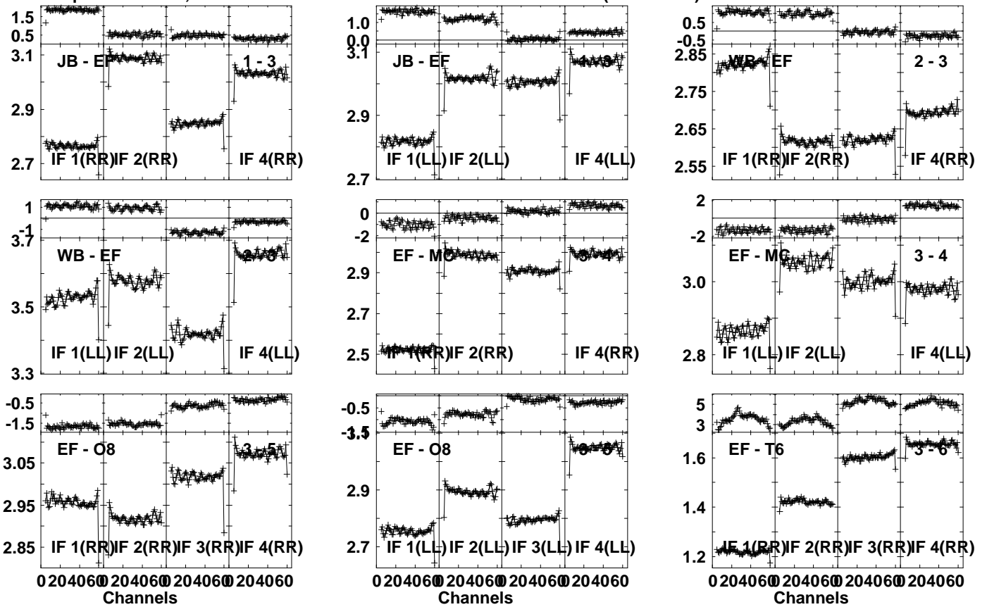
Lower frame: Ampl Jy Top frame: Phas deg Vector averaged cross-power spectrum Several baselines displayed Timerange: 00/02:37:01 to 00/02:41:59
