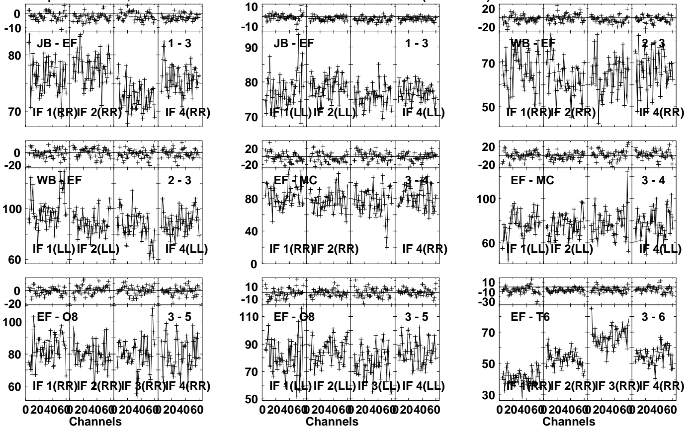
Lower frame: Milli Ampl Jy Top frame: Phas deg Vector averaged cross-power spectrum Several baselines displayed Timerange: 00/02:29:01 to 00/02:30:29
