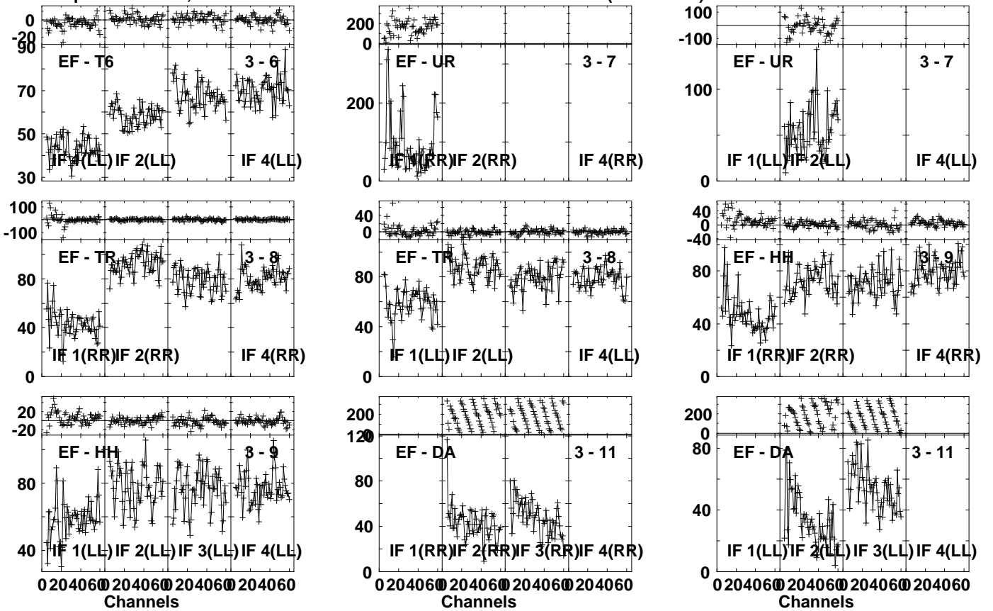
Lower frame: Milli Ampl Jy Top frame: Phas deg Vector averaged cross-power spectrum Several baselines displayed Timerange: 00/02:53:31 to 00/02:54:59
