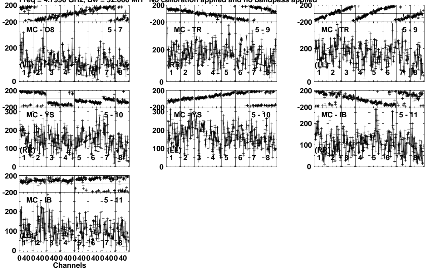
Lower frame: Micro Ampl Jy Top frame: Phas deg Vector averaged cross-power spectrum Several baselines displayed Timerange: 00/14:07:51 to 00/14:11:29
