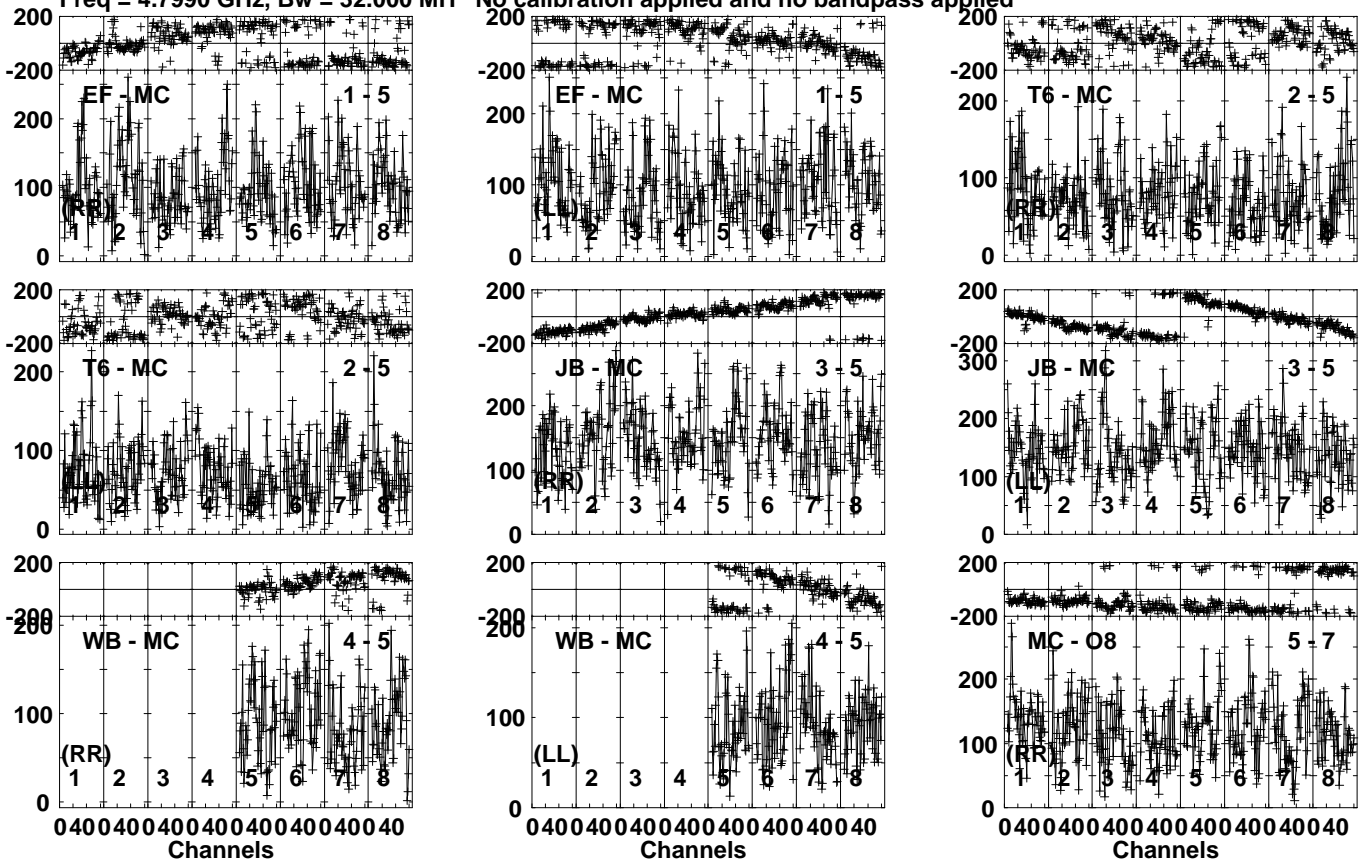
Lower frame: Micro Ampl Jy Top frame: Phas deg Vector averaged cross-power spectrum Several baselines displayed Timerange: 00/13:10:21 to 00/13:13:59
