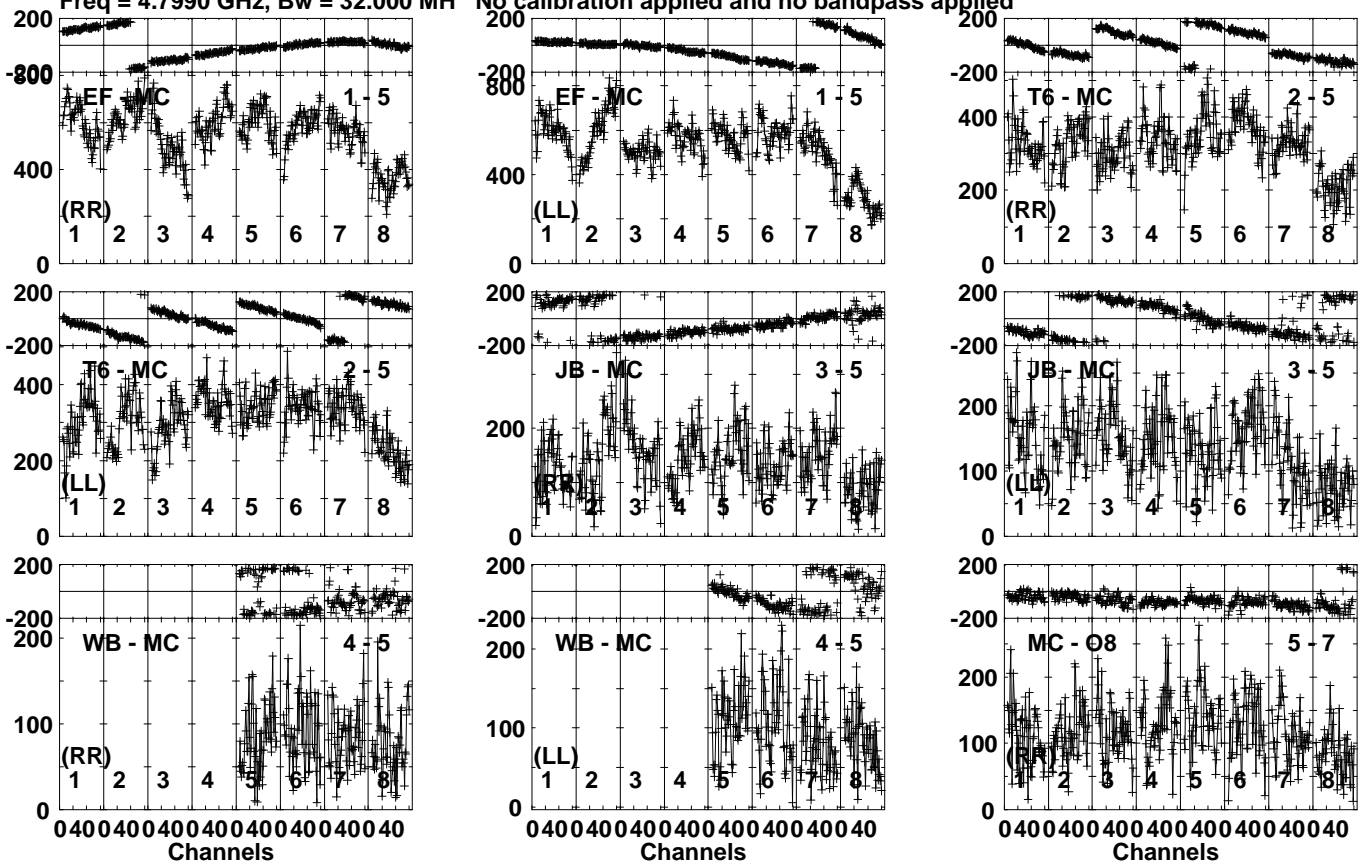
Lower frame: Micro Ampl Jy Top frame: Phas deg Vector averaged cross-power spectrum Several baselines displayed Timerange: 00/14:18:21 to 00/14:21:59
