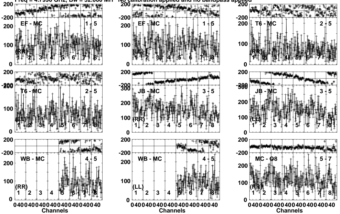
Lower frame: Micro Ampl Jy Top frame: Phas deg Vector averaged cross-power spectrum Several baselines displayed Timerange: 00/14:23:51 to 00/14:27:29
