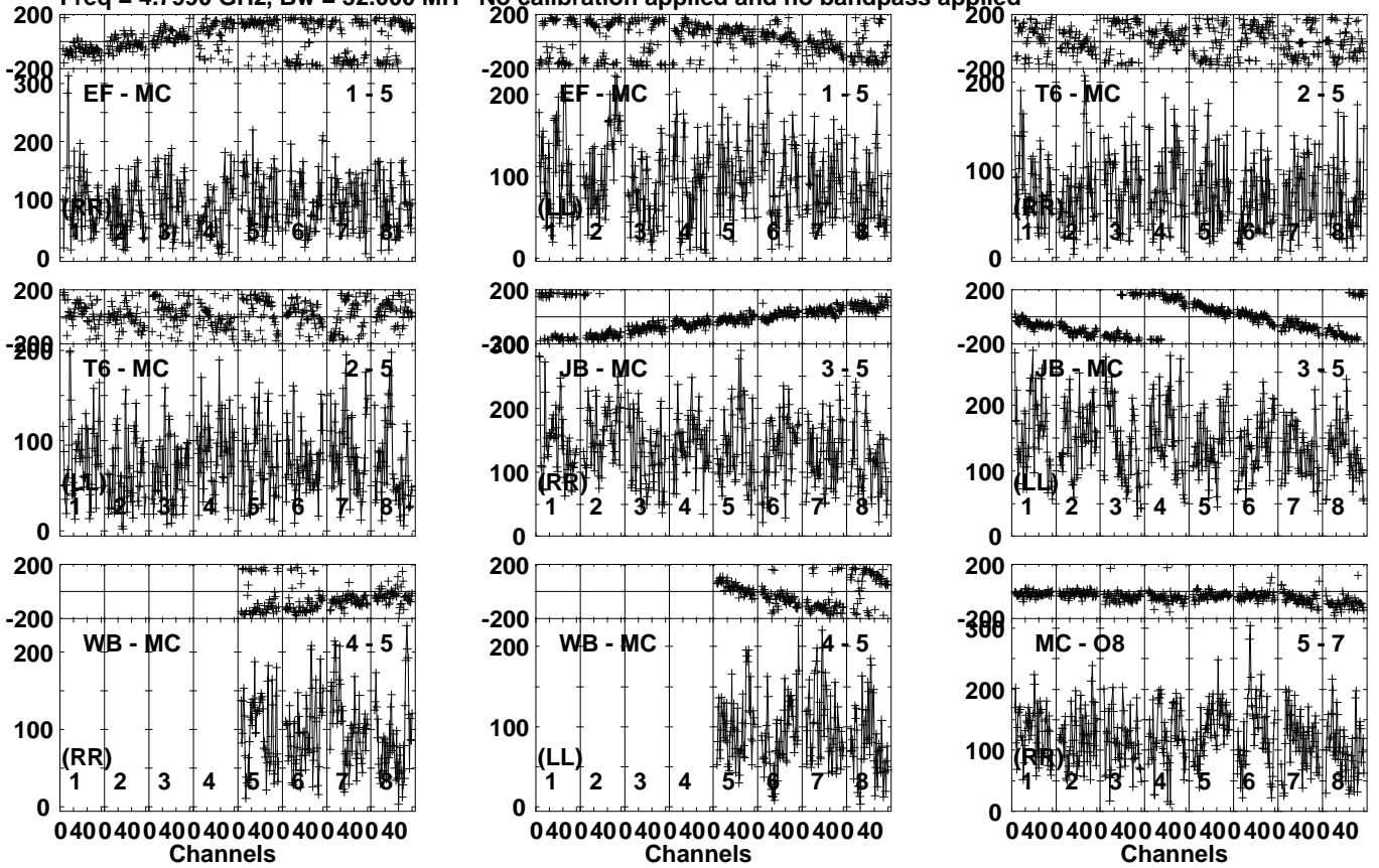
Lower frame: Micro Ampl Jy Top frame: Phas deg Vector averaged cross-power spectrum Several baselines displayed Timerange: 00/14:44:51 to 00/14:48:29
