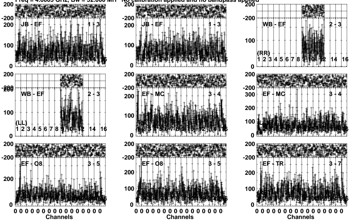
Lower frame: Micro Ampl Jy Top frame: Phas deg Vector averaged cross-power spectrum Several baselines displayed Timerange: 00/06:25:03 to 00/06:28:59
