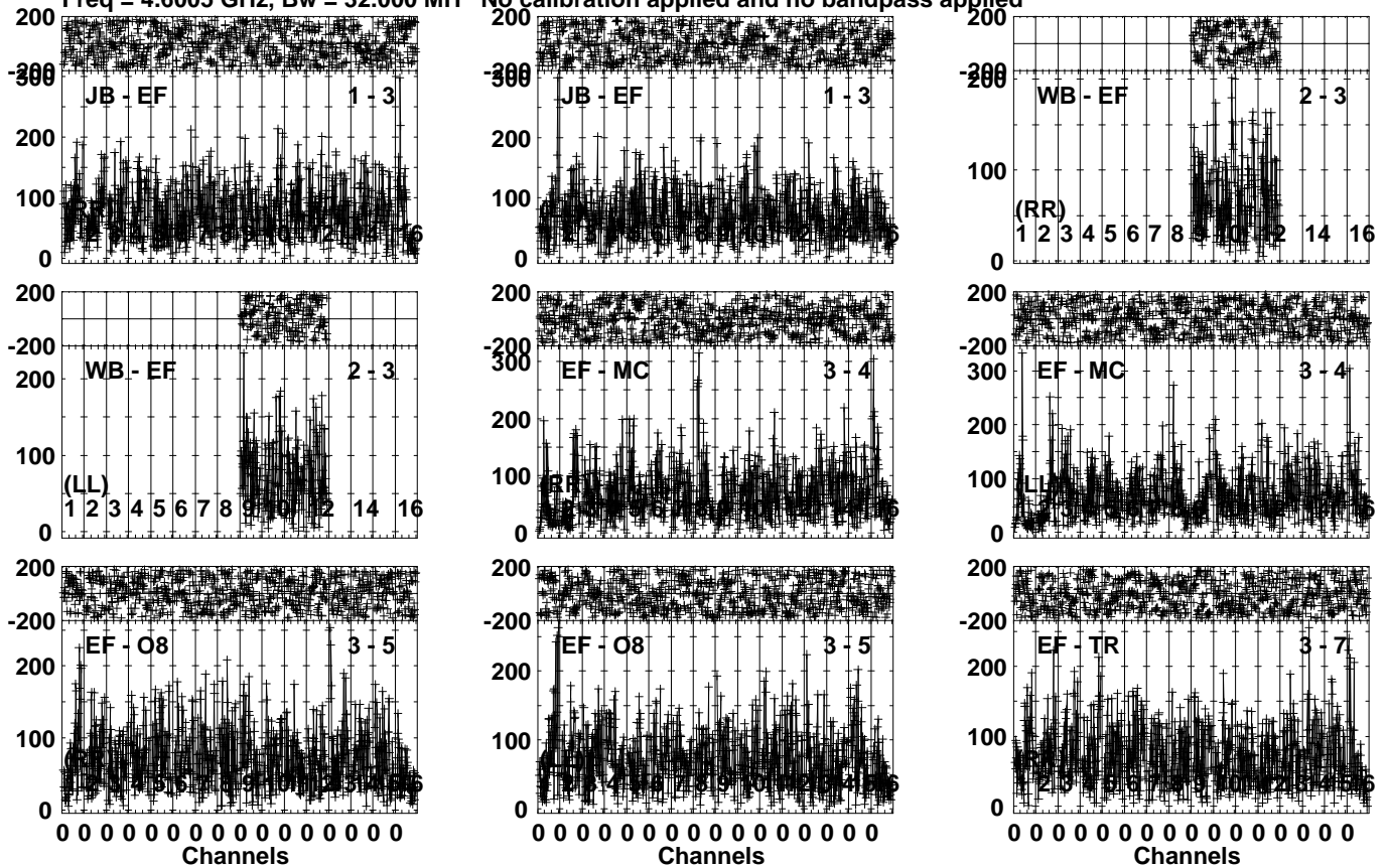
Lower frame: Micro Ampl Jy Top frame: Phas deg Vector averaged cross-power spectrum Several baselines displayed Timerange: 00/09:19:03 to 00/09:22:59
