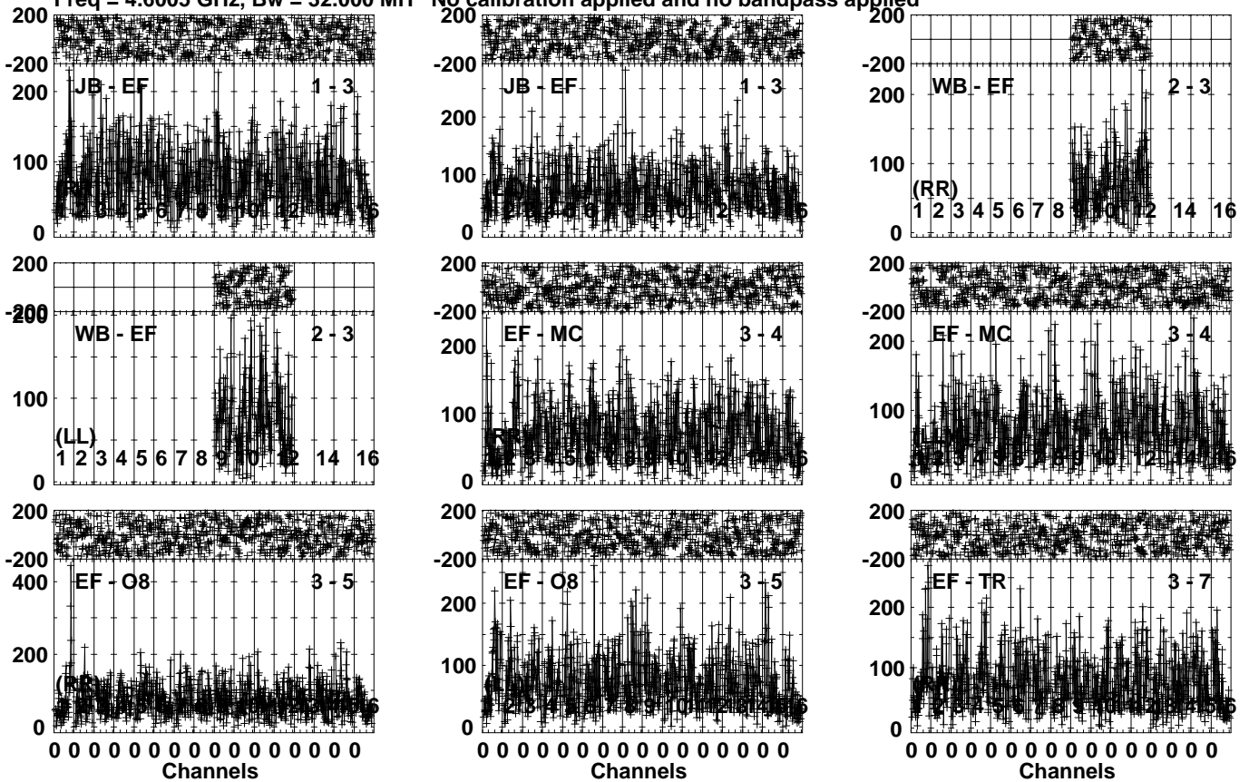
Lower frame: Micro Ampl Jy Top frame: Phas deg Vector averaged cross-power spectrum Several baselines displayed Timerange: 00/08:19:03 to 00/08:22:59
