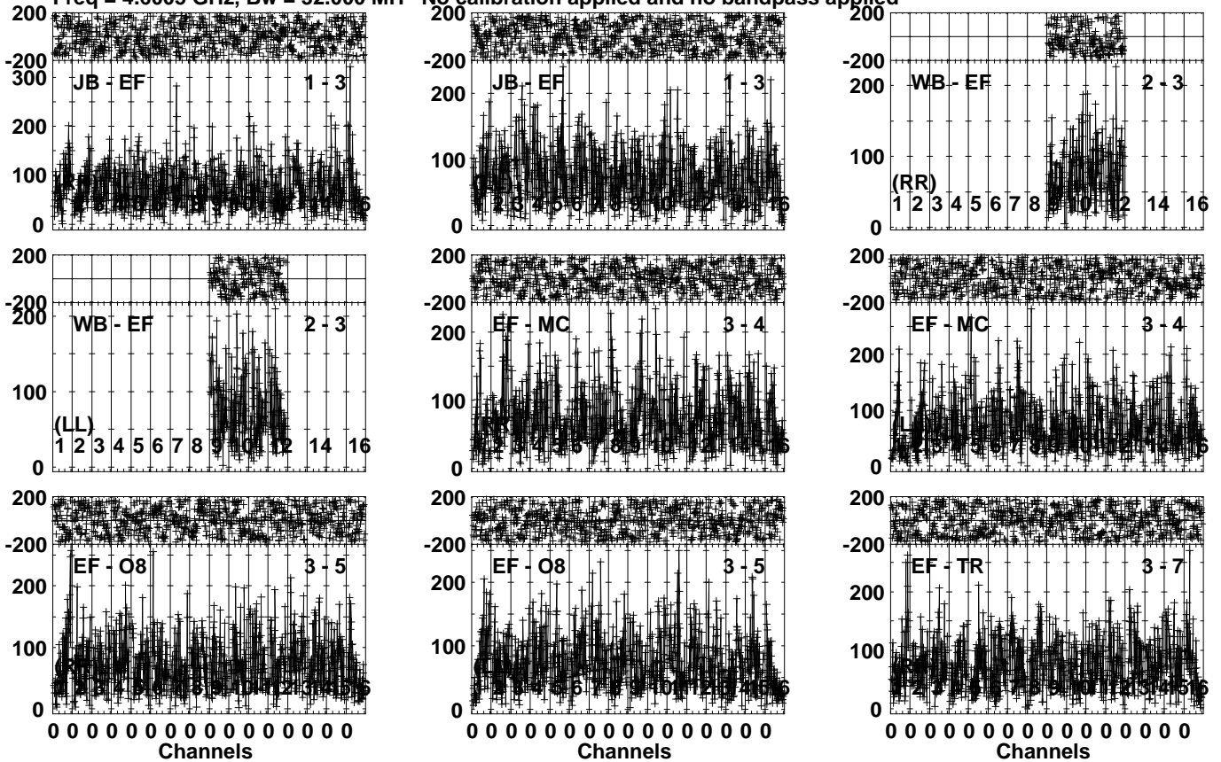
Lower frame: Micro Ampl Jy Top frame: Phas deg Vector averaged cross-power spectrum Several baselines displayed Timerange: 00/09:07:03 to 00/09:10:59
