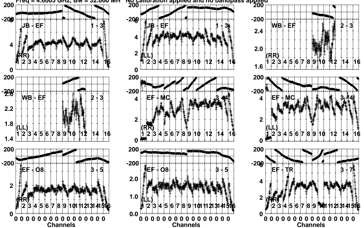
Lower frame: Milli Ampl Jy Top frame: Phas deg Vector averaged cross-power spectrum Several baselines displayed Timerange: 00/06:17:33 to 00/06:18:59
