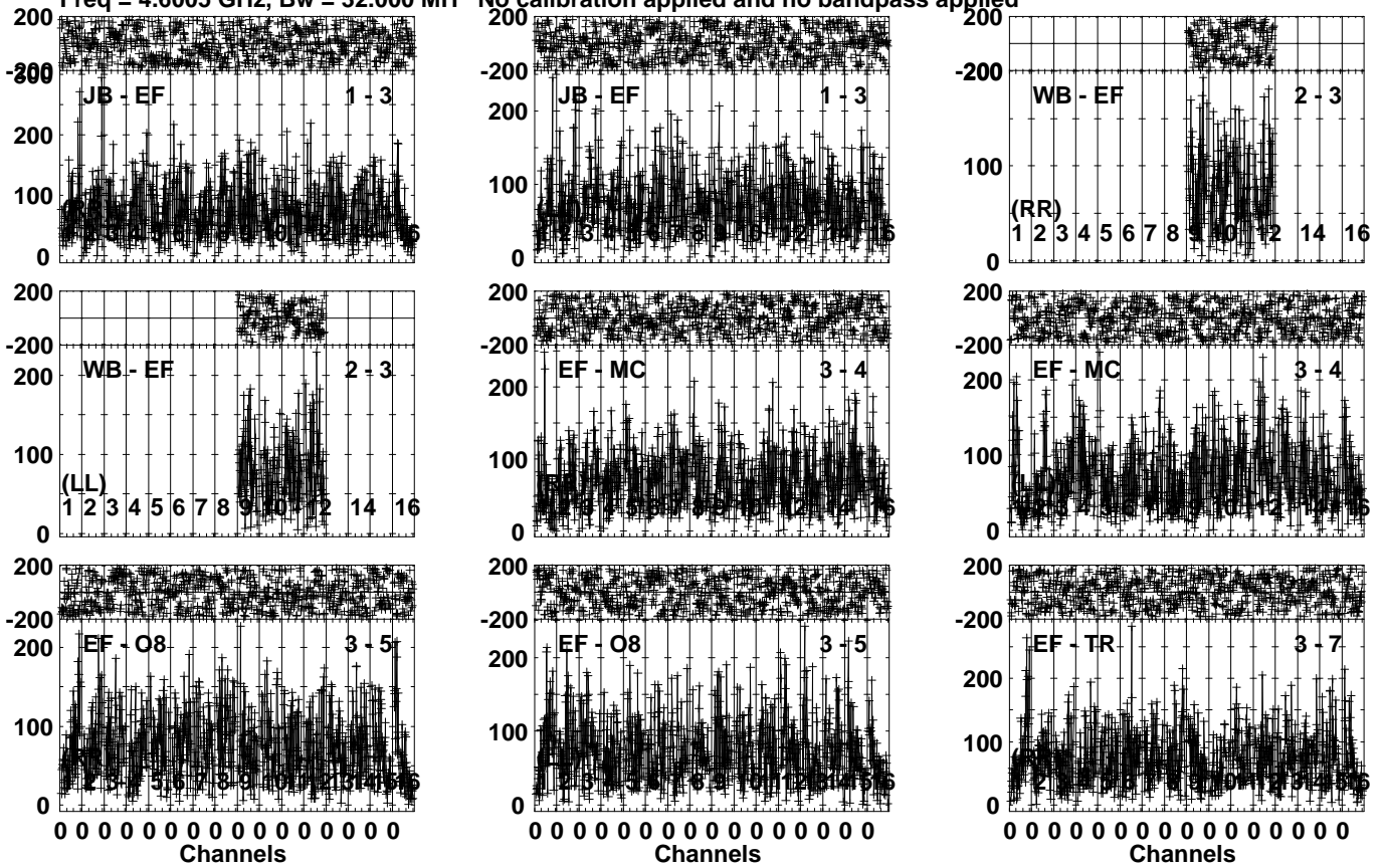
Lower frame: Micro Ampl Jy Top frame: Phas deg Vector averaged cross-power spectrum Several baselines displayed Timerange: 00/06:37:03 to 00/06:40:59
