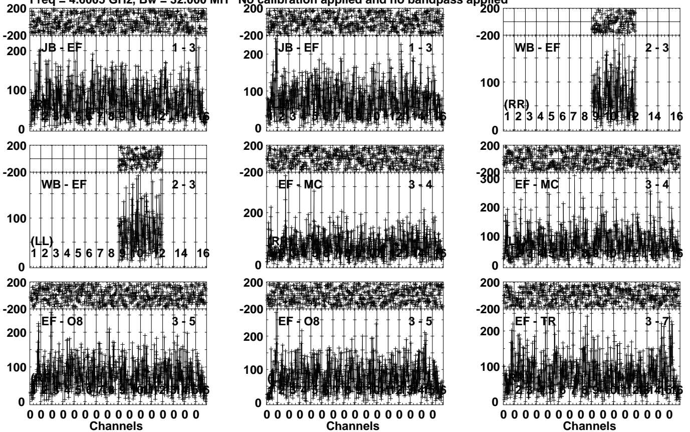
Lower frame: Micro Ampl Jy Top frame: Phas deg Vector averaged cross-power spectrum Several baselines displayed Timerange: 00/06:13:01 to 00/06:16:59
