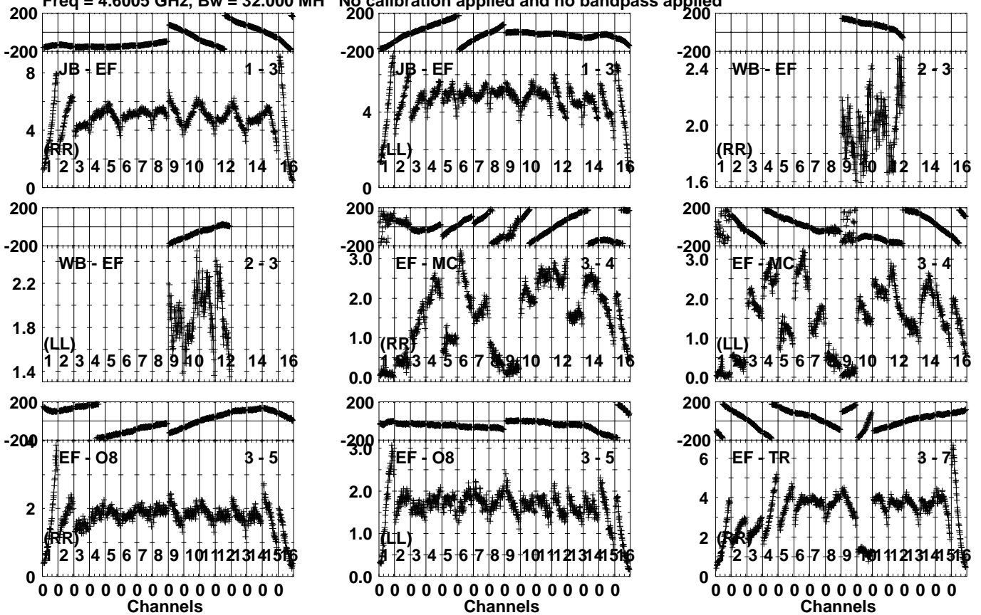
Lower frame: Milli Ampl Jy Top frame: Phas deg Vector averaged cross-power spectrum Several baselines displayed Timerange: 00/07:17:33 to 00/07:18:59
