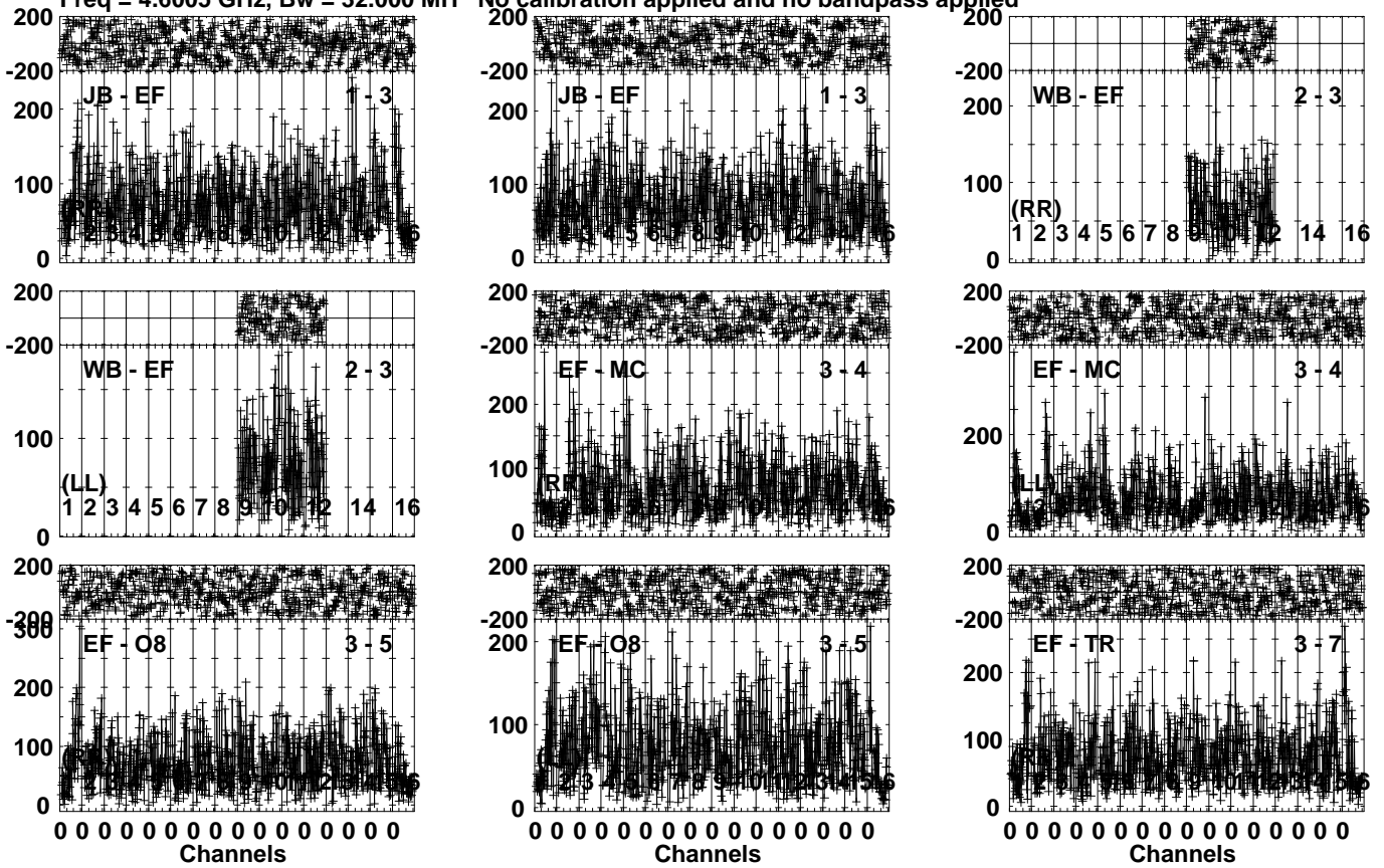
Lower frame: Micro Ampl Jy Top frame: Phas deg Vector averaged cross-power spectrum Several baselines displayed Timerange: 00/06:55:03 to 00/06:58:59
