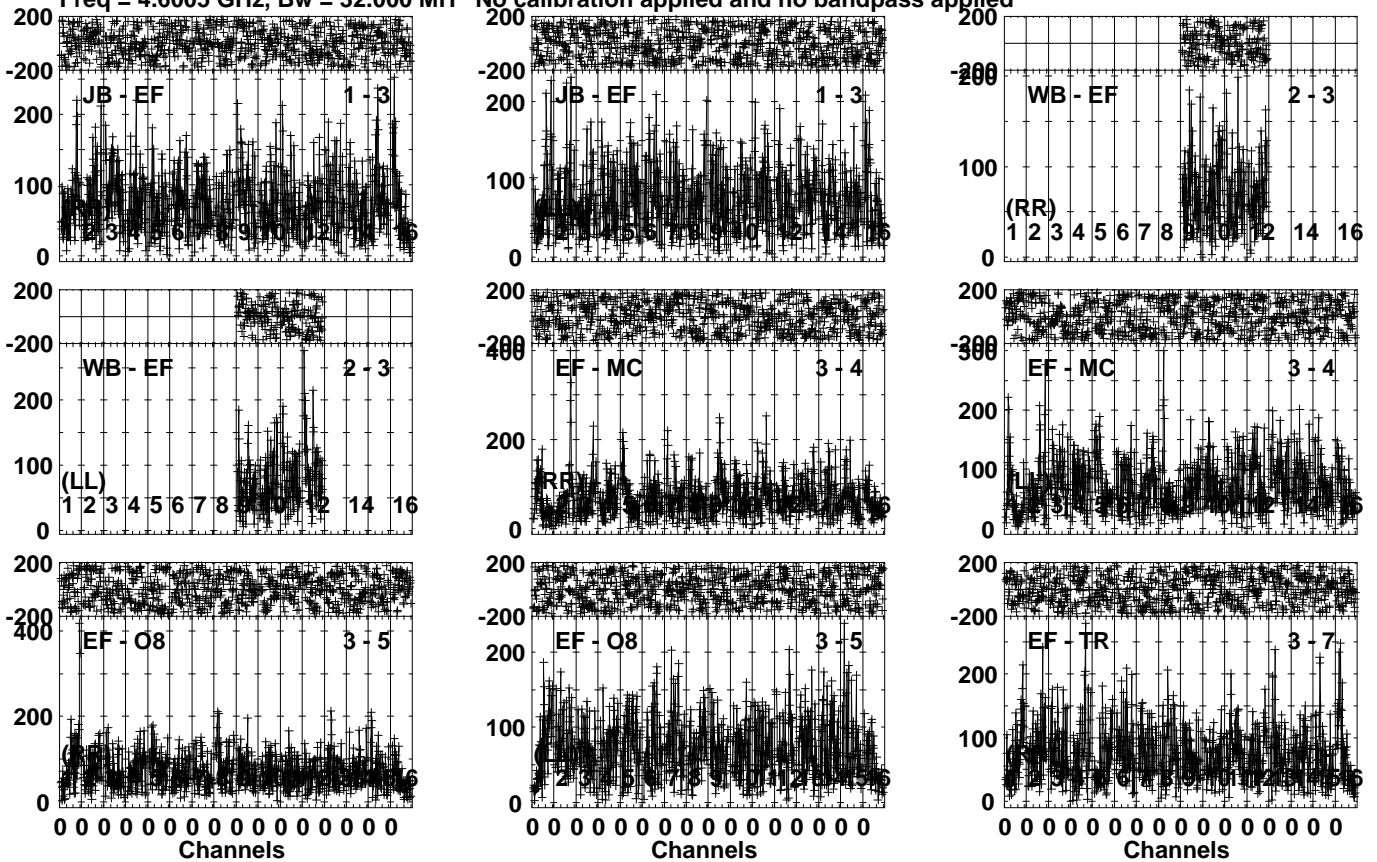
Lower frame: Micro Ampl Jy Top frame: Phas deg Vector averaged cross-power spectrum Several baselines displayed Timerange: 00/09:31:03 to 00/09:34:59
