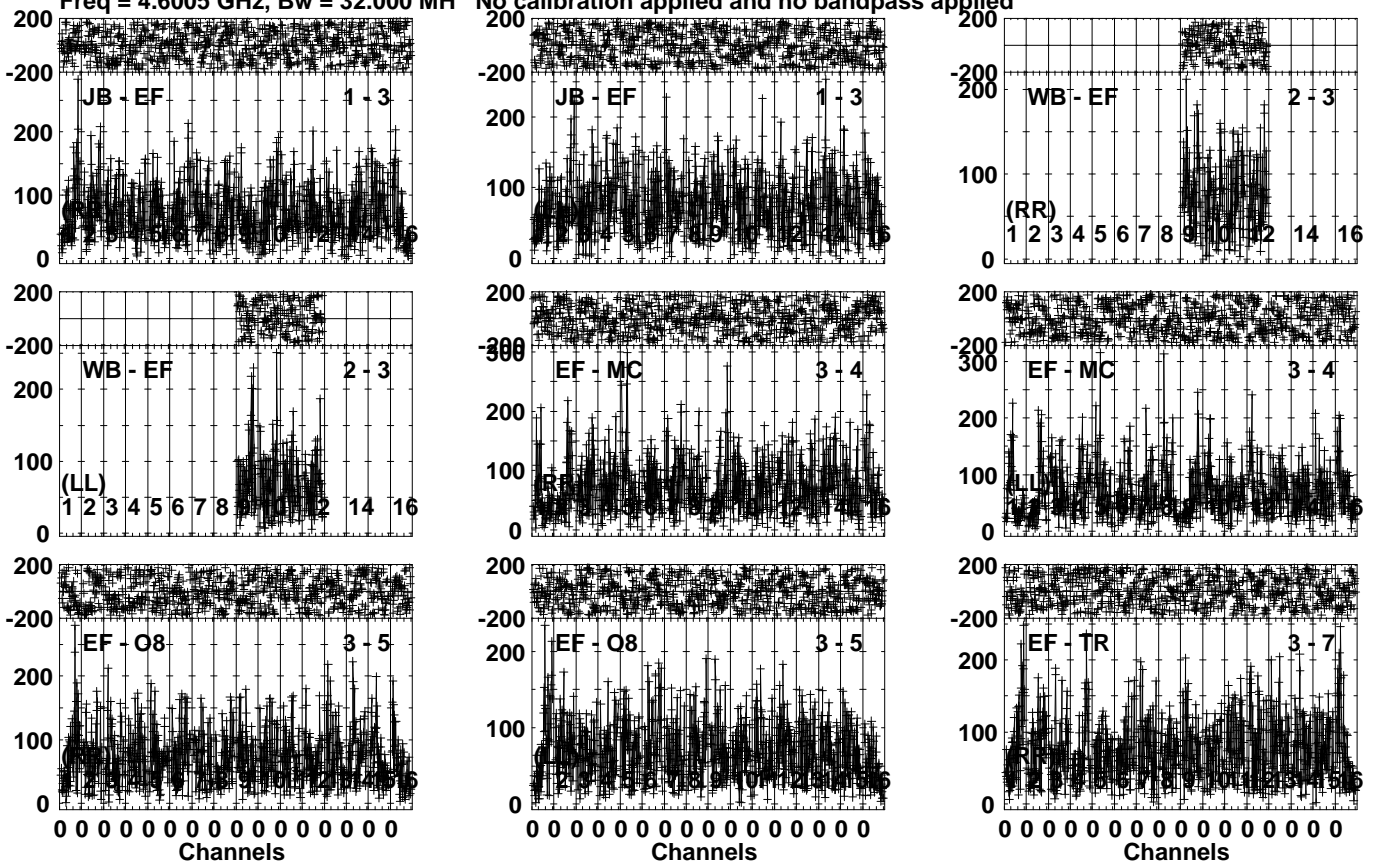
Lower frame: Micro Ampl Jy Top frame: Phas deg Vector averaged cross-power spectrum Several baselines displayed Timerange: 00/09:37:03 to 00/09:40:59
