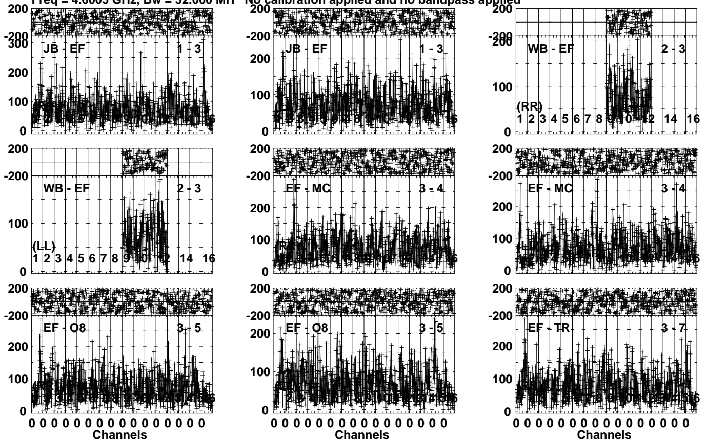
Lower frame: Micro Ampl Jy Top frame: Phas deg Vector averaged cross-power spectrum Several baselines displayed Timerange: 00/07:19:03 to 00/07:22:59
