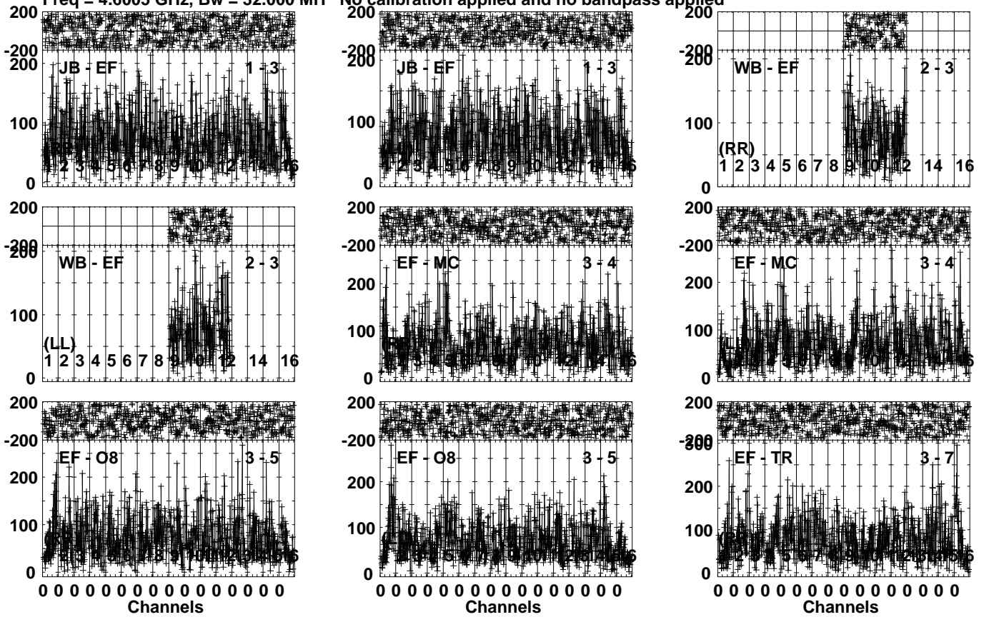
Lower frame: Micro Ampl Jy Top frame: Phas deg Vector averaged cross-power spectrum Several baselines displayed Timerange: 00/09:13:03 to 00/09:16:59
