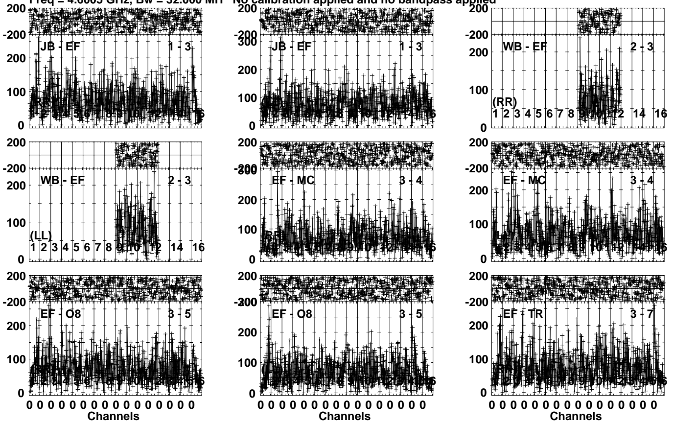
Lower frame: Micro Ampl Jy Top frame: Phas deg Vector averaged cross-power spectrum Several baselines displayed Timerange: 00/07:55:03 to 00/07:58:59
