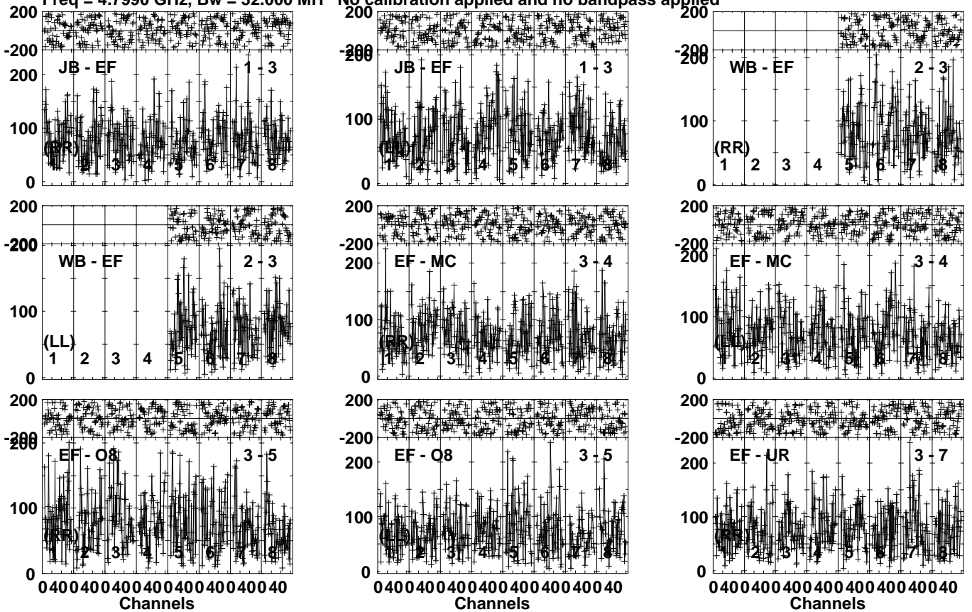
Lower frame: Micro Ampl Jy Top frame: Phas deg Vector averaged cross-power spectrum Several baselines displayed Timerange: 00/12:20:03 to 00/12:23:59
