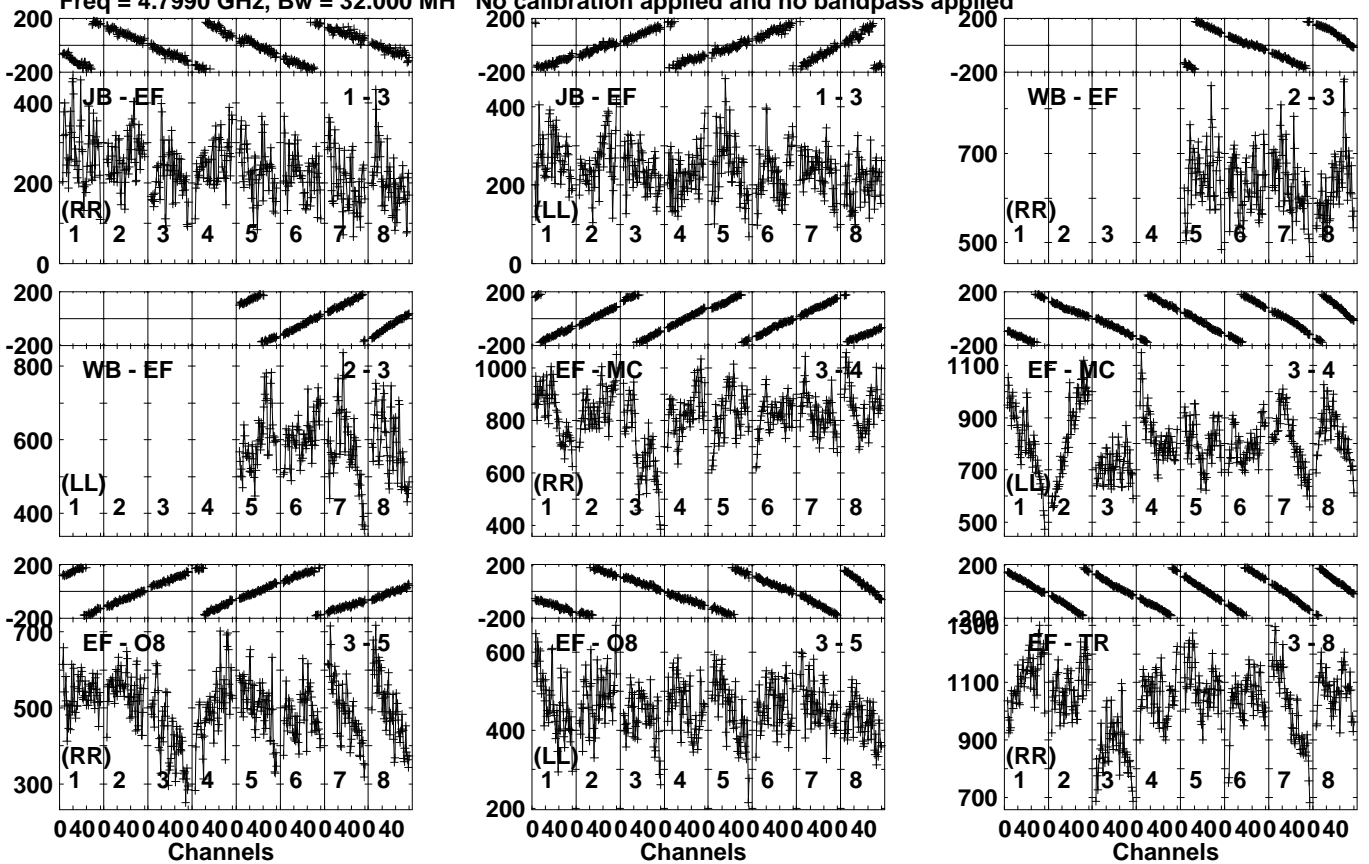
Lower frame: Micro Ampl Jy Top frame: Phas deg Vector averaged cross-power spectrum Several baselines displayed Timerange: 00/18:48:01 to 00/18:51:59
