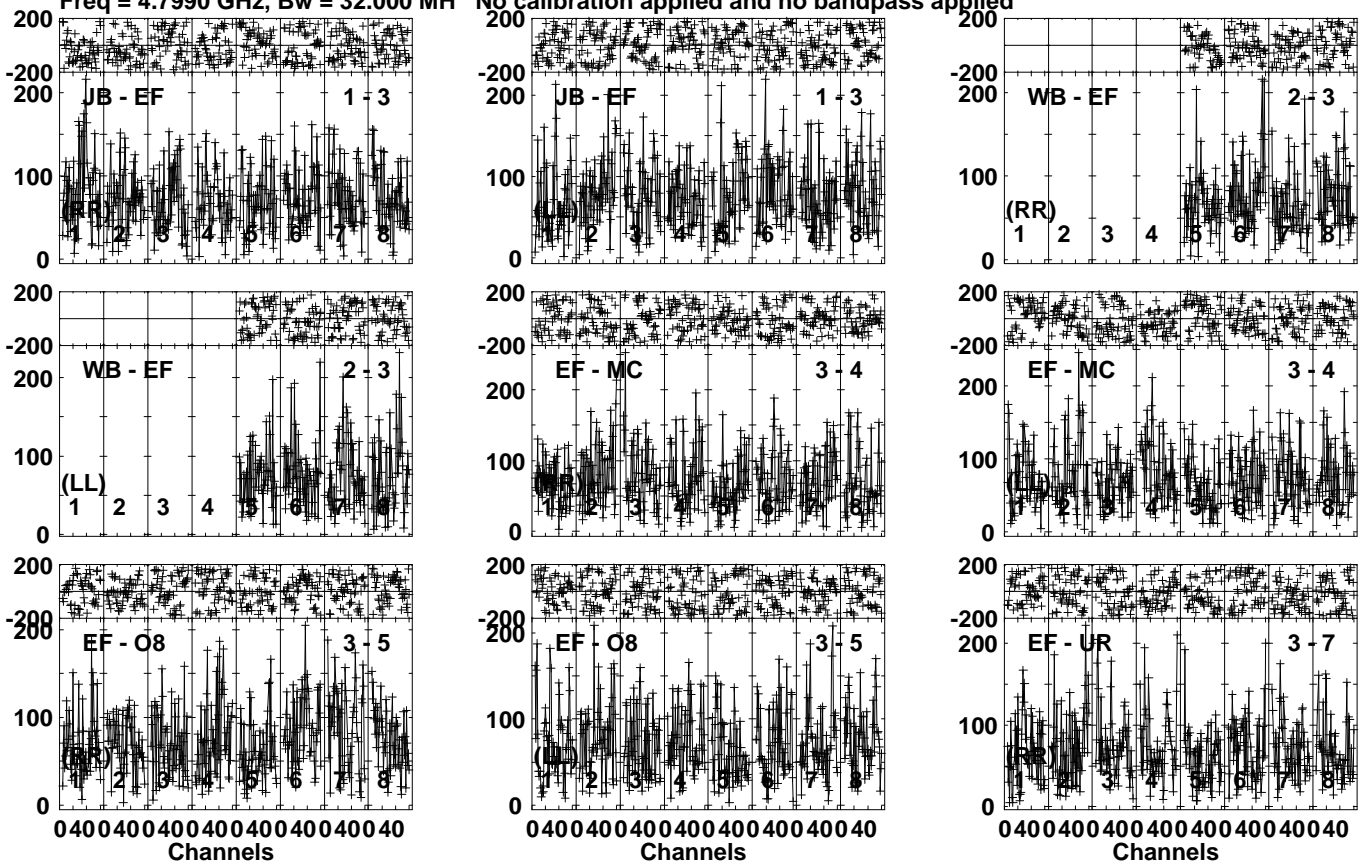
Lower frame: Micro Ampl Jy Top frame: Phas deg Vector averaged cross-power spectrum Several baselines displayed Timerange: 00/14:14:01 to 00/14:17:59
