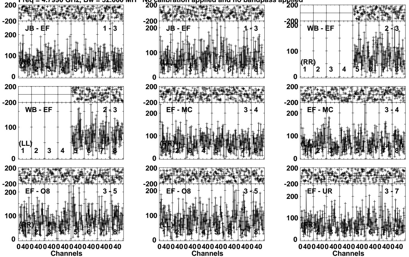
Lower frame: Micro Ampl Jy Top frame: Phas deg Vector averaged cross-power spectrum Several baselines displayed Timerange: 00/14:50:01 to 00/14:53:59
