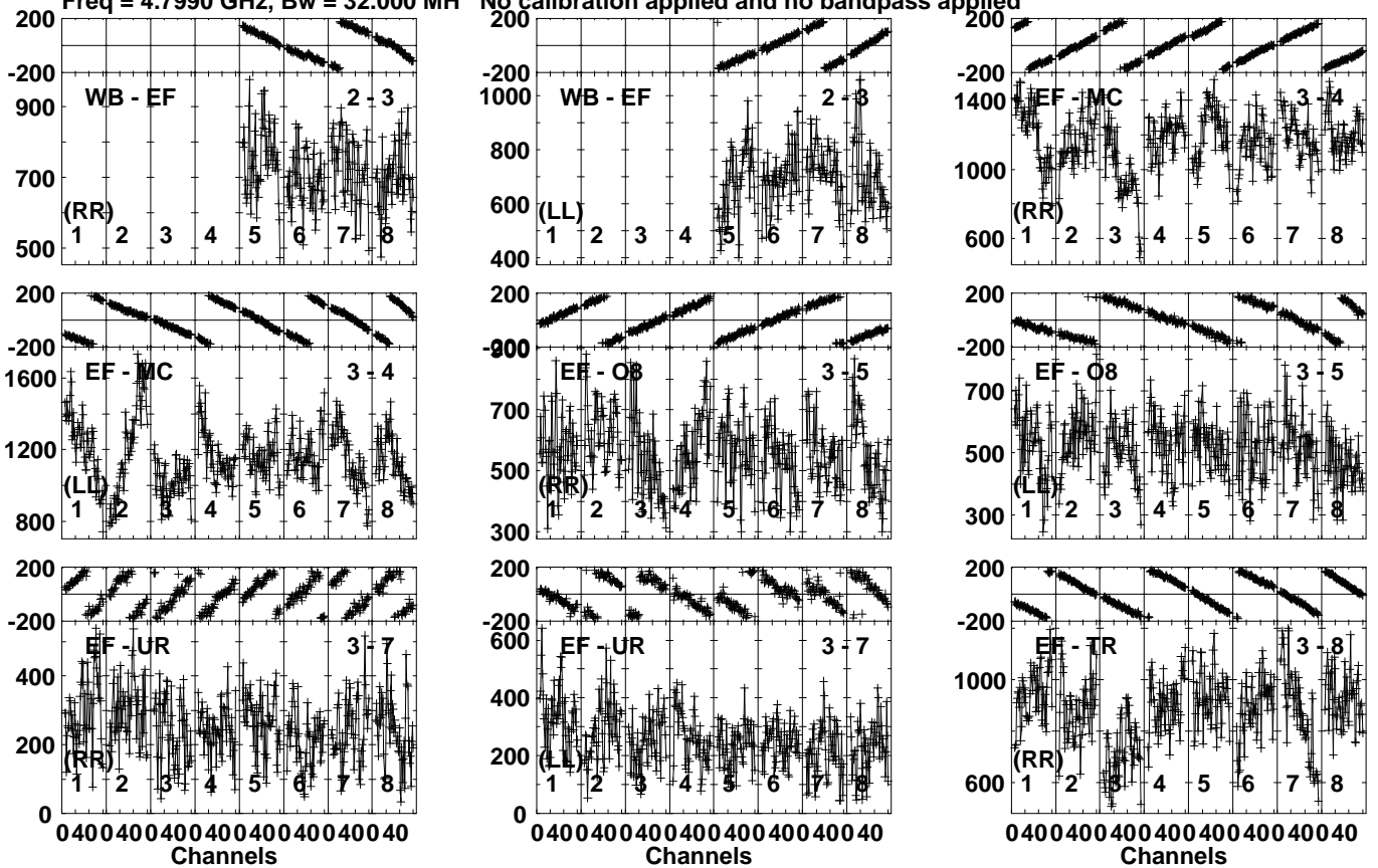
Lower frame: Micro Ampl Jy Top frame: Phas deg Vector averaged cross-power spectrum Several baselines displayed Timerange: 00/12:12:31 to 00/12:13:59
