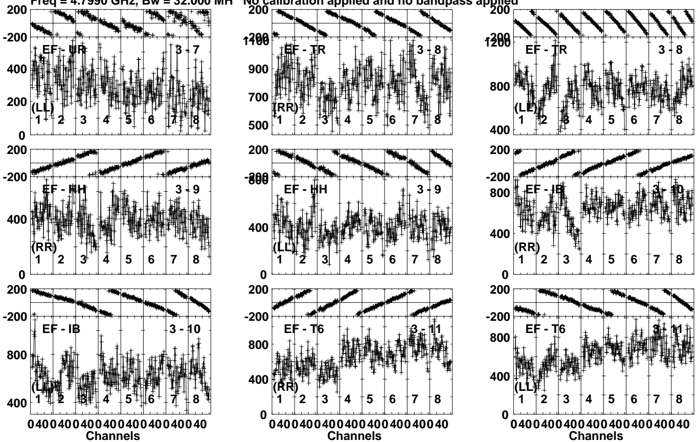
Lower frame: Micro Ampl Jy Top frame: Phas deg Vector averaged cross-power spectrum Several baselines displayed Timerange: 00/12:42:31 to 00/12:43:59
