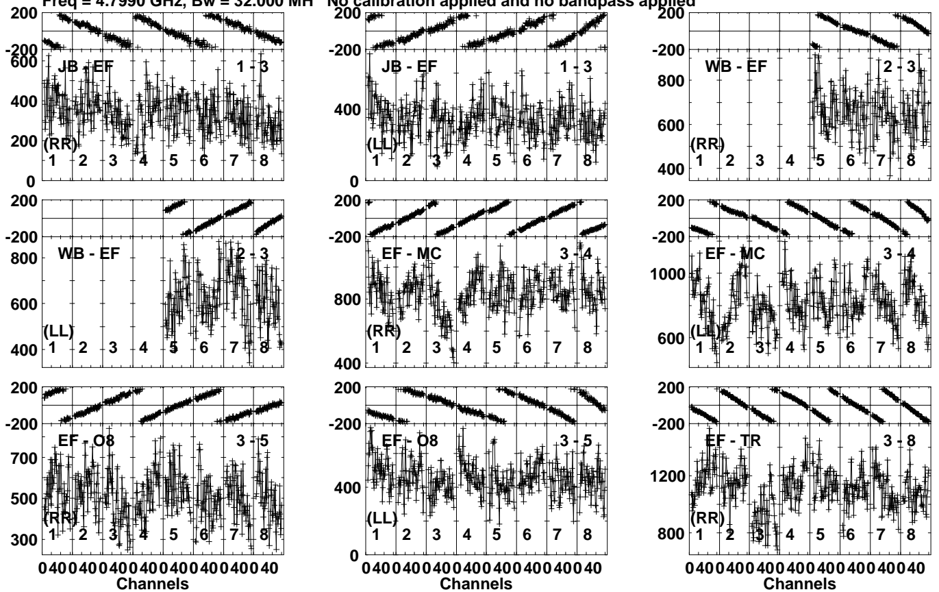
Lower frame: Micro Ampl Jy Top frame: Phas deg Vector averaged cross-power spectrum Several baselines displayed Timerange: 00/18:42:31 to 00/18:43:59
