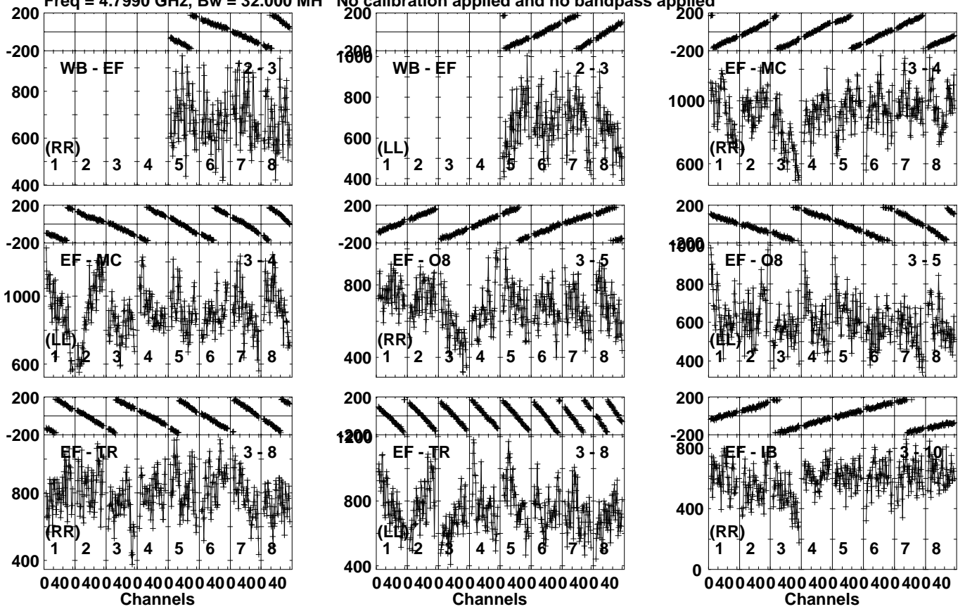
Lower frame: Micro Ampl Jy Top frame: Phas deg Vector averaged cross-power spectrum Several baselines displayed Timerange: 00/17:12:31 to 00/17:13:59
