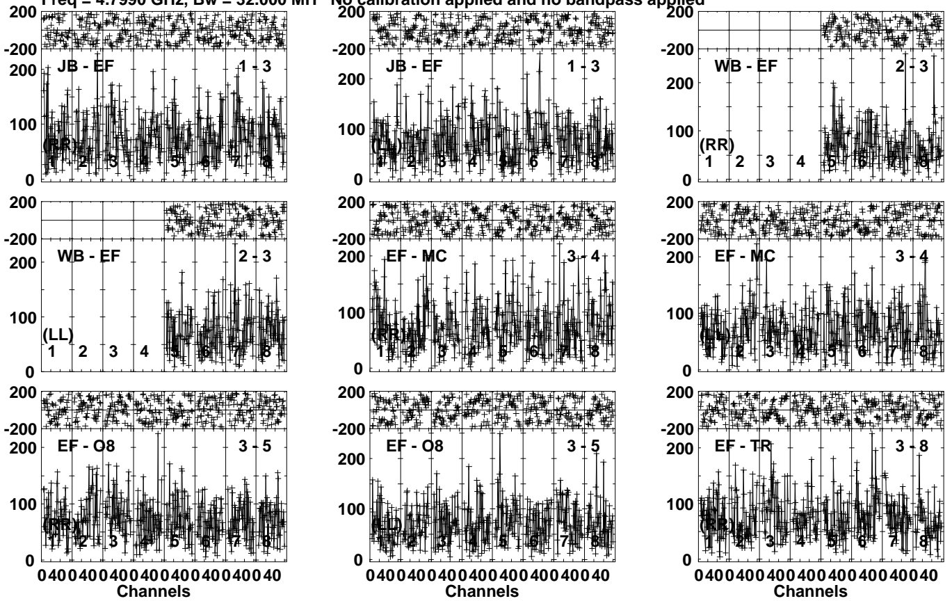
Lower frame: Micro Ampl Jy Top frame: Phas deg Vector averaged cross-power spectrum Several baselines displayed Timerange: 00/17:26:01 to 00/17:29:59
