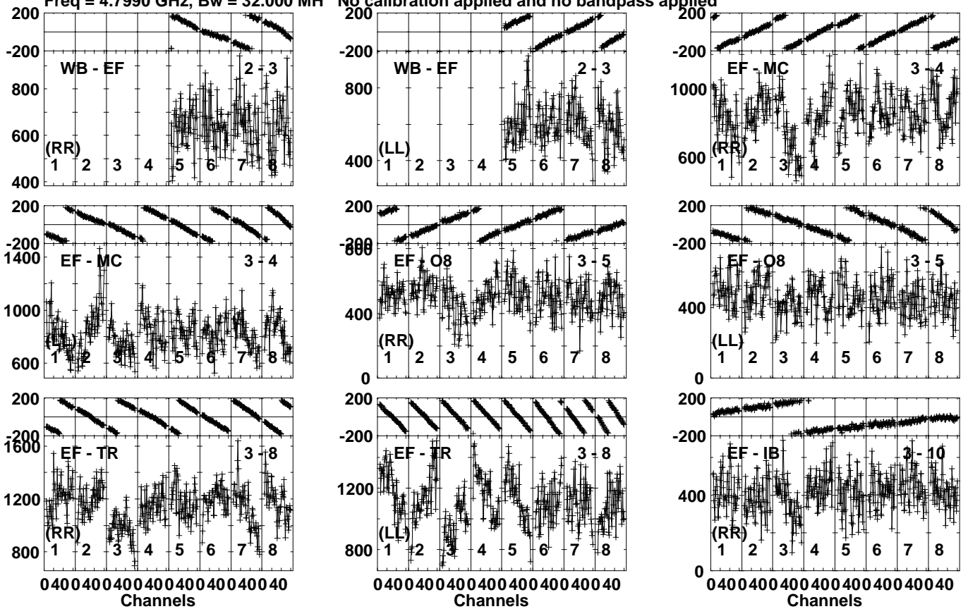
Lower frame: Micro Ampl Jy Top frame: Phas deg Vector averaged cross-power spectrum Several baselines displayed Timerange: 00/18:36:31 to 00/18:37:59
