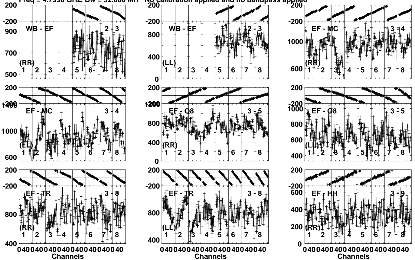
Lower frame: Micro Ampl Jy Top frame: Phas deg Vector averaged cross-power spectrum Several baselines displayed Timerange: 00/16:36:31 to 00/16:37:59
