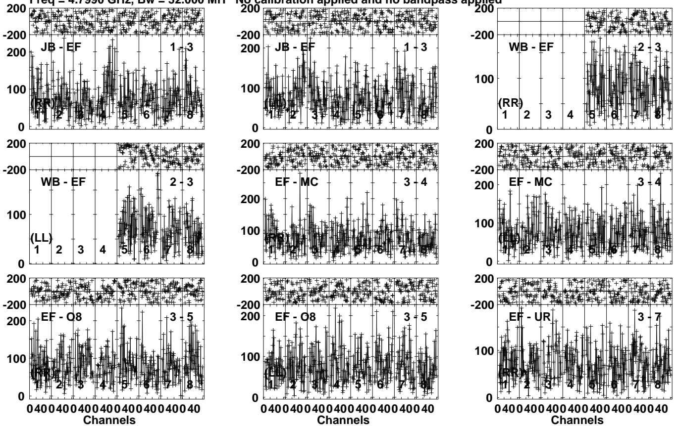
Lower frame: Micro Ampl Jy Top frame: Phas deg Vector averaged cross-power spectrum Several baselines displayed Timerange: 00/11:20:03 to 00/11:23:59
