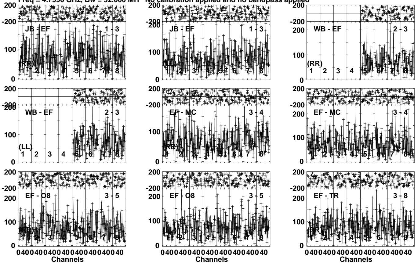
Lower frame: Micro Ampl Jy Top frame: Phas deg Vector averaged cross-power spectrum Several baselines displayed Timerange: 00/16:56:03 to 00/16:59:59
