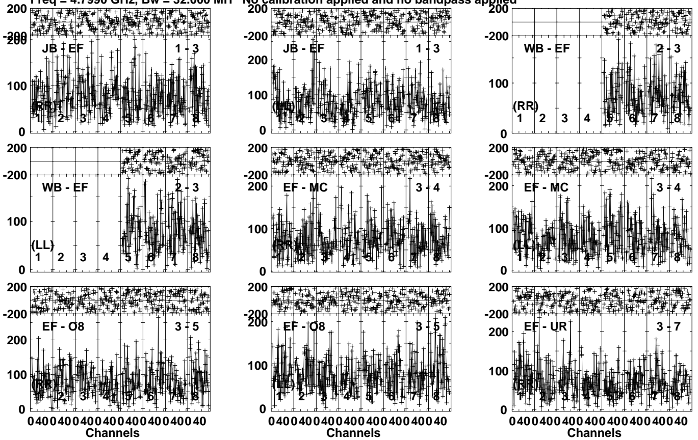
Lower frame: Micro Ampl Jy Top frame: Phas deg Vector averaged cross-power spectrum Several baselines displayed Timerange: 00/11:44:03 to 00/11:47:59
