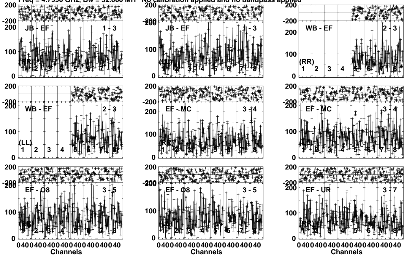
Lower frame: Micro Ampl Jy Top frame: Phas deg Vector averaged cross-power spectrum Several baselines displayed Timerange: 00/13:20:01 to 00/13:23:59
