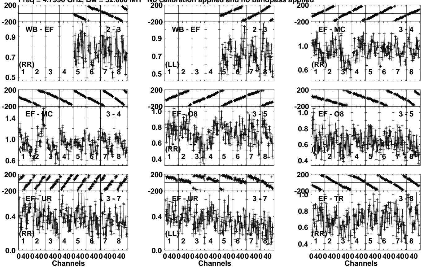
Lower frame: Milli Ampl Jy Top frame: Phas deg Vector averaged cross-power spectrum Several baselines displayed Timerange: 00/14:24:31 to 00/14:25:59
