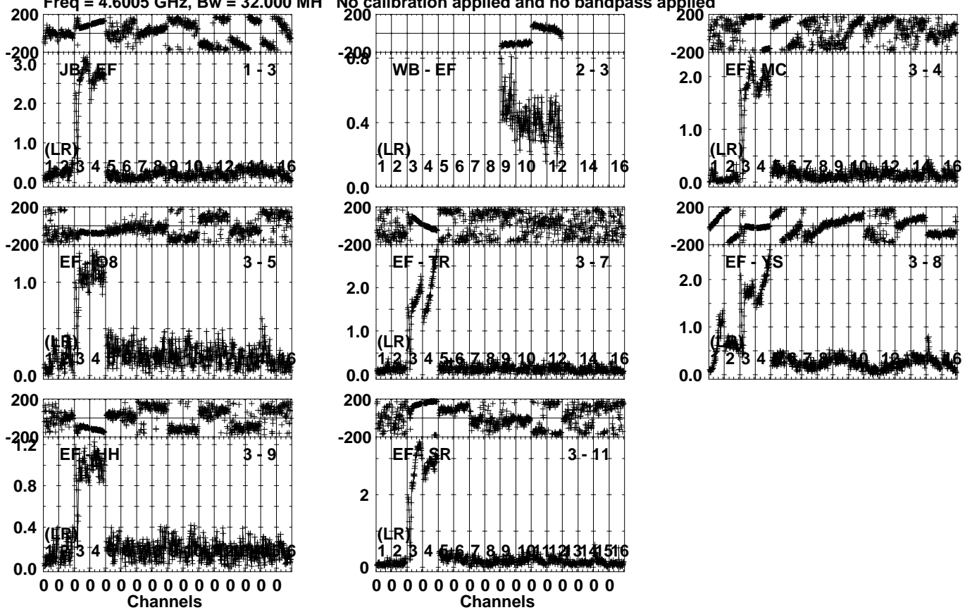
Lower frame: Milli Ampl Jy Top frame: Phas deg Vector averaged cross-power spectrum Several baselines displayed Timerange: 01/00:26:33 to 01/00:28:29
