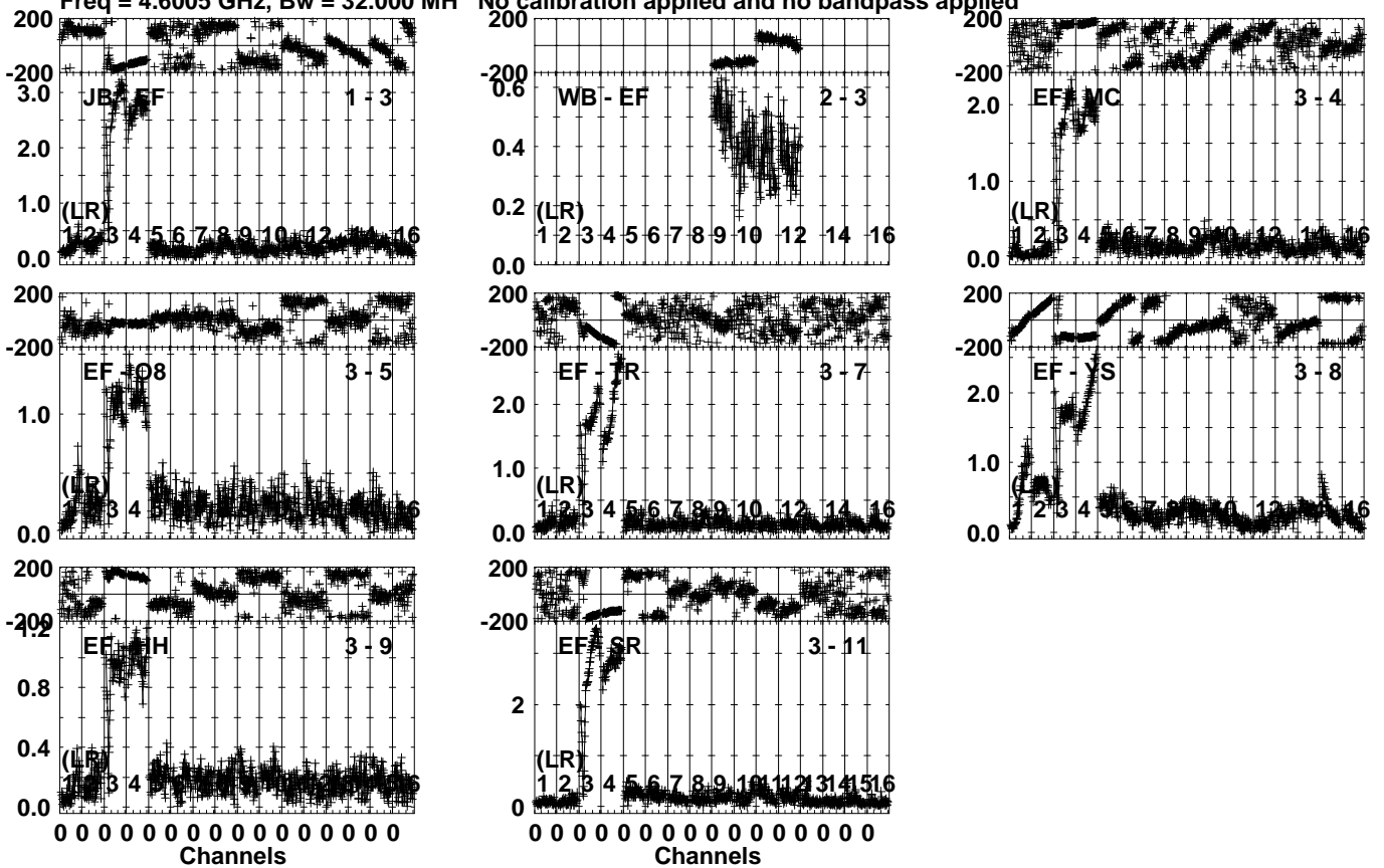
Lower frame: Milli Ampl Jy Top frame: Phas deg Vector averaged cross-power spectrum Several baselines displayed Timerange: 01/00:14:03 to 01/00:15:59
