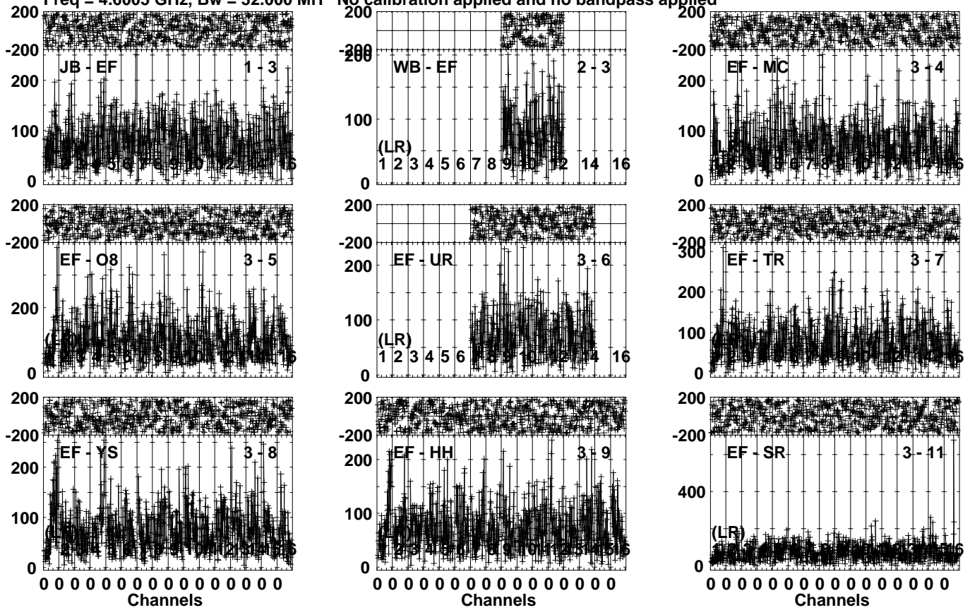
Lower frame: Micro Ampl Jy Top frame: Phas deg Vector averaged cross-power spectrum Several baselines displayed Timerange: 00/23:19:33 to 00/23:23:29
