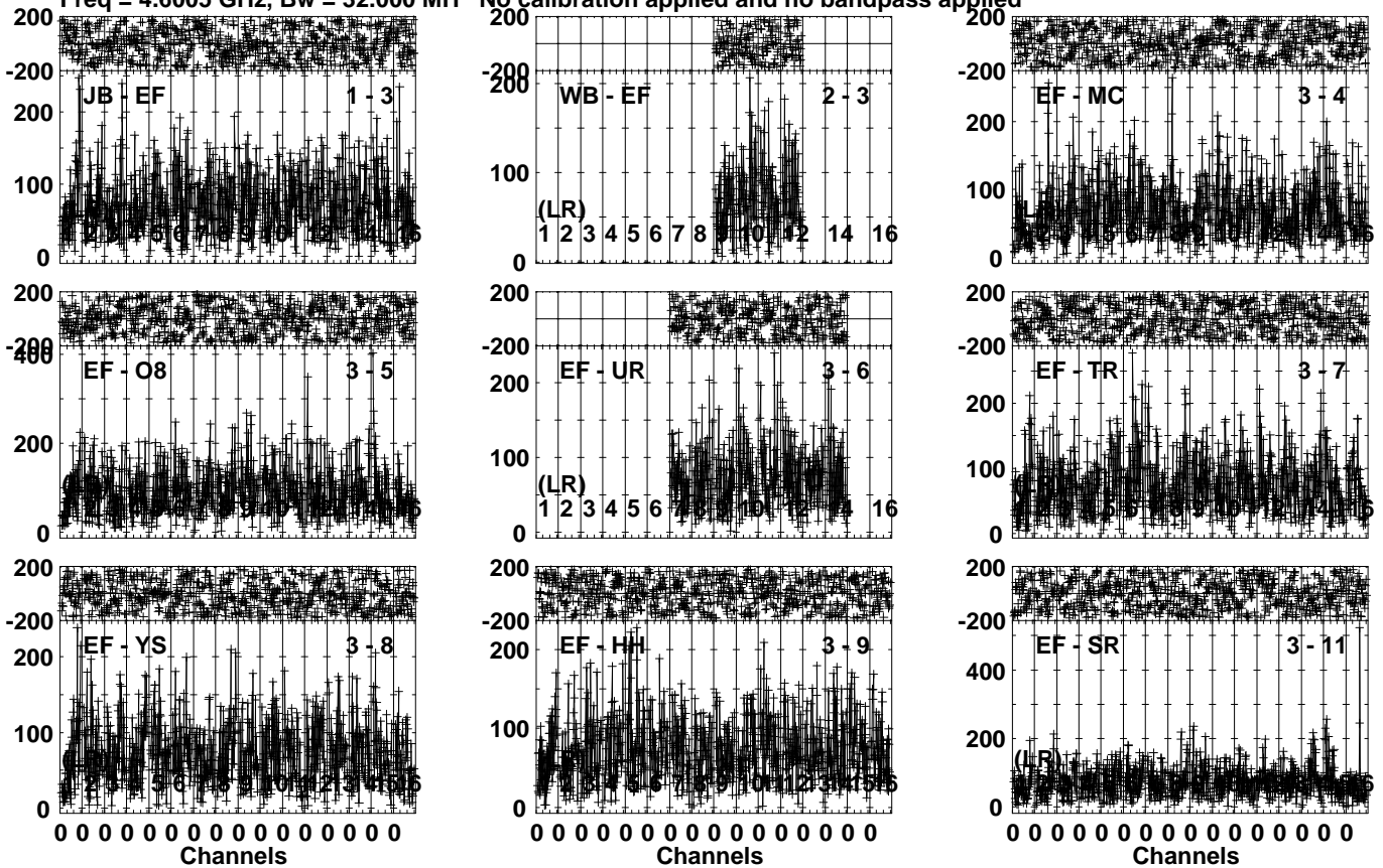
Lower frame: Micro Ampl Jy Top frame: Phas deg Vector averaged cross-power spectrum Several baselines displayed Timerange: 00/23:01:03 to 00/23:04:59
