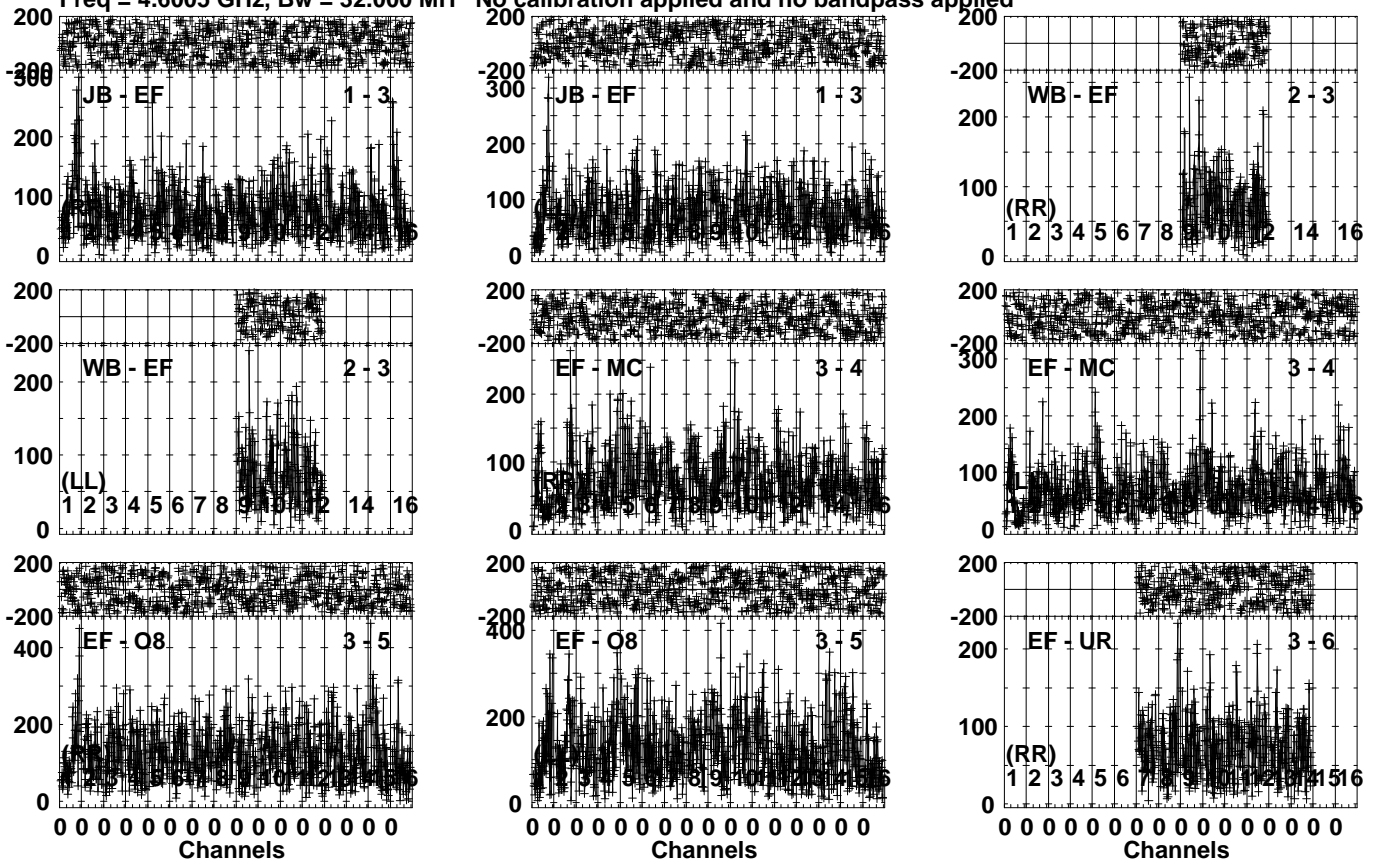
Lower frame: Micro Ampl Jy Top frame: Phas deg Vector averaged cross-power spectrum Several baselines displayed Timerange: 00/22:48:33 to 00/22:52:29
