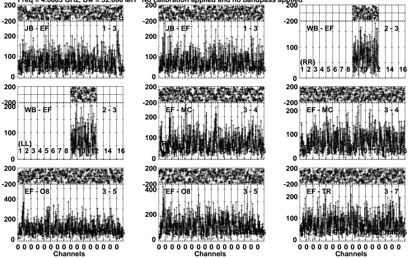
Lower frame: Micro Ampl Jy Top frame: Phas deg Vector averaged cross-power spectrum Several baselines displayed Timerange: 01/00:03:33 to 01/00:07:29
