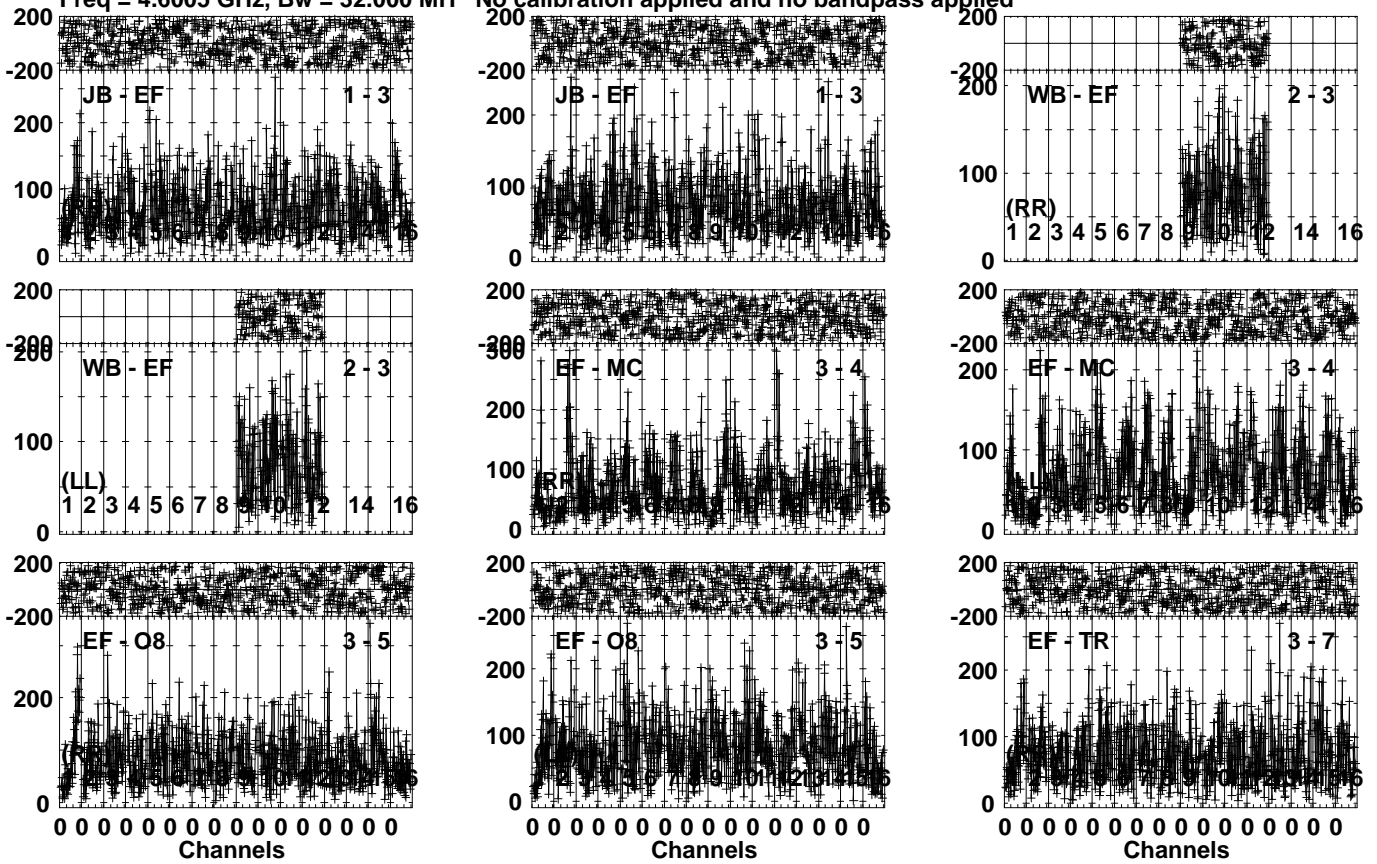
Lower frame: Micro Ampl Jy Top frame: Phas deg Vector averaged cross-power spectrum Several baselines displayed Timerange: 01/02:02:03 to 01/02:05:59
