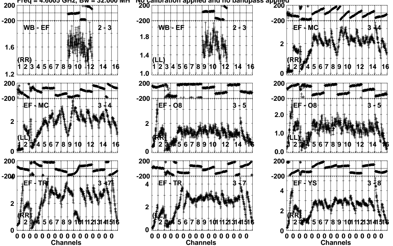
Lower frame: Milli Ampl Jy Top frame: Phas deg Vector averaged cross-power spectrum Several baselines displayed Timerange: 00/23:43:03 to 00/23:44:29
