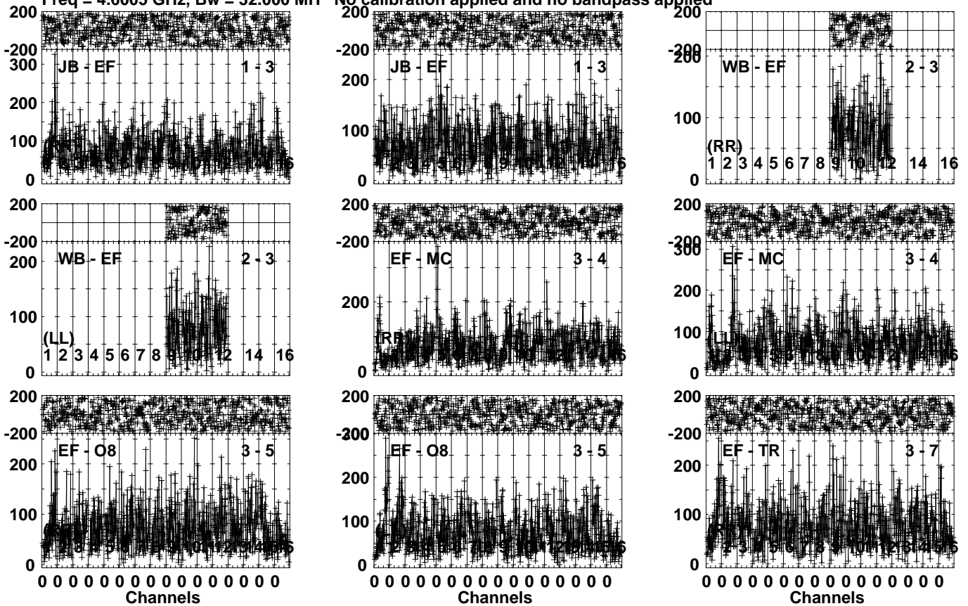
Lower frame: Micro Ampl Jy Top frame: Phas deg Vector averaged cross-power spectrum Several baselines displayed Timerange: 01/01:49:33 to 01/01:53:29
