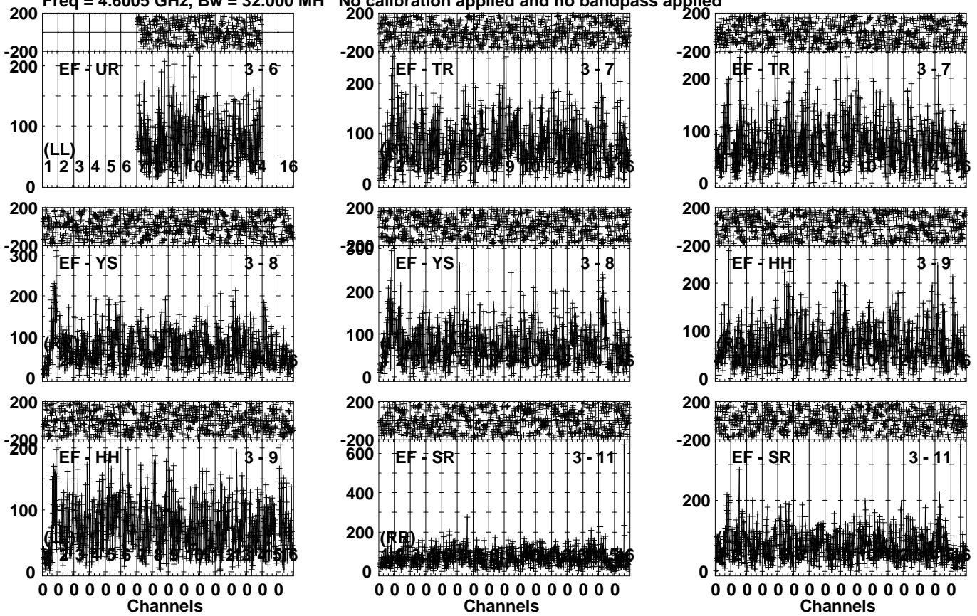
Lower frame: Micro Ampl Jy Top frame: Phas deg Vector averaged cross-power spectrum Several baselines displayed Timerange: 00/22:42:01 to 00/22:45:59
