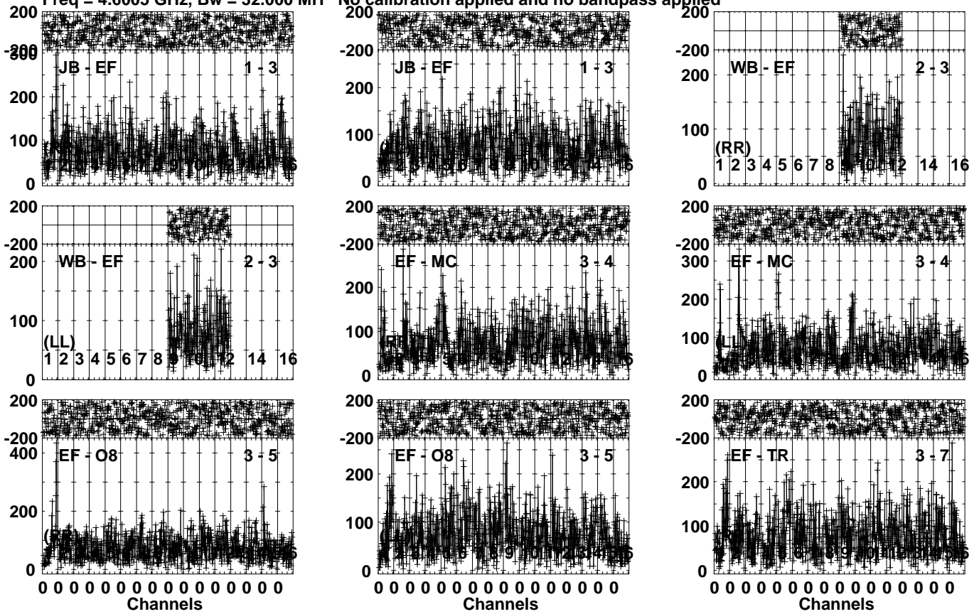
Lower frame: Micro Ampl Jy Top frame: Phas deg Vector averaged cross-power spectrum Several baselines displayed Timerange: 01/02:14:33 to 01/02:18:29
