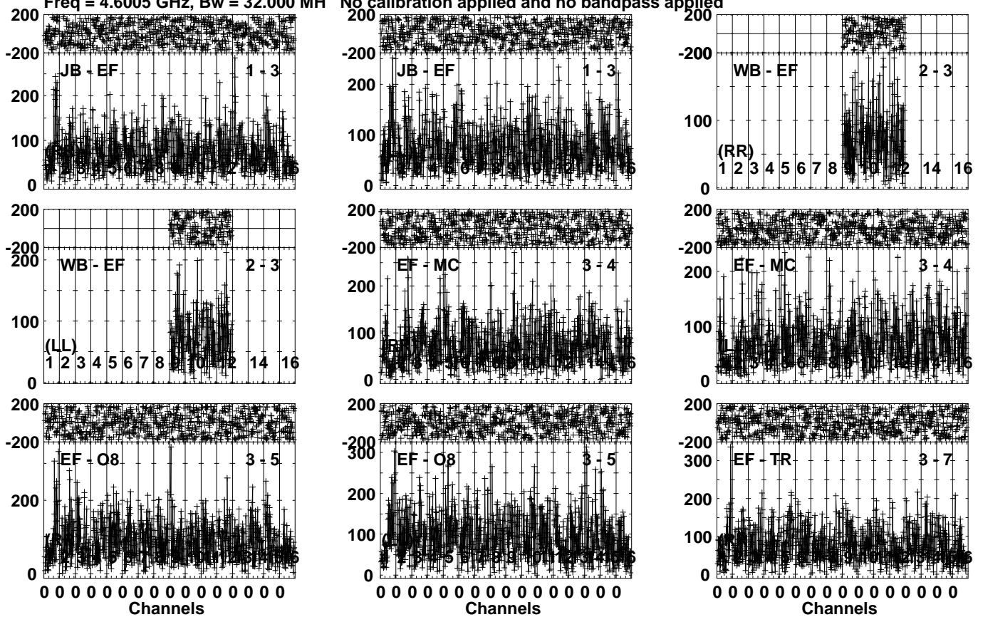
Lower frame: Micro Ampl Jy Top frame: Phas deg Vector averaged cross-power spectrum Several baselines displayed Timerange: 01/00:41:03 to 01/00:44:59
