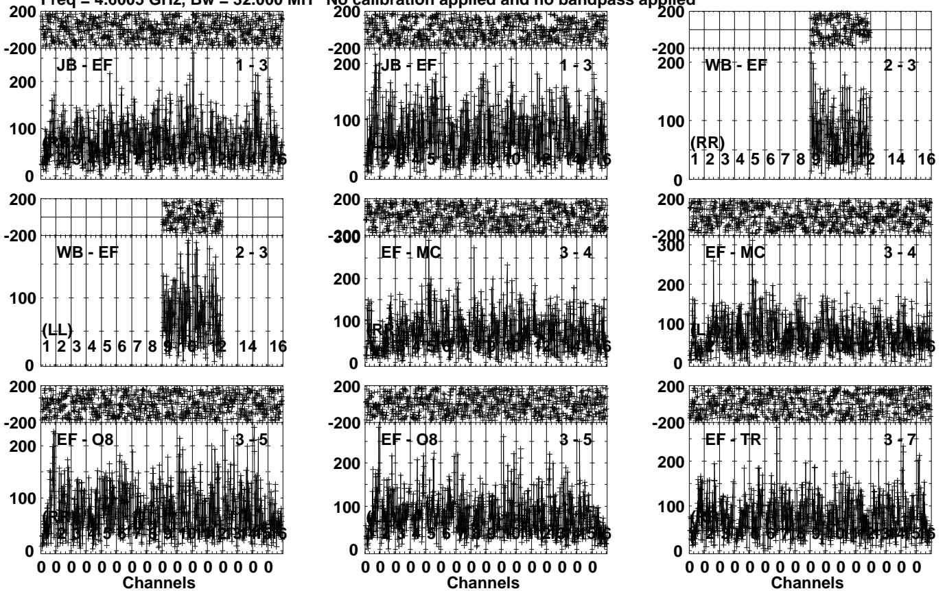
Lower frame: Micro Ampl Jy Top frame: Phas deg Vector averaged cross-power spectrum Several baselines displayed Timerange: 01/01:12:03 to 01/01:15:59
