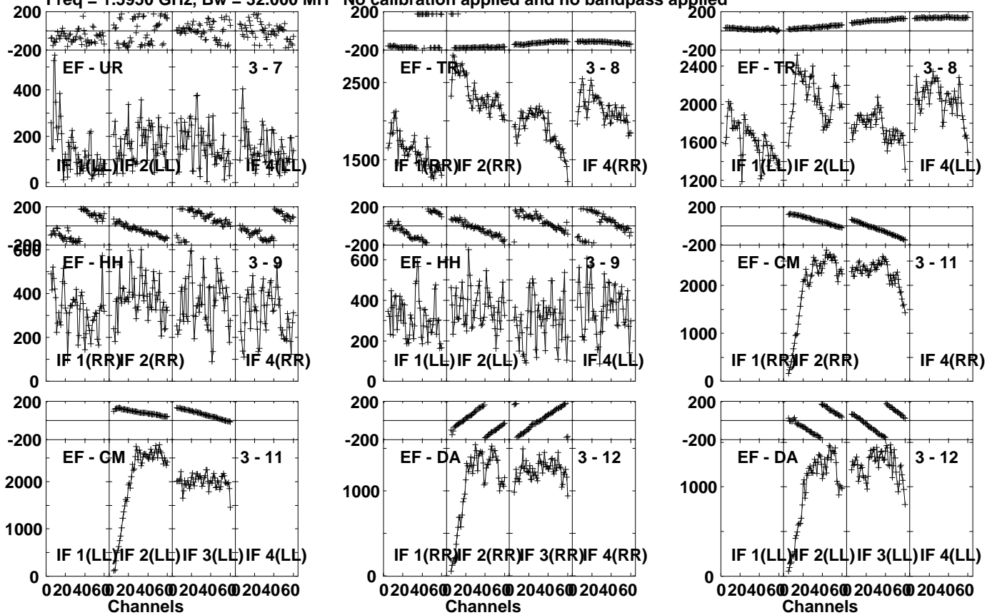
Lower frame: Micro Ampl Jy Top frame: Phas deg Vector averaged cross-power spectrum Several baselines displayed Timerange: 00/12:31:11 to 00/12:32:09
