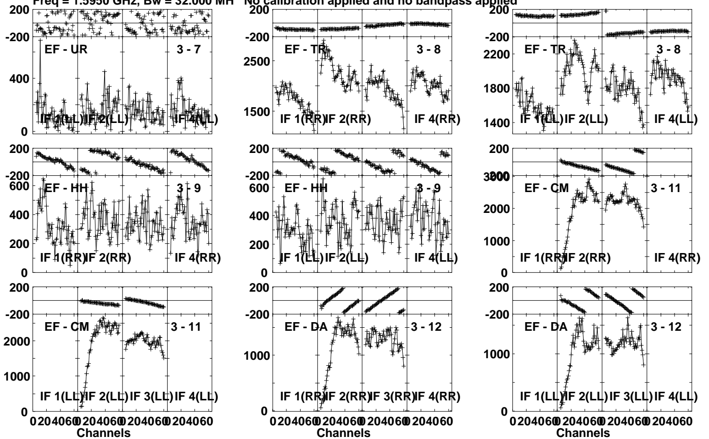
Lower frame: Micro Ampl Jy Top frame: Phas deg Vector averaged cross-power spectrum Several baselines displayed Timerange: 00/12:11:11 to 00/12:12:09
