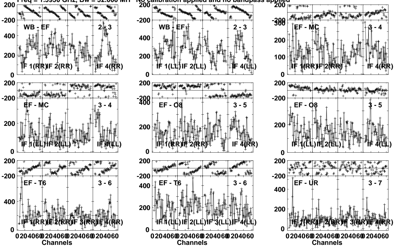
Lower frame: Micro Ampl Jy Top frame: Phas deg Vector averaged cross-power spectrum Several baselines displayed Timerange: 00/09:45:31 to 00/09:47:09
