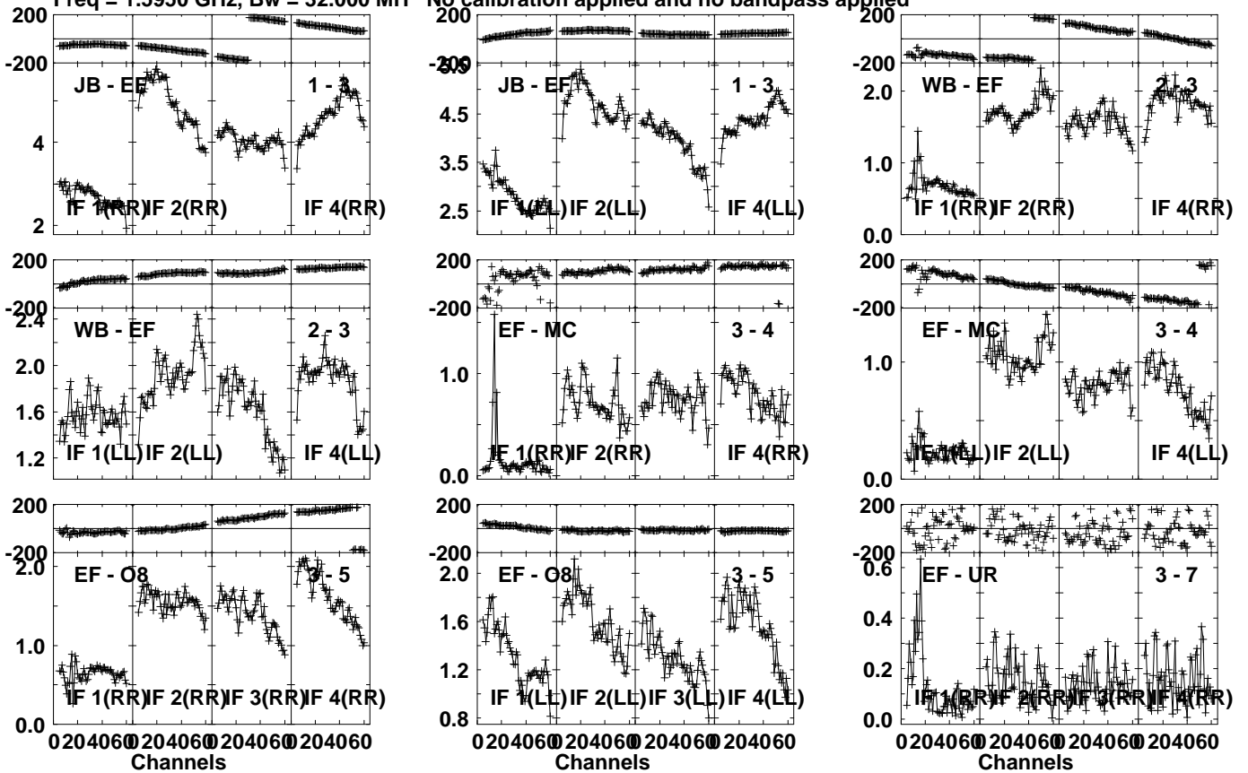
Lower frame: Milli Ampl Jy Top frame: Phas deg Vector averaged cross-power spectrum Several baselines displayed Timerange: 00/12:51:11 to 00/12:52:09
