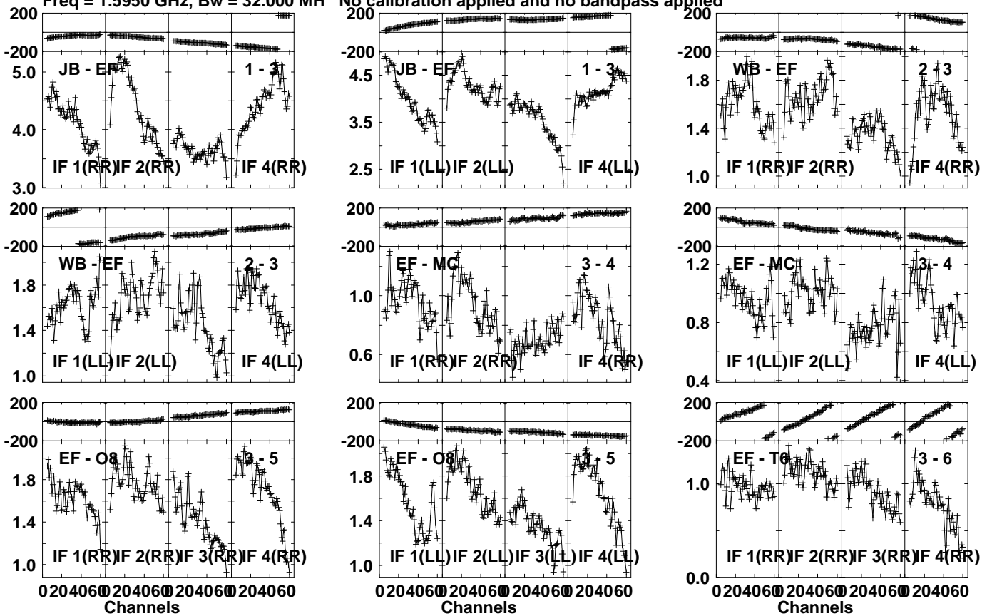
Lower frame: Milli Ampl Jy Top frame: Phas deg Vector averaged cross-power spectrum Several baselines displayed Timerange: 00/09:24:11 to 00/09:25:09
